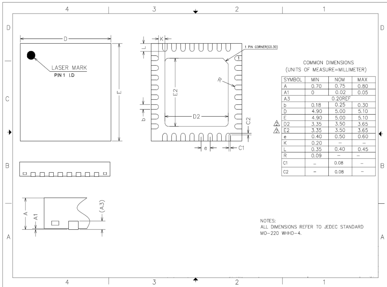
Figure 5-5 QFN32 (5mmx5mm) package outline
