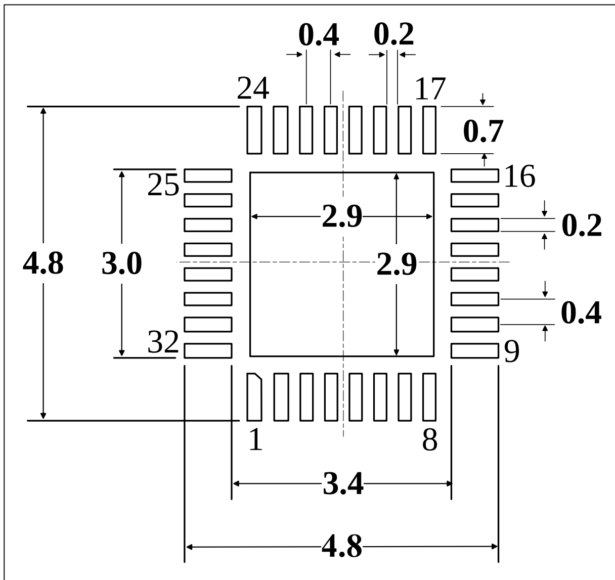
Figure 5-8 QFP32(4mm x 4mm) Recommended footprint (1)
