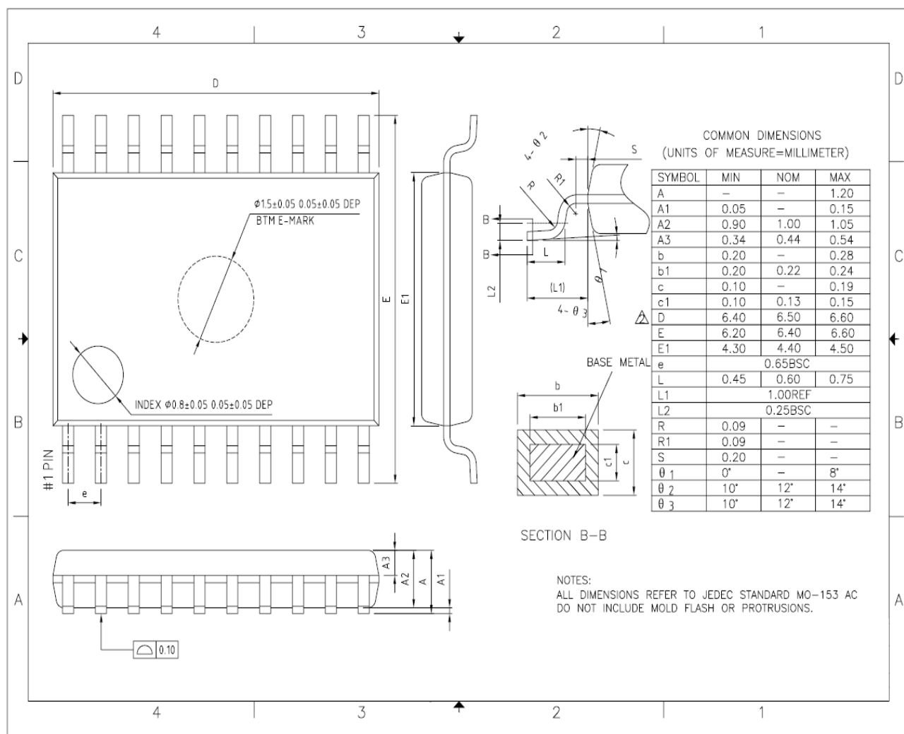
Figure 5-11 TSSOP20 package outline
