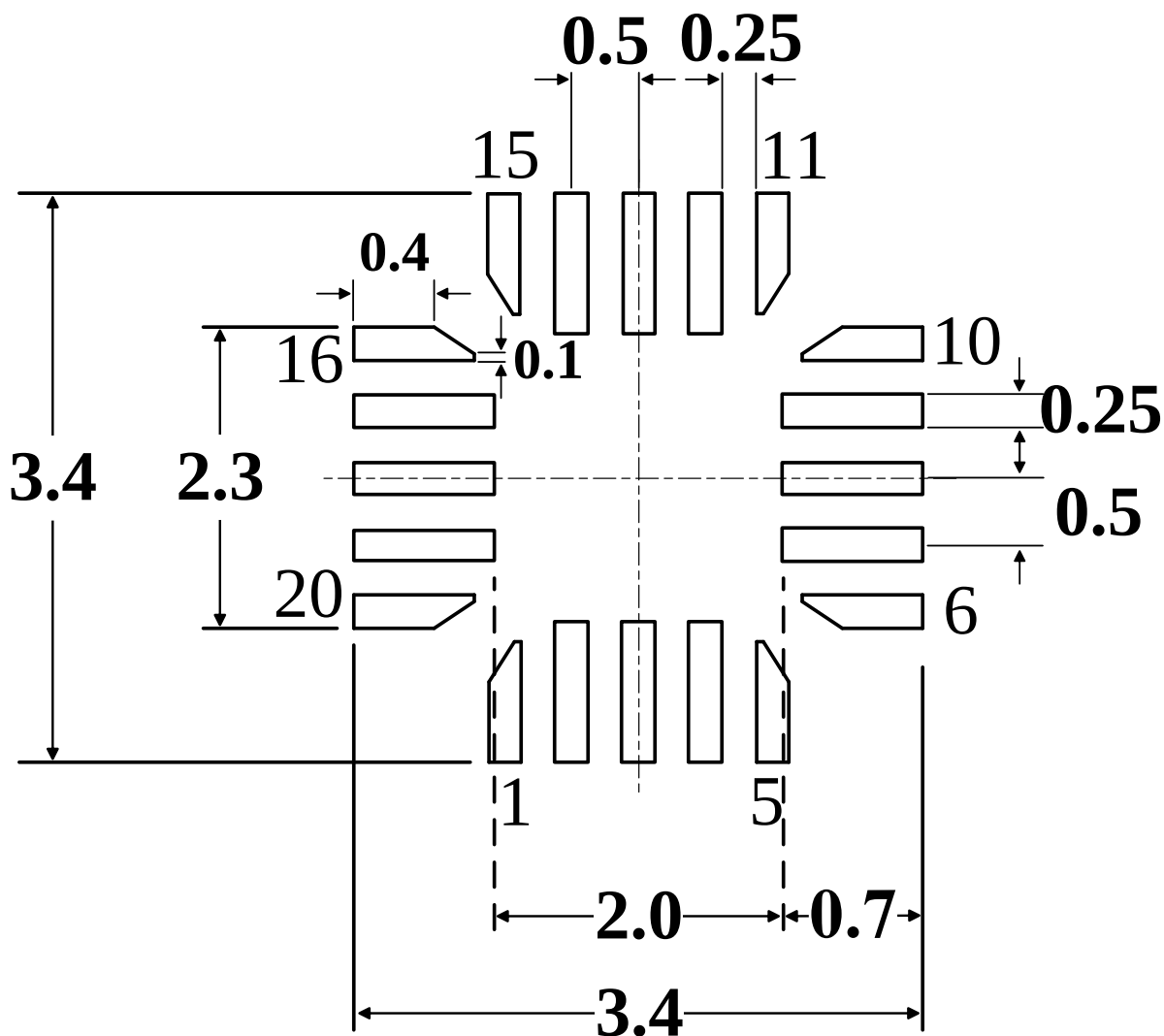
Figure 5-10 UFQFPN20 Recommended footprint (1)
