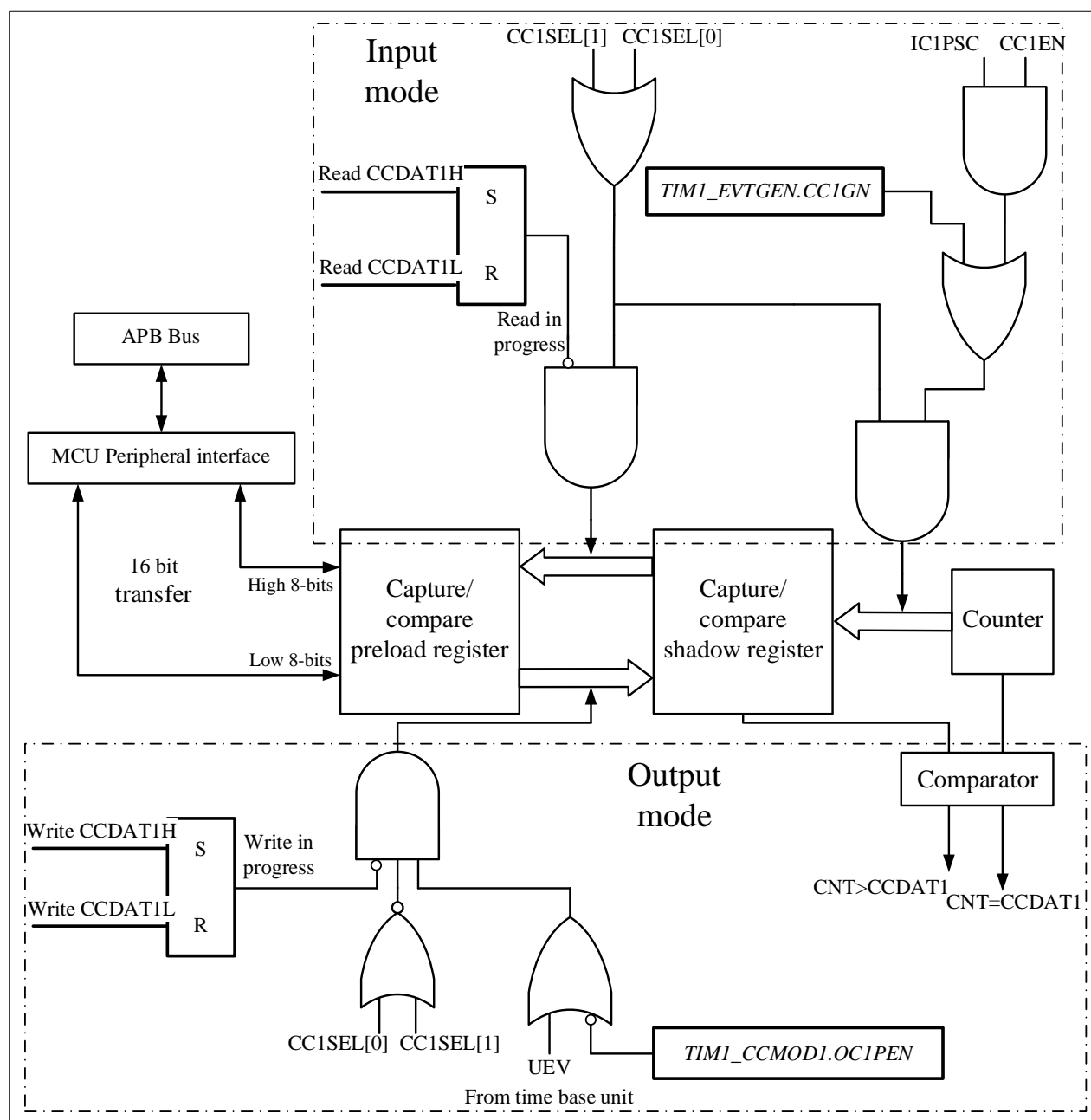
Figure 9-18 Output part of channelx (x= 1,2,3, take channel 1 as example)
