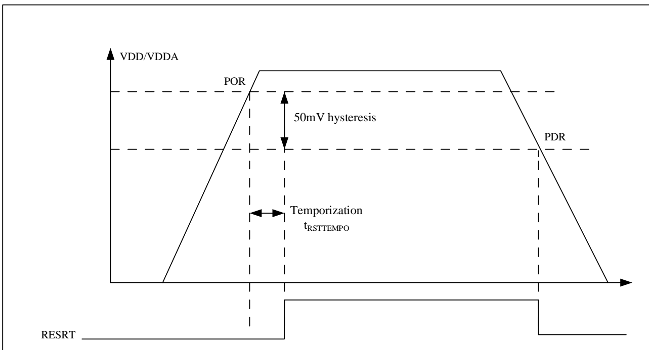
Figure 3-2 Power on reset/power down reset waveform
