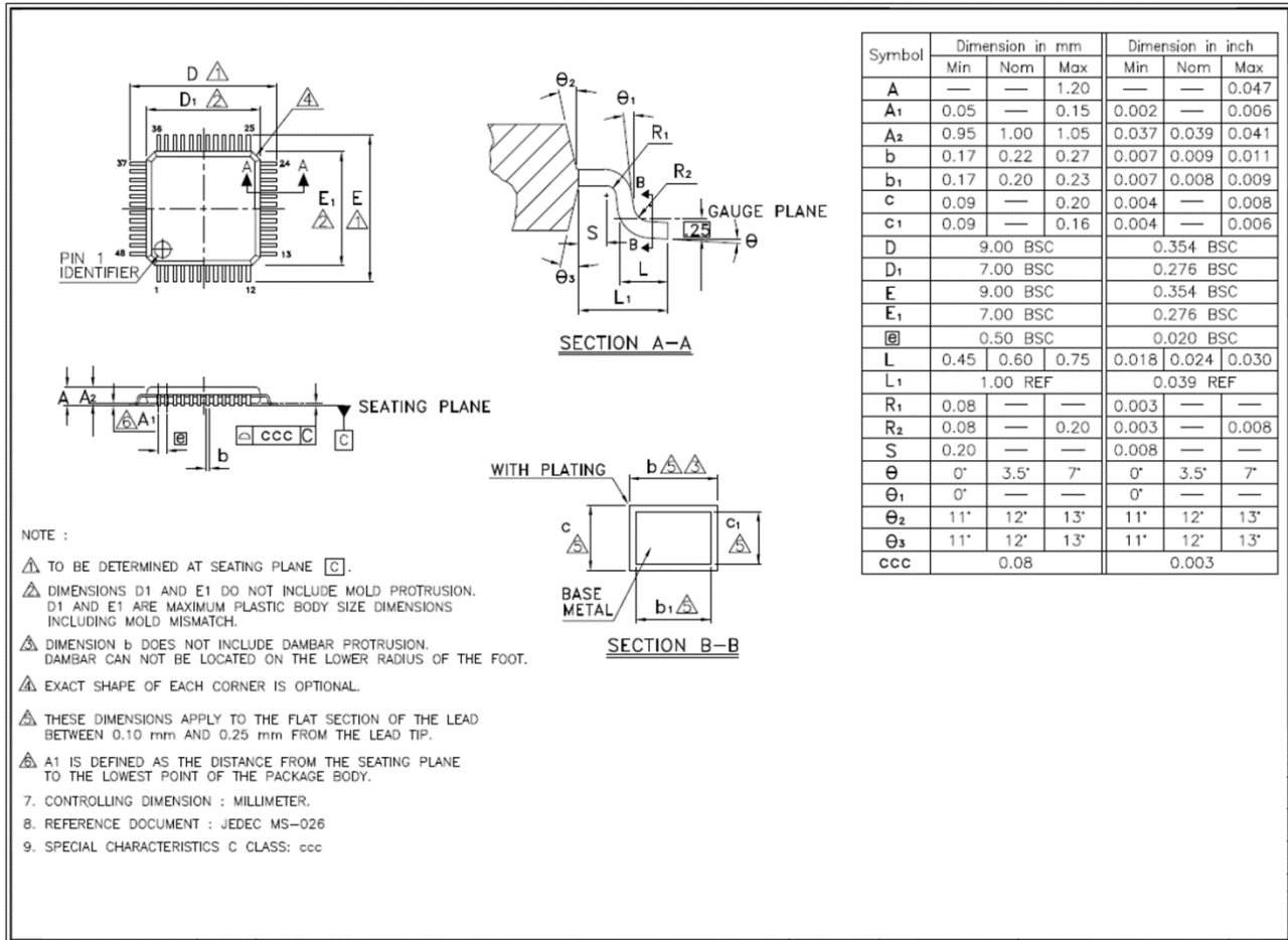
Figure 5-3 TQFP48 package outline
