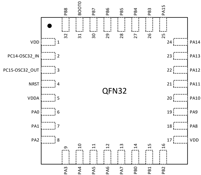
Figure 3-5 N32G030 Series QFN32 (4mmx4mm) pinouts
