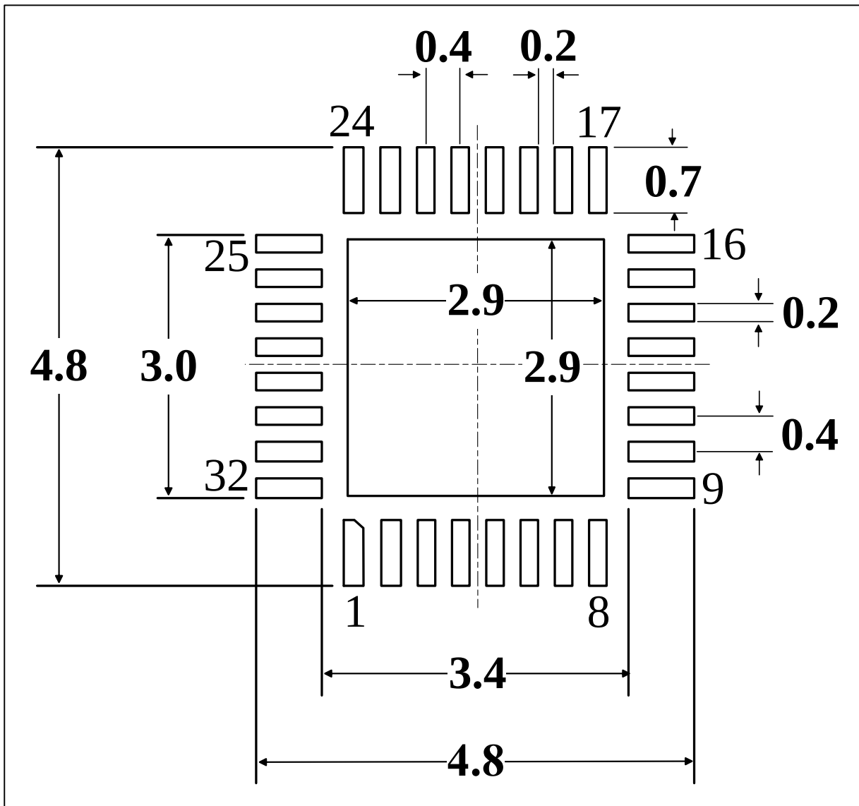
Figure 5-10 QFP32(4mm x 4mm) Recommended footprint (1)
