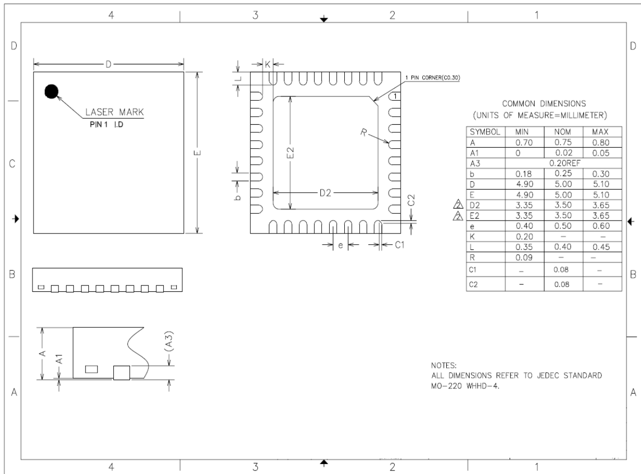
Figure 5-7 QFN32 (5mmx5mm) package outline
