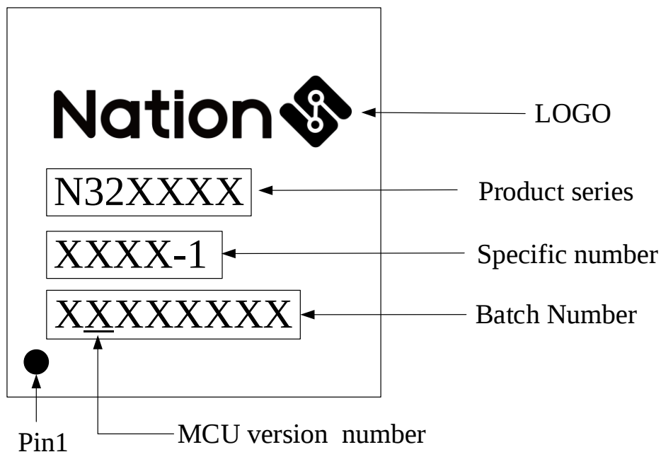
Figure 5-16 QFN32(4mm x 4mm) screen printing instructions
