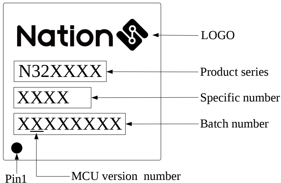
Figure 5-15 LQFP48/TQFP48/LQFP32/QFN32(5mm x 5mm) screen printing instructions
