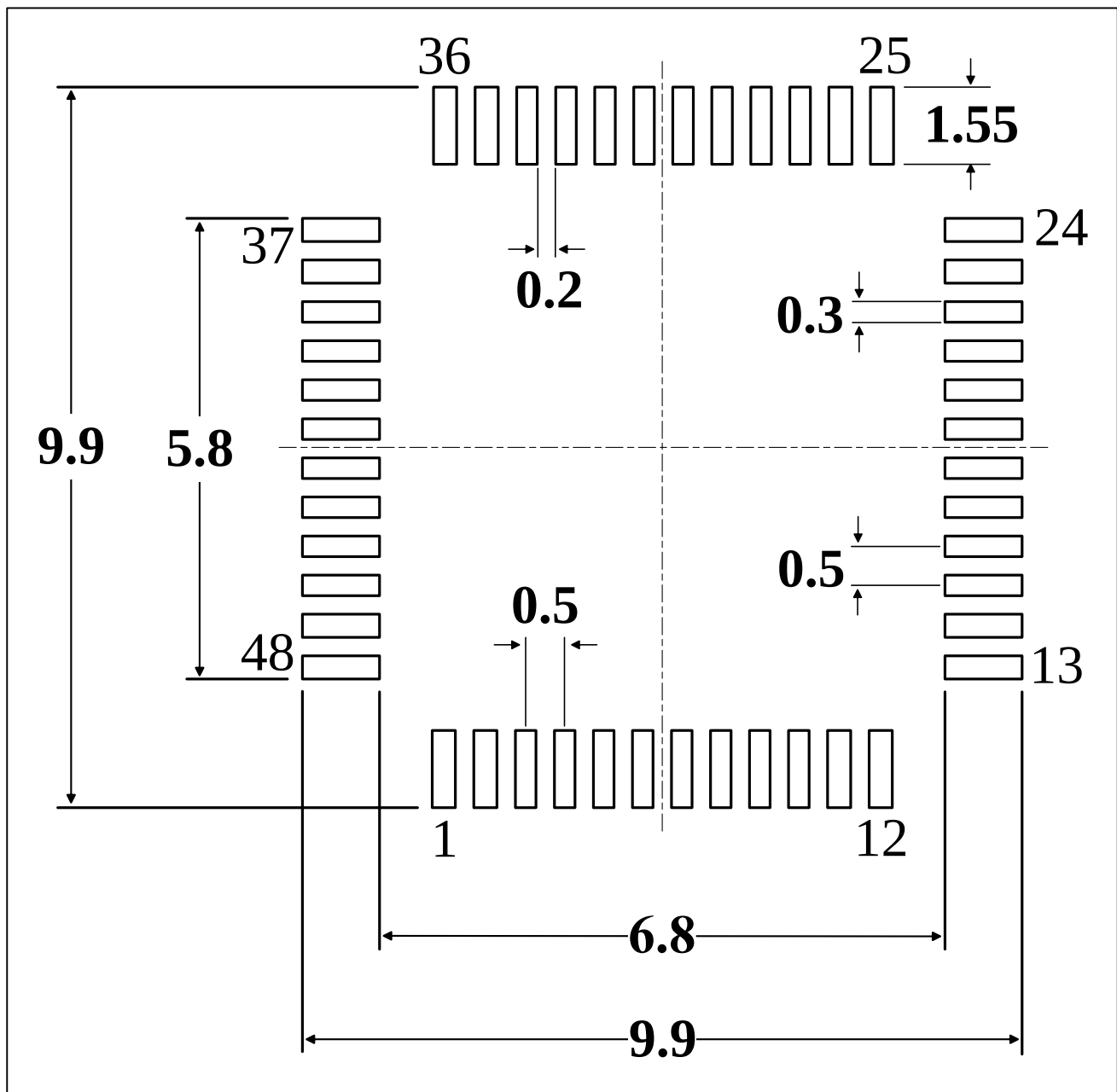
Figure 5-4 TQFP48 Recommended footprint (1)
