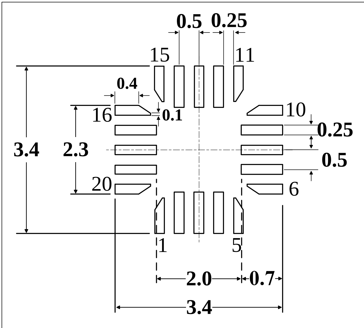
Figure 5-12 UFQFPN20 Recommended footprint (1)
