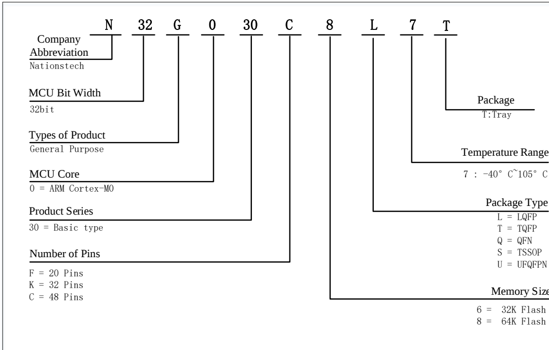
Figure 6-1 N32G030 Series Part Number Information
