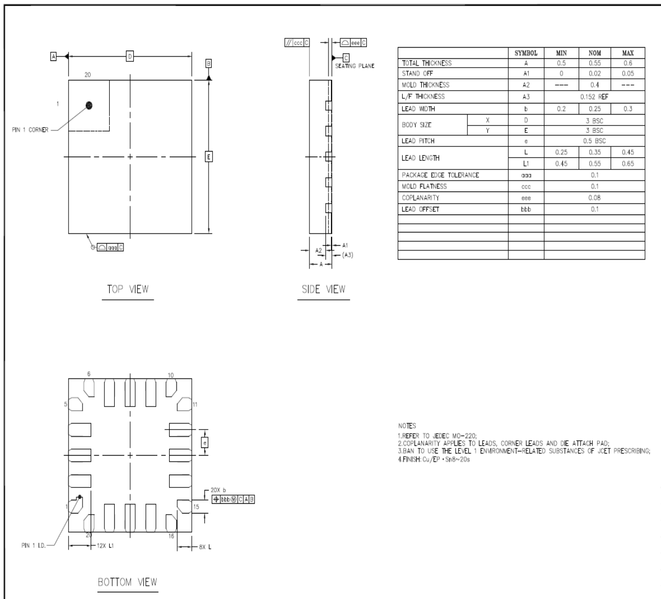
Figure 5-11 UFQFPN20 package outline
