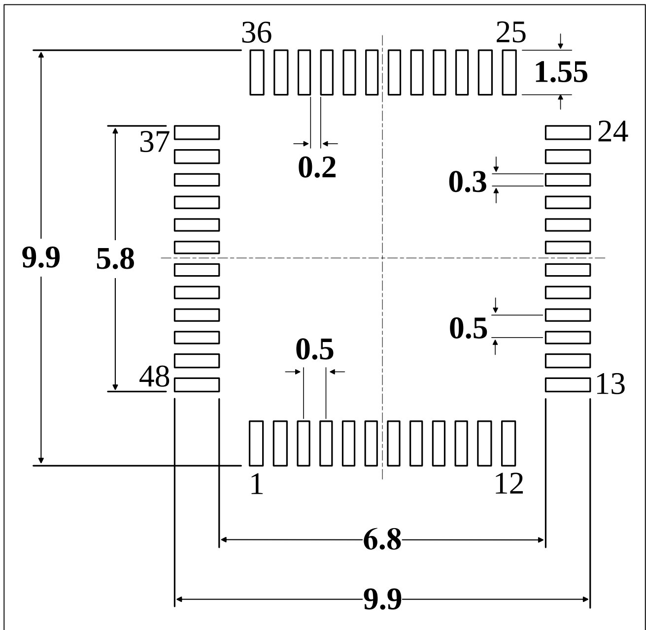
Figure 5-2 LQFP48 Recommended footprint (1)
