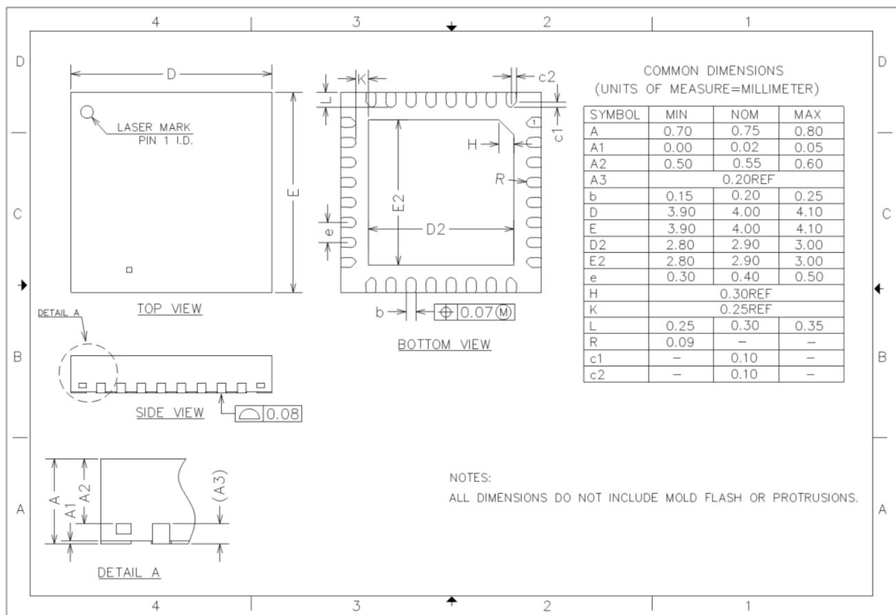
Figure 5-9 QFN32 (4mmx4mm) package outline
