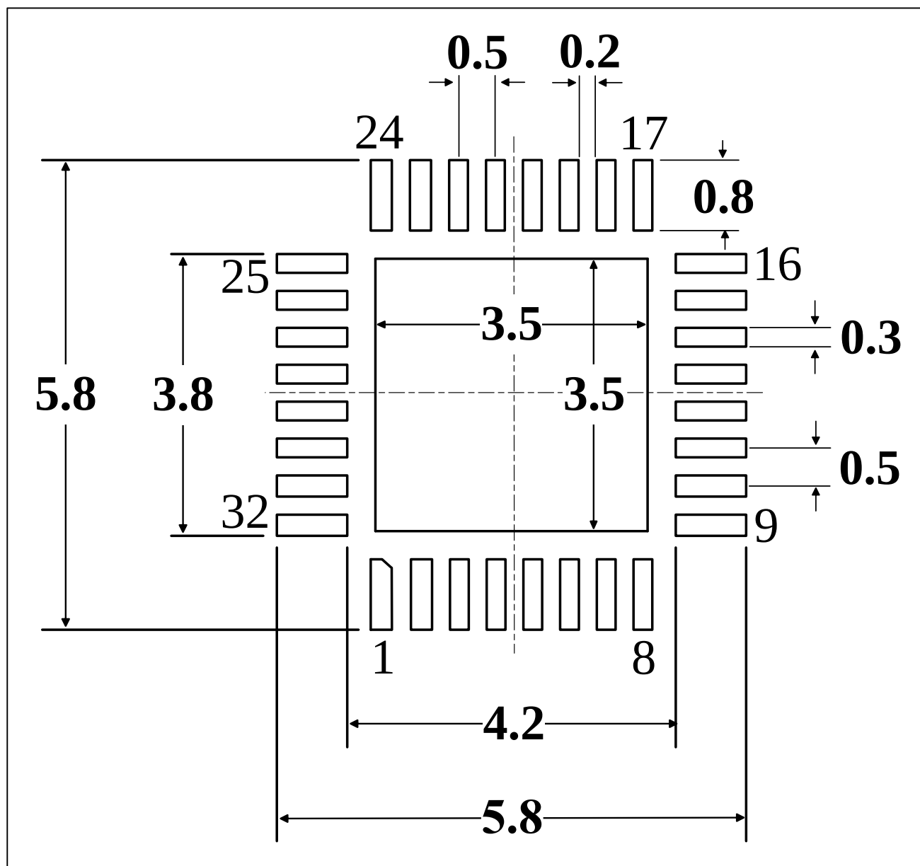
Figure 5-8 QFP32(5mm x 5mm) Recommended footprint (1)
