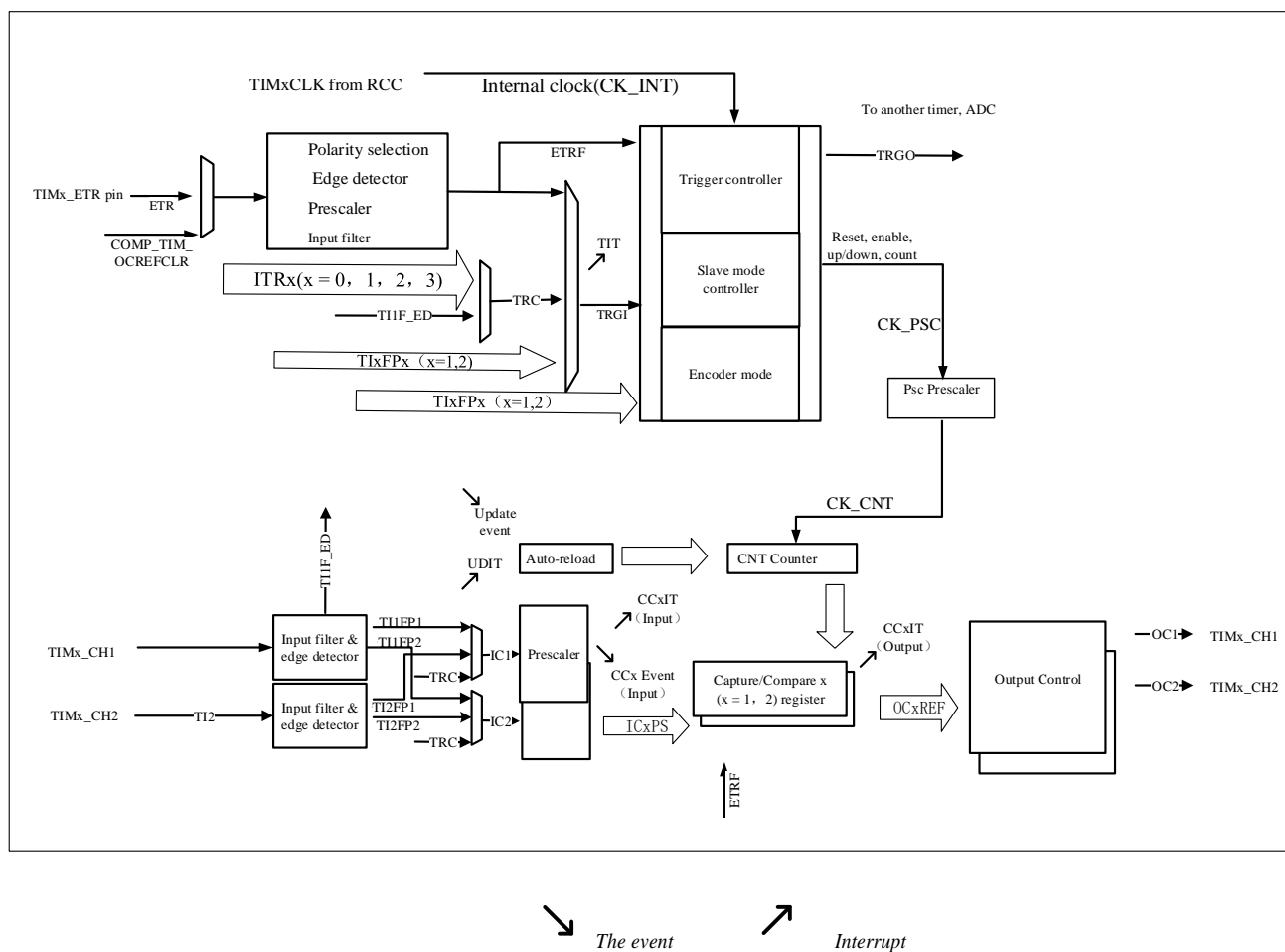
Figure 9-1 Block diagram of TIMx (x=3)
