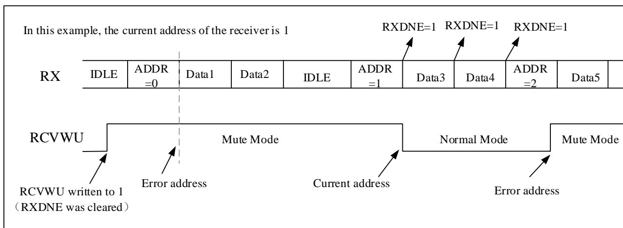
Figure 15-8 Mute mode detected using address mark
