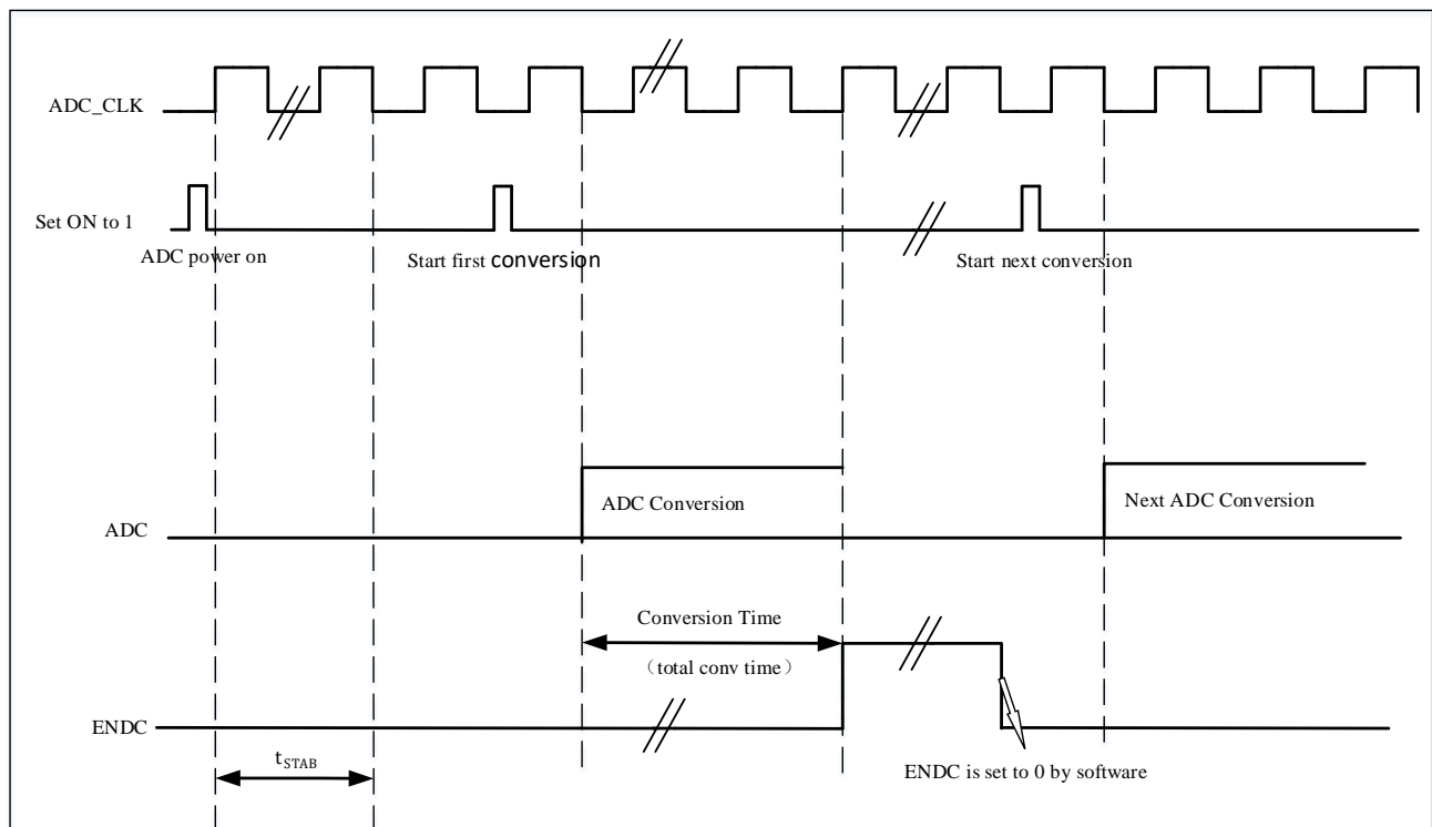
Figure 12-2 Timing diagram
