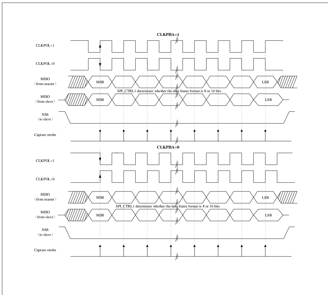
Figure 16-4 Data clock timing diagram
