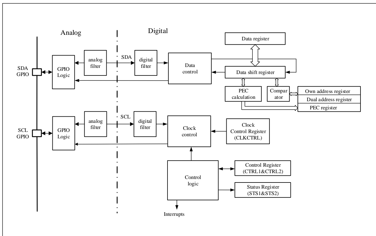
Figure 14-1 I2C functional block diagram
