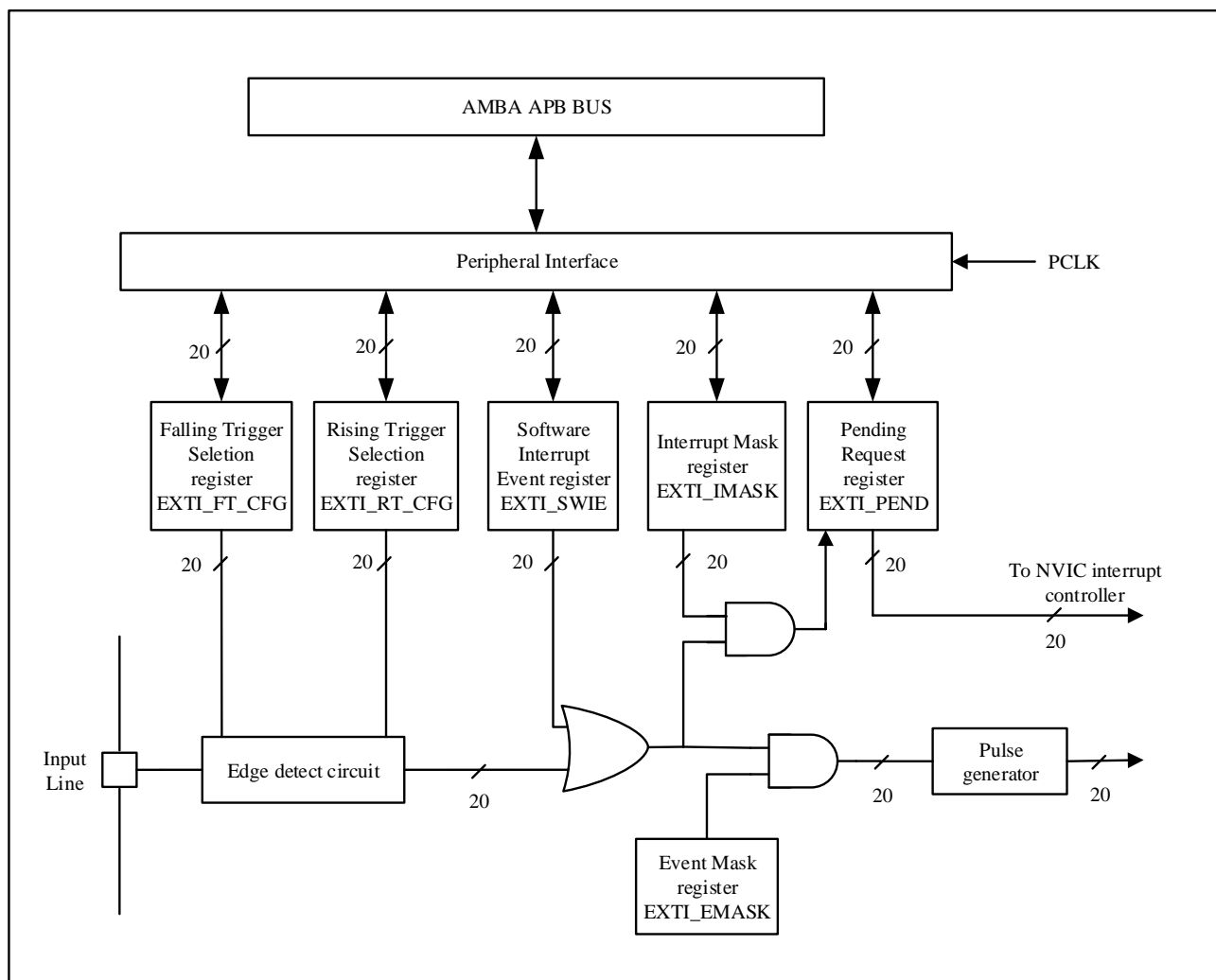
Figure 6-1 Extenal interrupt/event controller block diagram
