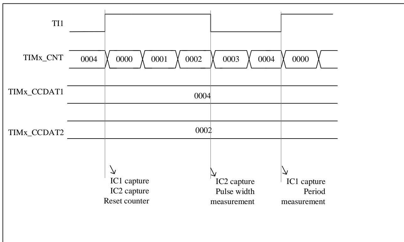
Figure 9-16 PWM input mode timing
