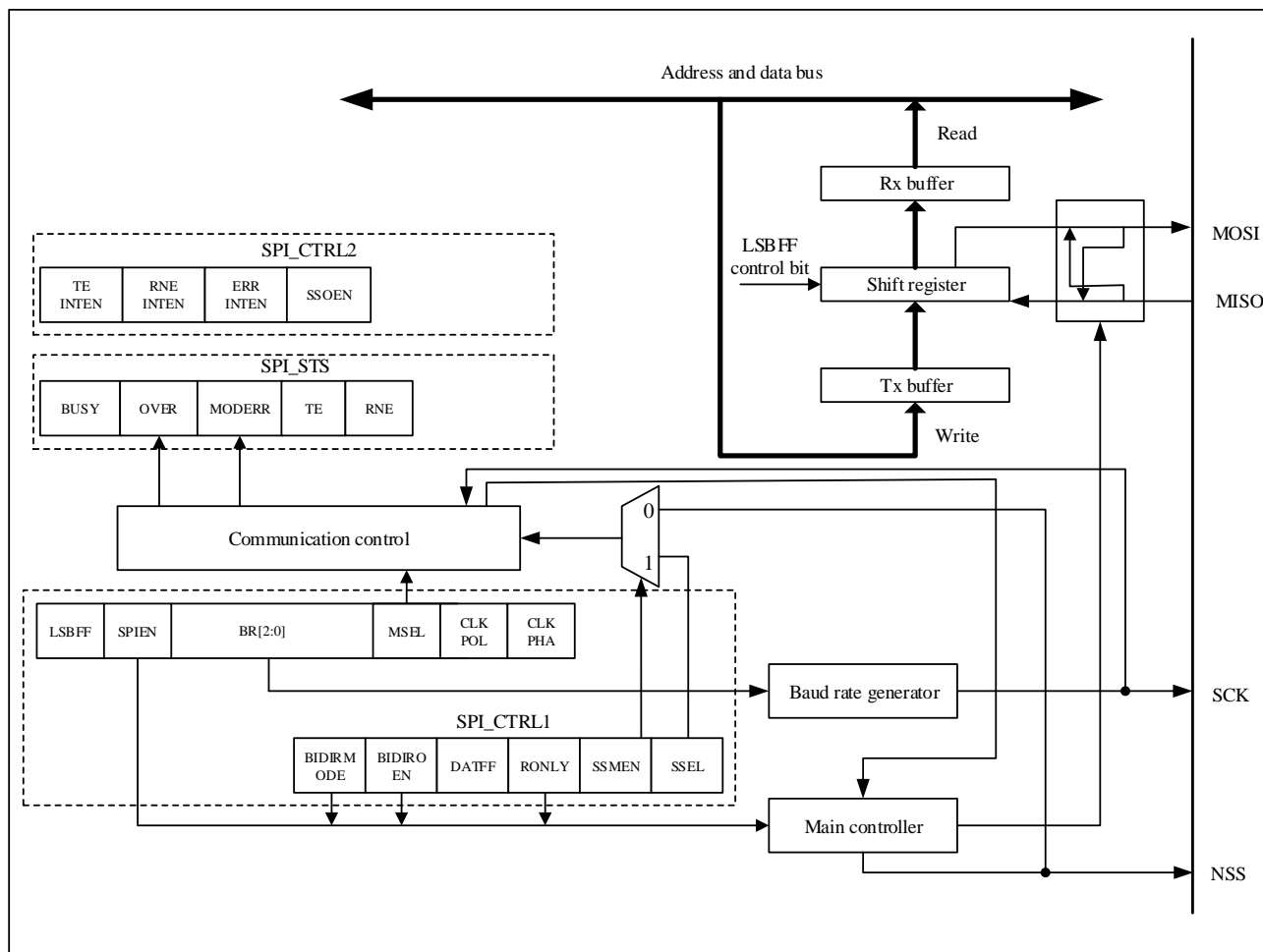
Figure 16-1 SPI block diagram
