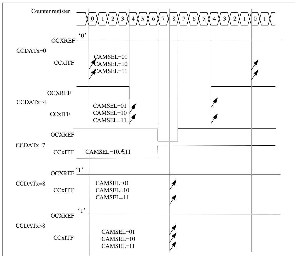
Figure 9-18 Center-aligned PWM waveform (AR=8)
