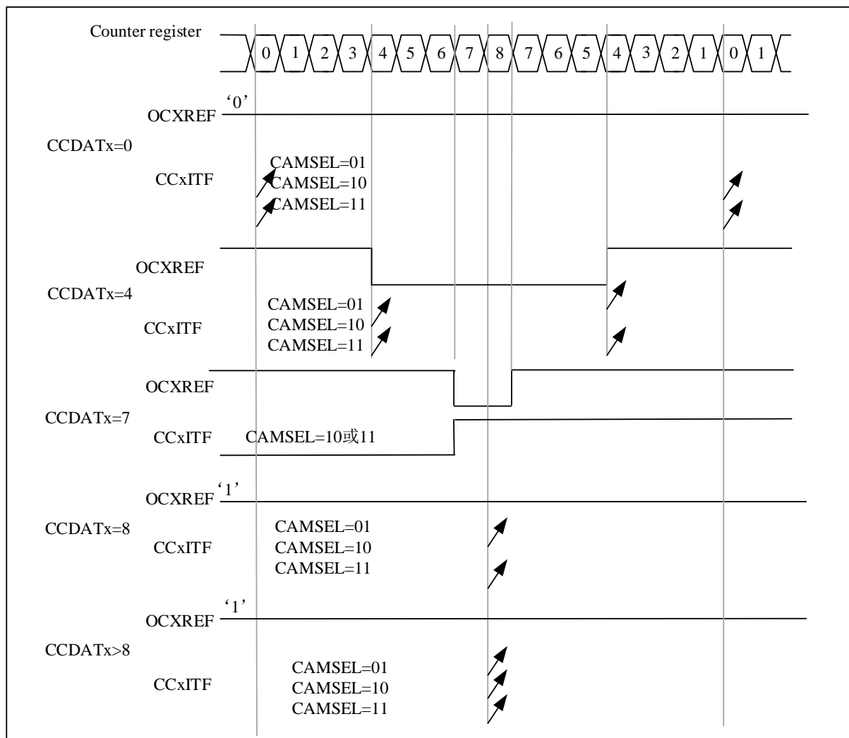
Figure 8-22 Center-aligned PWM waveform (AR=8)
