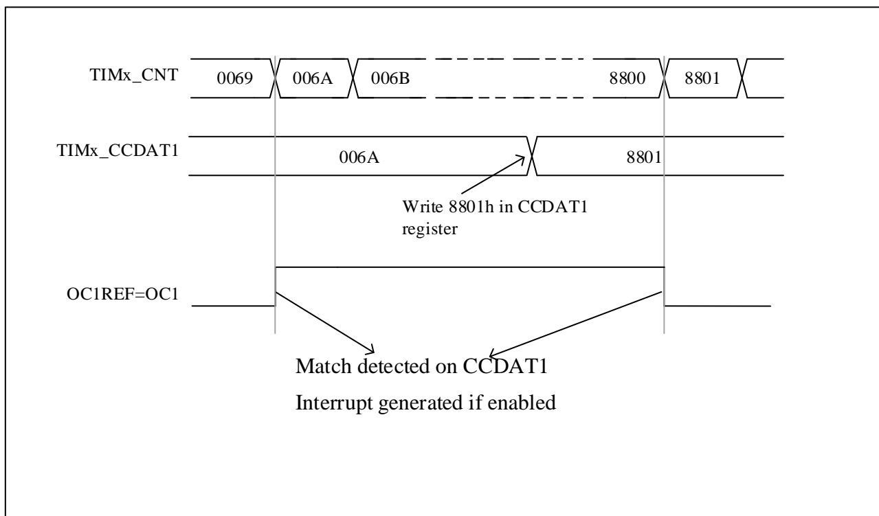
Figure 9-17 Output compare mode, toggle on OC1
