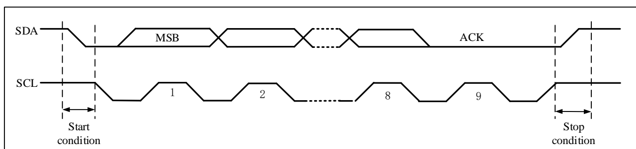
Figure 14-2 I2C bus protocol
