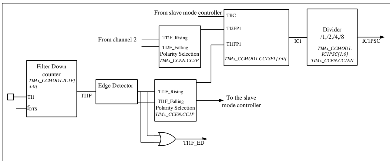
Figure 9-13 Capture/compare channel (example: channel 1 input stage)
