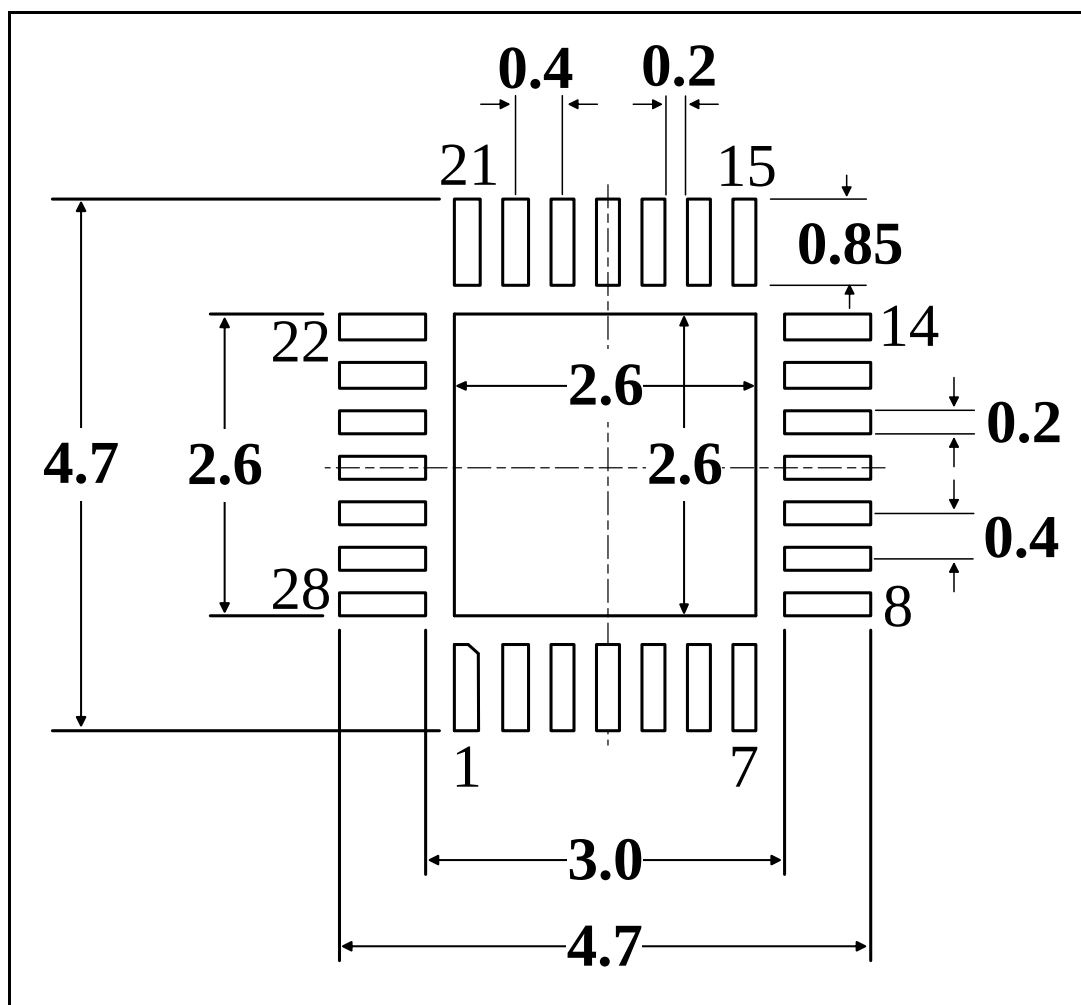
Figure 5-2 QFN28(4mmx4mm) Recommended footprint (1)
