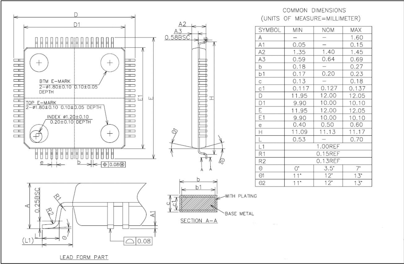
Figure 5-7 LQFP64 (10mm×10mm) package outline
