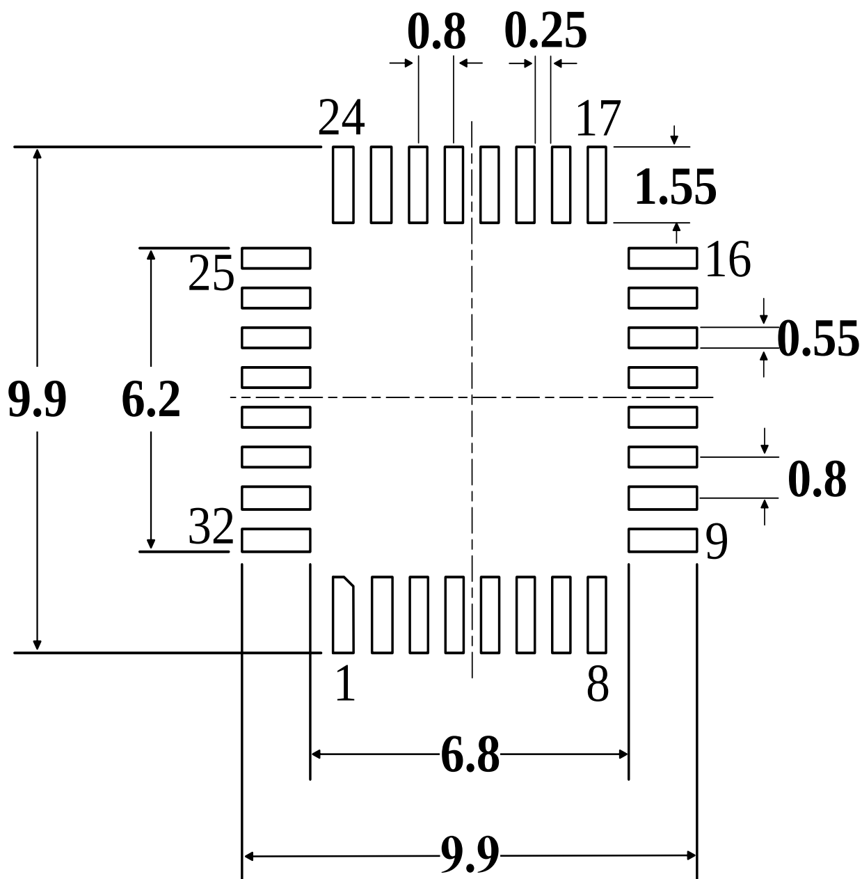
Figure 5-4 LQFP32(7mmx7mm) Recommended footprint (1)
