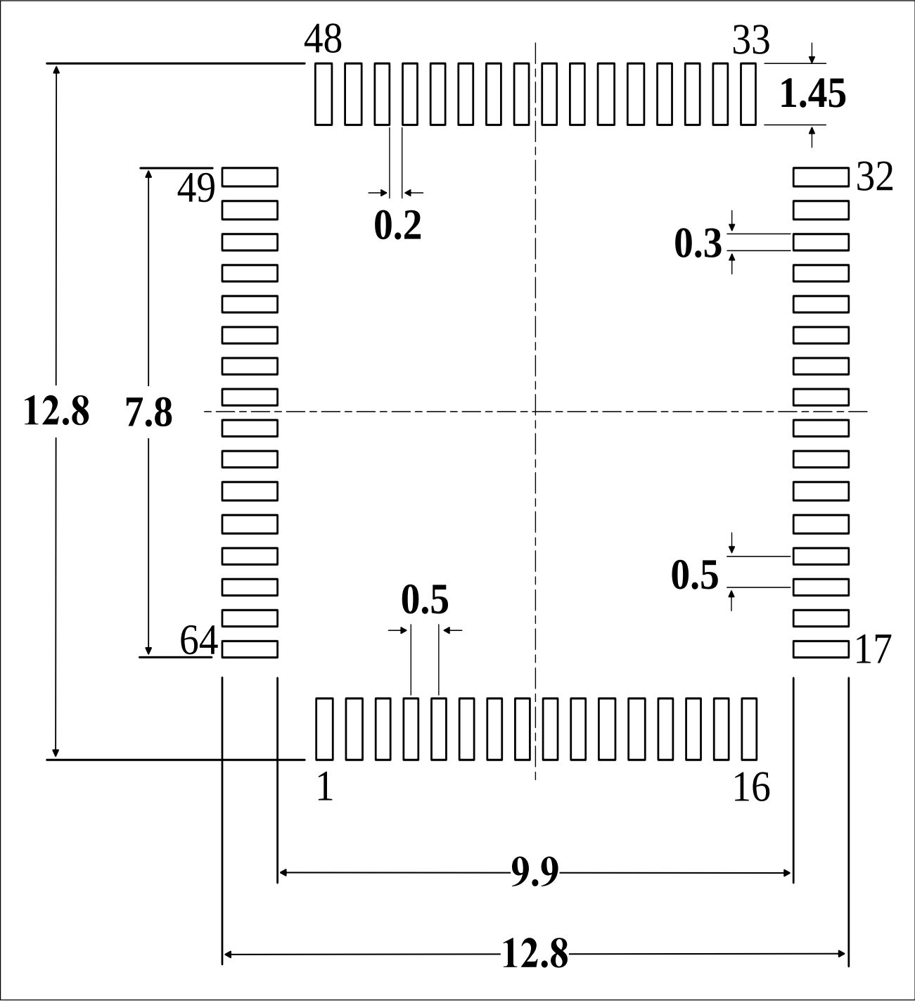
Figure 5-8 LQFP64(10mmx10mm) Recommended footprint (1)
