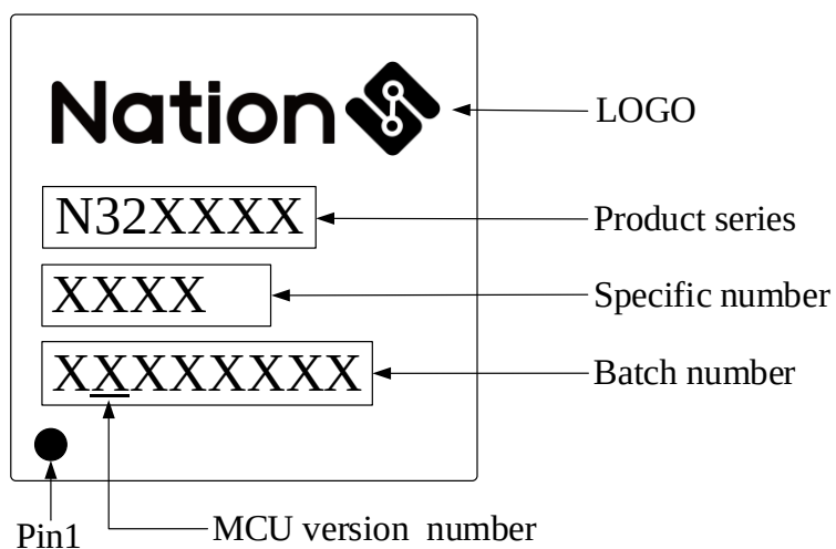
Figure 5-11 Marking information
