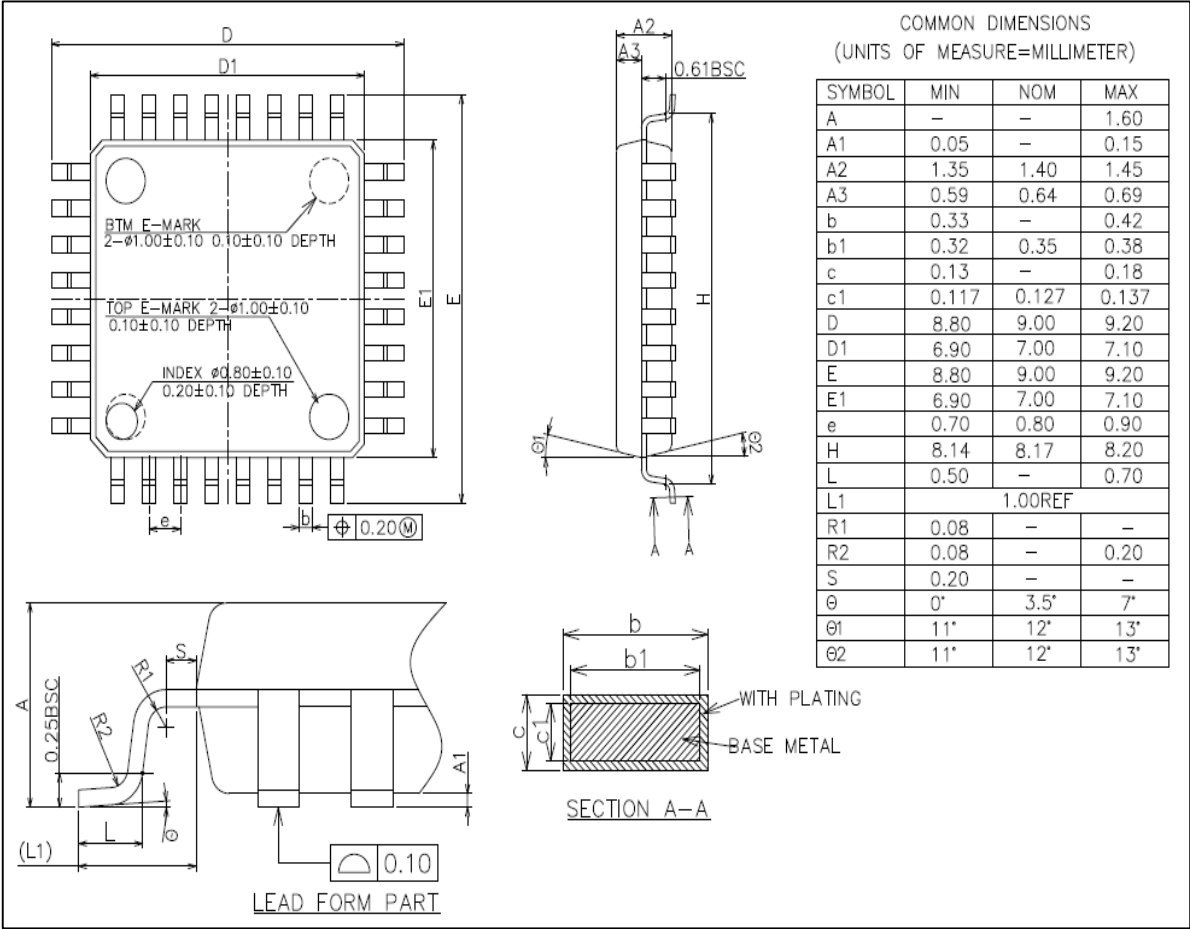
Figure 5-3 LQFP32(7mmx7mm) package outline
