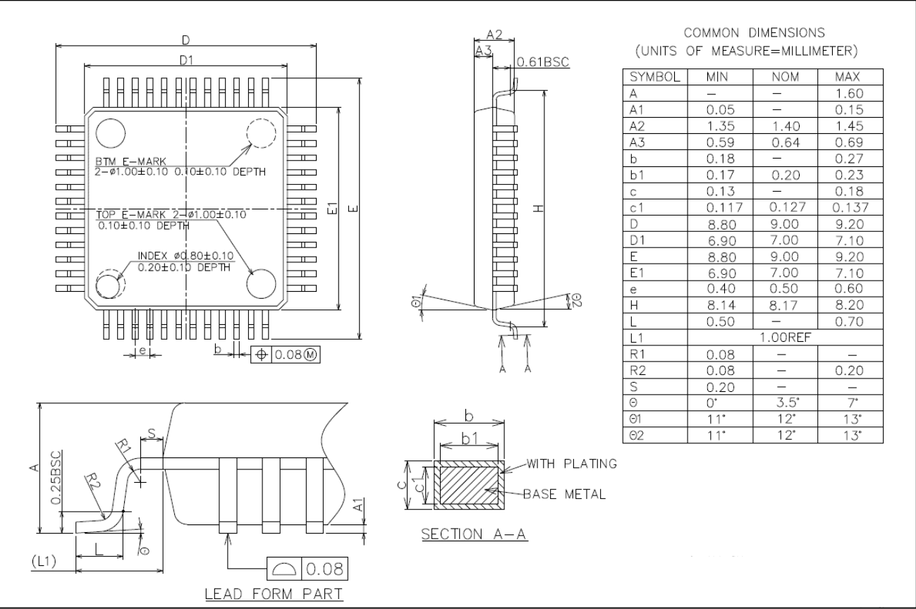
Figure 5-5 LQFP48(7mmx7mm) package outline
