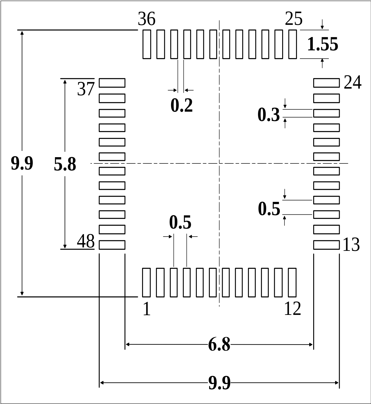
Figure 5-6 LQFP48(7mmx7mm) Recommended footprint (1)
