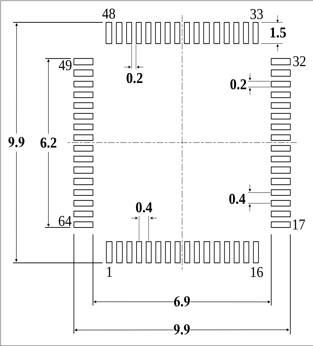
Figure 5-10 LQFP64(7mmx7mm) Recommended footprint (1)
