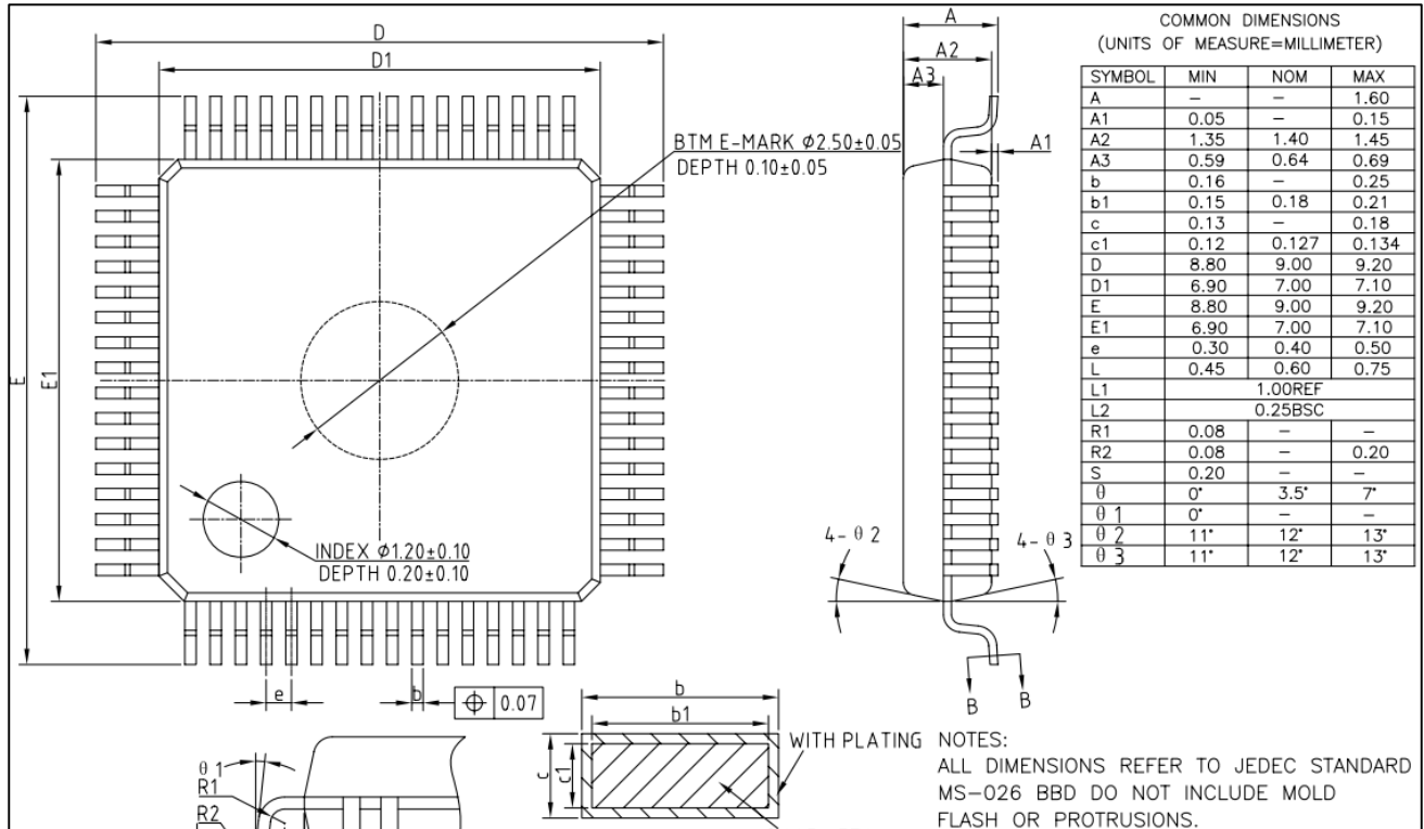
Figure 5-9 LQFP64(7mm×7mm) package outline
