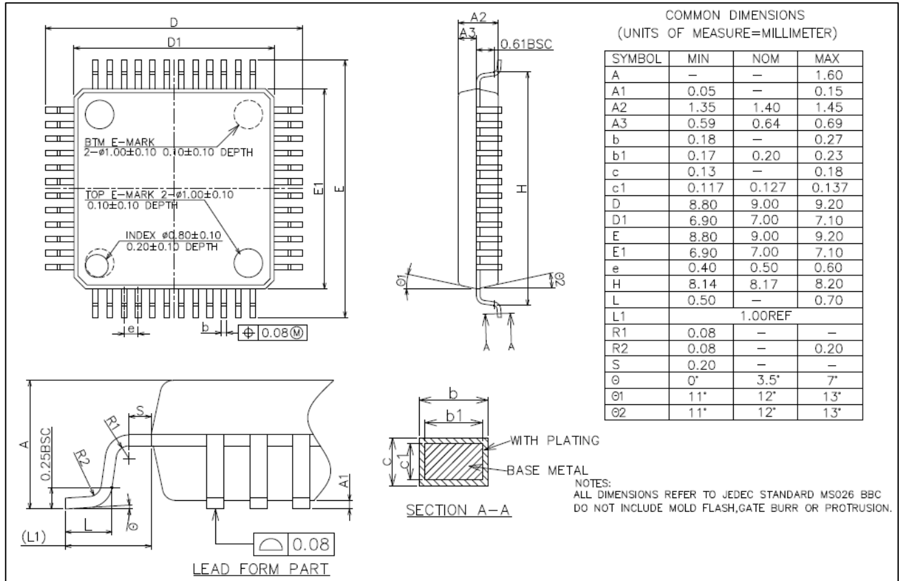
Figure 5-3 LQFP48(7mm×7mm) package outline
