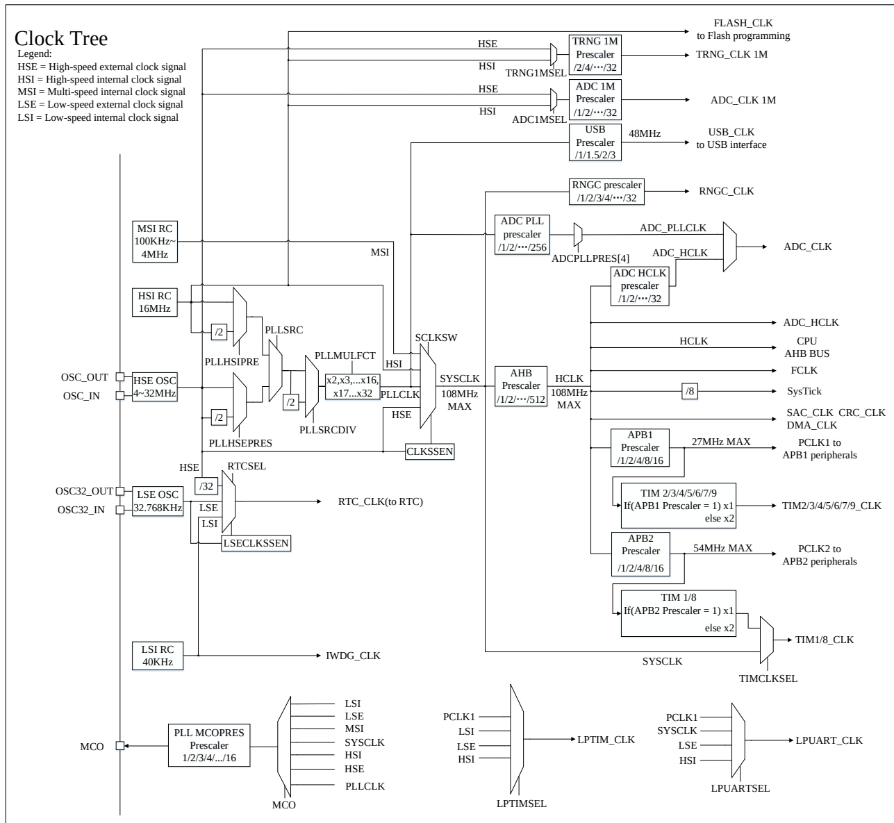
Figure 2-2 Clock tree
