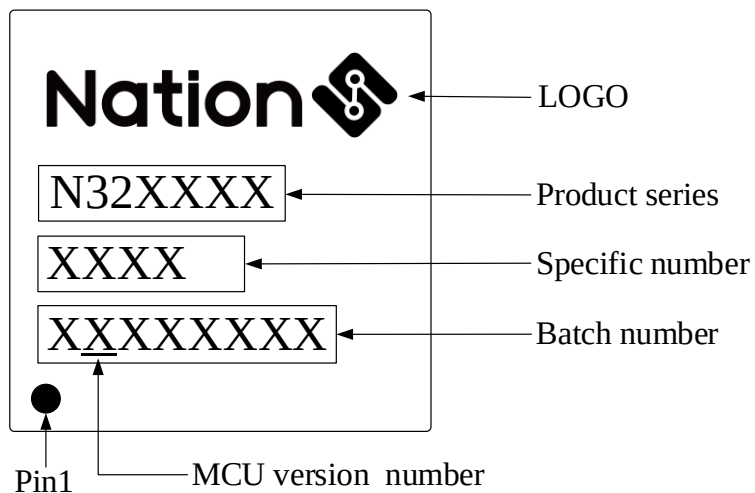
Figure 5-7 Marking information
