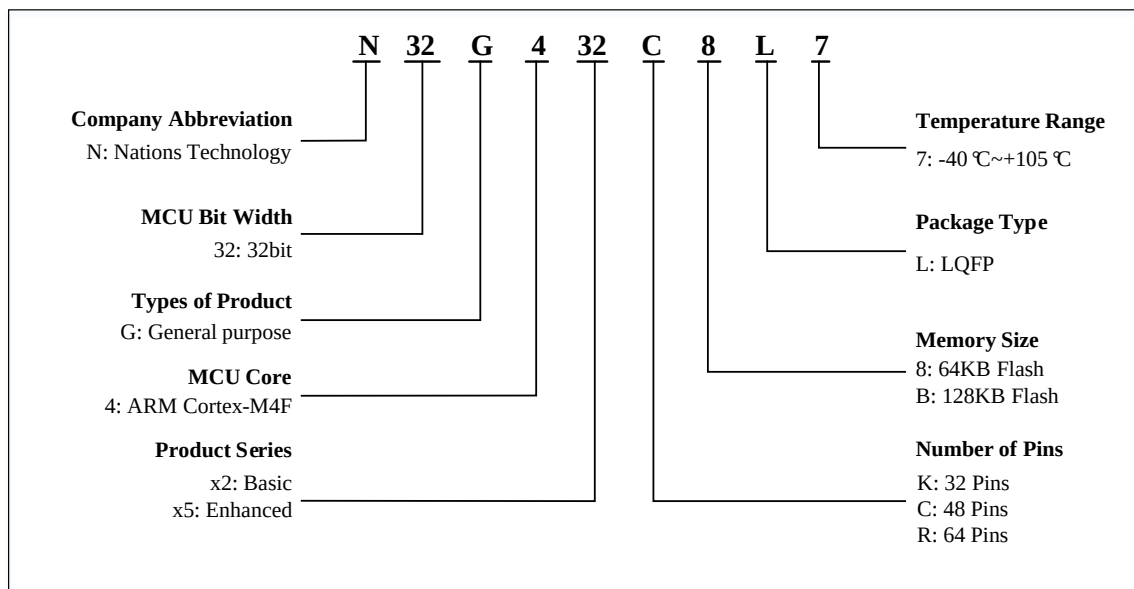
Figure 6-1 N32G432 series part number information
