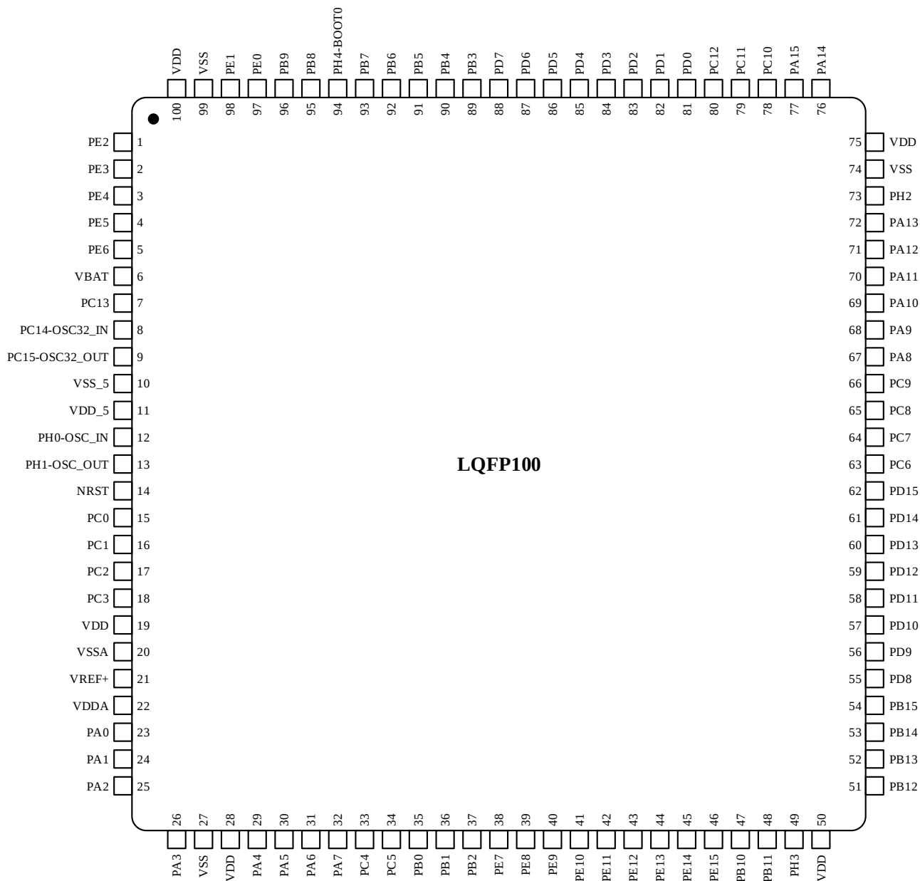
Figure 3-2 N32H482 Series LQFP100 Pinout
