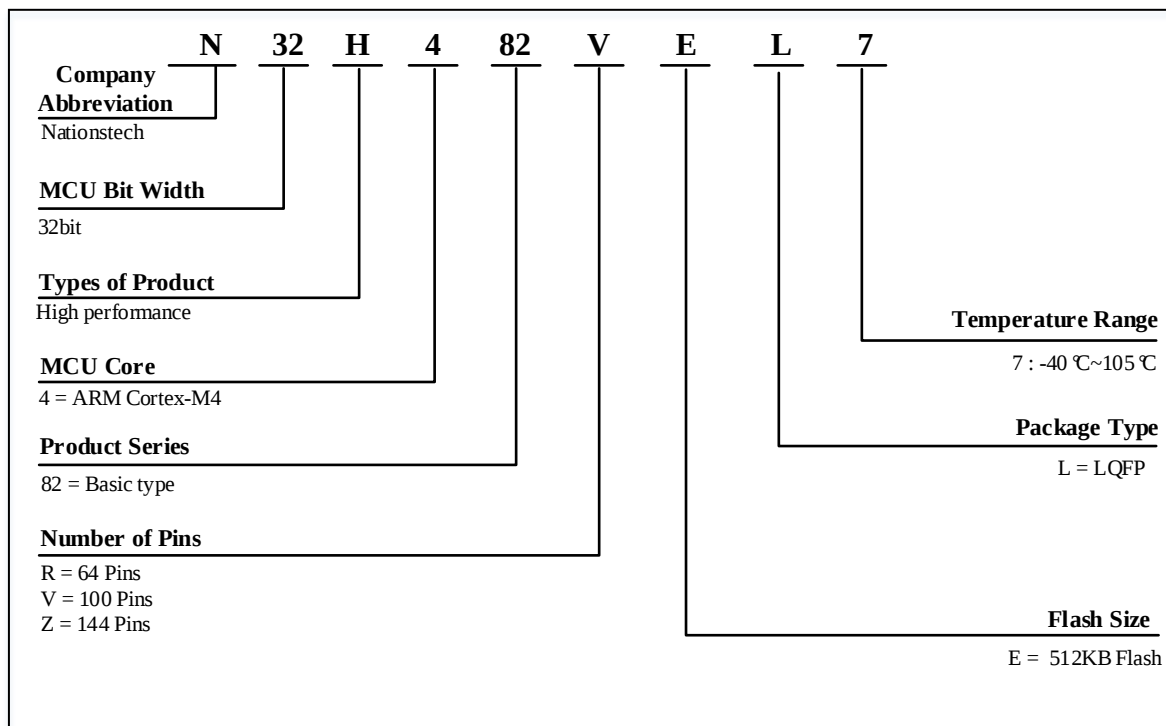
Figure 7-1 N32H482 Series Part Number Information
