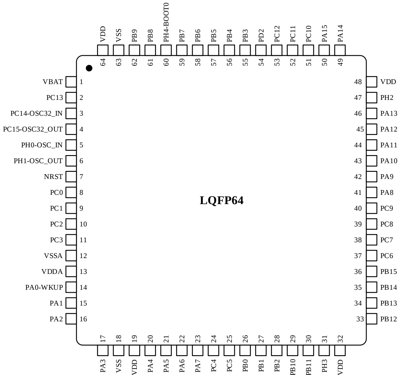
Figure 3-1. N32H482 Series LQFP64 Pinout
