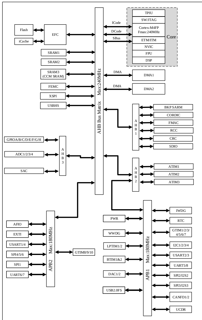
Figure 1-1 N32H482 Series Block Diagram
