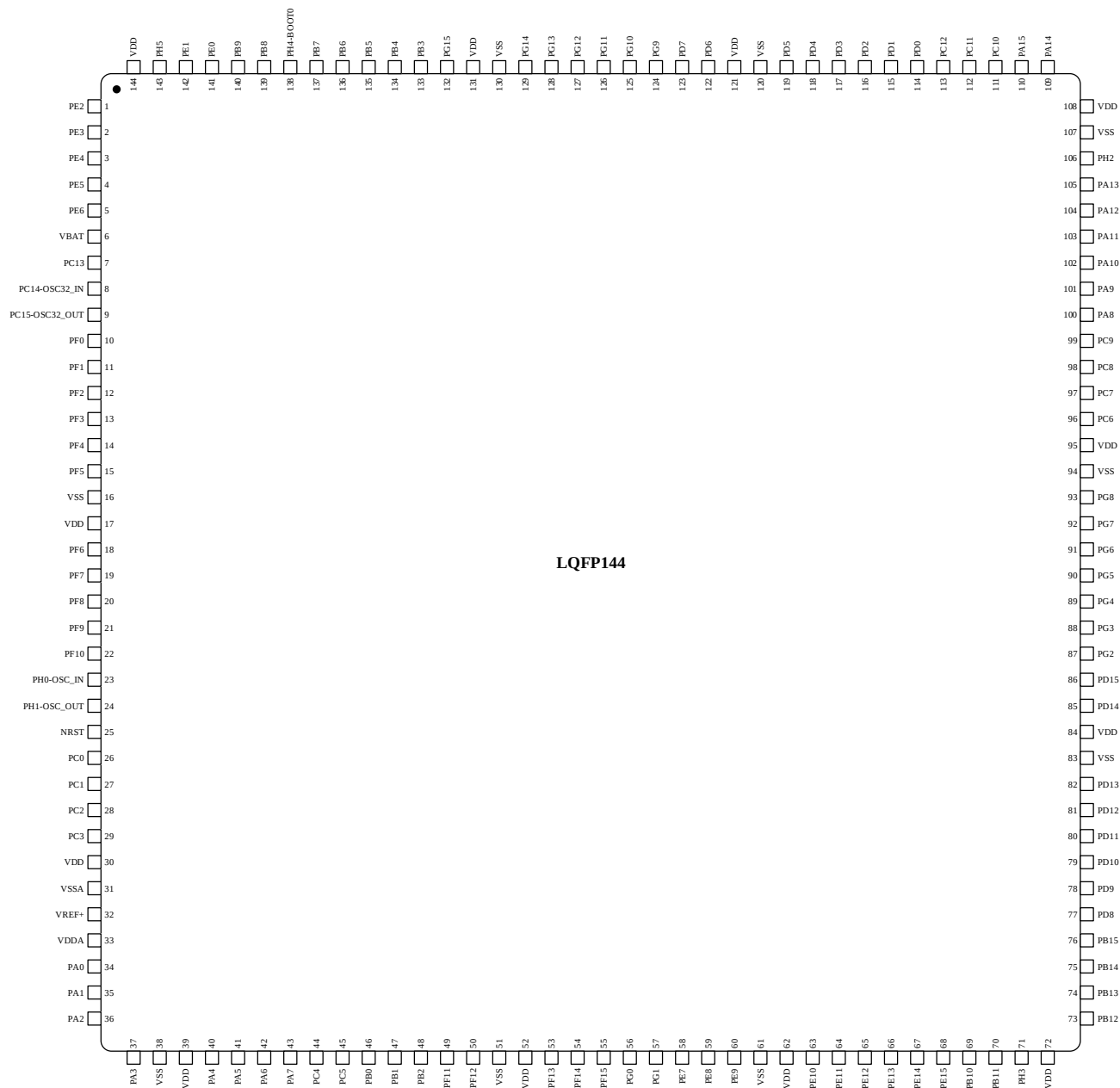
Figure 3-3 N32H482 Series LQFP144 Pinout
