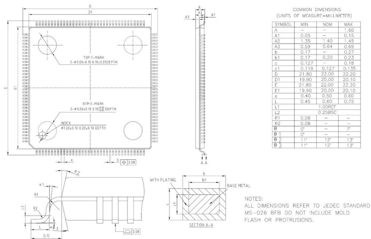
Figure 5-5 LQFP144 Package Dimensions
