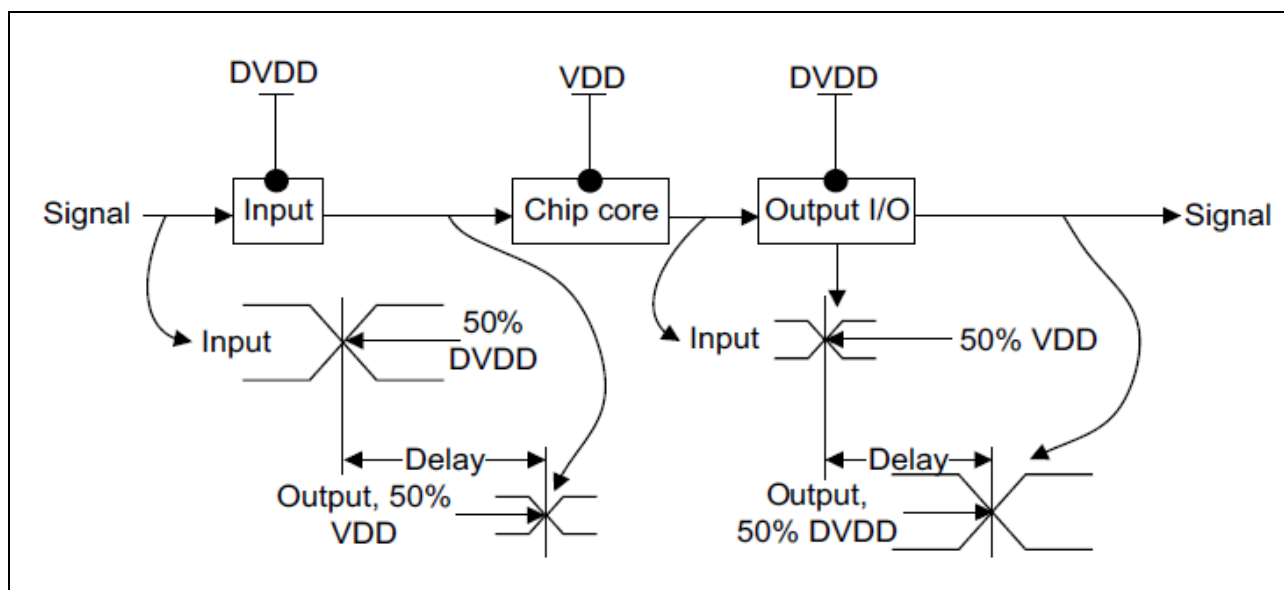
Figure 4-10 Transmission Delay
