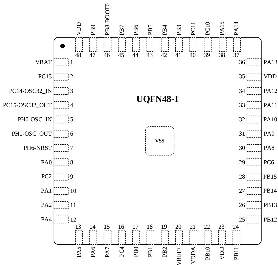
Figure 3-4 UQFN48-1 Pinout
