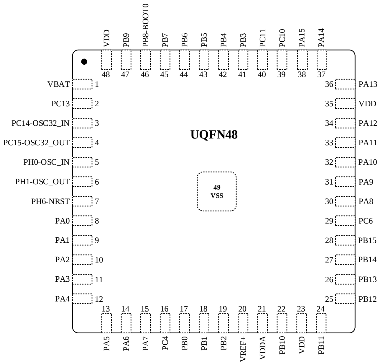
Figure 3-3 UQFN48 Pinout
