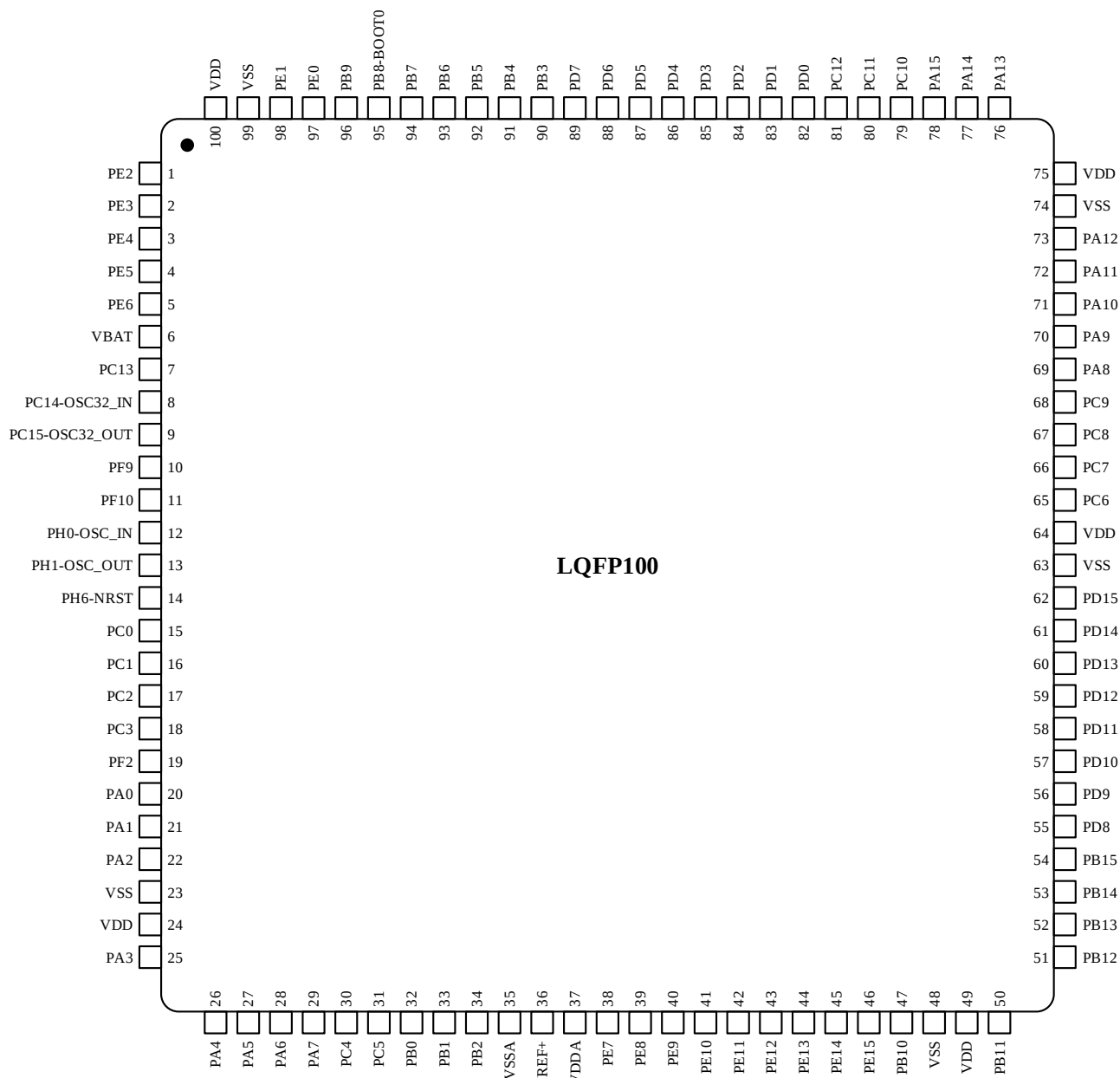
Figure 3-8 LQFP100 Pinout
