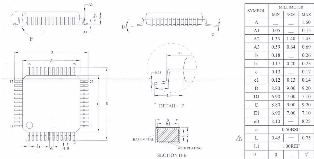
Figure 5-7 LQFP48 Package Dimensions
