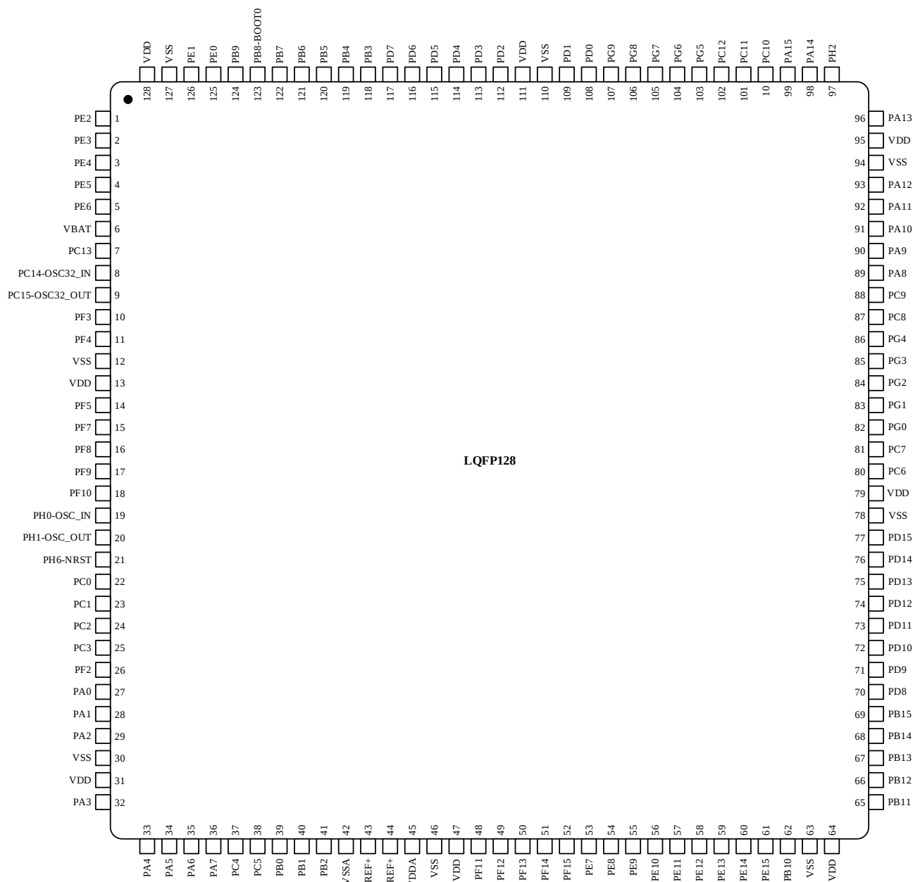
Figure 3-9 LQFP128 Pinout
