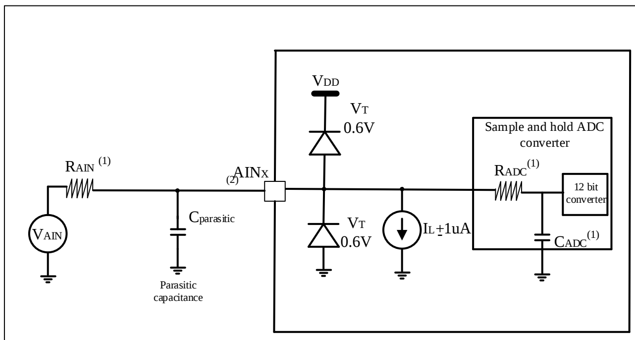
Figure 4-35 Typical Connection Diagram Using ADC
