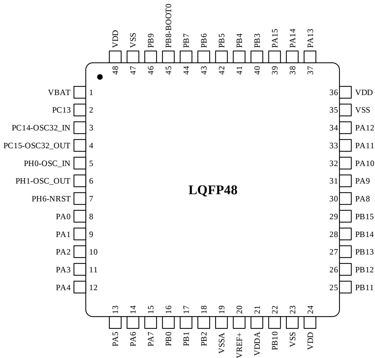
Figure 3-5 LQFP48 Pinout
