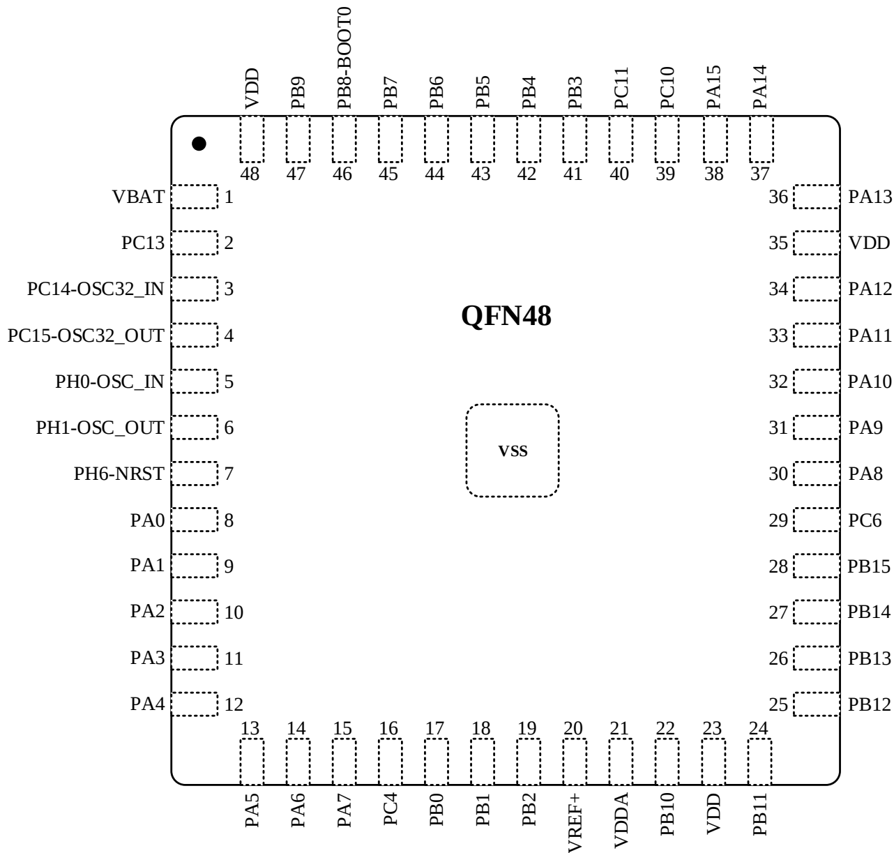
Figure 3-2 QFN48 Pinout
