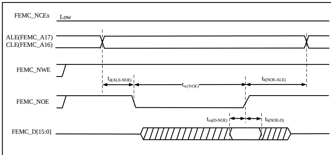
Figure 4-32 NAND Controller Waveforms For Common Memory Write Access
