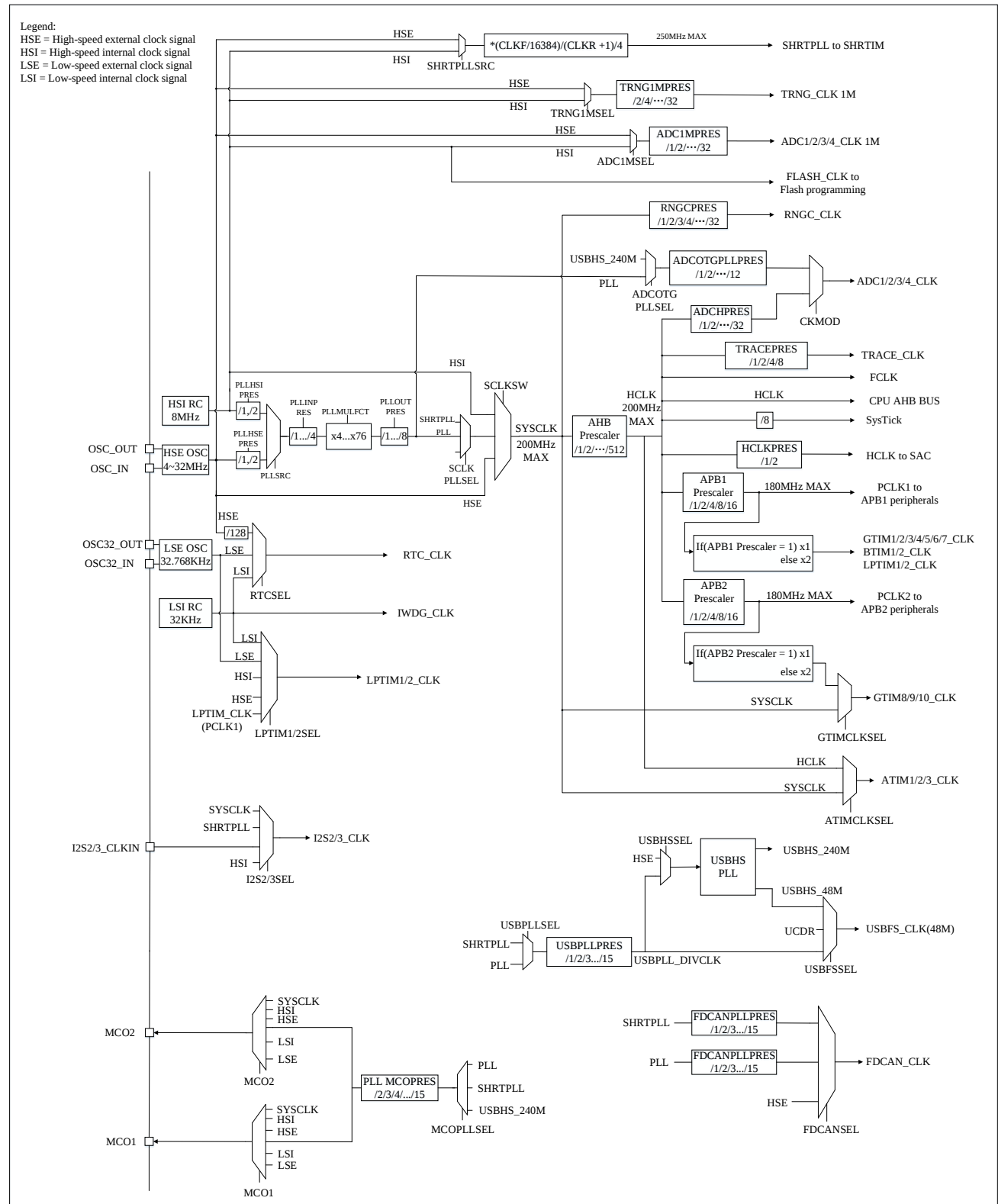
Figure 2-2 Clock Tree
