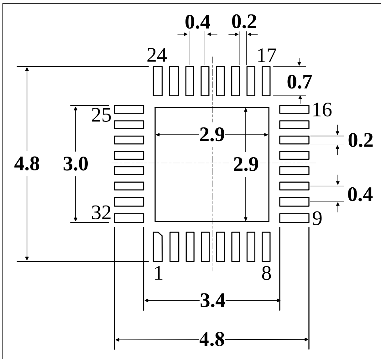
图 5-10 QFP32(4mm x 4mm)封装焊盘建议 (1)
