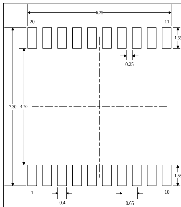
Figure 5-4 TSSOP20 Recommended Footprint (1)
