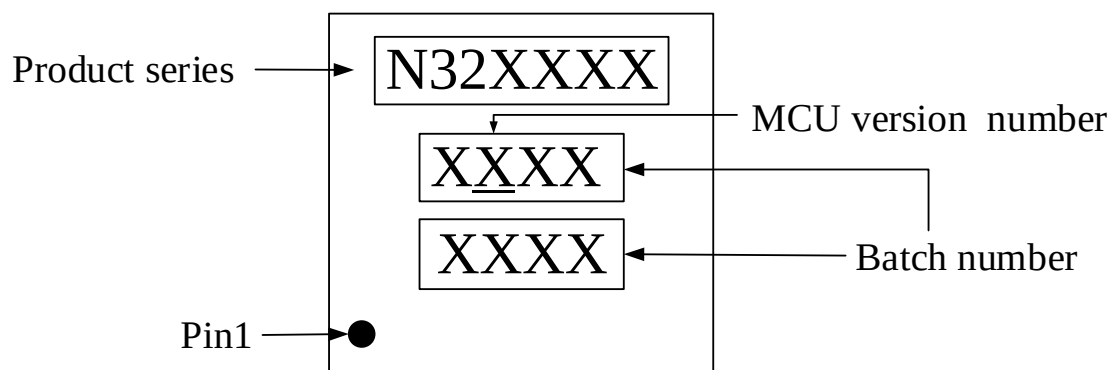
Figure 5-5 QFN20 Marking information
