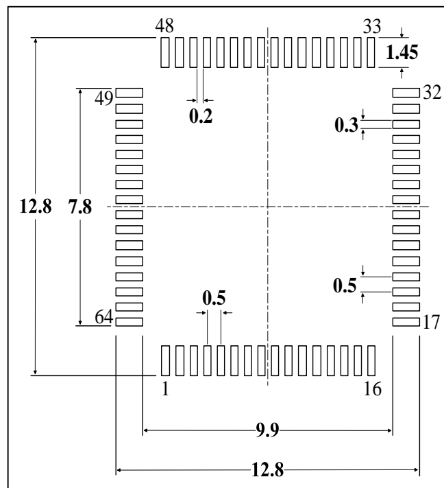
Figure 5-2 LQFP64 recommended footprint (1)
