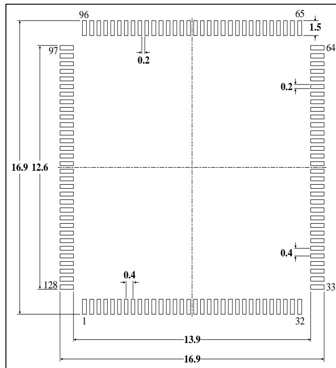
Figure 5-8 LQFP128 recommended footprint (1)
