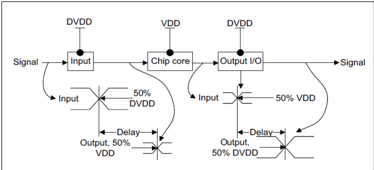
Figure 4-10 Transmission delay
