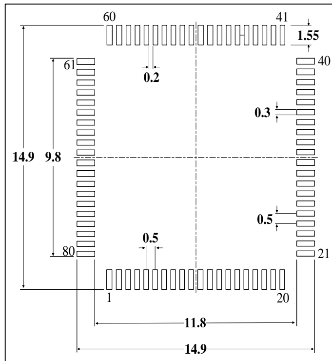
Figure 5-4 LQFP80 recommended footprint (1)
