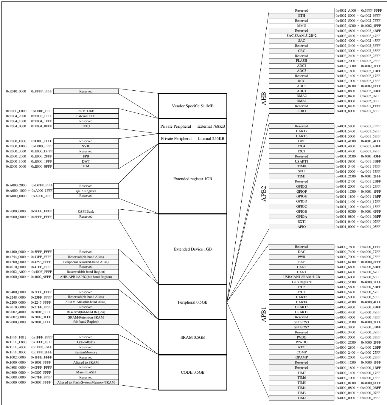
Figure 2-1 Memory map
