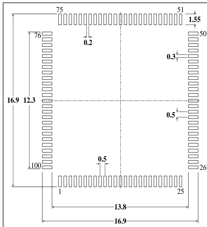
Figure 5-6 LQFP100 recommended footprint (1)
