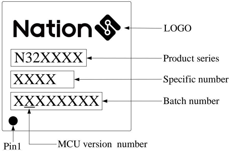
Figure 5-9 LQFP64/LQFP80/LQFP100/LQFP128 marking information
