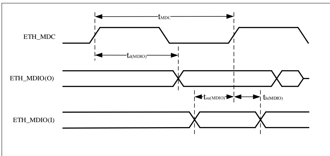
Figure 4-23 Ethernet SMI timing diagram
