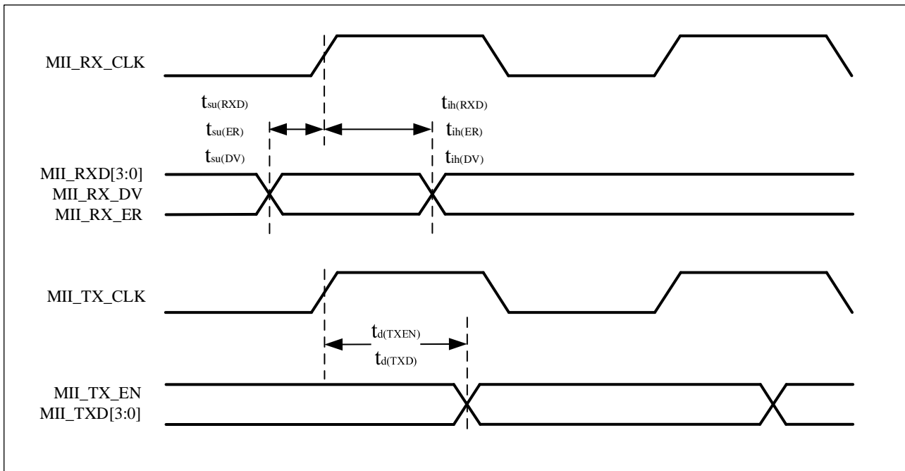
Figure 4-25 Ethernet MII timing diagram
