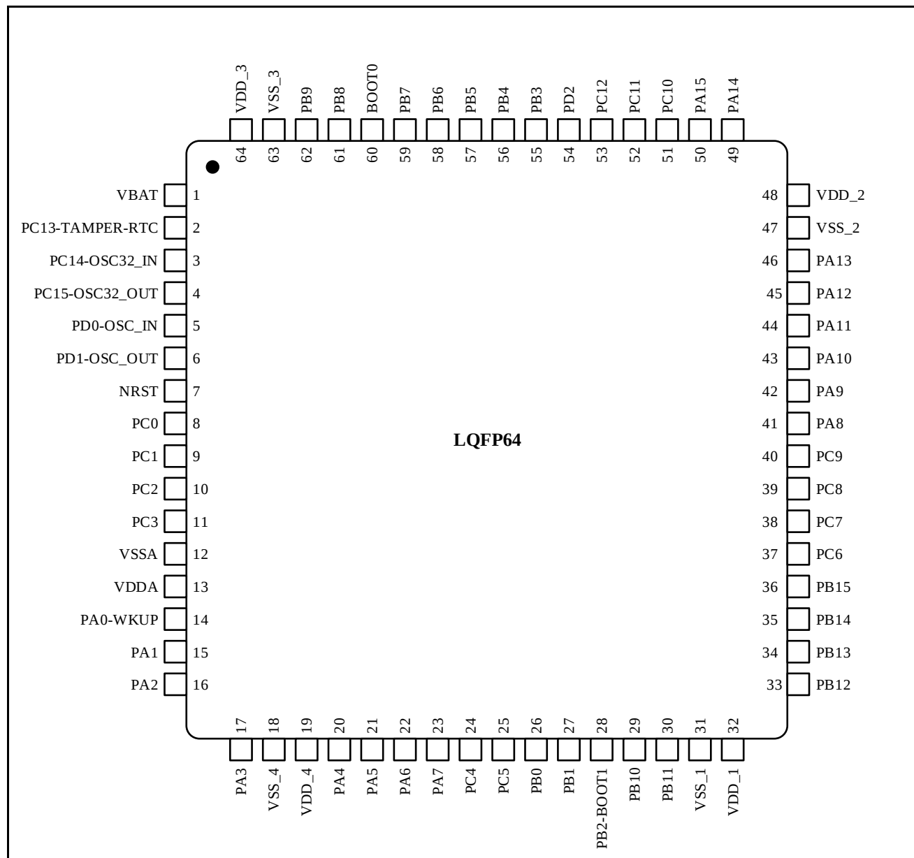
Figure 3-2 N32G451 Series LQFP64 pinout
