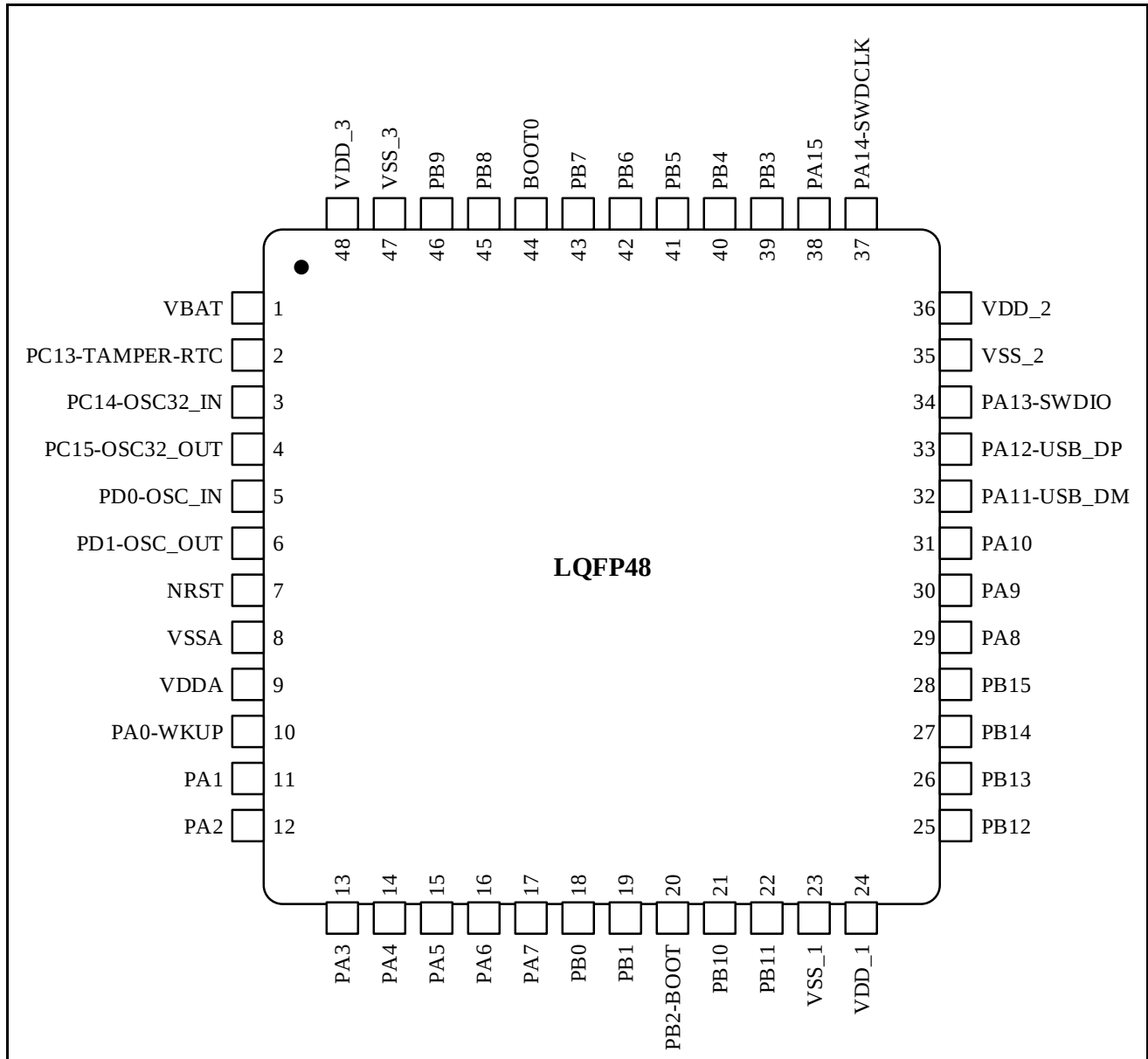
Figure 3-1 N32G451 Series LQFP48 pinout
