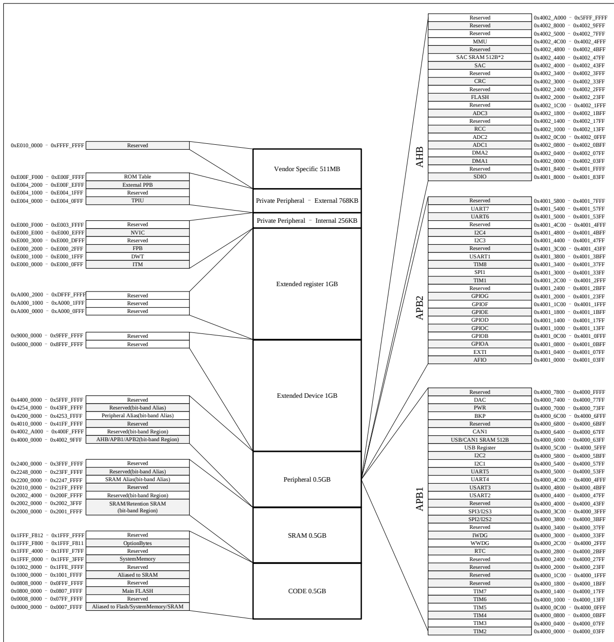
Figure 2-1 Memory map
