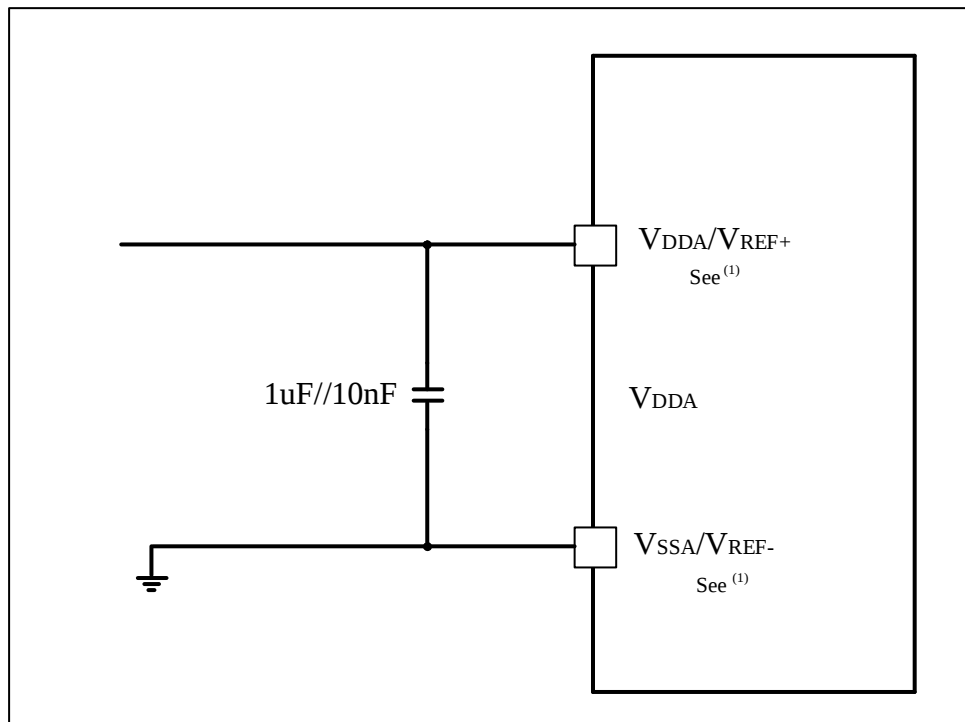
Figure 4-24 Decoupling circuit of power supply and reference power supply ( V_{REF+} is connected with V_{DDA} )
