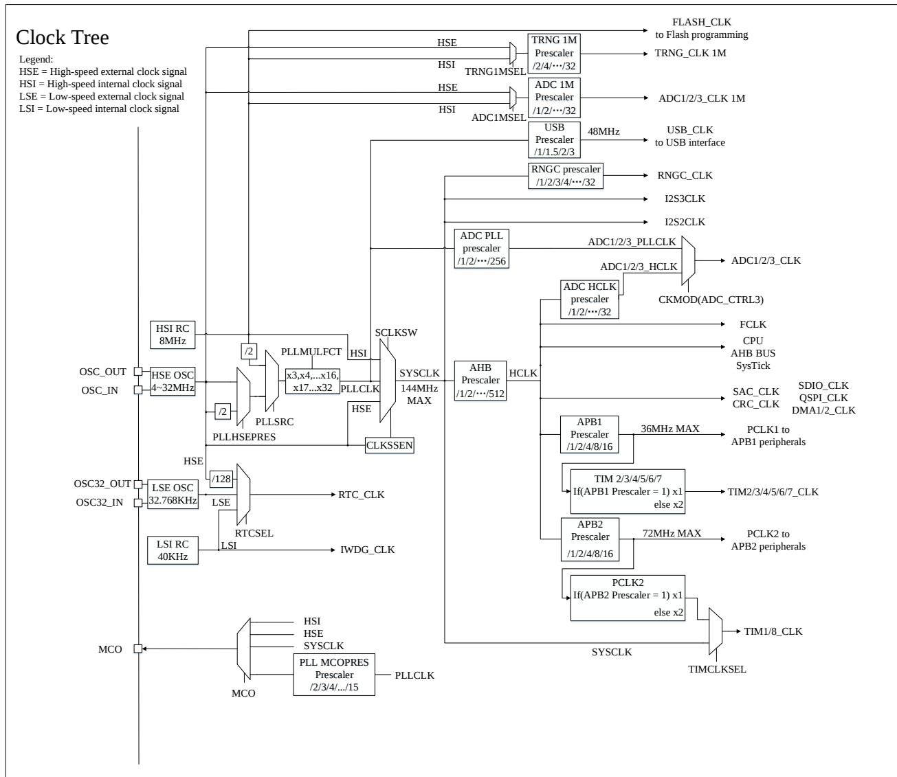
Figure 2-2 Clock tree
