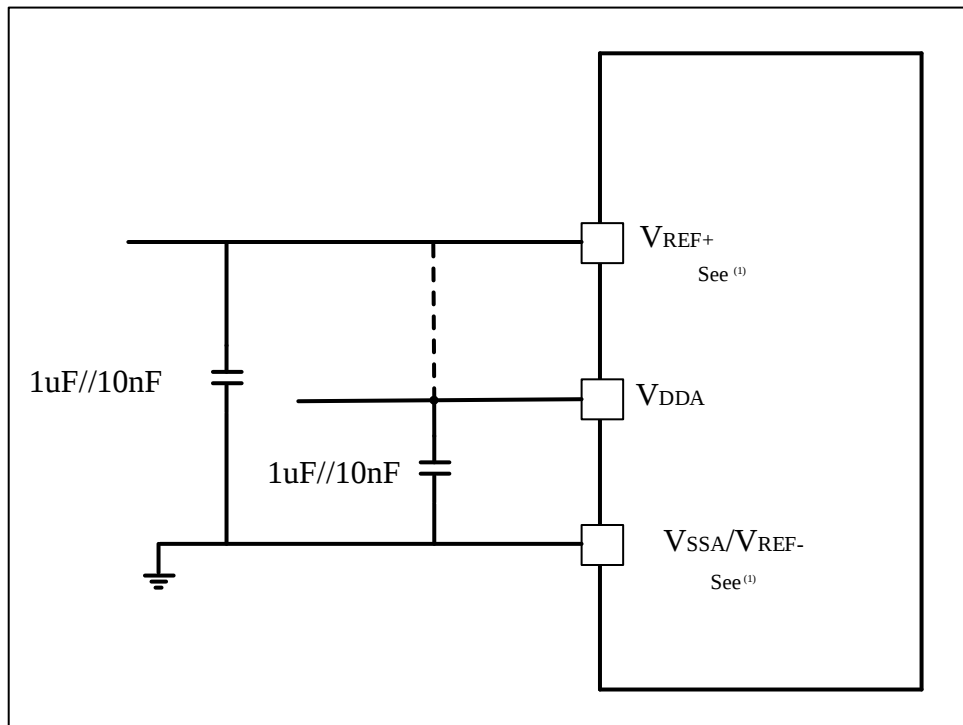
Figure 4-23 Decoupling circuit of power supply and reference power supply ( V_{REF+} is not connected to V_{DDA} )
