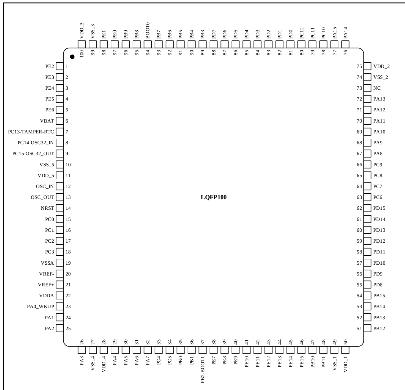
Figure 3-3 N32G451 Series LQFP100 pinout
