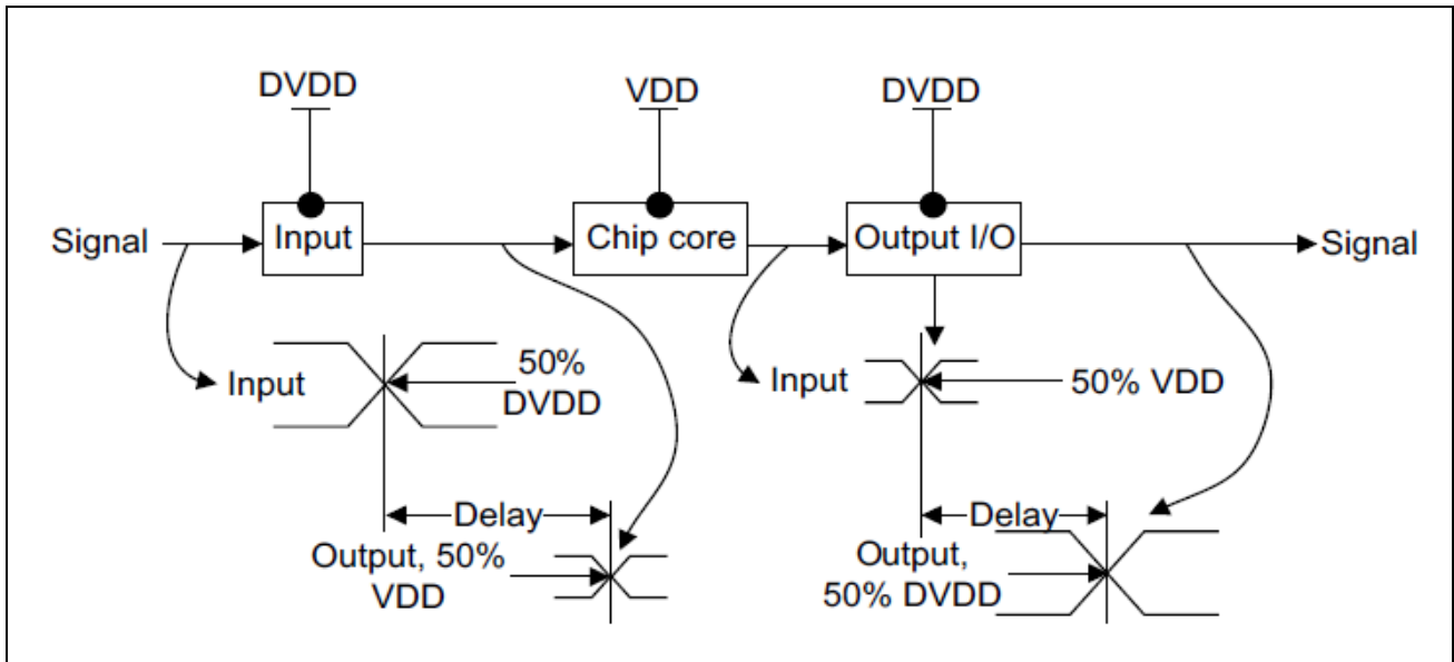
Figure 4-10 Transfer delay
