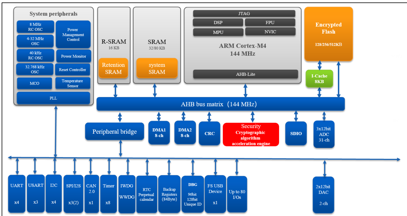
Figure 1-1 Block diagram of N32G451 series
