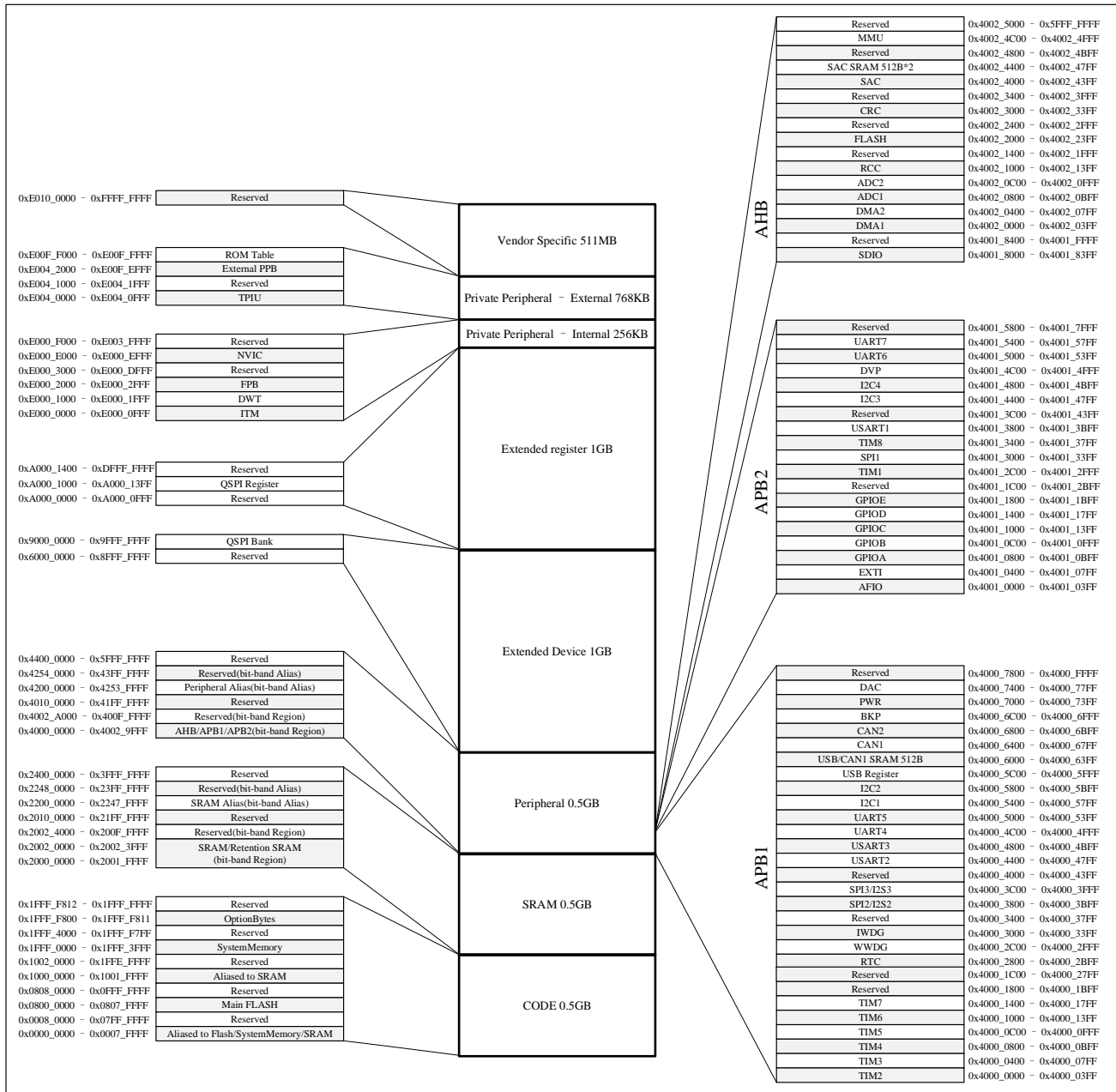
Figure 2-1 Memory map
