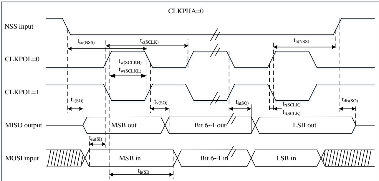
Figure 4-13 SPI timing diagram-slave mode and CLKPHA=0
