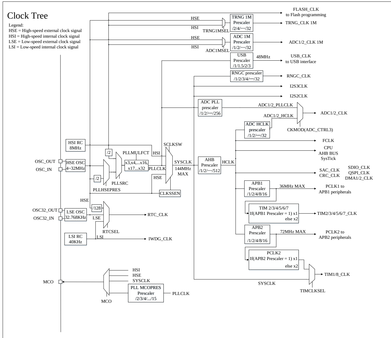
Figure 5-2 Clock Tree
