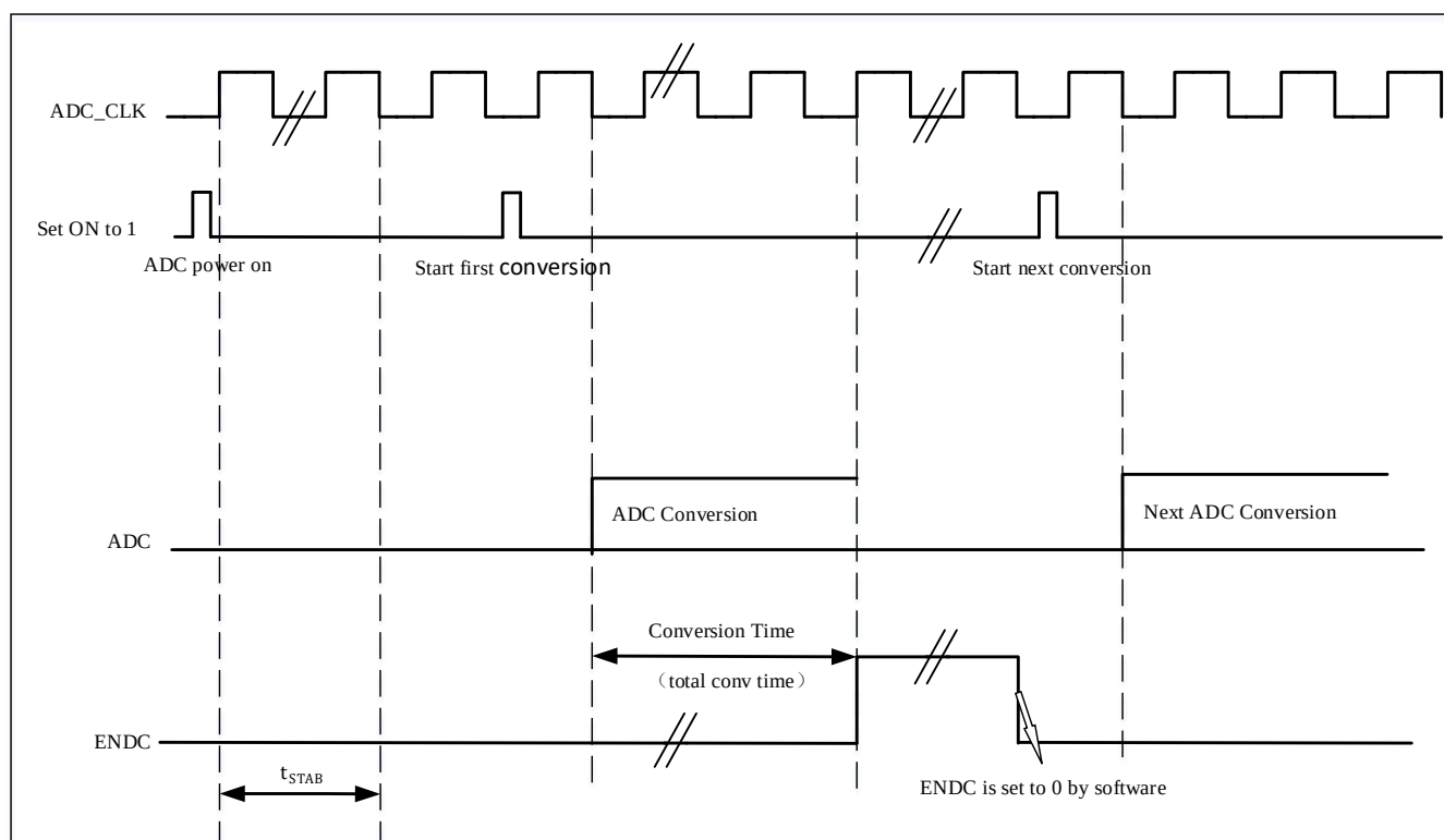
Figure 9-4 Timing diagram
