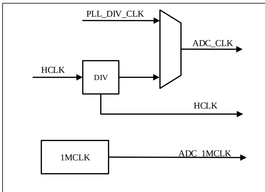
Figure 9-2 ADC clock
