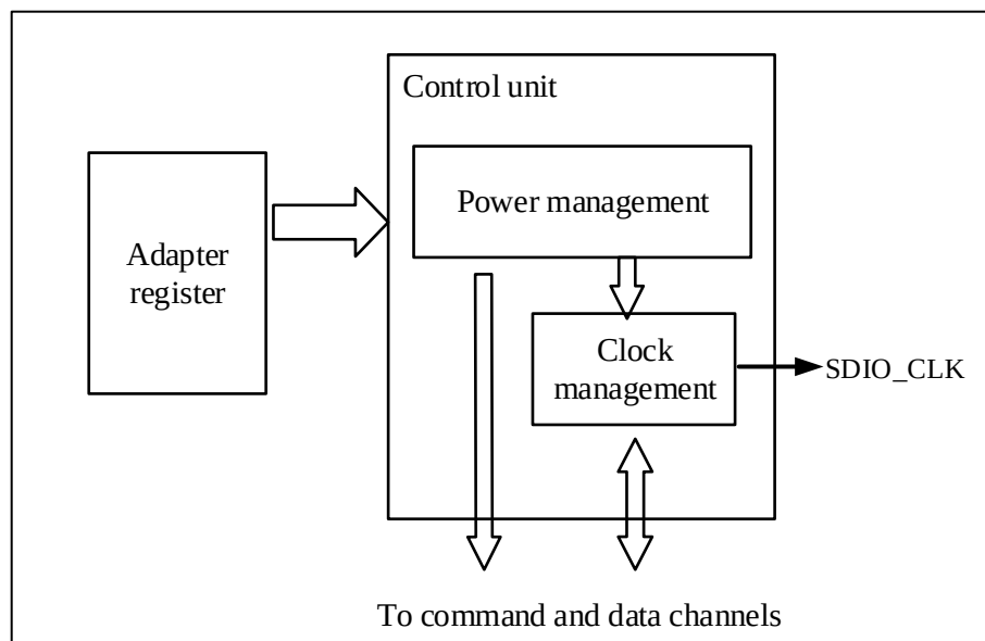
Figure 18-8 Control unit
