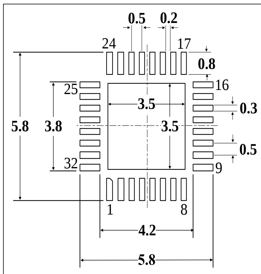
图 5-12 QFN32-1封装焊盘建议 (1)
