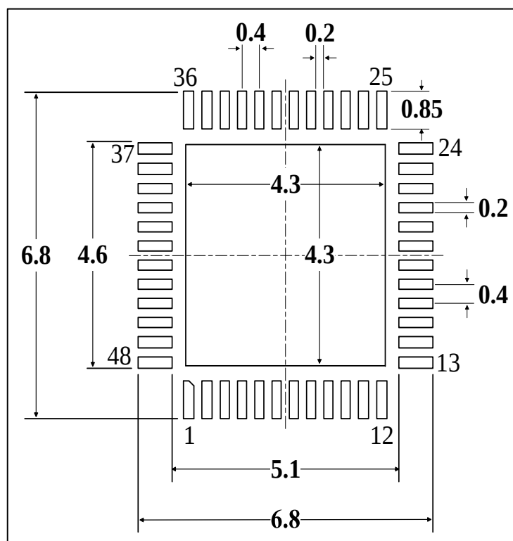
Figure 5-16 QFN48 Recommended footprint (1)
