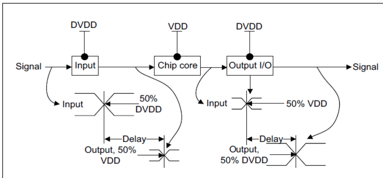
Figure 4-10 Propagation delay
