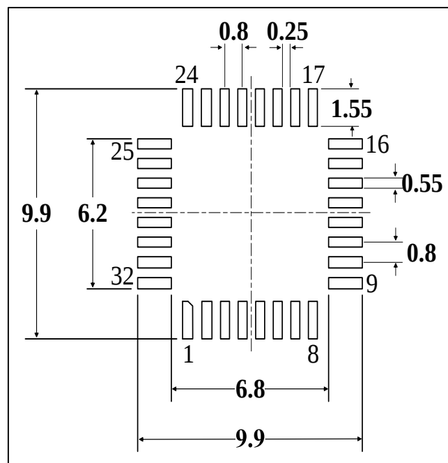
Figure 5-2 LQFP32 Recommended footprint (1)
