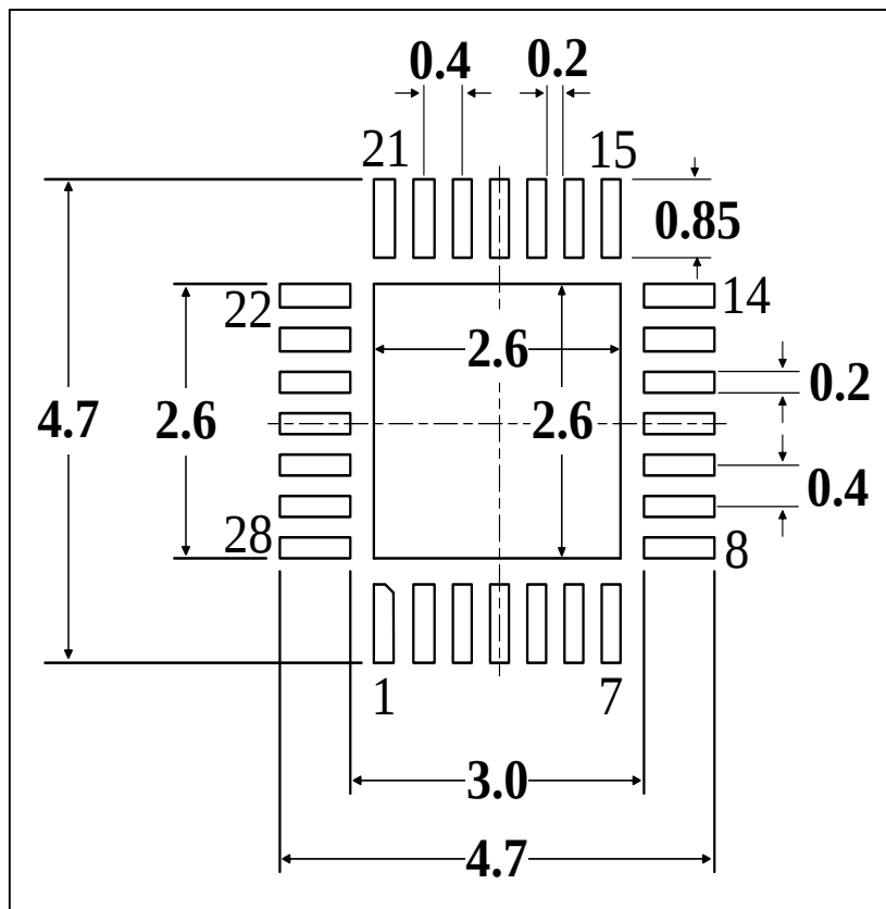
Figure 5-8 QFN28 Recommended footprint (1)
