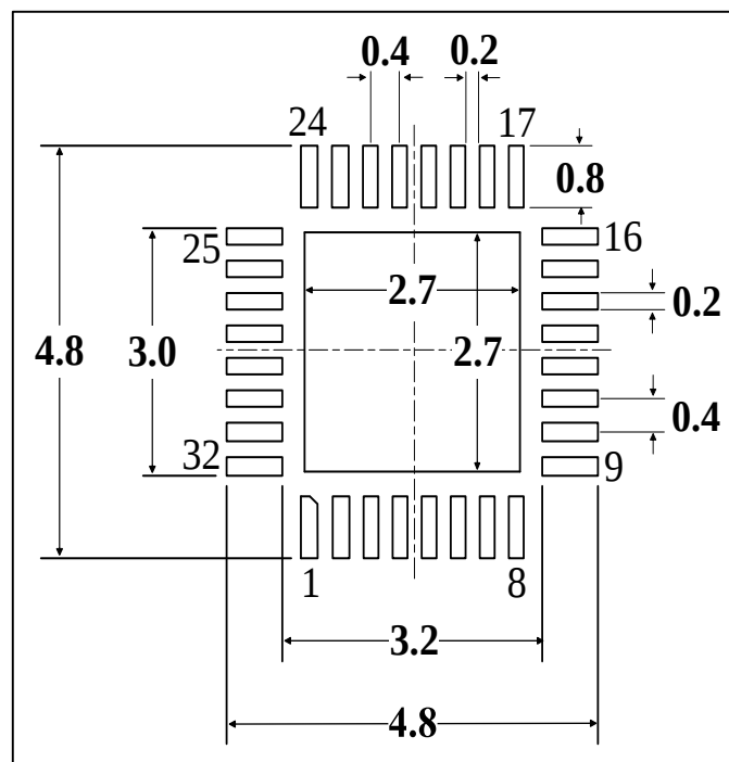
Figure 5-10 QFN32 Recommended footprint (1)
