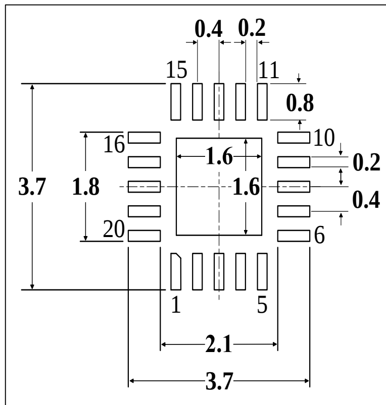
Figure 5-6 QFN20 Recommended footprint (1)
