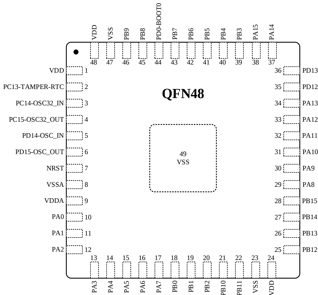
Figure 3-8 N32G401 Series QFN48 pinout
