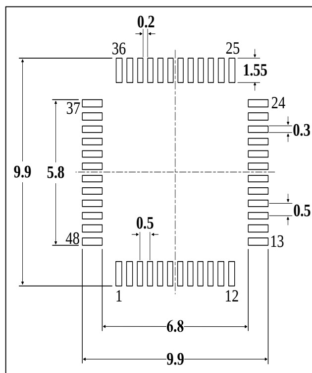
Figure 5-4 LQFP48 Recommended footprint (1)
