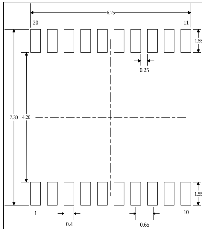
Figure 5-18 TSSOP20 Recommended footprint (1)
