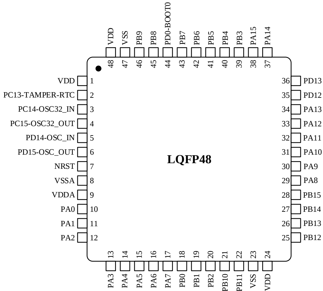
Figure 3-2 N32G401 Series LQFP48 pinout
