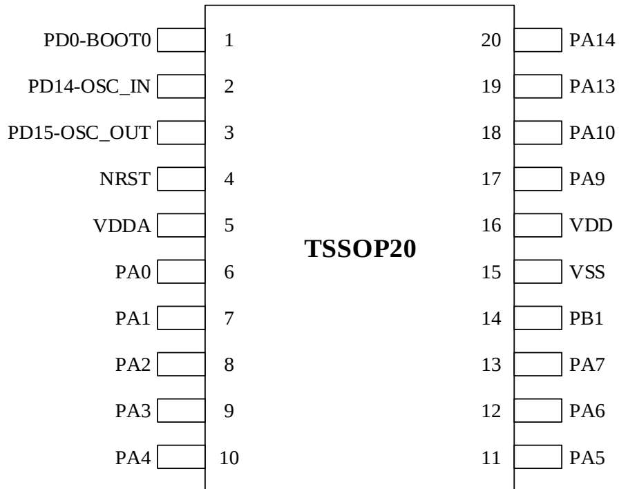
Figure 3-9 N32G401 Series TSSOP20 pinout
