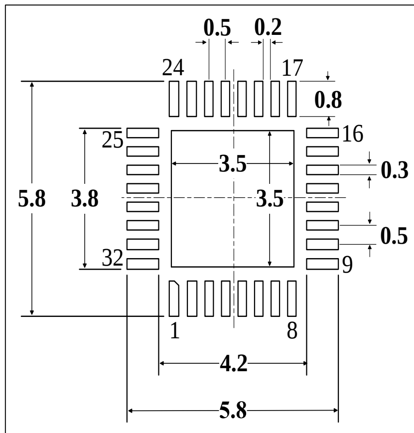
Figure 5-12 QFN32-1 Recommended footprint (1)
