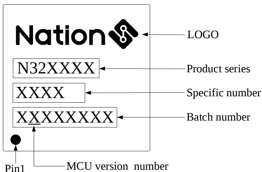
Figure 5-19 LQFP48/LQFP32/LQFP28/QFN48/QFN32/QFN32-1/QFN32-2/QFN28 Marking information
