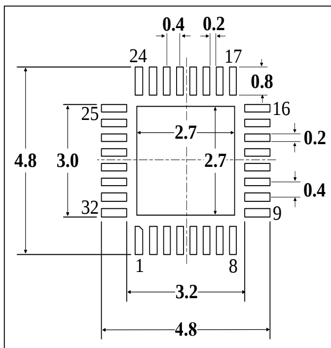
Figure 5-14 QFN32-2 Recommended footprint (1)
