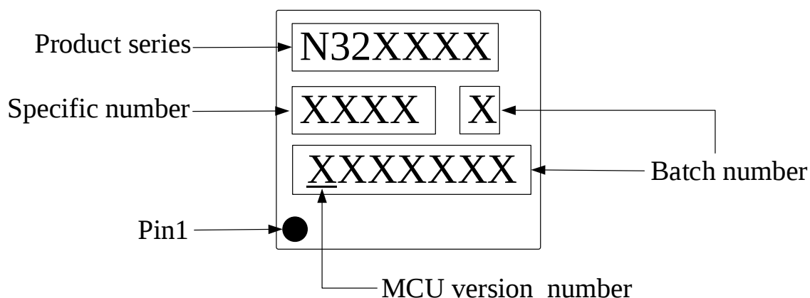
Figure 5-21 QFN20 Marking information
