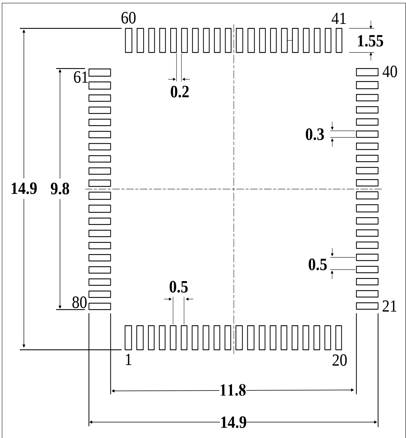
Figure 5-16 LQFP80 (12mmx12mm) Recommended footprint (1)
