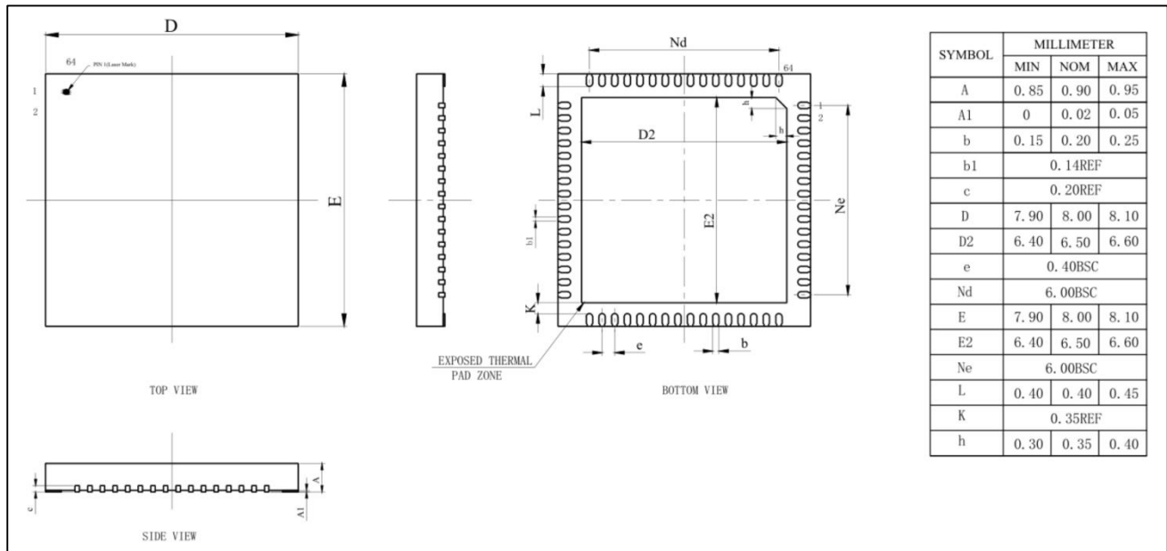
Figure 5-9 QFN64 (8mmx8mm) package outline
