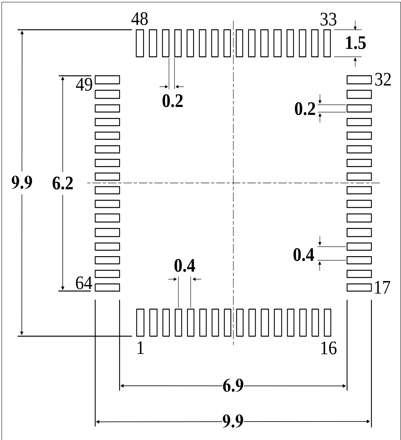
Figure 5-12 LQFP64 (7mmx7mm) Recommended footprint (1)
