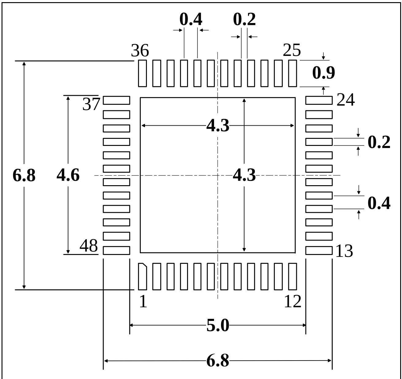
Figure 5-6 QFN48 (6mmx6mm) Recommended footprint (1)
