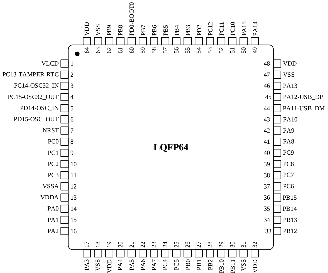
Figure 3-6 N32L406 (7mm x 7mm) series LQFP64 pinout
