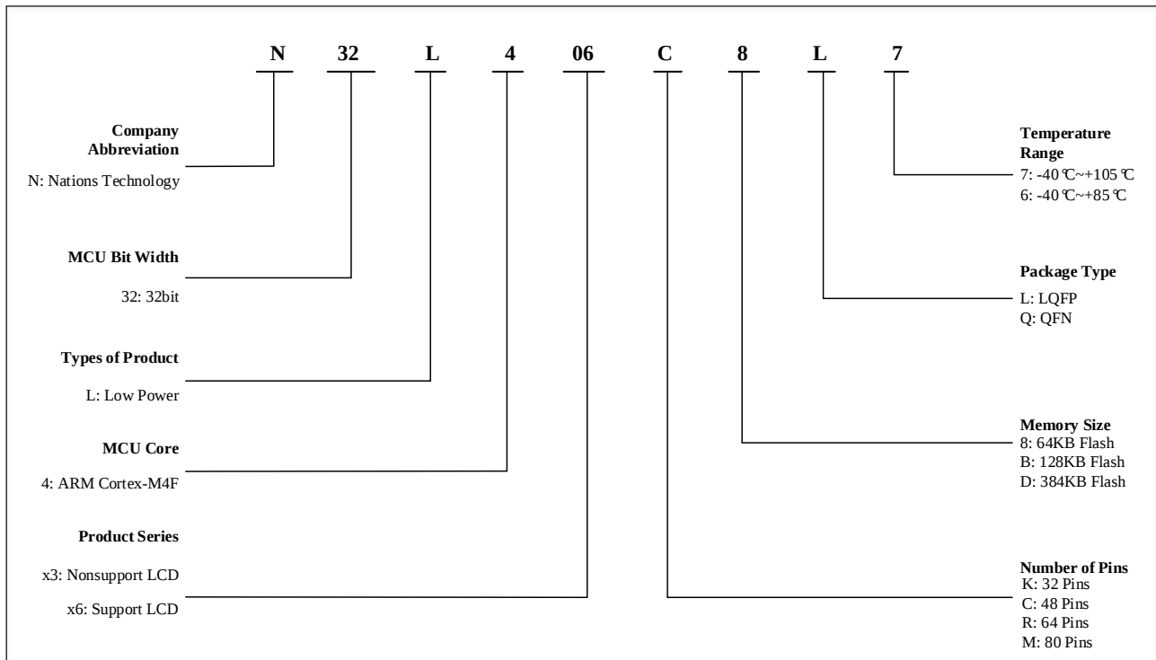
Figure 6-1 N32L40x series part number information
