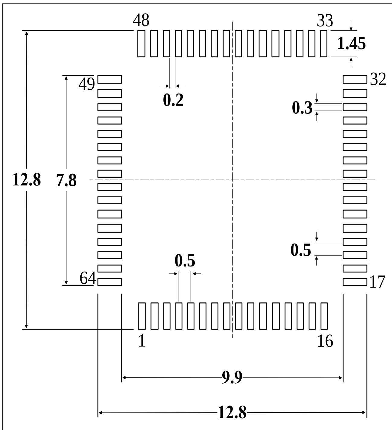
Figure 5-14 LQFP64 (10mmx10mm) Recommended footprint (1)
