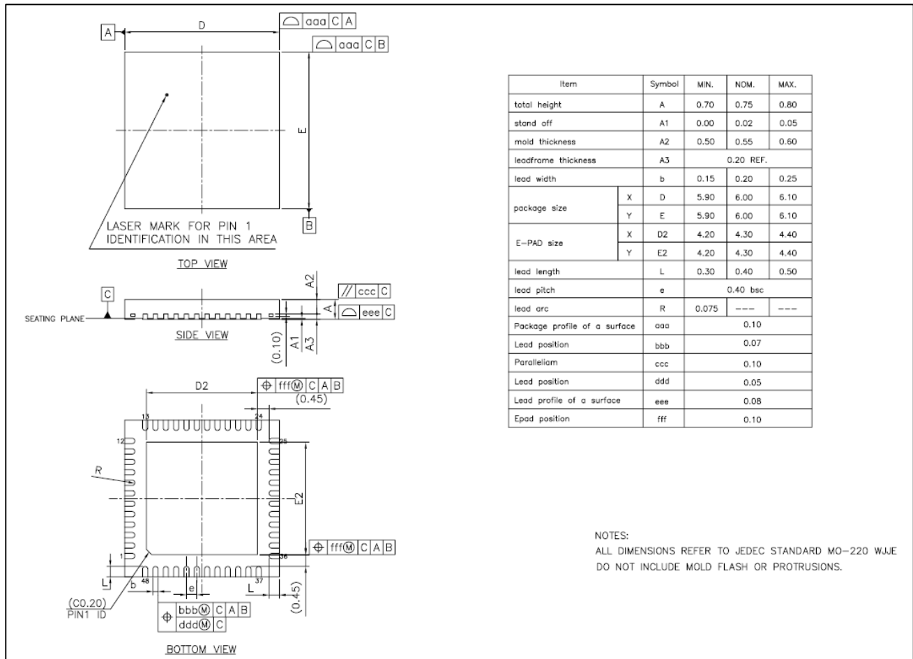
Figure 5-5 QFN48 (6mmx6mm) package outline
