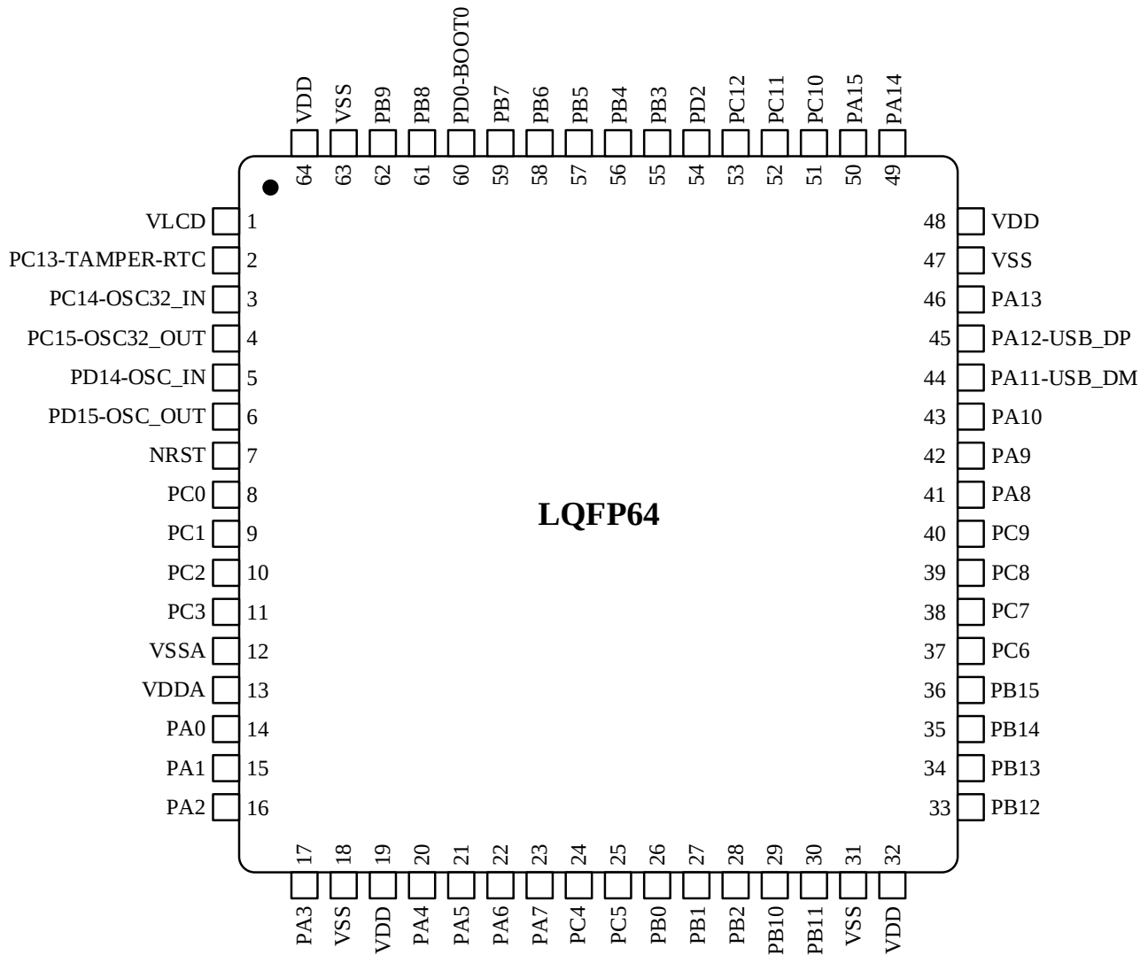
Figure 3-7 N32L402/N32L406 (10mm x 10mm) series LQFP64 pinout
