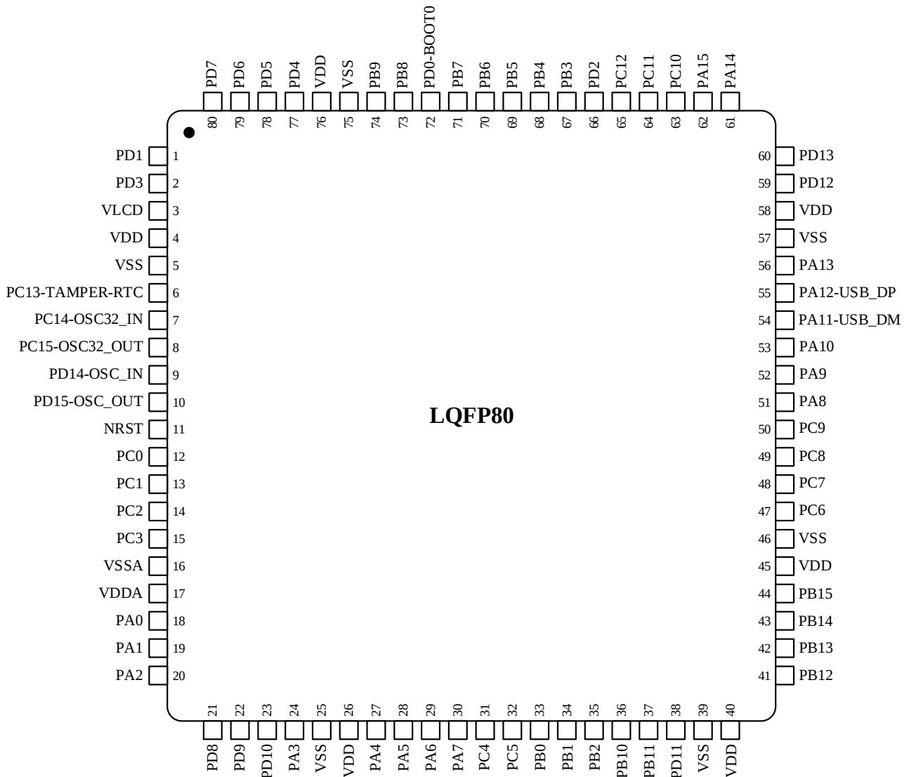
Figure 3-8 N32L406 (12mm x 12mm) series LQFP80 pinout
