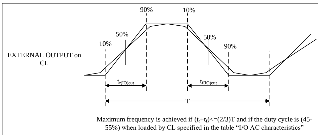
Figure 4-9 Definition of input/output AC characteristics
