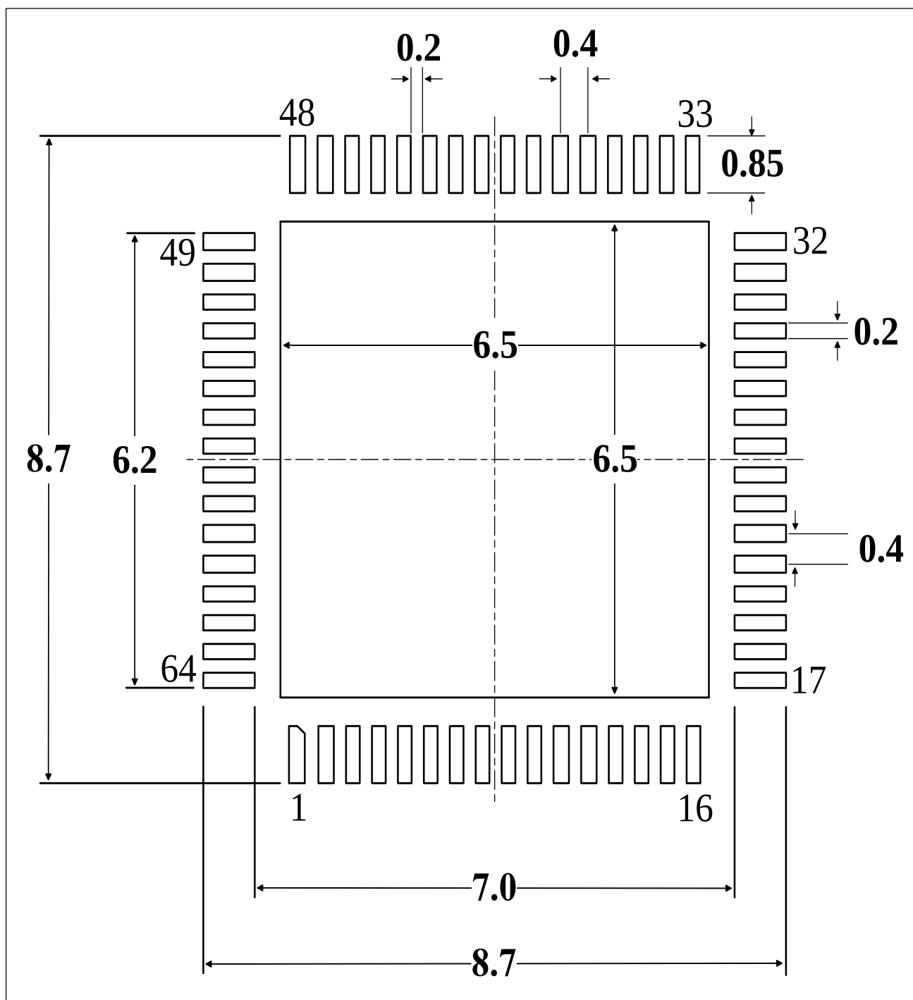
Figure 5-10 QFN64 (8mmx8mm) Recommended footprint (1)
