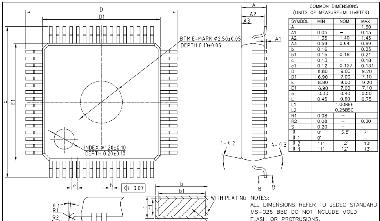
Figure 5-11 LQFP64 (7mmx7mm) package outline
