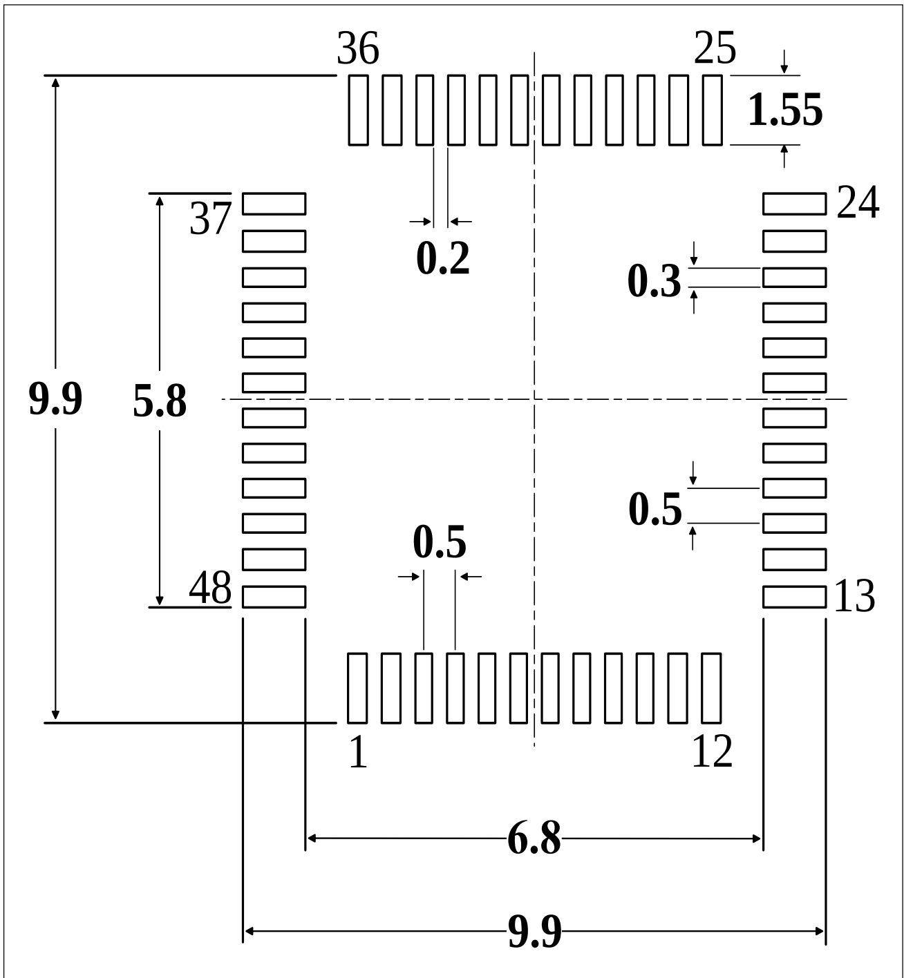
Figure 5-8 LQFP48 (7mmx7mm) Recommended footprint (1)
