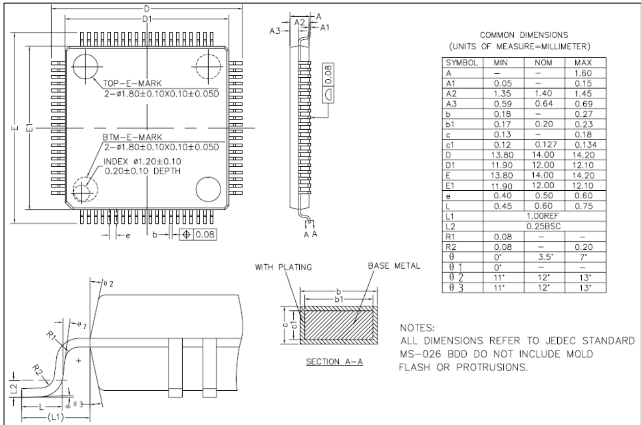
Figure 5-15 LQFP80 (12mmx12mm) package outline
