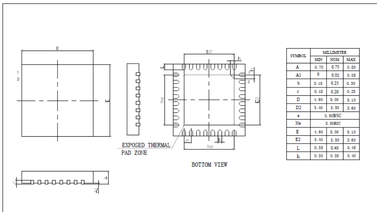
Figure 5-3 QFN32 (5mmx5mm) package outline
