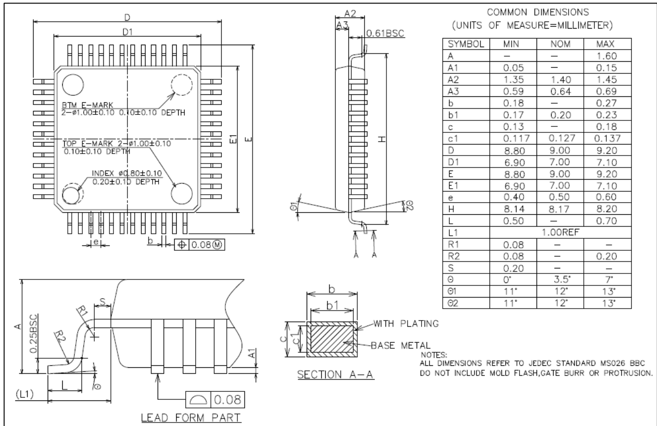
Figure 5-7 LQFP48 (7mmx7mm) package outline
