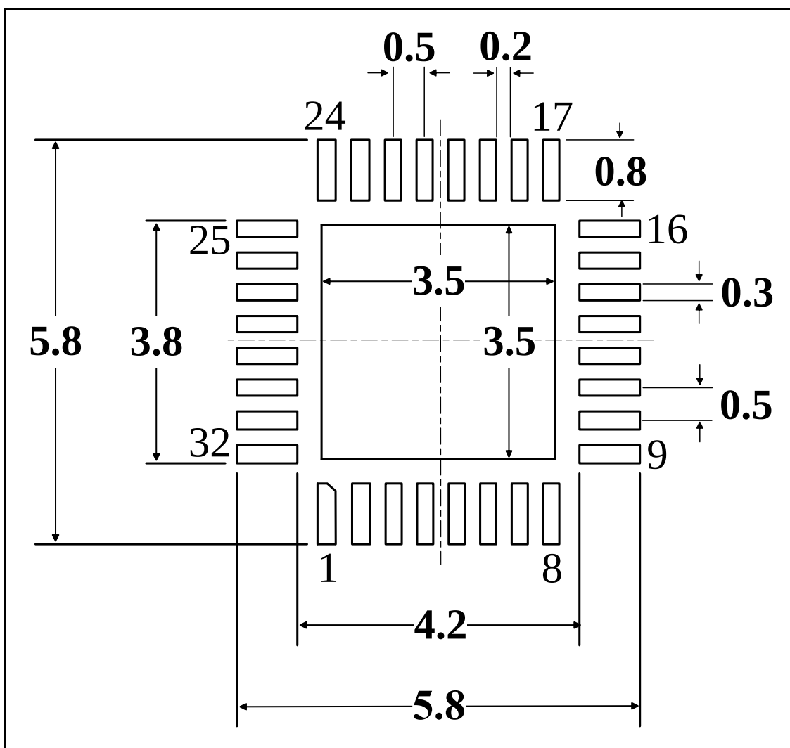
Figure 5-4 QFN32 (5mmx5mm) Recommended footprint (1)
