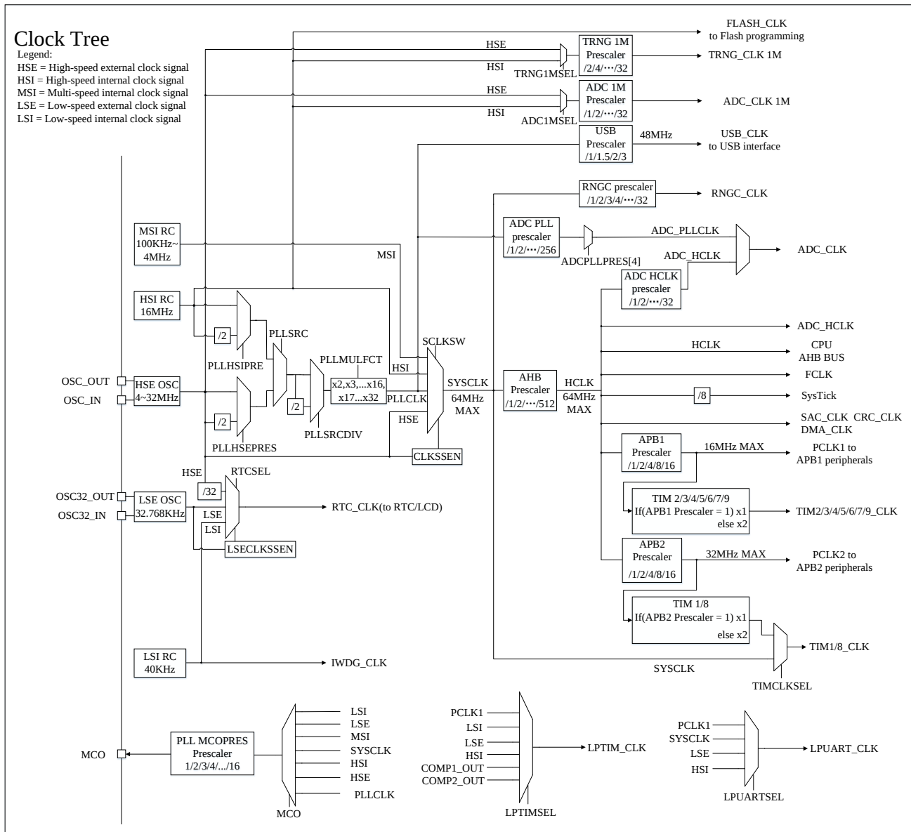
Figure 2-2 Clock tree
