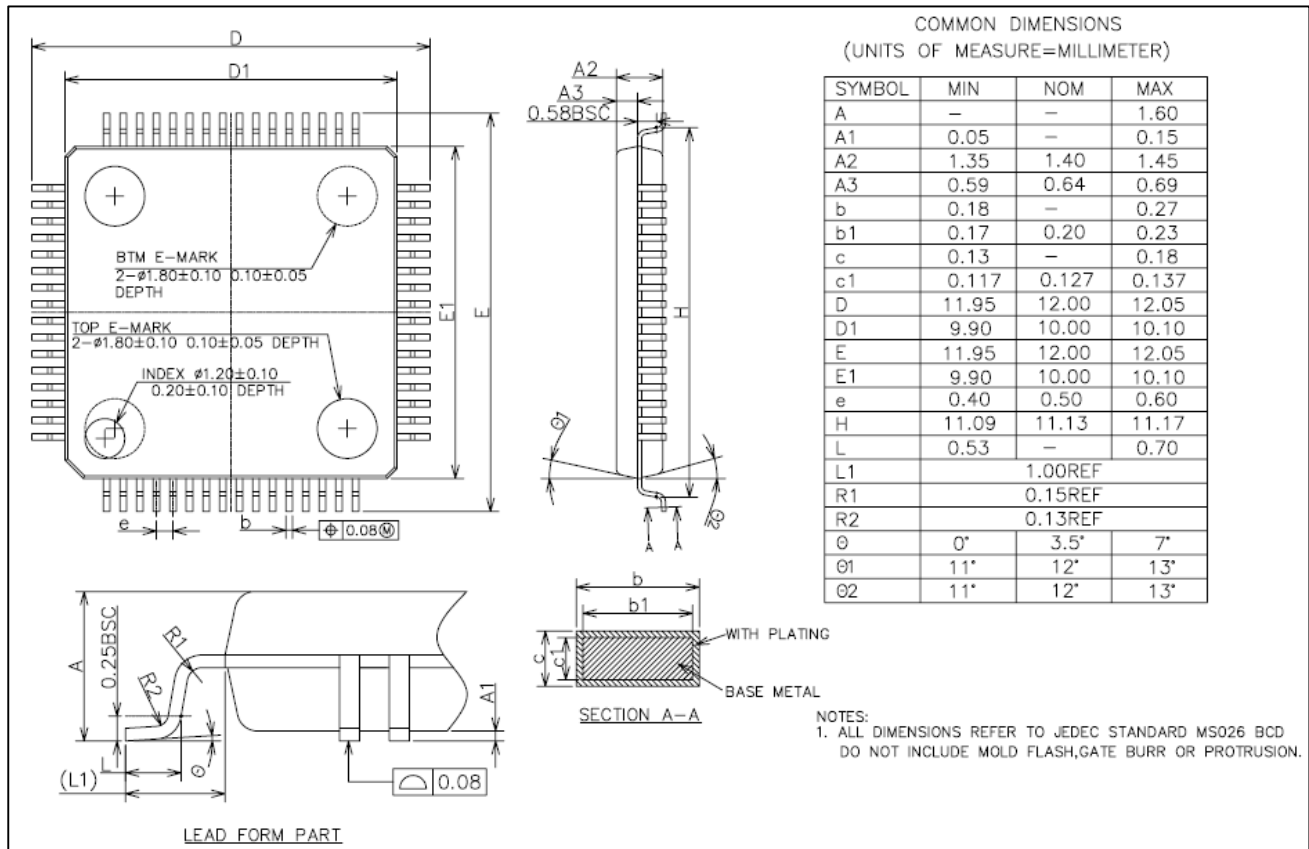
Figure 5-13 LQFP64 (10mmx10mm) package outline
