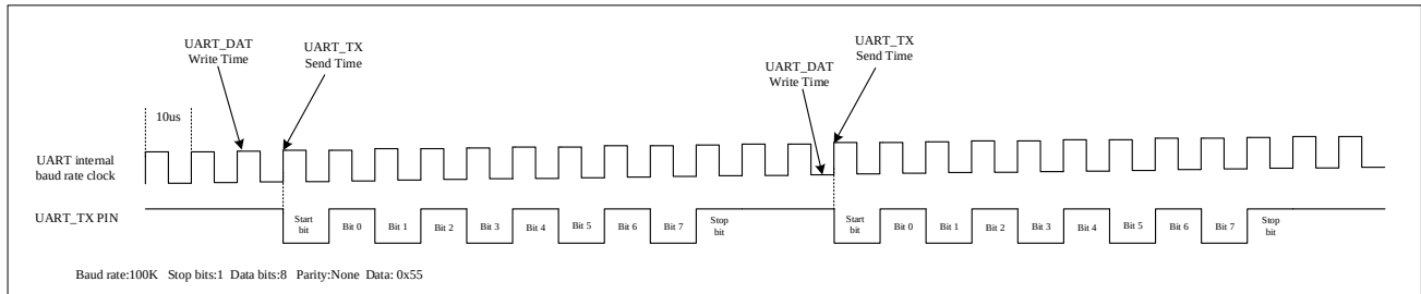
Figure 23-5 Transmit timing difference
