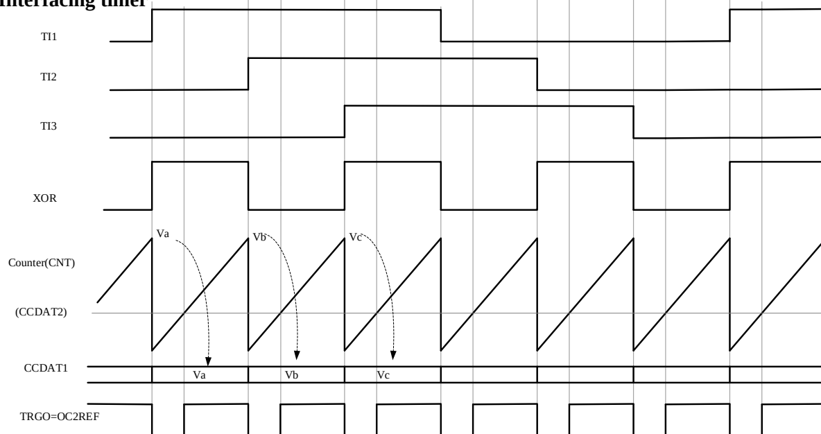
Interfacing timer
