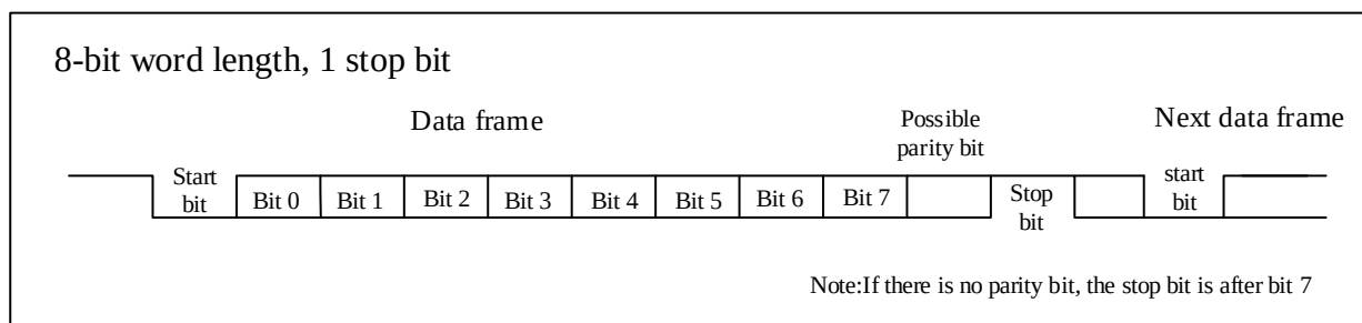
Figure 24-2 frame format
