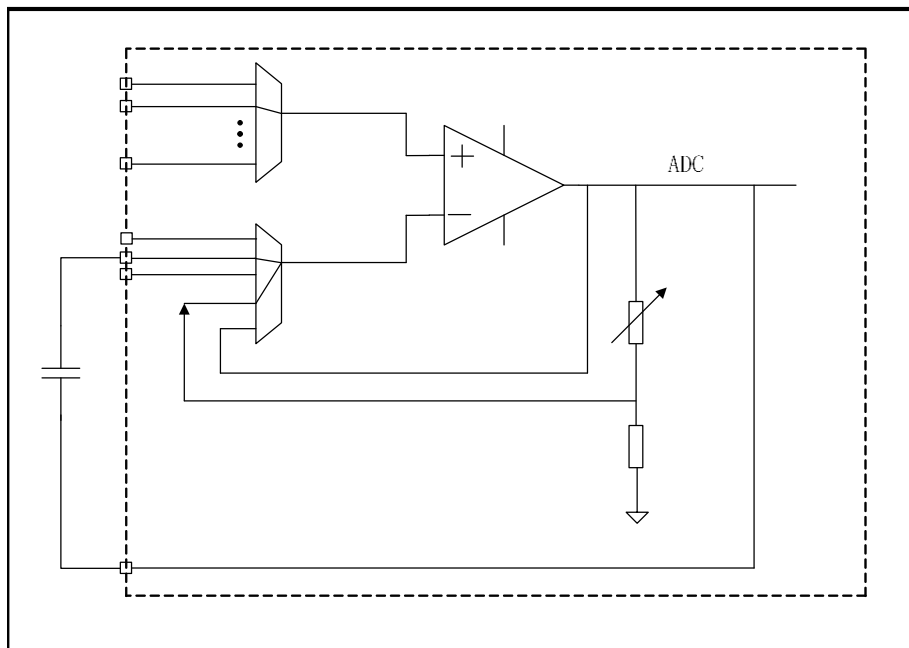
Figure 20-5 Internal gain mode with filtering
