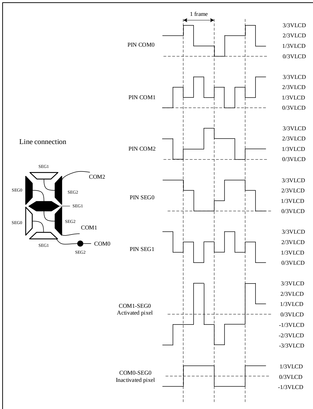
Figure 21-5 1/3 duty cycle, 1/3 bias
