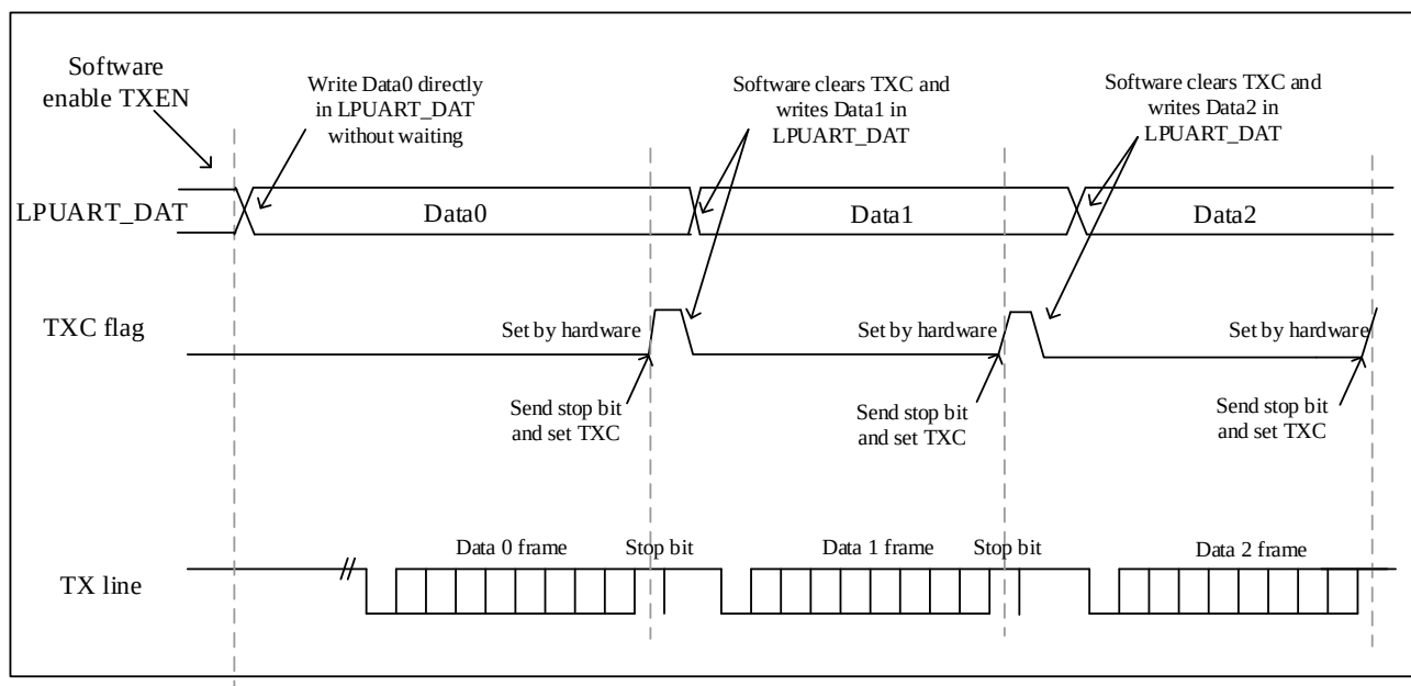
Figure 24-3 TxC changes during transmission
