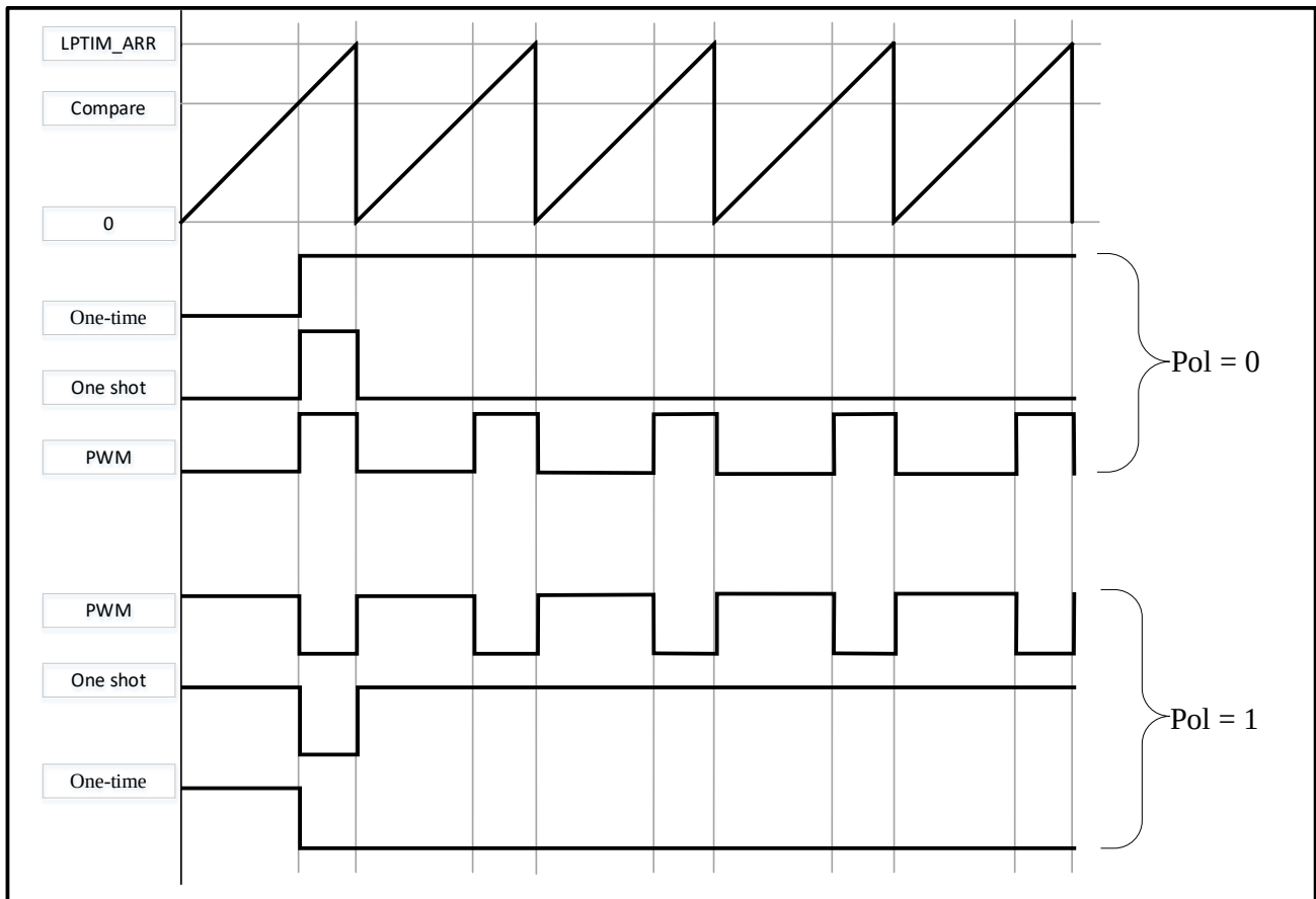
Figure 13-6 Waveform generation
