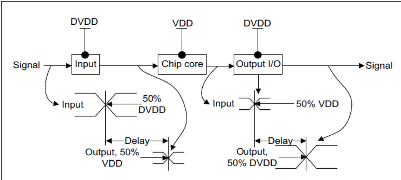
Figure 4-10 Transmission delay
