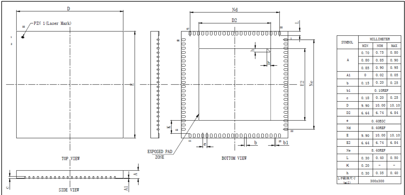
Figure 5-5 QFN88 package outline
