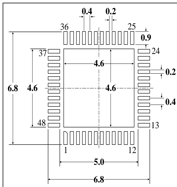
Figure 5-2 QFN48 recommended footprint (1)
