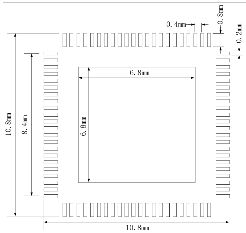
Figure 5-6 QFN88recommended footprint (1)
