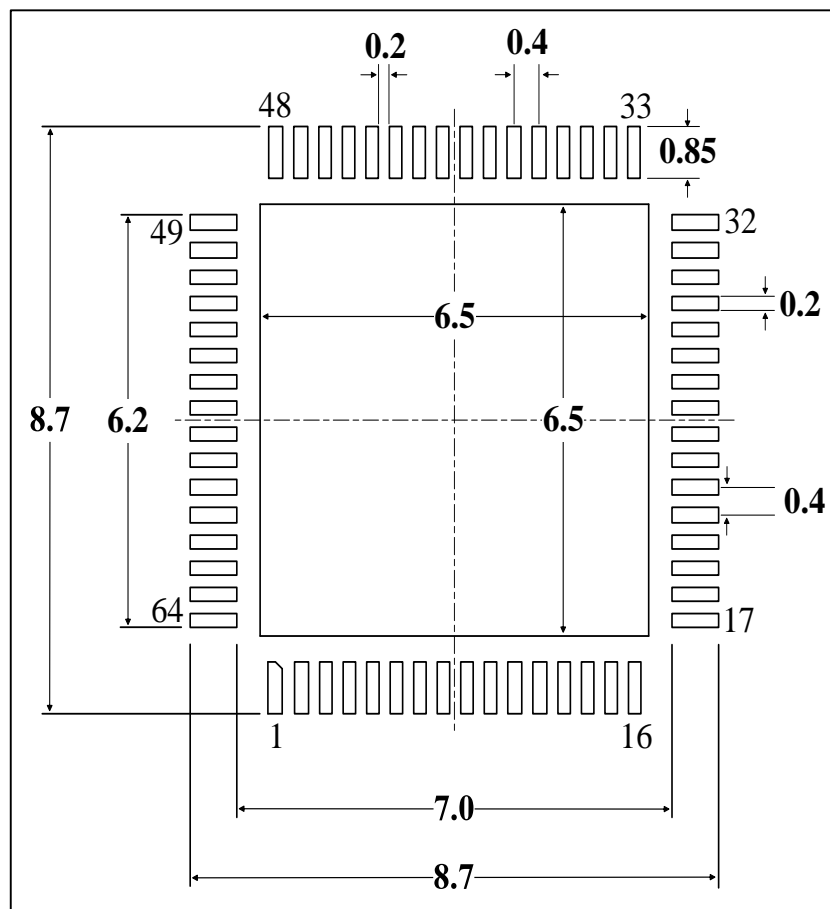
Figure 5-4 QFN64 recommended footprint (1)
