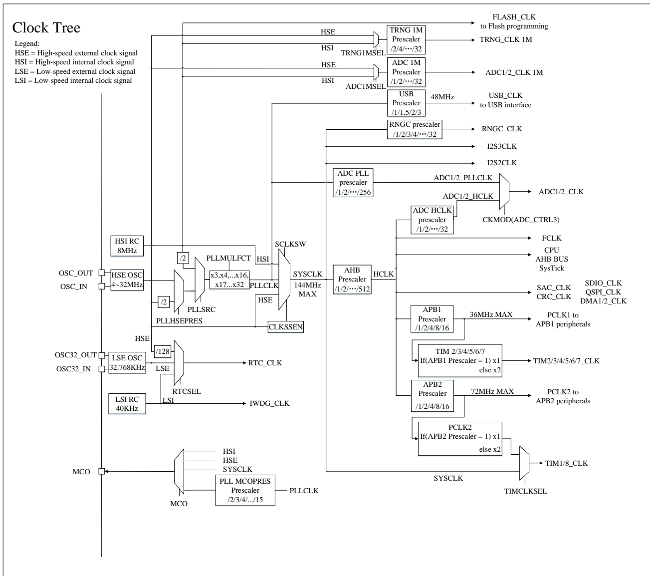
Figure 2-2 Clock tree
