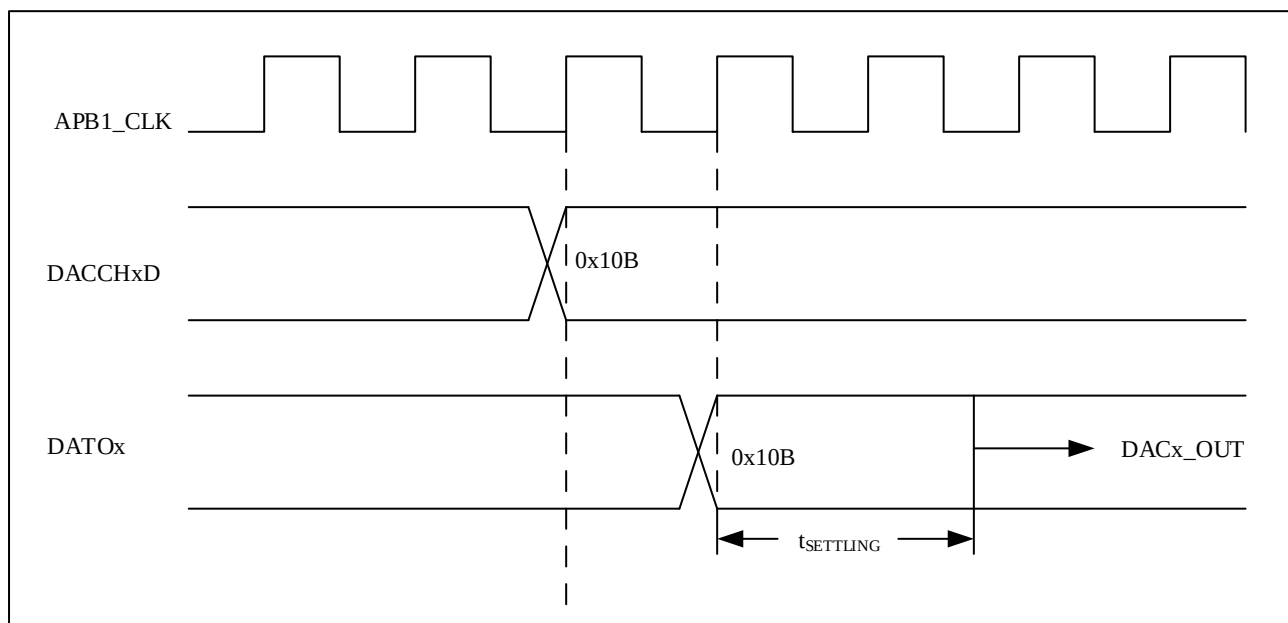
Figure 11-4 Time diagram of transitions with trigger disabled
