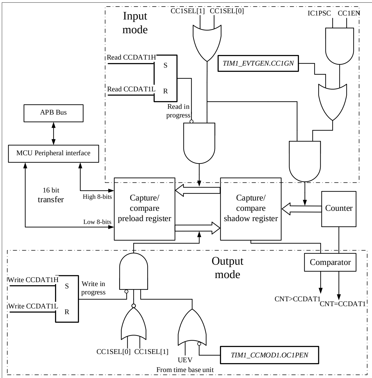
Figure 12-17 Capture/compare channel 1 main circuit
