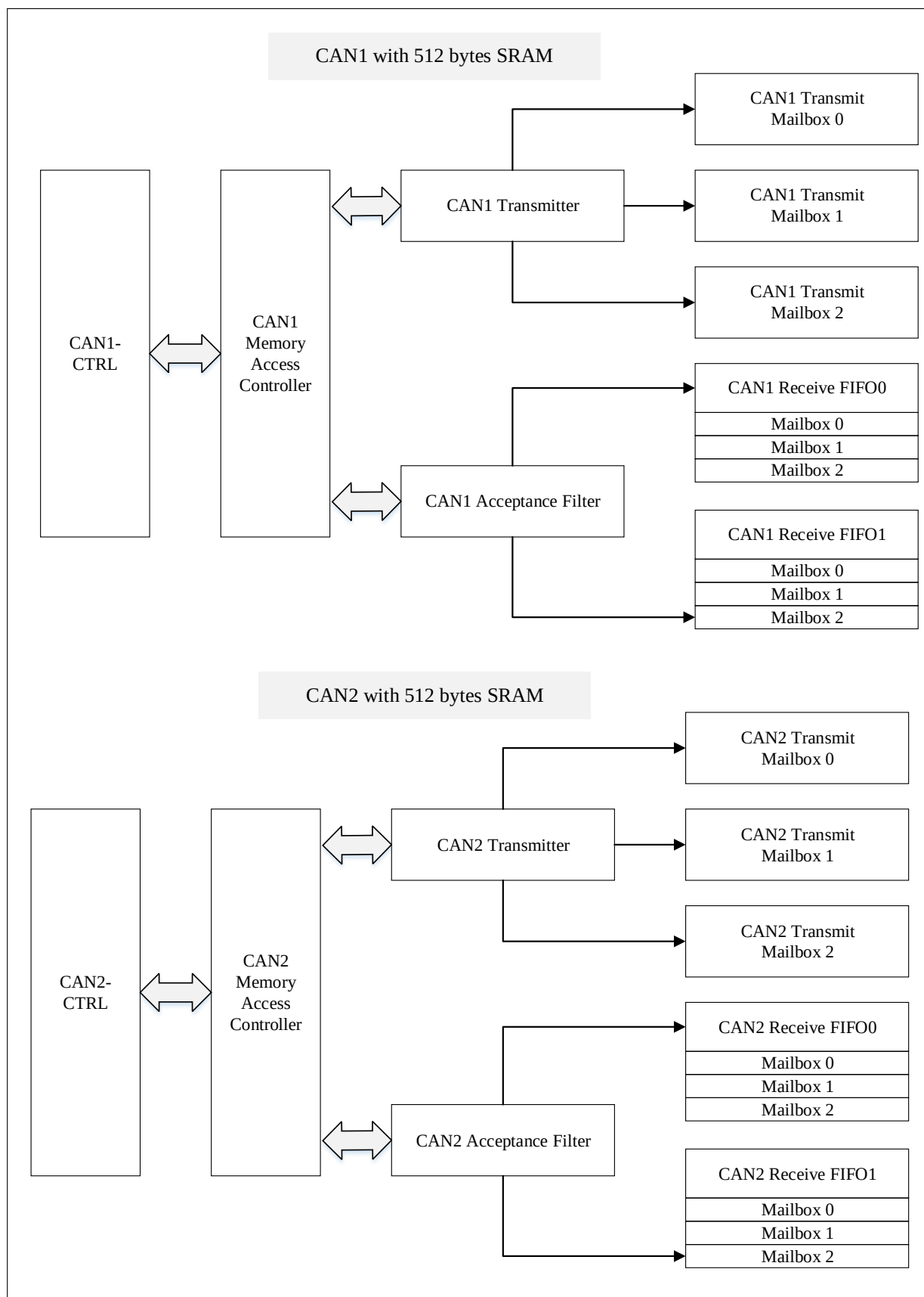
Figure 21-3 Dual CAN block diagram
