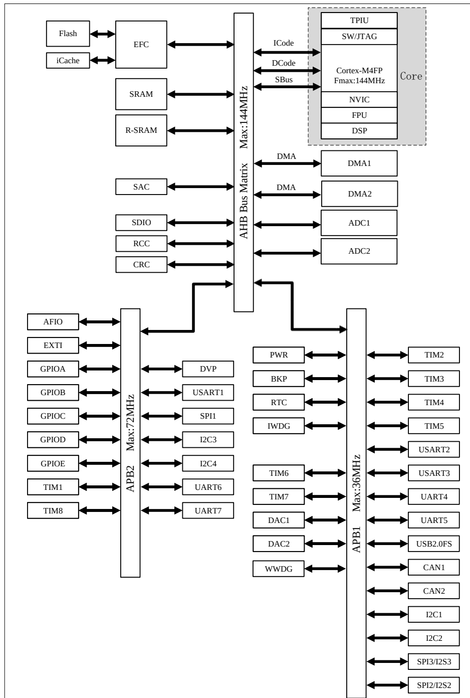
Figure 2-2 Bus architecture
