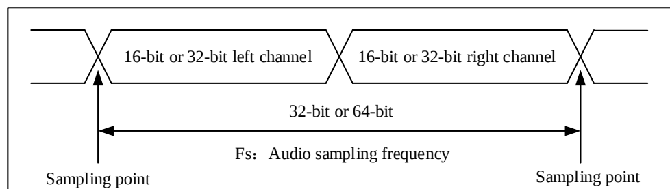
Figure 22-26 Audio sampling frequency definition
