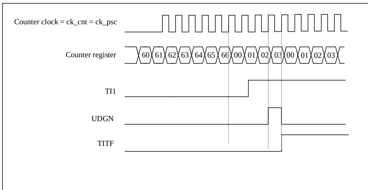
Figure 12-27 Control circuit in reset mode
