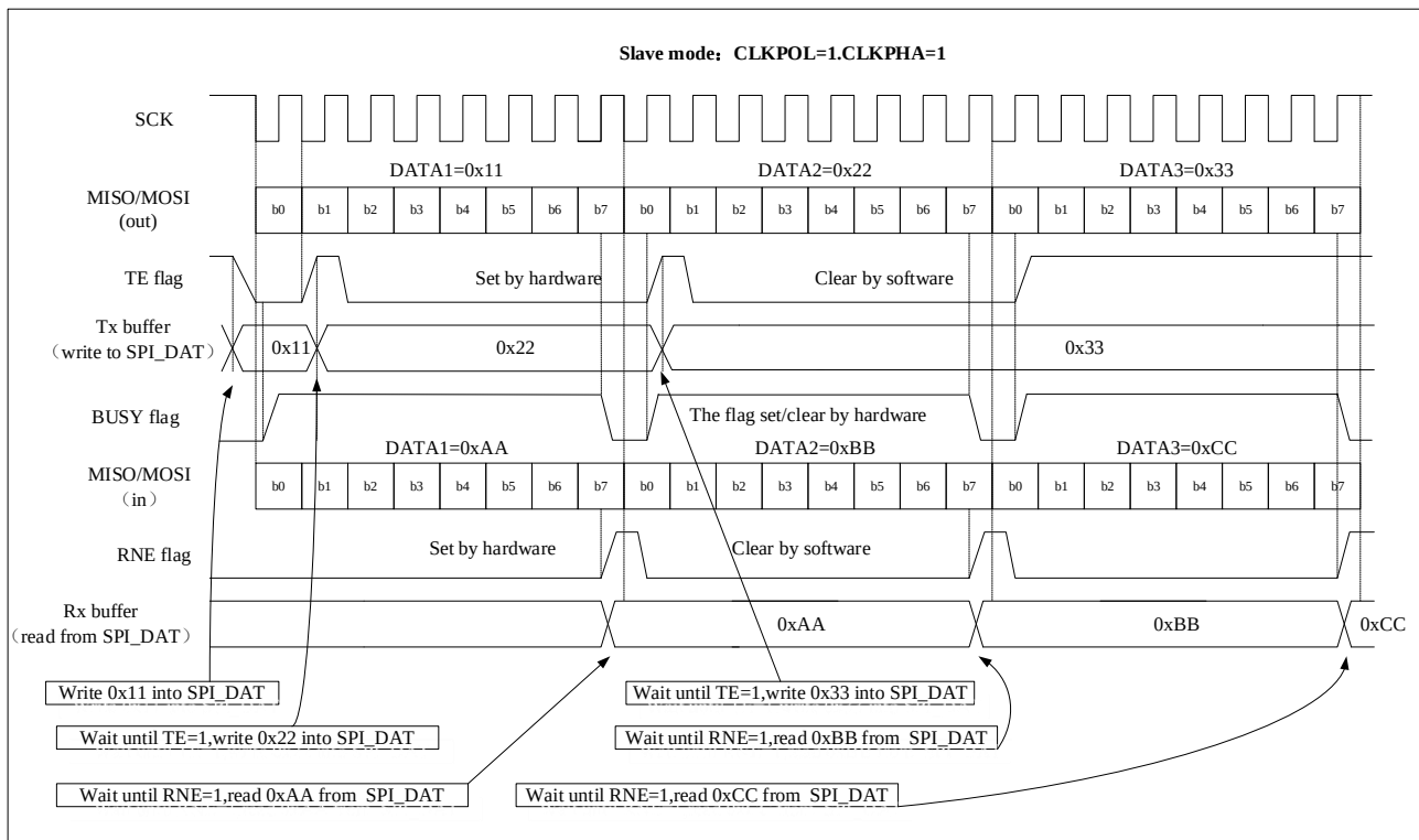
Figure 22-8 Schematic diagram of the change of TE/RNE/BUSY when the slave is continuously transmitting in full duplex mode
