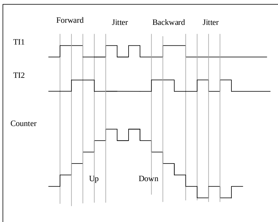
Figure 12-32 Example of counter operation in encoder interface mode
