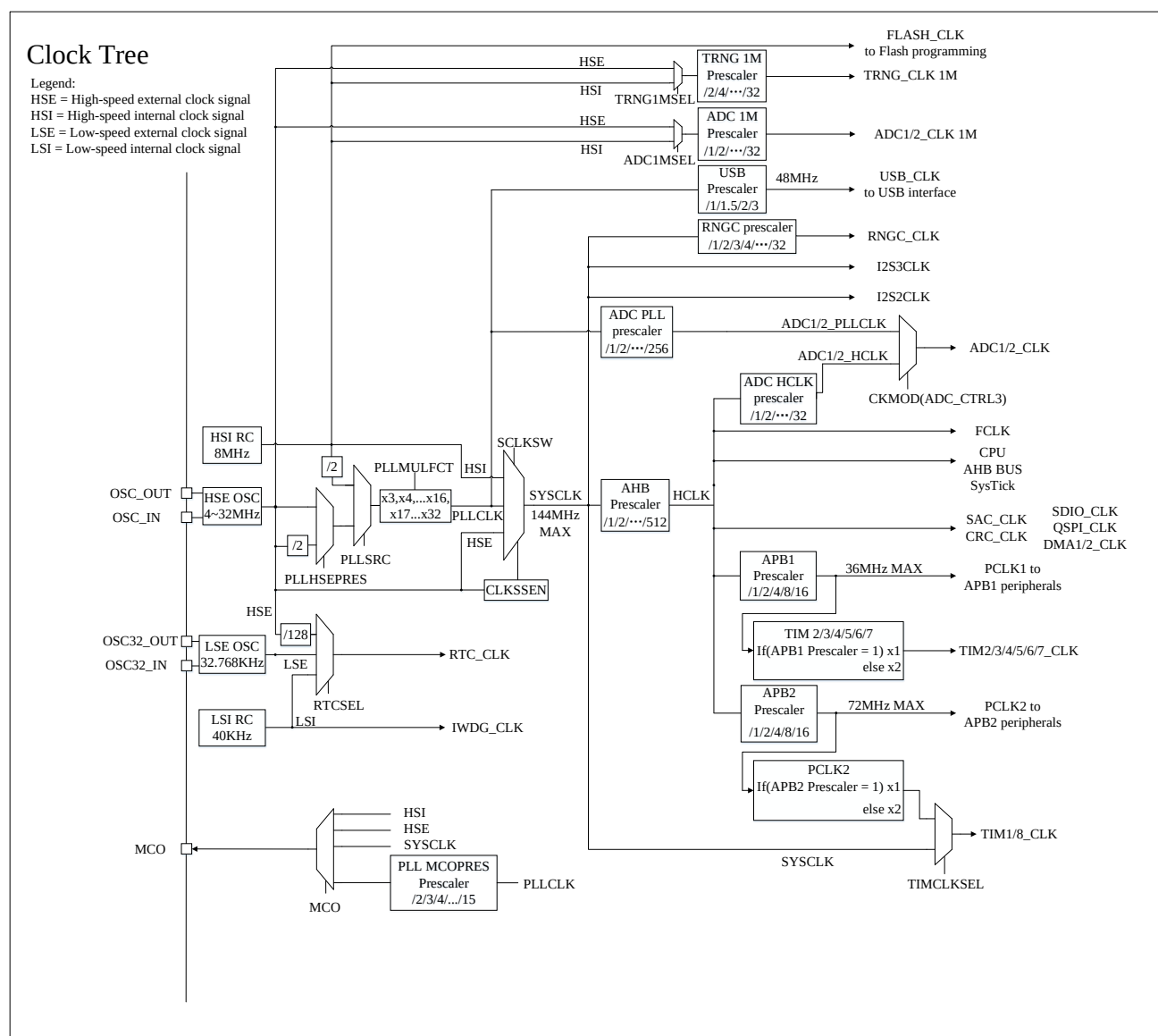
Figure 5-2 Clock Tree
