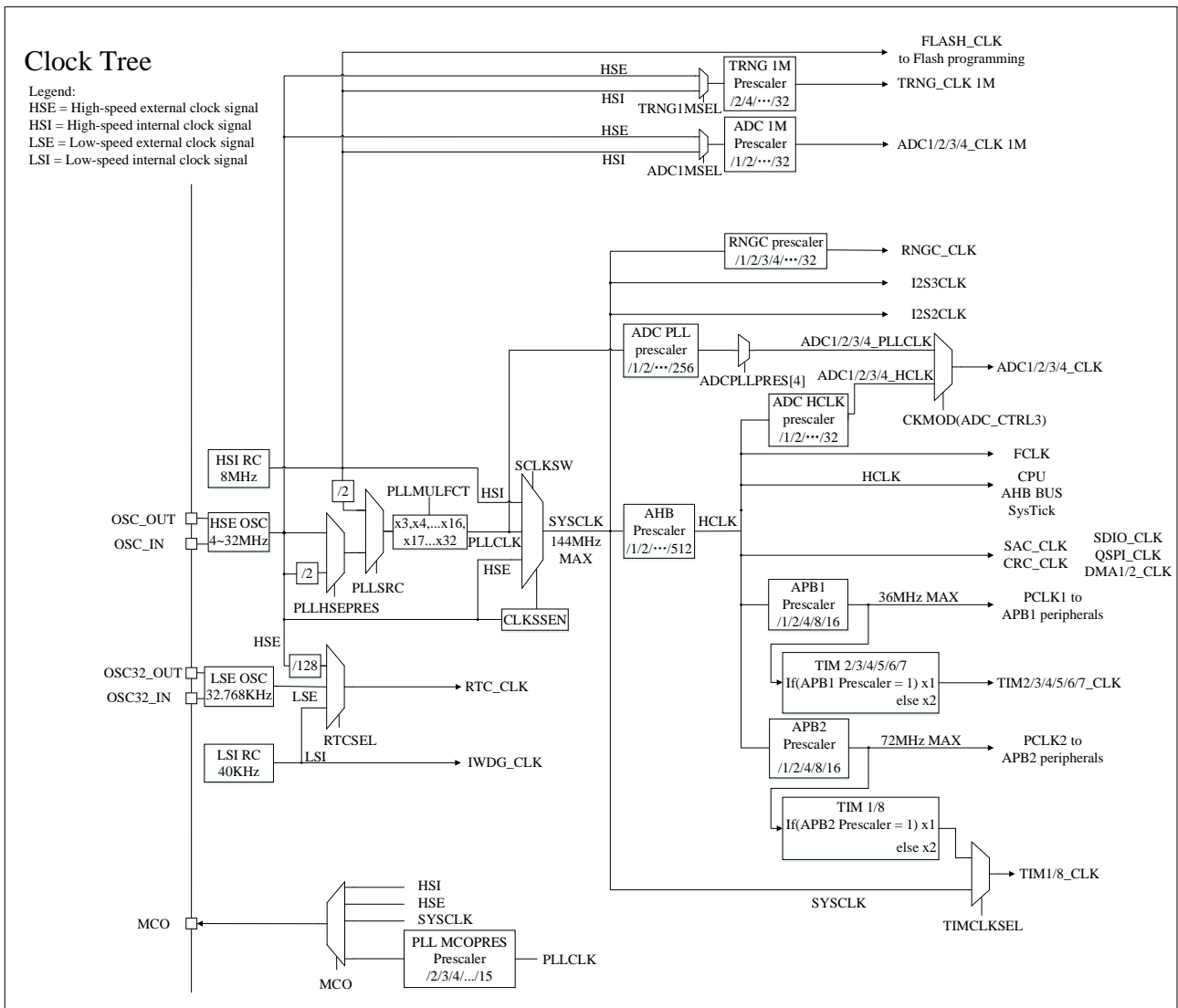
Figure 2-2 Clock tree
