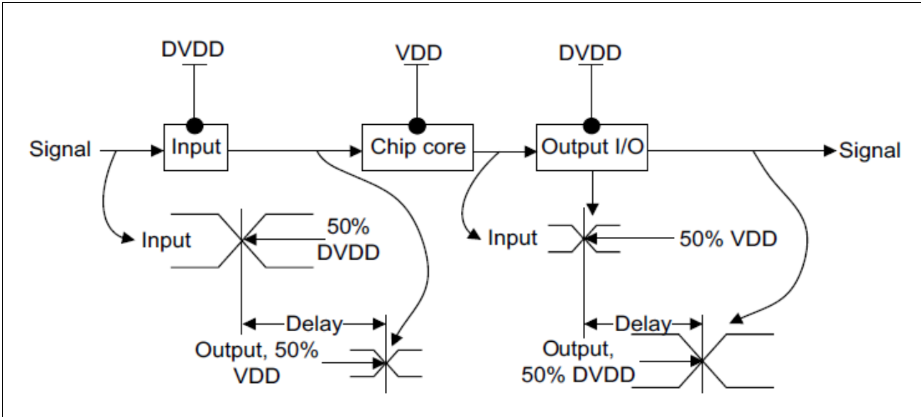
Figure 4-10 Transmission delay
