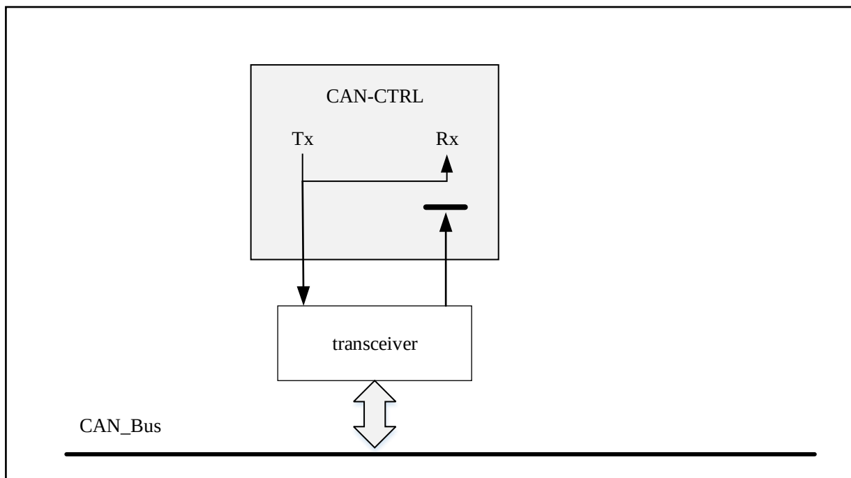
Figure 19-4 loopback mode
