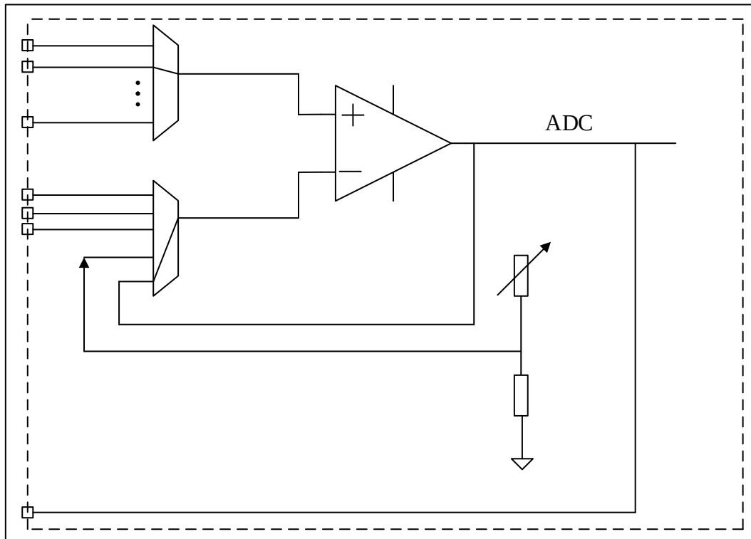
Figure 25-6 Follow mode
