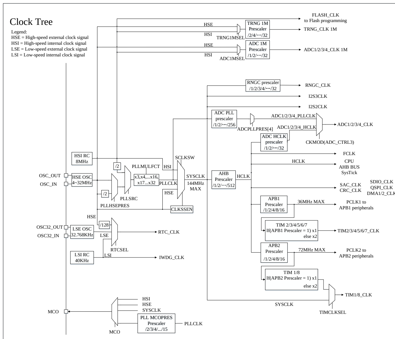
Figure 6-2 Clock Tree
