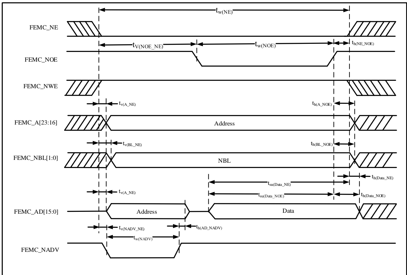
Figure 4-23 Asynchronous Multiplexed PSRAM /NOR Read Waveforms
