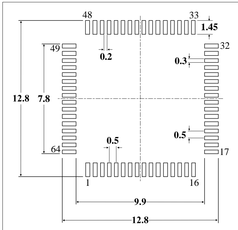
Figure 5-8 LQFN64 Recommended Footprint (1)
