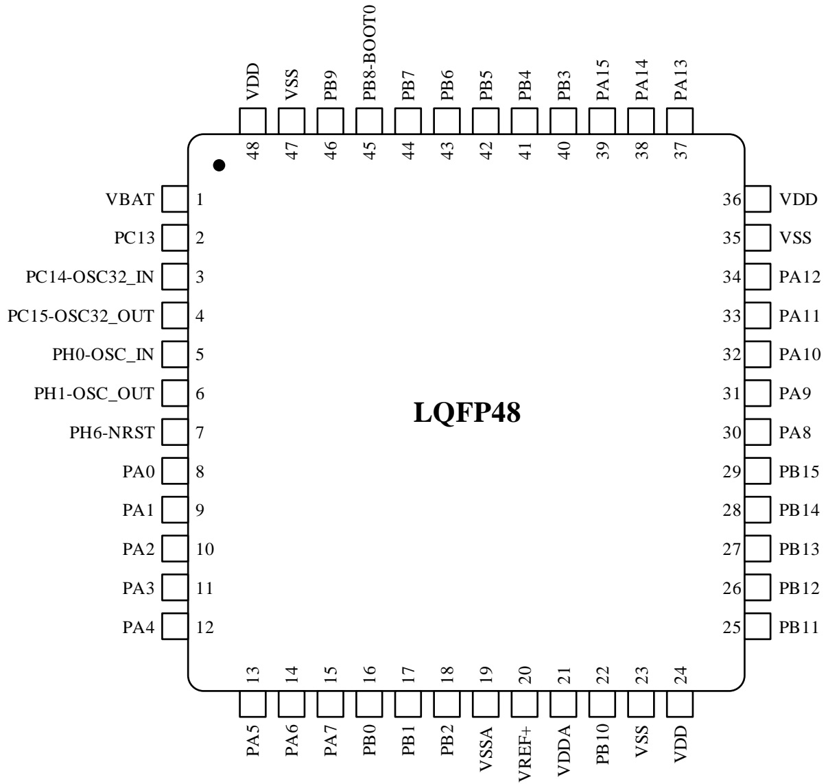
Figure 3-3 LQFP48 Pinout
