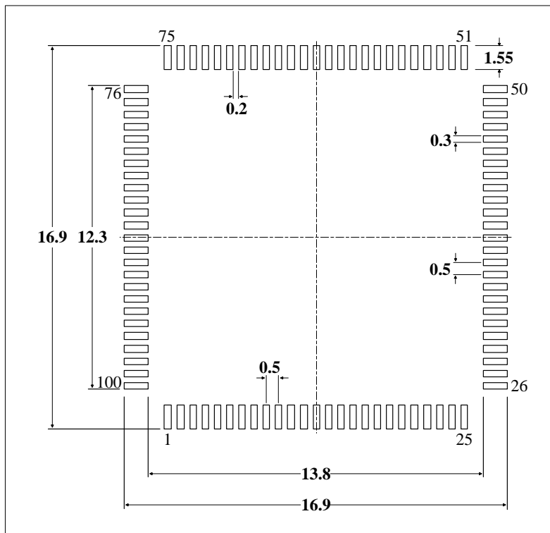
Figure 5-12 LQFN100 Recommended Footprint (1)
