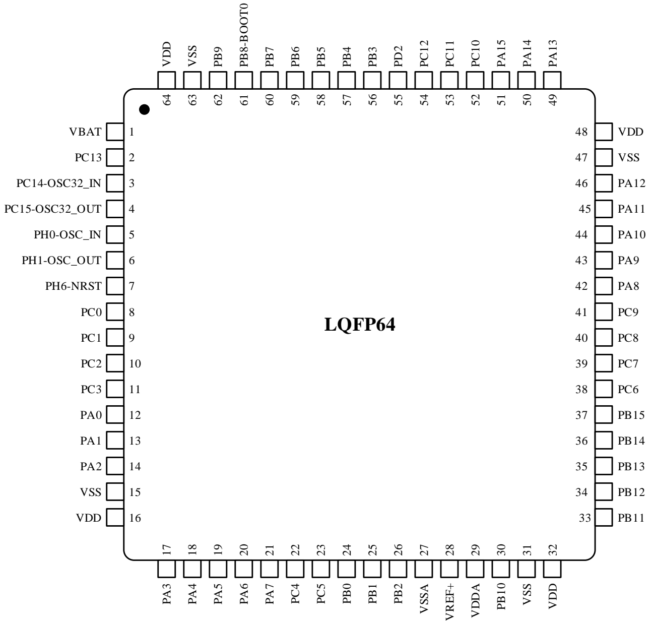
Figure 3-4 LQFP64 Pinout
