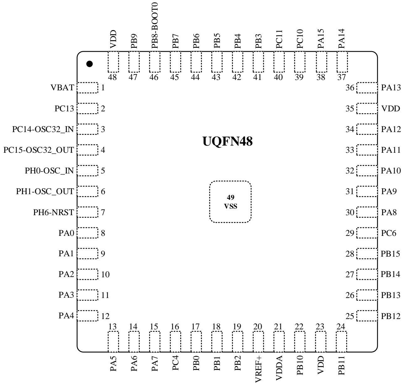
Figure 3-2 UQFN48 Pinout
