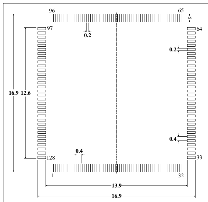
Figure 5-14 LQFN128 Recommended Footprint (1)
