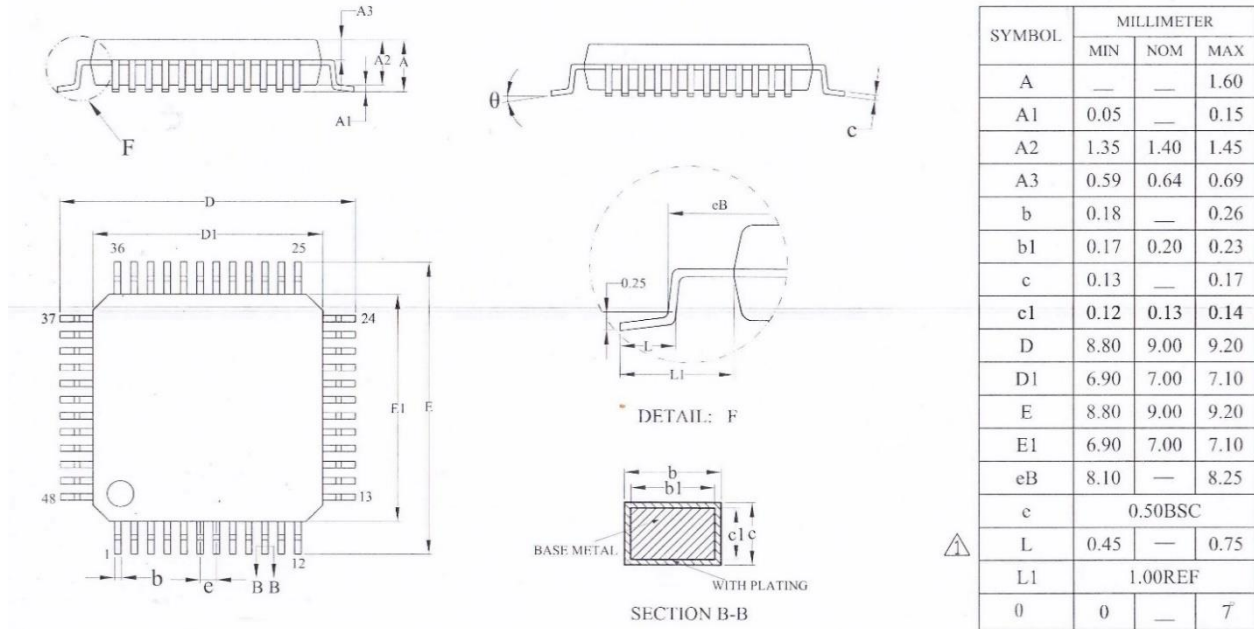
Figure 5-5 LQFP48 Package Dimensions
