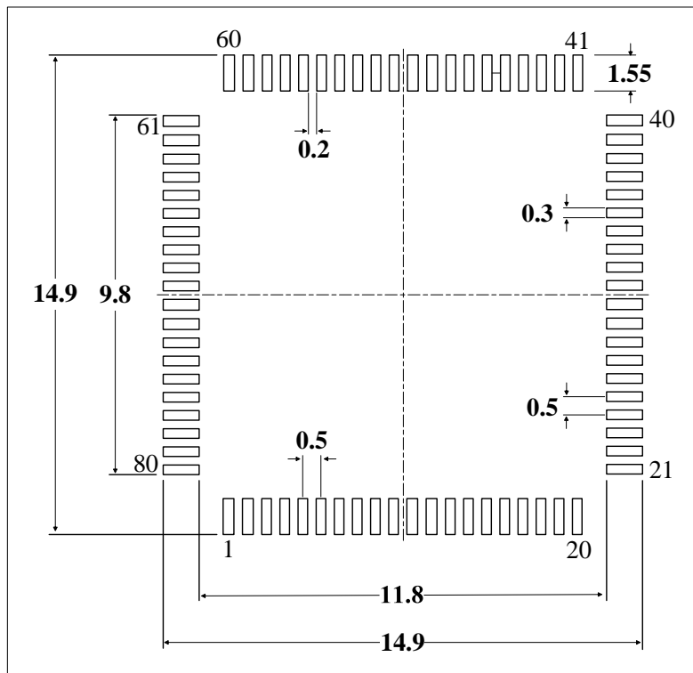
Figure 5-10 LQFN80 Recommended Footprint (1)
