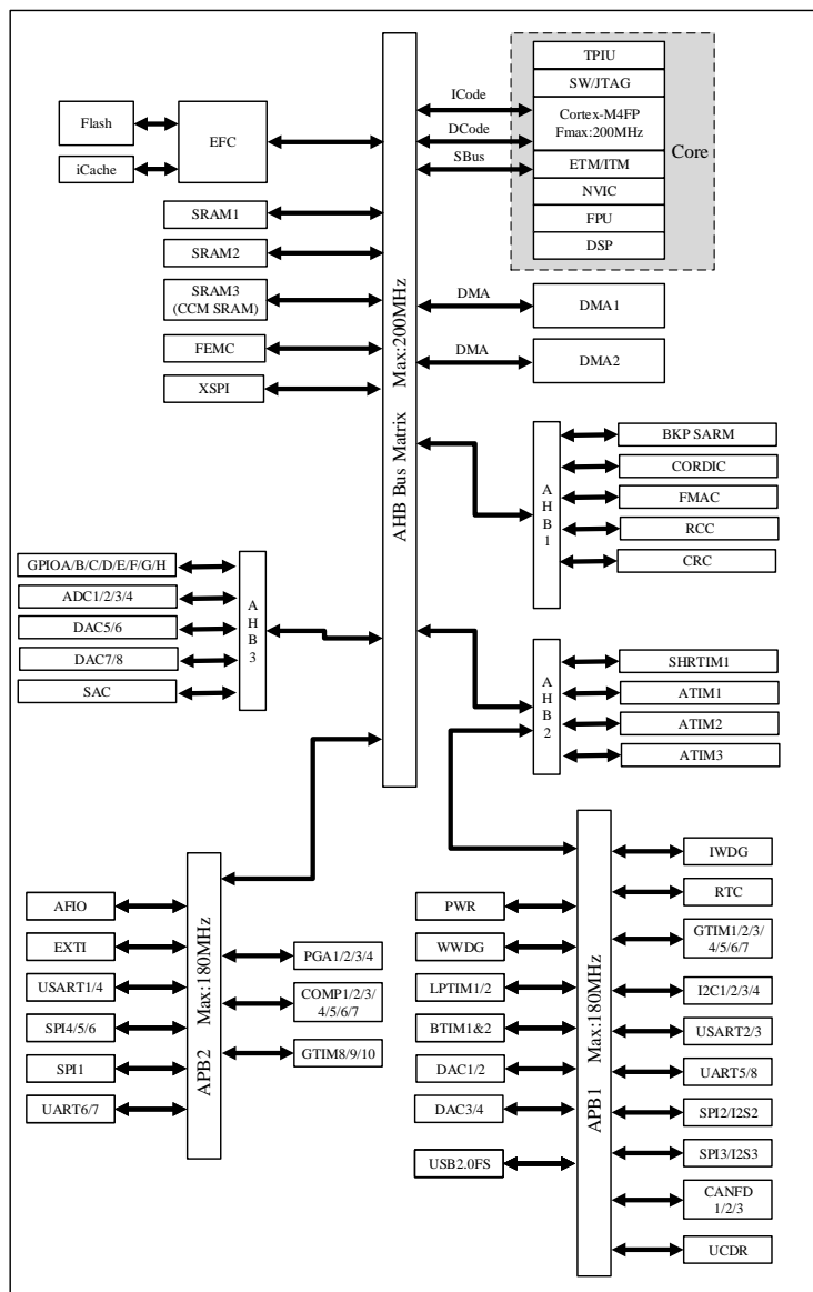
Figure 1-1 N32H474 Series Block Diagram
