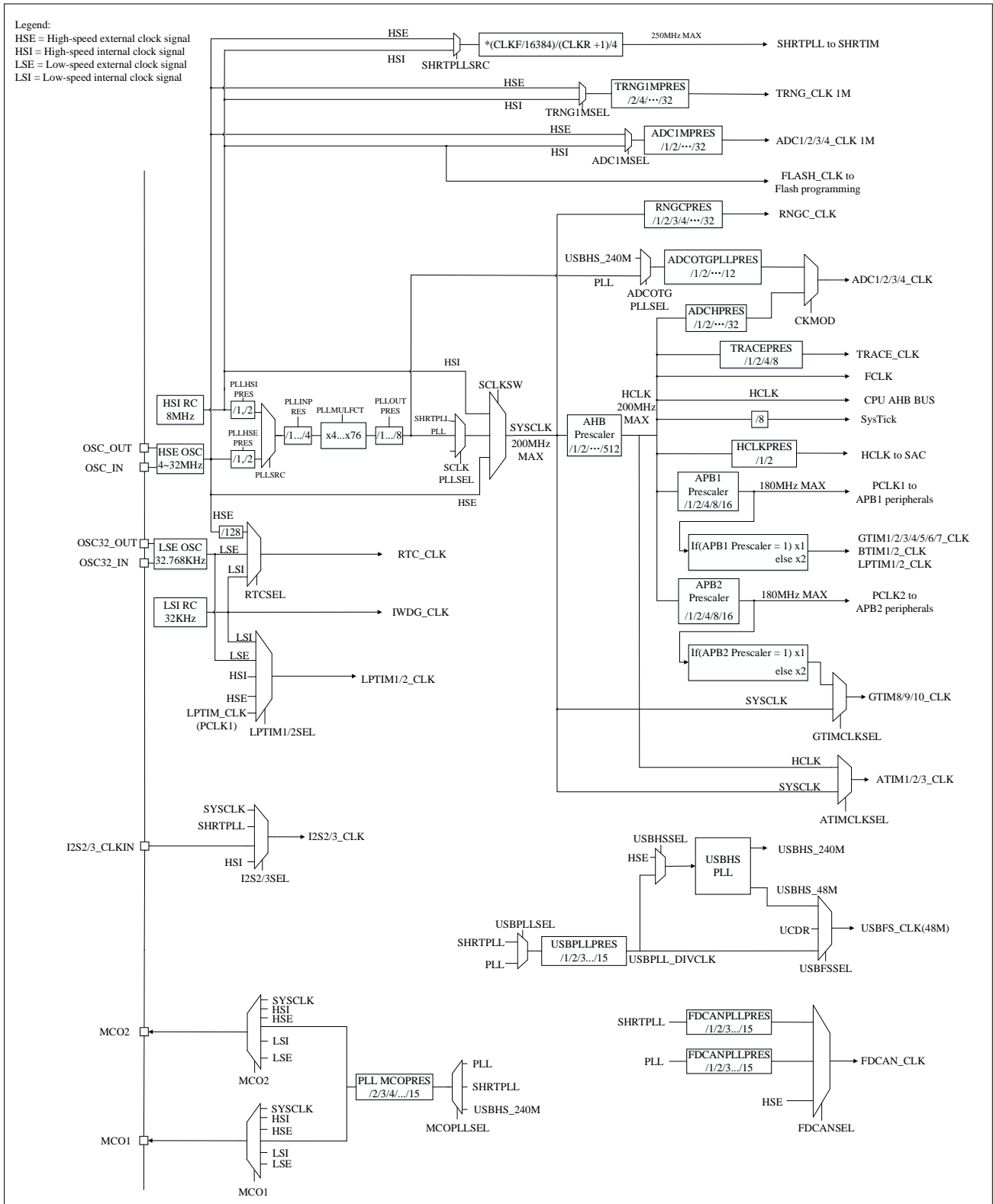
Figure 2-2 Clock Tree
