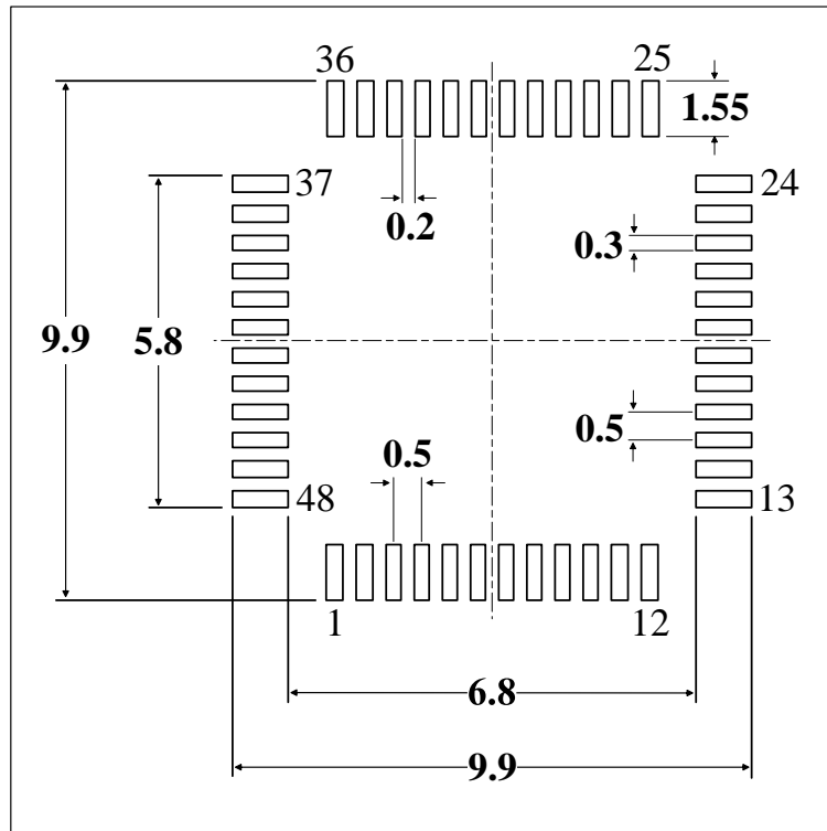
Figure 5-6 LQFN48 Recommended Footprint (1)
