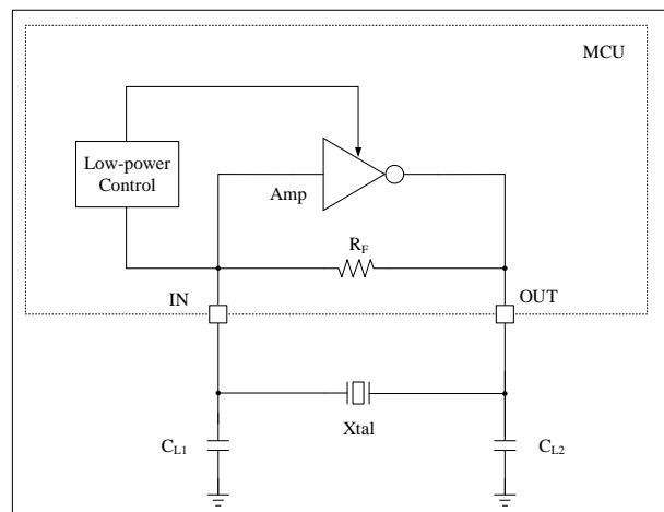
Figure 4-8 Typical Application Of 32.768KHz Crystal
