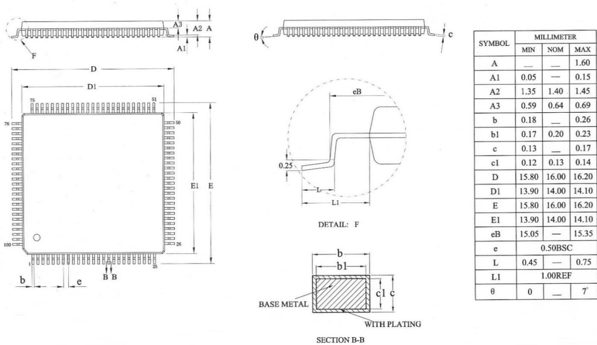
Figure 5-11 LQFP100 Package Dimensions
