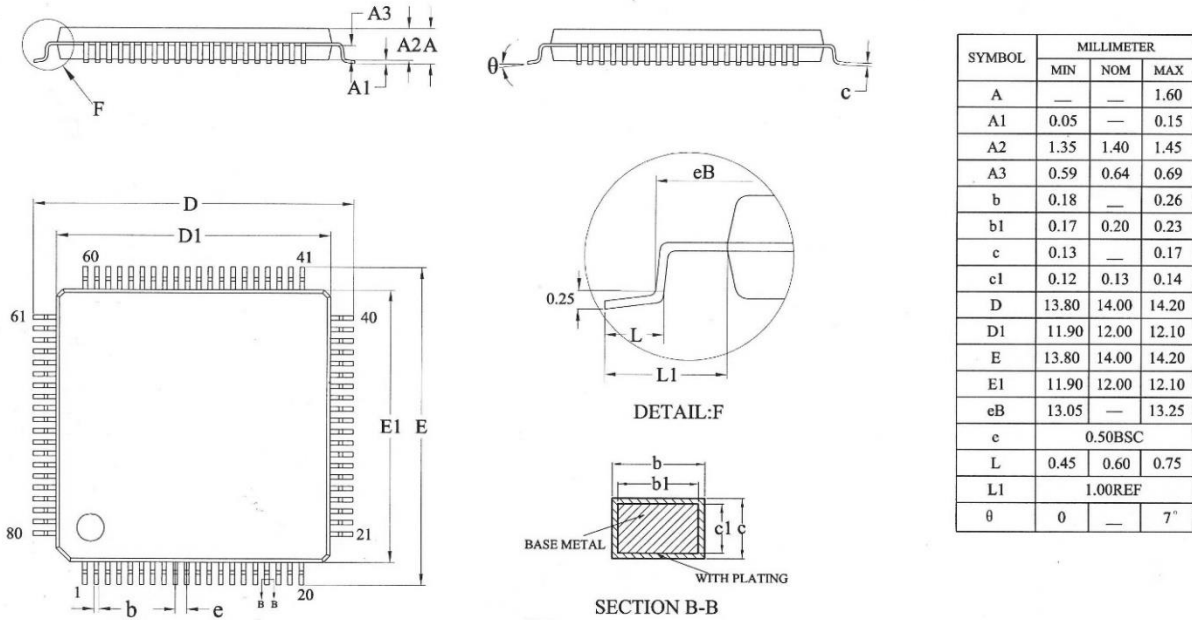
Figure 5-9 LQFP80 Package Dimensions
