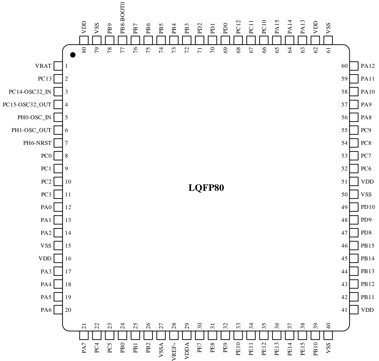
Figure 3-5 LQFP80 Pinout
