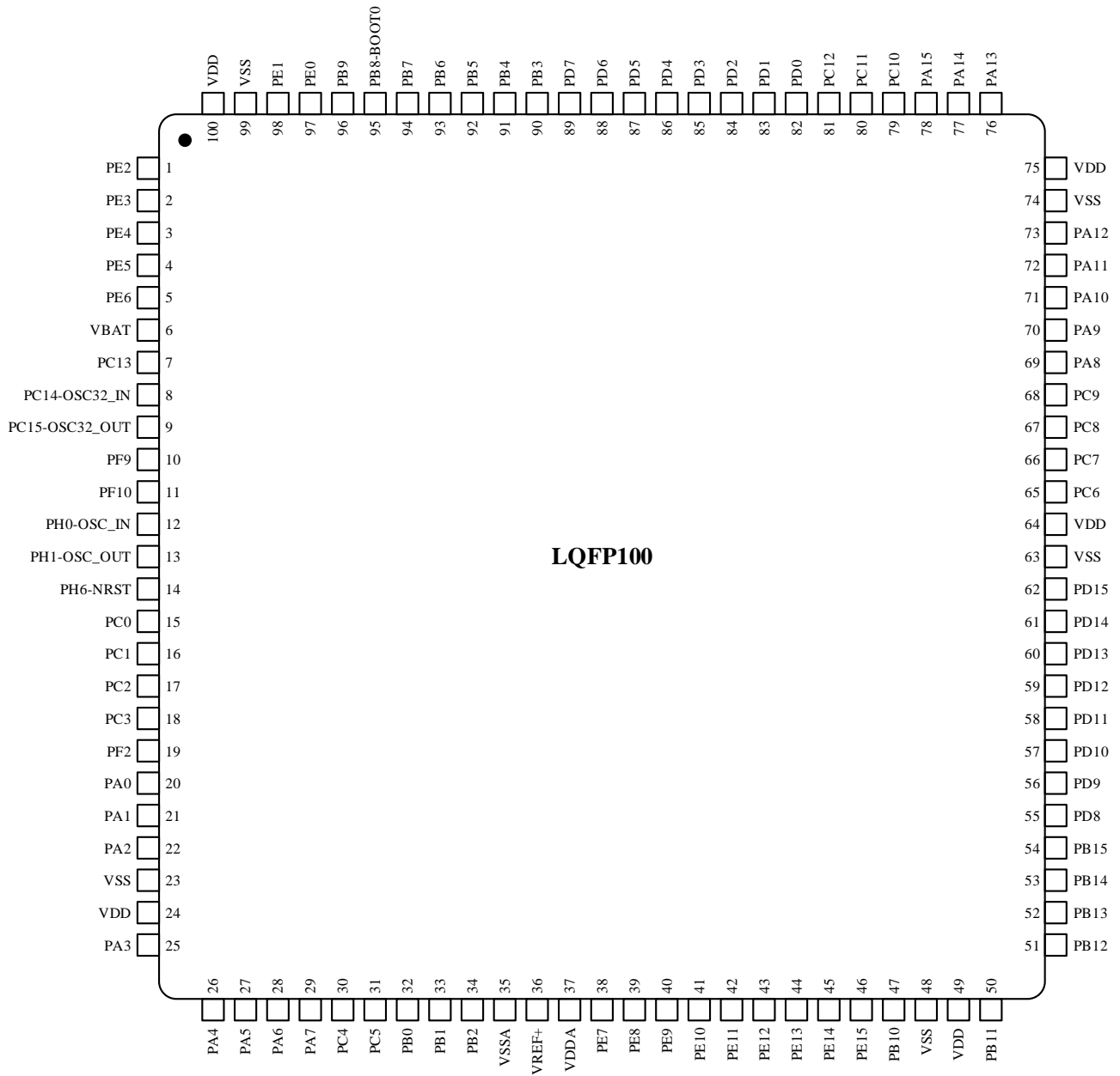
Figure 3-6 LQFP100 Pinout
