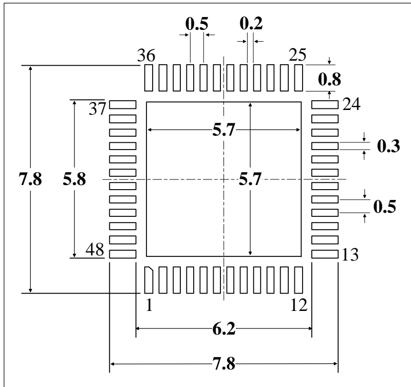
Figure 5-4 UQFN48 Recommended Footprint (1)
