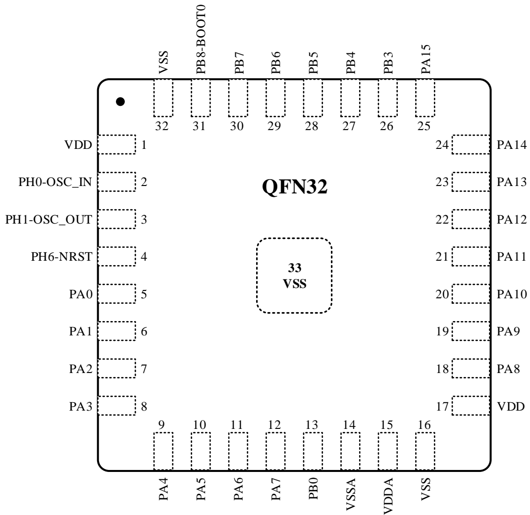
Figure 3-1 QFN32 Pinout
