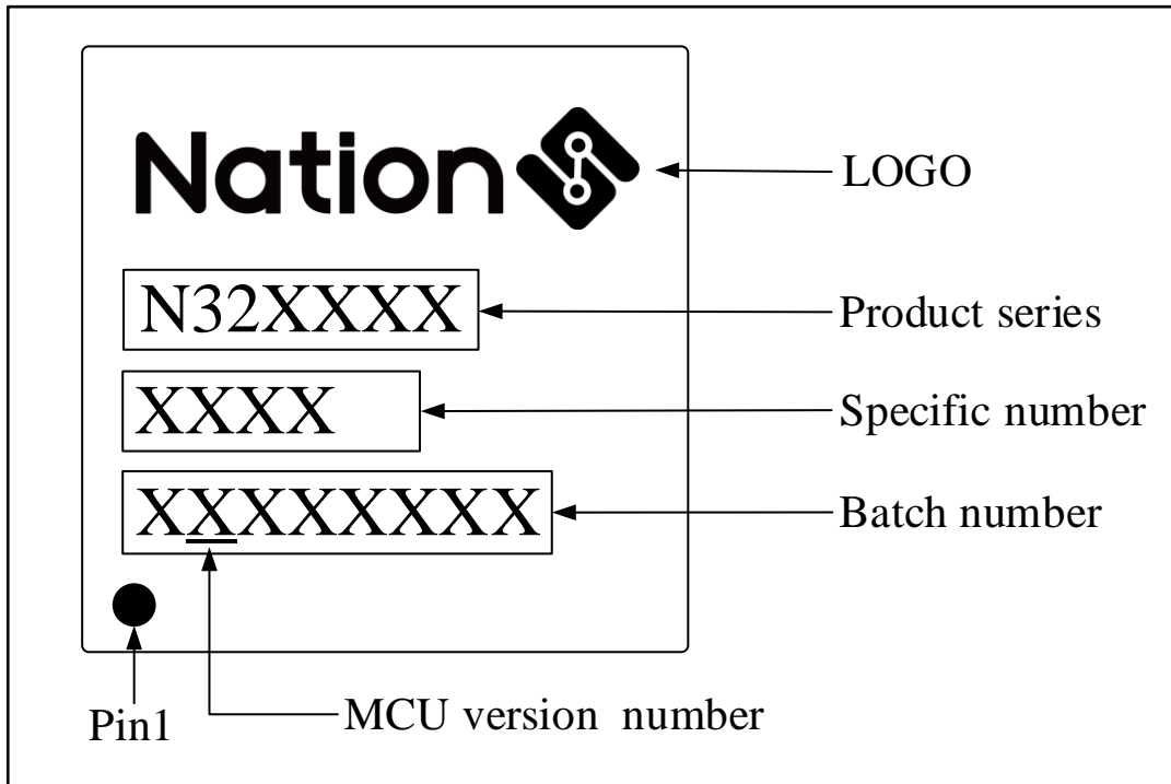
Figure 6-1 Marking Information
