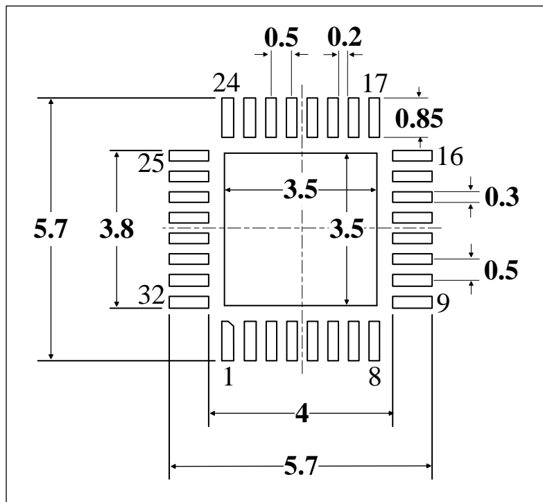
Figure 5-2 QFN32 Recommended Footprint (1)
