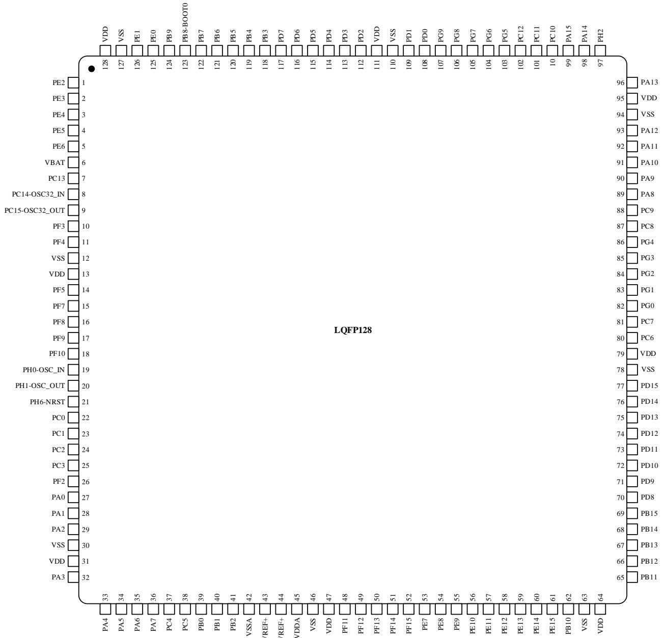
Figure 3-7 LQFP128 Pinout
