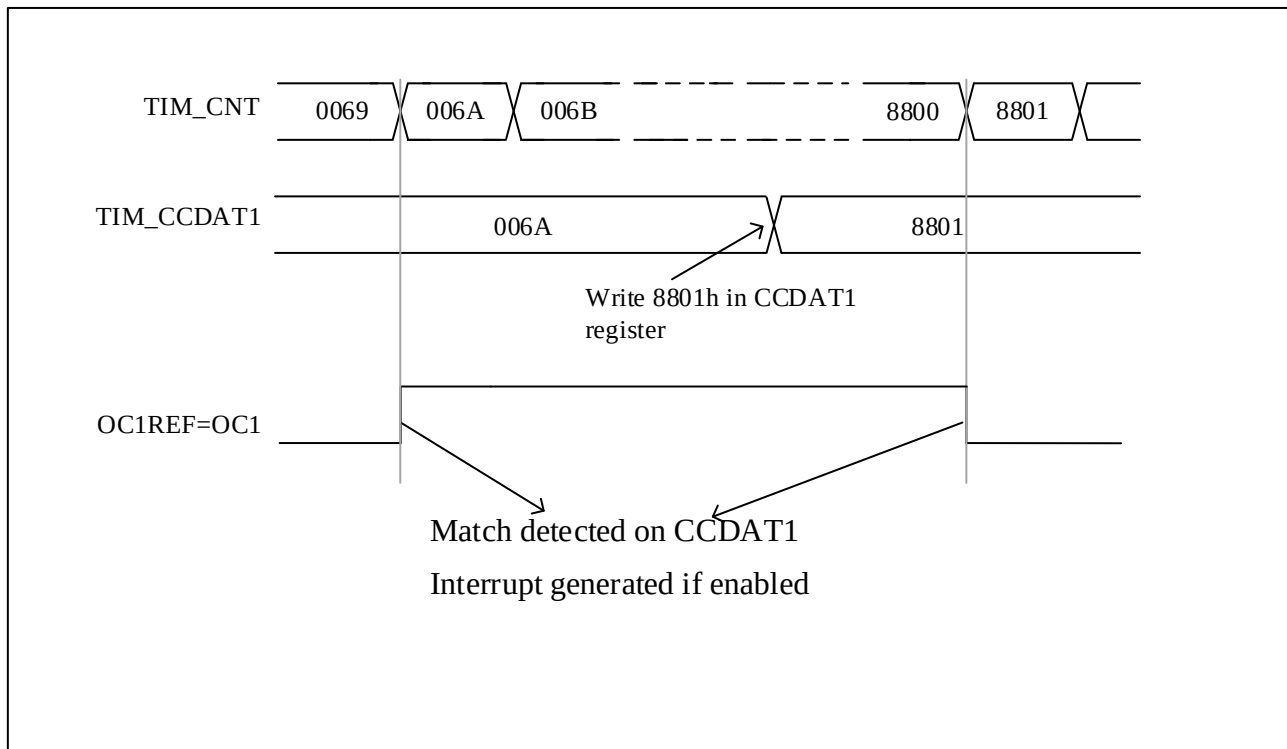
Figure 14-18 Output Compare Mode, Toggle on OC1
