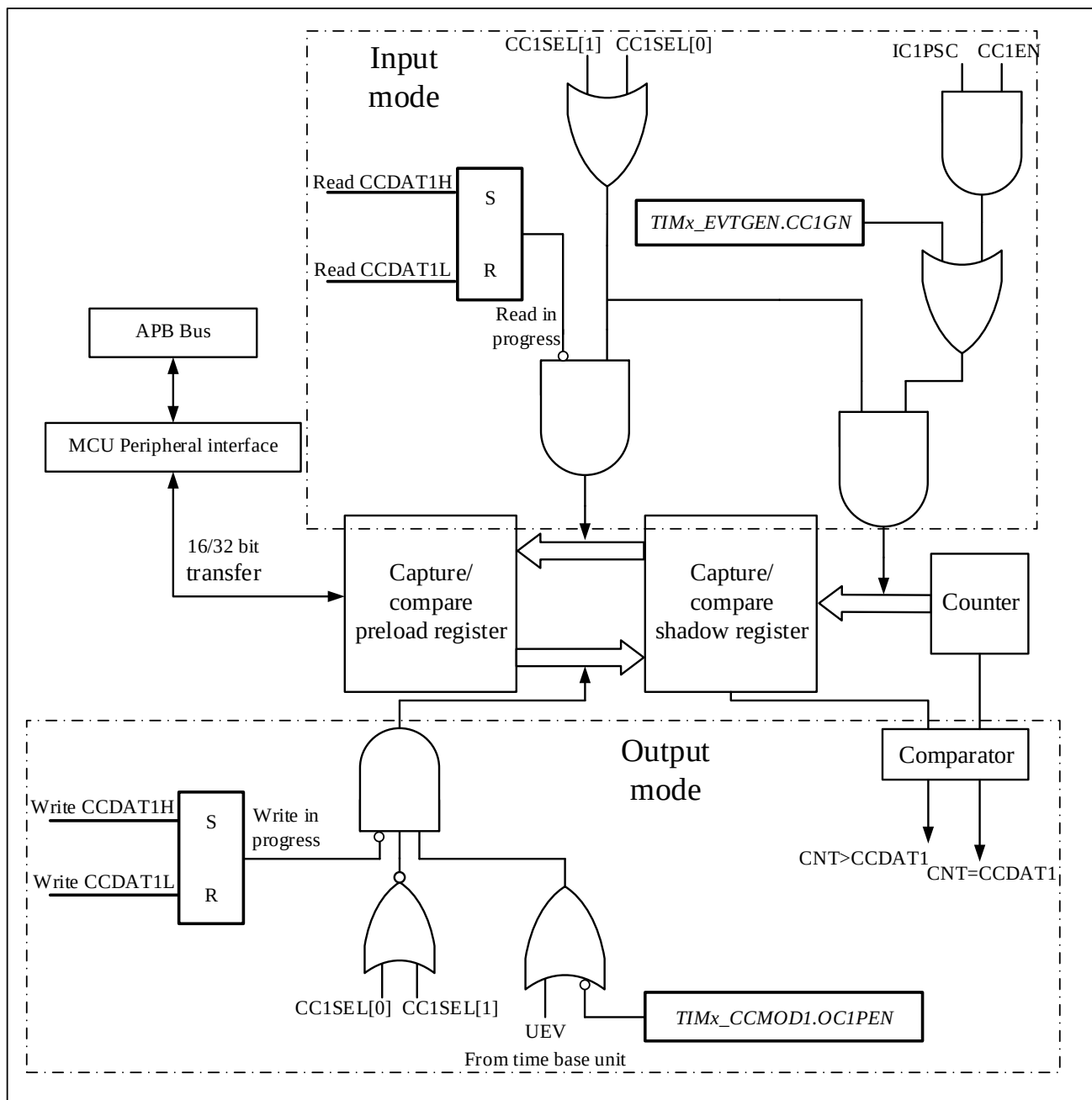
Figure 12-18 Capture/Compare Channel 1 Main Circuit
