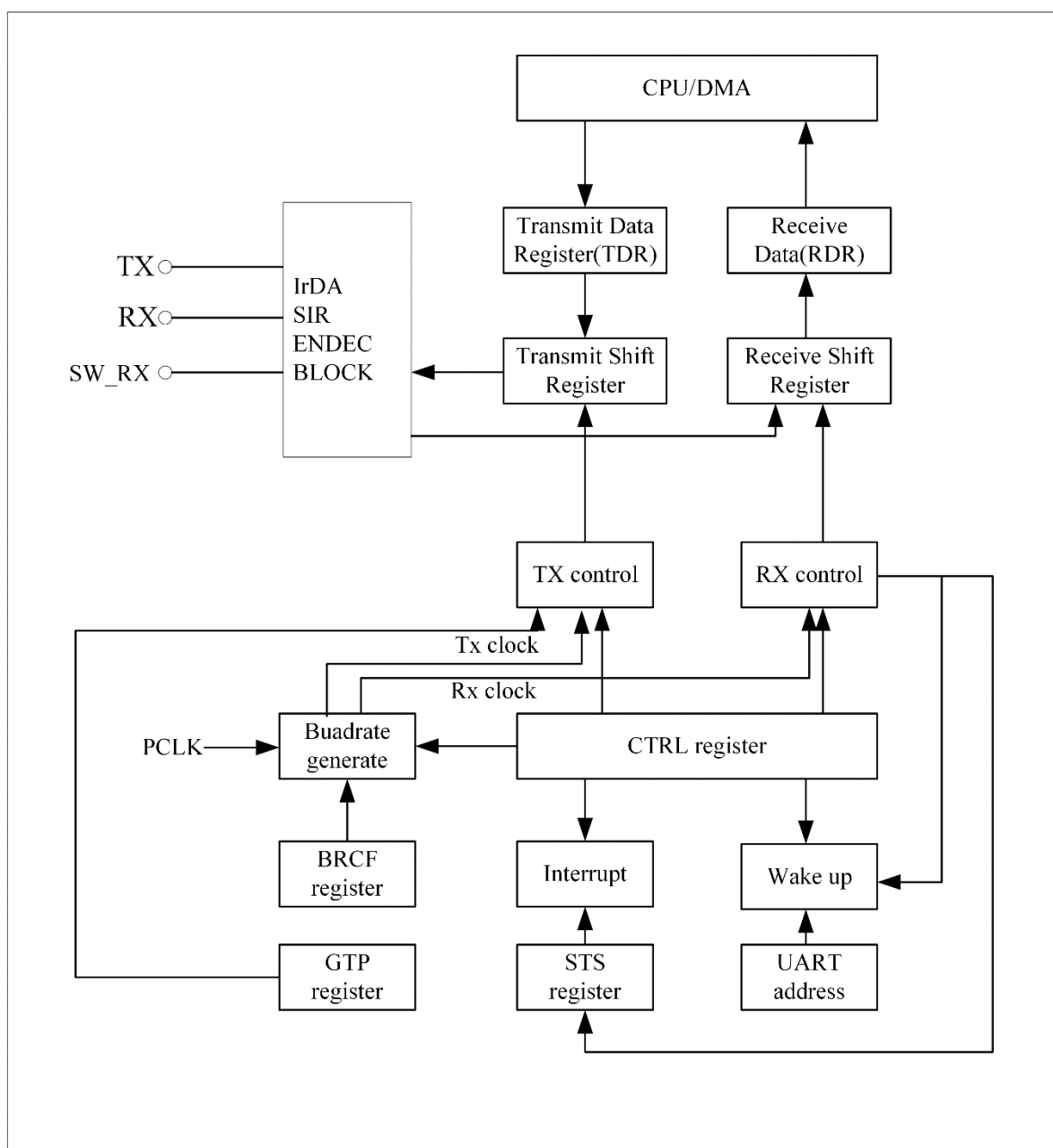
Figure 9-1 UART Block Diagram
