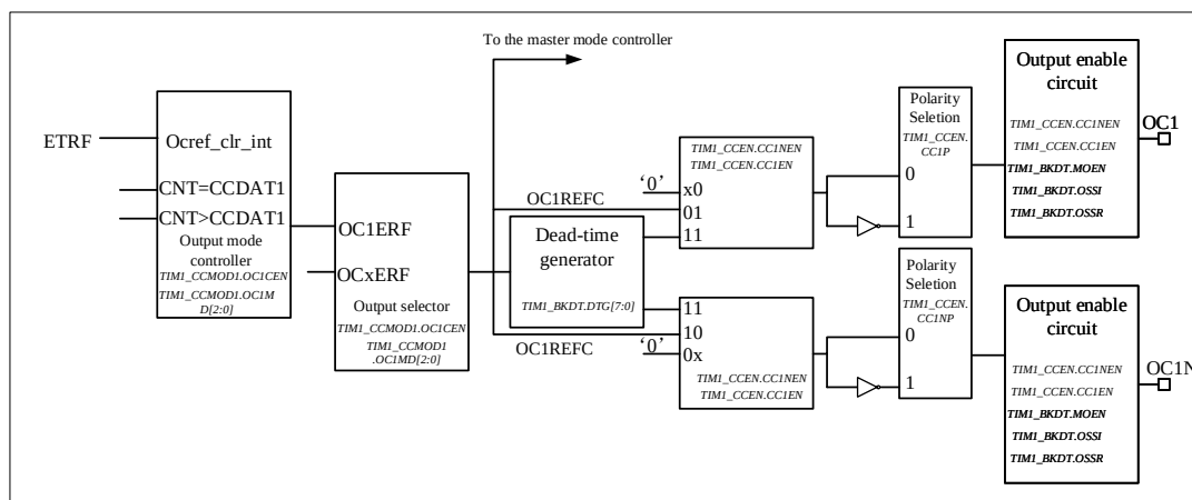
Figure 12-19 Output Part of Channelx (Take Channel 1 as Example)
