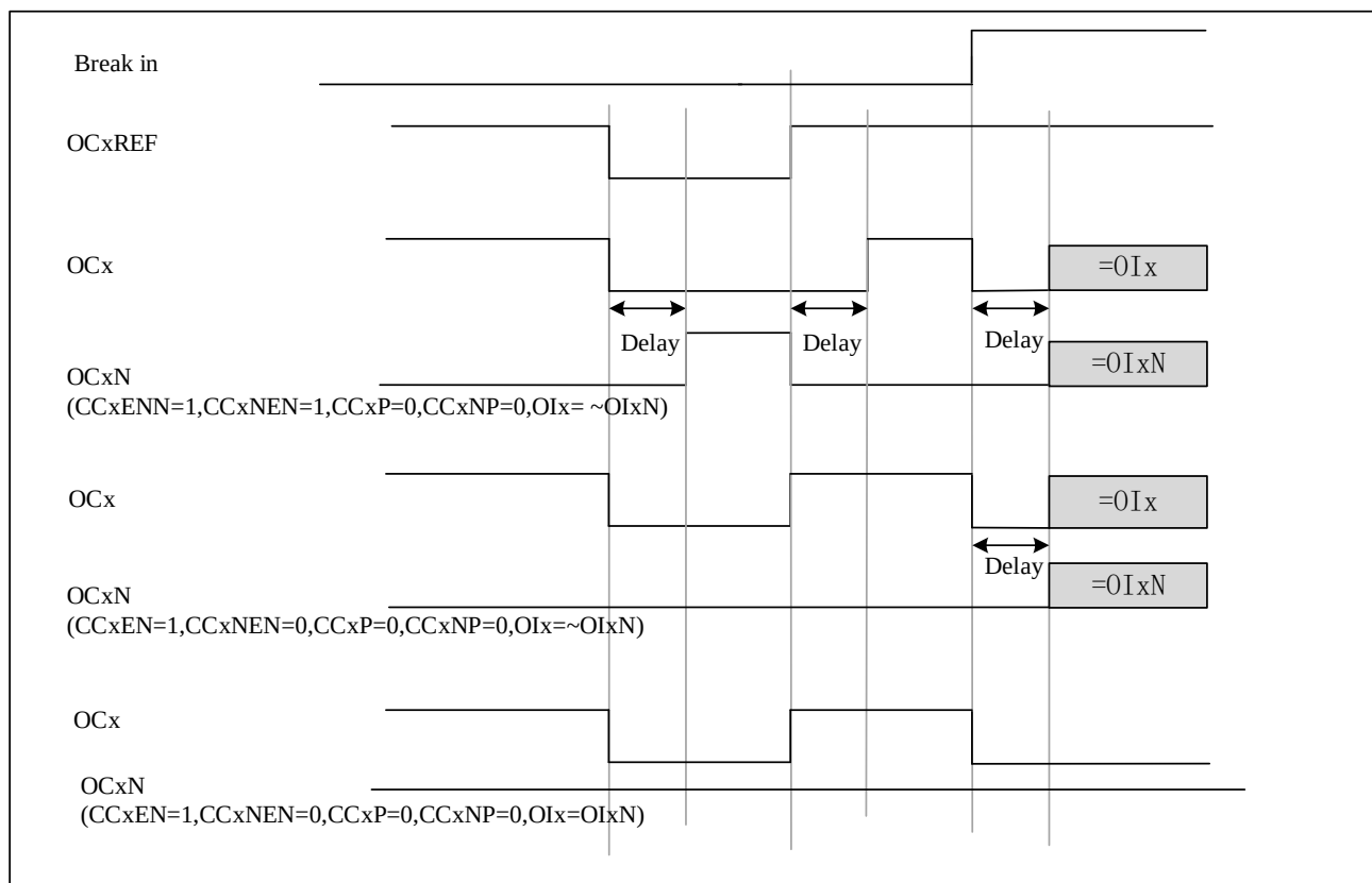
Figure 12-28 Output Behavior in Response to a Break
