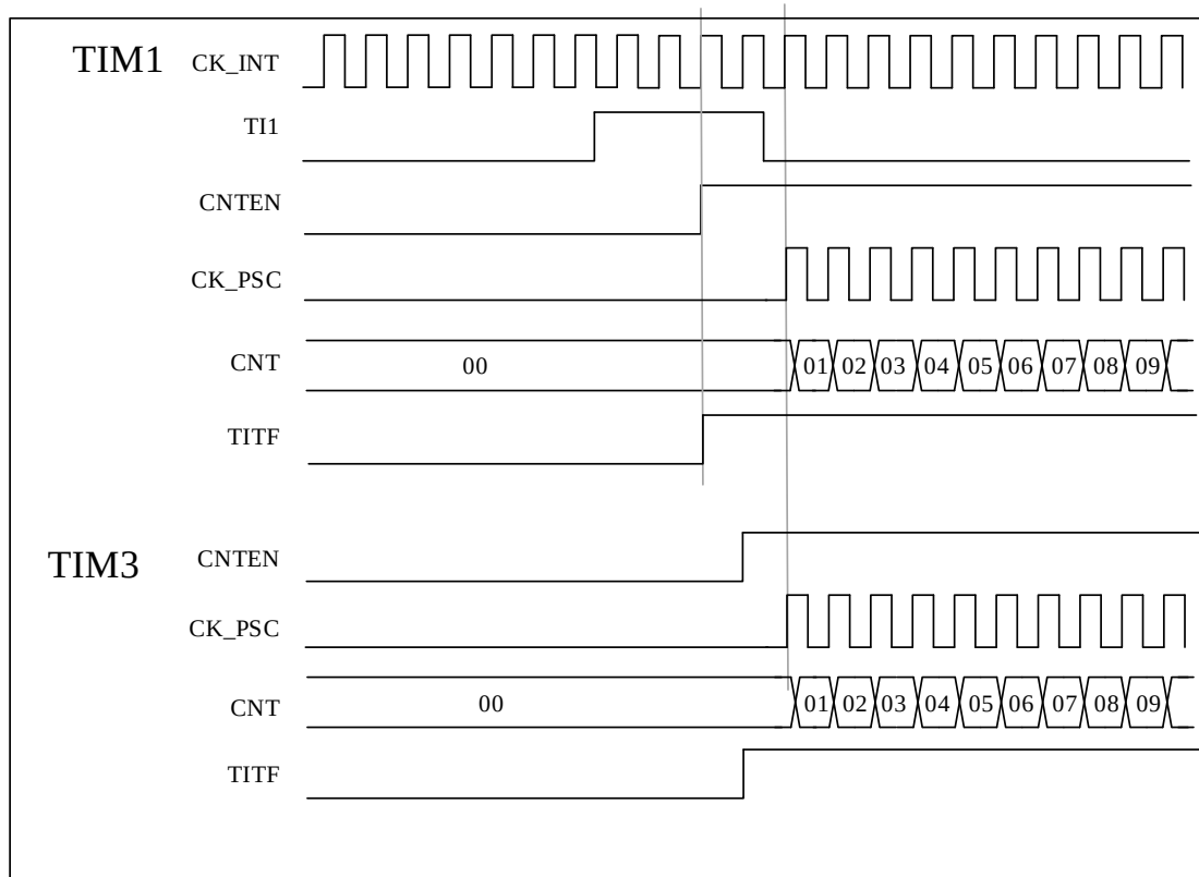
Figure 13-29 Triggers TIM1 and TIM3 Using the TI1 Input of TIM1
