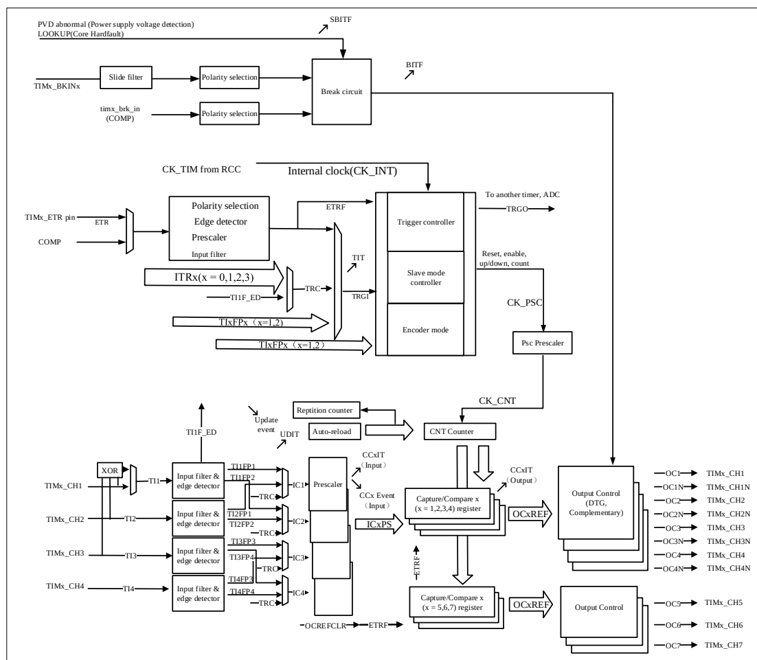
Figure 12-1 Block Diagram of TIM1
