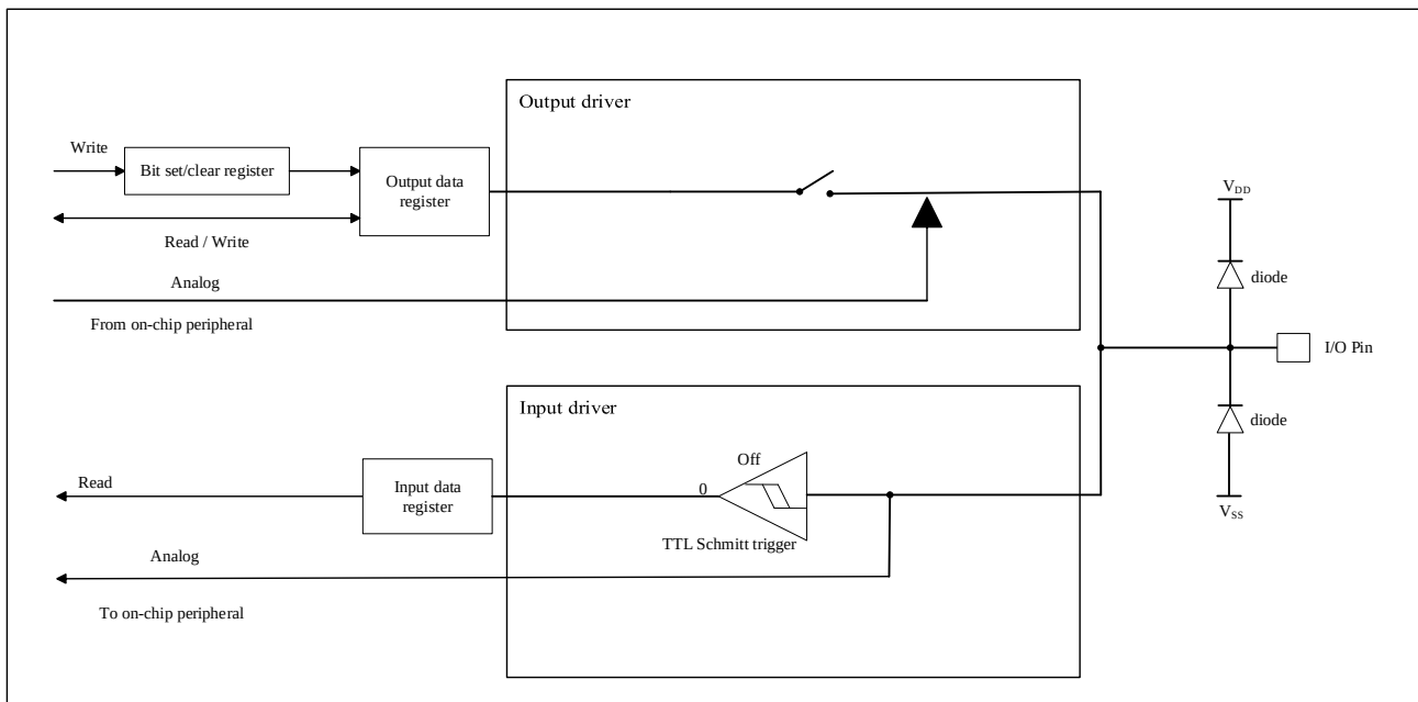
Figure 6-5 High-impedance Analog Function Mode (Fail-safe Not Supported)
