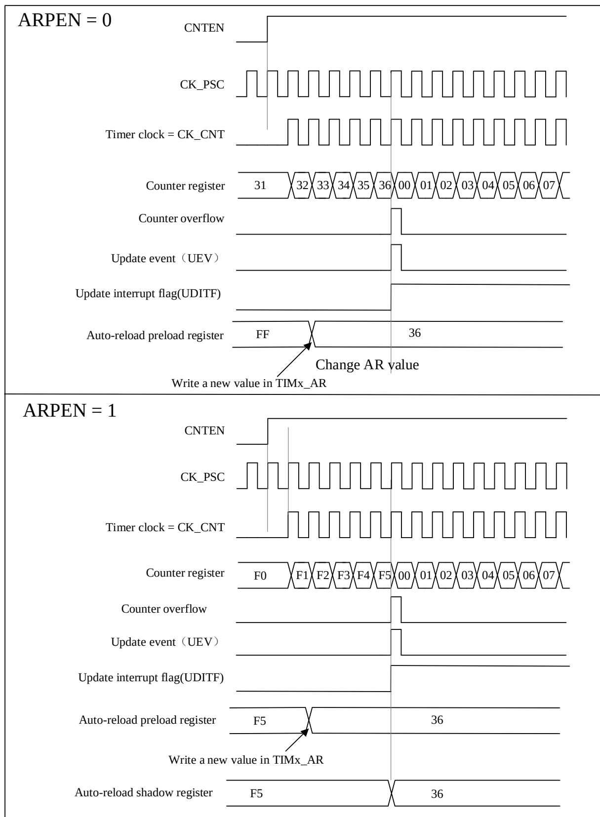
Figure 15-4 Timing diagram of up-counting and update event when ARPEN=0/1
