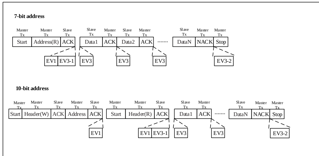
Figure 8-3 Slave Transmitter Transfer Sequence Diagram
