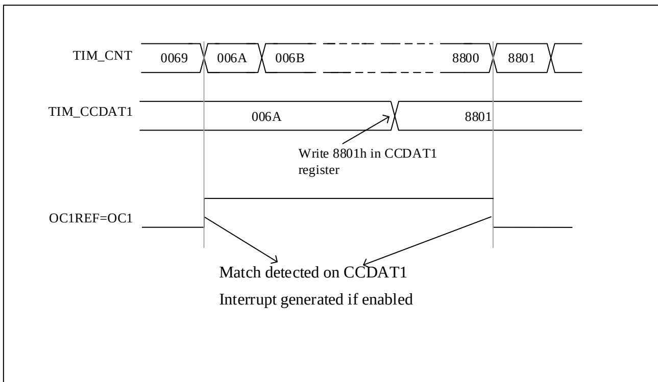
Figure 12-21 Output Compare Mode, Toggle on OC1
