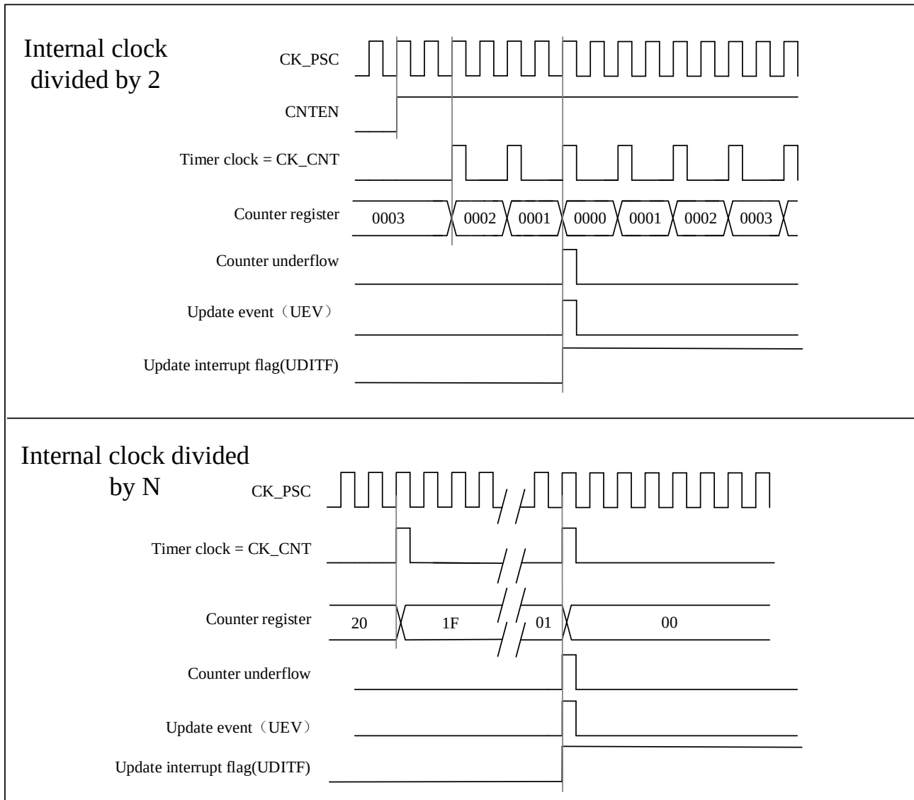
Figure 14-6 Timing Diagram of the Center-aligned, Internal Clock Divided Factor = 2/N
