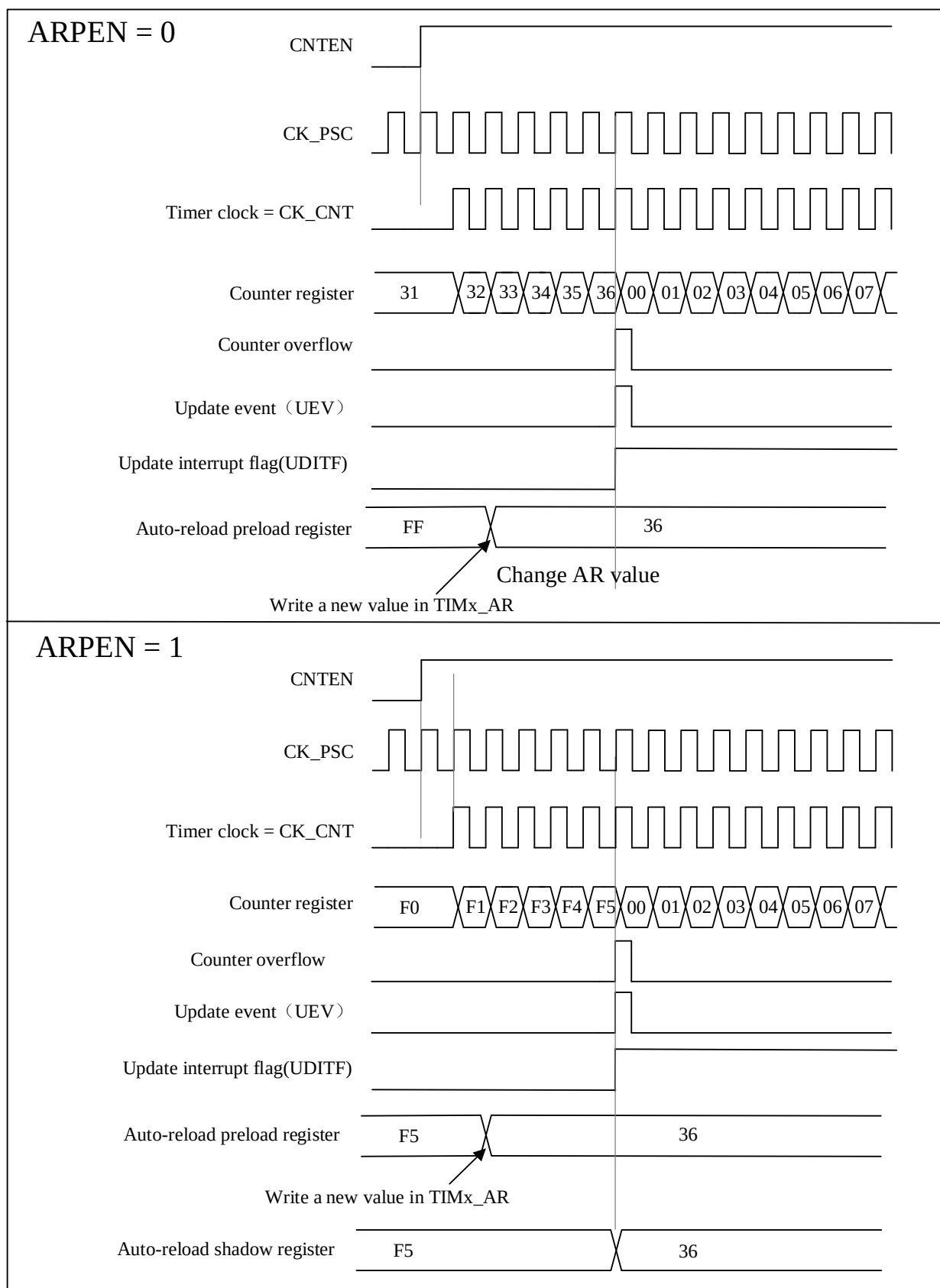
Figure 13-4 Timing Diagram of The Up-counting, Update Event When ARPEN = 0/1
