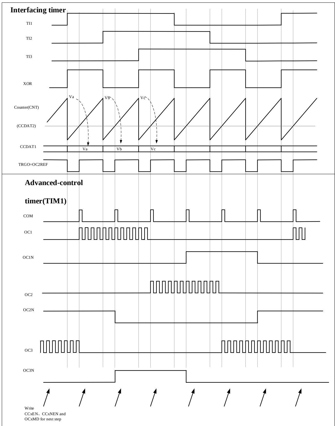
Figure 12-39 Example of Hall Sensor Interface
