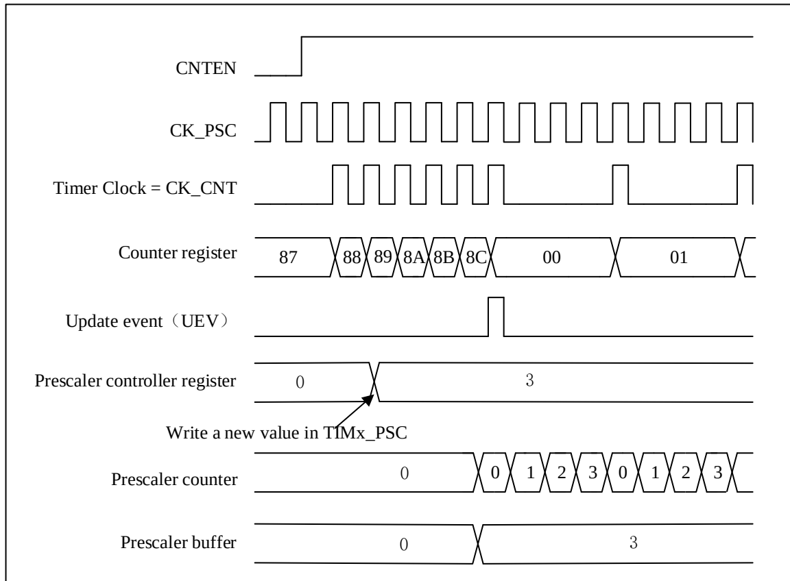
Figure 15-2 Counter Timing Diagram With Prescaler Division Change From 1 To 4
