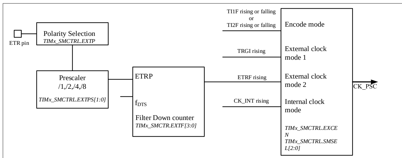
Figure 12-15 External Trigger Input Block Diagram
