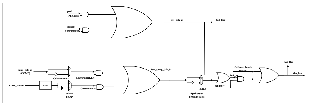
Figure 13-22 Break input
