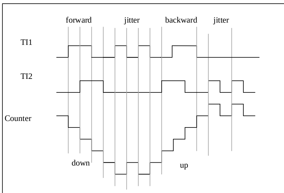
Figure 13-31 Encoder Interface Mode Example with IC1FP1 Polarity Inverted
