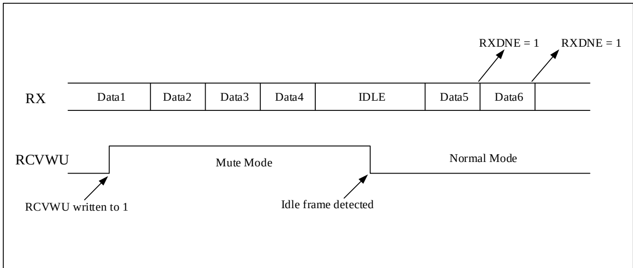
Figure 9-10 Mute Mode Using Idle Line Detection
