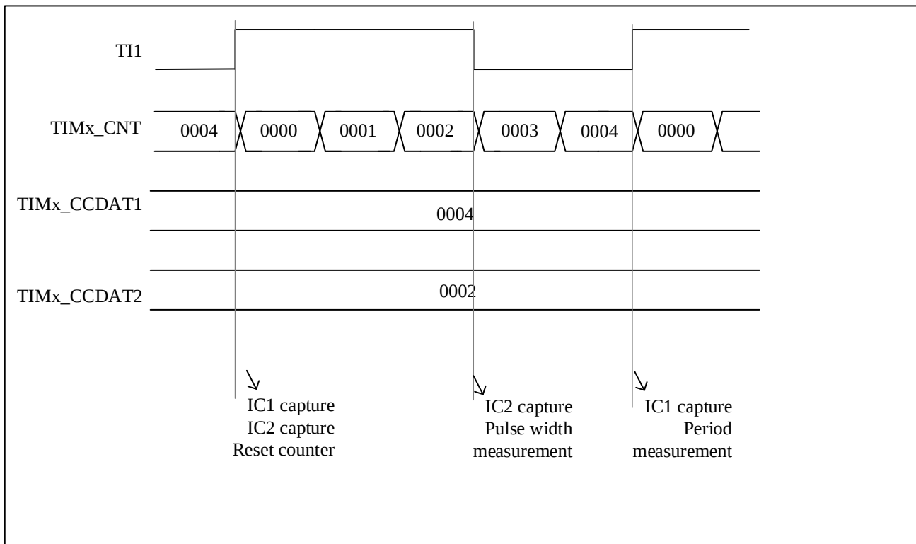
Figure 12-20 PWM Input Mode Timing
