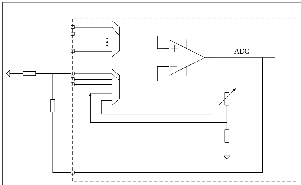
Figure 18-2 OPAMP1 External Amplification Mode
