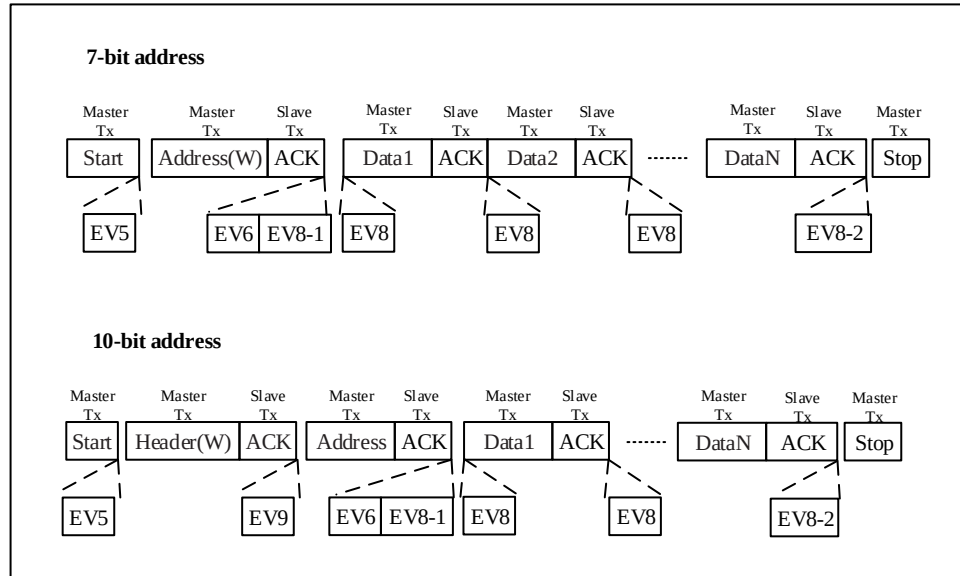
Figure 8-5 Master Transmitter Transfer Sequence Diagram
