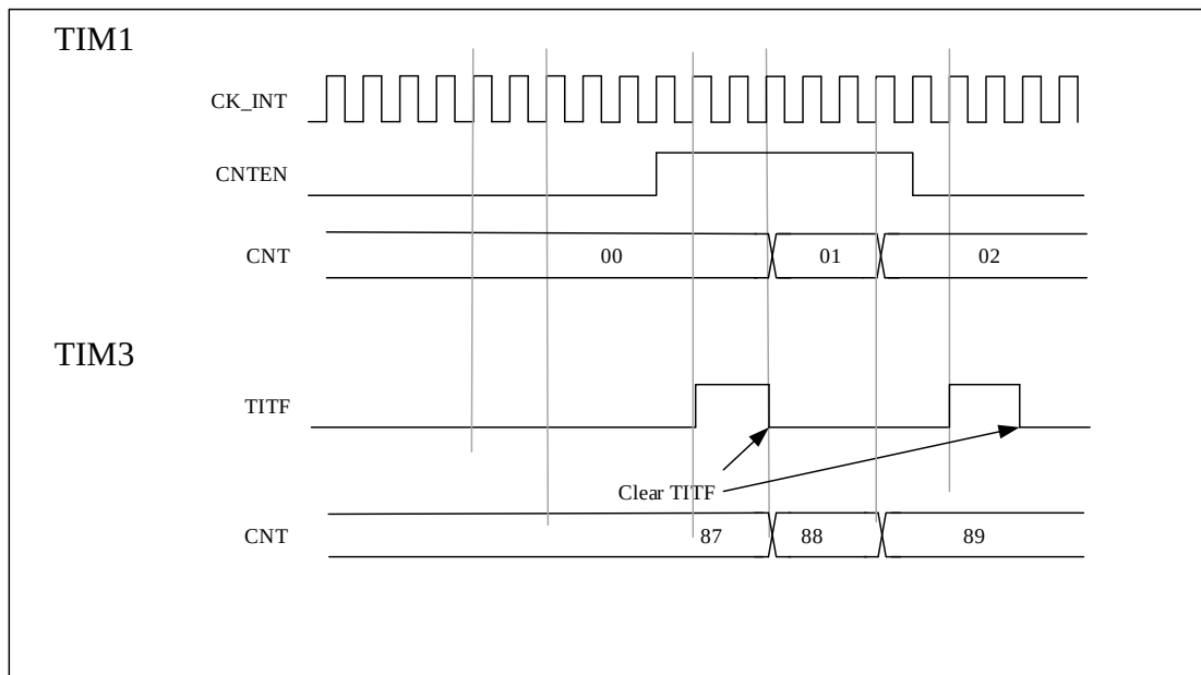
Figure 13-27 TIM3 Gated by Enable Signal of TIM1
