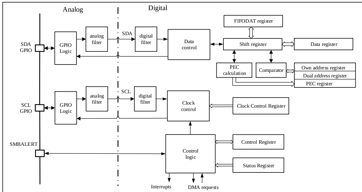
Figure 8-1 I2C Functional Block Diagram
