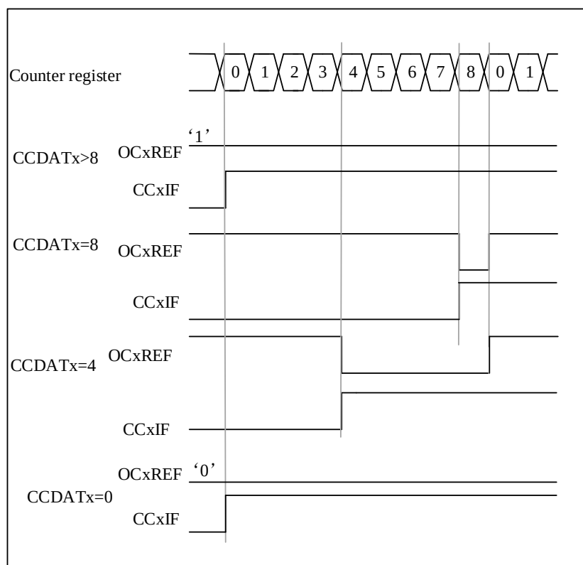
Figure 12-23 Edge-aligned PWM Waveform (APR=8)
