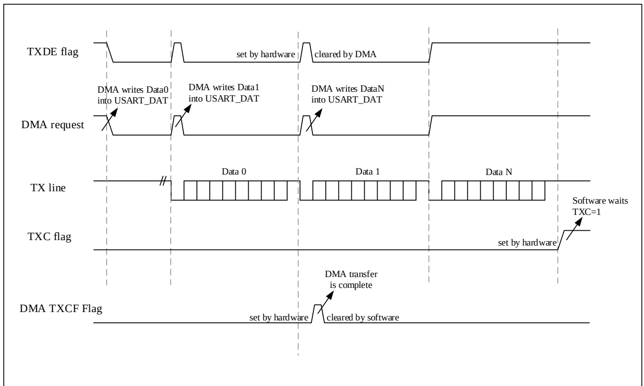
Figure 9-8 Transmission Using DMA
