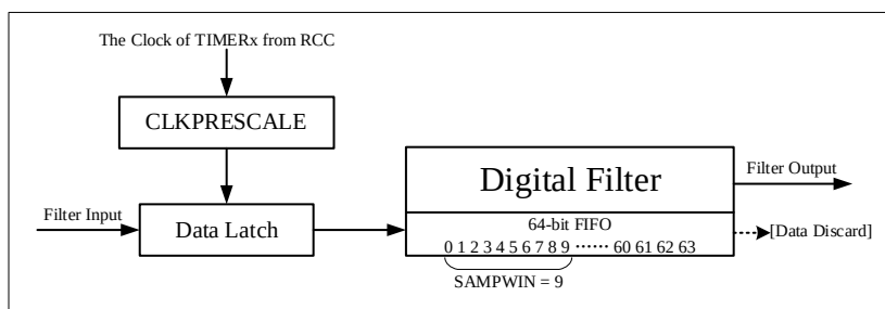
Figure 12-29 Silde Filter
