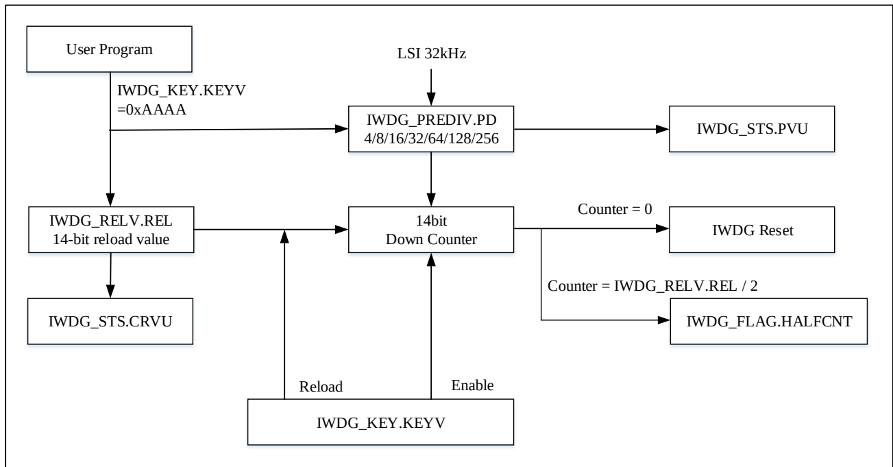
Figure 19-1 Independent Watchdog Functional Block Diagram
