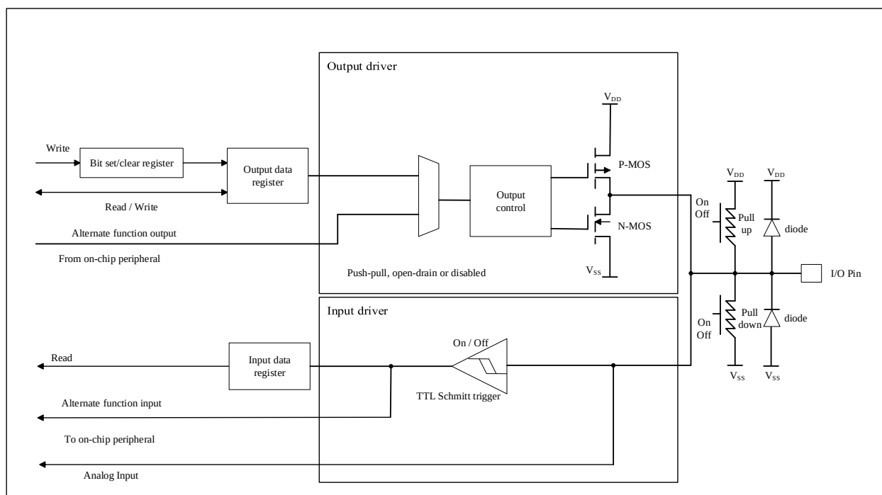
Figure 6-1 Basic Structure of I/O Ports (Fail-safe Not Supported)
