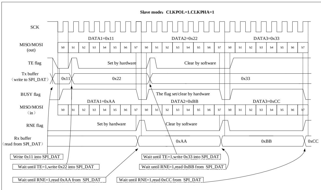
Figure 20-8 TE/RNE/BUSY Behavior in Slave / Full-Duplex Mode in Case of Continuous Transfers
