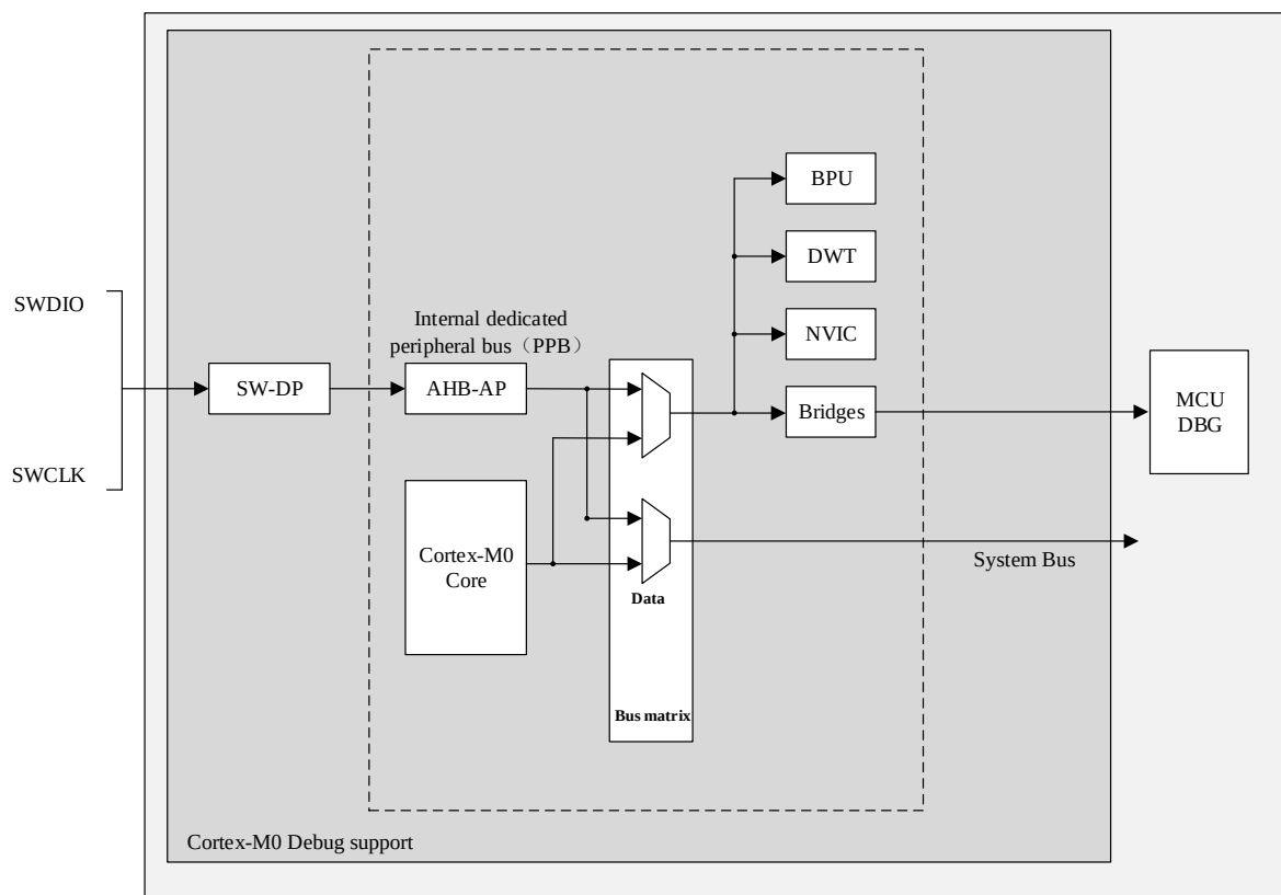
Figure 21-1 N32G033 Level And Cortex®-M0 Level Debugging Block Diagram
