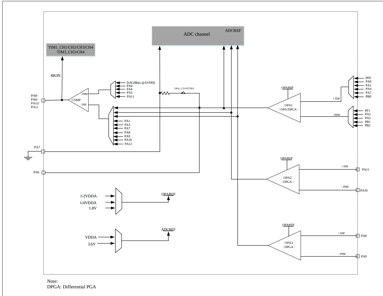
Figure 18-1 OPAMP System Connection Diagram
