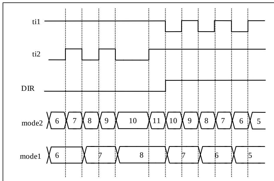
Figure 14-33 Dual-pulse coding mode (CC1P = CC2P = 1)
