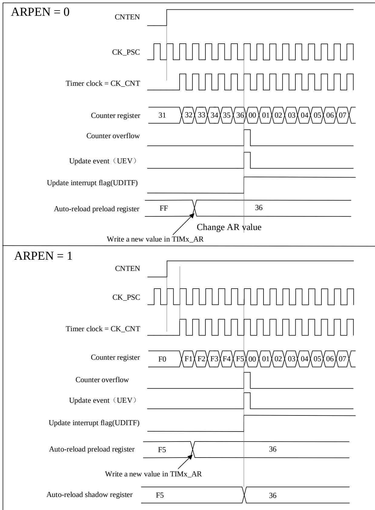
Figure 14-4 Timing Diagram of The Up-counting, Update Event When ARPEN = 0/1
