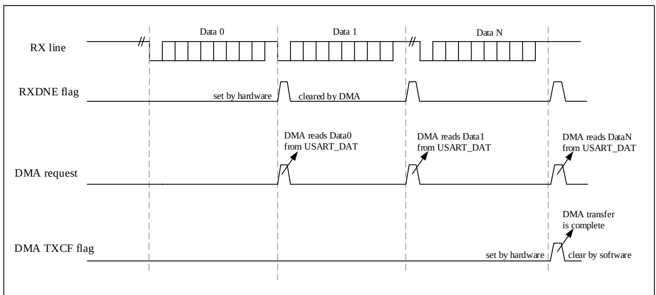
Figure 9-9 Reception Using DMA
