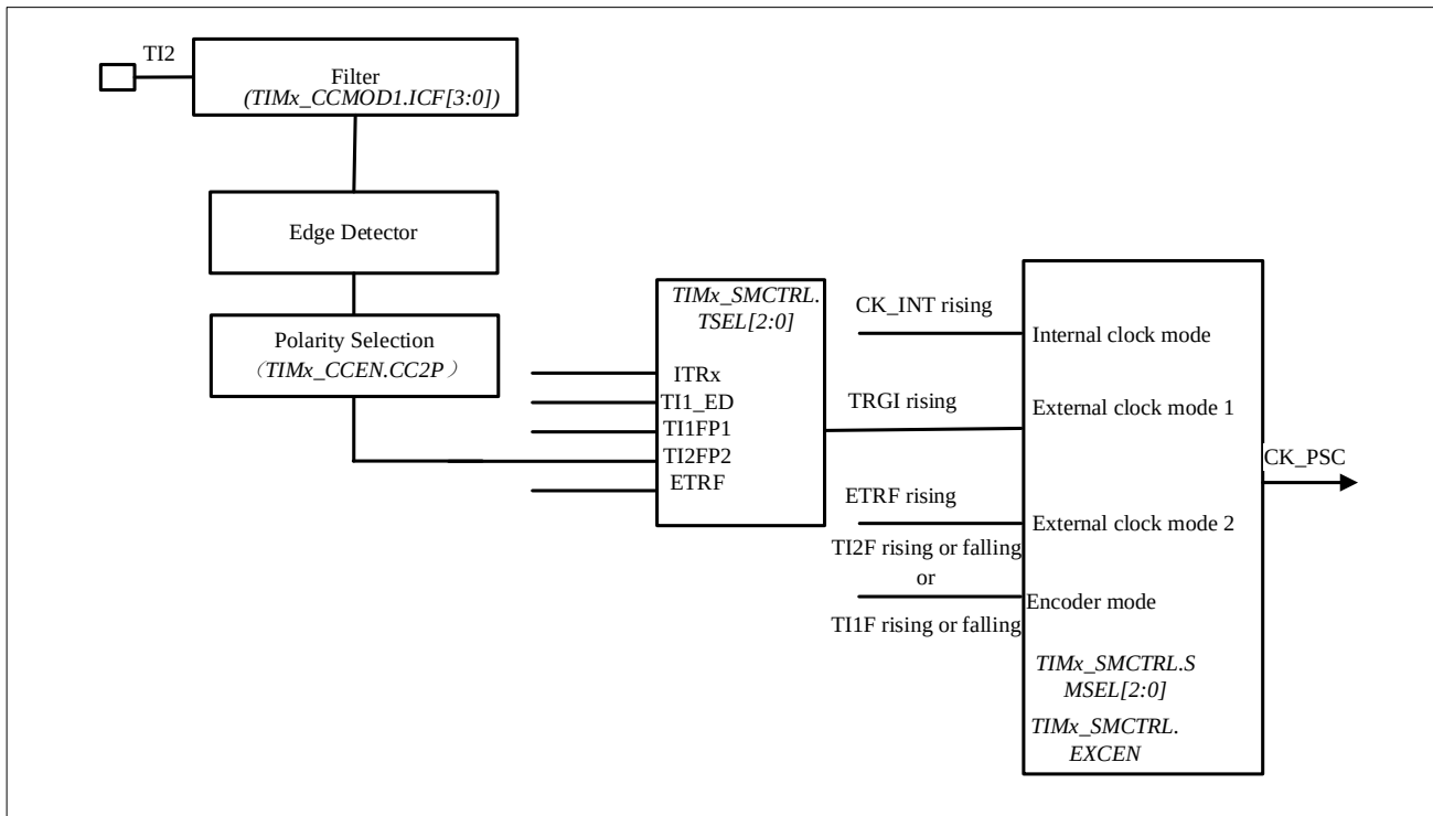
Figure 14-9 TI2 External Clock Connection Example
