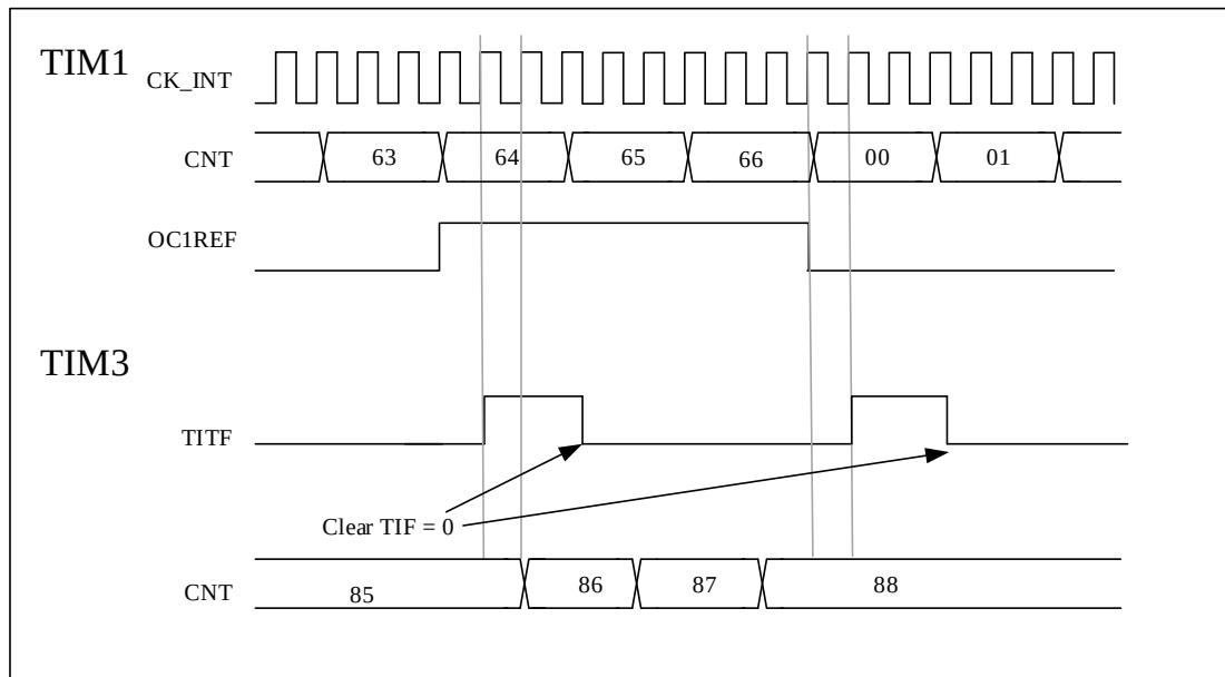
Figure 13-26 TIM3 Gated by OC1REF of TIM1
