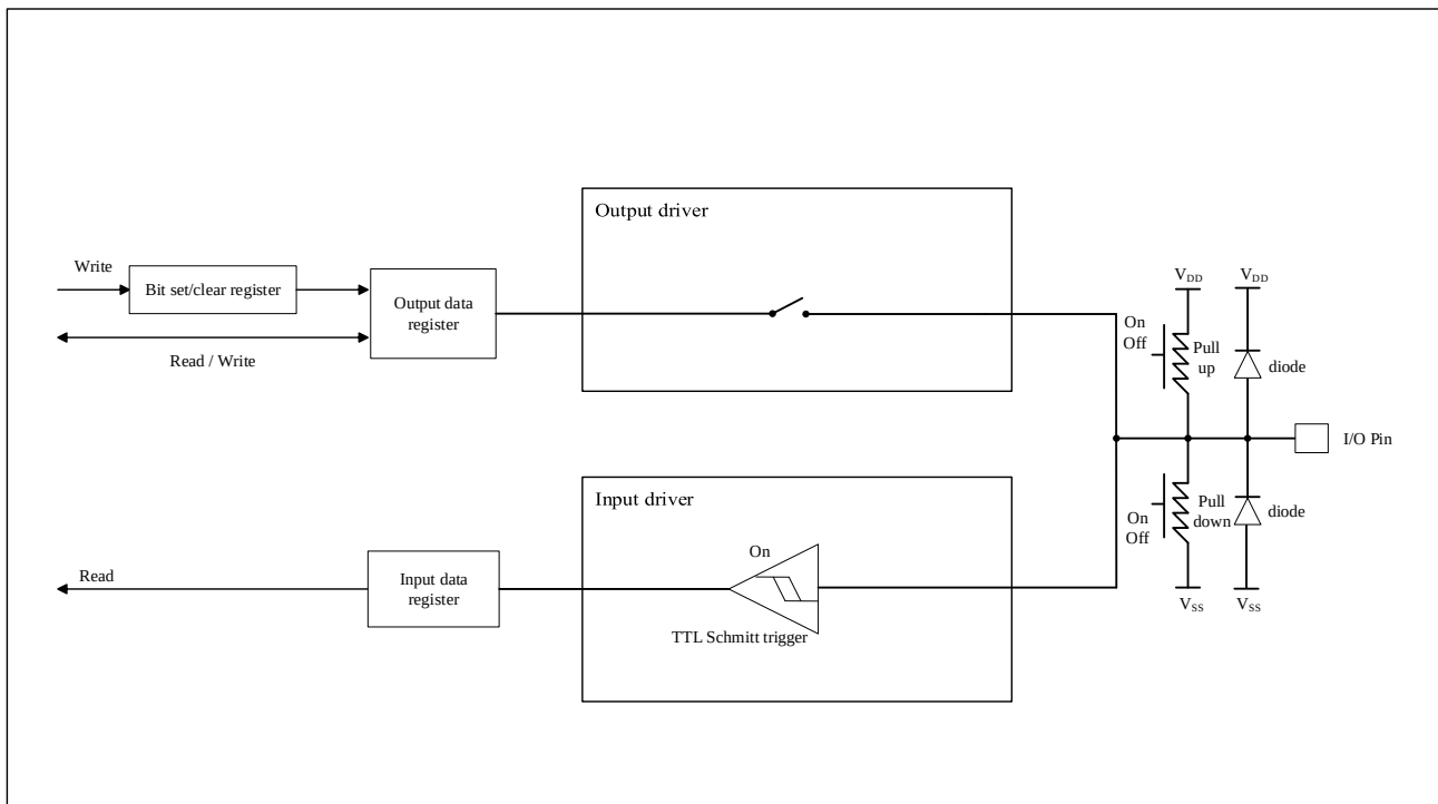
Figure 6-2 Input Floating/Pull-Up/Pull-Down Mode (Fail-safe Not Supported)
