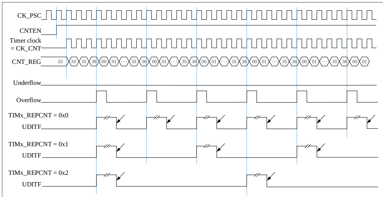
Figure 12-10 Repeat Count Sequence Diagram in Up-counting Mode
