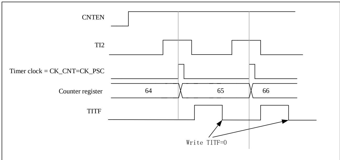
Figure 14-10 Control Circuit in External Clock Mode 1
