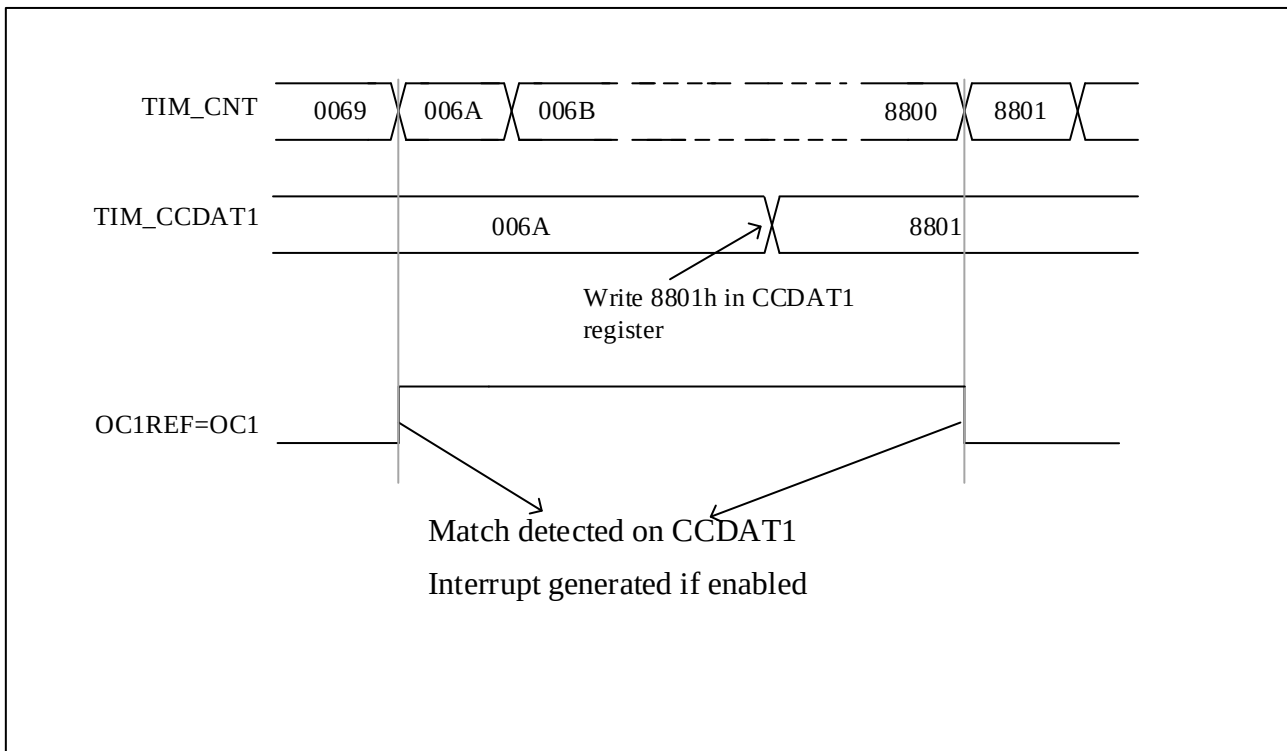
Figure 13-17 Output Compare Mode, Toggle on OC1
