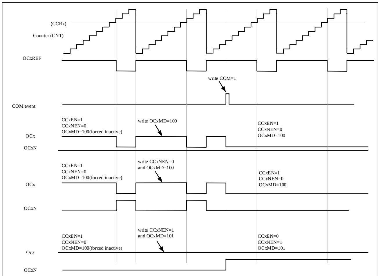
Figure 12-36 6-step PWM Generation, COM Example (OSSR=1)
