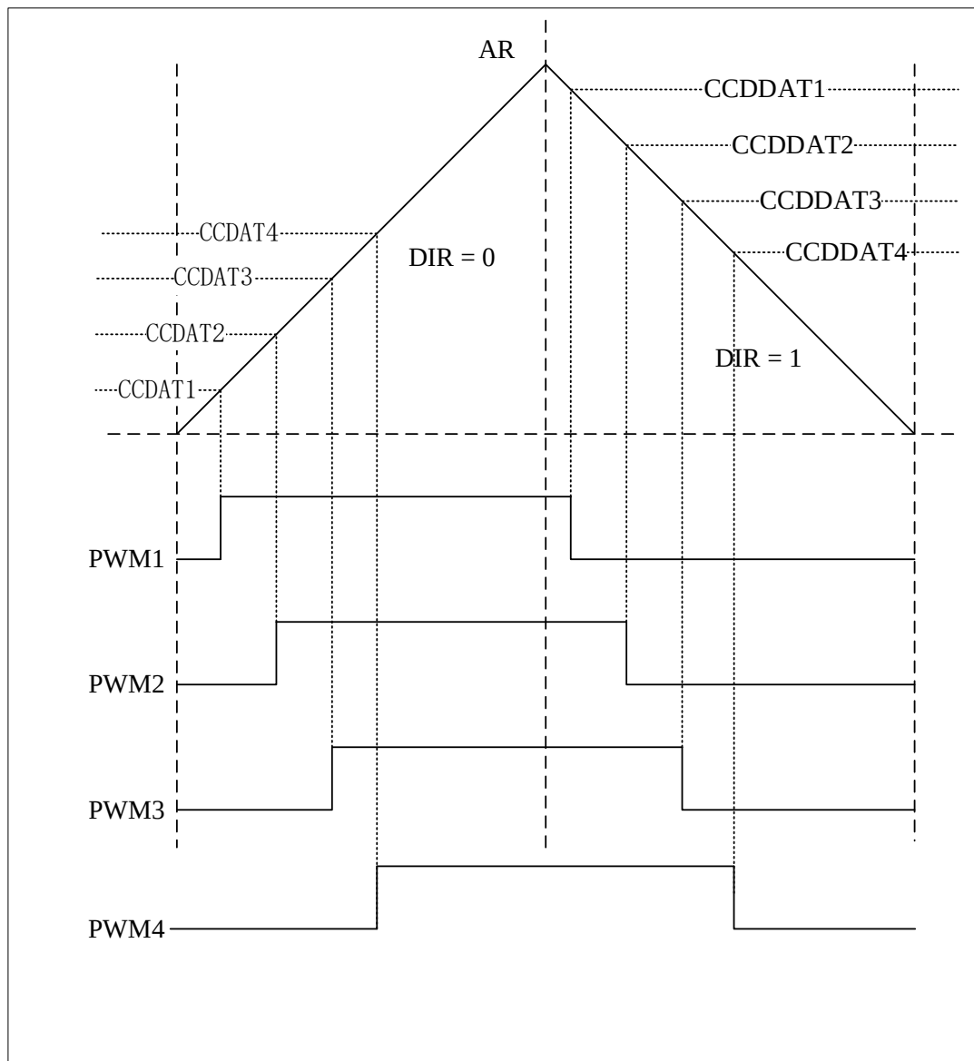
Figure 12-8 The Output Waveform Corresponding to the Asymmetric Mode
