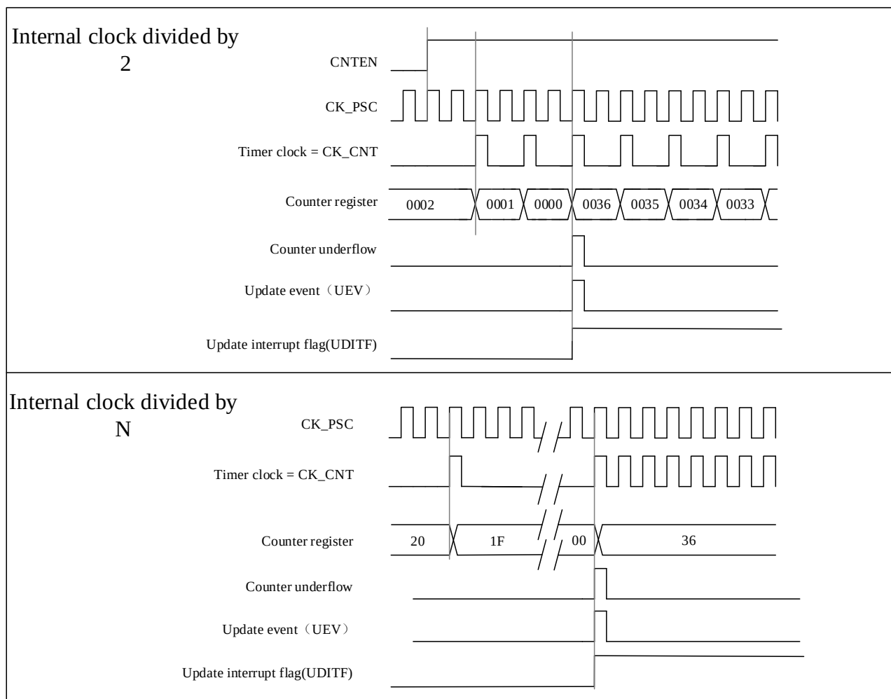
Figure 13-5 Timing Diagram of the Down-counting, Internal Clock Divided Factor = 2/N
