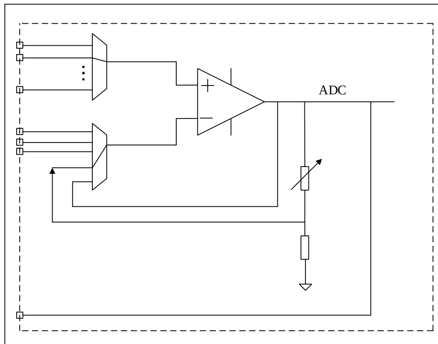
Figure 18-4 Internal gain mode
