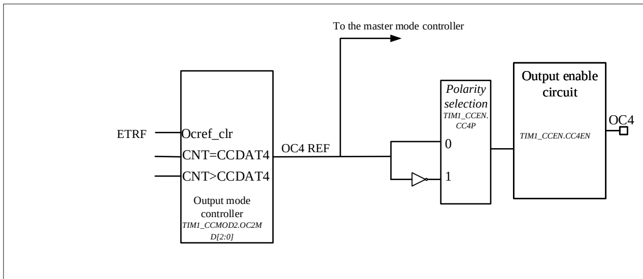
Figure 13-15 Output Part of Channelx (x = 1,2,3,4; Take Channel 4 as an Example)
