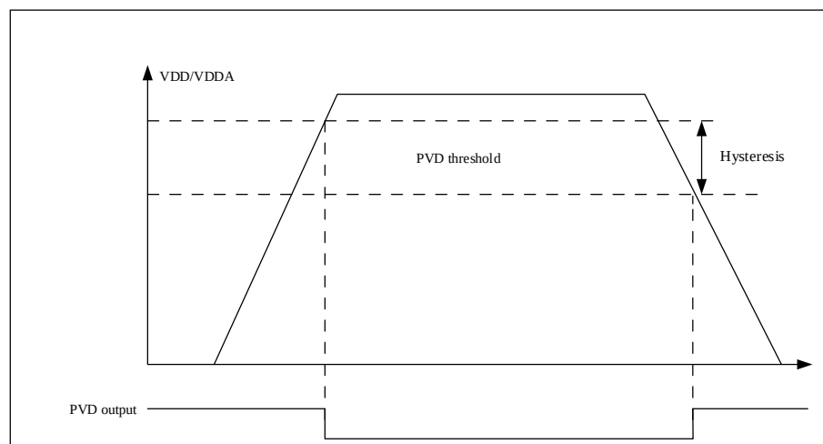
Figure 3-3 PVD Threshold Diagram
