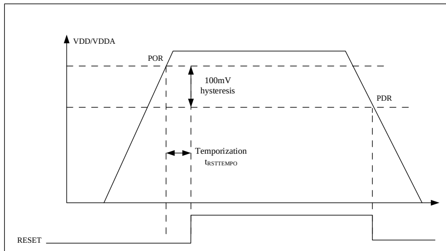
Figure 3-2 Power on Reset/Power down Reset Waveform
