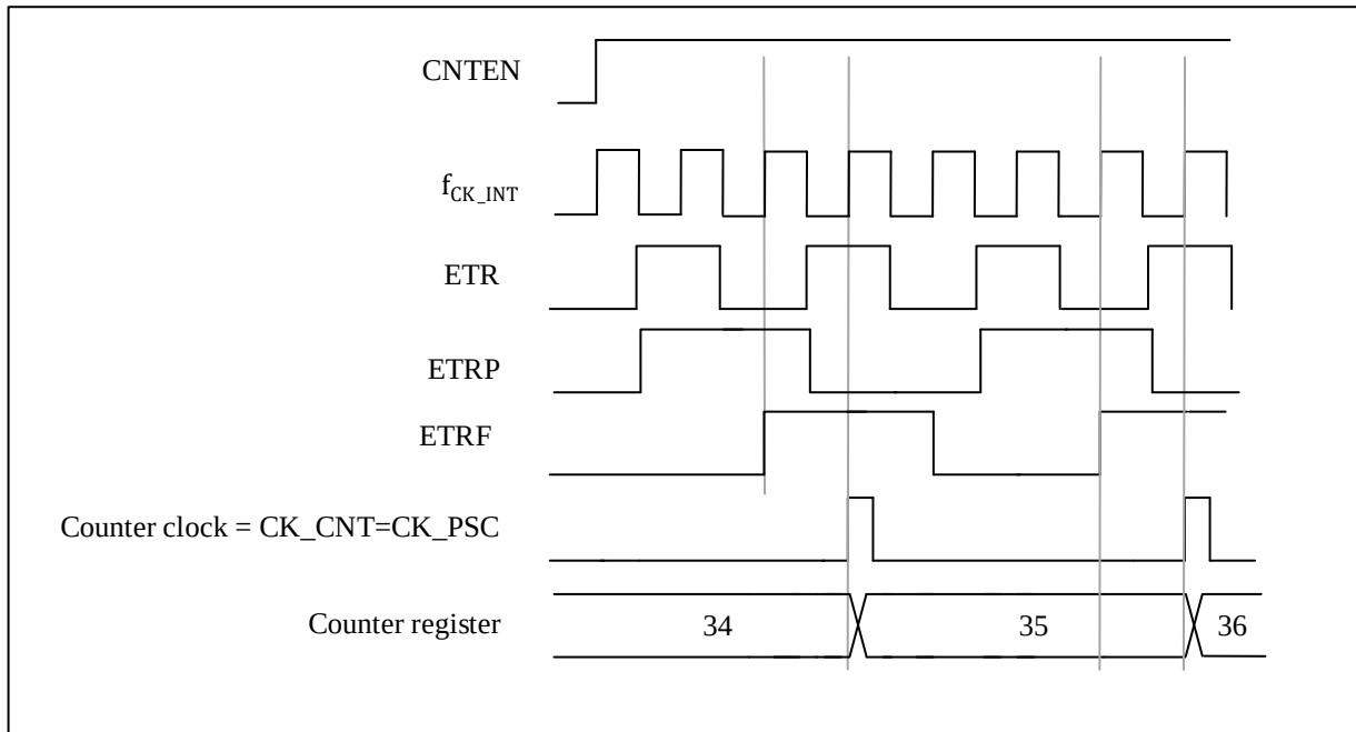
Figure 12-16 Control Circuit in External Clock Mode 2
