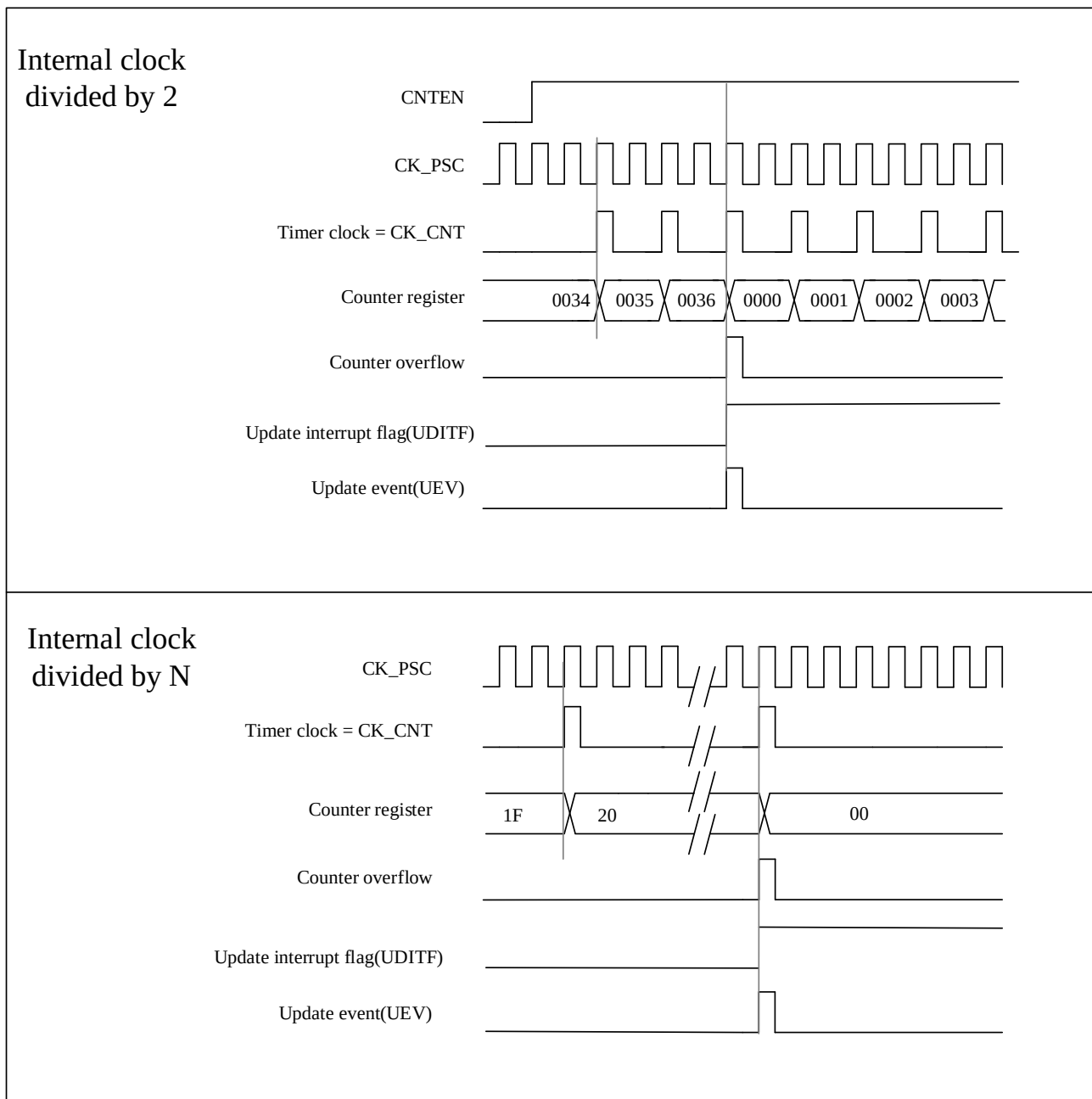
Figure 15-3 Timing Diagram Of Up-Counting. The Internal Clock Divider Factor = 2/N
