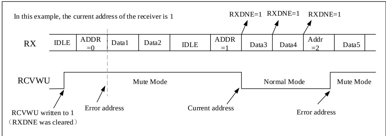
Figure 9-11 Mute Mode Detected Using Address Mark
