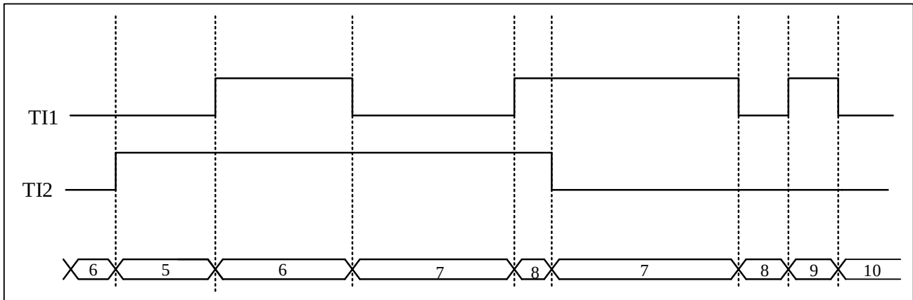
Figure 14-35 CCW/CW Encoding Mode 1 (CC1P=CC2P=0)
