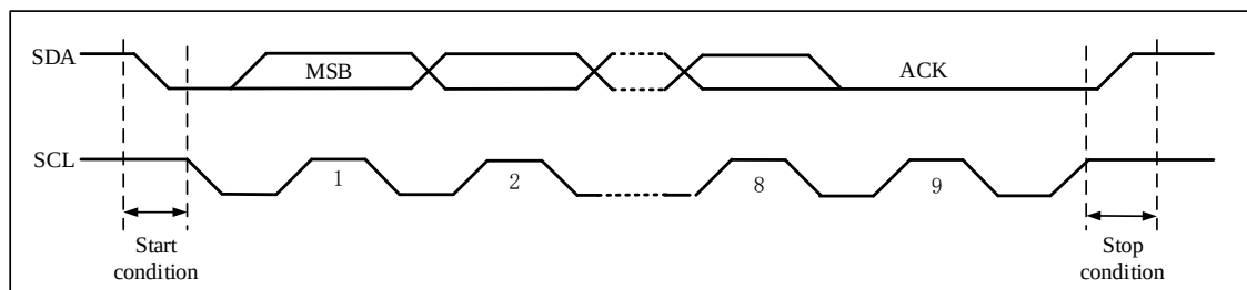
Figure 8-2 I2C Bus Protocol
