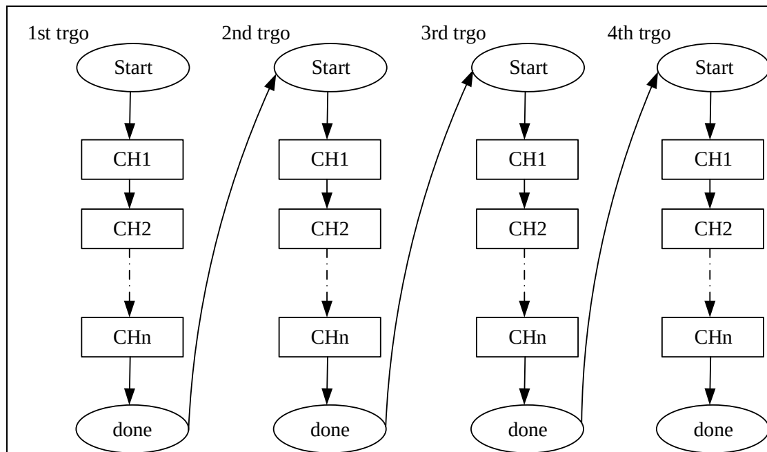
Figure 16-2 ADC segment conversion
