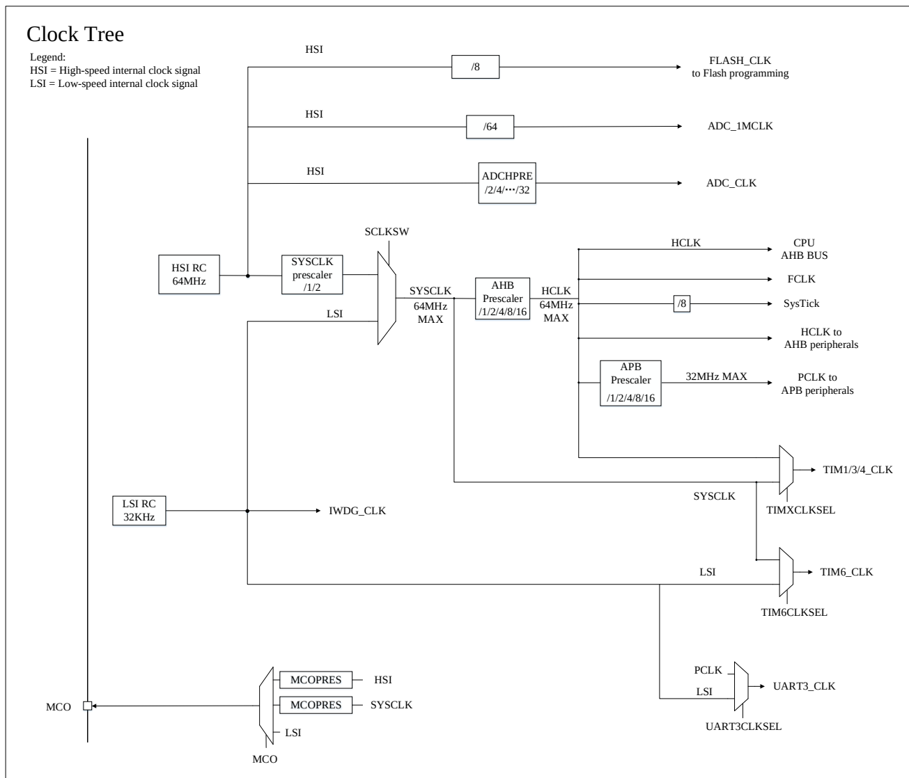
Figure 4-2 Clock Tree
