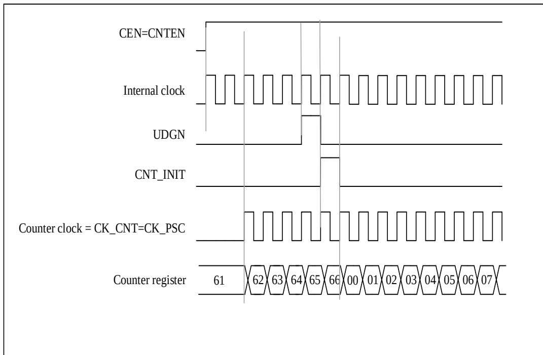
Figure 15-5 Control Circuit In Normal Mode, Internal Clock Divided By 1
