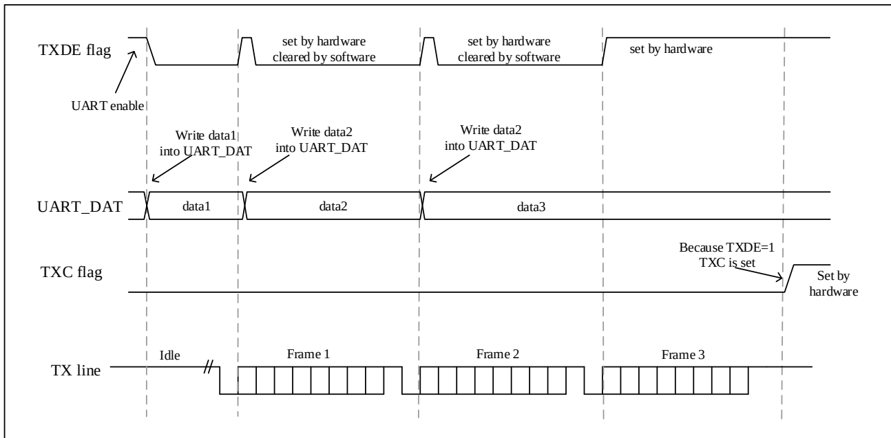
Figure 9-6 TXC/TXDE Changes During Transmission
