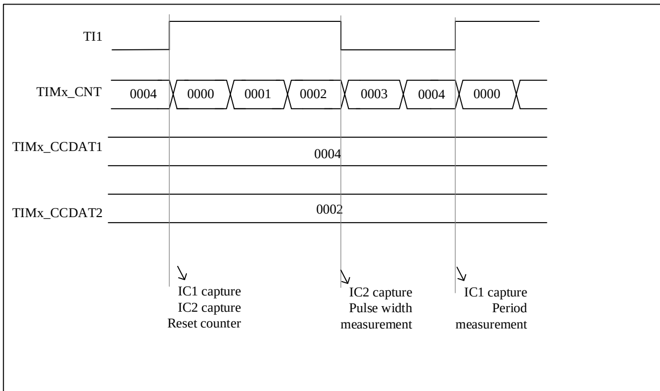
Figure 13-16 PWM Input Mode Timing
