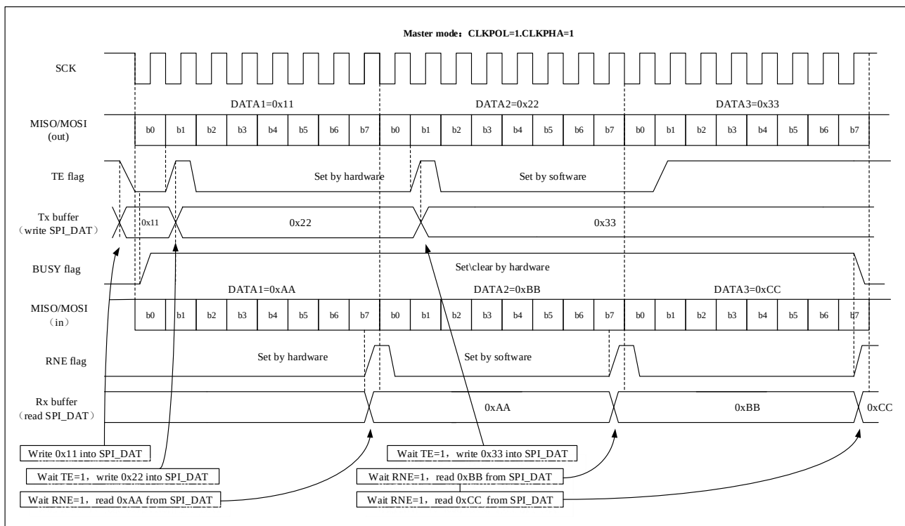
Figure 20-5 TE/RNE/BUSY Behavior in Master / Full-Duplex Mode (BIDIRMODE = 0, RONLY = 0) in Case of Continuous Transfers
