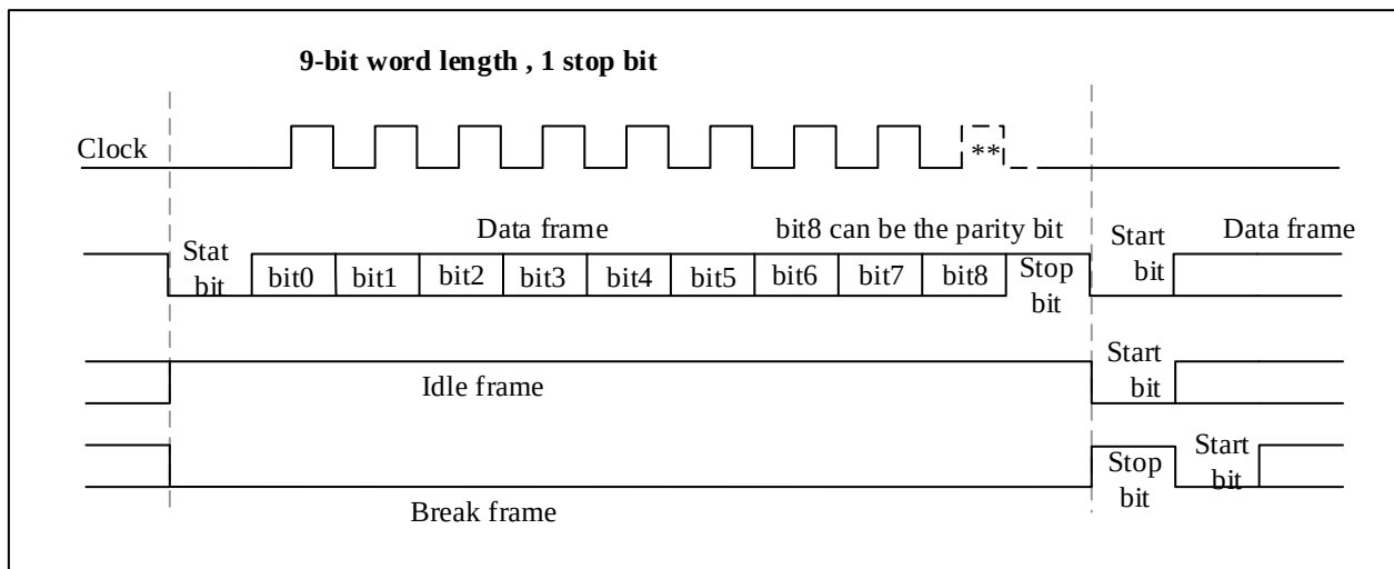
Figure 9-3 Word Length = 9 Setting
