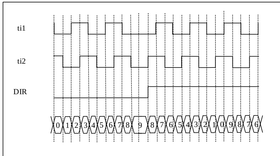
Figure 14-27 When T2 is high, the counter only increments during TI1
