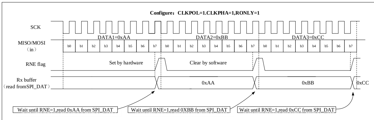
Figure 20-7 RNE Behavior in Receive-Only Mode in Case of Continuous Transfers (BIDIRMODE = 0, RONLY = 1)
