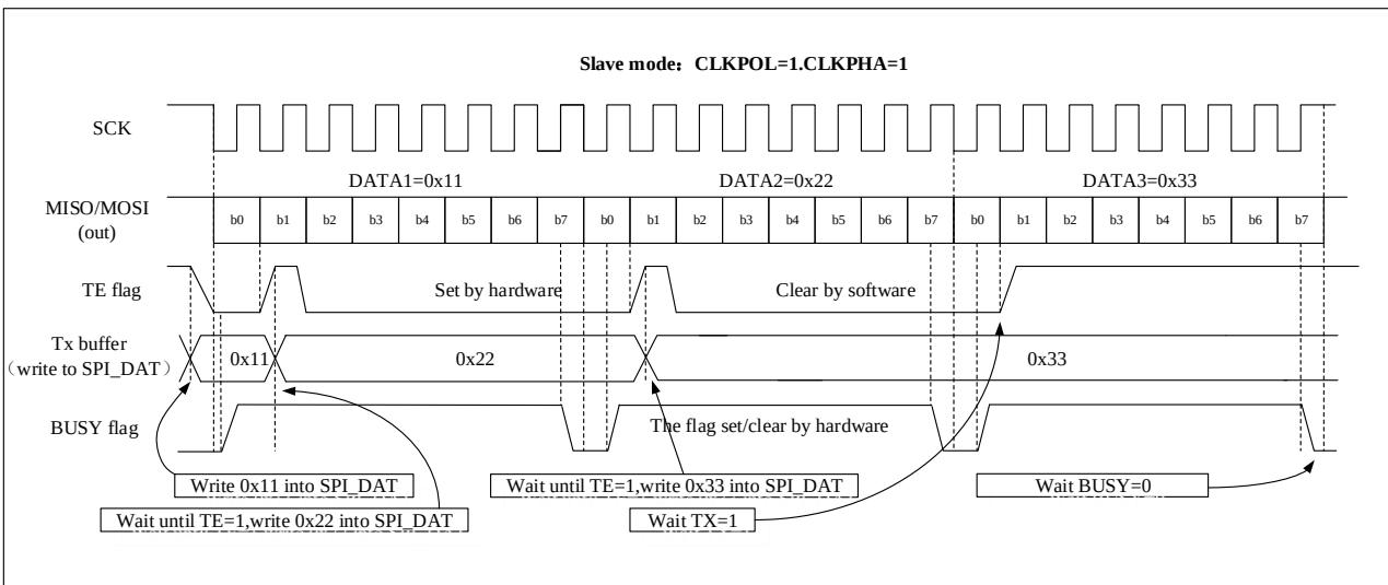
Figure 20-9 TE/BUSY Behavior in Slave Transmit-Only Mode in Case of Continuous Transfers
