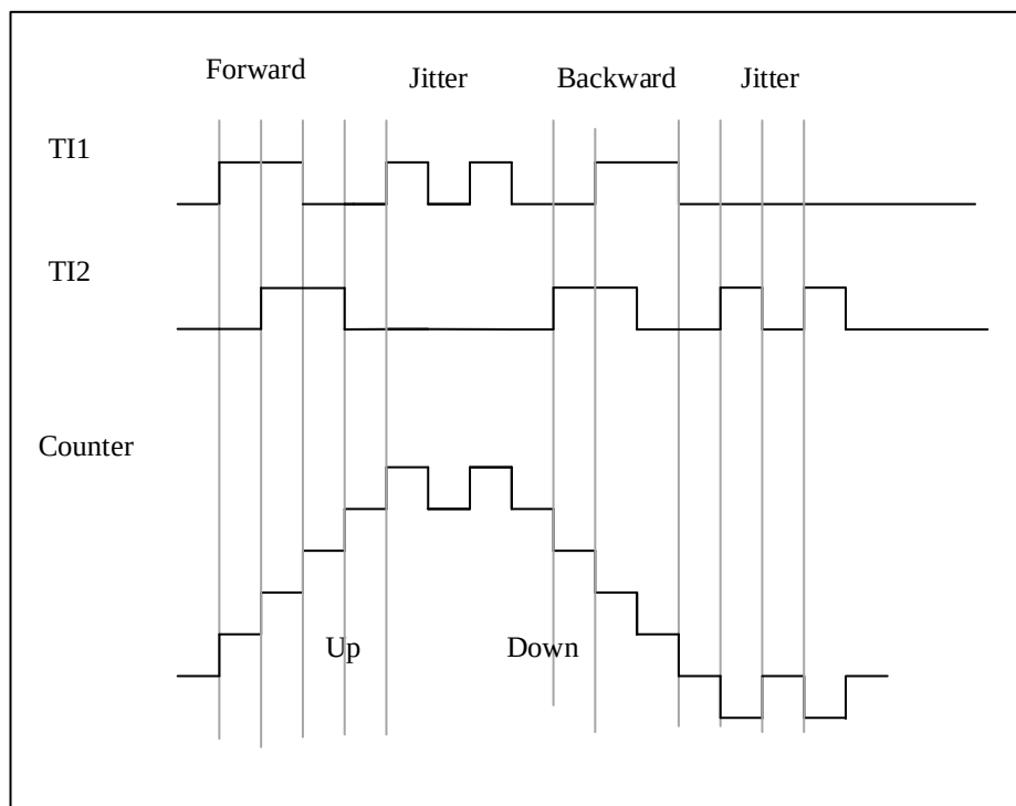
Figure 12-37 Example of Counter Operation in Encoder Interface Mode
