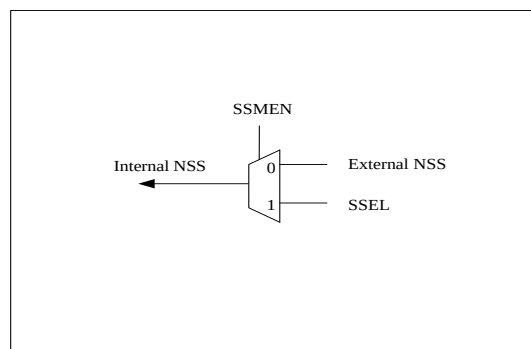
Figure 20-2 Selective Management of Hardware/Software
