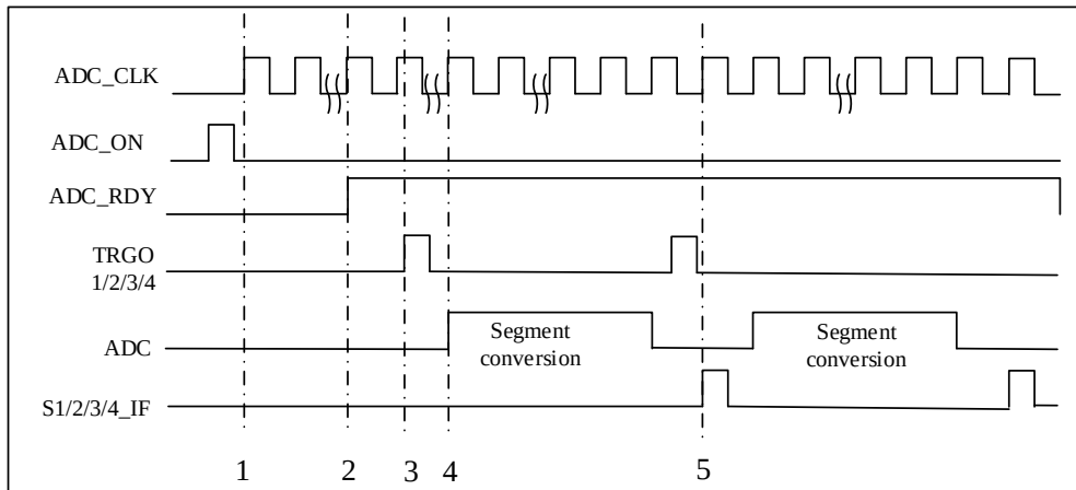
Figure 16-3 Timing Diagram
