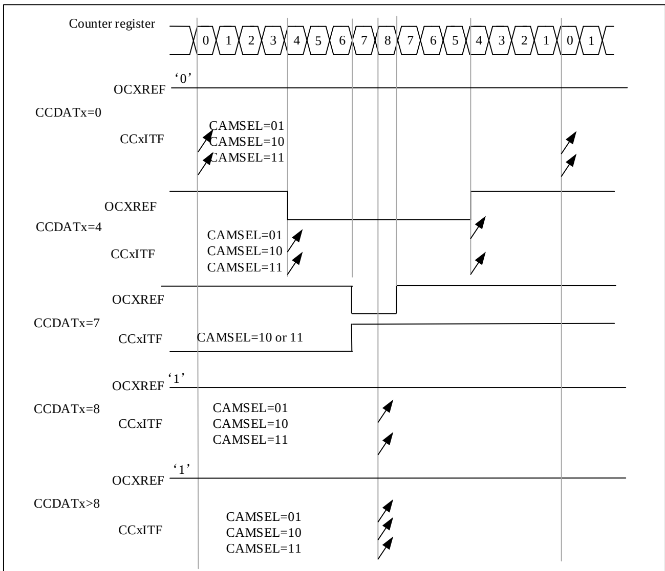
Figure 13-18 Center-aligned PWM Waveform (AR=8)
