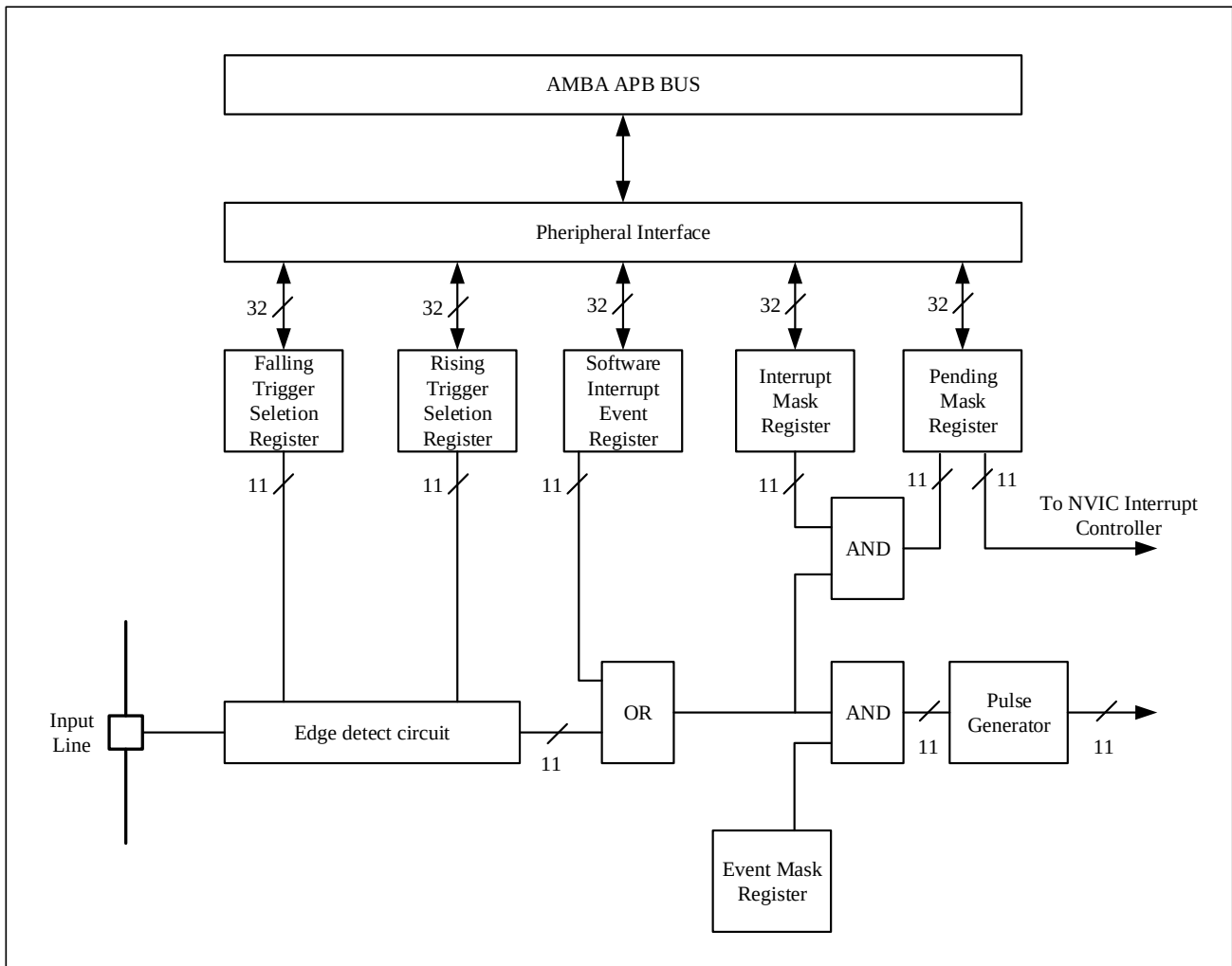
Figure 5-1 Extenal Interrupt/Event Controller Block Diagram
