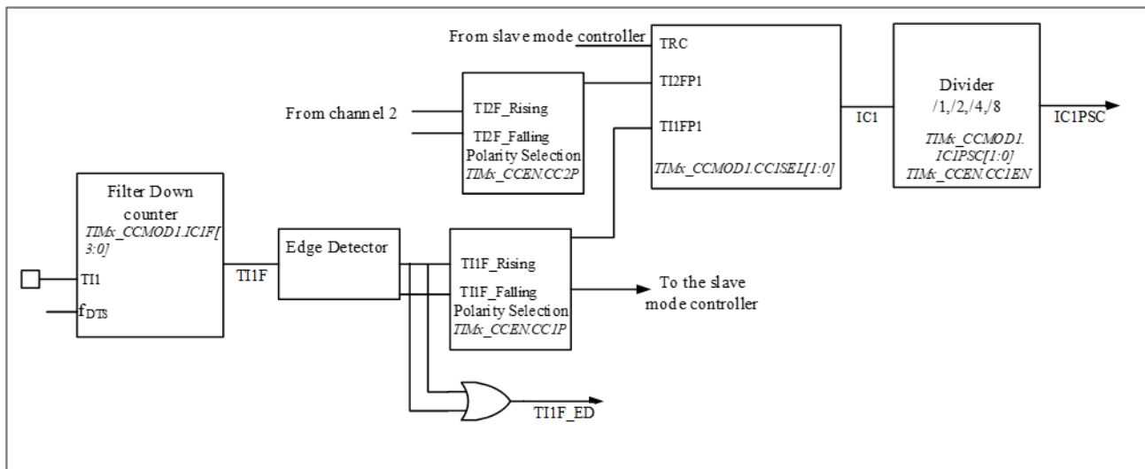
Figure 14-13 Capture/Compare Channel (Example: Channel 1 Input Stage)
