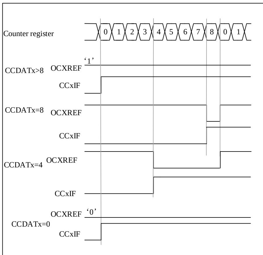
Figure 13-19 Edge-aligned PWM Waveform (APR=8)
