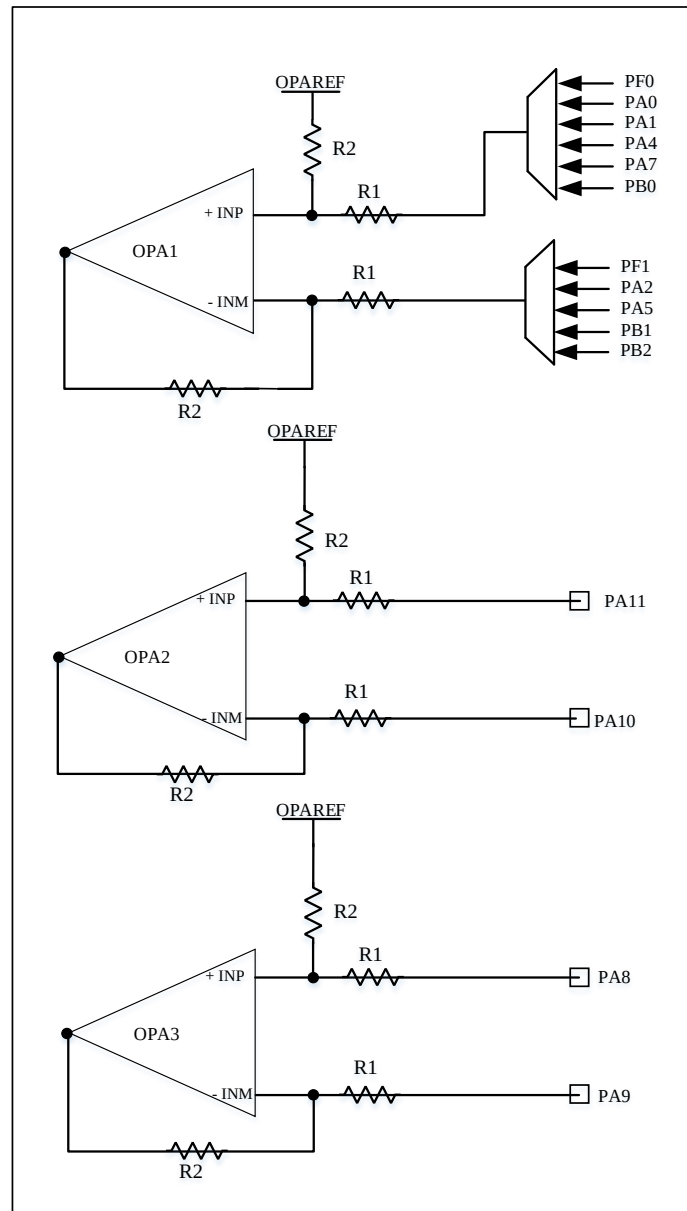
Figure 18-5 Differential Gain mode
