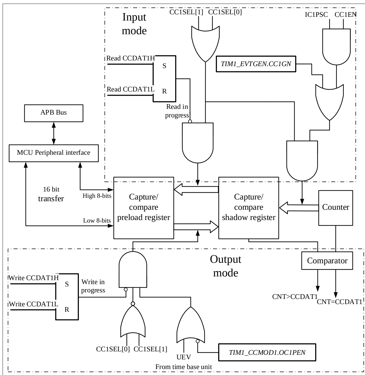
Figure 13-14 Capture/Compare Channel 1 Main Circuit
