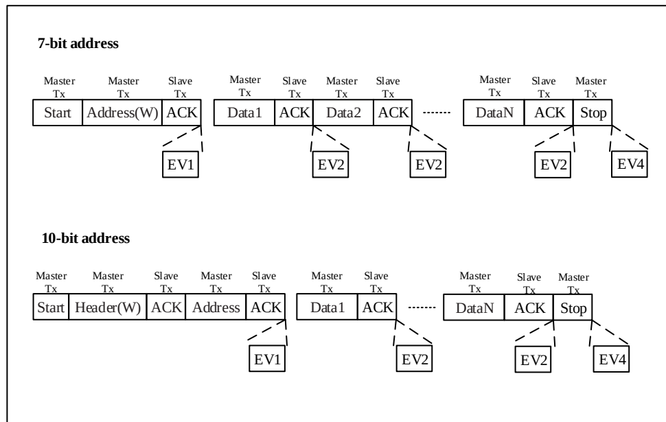
Figure 8-4 Slave receiver transmitting sequence
