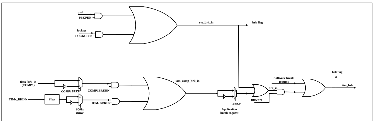
Figure 12-27 Brake input
