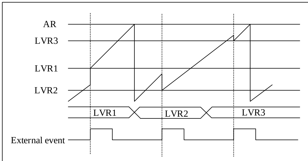
Figure 14-23 External event triggers loading
