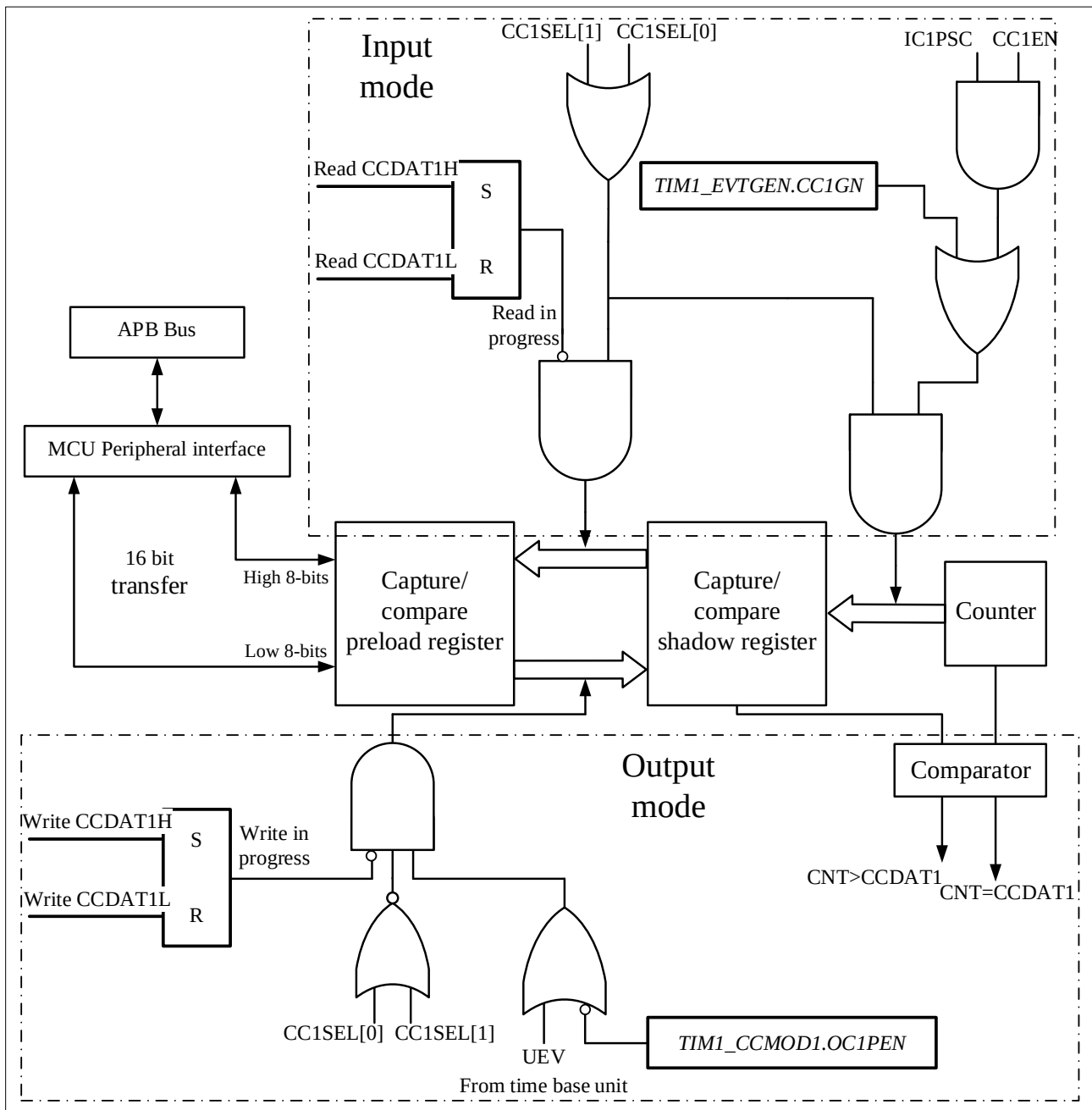
Figure 14-14 Capture/Compare Channel 1 Main Circuit
