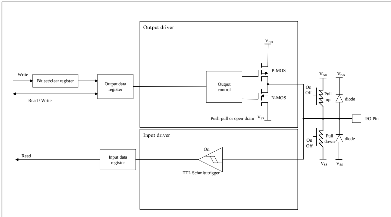
Figure 6-3 Output Mode (Fail-safe Not Supported)
