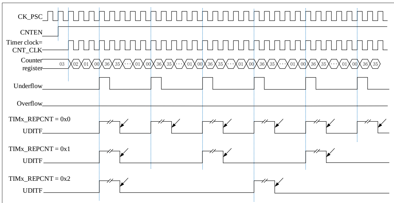
Figure 12-9 Repeat Count Sequence Diagram in Down-counting Mode
