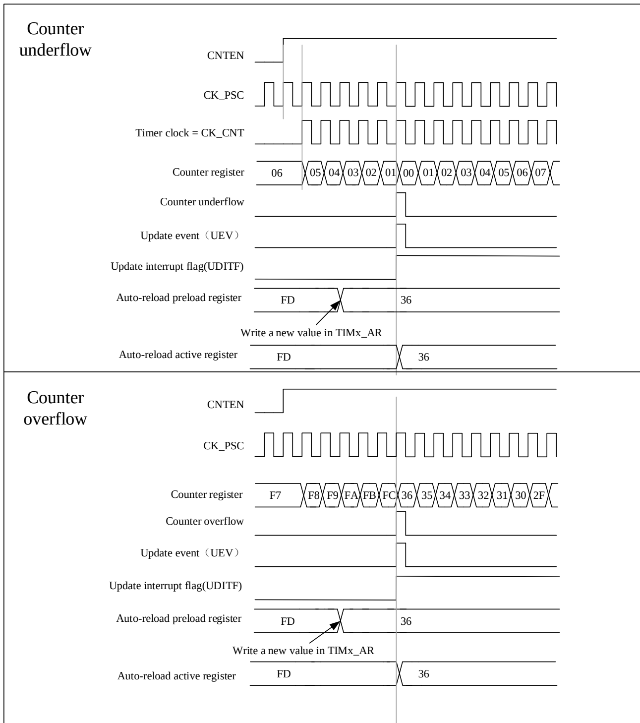
Figure 14-7 A Center-aligned Sequence Diagram That Includes Counter Overflows and Underflows (ARPEN = 1)
