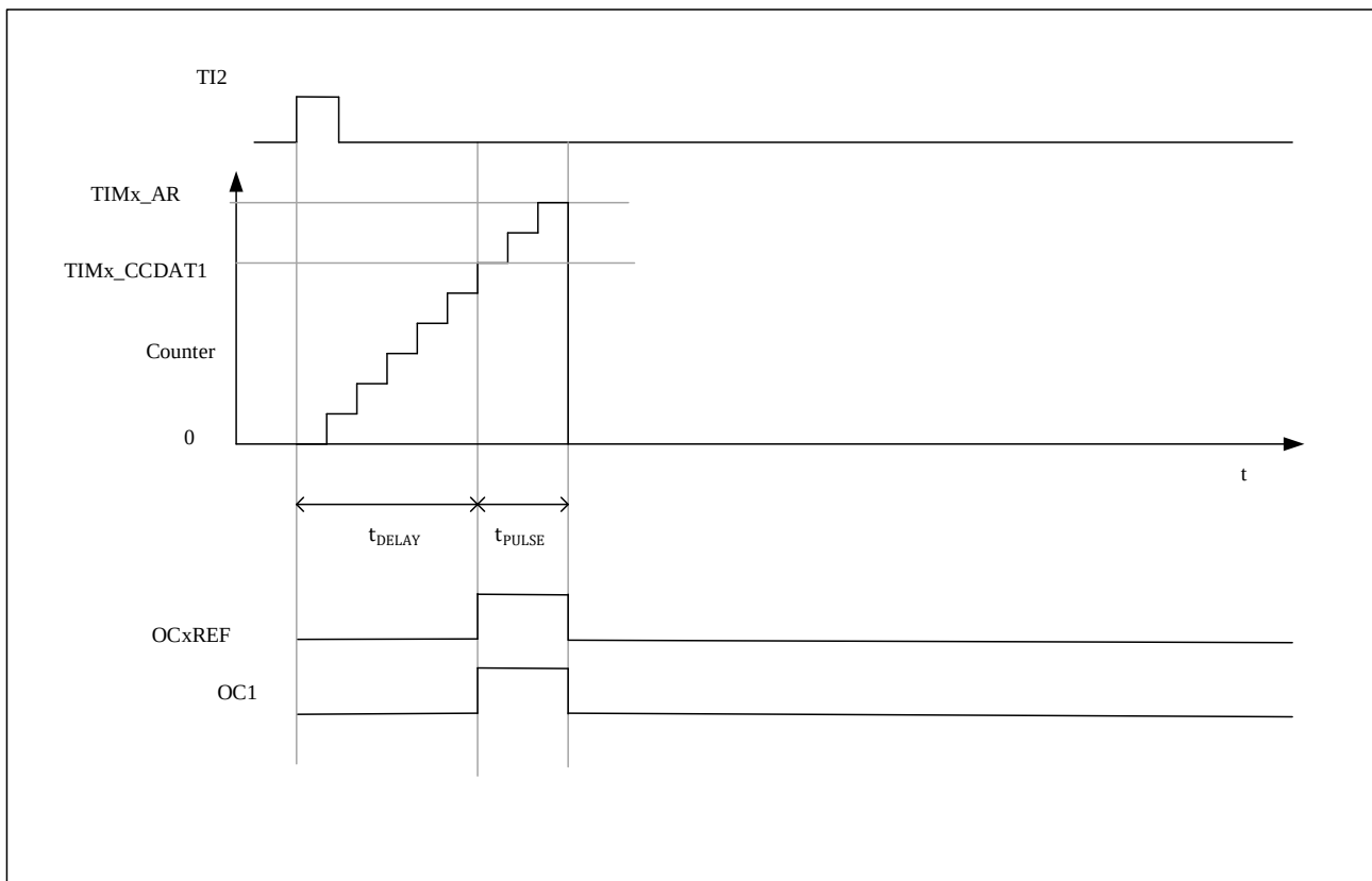
Figure 13-20 Example of One-pulse Mode
