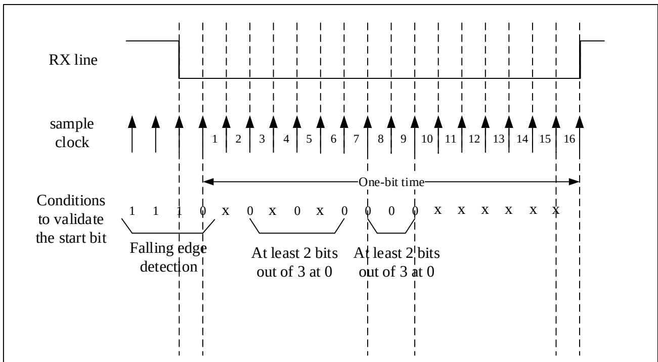
Figure 9-7 Start Bit Detection
