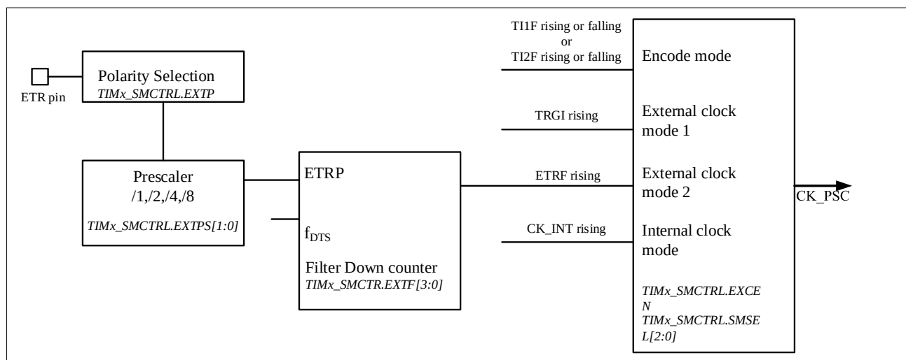
Figure 13-11 External Trigger Input Block Diagram
