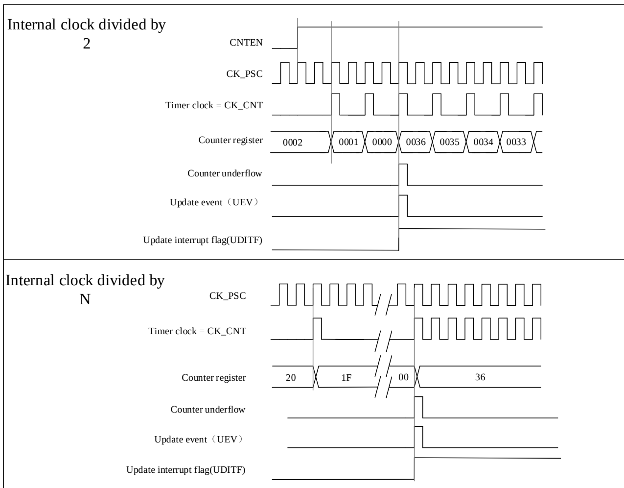
Figure 14-5 Timing Diagram of the Down-counting, Internal Clock Divided Factor = 2/N
