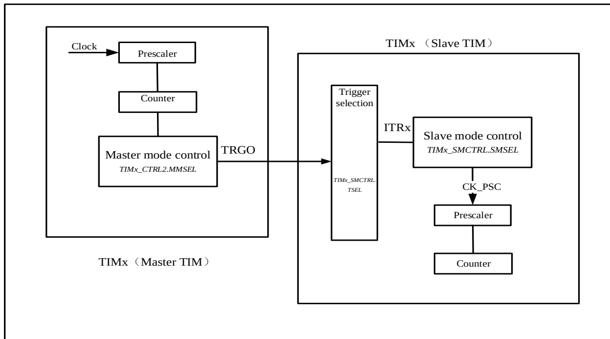
Figure 13-25 Master/Slave Timer Connection
