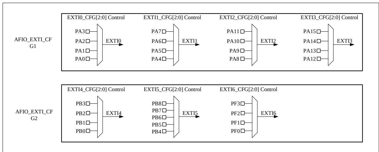
Figure 5-2 External Interrupt Generic I/O Mapping
