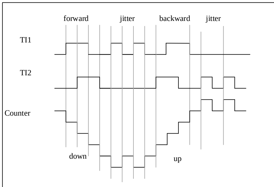
Figure 14-30 Example of IC1FP1 Inverted Encoder Interface Mode
