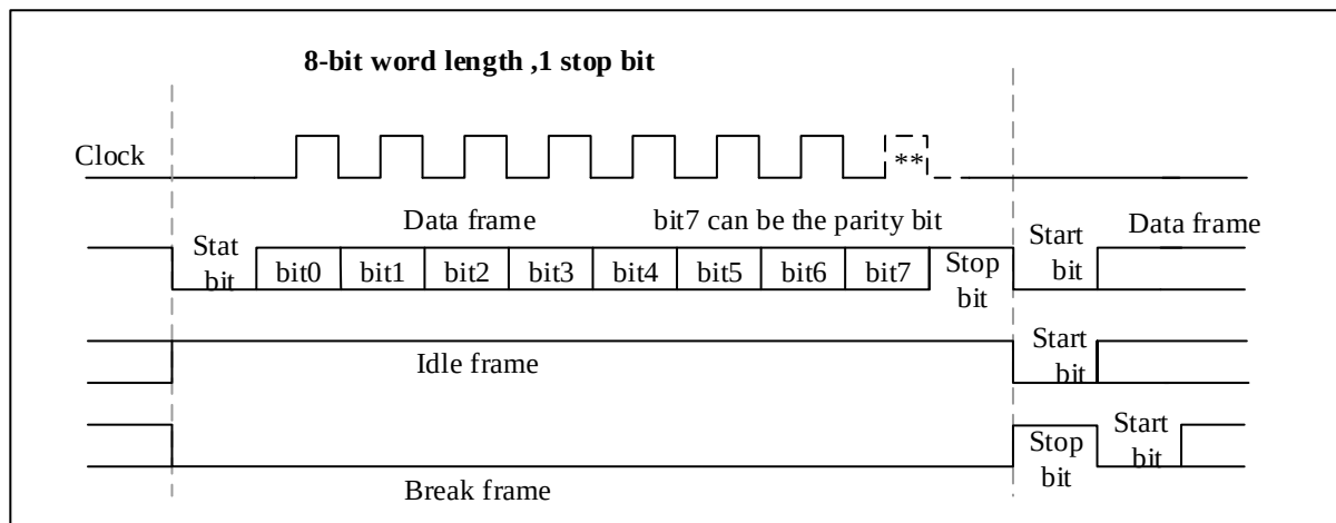
Figure 9-2 Word Length = 8 Setting
