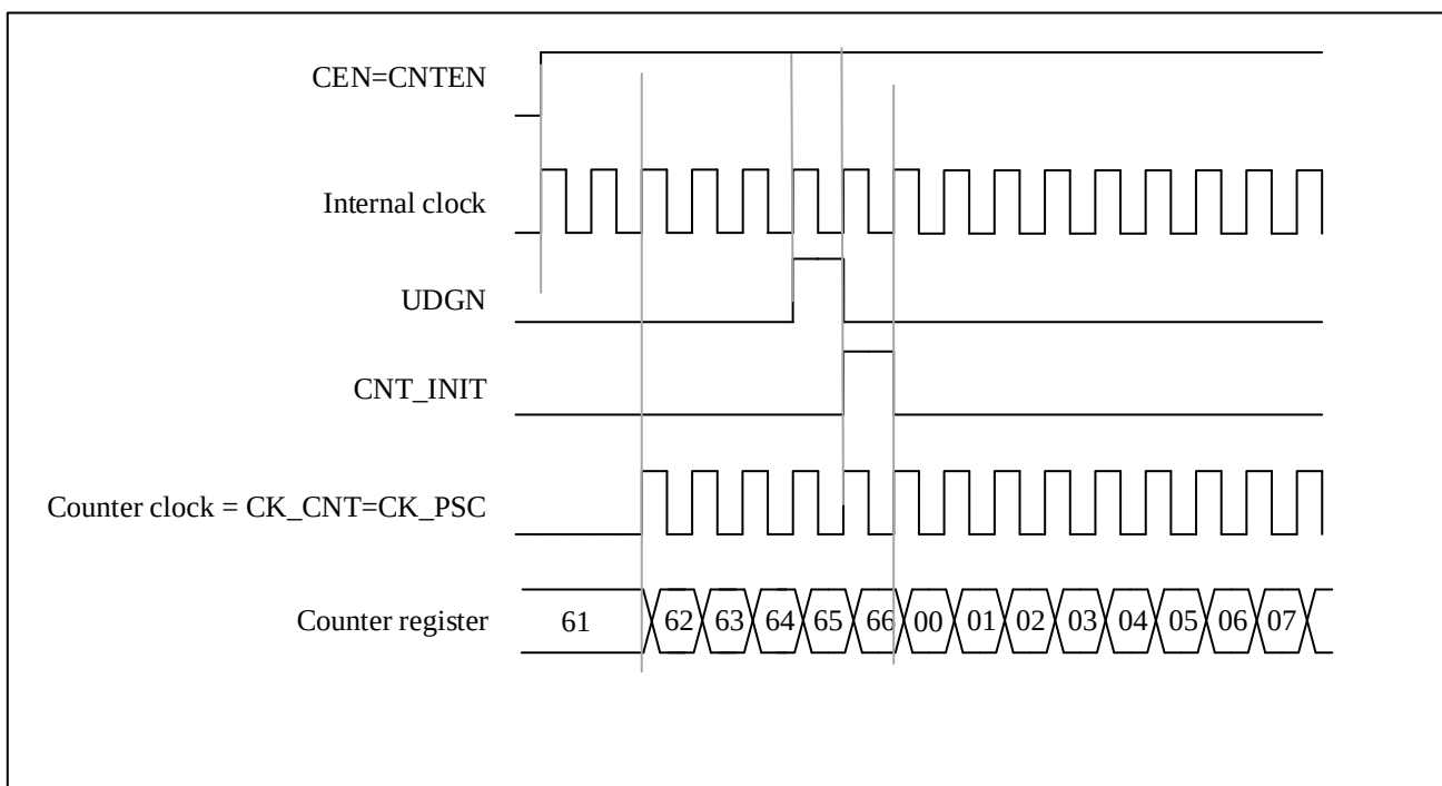
Figure 12-12 Control Circuit in Normal Mode, Internal Clock Divided By 1
