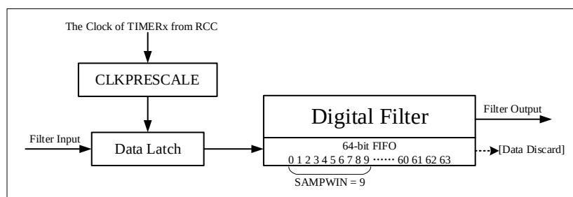
Figure 13-23 Sliding filter
