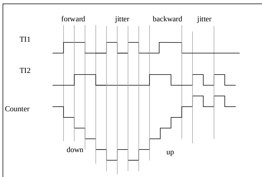
Figure 12-38 Encoder Interface Mode Example with IC1FP1 Polarity Inverted
