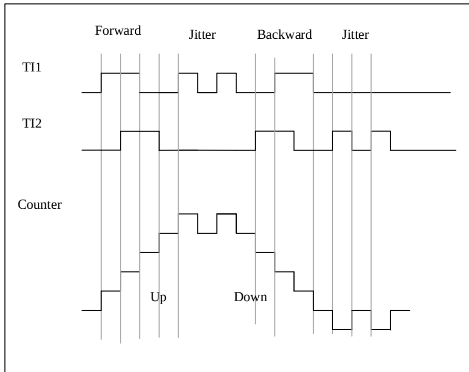
Figure 14-29 Examples of counter operations in encoder mode
