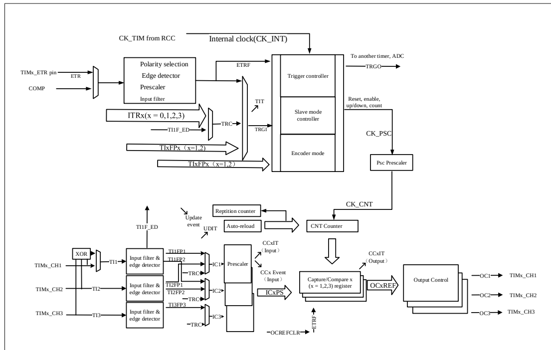
Figure 14-1 Block Diagram of TIM4
