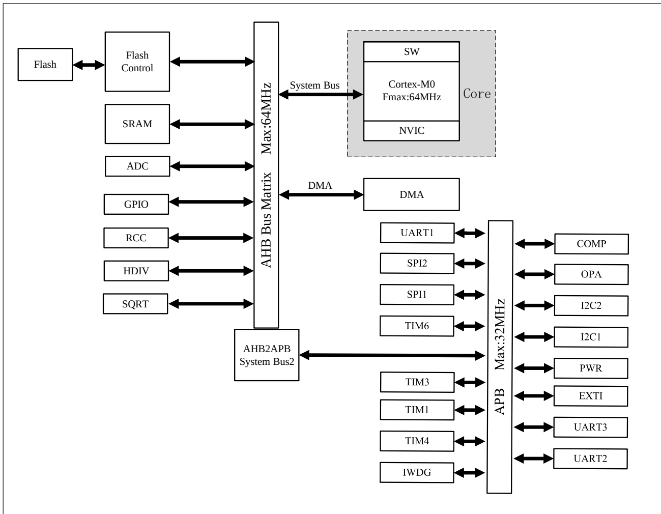
Figure 2-1 Bus Architecture
