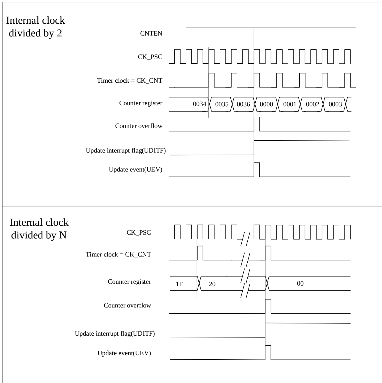
Figure 14-3 Timing Diagram of Up-counting, The Internal Clock Divider Factor = 2/N
