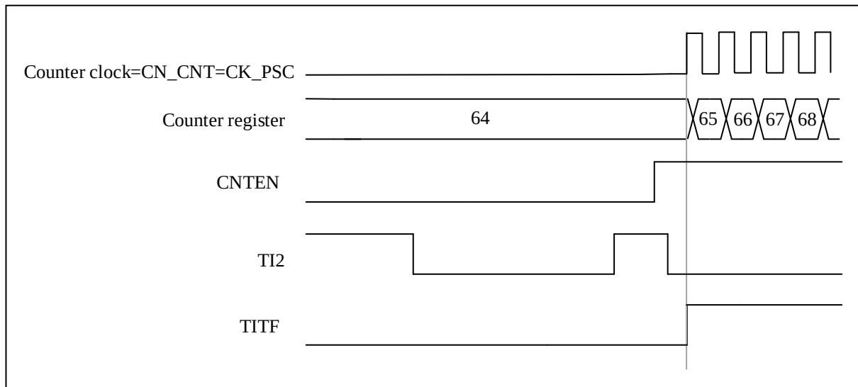
Figure 12-31 Control Circuit in Trigger Mode
