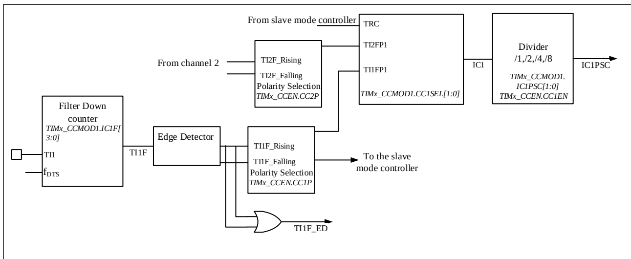
Figure 12-17 Capture/Compare Channel (Example: Channel 1 Input Stage)
