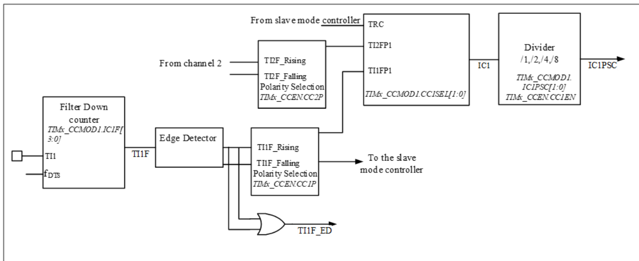
Figure 13-13 Capture/Compare Channel (Example: Channel 1 Input Stage)
