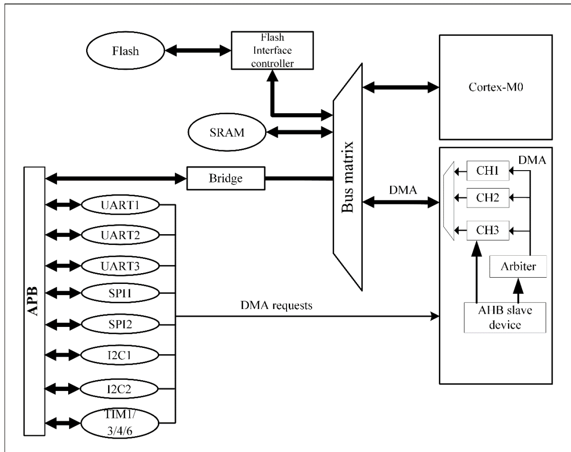
Figure 7-1 DMA Block Diagram
