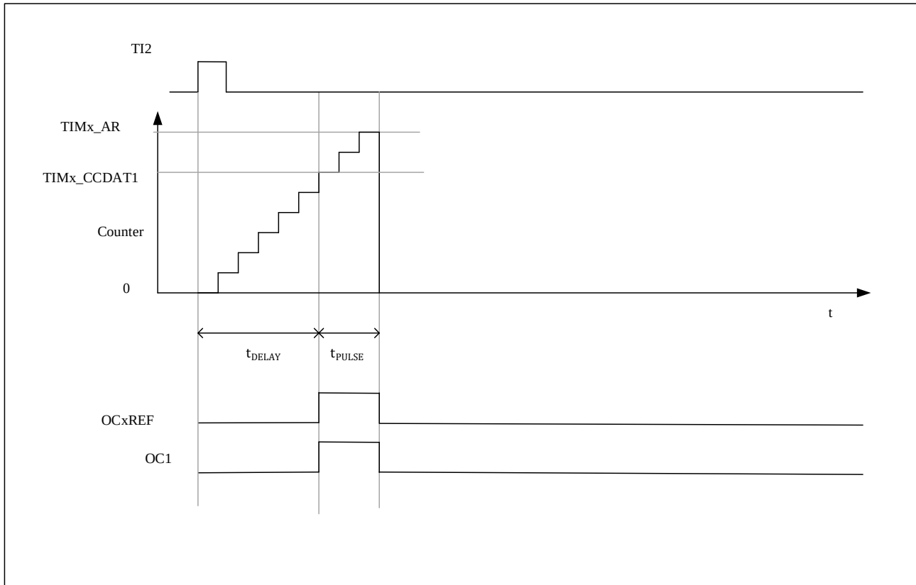
Figure 12-24 Example of One-pulse Mode
