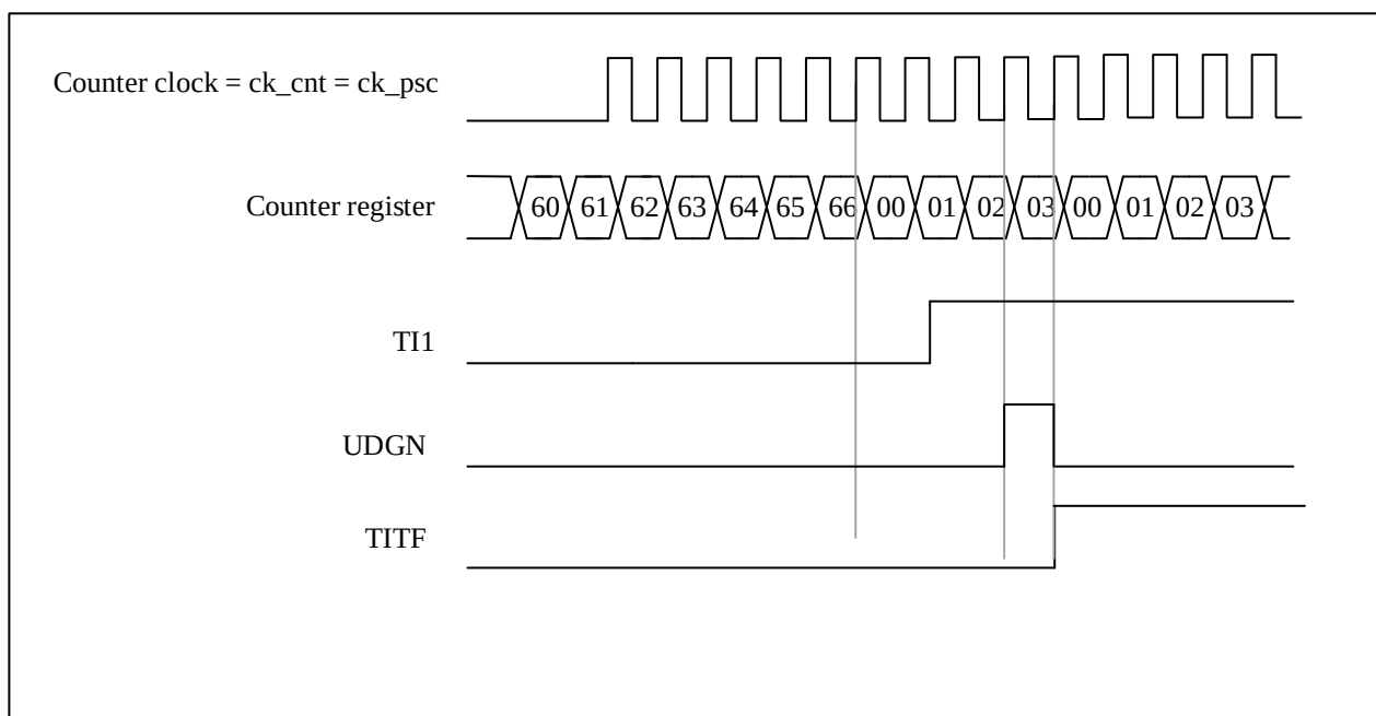
Figure 12-30 Control Circuit in Reset Mode
