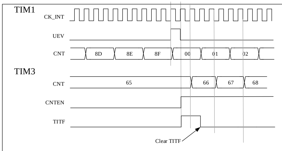
Figure 13-28 Trigger TIM3 with an Update of TIM1
