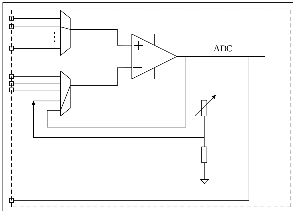
Figure 18-3 OPAMP1 Follow mode
