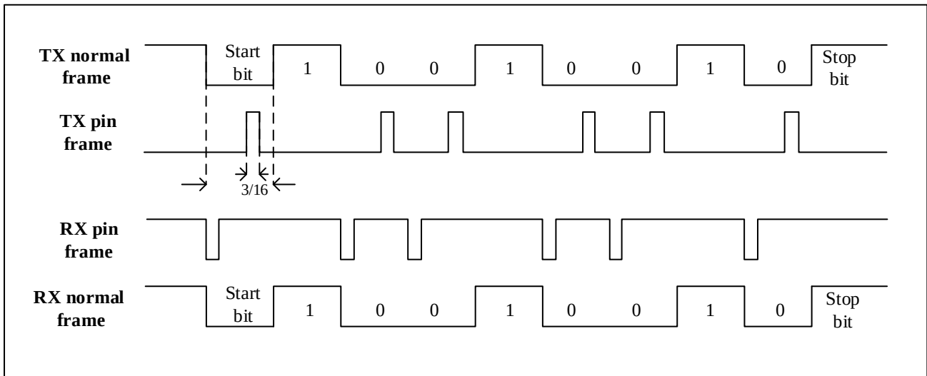
Figure 9-13 IrDA Data Modulation (3/16)-Normal Mode
