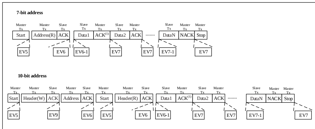
Figure 8-6 Master receiver transmission sequence diagram
