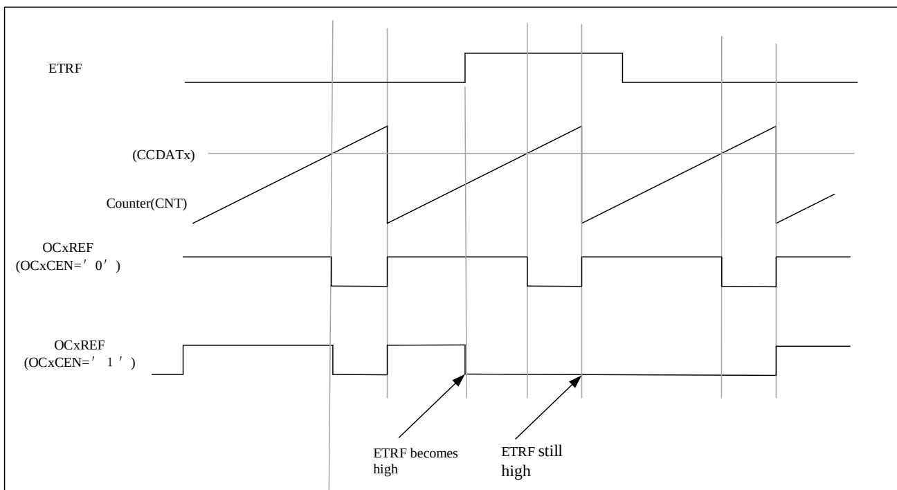
Figure 12-25 Clearing the OCxREF of TIMx
