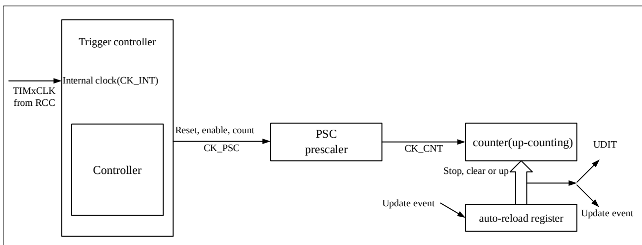
Figure 15-1 Block Diagram Of TIM6
