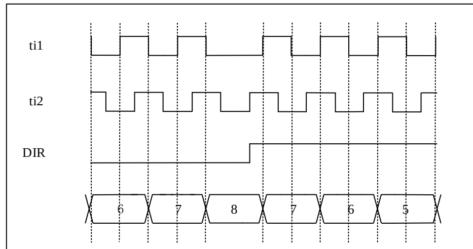
Figure 14-28 When T1 is high, the counter only increments during TI2
