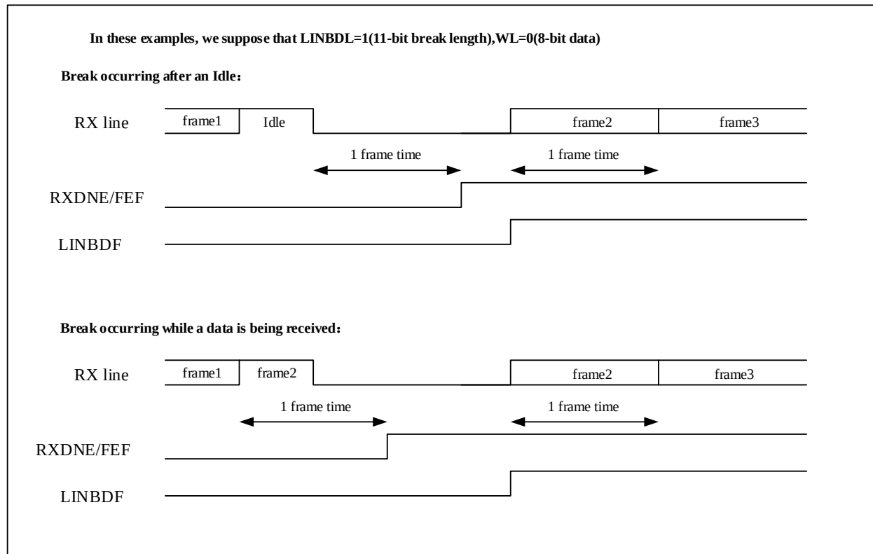
Figure 9-15 Break Detection and Framing Error Detection in LIN Mode
