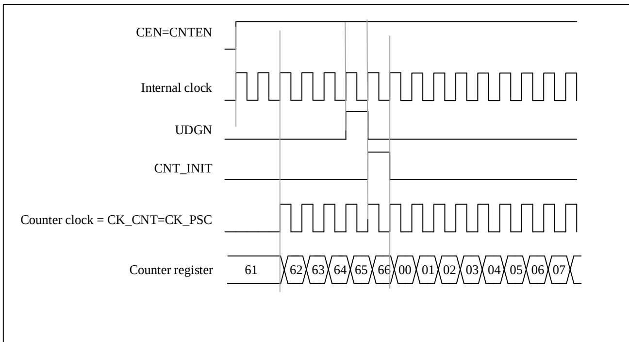
Figure 14-8 Control Circuit in Normal Mode, Internal Clock Divided by 1
