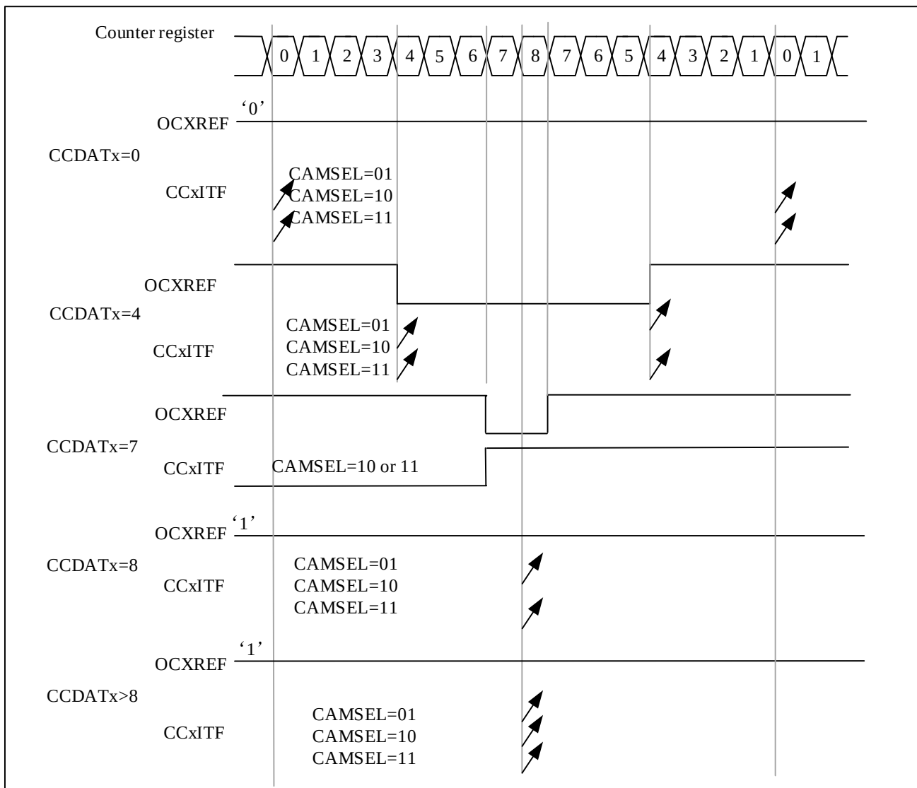
Figure 12-22 Center-aligned PWM Waveform (AR=8)
