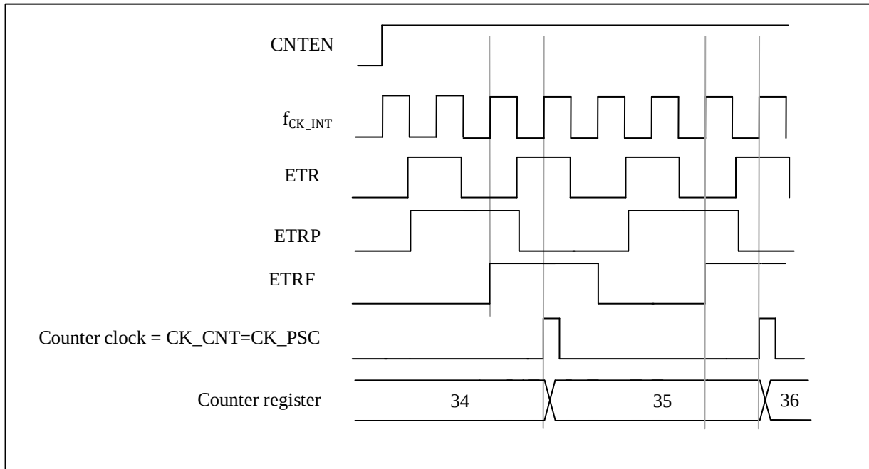
Figure 13-12 Control Circuit in External Clock Mode 2
