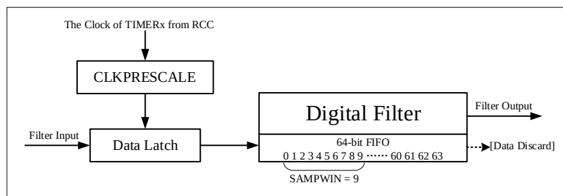
Figure 14-16 Sliding Filtering
