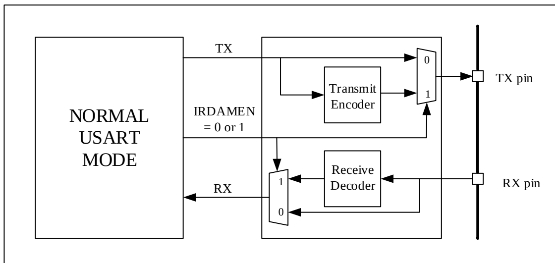
Figure 9-12 IrDA SIR ENDEC-Block Diagram
