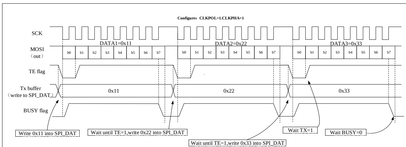
Figure 20-10 TE/BUSY Behavior in Non-Continuous Transmission (BIDIRMODE = 0 and ONLY = 0).
