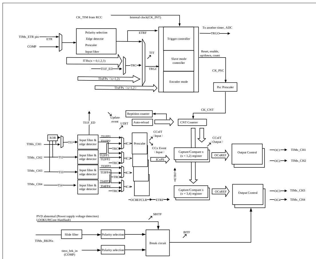
Figure 13-1 Block Diagram of TIM3
