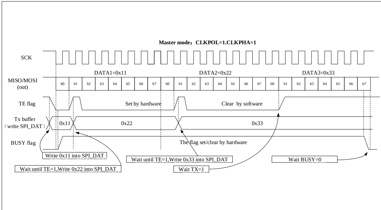
Figure 20-6 TXE/BSY Behavior in Master Transmit-Only Mode (BIDIRMODE = 0, RONLY = 0) in Case of Continuous Transfers
