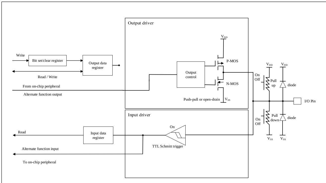
Figure 6-4 Alternate Function Mode (Fail-safe Not Supported)
