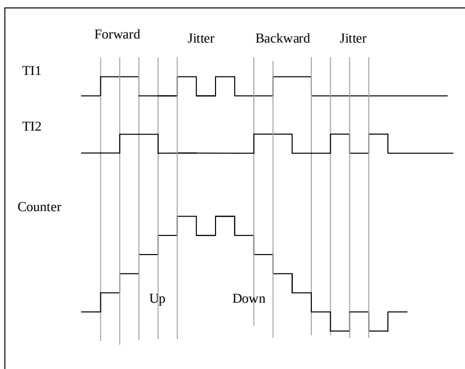
Figure 13-30 Example of Counter Operation in Encoder Interface Mode
