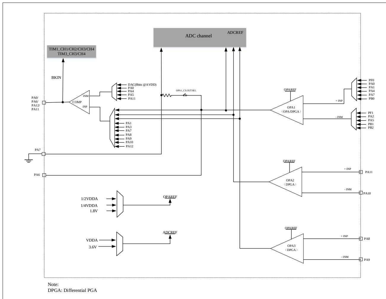
Figure 17-1 Comparator System Connection Diagram
