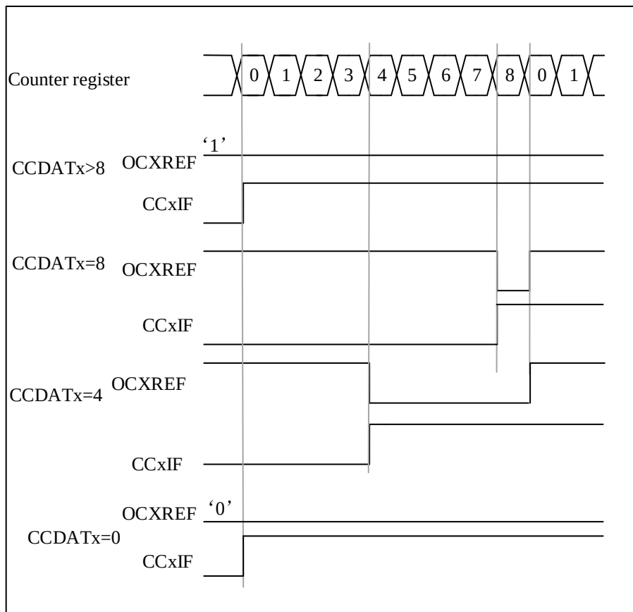
Figure 14-20 Edge-aligned PWM Waveform (APR=8)
