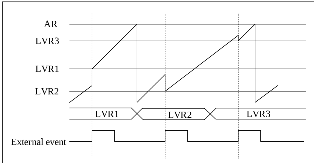
Figure 13-24 CNT counting method when an external event triggers LVR loading
