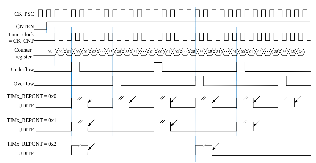
Figure 12-11 Repeat Count Sequence Diagram in Center-aligned Mode
