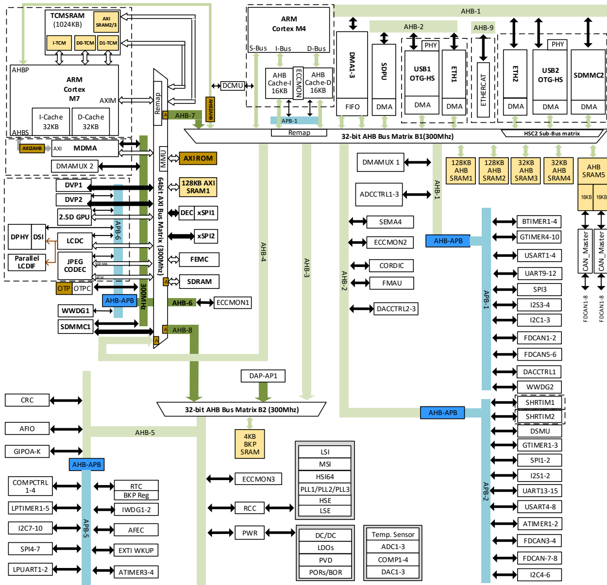
Figure 1-1 N32H785EC System Block Diagram
