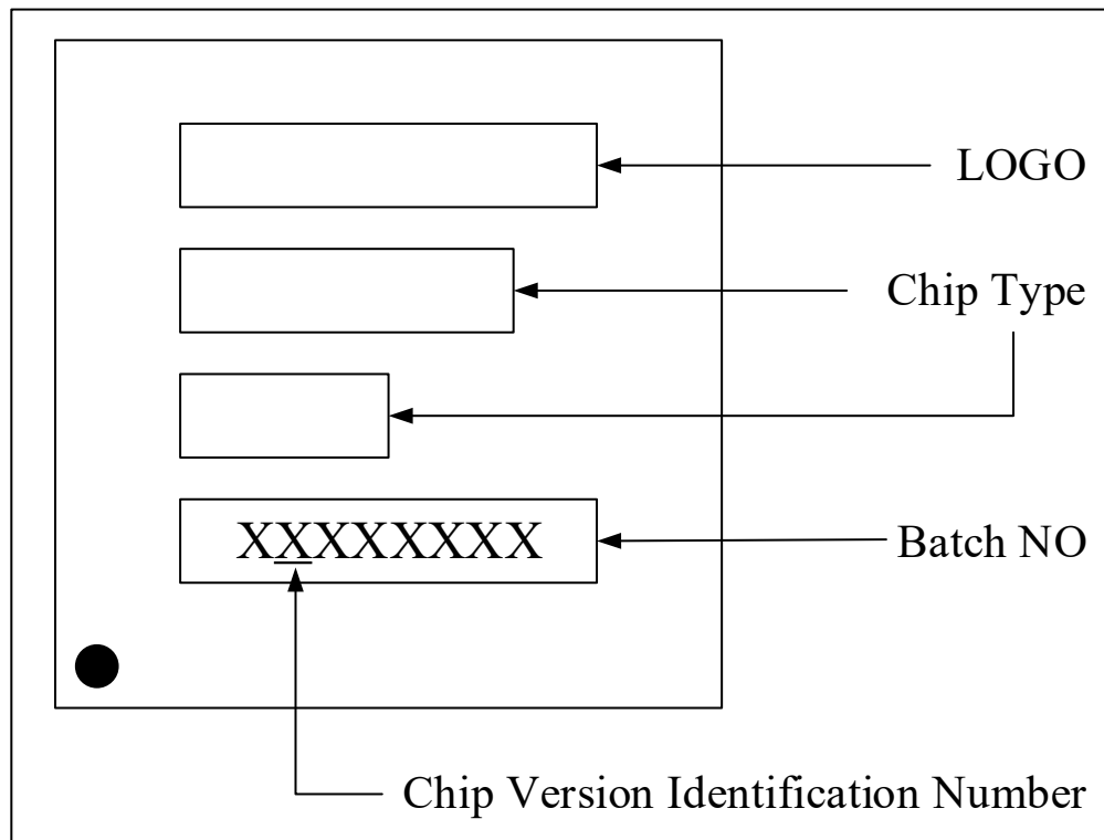
Figure 5-6 Silkscreen Diagram
