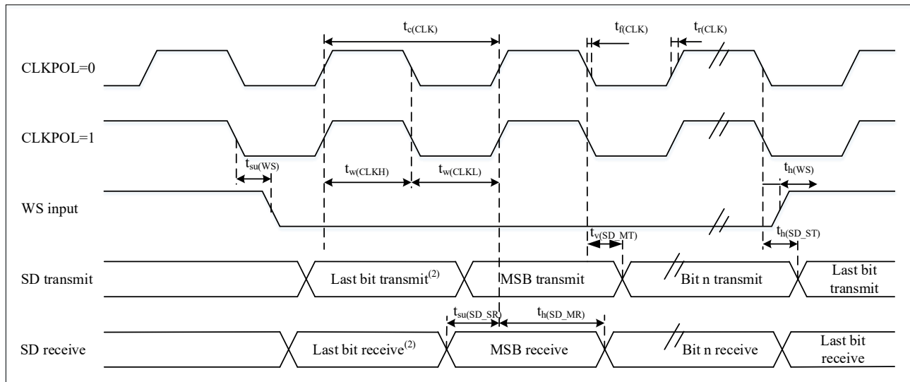
Figure 4-21 I2S Master Mode Timing Diagram (Philips Protocol) (1)
