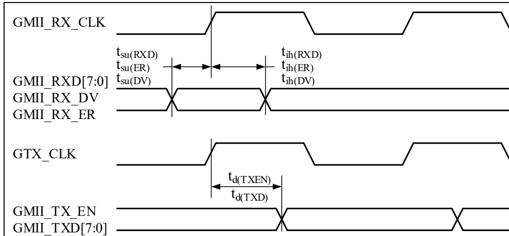
Figure 4-42 MII Timing Diagram
