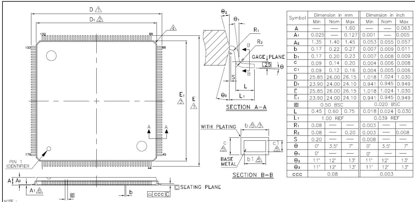
Figure 5-1 LQFP176 Package Dimensions
