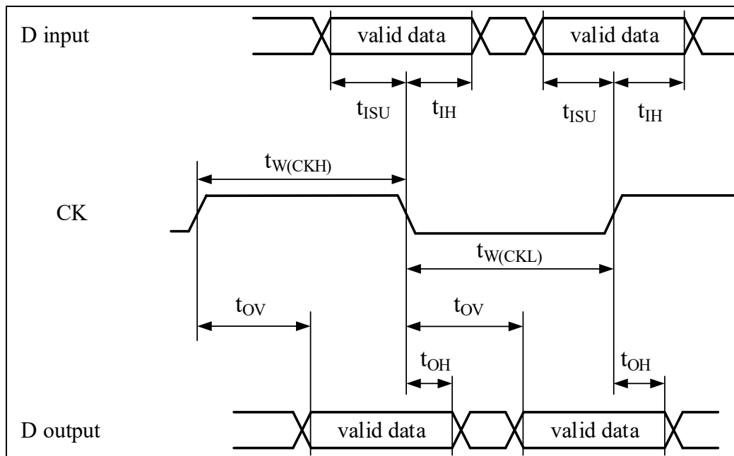
Figure 4-39 SDMMC DDR Mode
