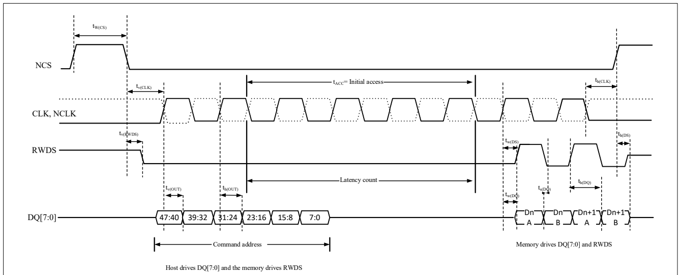
Figure 4-25 xSPI Hyperbus Clock Read Timing Diagram
