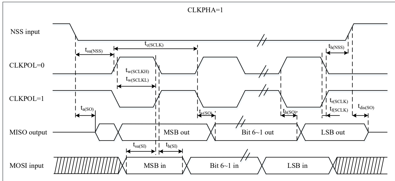
Figure 4-18 SPI Timing Diagram — Slave Mode and CLKPHA=1 (1)
