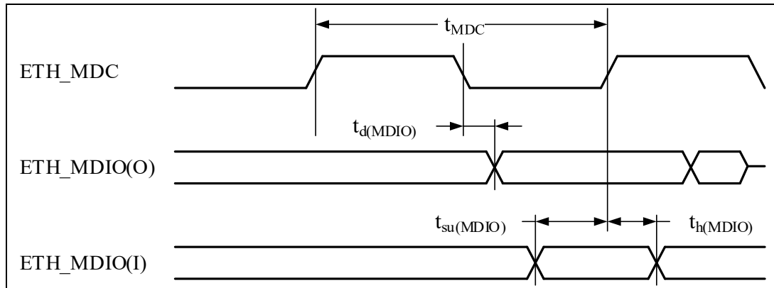
Figure 4-40 MDIO/SMA Timing Diagram
