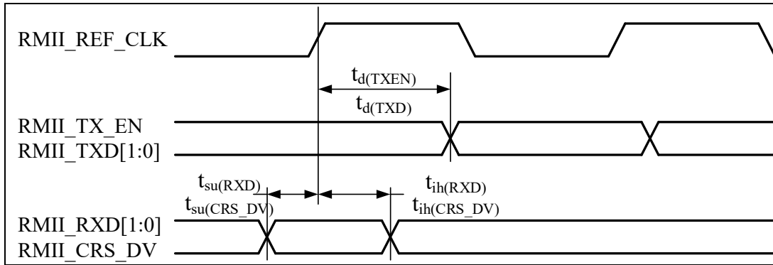
Figure 4-41 RMII Timing Diagram
