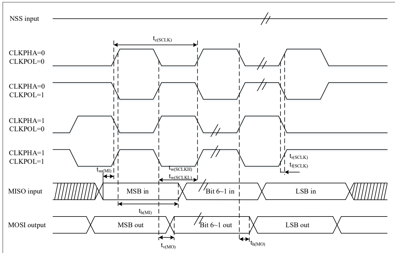
Figure 4-19 SPI Timing Diagram — Master Mode (1)
