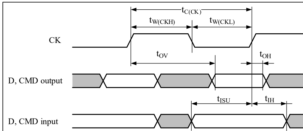
Figure 4-38 SDMMC DDR Mode
