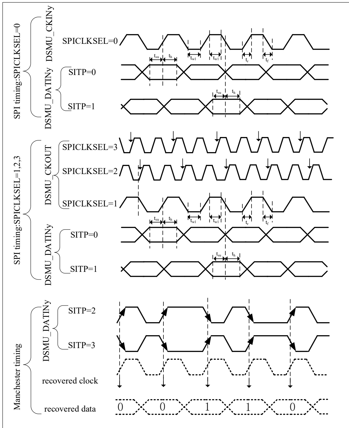
Figure 4-51 DSMU Channel Transceiver Timing Diagram
