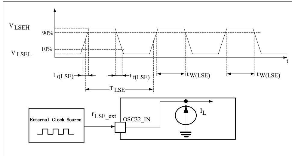
Figure 4-8 Low-speed external clock source AC timing diagram
