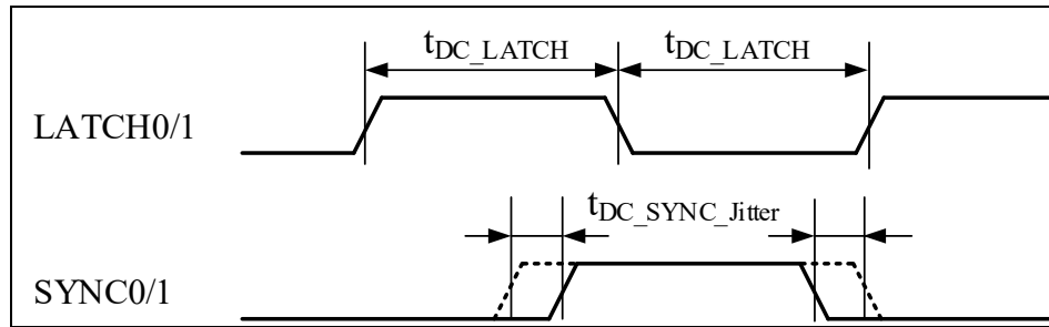
Figure 4-47 ESC Sync/Latch Timing Diagram
