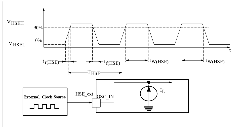
Figure 4-7 High-speed external clock source AC timing diagram
