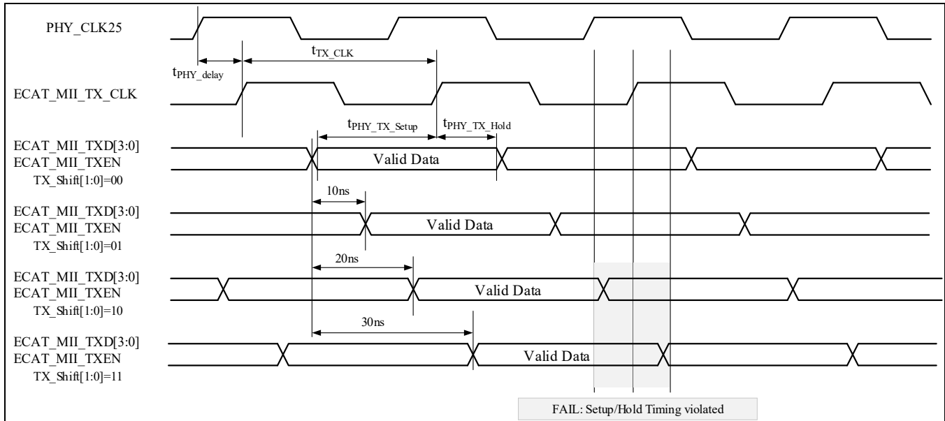
Figure 4-45 ESC MII TX Signal Timing Diagram
