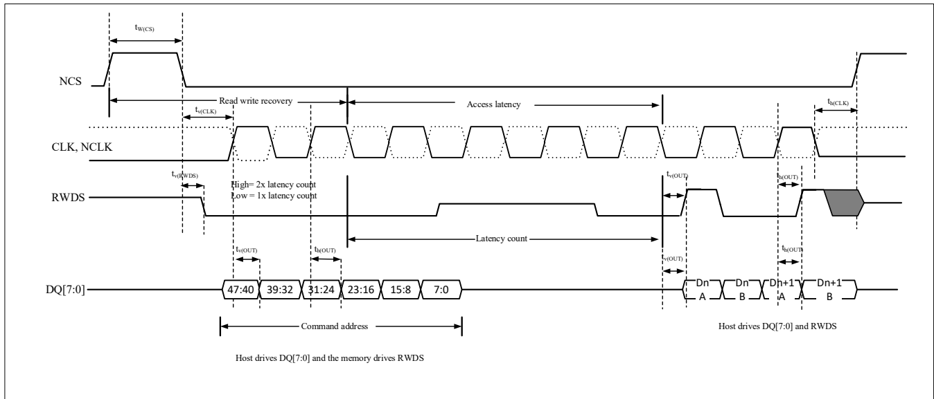
Figure 4-26 xSPI Hyperbus Clock Write Timing Diagram4-1 xSPI Hyperbus
