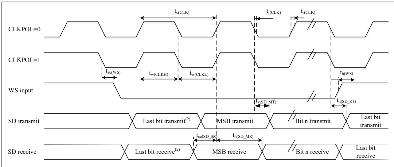
Figure 4-20 I2S Slave Mode Timing Diagram (Philips Protocol) (1)
