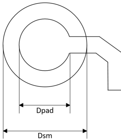
Figure 5-4 Recommended Pads for BGA240+25 Package
