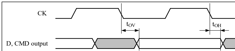
Figure 4-39 SDMMC DDR Mode
