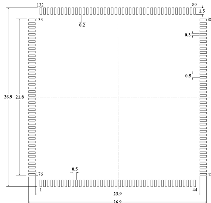
Figure 5-2 Suggestions for LQFP176 Package Pads (1)
