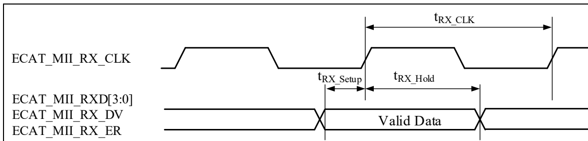
Figure 4-46 ESC MII RX Signal Timing Diagram
