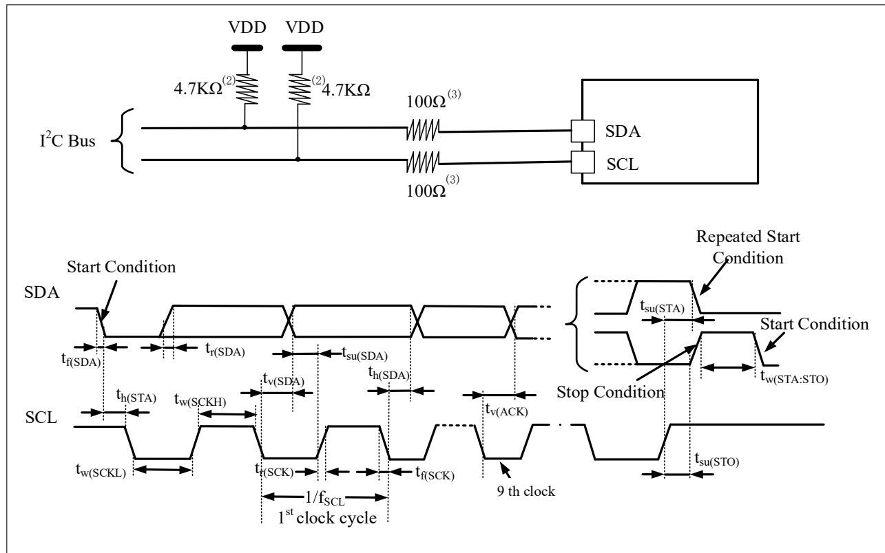
Figure 4-16 I 2 C Bus AC Waveform and Measurement Circuit (1)
