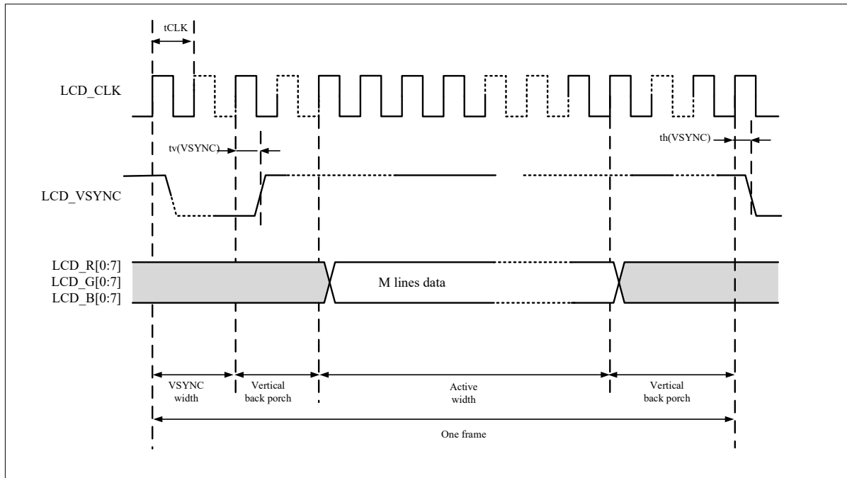
Figure 4-50 LCD-TFT vertical timing diagram
