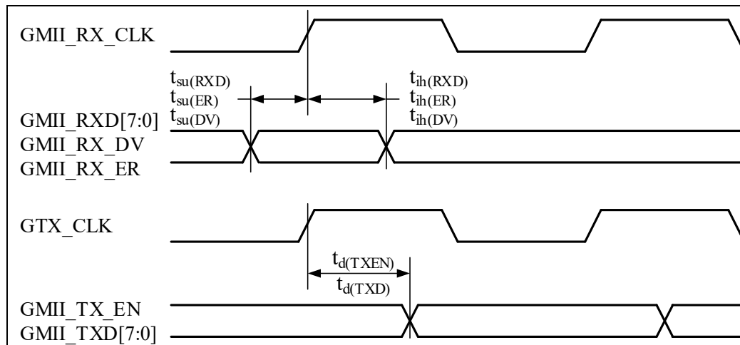
Figure 4-43 GMII Timing Diagram
