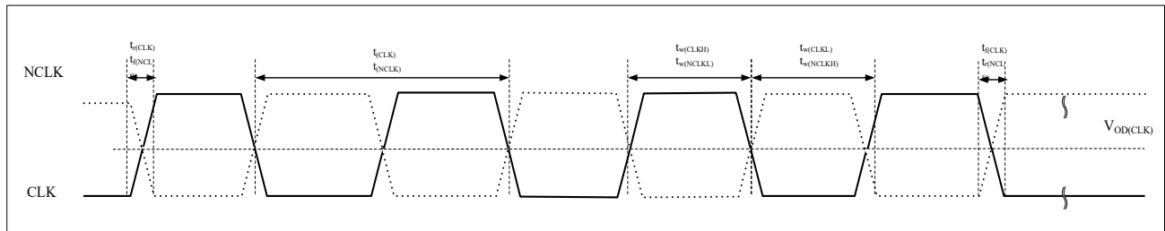
Figure 4-25 xSPI Hyperbus Clock Read Timing Diagram
