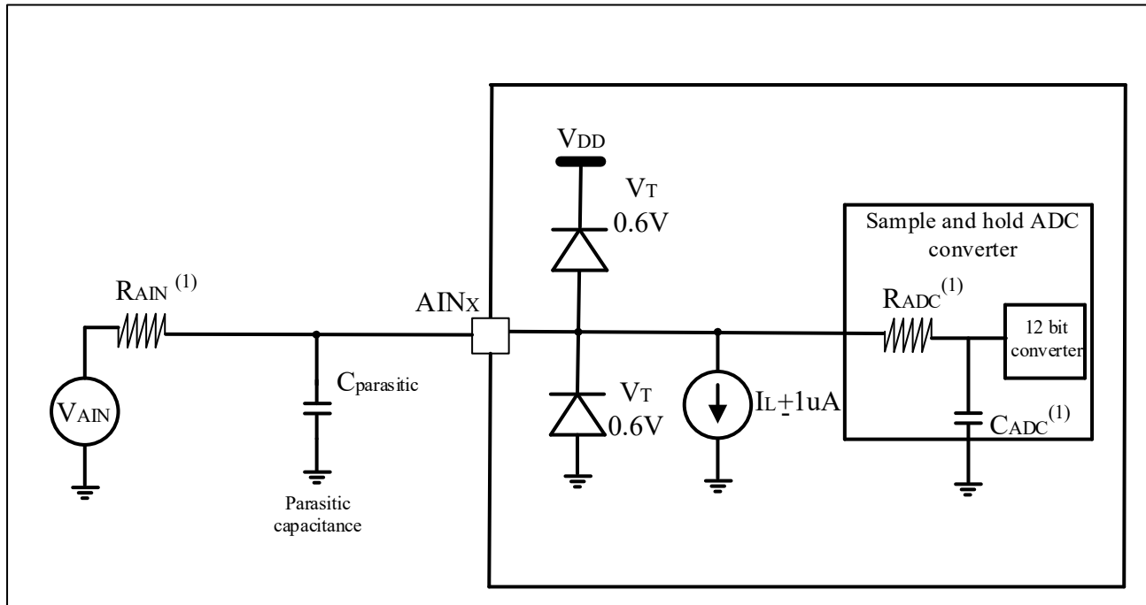
Figure 4-53 Typical Connection Diagram Using ADC
