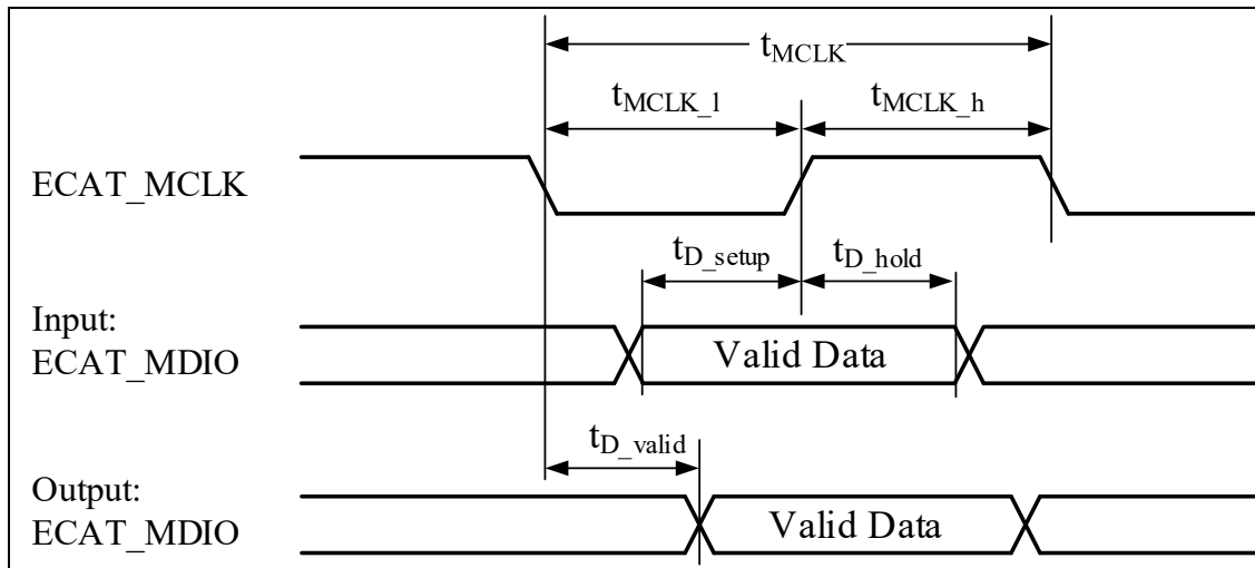
Figure 4-44 MI (MCLK, MDIO) Timing Diagram
