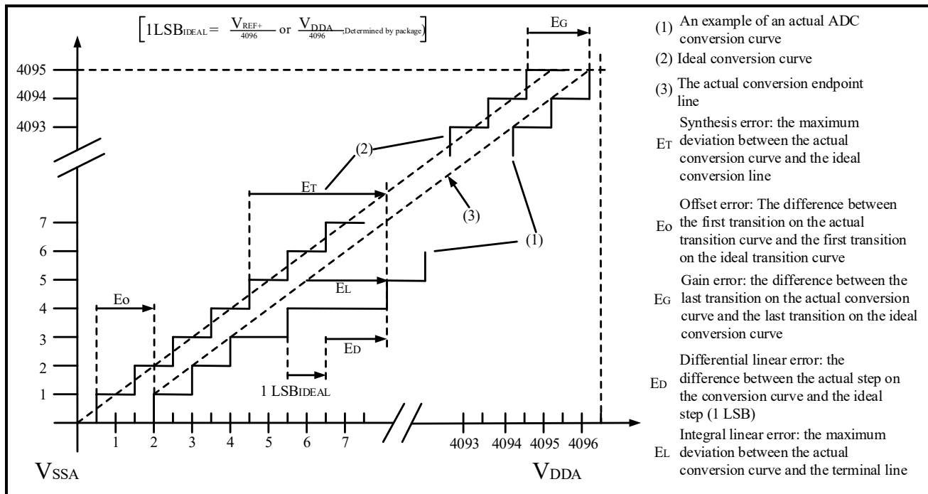
Figure 4-52 ADC Accuracy Characteristics
