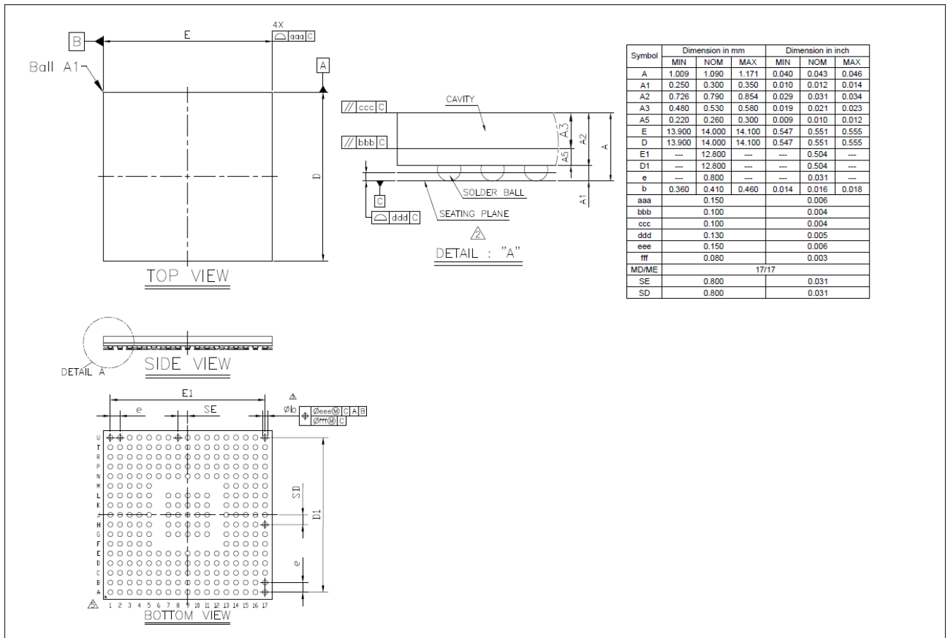
Figure 5-3 BGA240+25 Package Dimension
