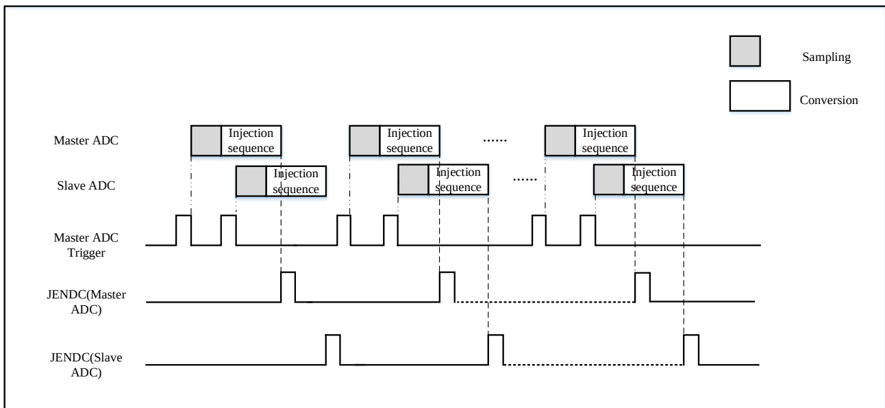
Figure 17-29 Alternate trigger: injection channel group
