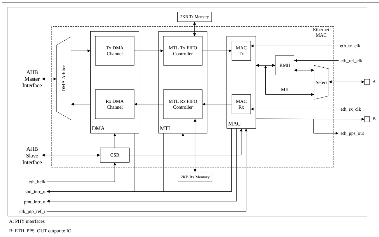
Figure 34-1 Ethernet Architecture Diagram
