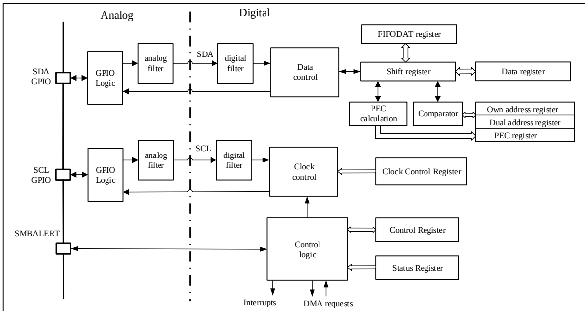
Figure 22-1 I2C Functional Block Diagram
