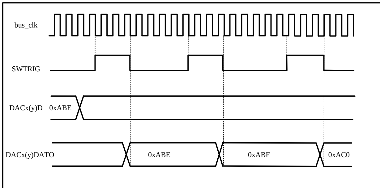
Figure 18-8 DAC Conversion with Triangular Wave Generation (Enable Software Trigger, HFSEL[1:0] = 0b'01)
