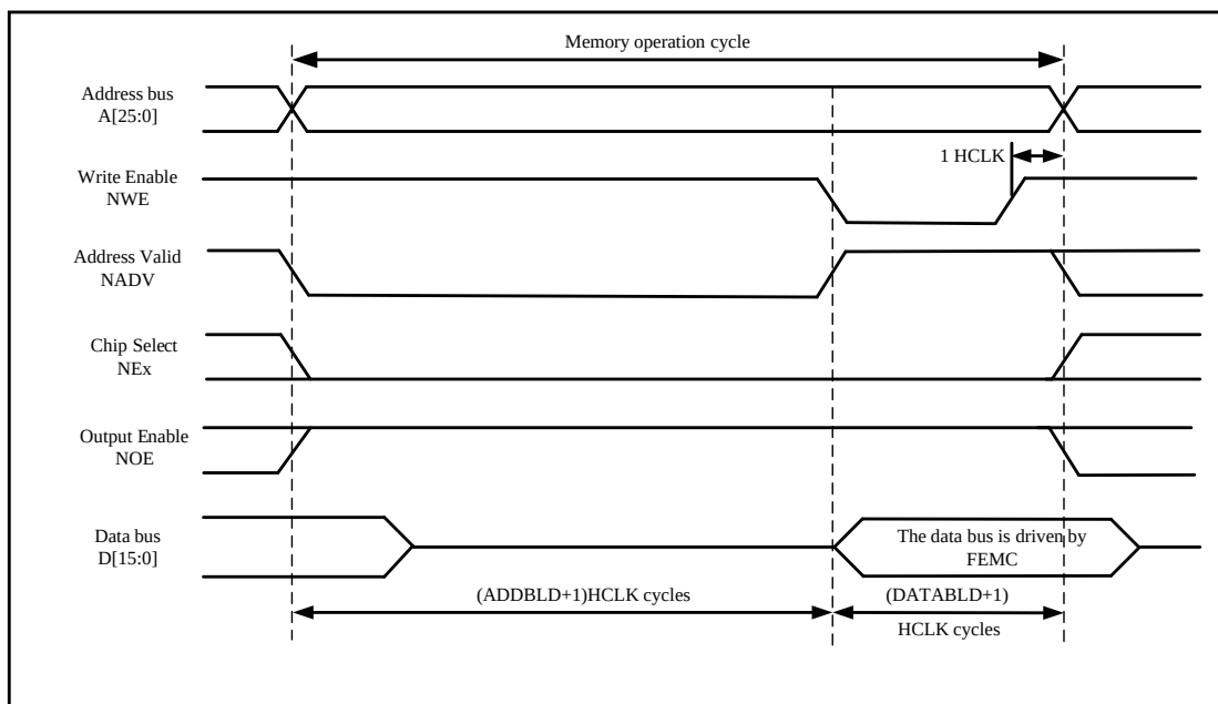
Figure 28-9 Mode B Write Accesses
