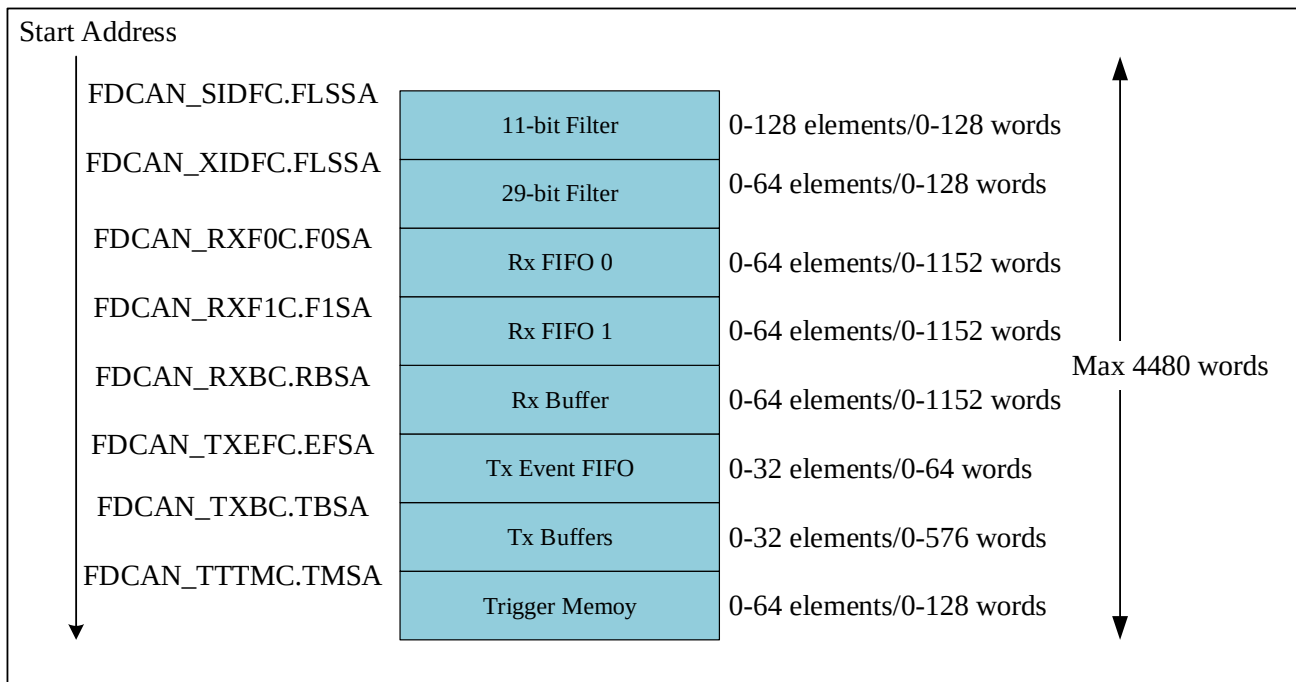
Figure 23-1 Example diagram of FDCAN Message RAM allocation
