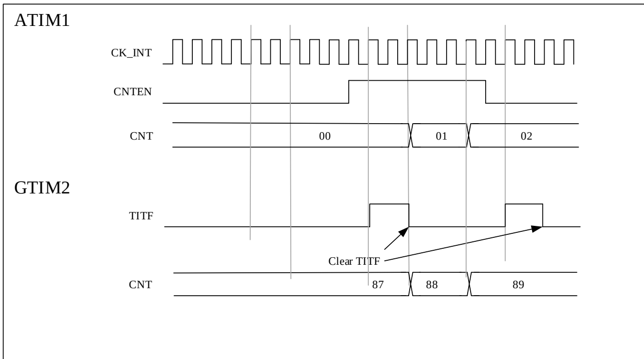
Figure 11-30 GTIM2 Gated By Enable Signal Of TIM1
