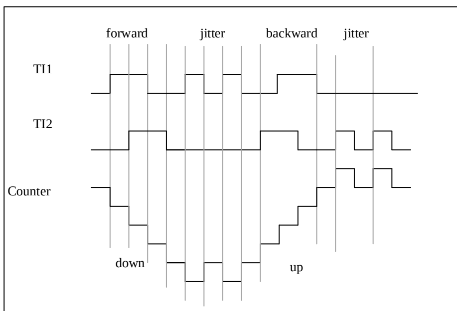
Figure 9-50 Encoder Interface Mode Example with IC1FP1 Polarity Inverted
