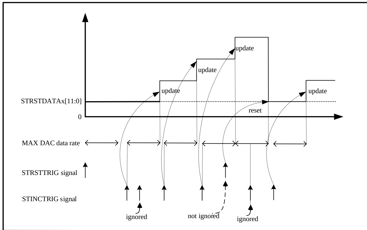
Figure 18-10 DAC Increasing Sawtooth Wave Reset Signal Trigger Priority over Step Trigger
