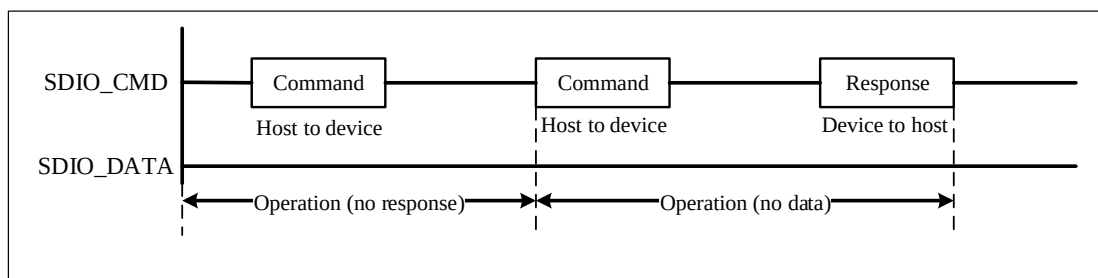
Figure 30-1 SDIO "No Response" And "No Data" Operations
