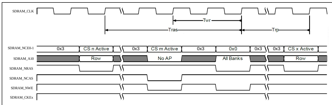
Figure 29-13 Precharge All SDRAM Banks
