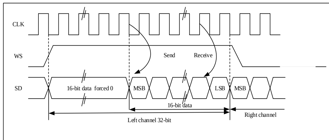
Figure 26-24-27 LSB Aligned 16-Bit Data Is Extended to 32-Bit Packet Frame, CLKPOL = 0
