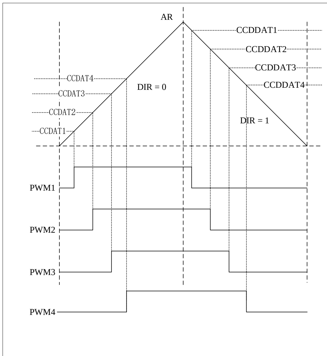
Figure 12-8 Output WaveformCorrespo Asymmetric Mode
