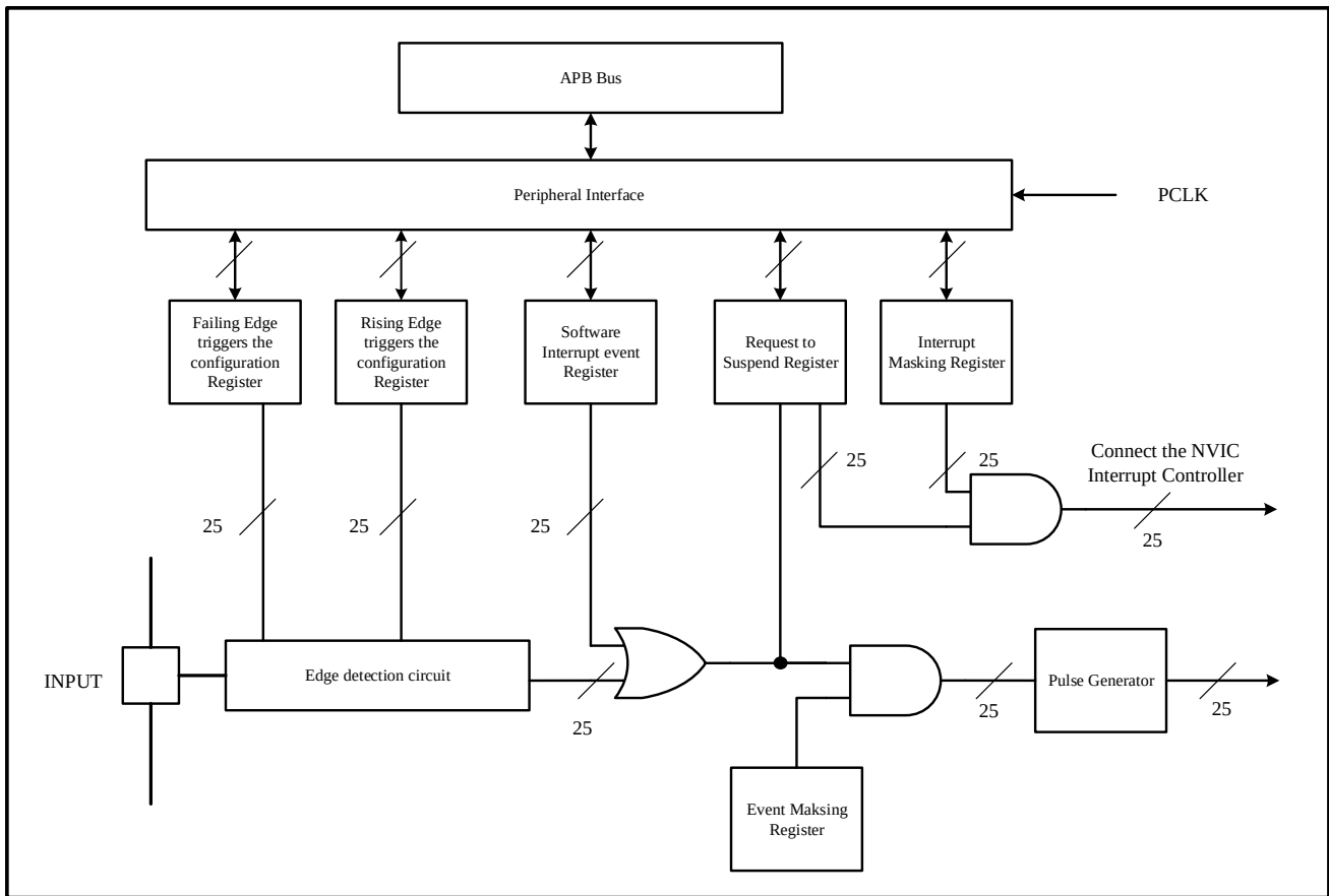
Figure 6-1 External Interrupt/Event Controller Block Diagram
