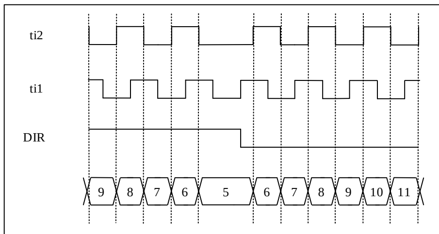
Figure 10-35 The Encoder Counts on Both TI1 and TI2
