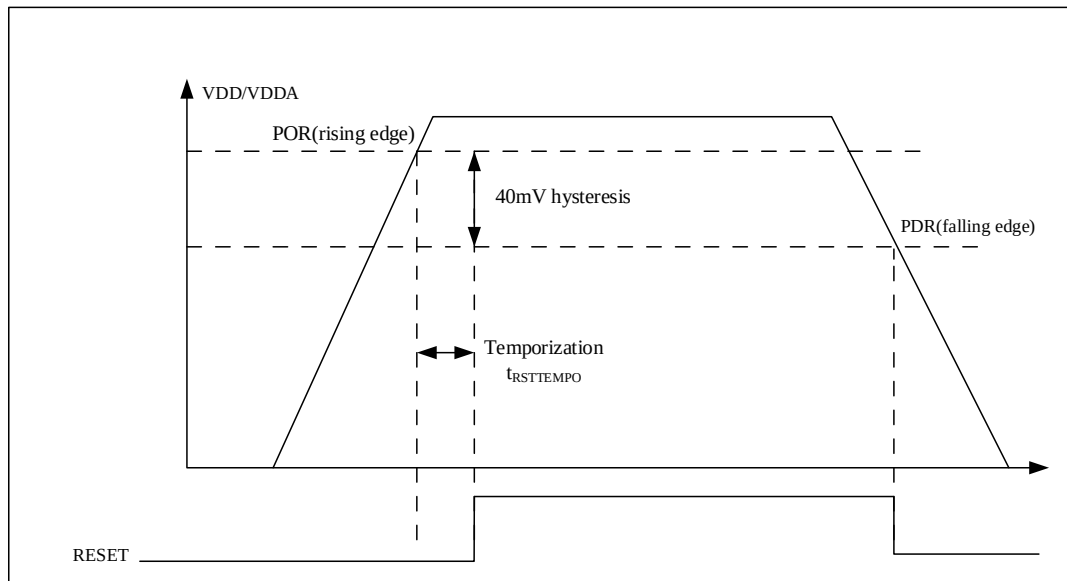
Figure 3-2 Power On Reset and Power Down Reset Waveform
