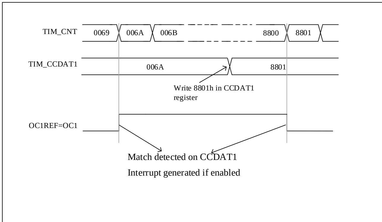
Figure 11-18 Output Compare Mode, Toggle On OC1
