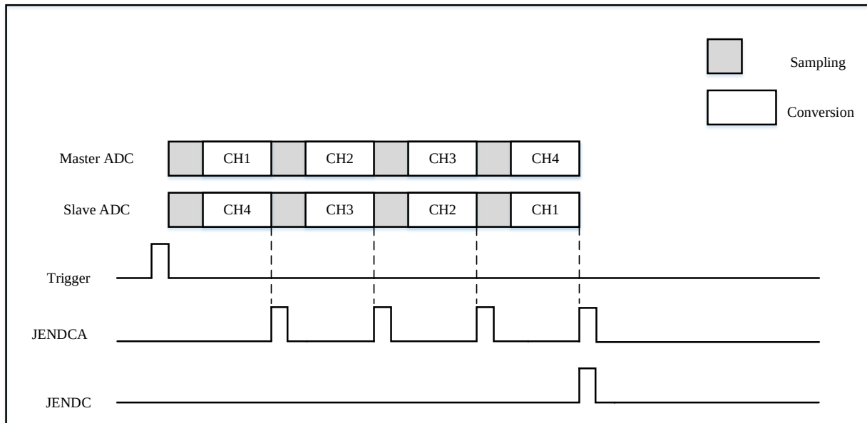
Figure 17-25 Synchronous Injection Mode with 4 channels for dual ADCs
