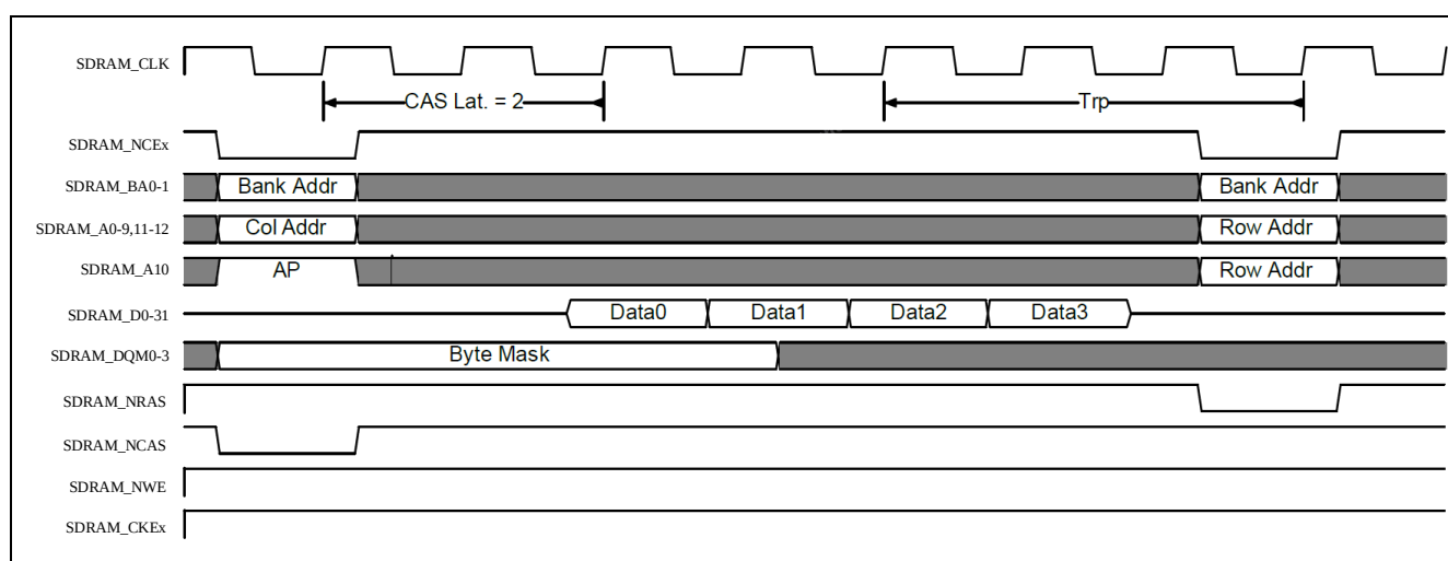
Figure 29-11 Burst SDRAM read with Auto Precharge
