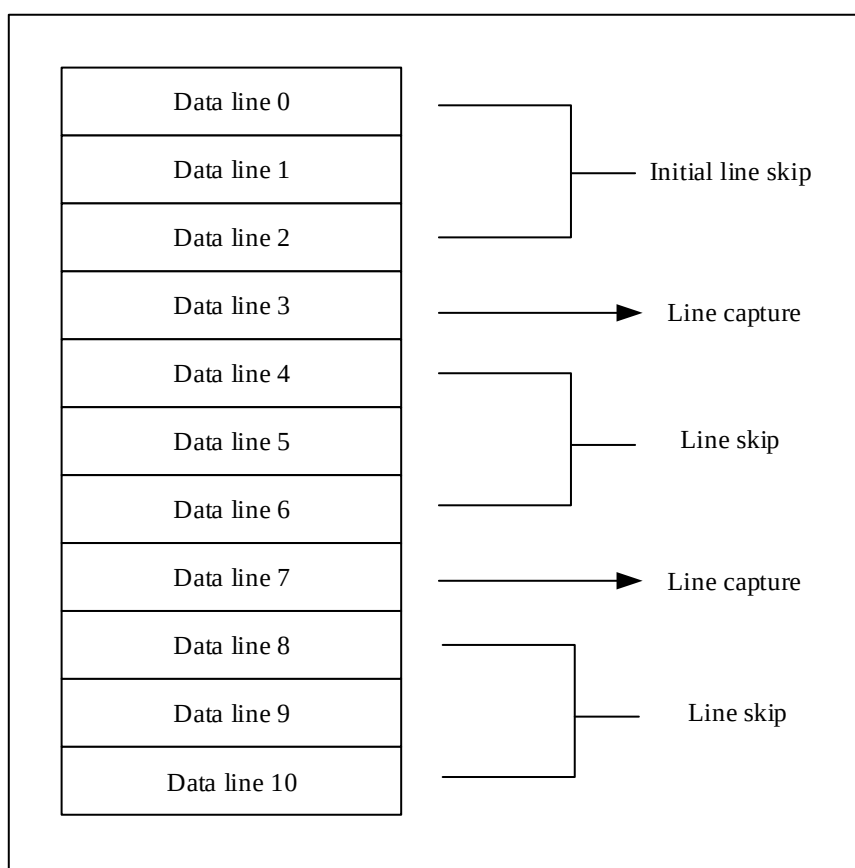
Figure 30-6 Line Skip Function(HISKIP=3, HRSKIP=3)
