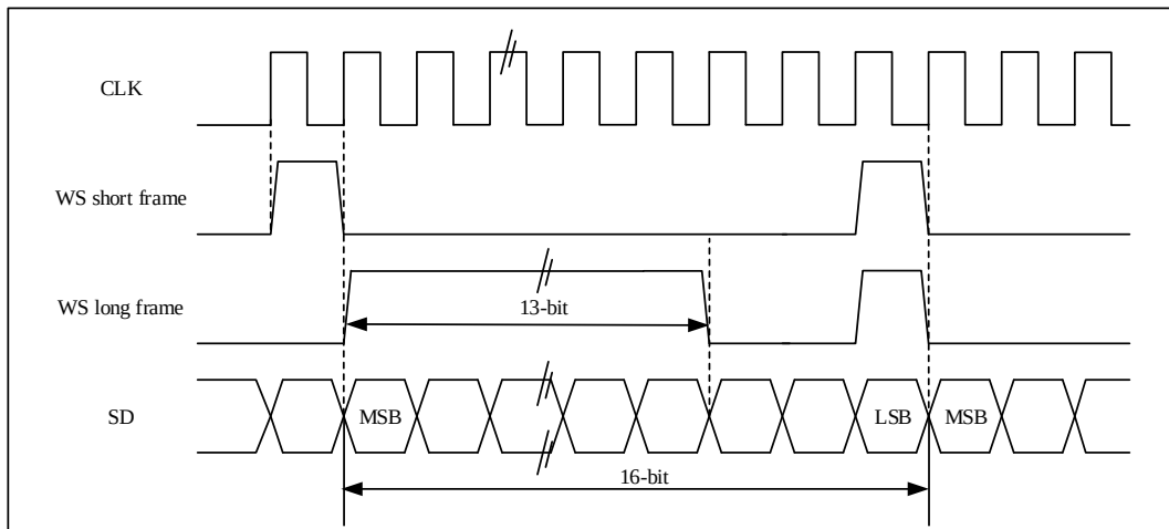
Figure 26-24-29 PCM Standard Waveform (16-Bit Extended to 32-Bit Packet Frame)
