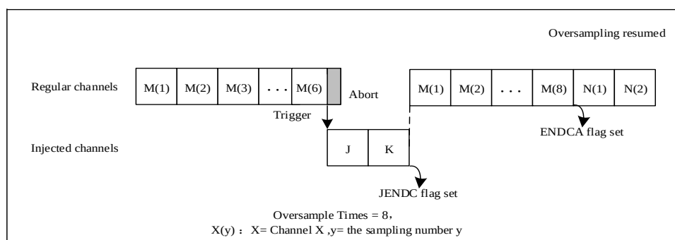
Figure 17-18 Regular Oversampling Reset Mode
