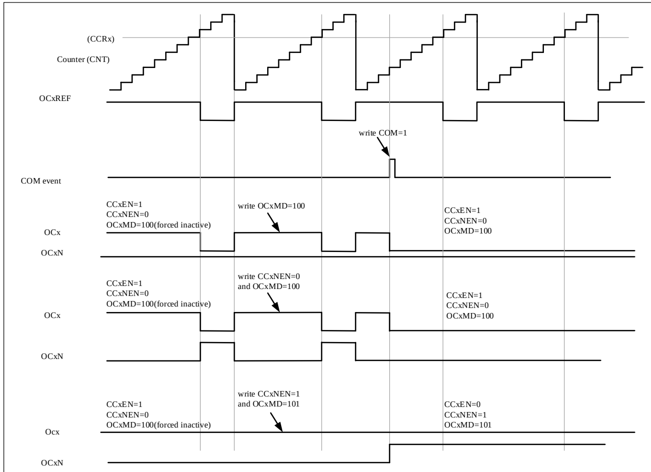
Figure 9-43 6-Step PWM Generation, COM Example (OSSR=1)
