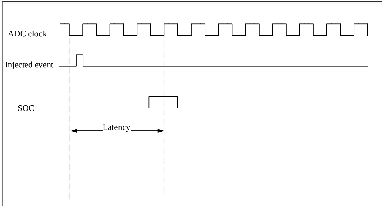
Figure 17-6 Injected Conversion Delay
