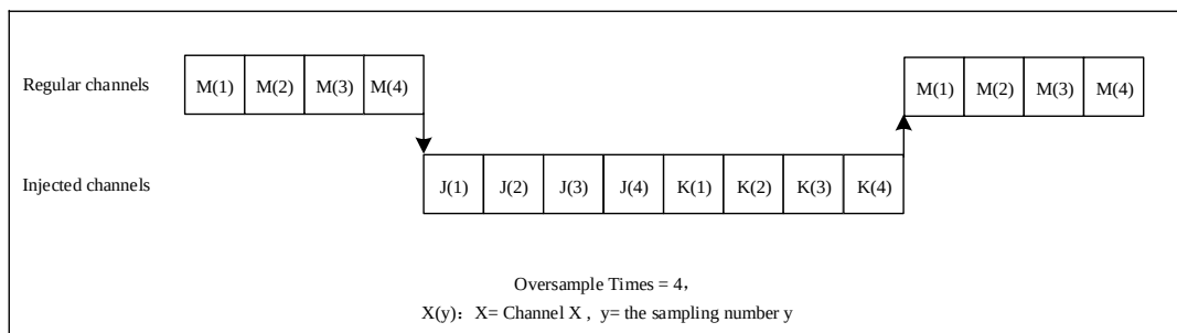
Figure 17-21 Oversampling in Automatic Injection Mode
