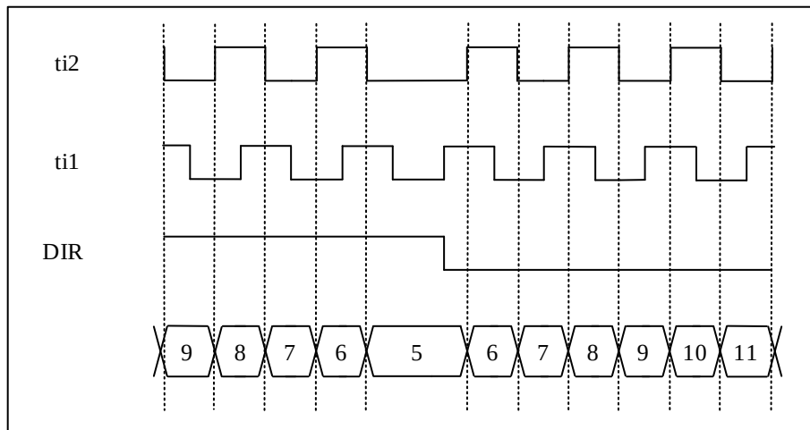
Figure 12-44 The Encoder Counts On Both TI1 and TI2
