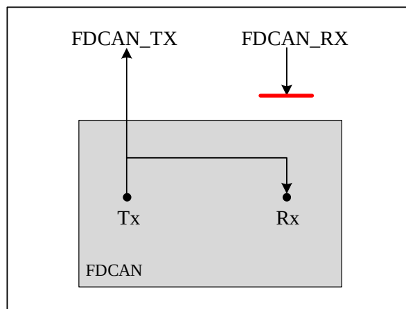
Figure 23-5 FDCAN External Loopback Mode Pin Control
