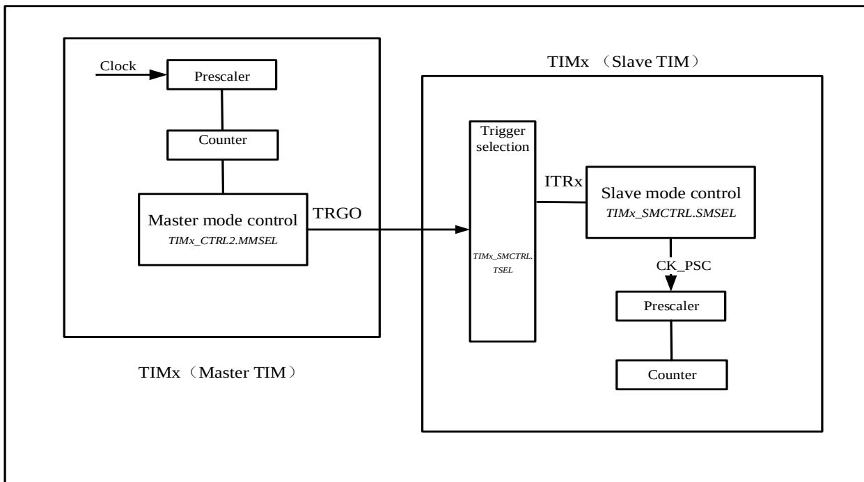
Figure 11-28 Master/Slave Timer Connection
