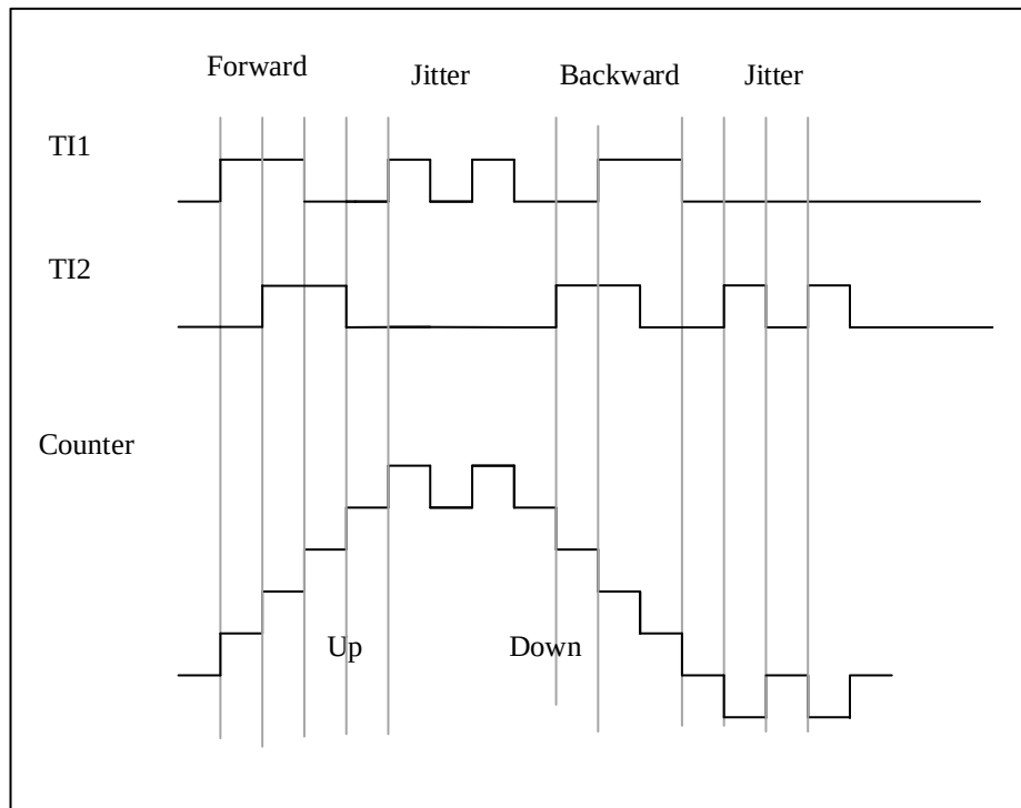
Figure 11-38 Example Of Counter Operation In Encoder Interface Mode
