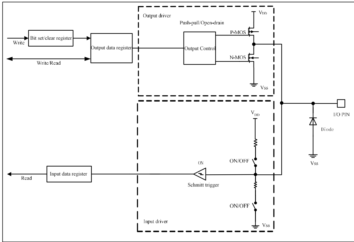
Figure 5-3 Output Mode Configuration
