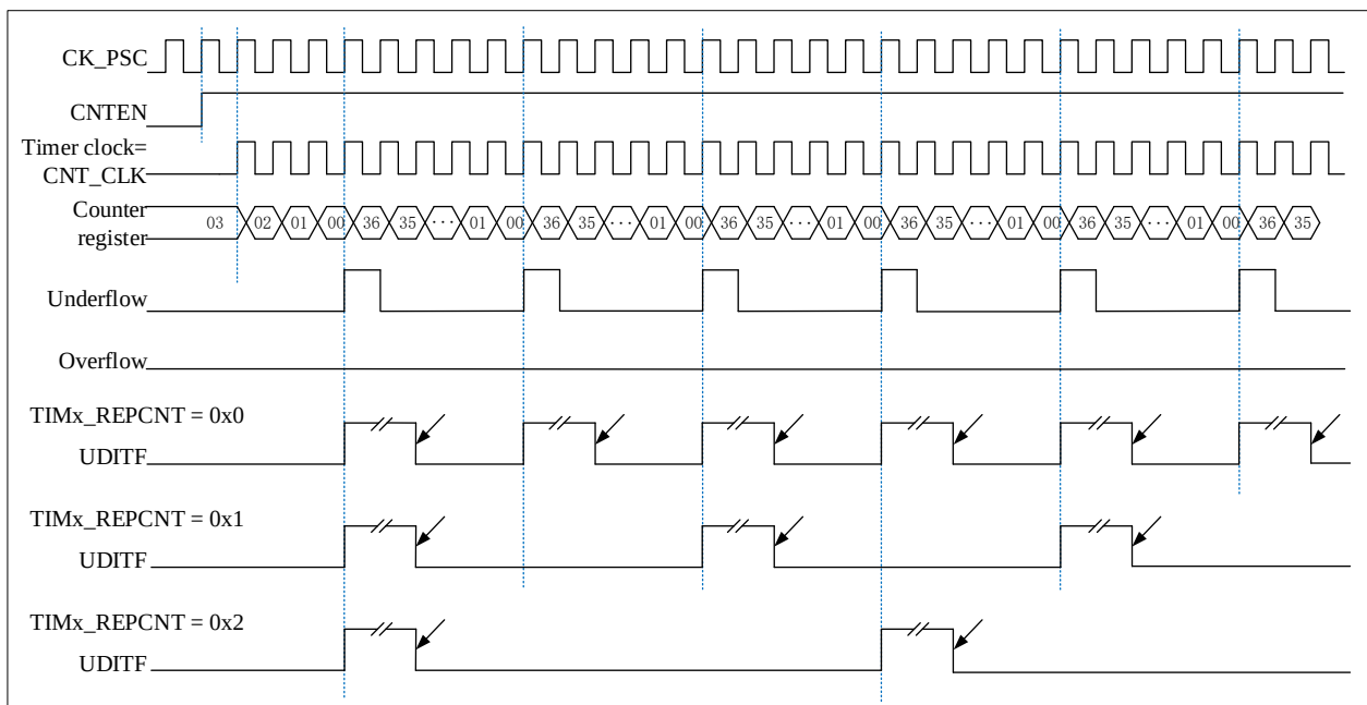
Figure 12-9 Timing diagram of the repetition counter in down-count mode
