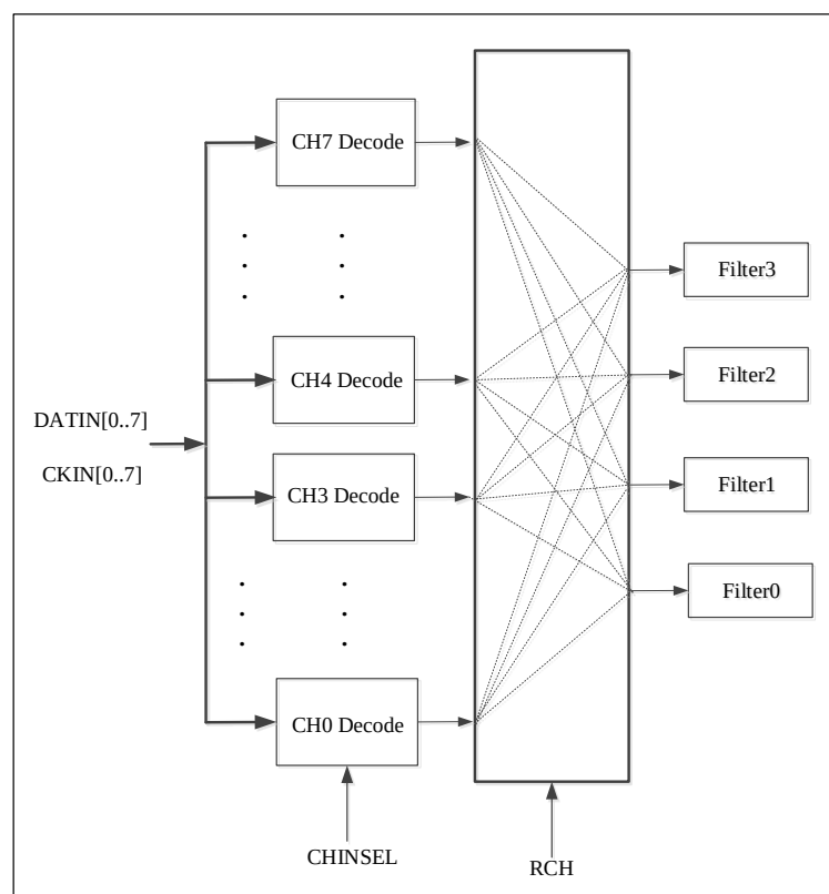
Figure 31-2 DSMU channel mux
