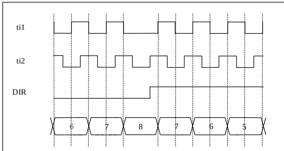
Figure 9-48 The Counter Counts Only on TI2 When TI1 is High
