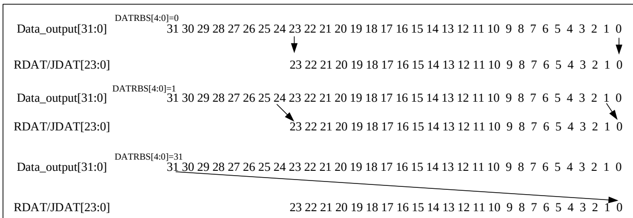
Figure 31-6 Data right bit shift example
