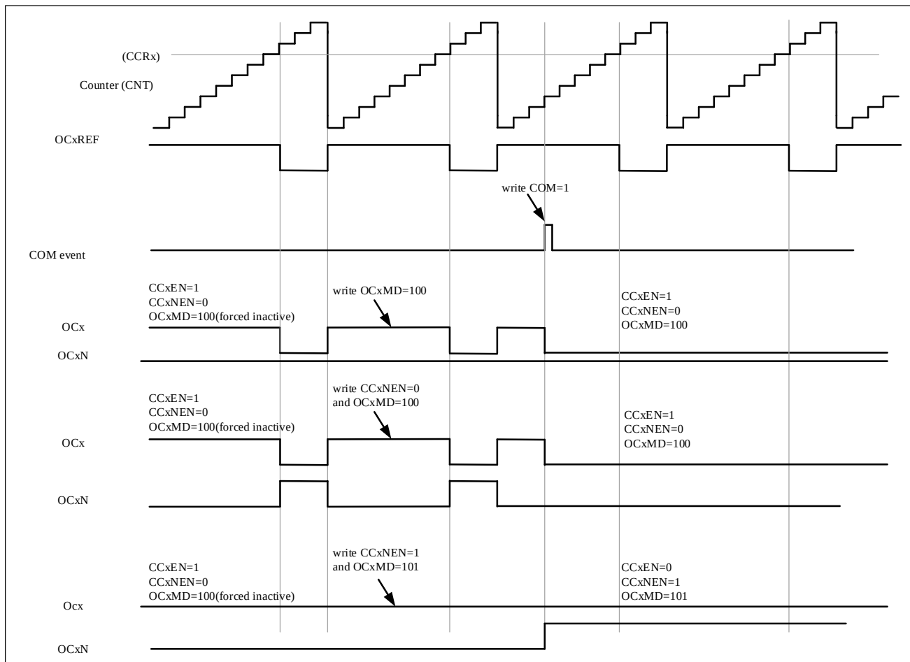
Figure 12-41 Generating Six-Step PWM Using COM as Example (OSSR=1)
