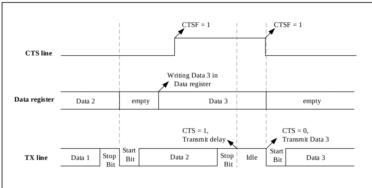
Figure 21-11 CTS Flow Control
