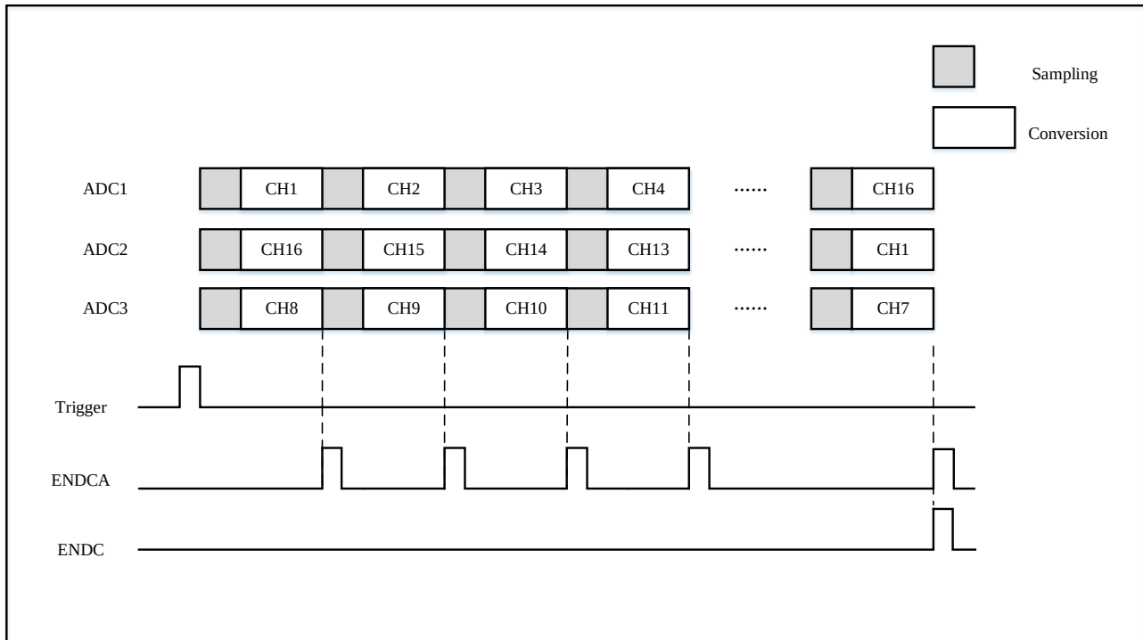
Figure 17-24 Synchronous regular mode with 16 channels
