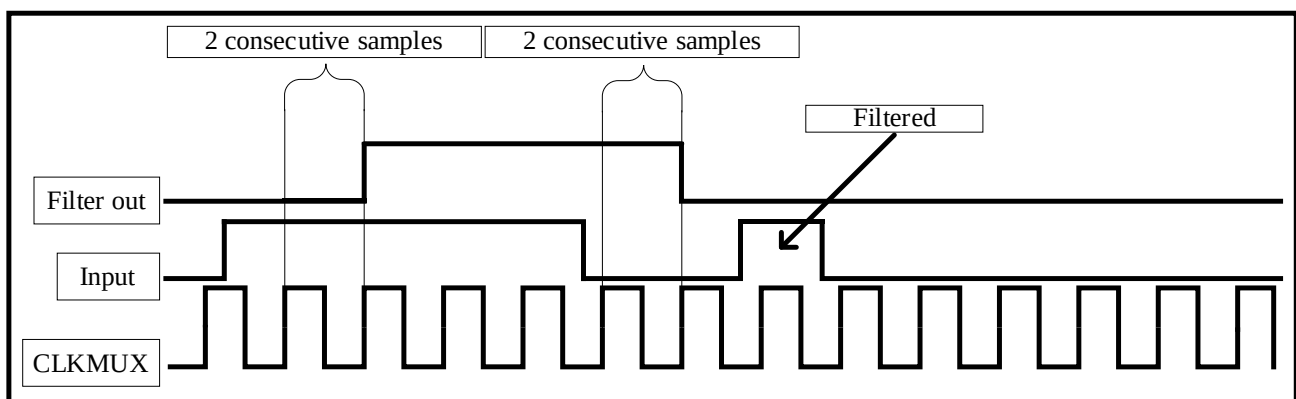
Figure 14-2 Glitch Ffilter Timing Diagram
