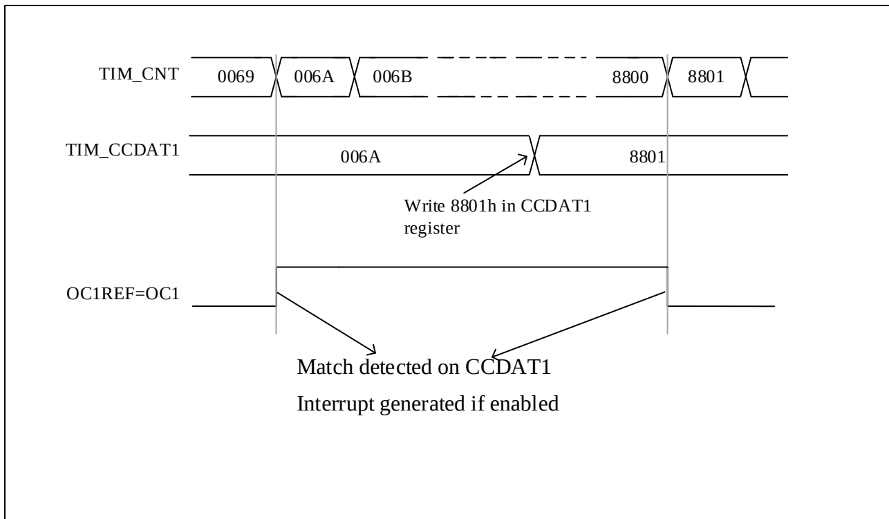
Figure 12-22 Output Compare Mode, Toggle On OC1
