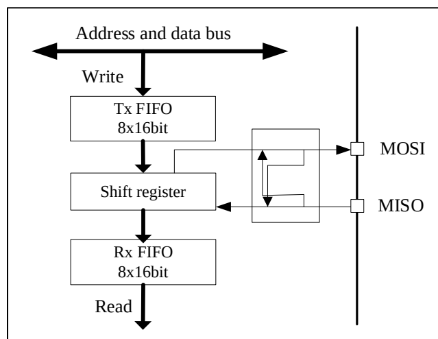
Figure 26-24-13 Reception Using DMA
