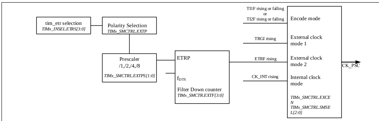
Figure 9-18 External Trigger Input Block Diagram
