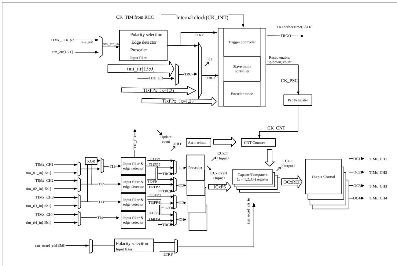
Figure 10-1 Block Diagram Of GTIMx (x=1,4)
