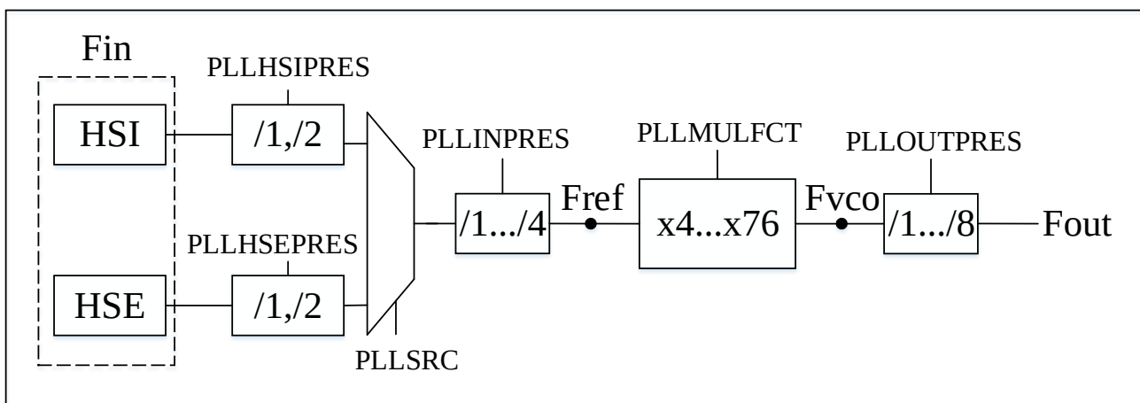
Figure 4-4 PLL Clock Source Selection
