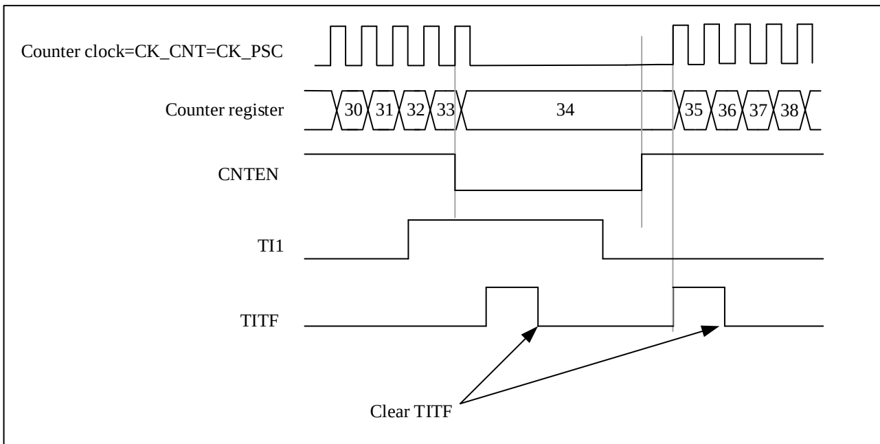
Figure 9-39 Control Circuit in Gated Mode
