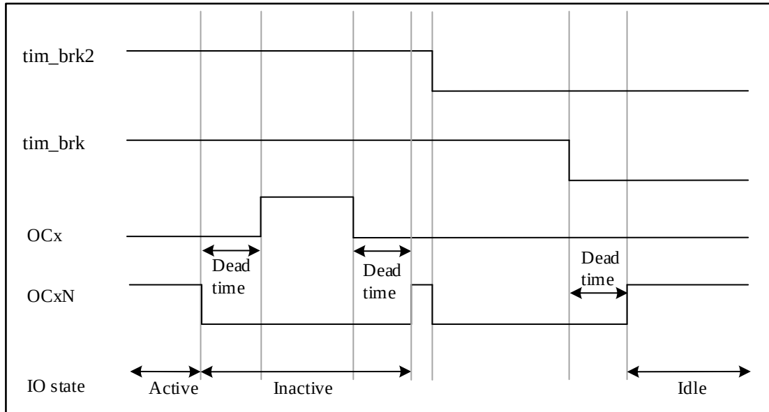
Figure 9-34 PWM Output State Following tim_brk Assertion (OSSI=0)
