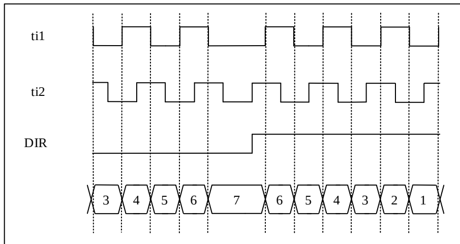
Figure 12-43 The Encoder Counts Only On TI2
