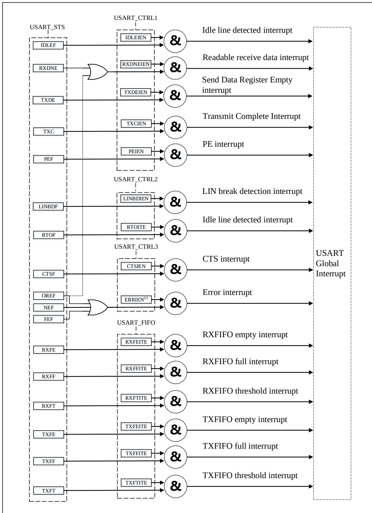
Figure 21-24 USART Interrupt Request
