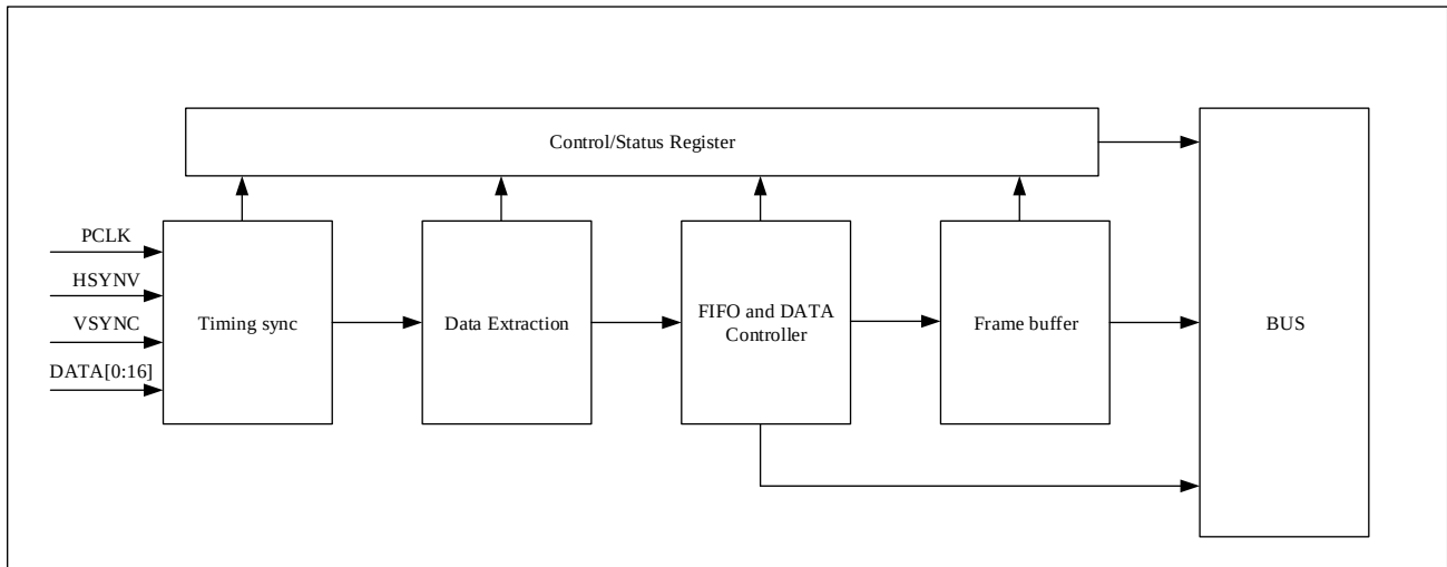
Figure 30-1 DVP Block Diagram
