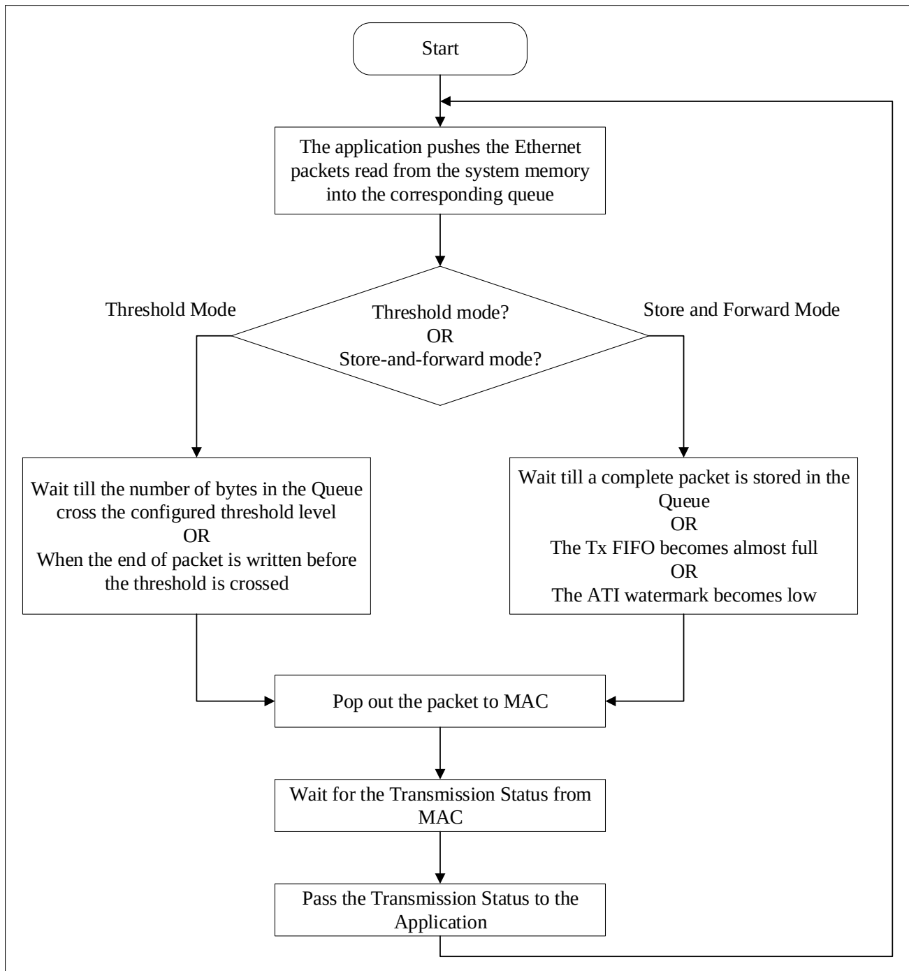
Figure 34-5 MTL Single Packet Transmit Flow
