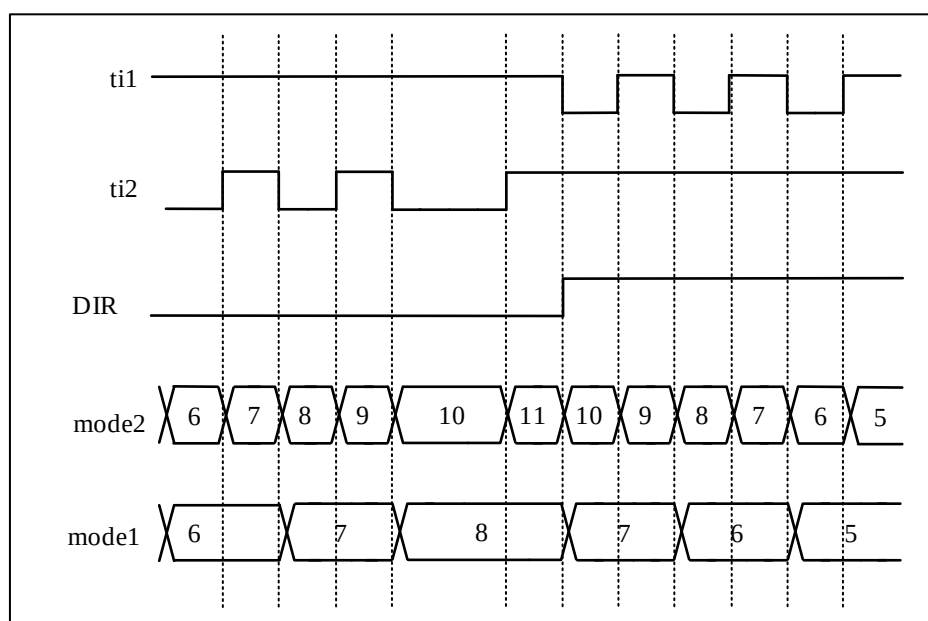
Figure 11-41 Dual Pulse Encoding Mode (CC1P = CC2P = 0)
