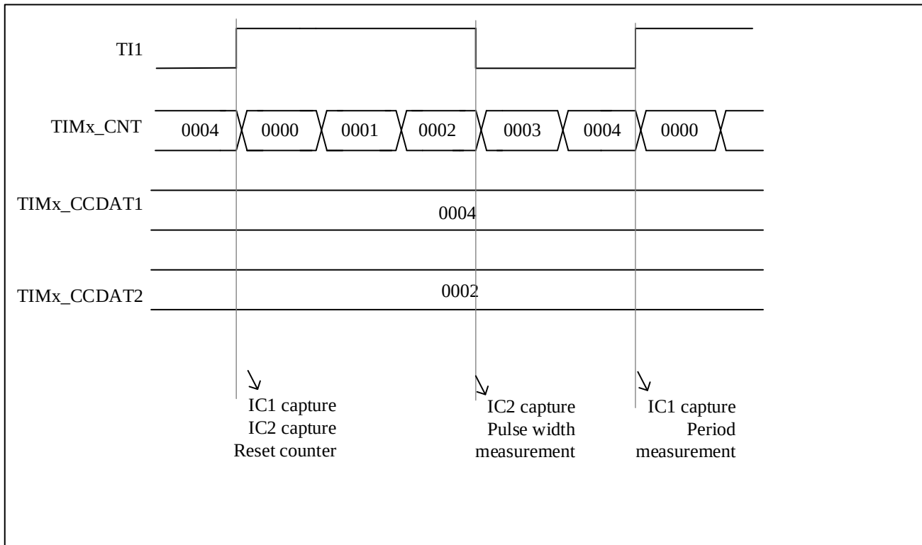
Figure 12-21 PWM Input Mode Timing
