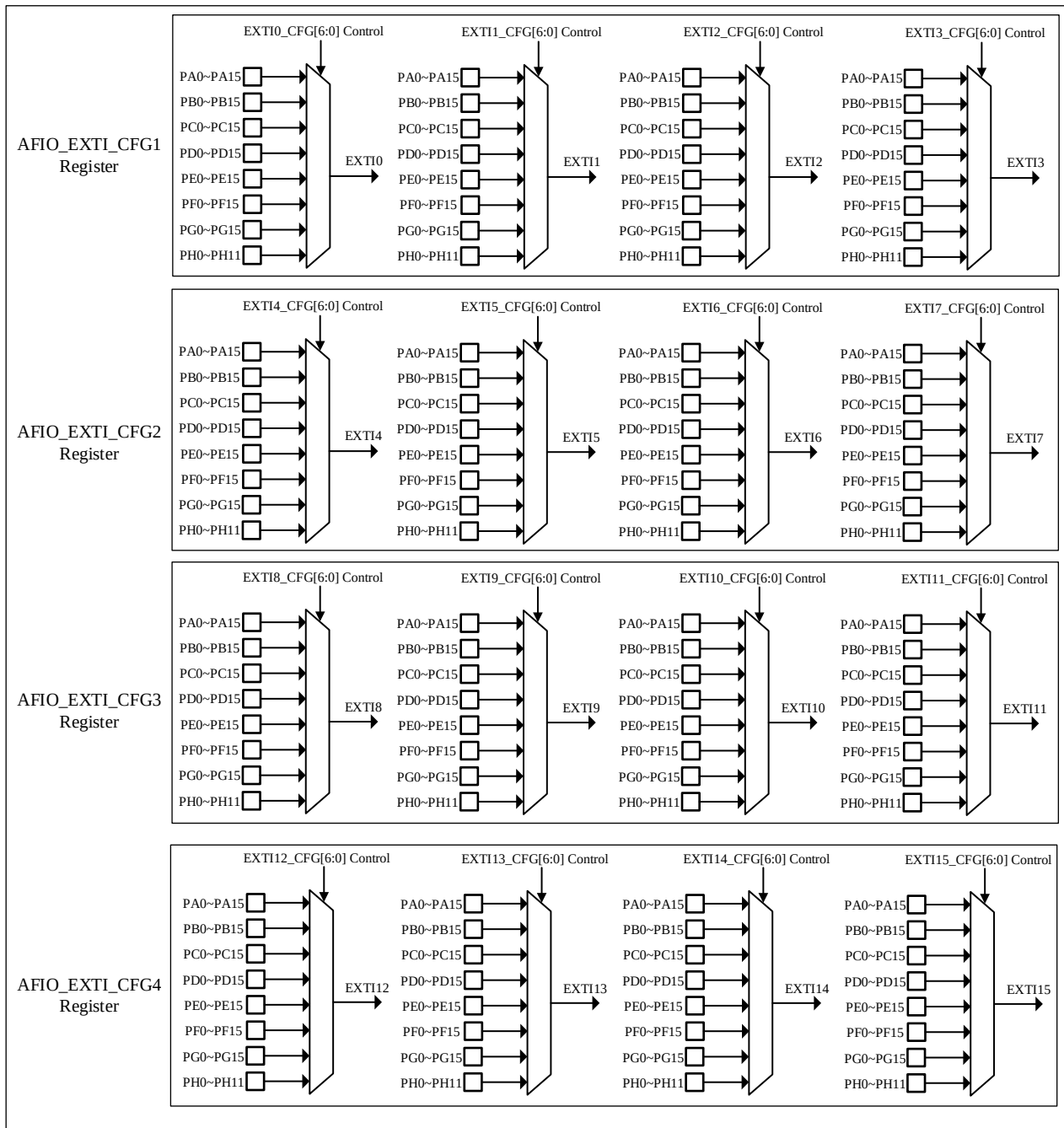
Figure 6-2 External Interrupt Generic I/O Mapping
