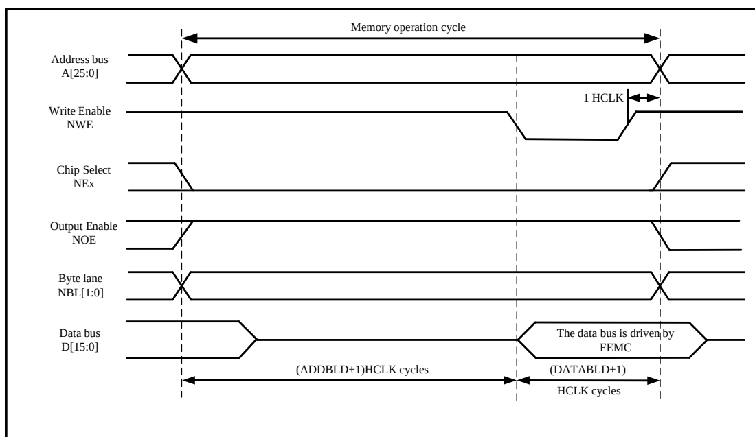
Figure 28-4 Mode1 Write Accesses
