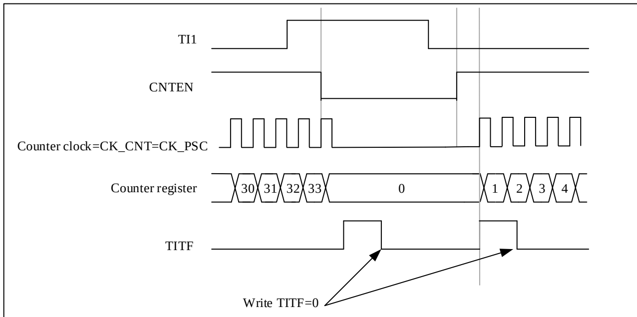
Figure 9-42 Control Circuit in Combined Gated + Reset Mode
