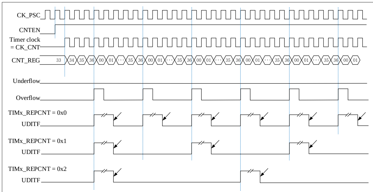
Figure 12-10 Timing diagram of the repetition counter in up-count mode
