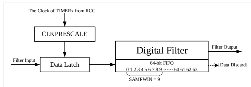
Figure 11-16 Sliding Filtering
