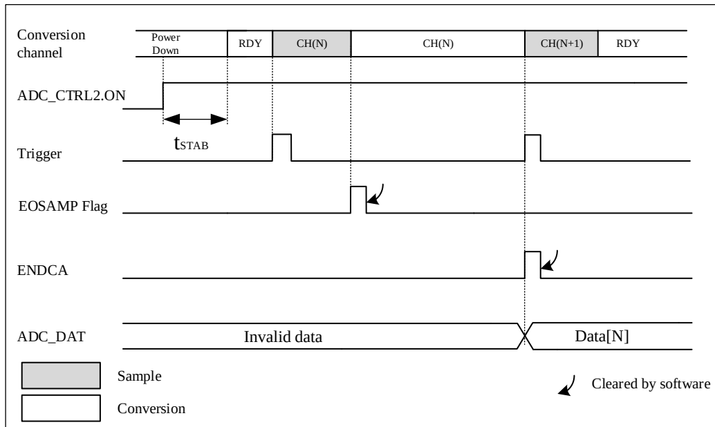
Figure 17-8 Timing Diagram
