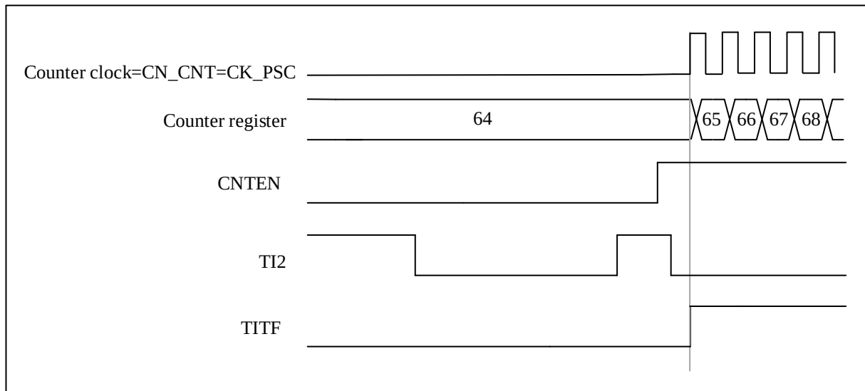
Figure 12-36 Control Circuit in Trigger Mode
