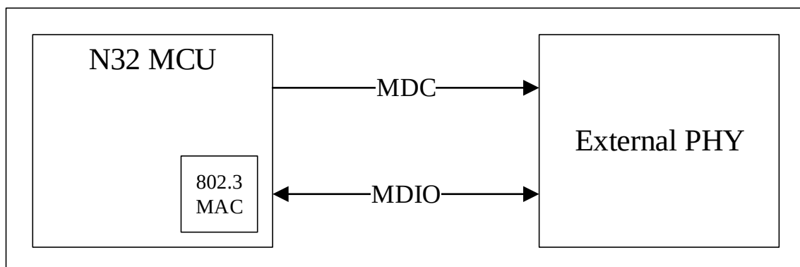
Figure 34-8 SMA Interfaces
