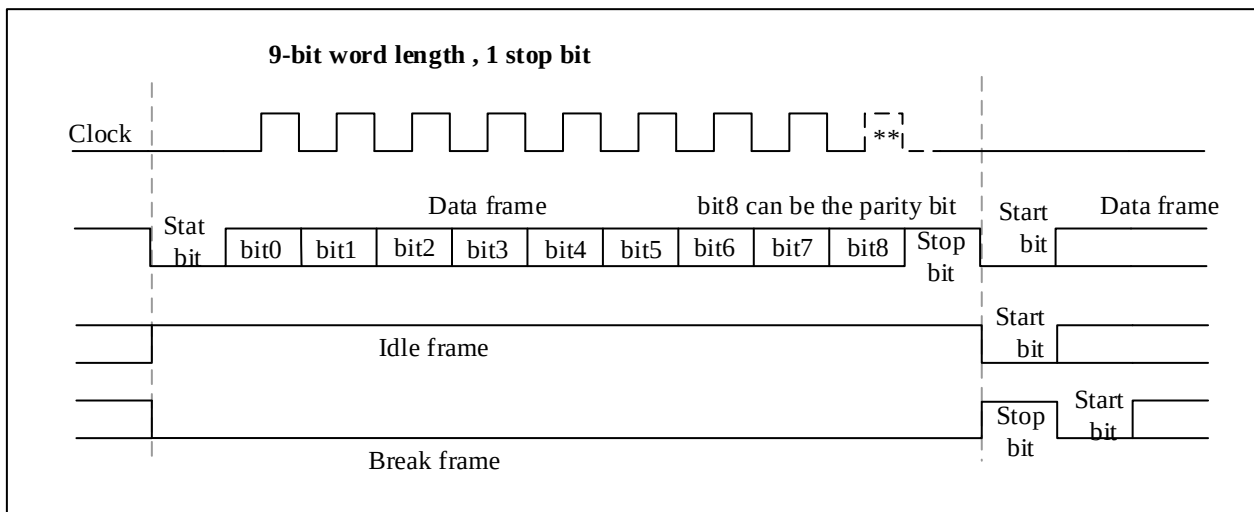
Figure 21-3 Programming for Word Length = 9
