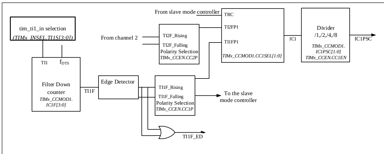
Figure 10-13 Capture/Compare Channel (Example: Channel 1 Input Stage)
