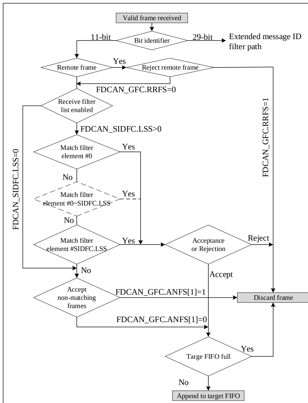
Figure 23-7 FDCAN Standard Message ID Filtering Process
