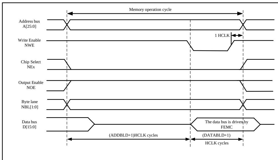
Figure 28-6 Mode A Write Accesses
