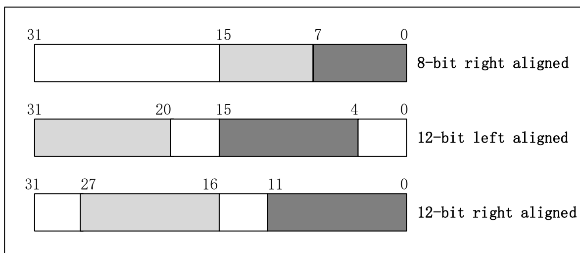
Figure 18-3 Data format when DAC outputs are synchronized
