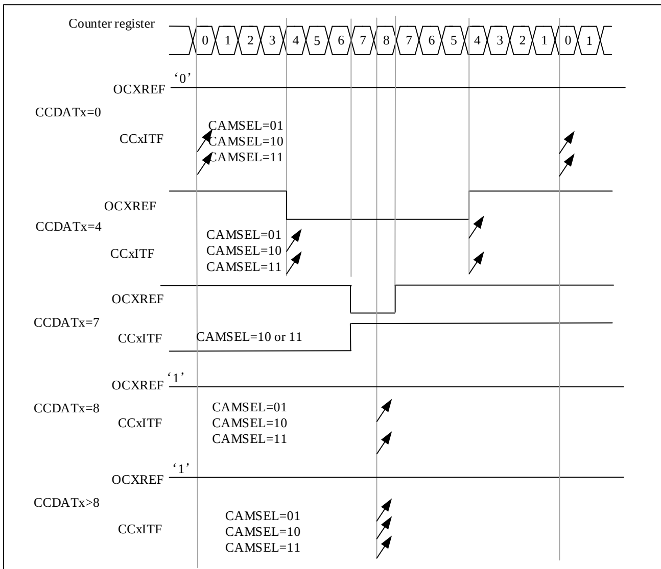
Figure 11-19 Center-Aligned PWM Waveform (AR=8)
