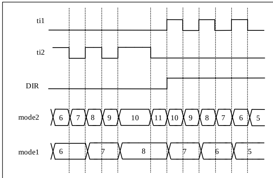
Figure 12-51 Dual Pulse Encoding Mode (CC1P = CC2P = 1)
