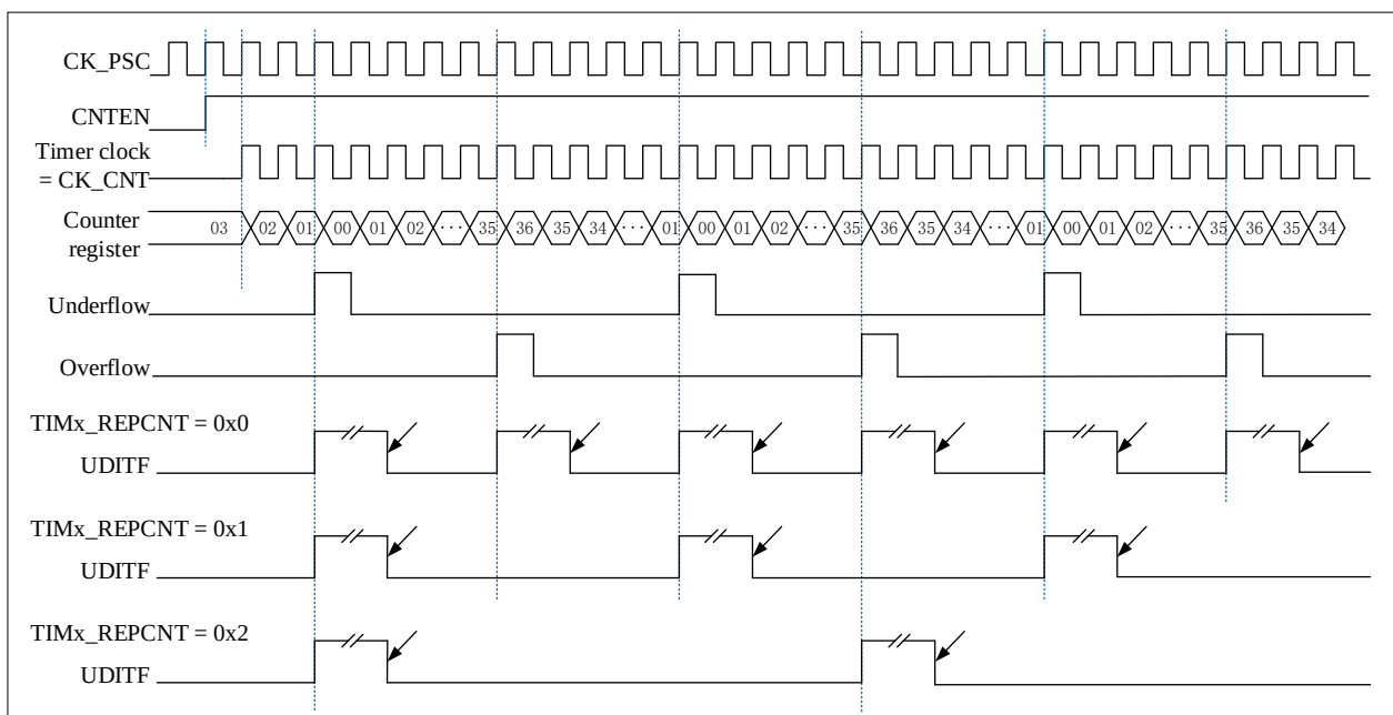
Figure 12-11 Timing diagram of the repetition counter in center-aligned mode
