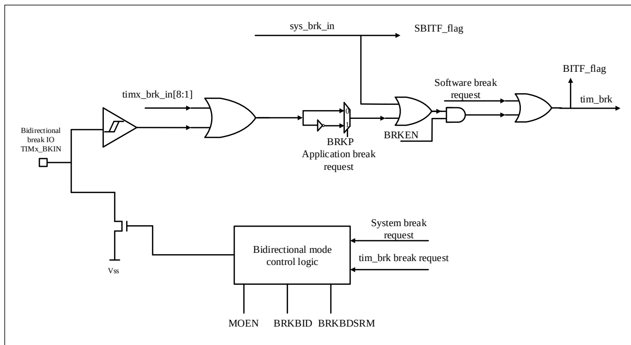
Figure 12-34 Output Redirection
