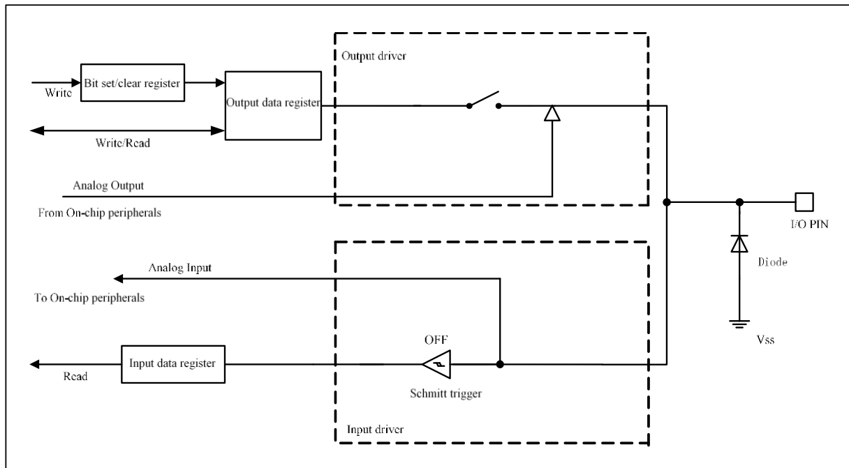
Figure 5-5 High Impedance Analog Mode Configuration
