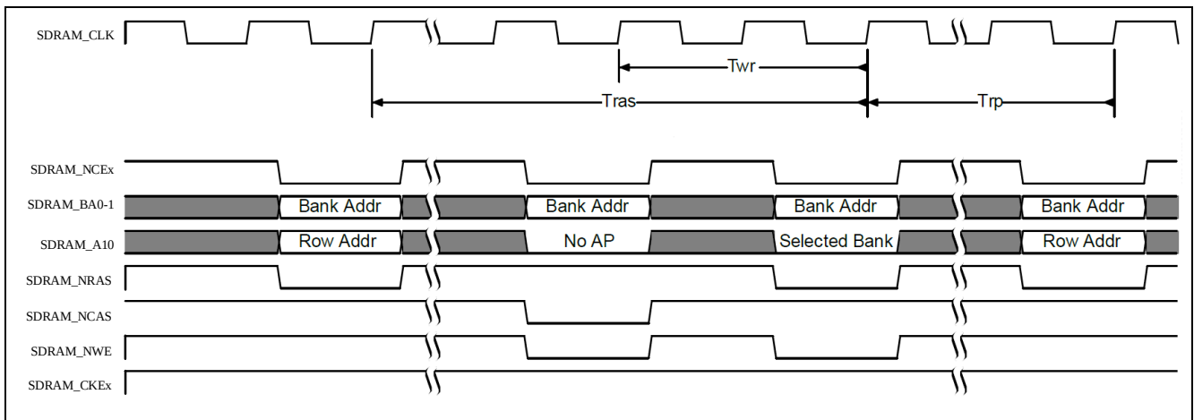
Figure 29-12 Precharge Selected SDRAM Bank
