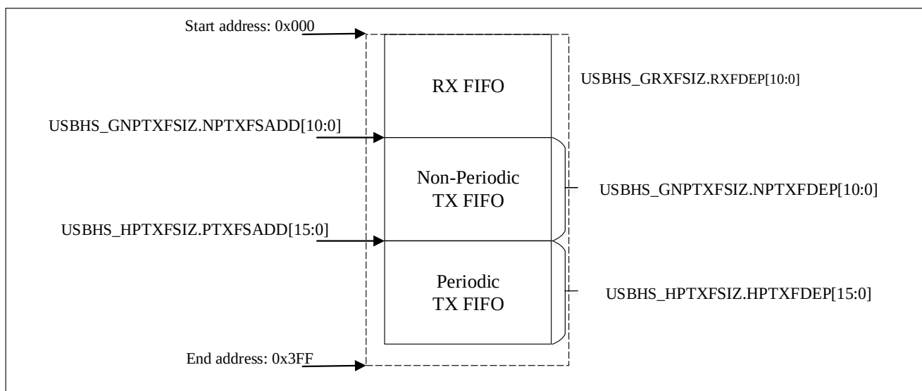
Figure33-3 Host-mode FIFO Address Mapping and AHB FIFO Access Mapping
