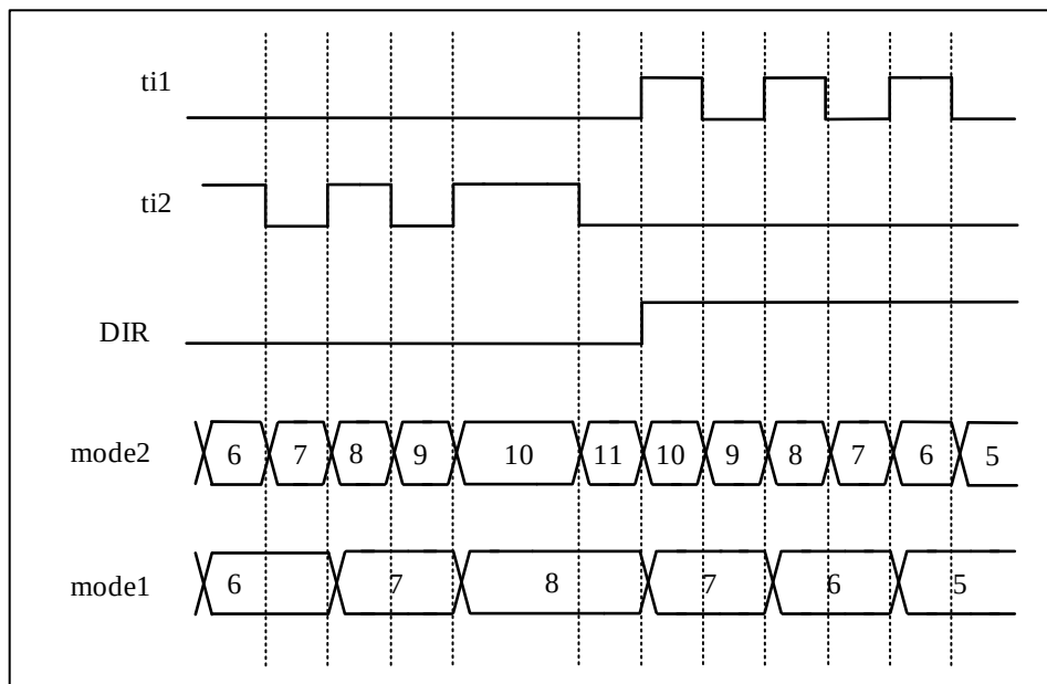
Figure 11-42 Dual Pulse Encoding Mode (CC1P = CC2P = 1)
