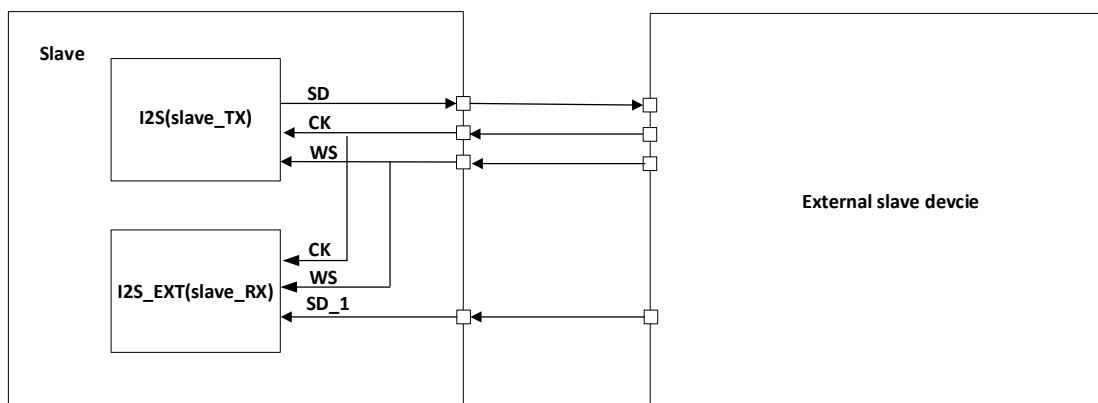
Figure 24-17 I2S slave transmit mode (I2SCFG=00), I2S_EXT slave receive (I2SCFG=01)
