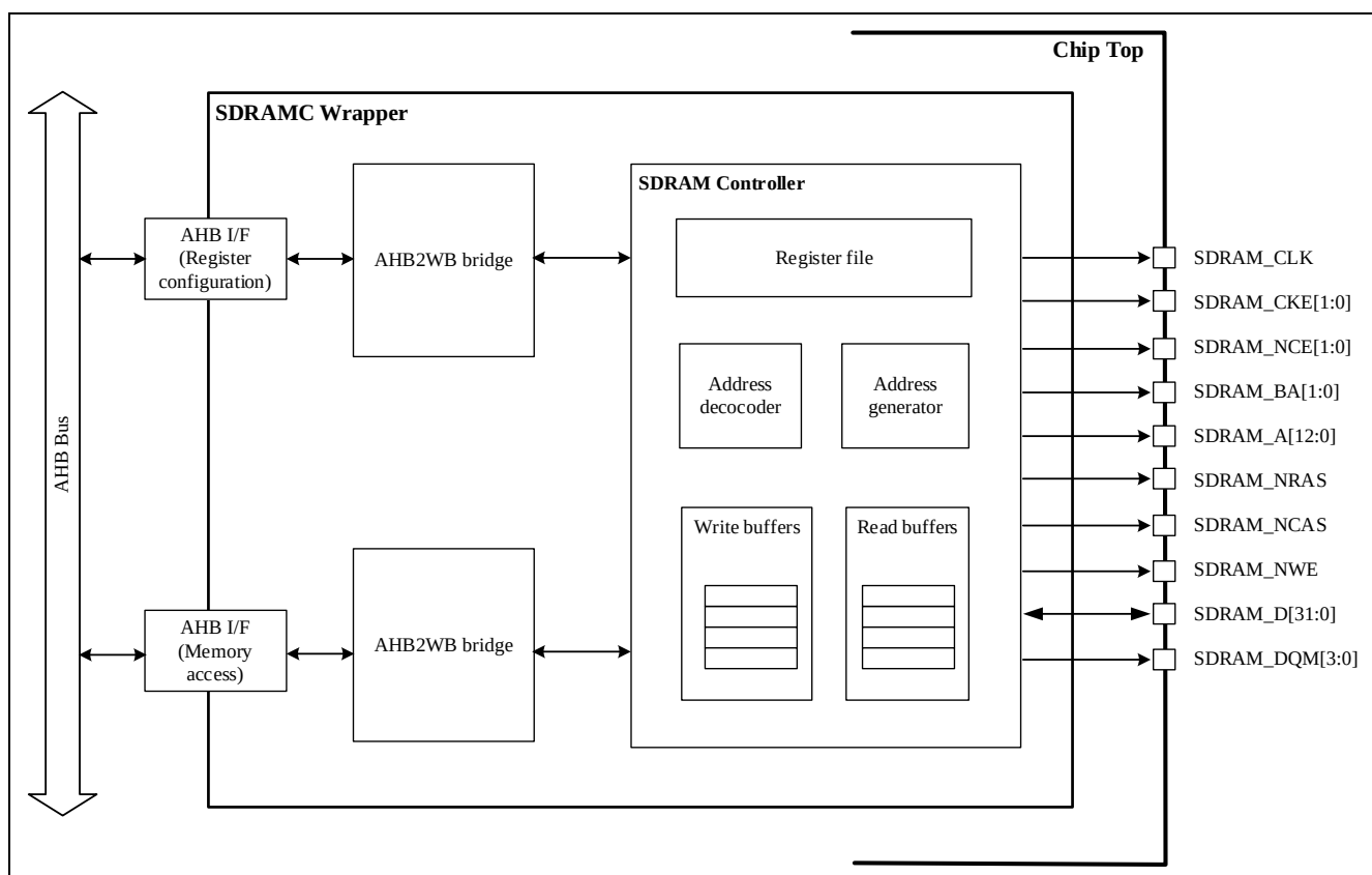
Figure 29-1 SDRAMC Block Diagram
