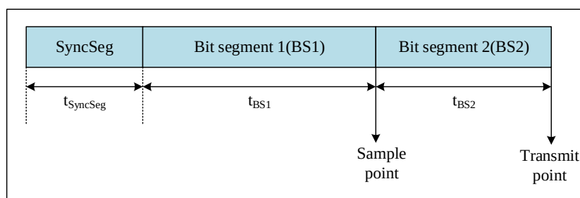
Figure 23-14 FDCAN Bit Timing
