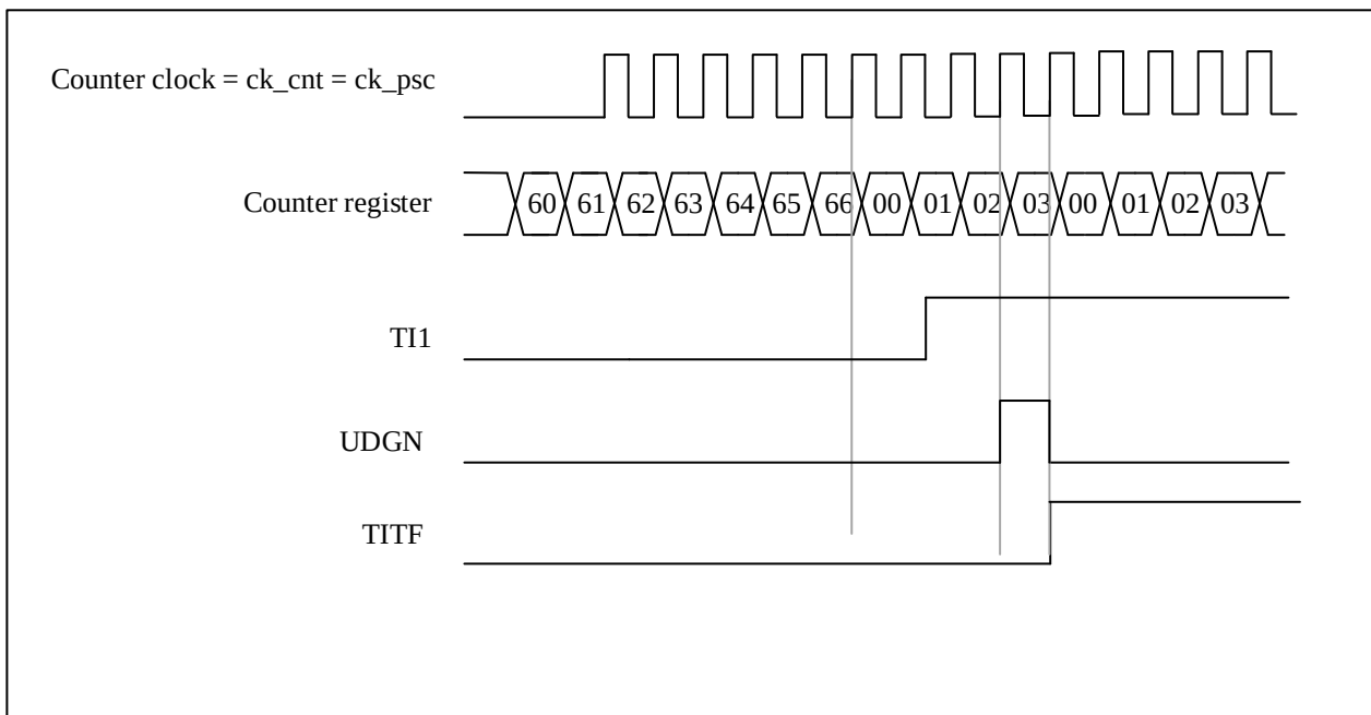
Figure 9-37 Control Circuit in Reset Mode
