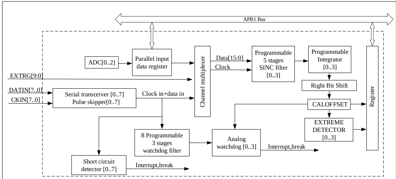
Figure 31-1 DSMU block diagram
