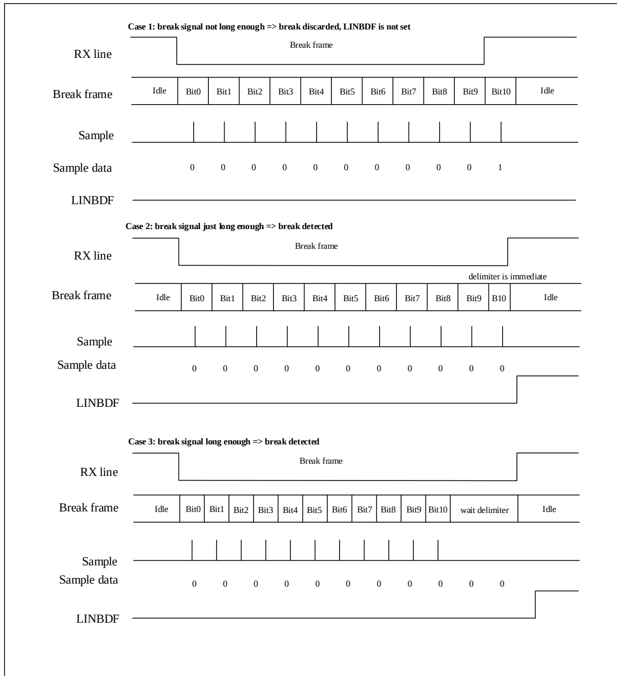
Figure 21-20 LIN Break Detection In LIN Mode (11-bit break length-the LINBDL bit is set)
