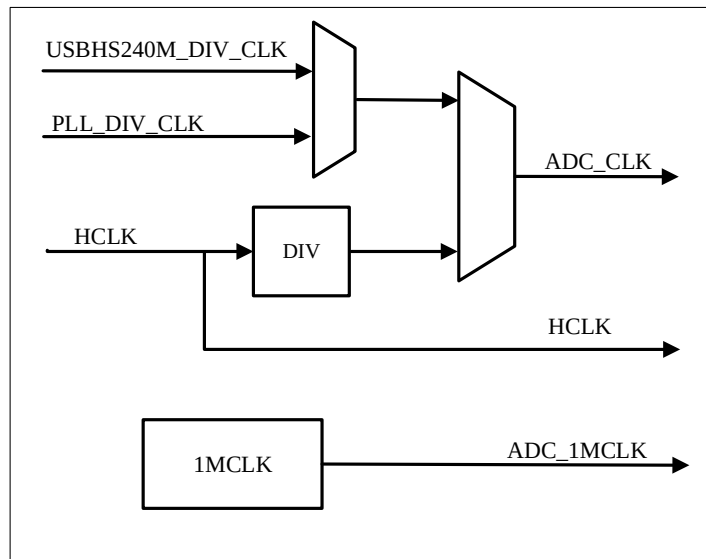
Figure 17-2 ADC Clock
