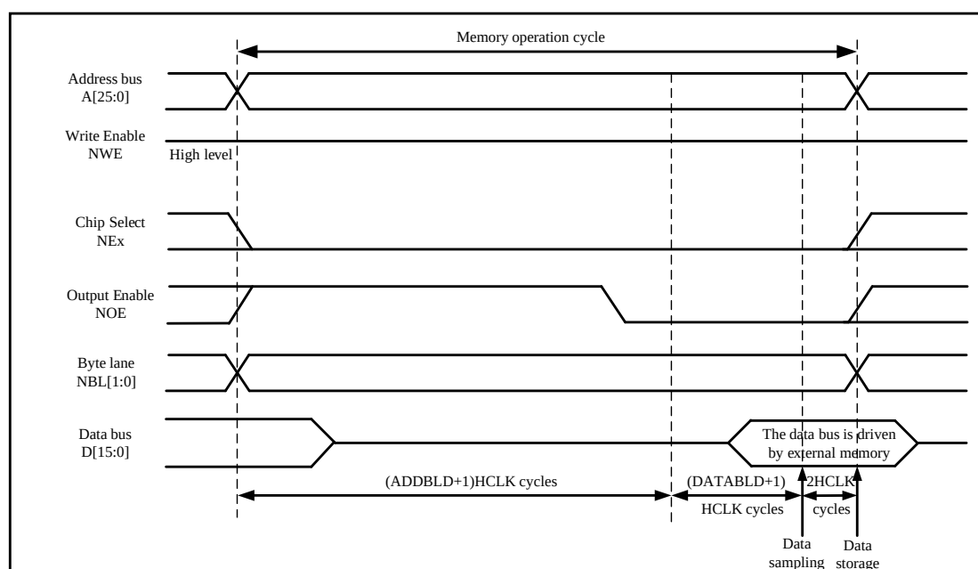
Figure 28-4 Mode A Read Accesses
