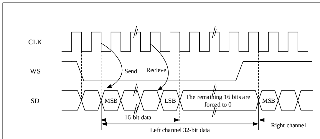
Figure 26-24-21 I2S Philips Protocol Standard Waveform (16-Bit Extended to 32-Bit Packet Frame, CLKPOL = 0)
