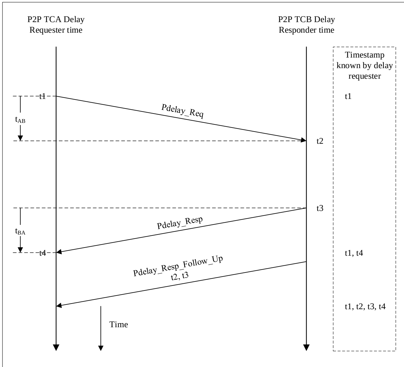
Figure 34-14 Propagation Delay Calculation in Clocks Supporting Peer-to-Peer Path Correction
