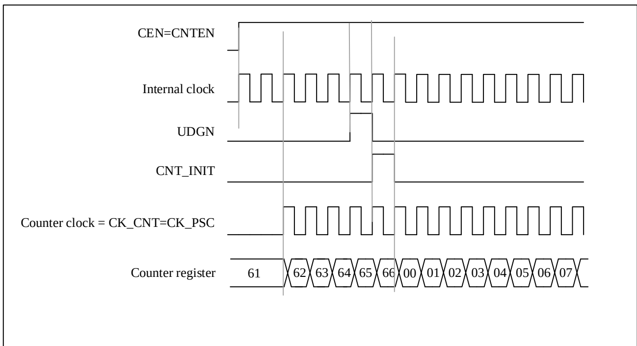
Figure 12-12 Control Circuit In Normal Mode With Internal Clock Divided By 1
