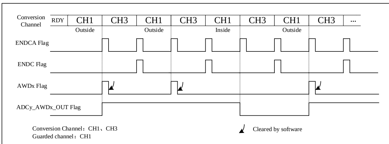
Figure 17-9 Generation of ADCx_AWDy_OUT (on a single regular channel)
