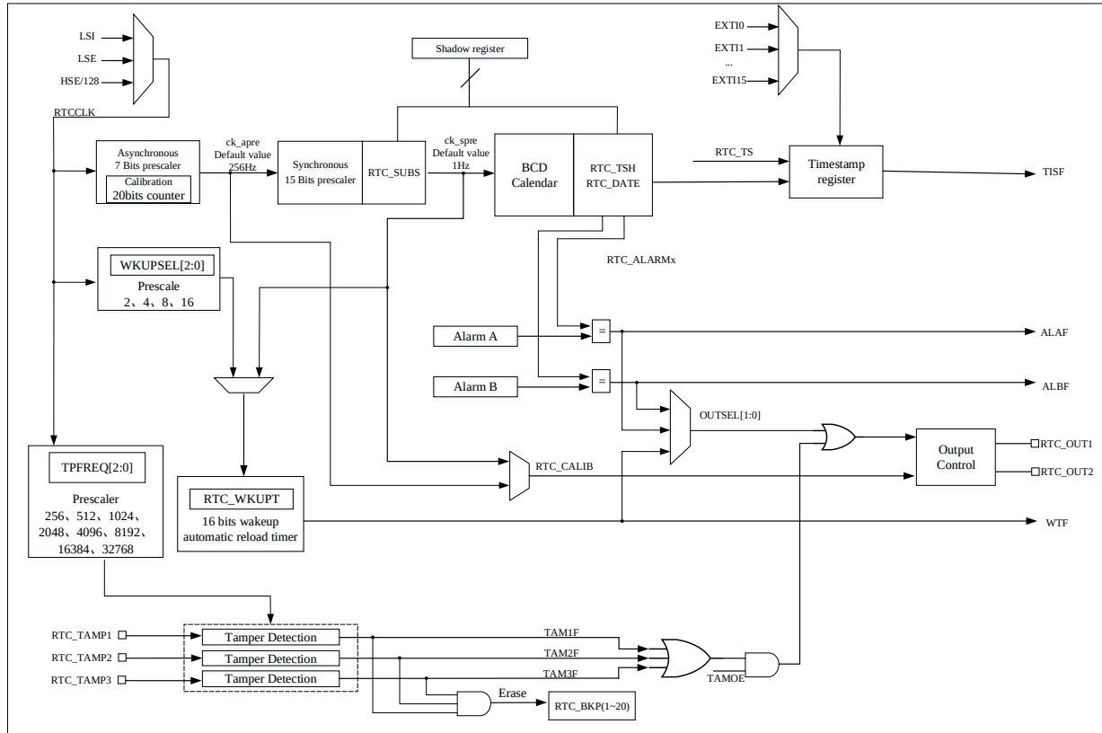
Figure 25-1 RTC Block Diagram
