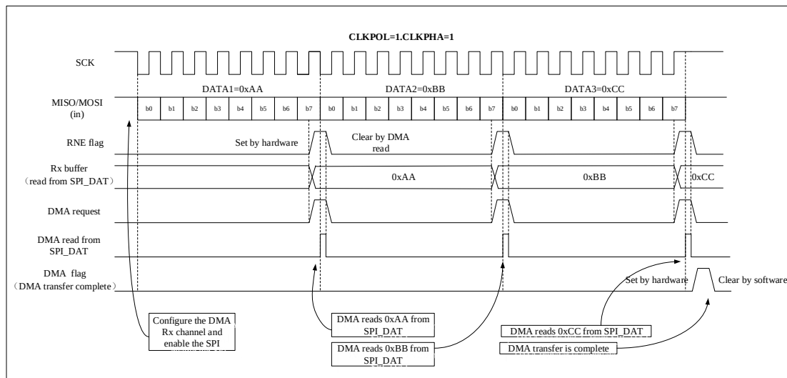
Figure 24-12 Reception Using DMA
