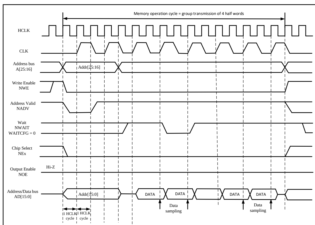
Figure 28-19 Synchronous Multiplexed Write Mode - PSRAM (CRAM)
