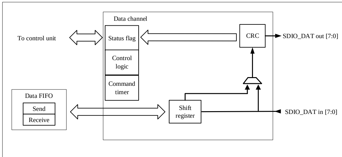
Figure 30-12 Data Channel
