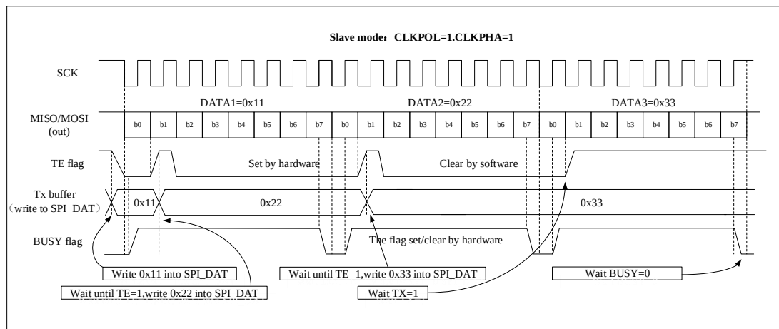
Figure 24-9 TE/BUSY Behavior in Slave Transmit-Only Mode in Case of Continuous Transfers
