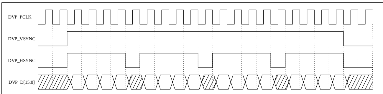
Figure 30-2 Example of DVP Interface Timing
