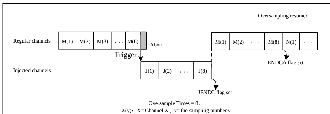
Figure 17-19 Regular and Injection Oversampling
