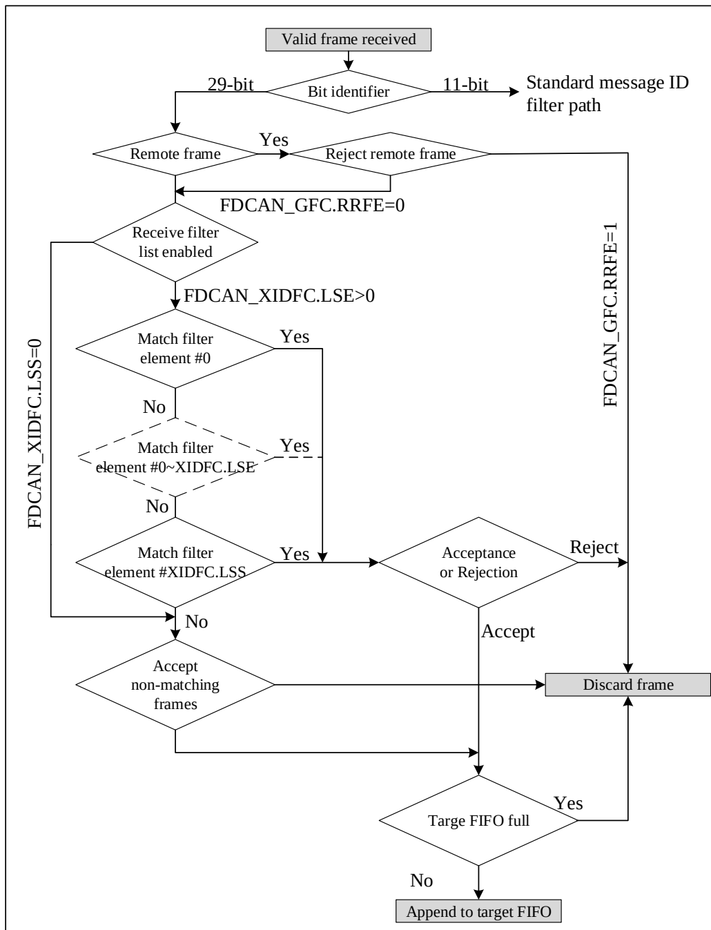
Figure 23-8 FDCAN Extended Message ID Filtering Process
