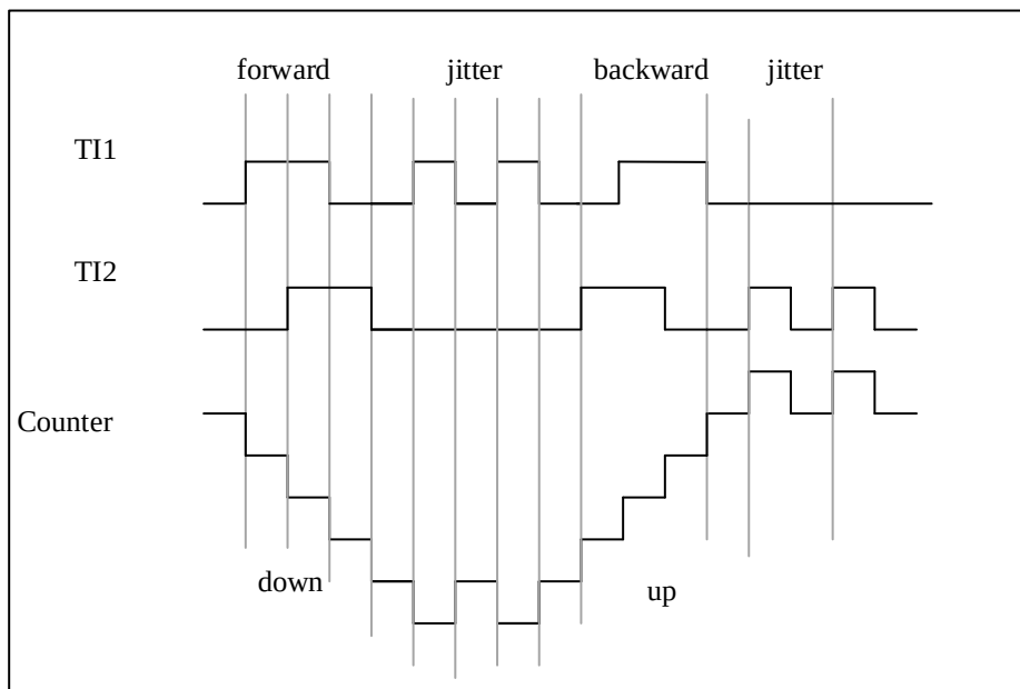
Figure 11-39 Encoder Interface Mode Example With IC1FP1 Polarity Inverted
