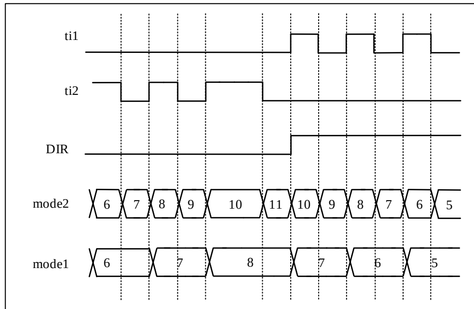
Figure 10-42 Dual Pulse Encoding Mode (CC1P = CC2P = 1)
