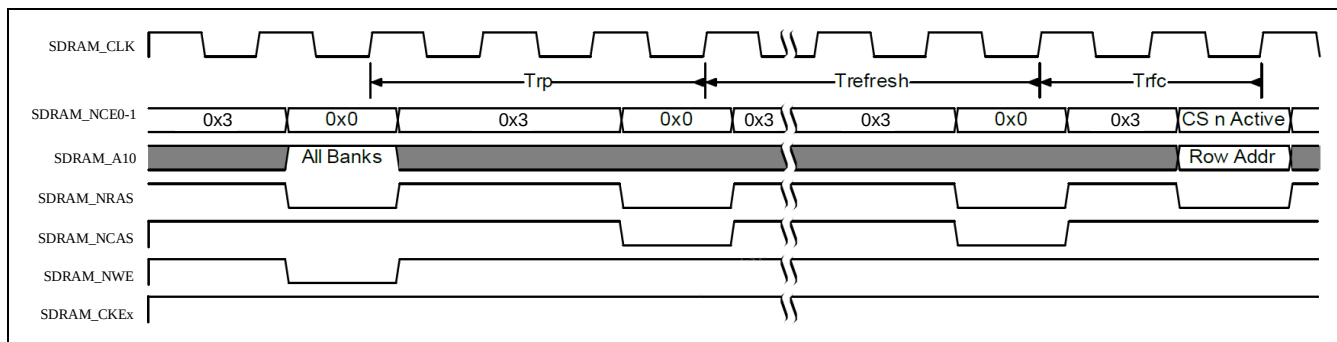
Figure 29-14 Auto Refresh
