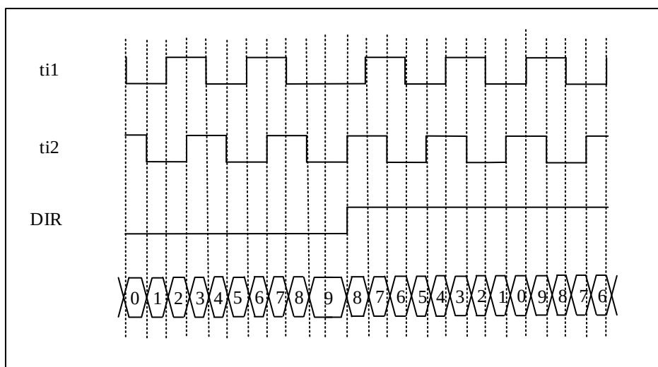
Figure 10-35 The Encoder Counts on Both TI1 and TI2
