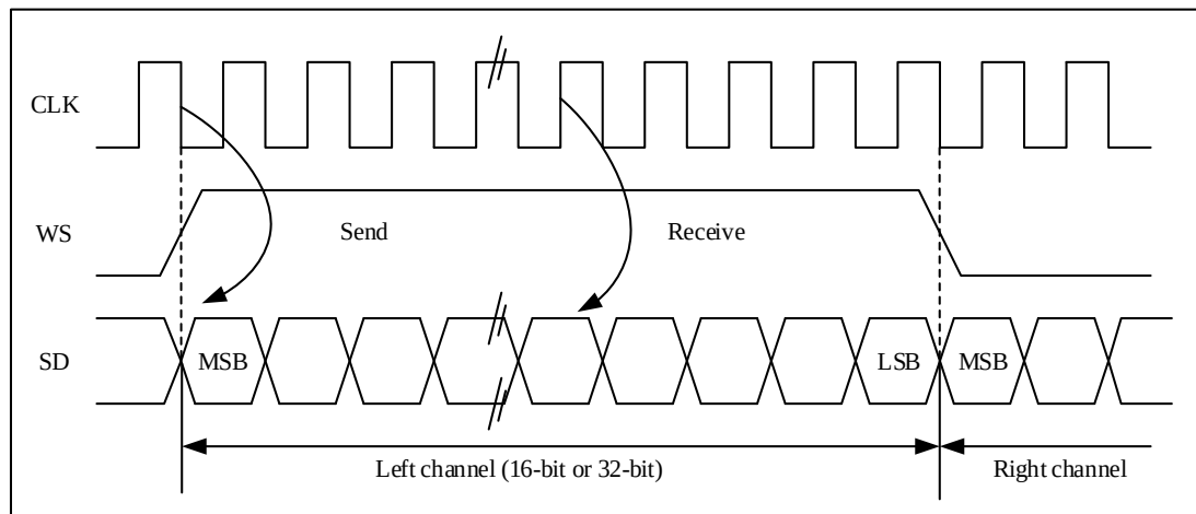
Figure 26-24-25 LSB Alignment 16-Bit or 32-Bit Full Precision, CLKPOL = 0
