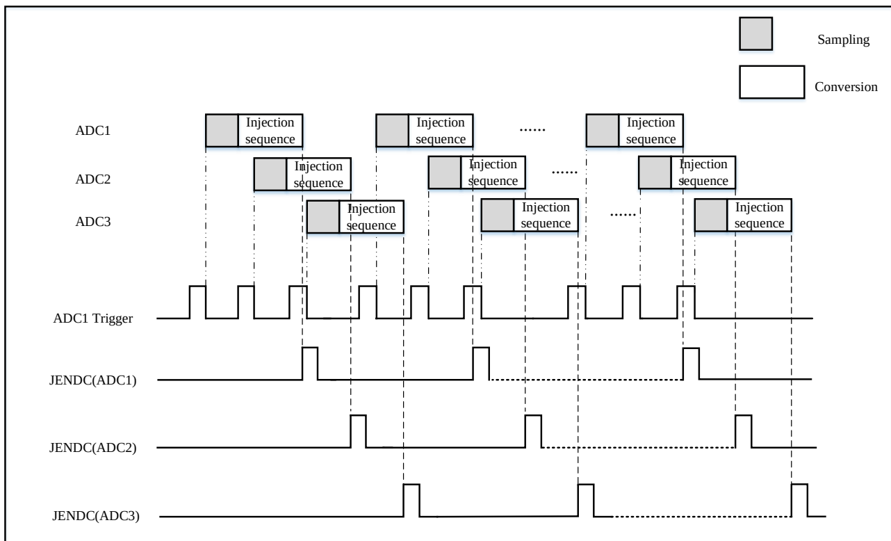
Figure 17-32 Alternate Trigger: Injection Channel Group in Discontinuous Mode
