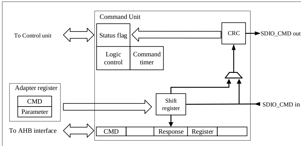
Figure 30-9 SDIO Adapter Command Unit
