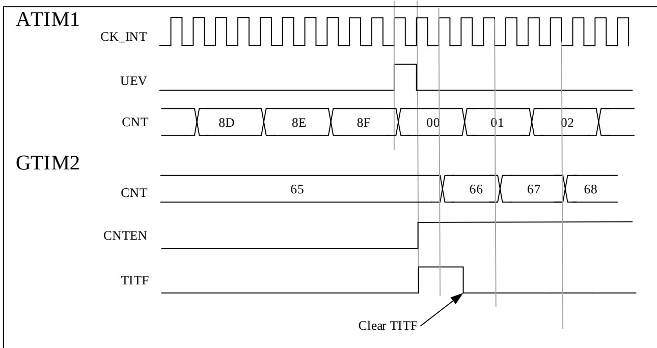
Figure 10-31 Trigger GTIM2 with An Update Of ATIM1
