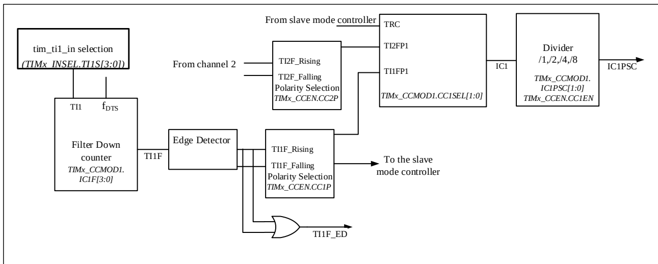
Figure 9-20 Capture/Compare Channel (Example: Channel 1 Input Stage)
