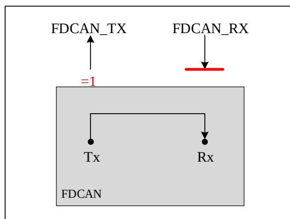
Figure 23-6 FDCAN Internal Loopback Mode Pin Control
