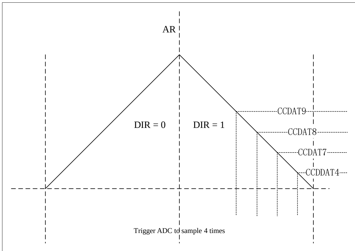
Figure 9-10 CCDATx(x=4,7,8,9) Triggers ADC When DIR = 1
