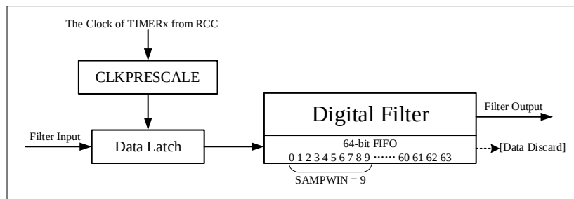
Figure 9-35 Slide Filter
