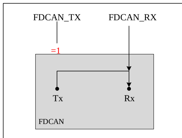
Figure 23-4 FDCAN Bus Monitoring Mode Pin Control
