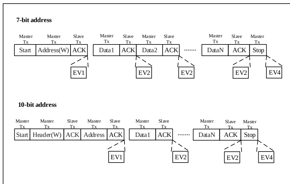
Figure 22-5 Slave receiver transmitting sequence
