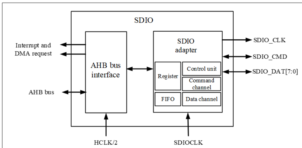
Figure 30-6 SDIO Block Diagram
