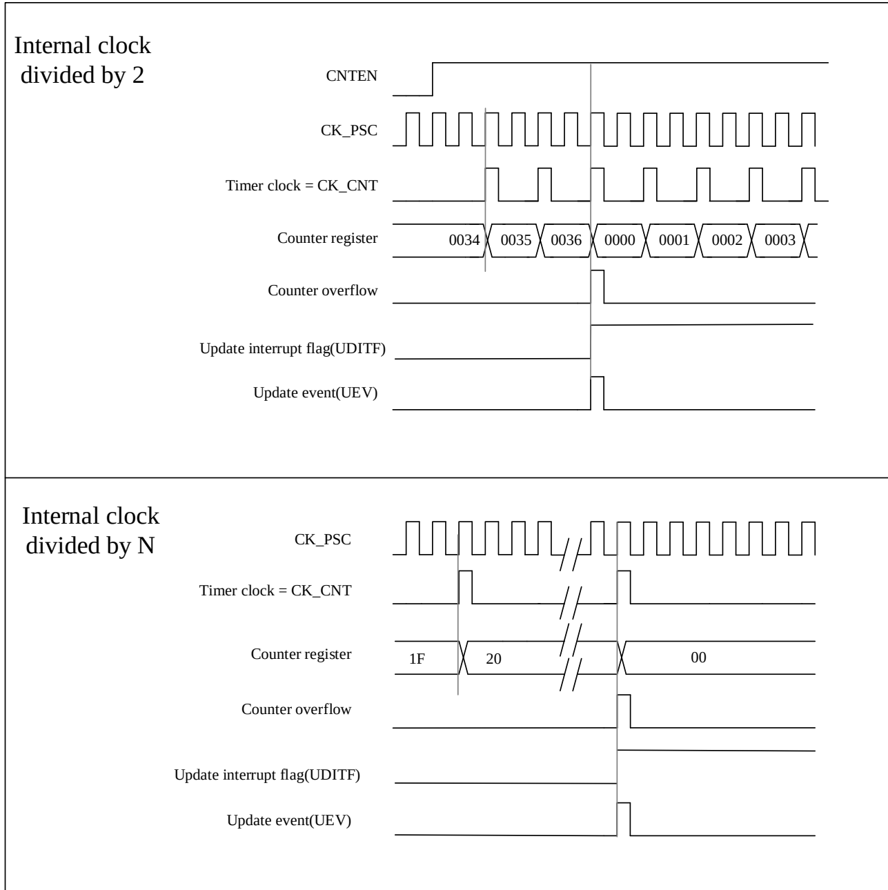
Figure 10-3 Timing Diagram Of Up-Counting. When The Internal Clock Divider Factor = 2/N
