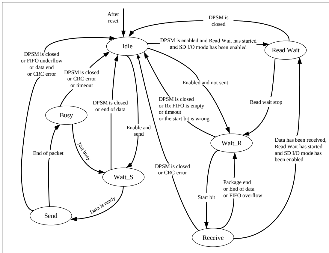
Figure 30-13 Data Path State Machine (DPSM)
