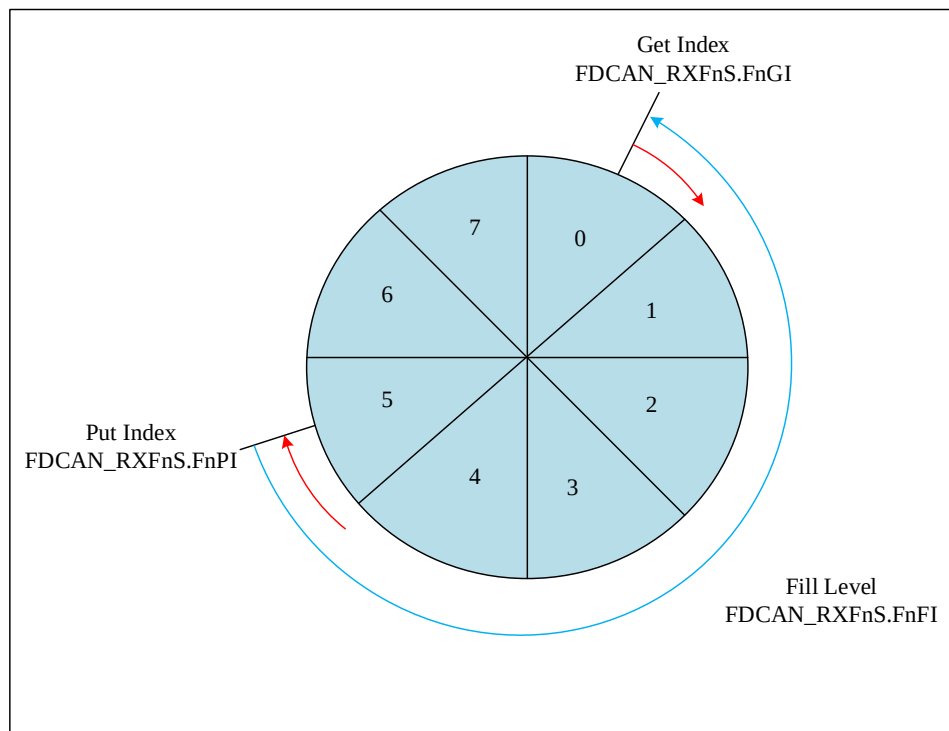
Figure 23-9 FDCAN Rx FIFO Status Diagram
