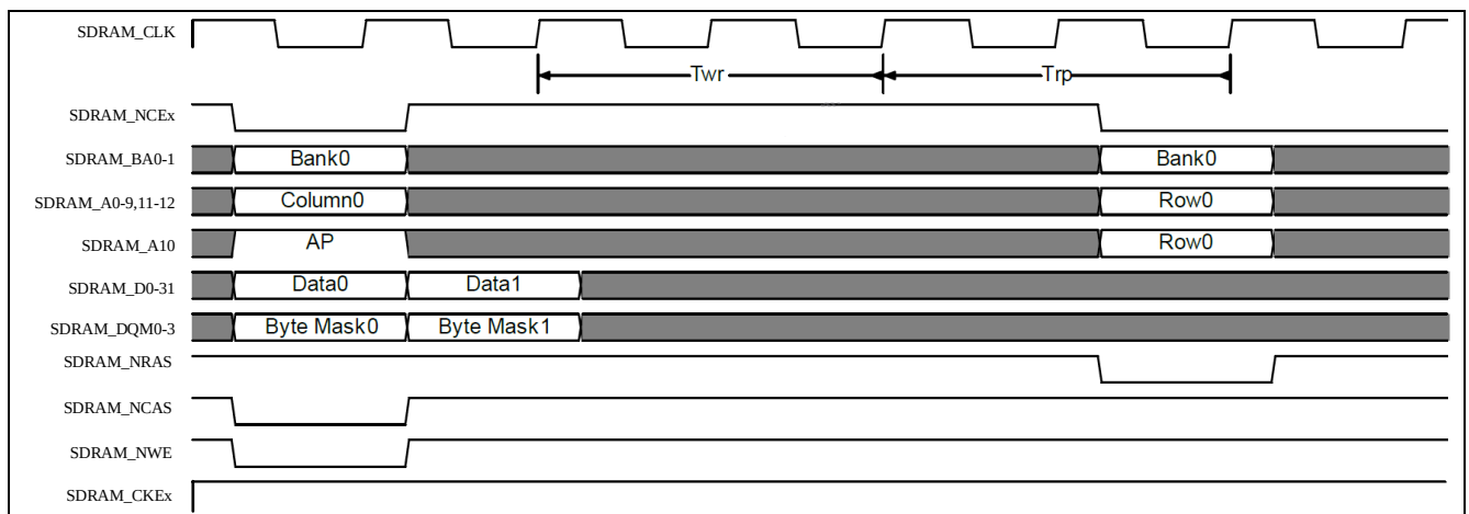
Figure 29-7 Burst SDRAM write with Auto Precharge
