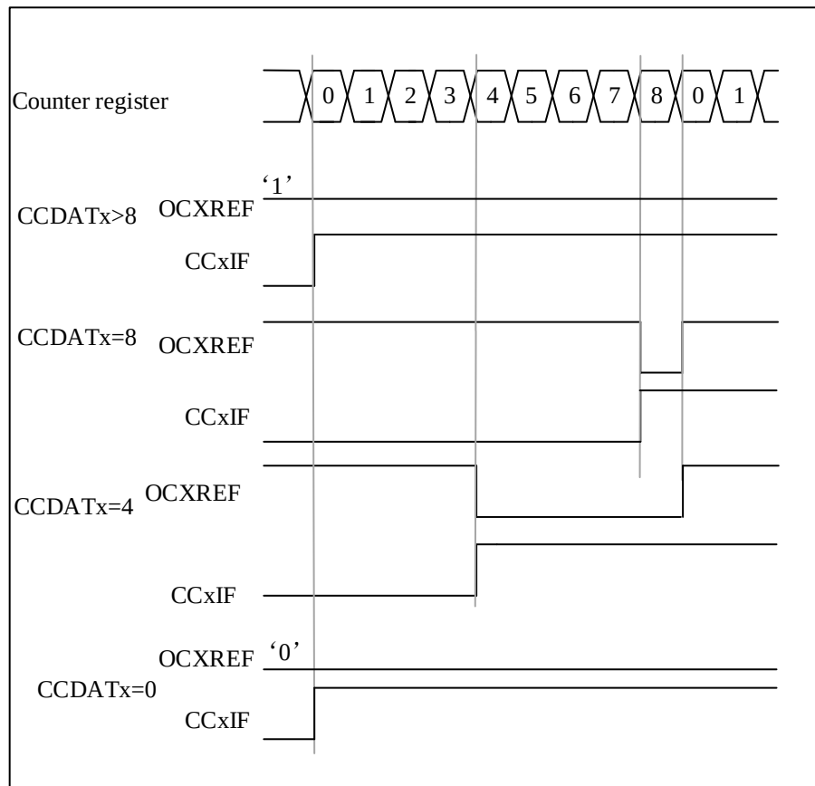
Figure 10-20 Edge-Aligned PWM waveform (AR=8)
