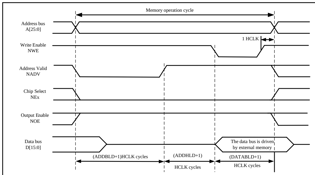
Figure 28-13 Mode D Write Accesses
