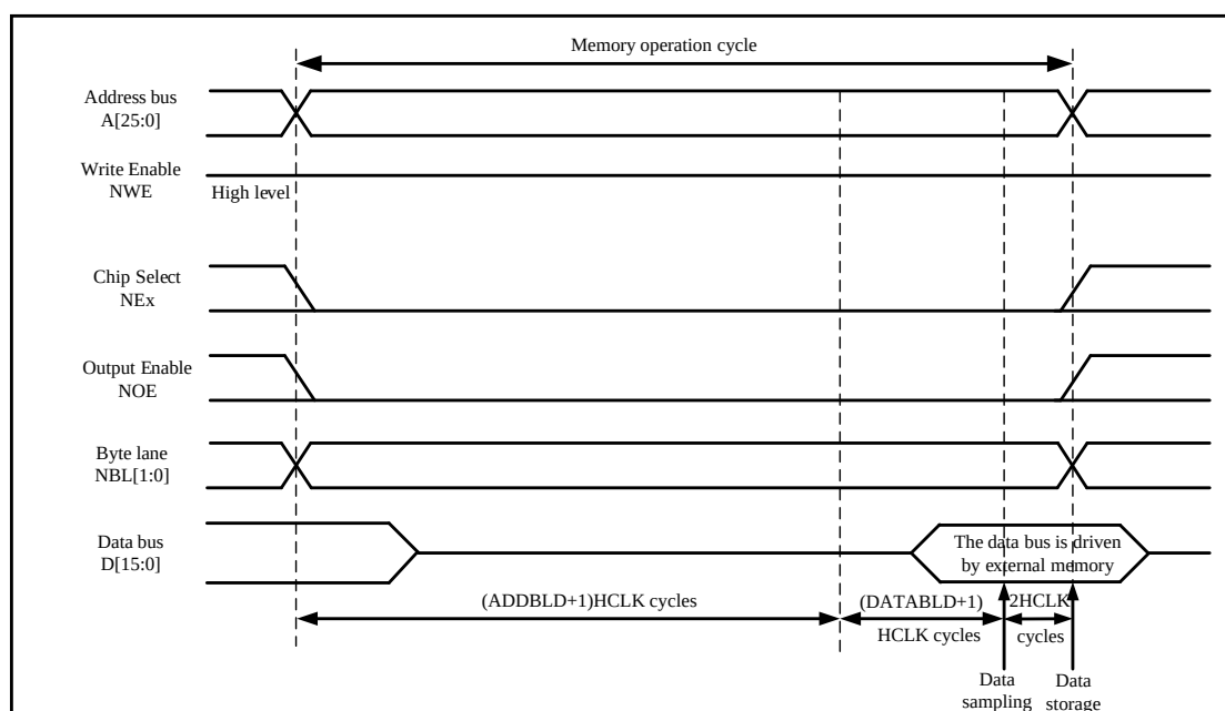
Figure 28-3 Model Read Accesses
