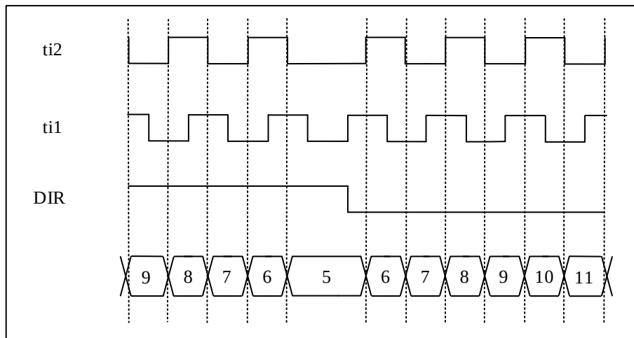
Figure 9-46 The Encoder Counts on Both TI1 and TI2
