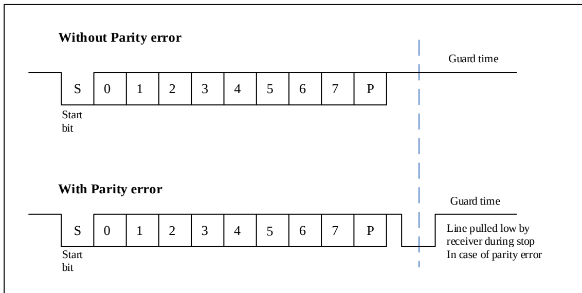
Figure 21-22 ISO7816-3 Asynchronous Protocol
