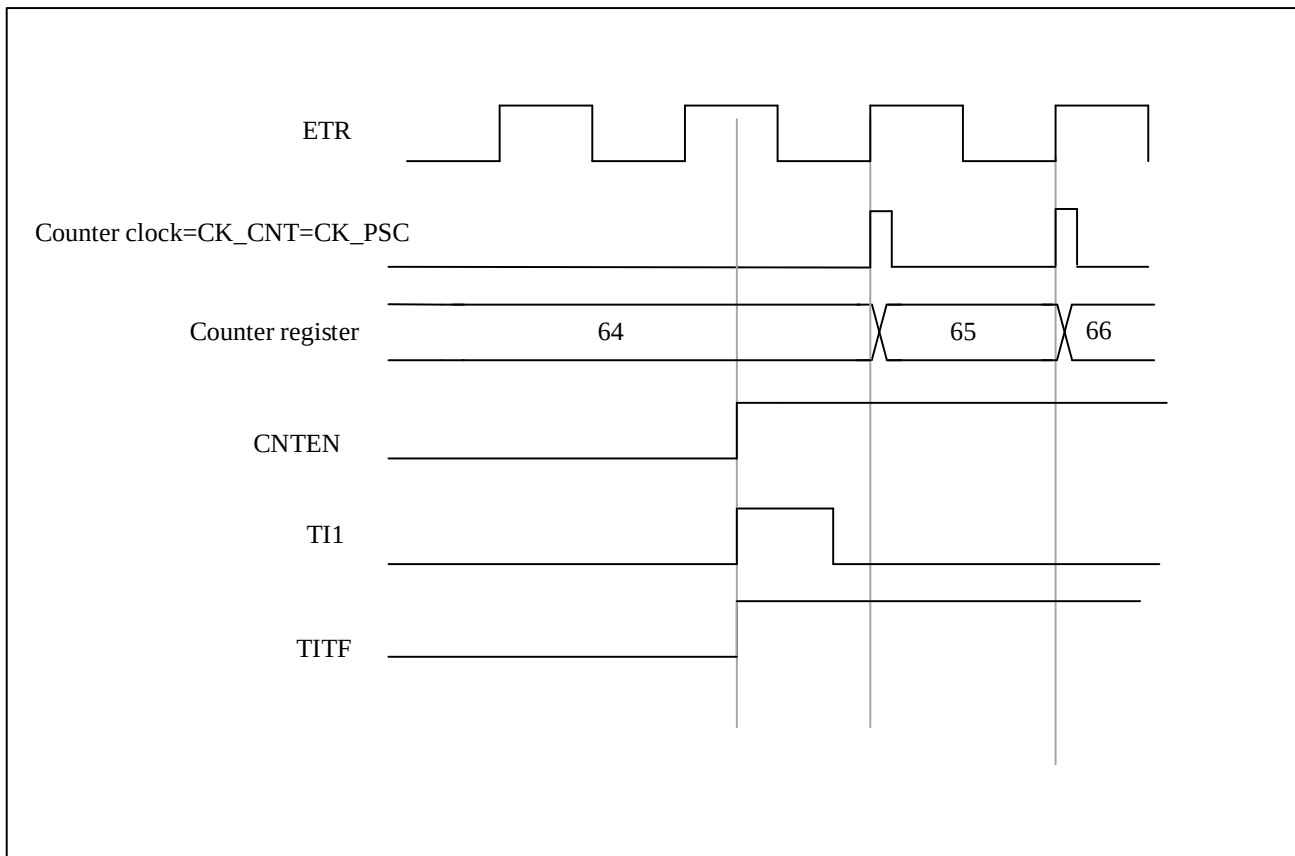
Figure 9-40 Control Circuit in Trigger Mode + External Clock Mode2
