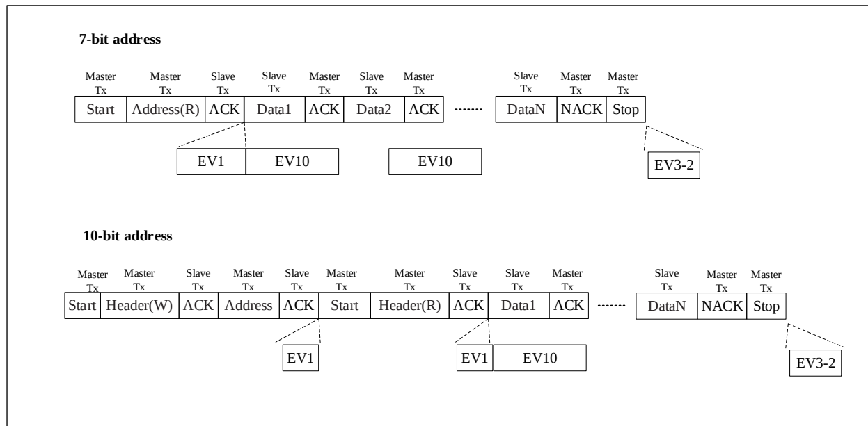
Figure 22-4 Enable FIFO to transmit sequences from the transmitter
