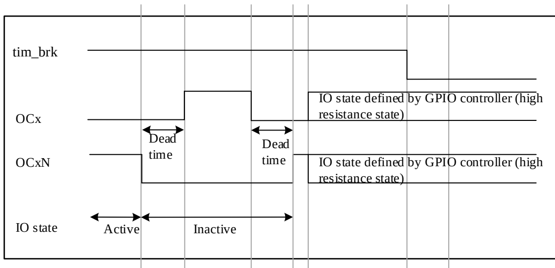
Figure 9-34 PWM Output State Following tim_brk Assertion (OSSI=0)
