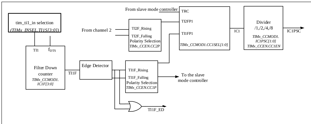
Figure 12-17 Capture/Compare Channel (Example: Channel 1 Input Stage)
