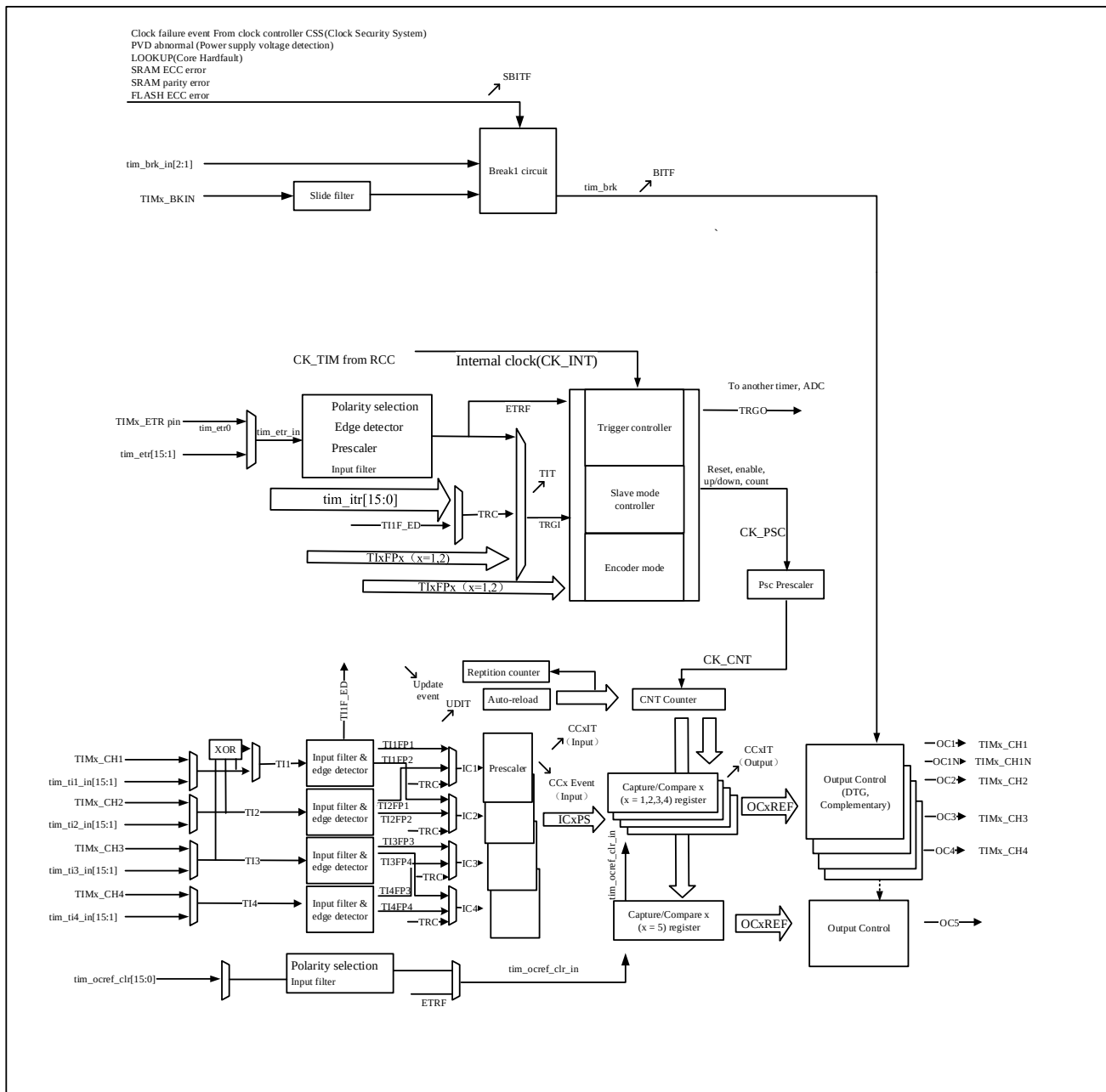
Figure 12-1 Block Diagram Of GTIMx
