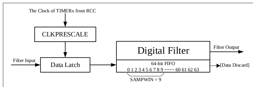
Figure 12-33 Sliding filter
