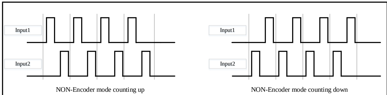
Figure 14-8 Input waveforms of Input1 and Input2 when the decoder module is working normally
