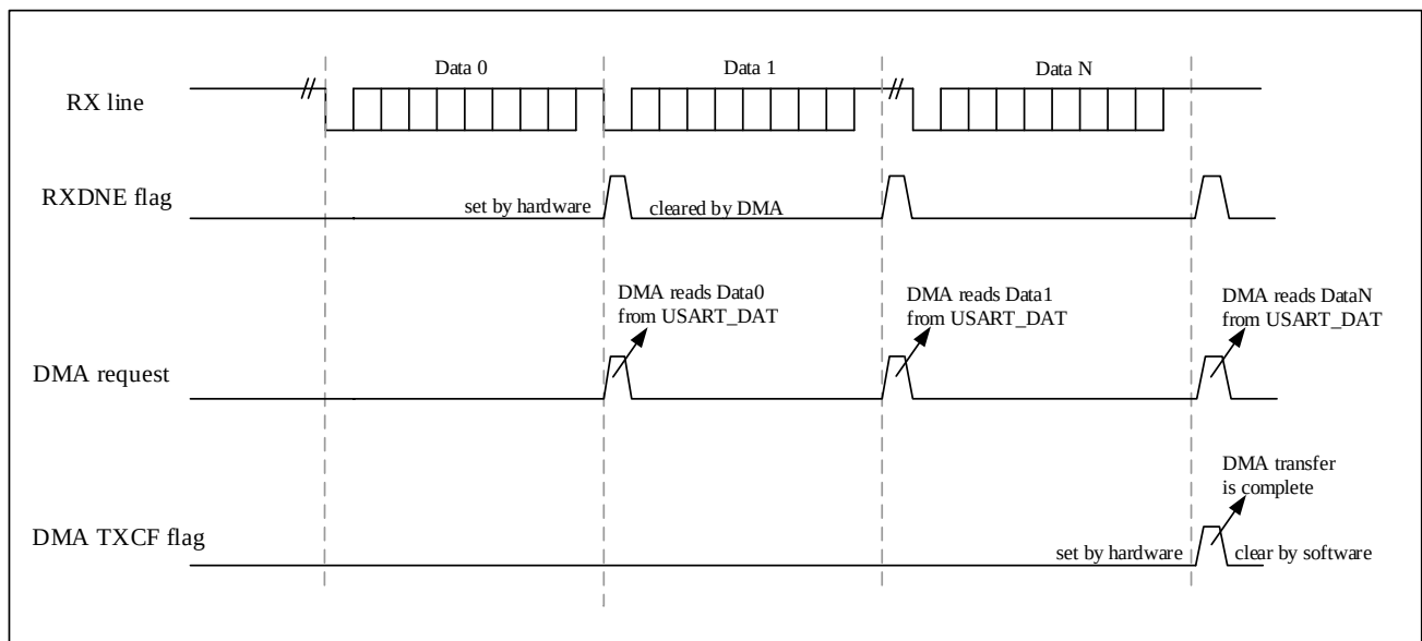
Figure 21-8 DMA Reception
