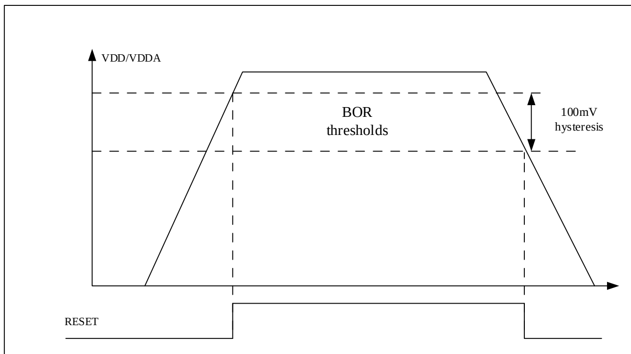
Figure 3-4 BOR Threshold Waveform
