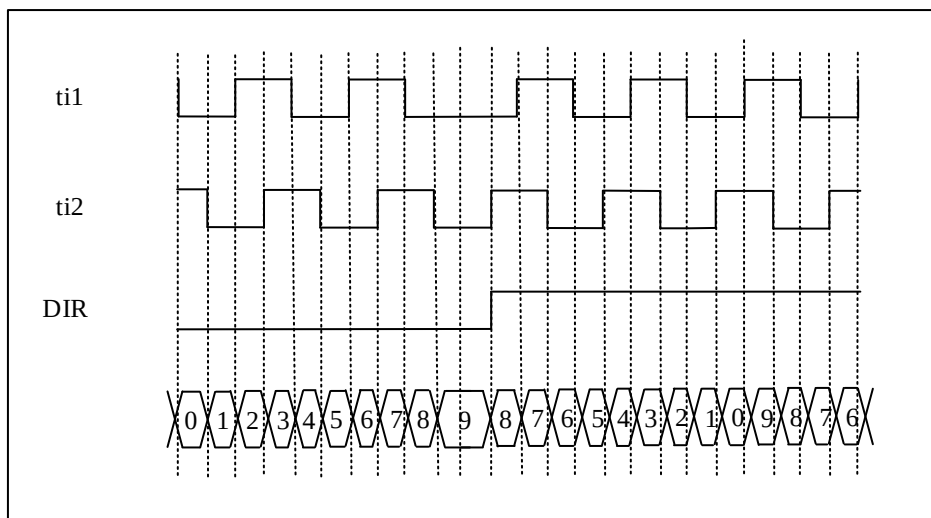
Figure 12-44 The Encoder Counts On Both TI1 and TI2
