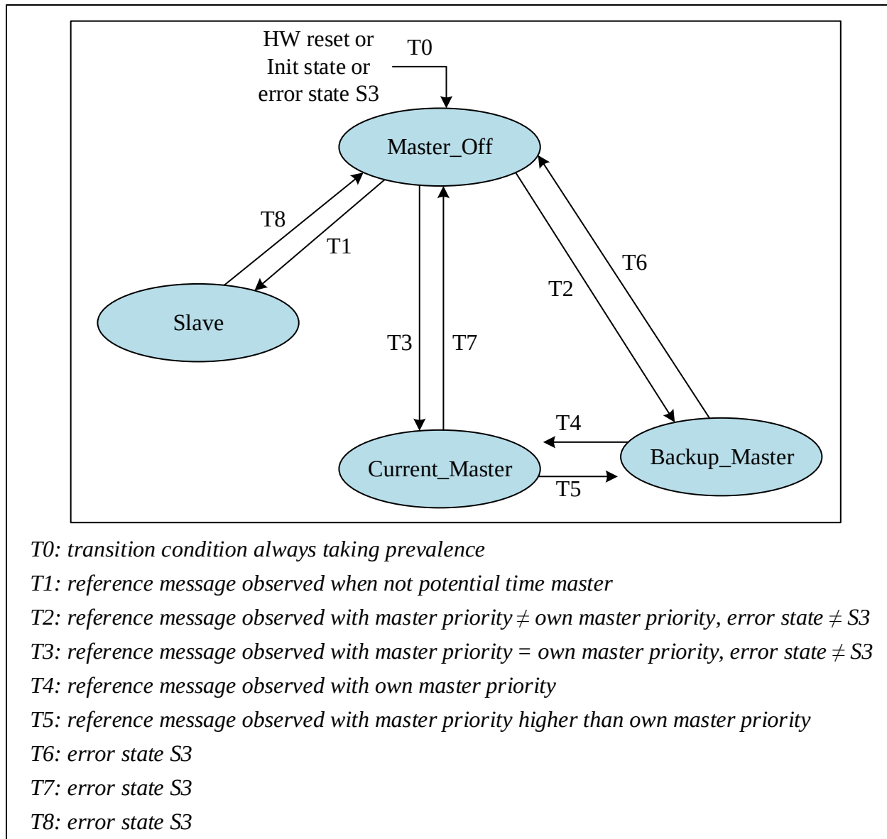
Figure 23-18 Level 0 master to slave relation
