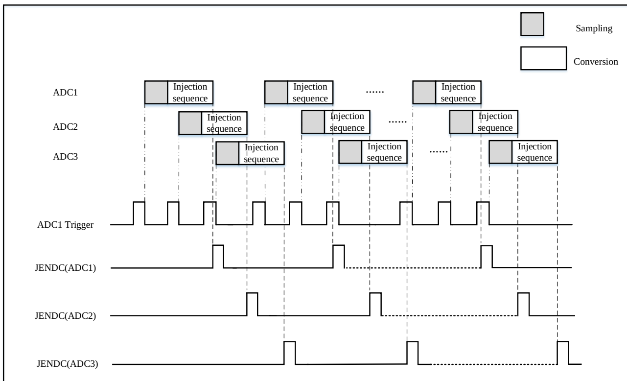
Figure 17-31 Alternate trigger: Injection channel group
