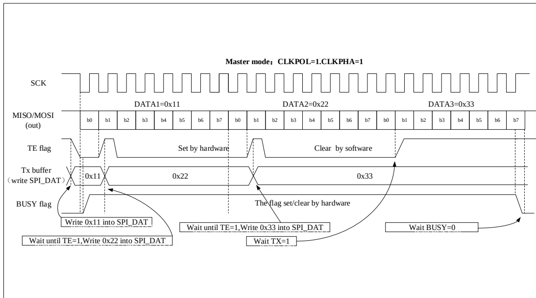
Figure 24-6 TXE/BSY Behavior in Master Transmit-Only Mode( BIDIRMODE = 0 , RONLY = 0 ) during Continuous Transmissions
