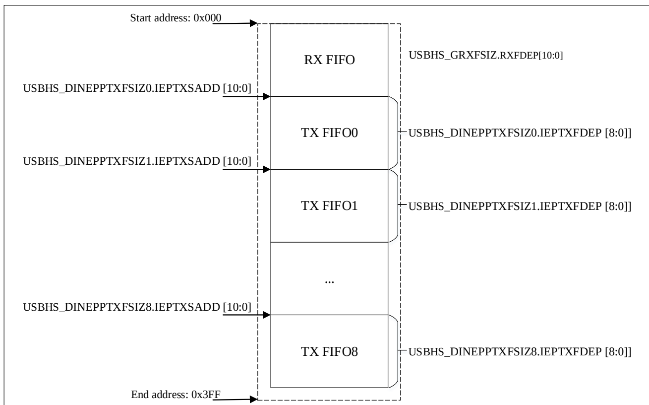
Figure33-2 Device-mode FIFO Address Mapping and AHB FIFO Access Mapping
