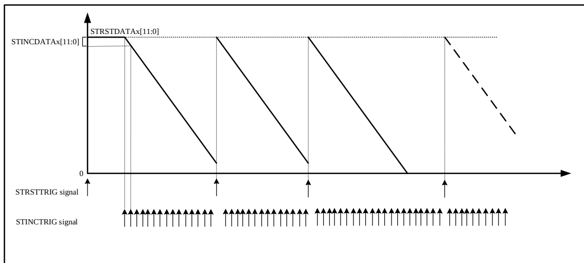
Figure 18-9 Decreasing Sawtooth Wave Generation
