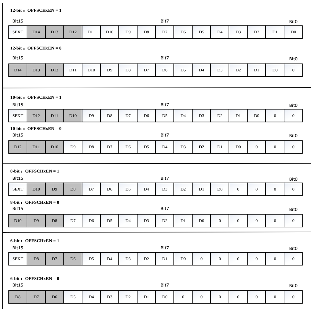
Figure 17-13 Left-Aligned Data
