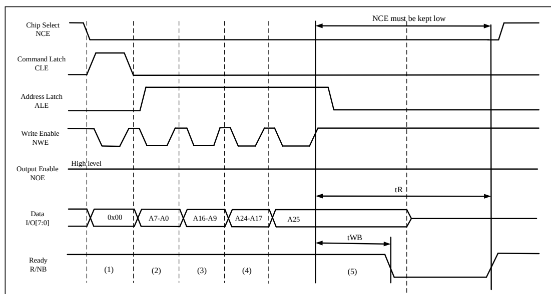
Figure 28-21 Transactions for CE-Sensitive NAND Flash
