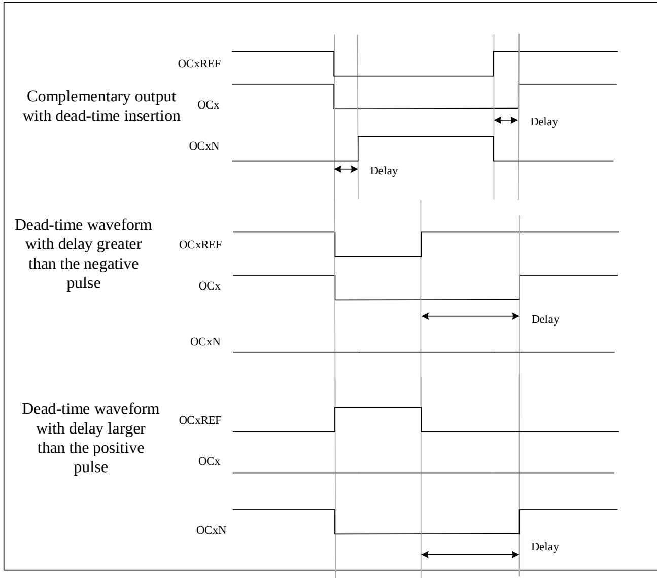
Figure 9-30 Complementary Output with Dead-Time Insertion
