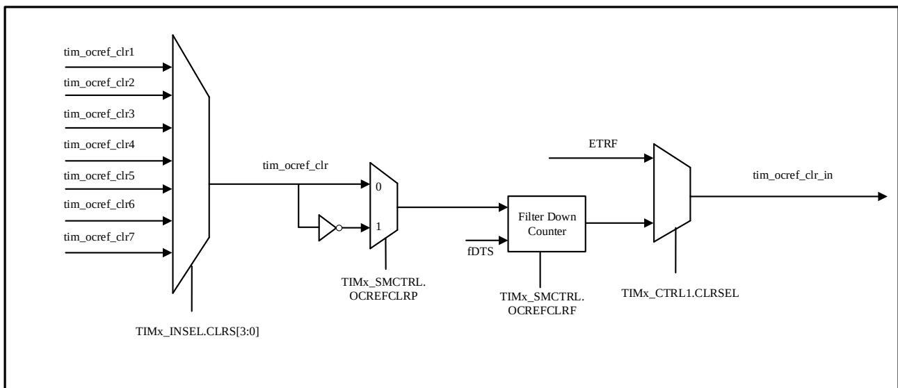
Figure 9-28 Diagram of External Event Clearing Ocxref Signal
