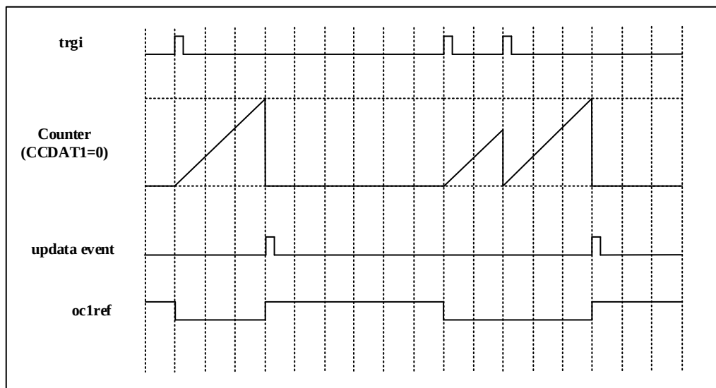
Figure 12-27 Retriggerable Single Pulse Mode 1
