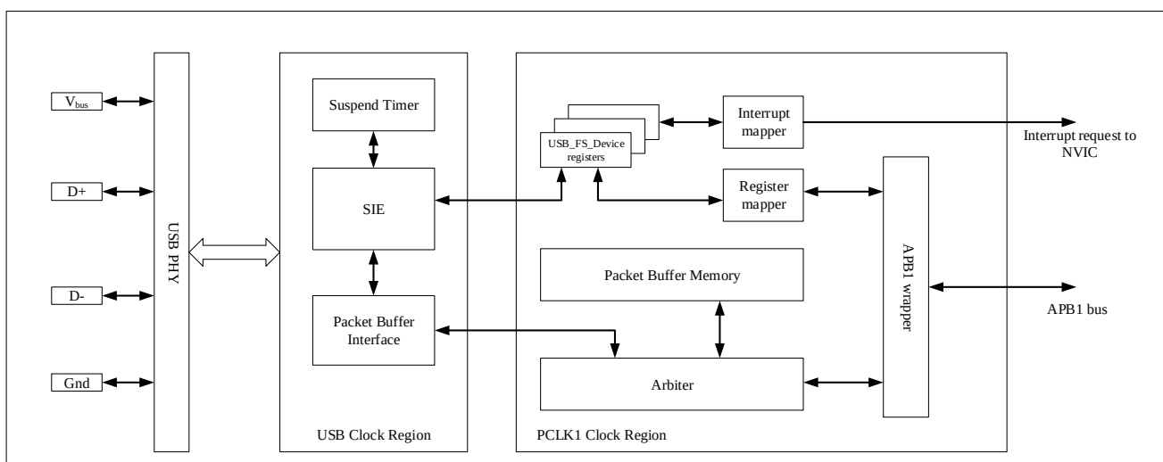
Figure 32-1 USB Device Block Diagram
