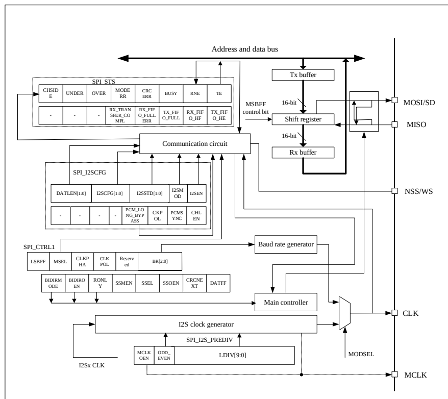
Figure 26-24-14 I2S Block Diagram
