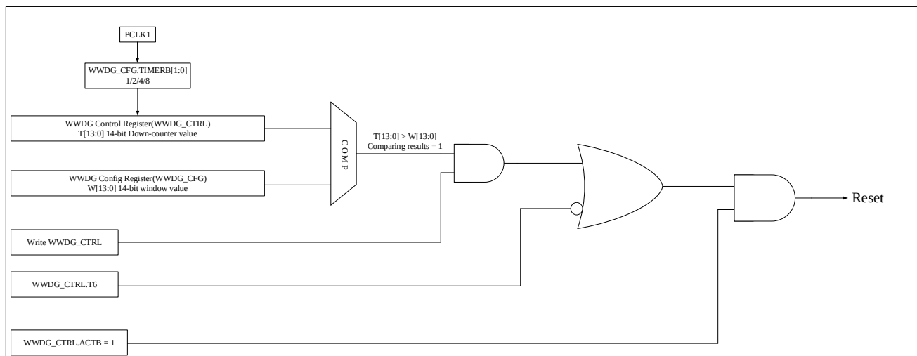
Figure 16-1 Window Watchdog Block Diagram
