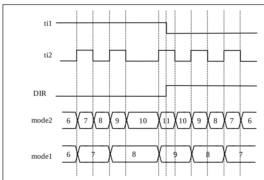
Figure 9-51 Pulse-Level Encoder Mode (CC1P=CC2P=0)
