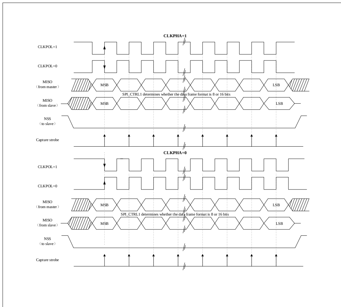
Figure 24-4 Data Clock Timing Diagram
