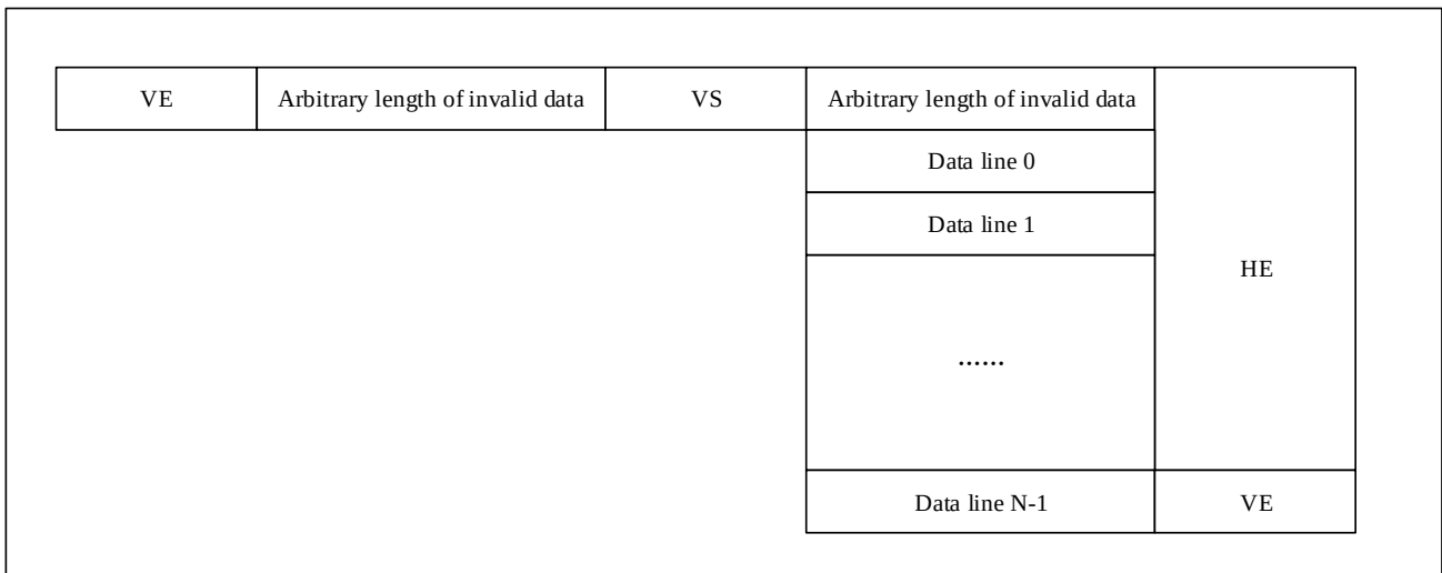
Figure 30-3 Frame Format in Normal Mode
