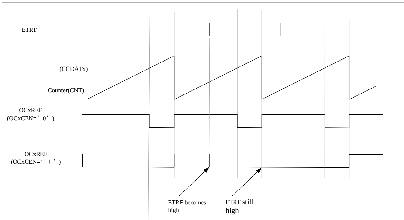
Figure 11-23 Clearing OCxREF of TIMx
