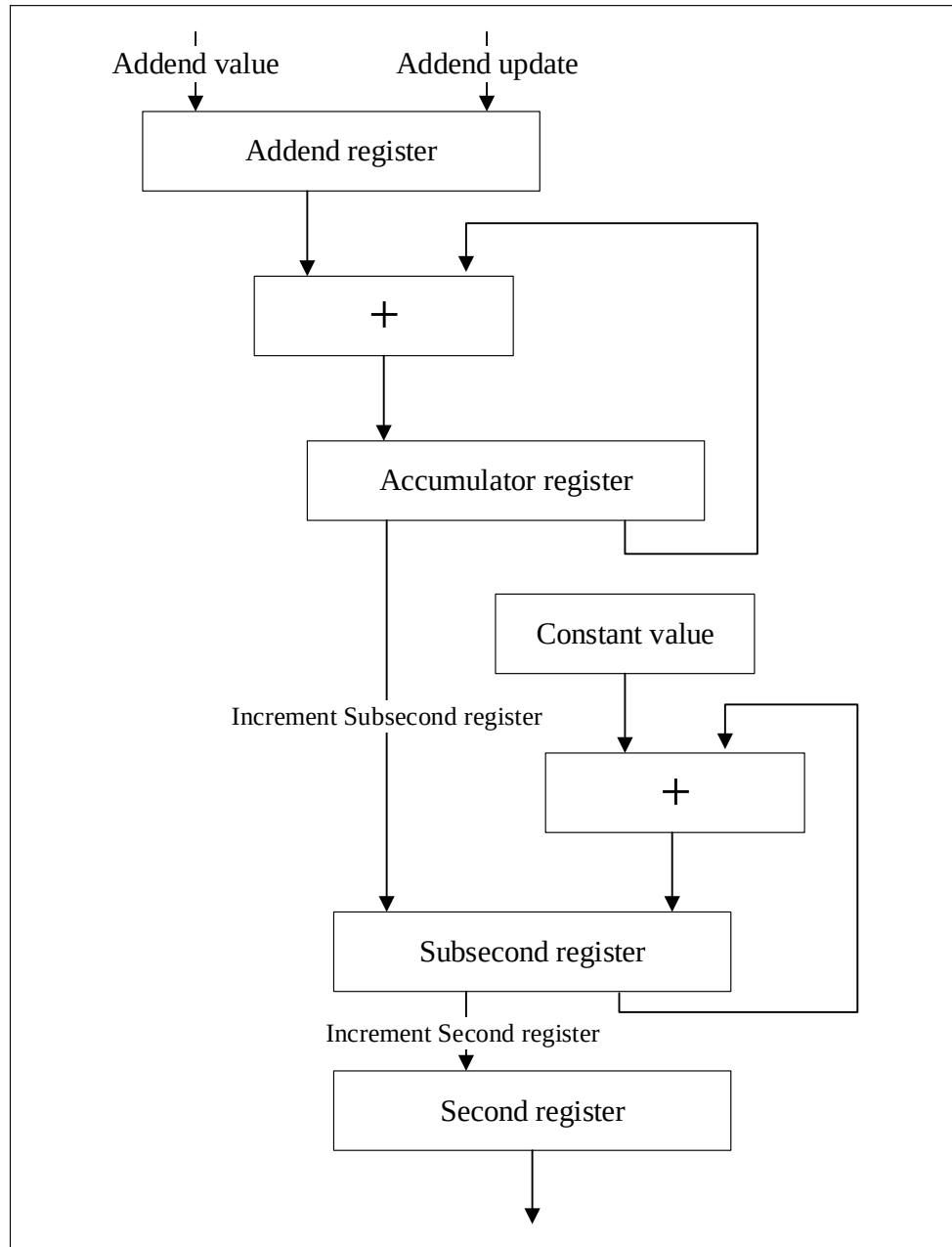
Figure 34-15 System Time Update Using Fine Method
