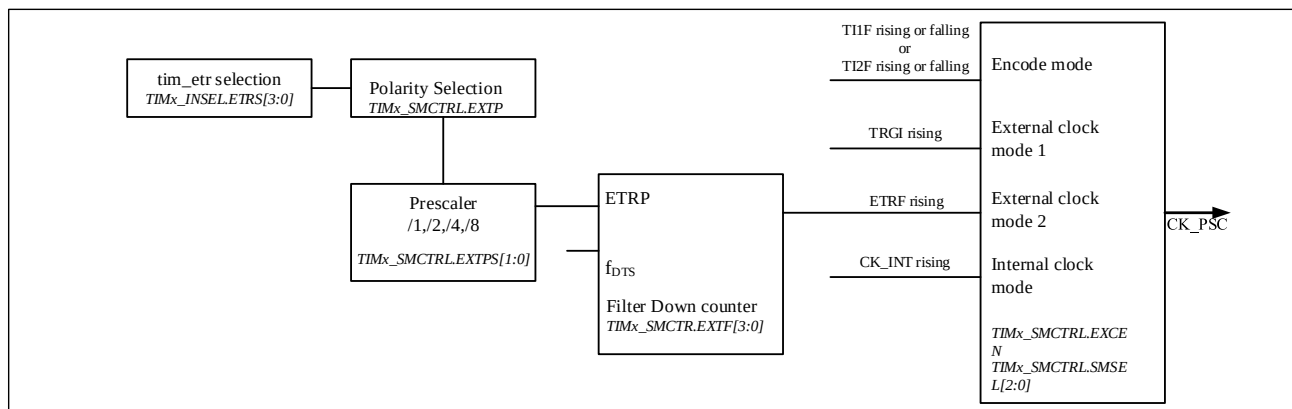
Figure 10-11 External Trigger Input Block Diagram
