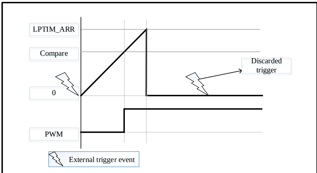
Figure 14-5 LPTIM Output Waveform, Single Counting Mode configuration And Set-Once Mode Activated
