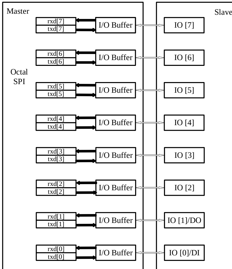
Figure 26-1 Octal SPI Block Diagram
