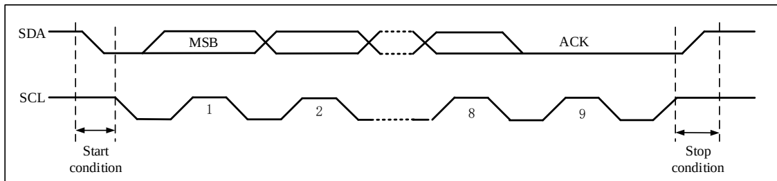
Figure 22-2 I2C Bus Protocol
