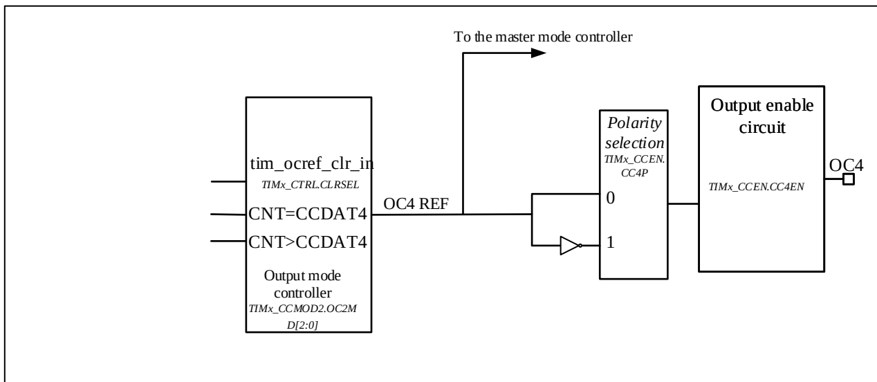
Figure 12-20 Output Part Of Channelx (X = 1,2,3,4;Take Channel 4 As An Example)
