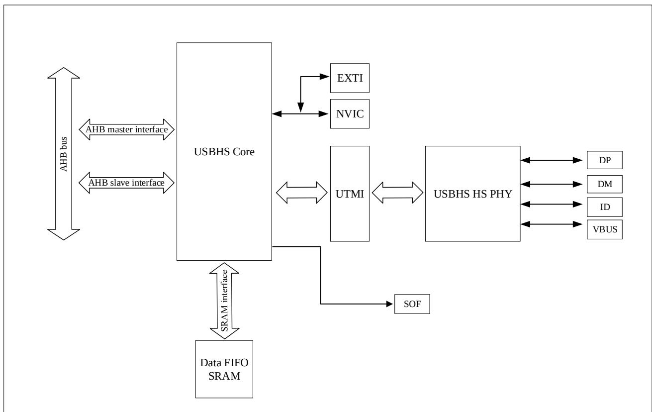
Figure 33-1 USBHS System-Level Block Diagram
