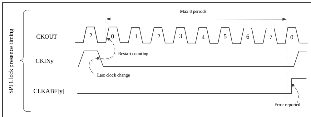
Figure 31-3 Clock absence timing diagram for SPI
