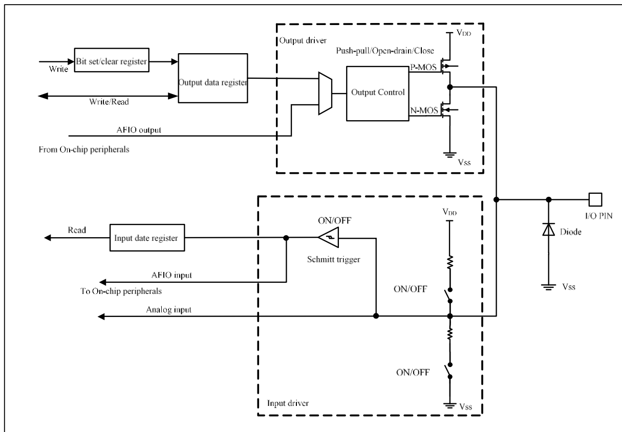
Figure 5-1 Basic Structure of I/O Port
