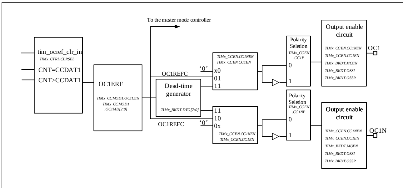
Figure 9-22 Output Part of Channelx (x= 1,2,3,4, Take Channel 1 as Example)
