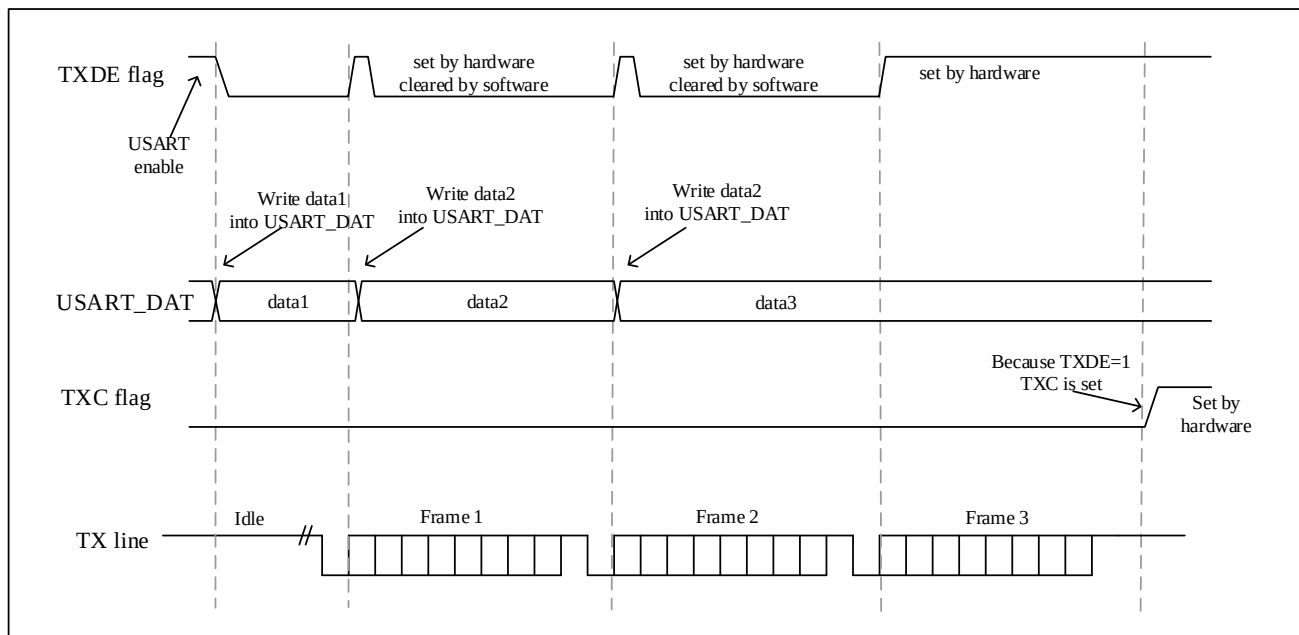
Figure 21-5 TXC/TXDE Changes During Transmission
