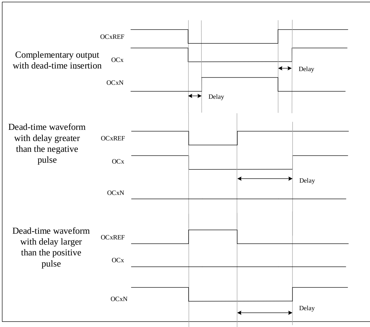
Figure 12-30 Complementary Output with Dead-Time Insertion
