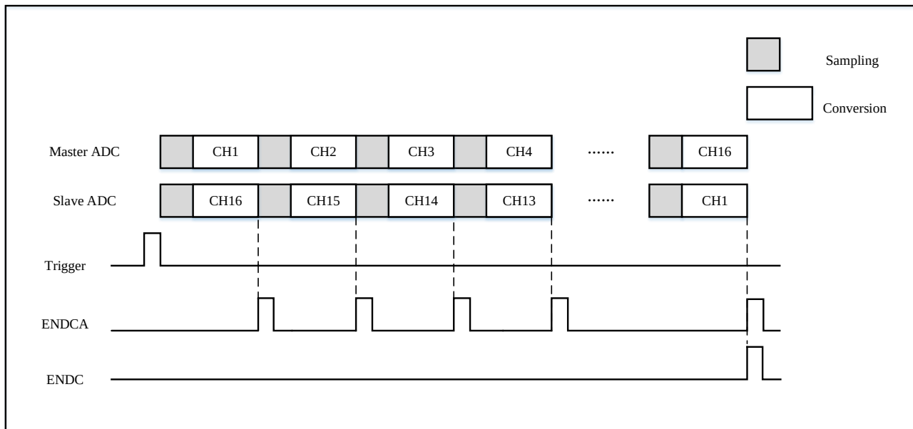
Figure 17-23 Synchronous regular mode with 16 channels.
