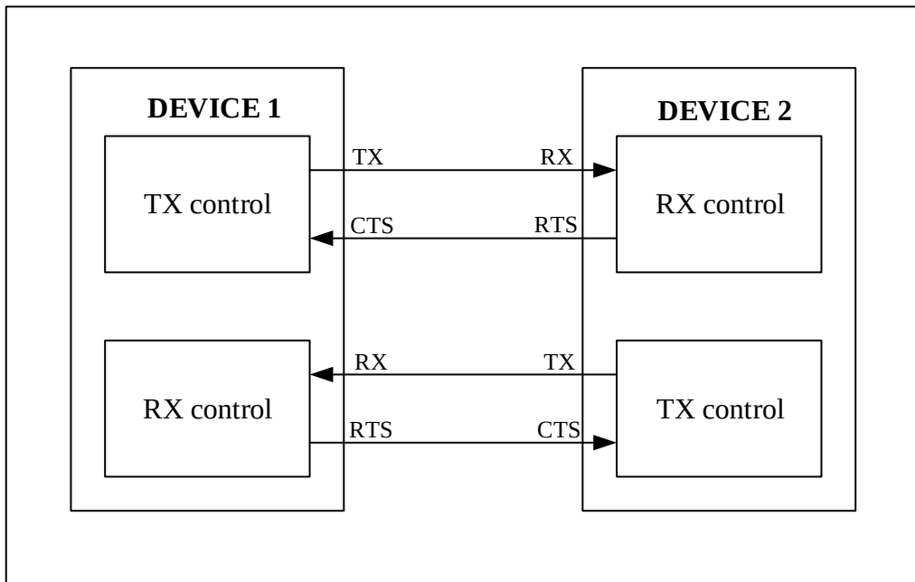
Figure 21-9 Hardware Flow Control Between Two USART
