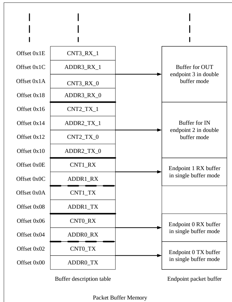
Figure 32-3 The Relationship between The Buffer Description Table and The Endpoint Packet Buffer
