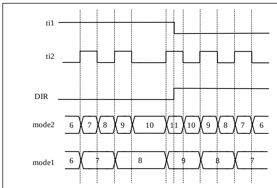
Figure 11-40 Pulse Level Encoding Mode (CC1P=CC2P=0)
