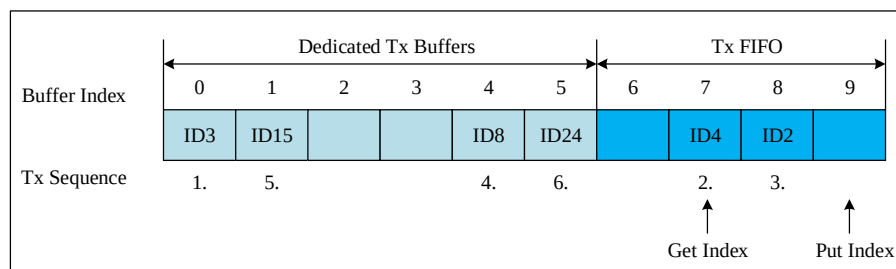
Figure 23-12 FDCAN dedicated Tx Buffer and Tx FIFO Hybrid Configuration Example Diagram
