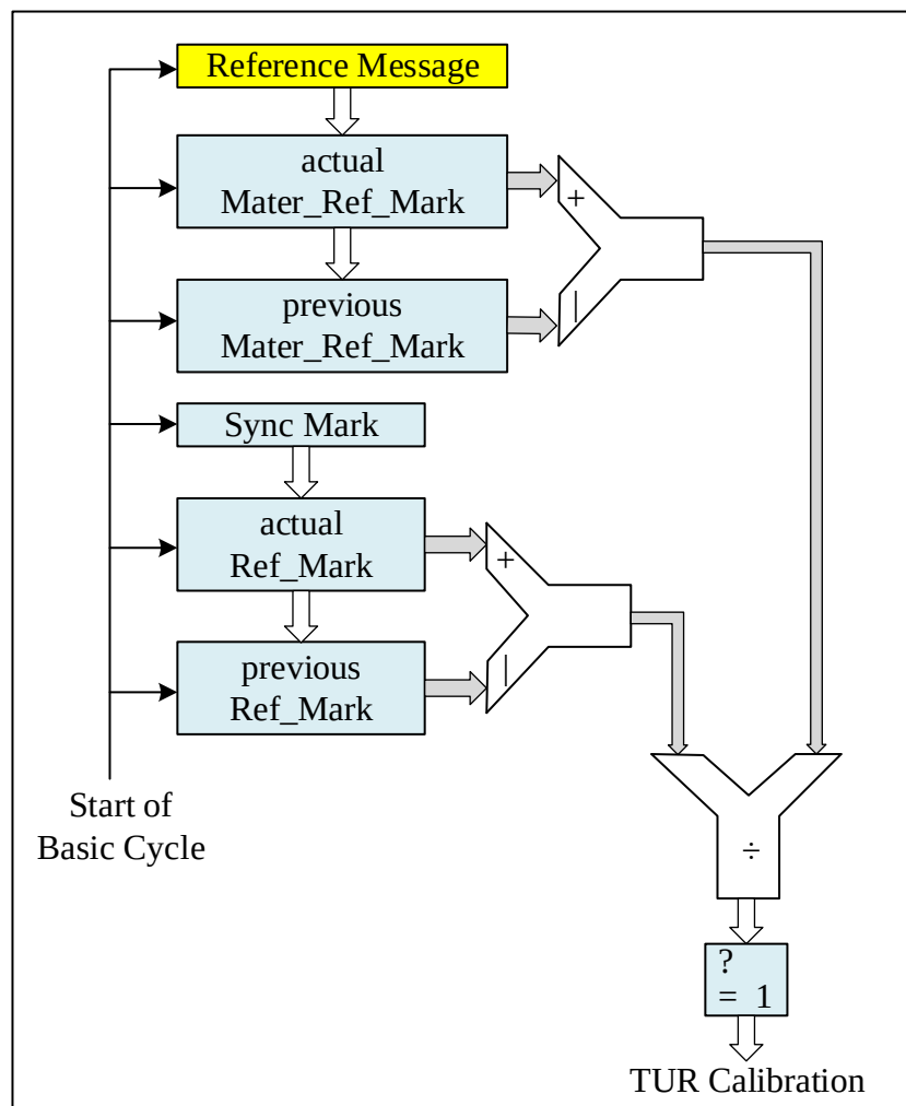
Figure 23-16 TTCAN level 0 and level 2 drift compensation
