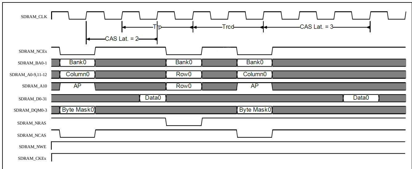
Figure 29-9 Single SDRAM read with Auto Precharge
