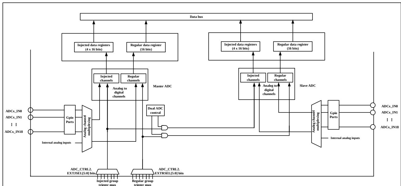
Figure 17-22 Dual ADC Block Diagram
