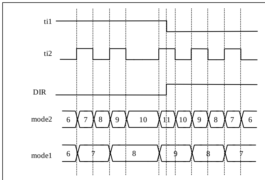
Figure 12-49 Pulse Level Encoding Mode (CC1P=CC2P=0)
