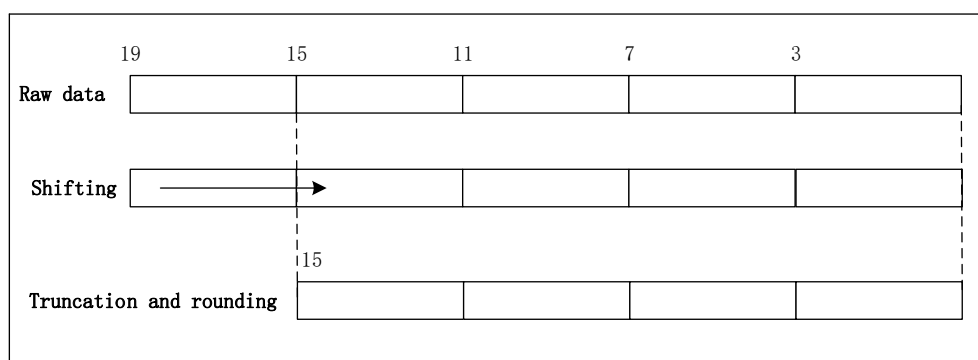
Figure 17-15 Diagram of data processing after a 5-bit right shift and rounding
