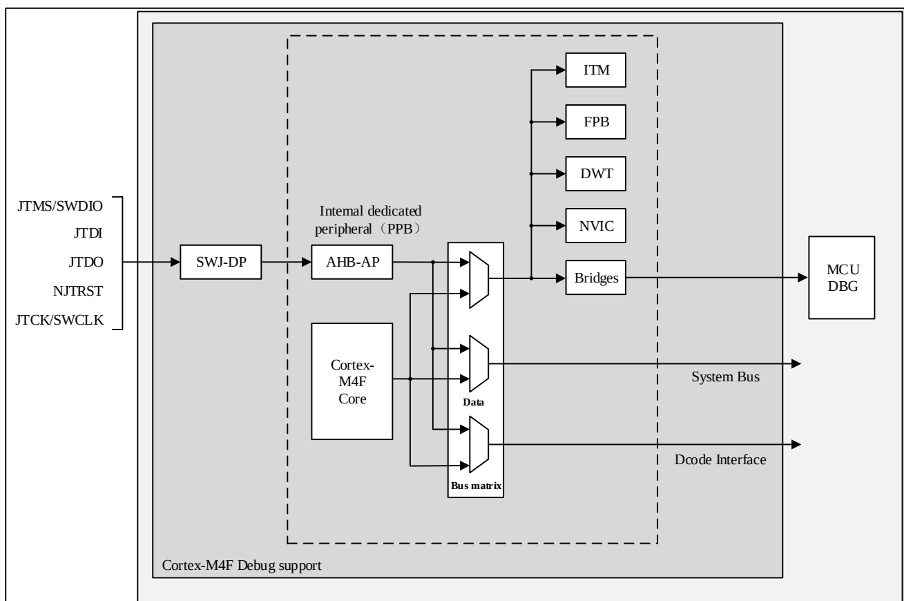
Figure 37-1 Chip Level And Cortex™-M4F Level Debugging Block Diagram
