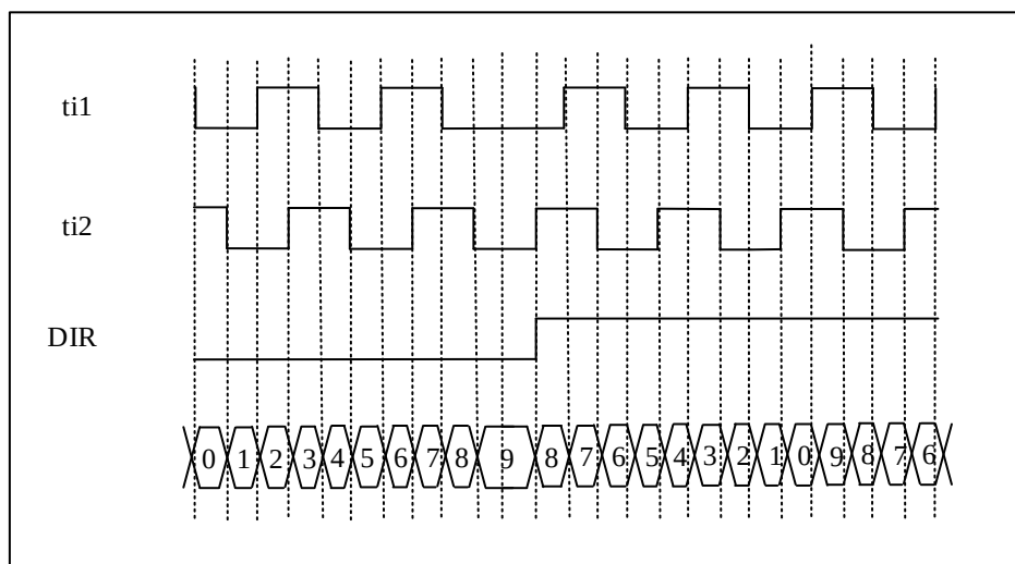
Figure 9-46 The Encoder Counts on Both TI1 and TI2
