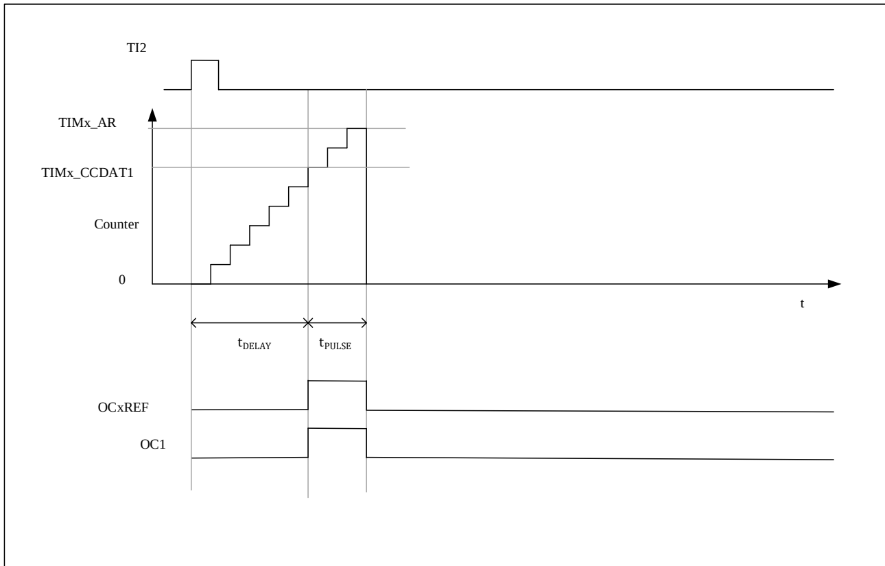
Figure 12-26 Example Of One-Pulse Mode
