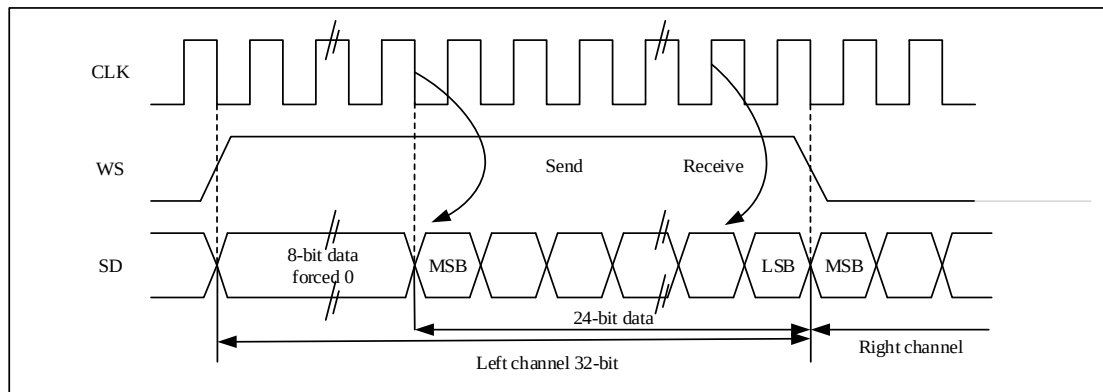
Figure 26-24-26 LSB Aligns 24-Bit Data, CLKPOL = 0
