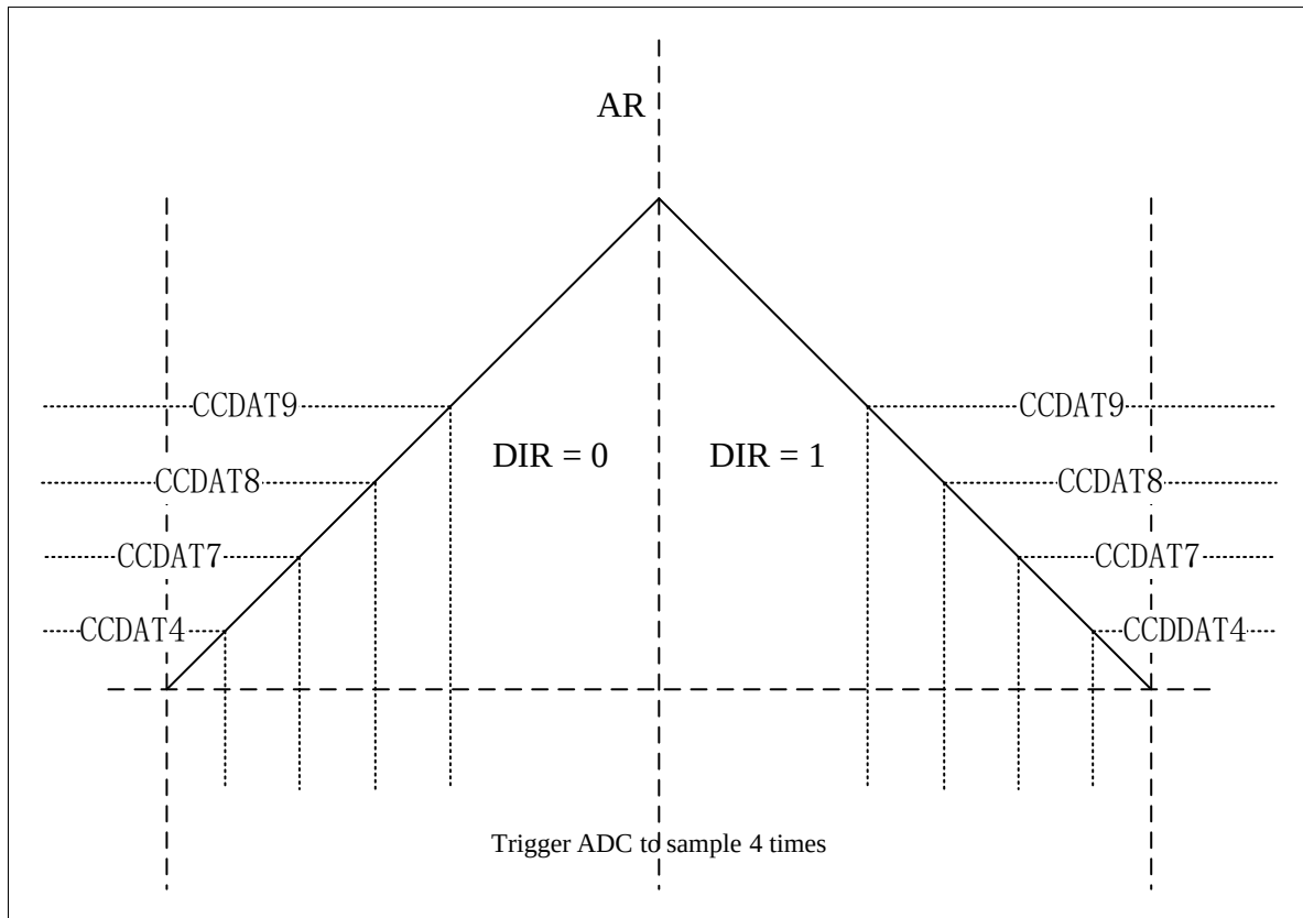
Figure 9-11 CCDATx(x=4,7,8,9) Triggers ADC When DIR = 0 or DIR = 1
