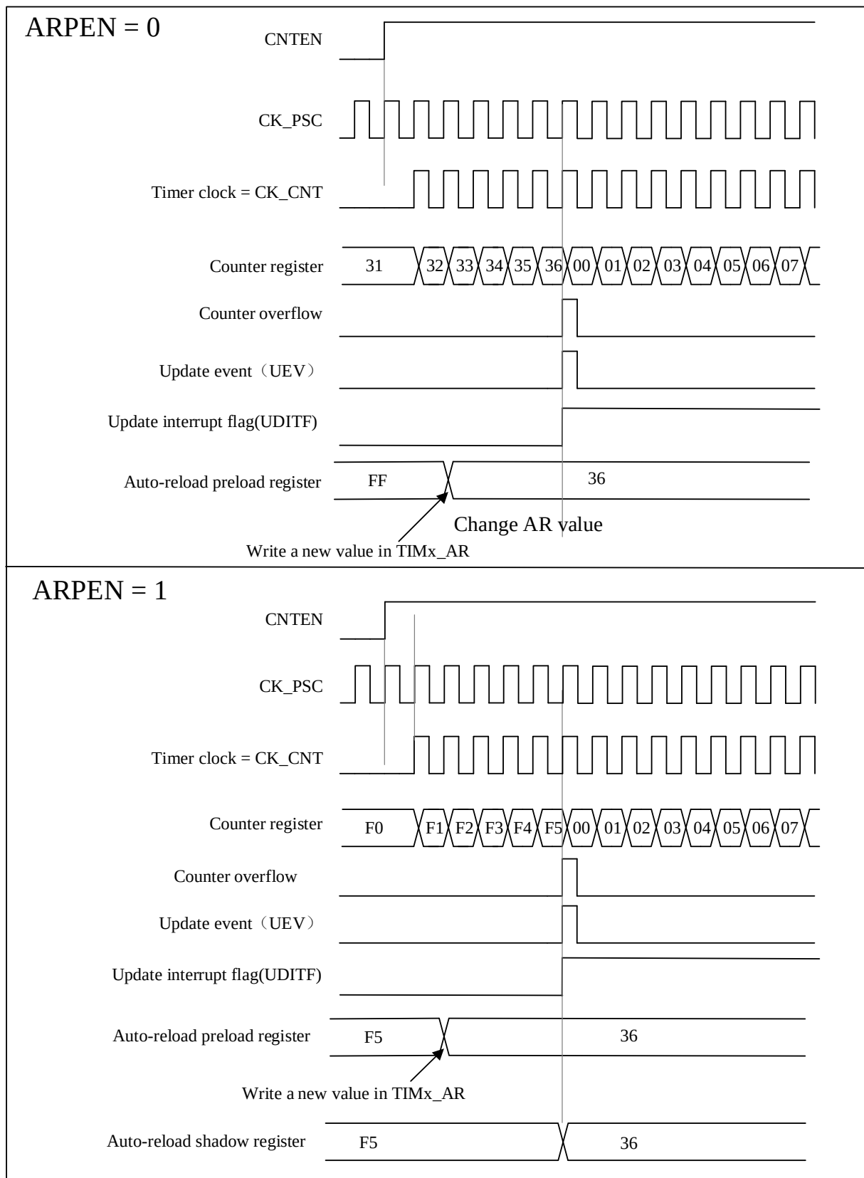
Figure 13-4 Timing diagram of up-counting and update event when ARPEN=0/1
