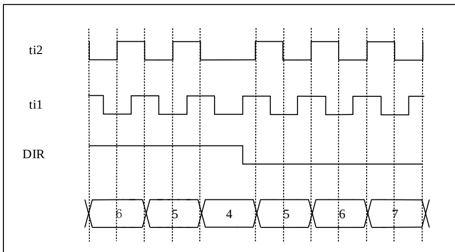
Figure 11-37 When T1 is high level, the counter only counts on TI2
