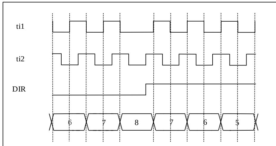
Figure 12-46 When T1 is high level, the counter counts only on TI2
