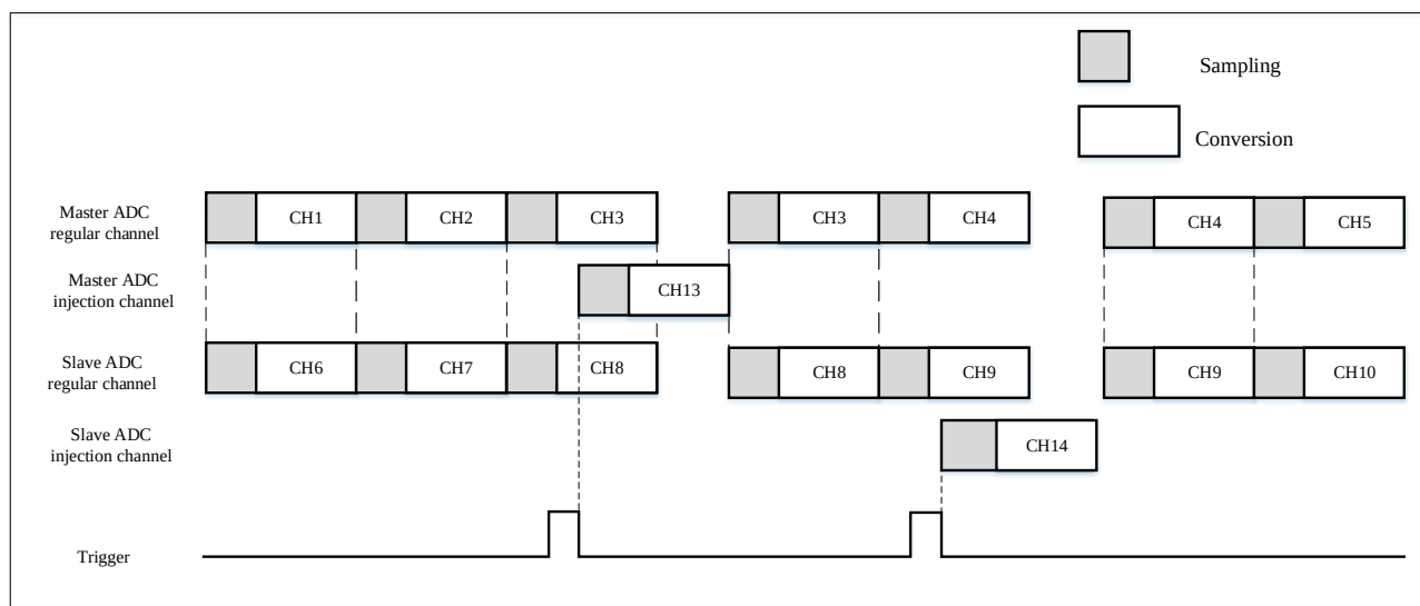
Figure 17-33 Combination of Alternate Mode and Synchronous Regular Mode
