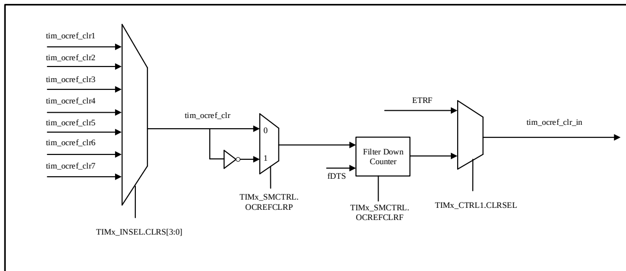
Figure 11-22 Clearing OCxREF Signal By External Event
