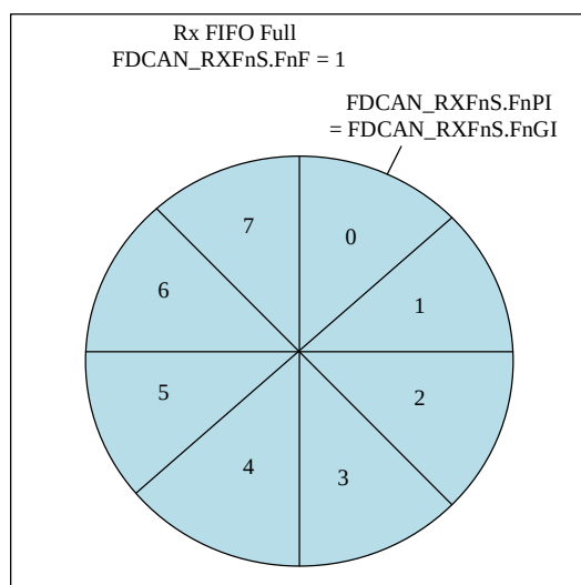
Figure 23-10 FDCAN Rx FIFO Full
