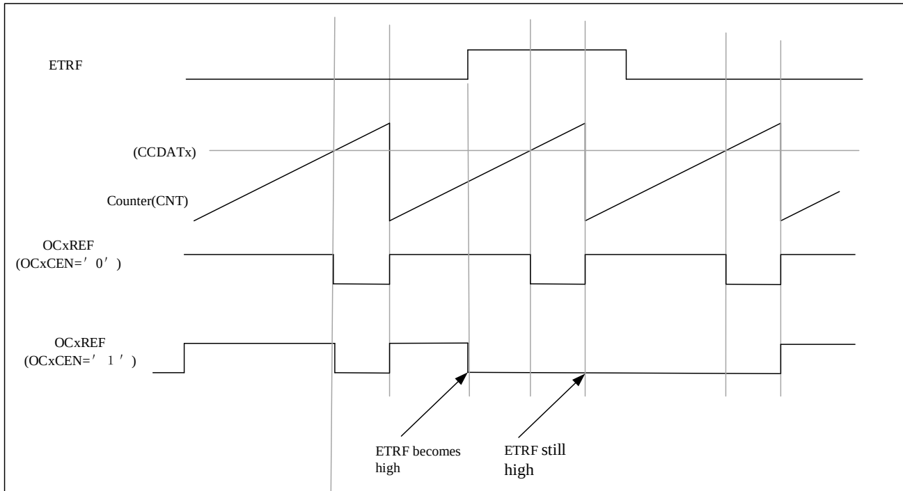
Figure 9-29 Clearing the Ocxref of TIMx
