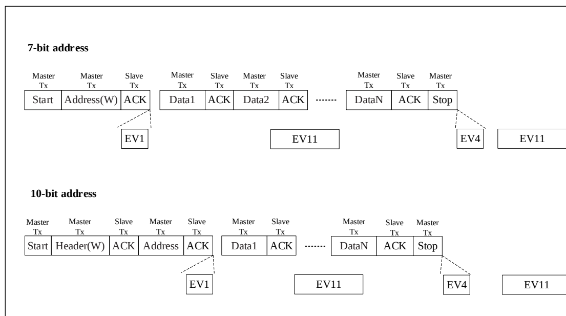
Figure 22-6 FIFO Enable opening the slave receiver to transmit sequences.
