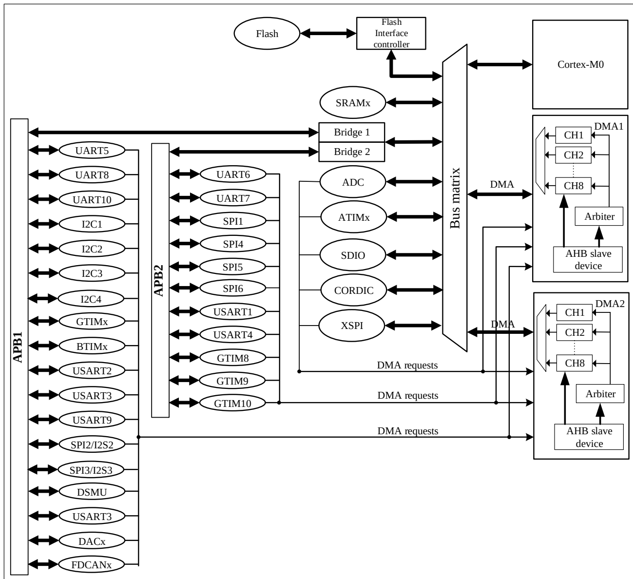
Figure 7-1 DMA Block Diagram
