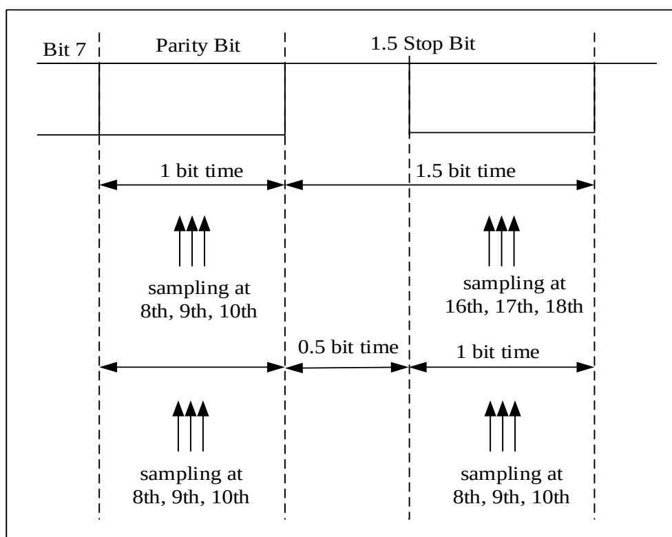
Figure 21-23 Use 1.5 Stop Bits To Detect Parity Errors
