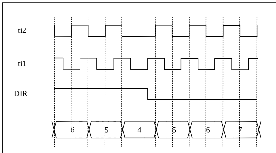
Figure 9-48 The Counter Counts Only on TI2 When TI1 is High
