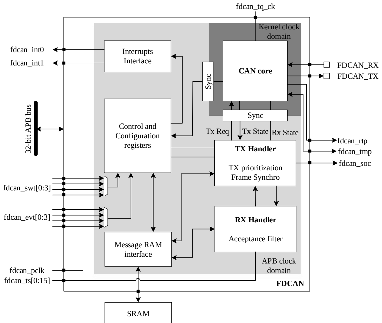
Figure 23-2 FDCAN Functional Block Diagram
