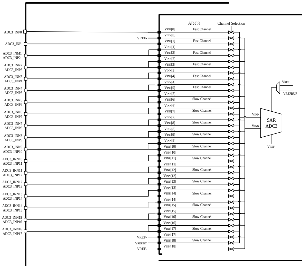
Figure 17-4 Connection ADC3 channels
