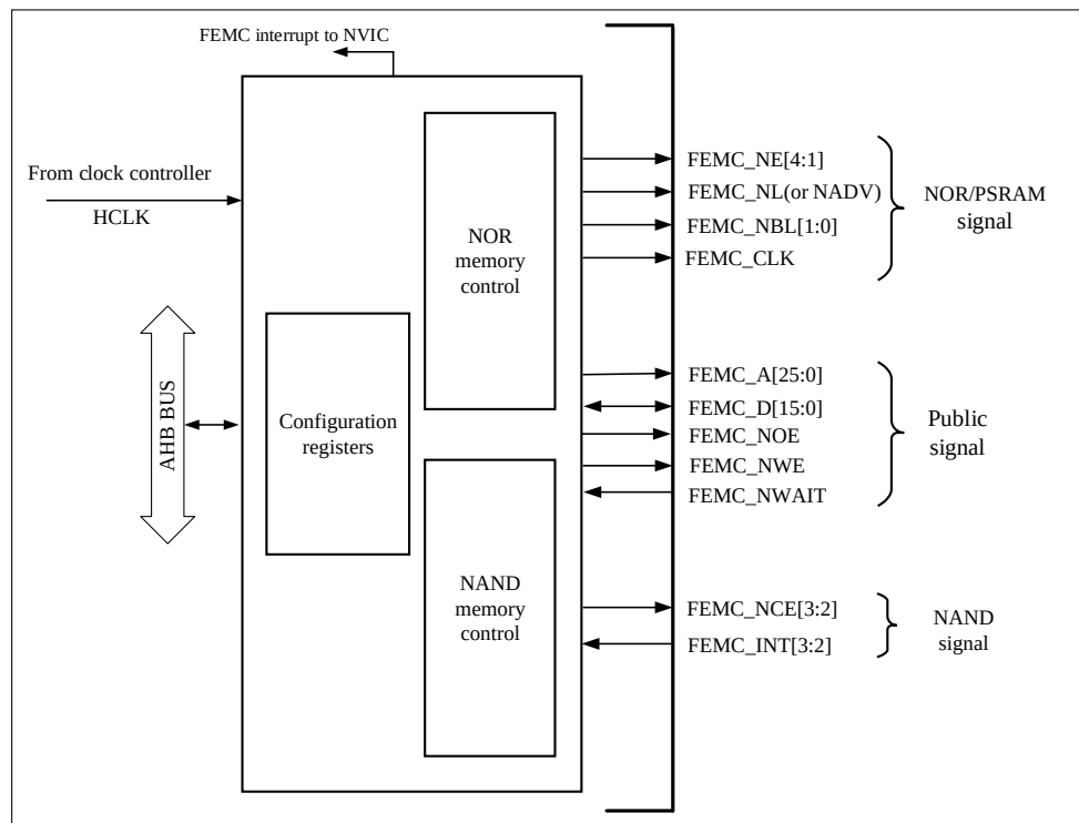
Figure 28-1 FEMC Block Diagram
