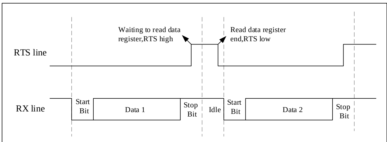
Figure 21-10 RTS Flow Control
