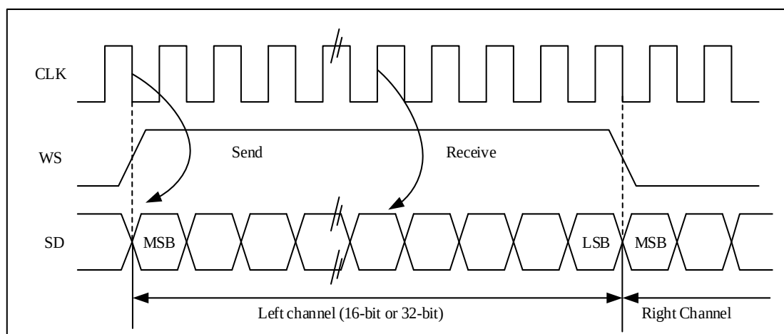
Figure 26-24-22 The MSB is Aligned With 16-Bit or 32-Bit Full Precision, CLKPOL = 0
