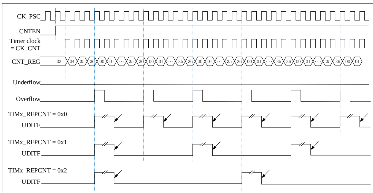
Figure 9-13 Repeat Count Sequence Diagram in Up-Counting Mode
