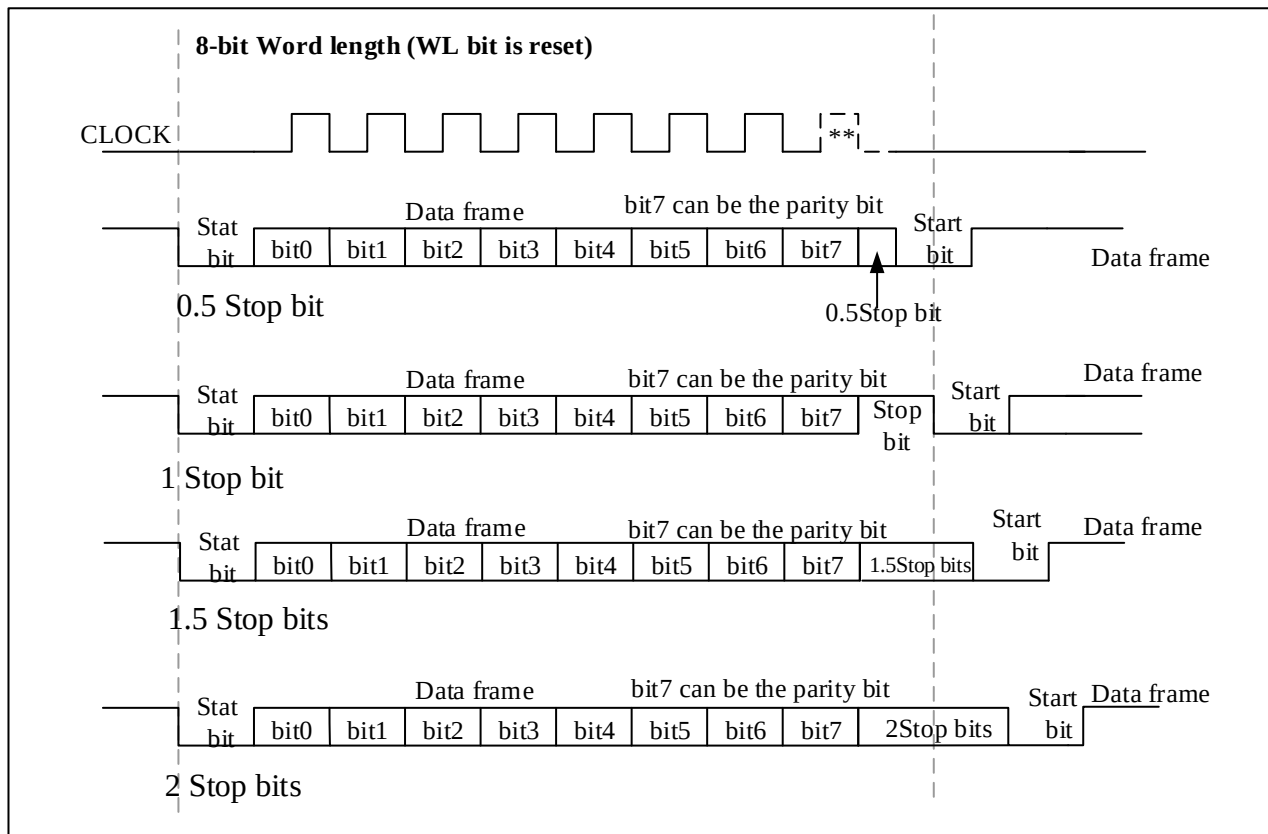
Figure 21-4 Configuration Stop Bit
