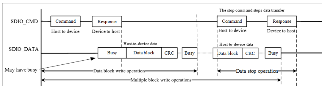
Figure 30-3 SDIO (Multi) Data Block Write Operation
