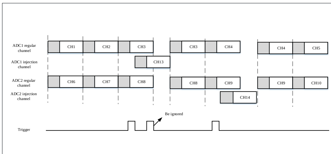
Figure 17-34 Injection trigger occurs during injection conversion
