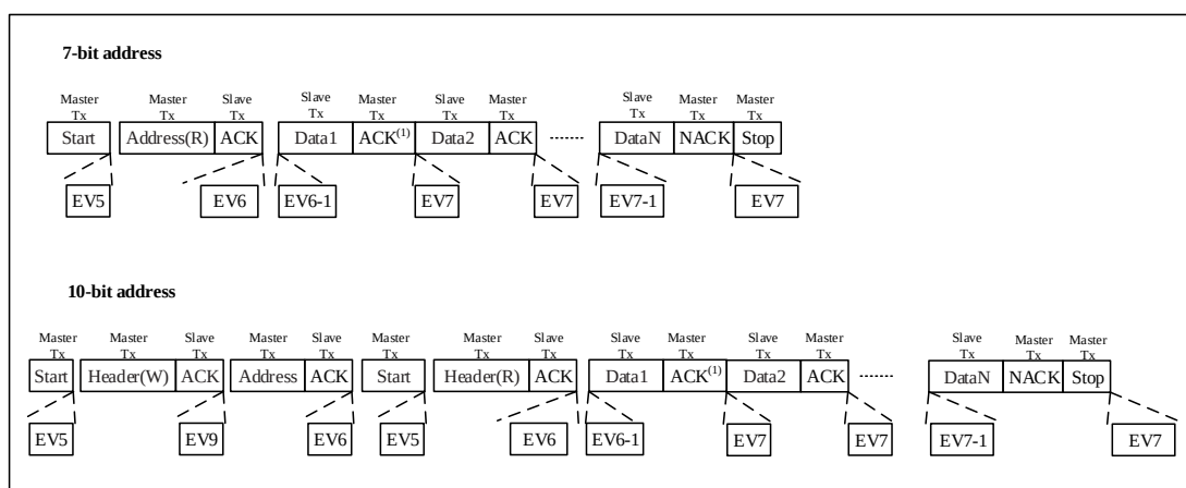
Figure 22-9 Master receiver transmission sequence diagram
