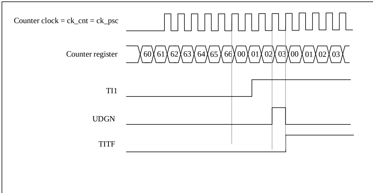
Figure 10-24 Control Circuit In Reset Mode
