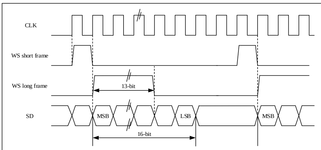
Figure 26-24-29 PCM Standard Waveform (16-Bit Extended to 32-Bit Packet Frame)
