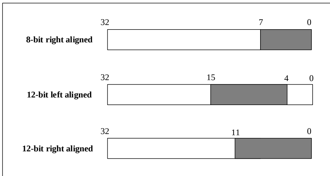
Figure 18-2 Data Register Of Single DAC Channel Mode
