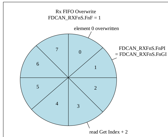
Figure 23-11 FDCAN Rx FIFO Overwrite Example
