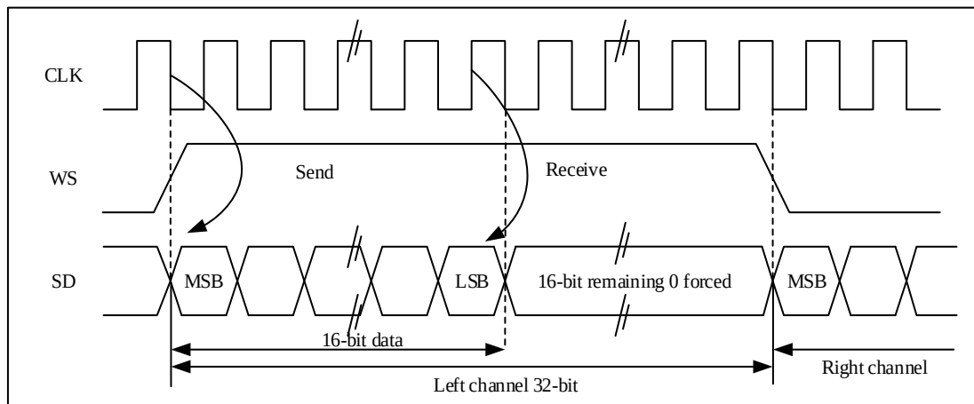
Figure 26-24-24 MSB-Aligned 16-Bit Data Is Extended to 32-Bit Packet Frame, CLKPOL = 0
