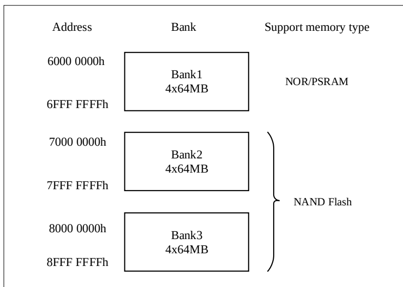
Figure 28-2 FEMC Memory Blocks
