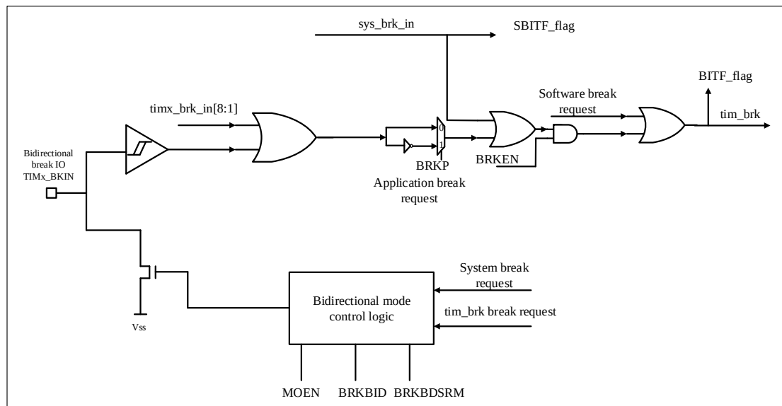
Figure 9-36 Output Redirection (tim_brk2 Request Not Represented)
