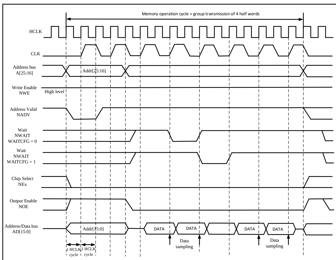
Figure 28-18 Synchronous Multiplexed Read Mode - NOR, PSRAM (CRAM)
