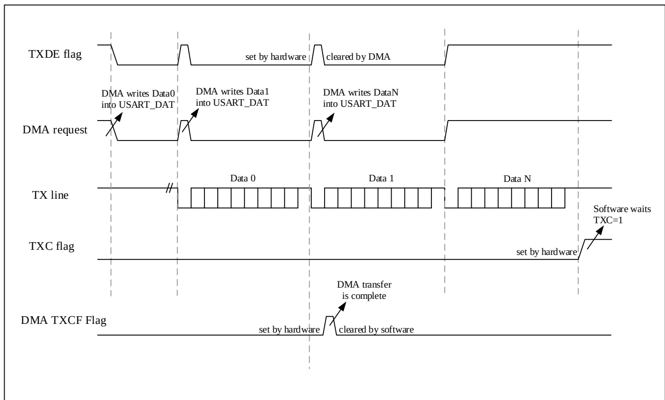
Figure 21-7 DMA Transmission
