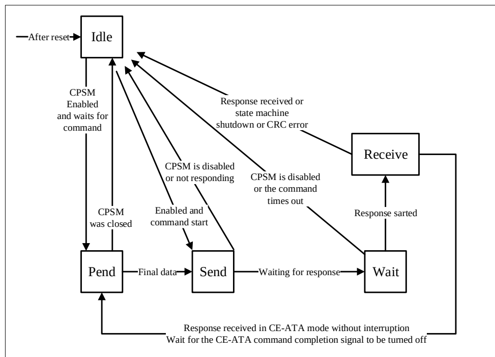
Figure 30-10 Command Path State Machine (CPSM)
