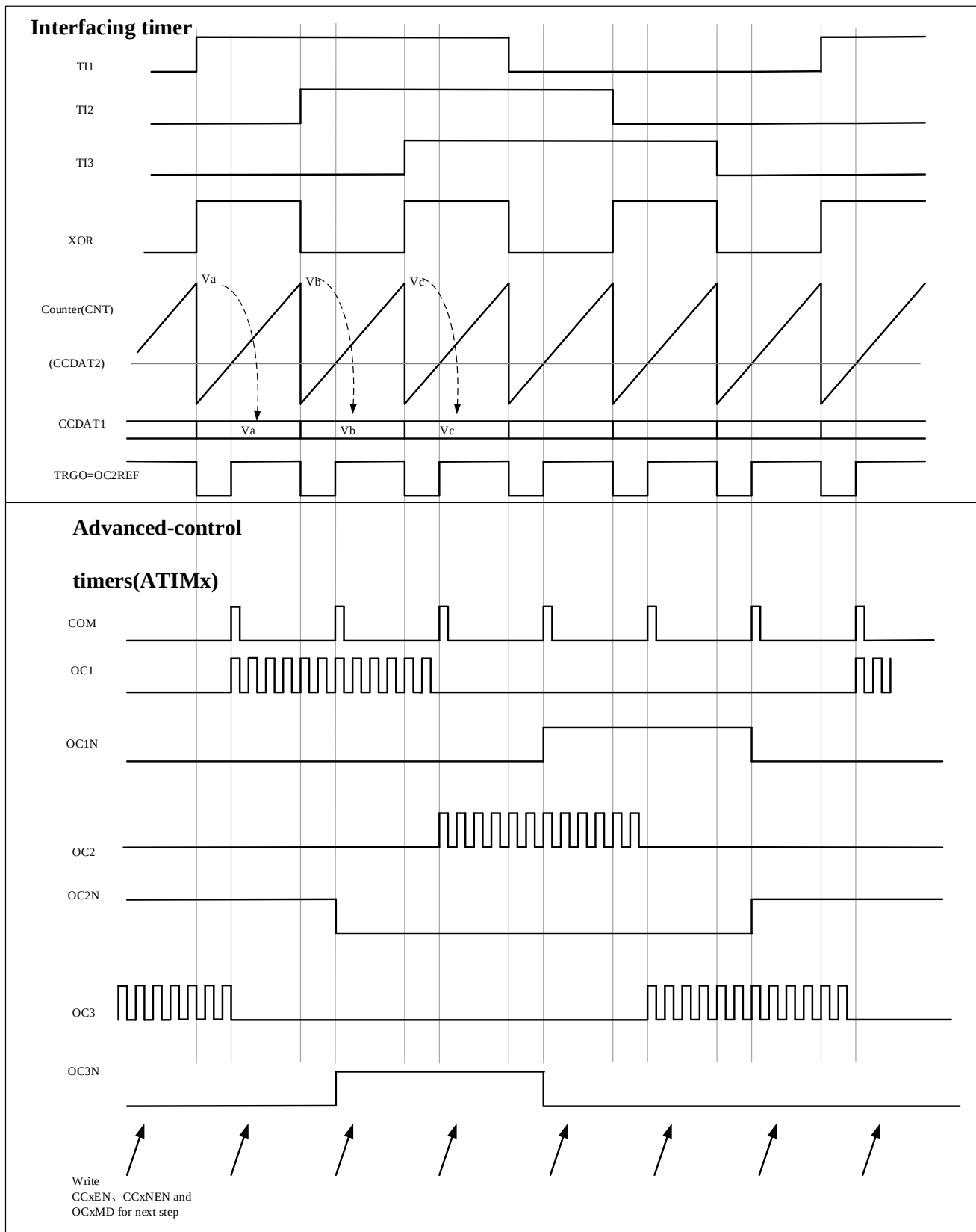
Figure 9-54 Example of Hall Sensor Interface
