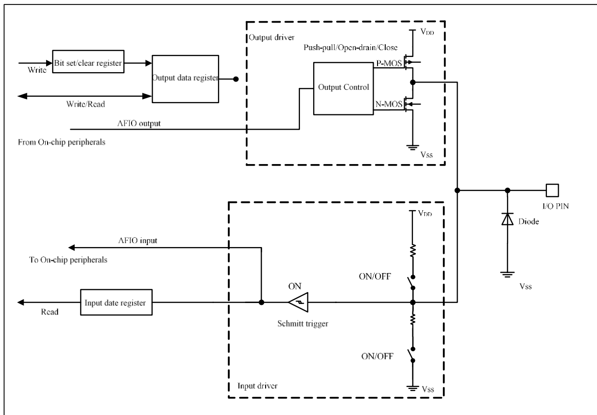
Figure 5-4 Alternate Function Configuration
