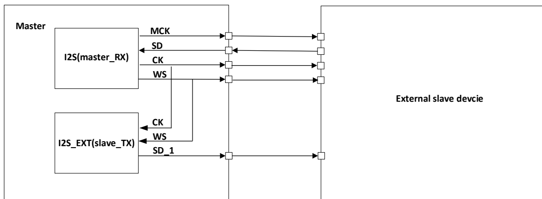
Figure 24-16 I2S master receive (I2SCFG=11), I2S_EXT slave transmit (I2SCFG=00)
