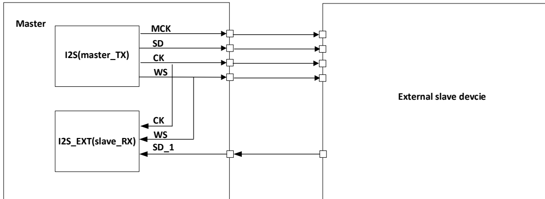
Figure 24-15 I2S master transmit (I2SCFG=10), I2S_EXT slave receive (I2SCFG=01)
