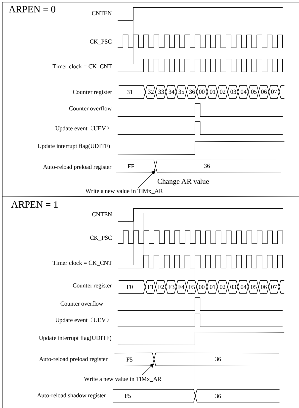
Figure 12-4 Timing Diagram Of The Up-Counting With Update Event When ARPEN=0/1
