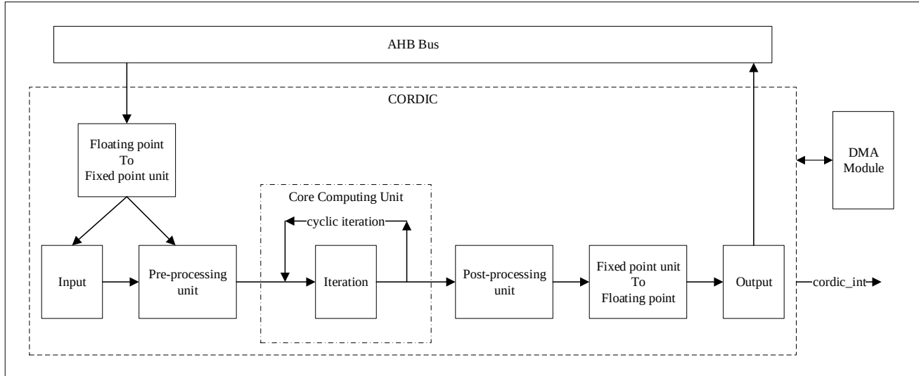
Figure 20-1 CORDIC Block Diagram
