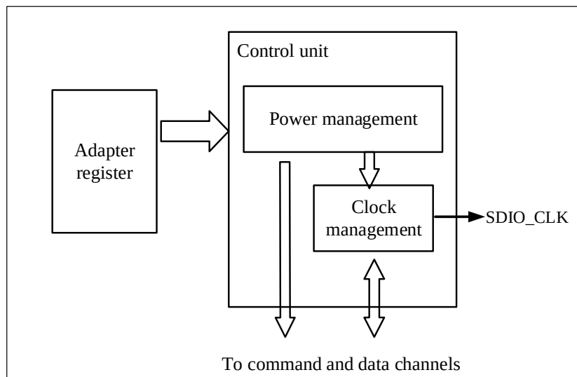
Figure 30-8 Control Unit
