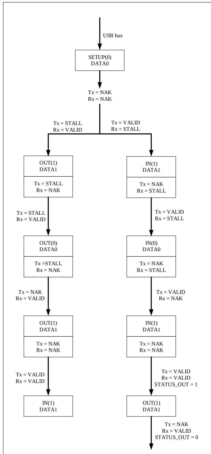
Figure 32-5 Control Transfer
