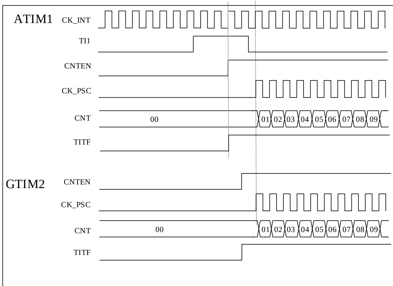
Figure 10-32 Triggers ATIM1 And GTIM2 Using The TI1 Input Of ATIM1
