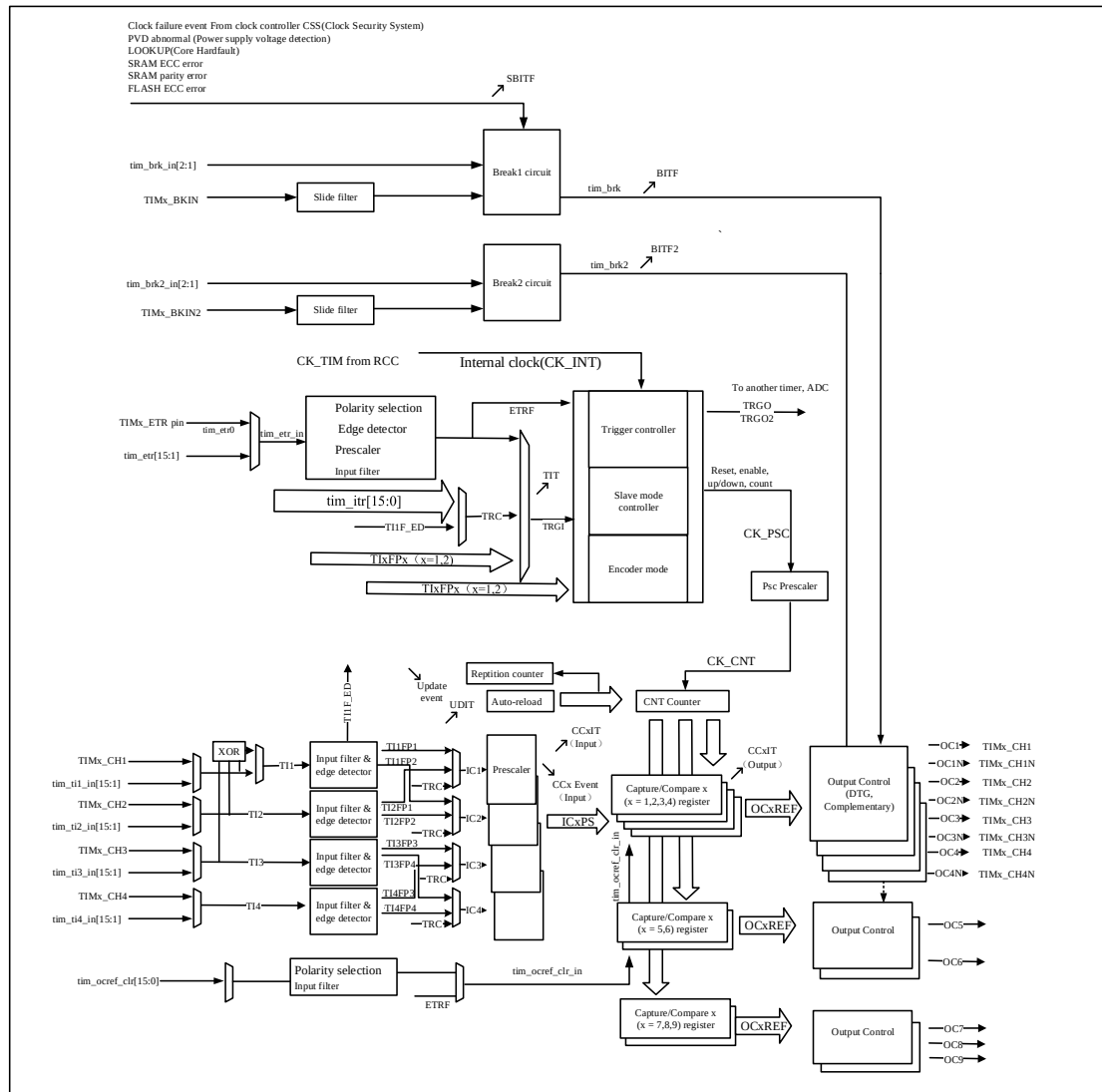
Figure 9-1 Block Diagram of ATIMx
