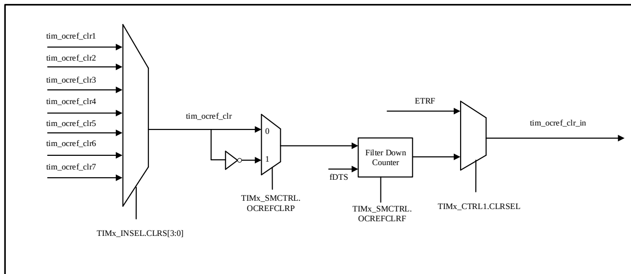
Figure 10-22 Clearing OCxREF Signal By External Event
