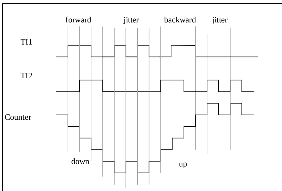
Figure 10-39 Encoder Interface Mode Example With IC1FP1 Polarity Inverted
