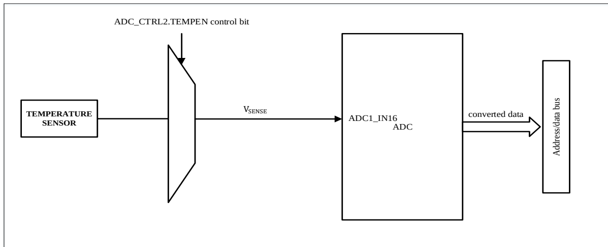
Figure 17-36 Temperature Sensor Channel Diagram
