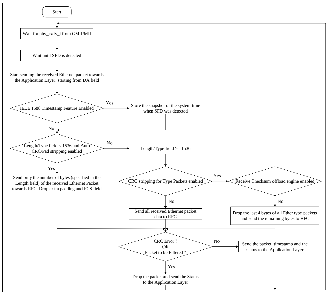
Figure 34-7 MAC Receive Flow Transmission
