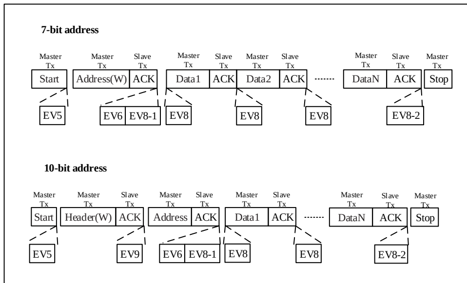
Figure 22-7 Master Transmitter Transfer Sequence Diagram
