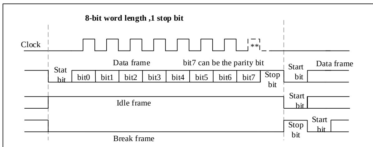
Figure 21-2 Programming for Word Length = 8
