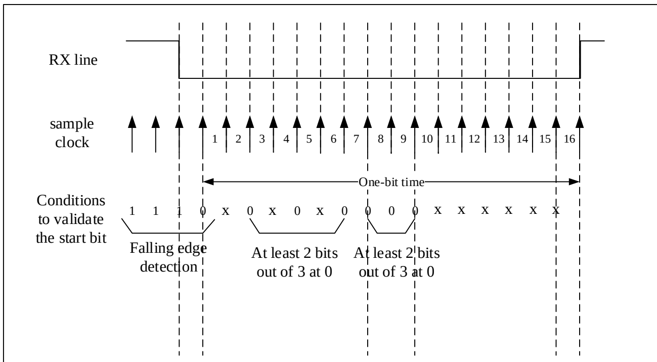
Figure 21-6 Start Bit Detection
