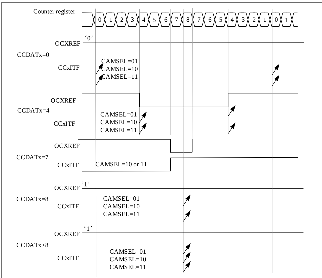
Figure 12-23 Center-Aligned PWM Waveform (AR=8)
