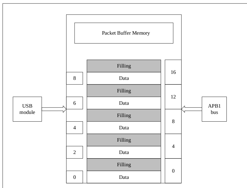
Figure 32-2 Accessing Packet Buffer Memory by the User Applications
