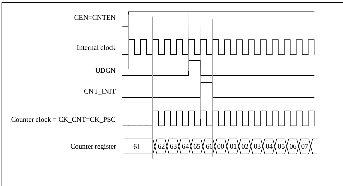
Figure 10-8 Control Circuit In Normal Mode With Internal Clock Divided By 1
