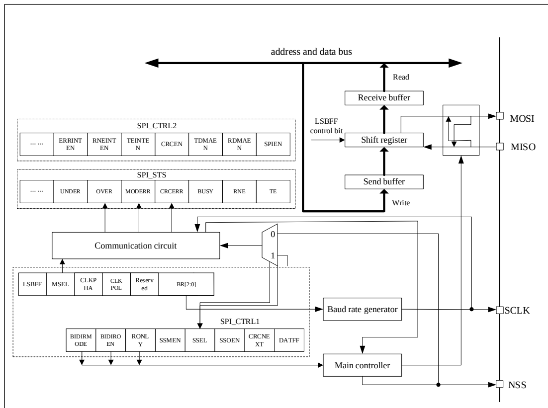
Figure 24-1 SPI Block Diagram
