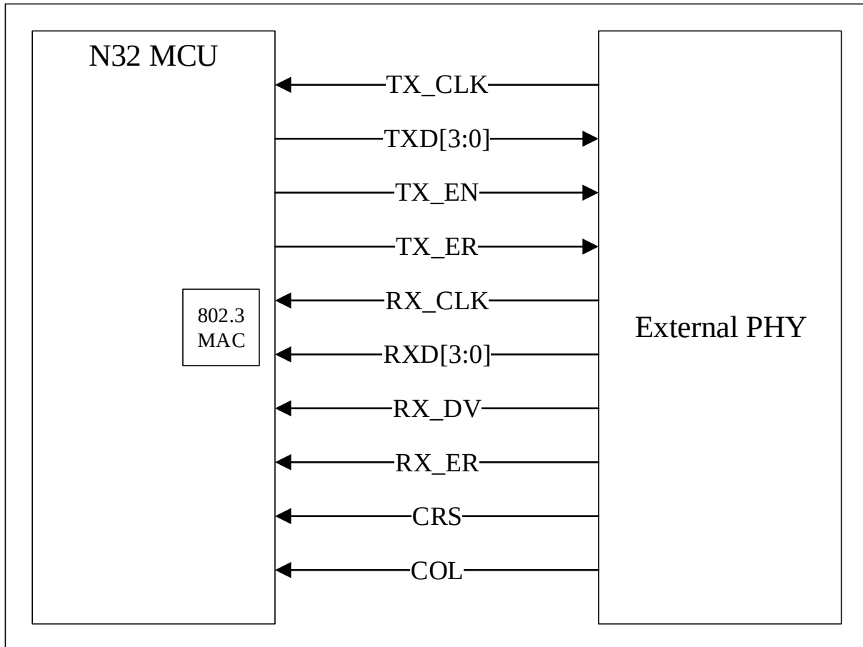
Figure 34-9 MII Interface
