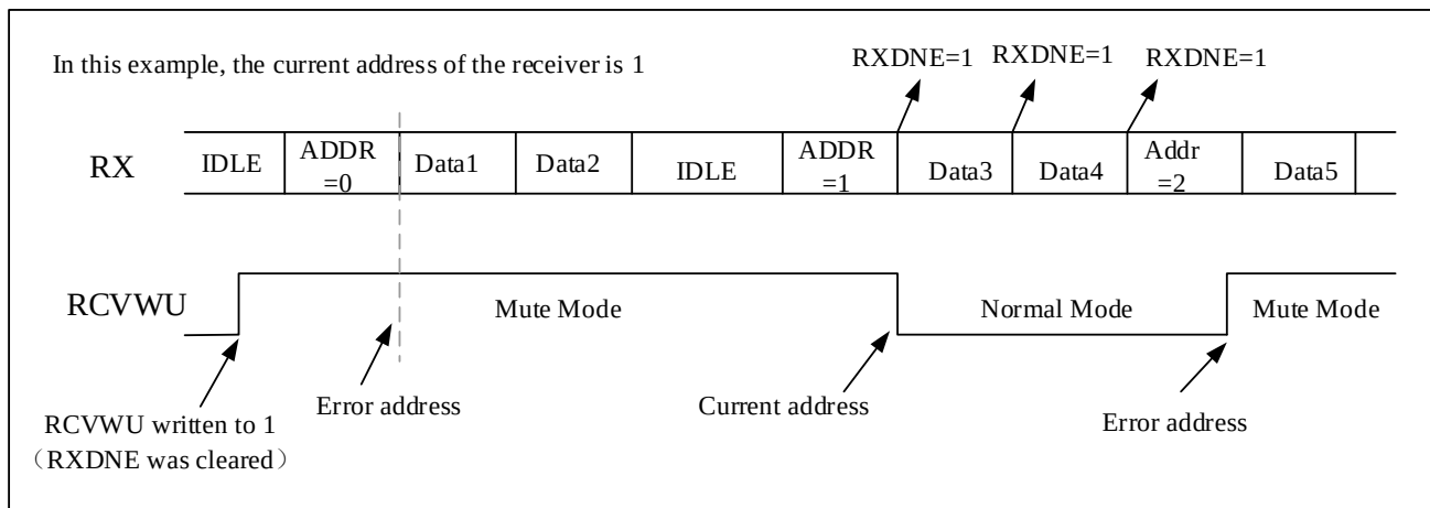
Figure 21-13 Mute Mode Detected Using Address Mark
