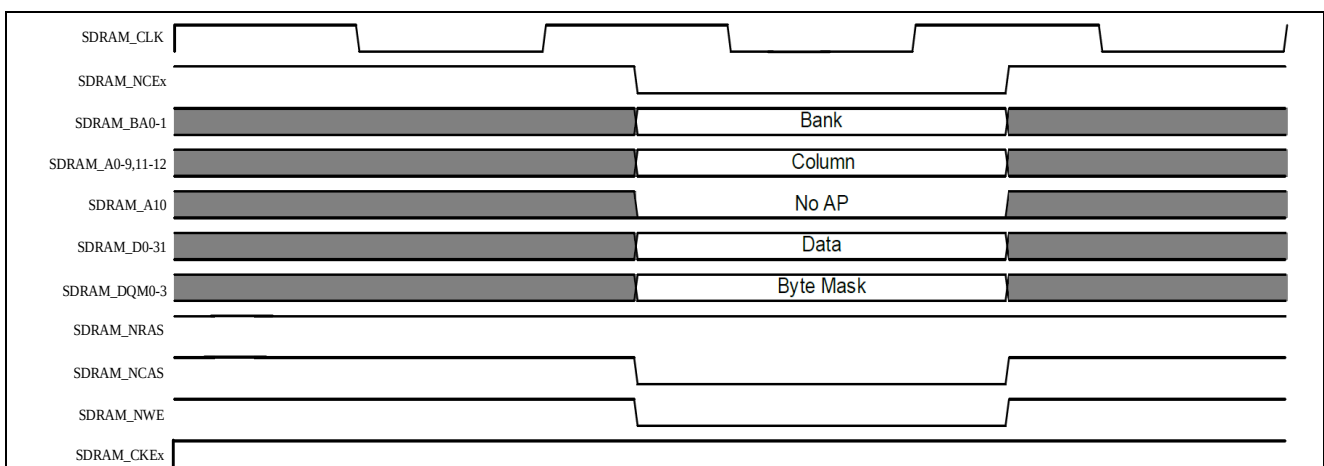
Figure 29-3 Single SDRAM Write without Auto Precharge
