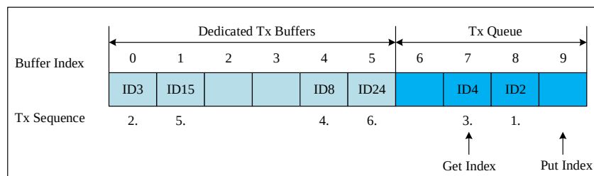
Figure 23-13 FDCAN dedicated Tx Buffer and Tx Queue Hybrid Configuration Example Diagram
