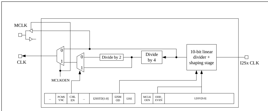
Figure 26-24-30 I2S Clock Generator Structure
