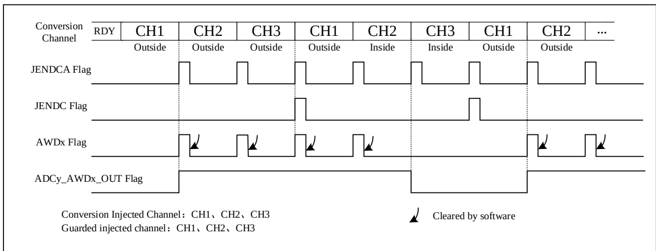
Figure 17-11 Generation of ADCx_AWDy_OUT (on multiple injected channels)
