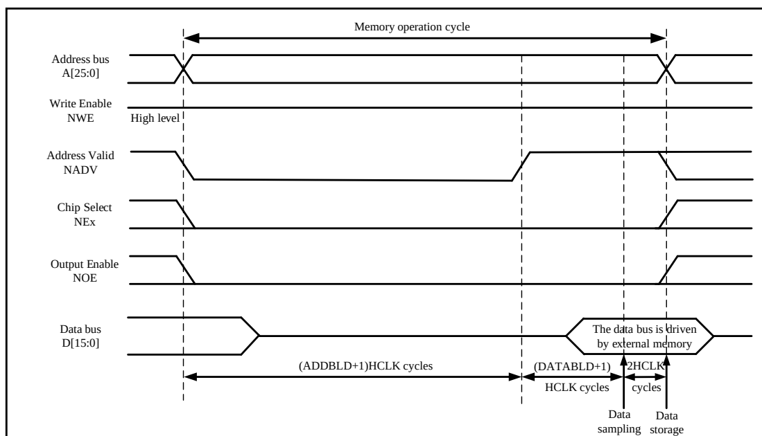
Figure 28-5 Mode 2/B Read Accesses
