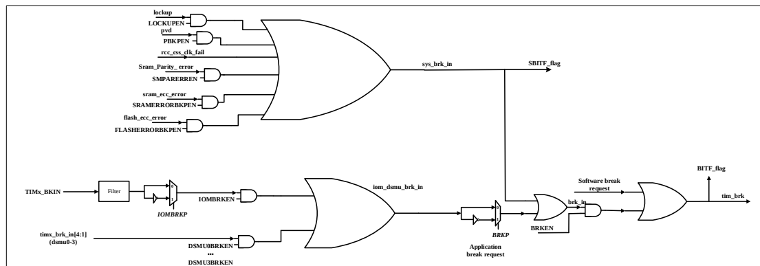
Figure 12-31 Break input
