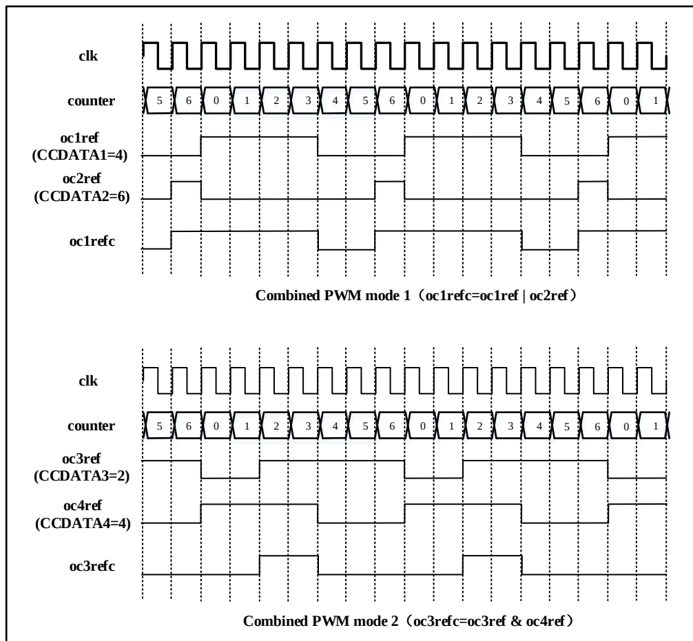
Figure 12-25 Combined PWM mode on channels 1 and 3
