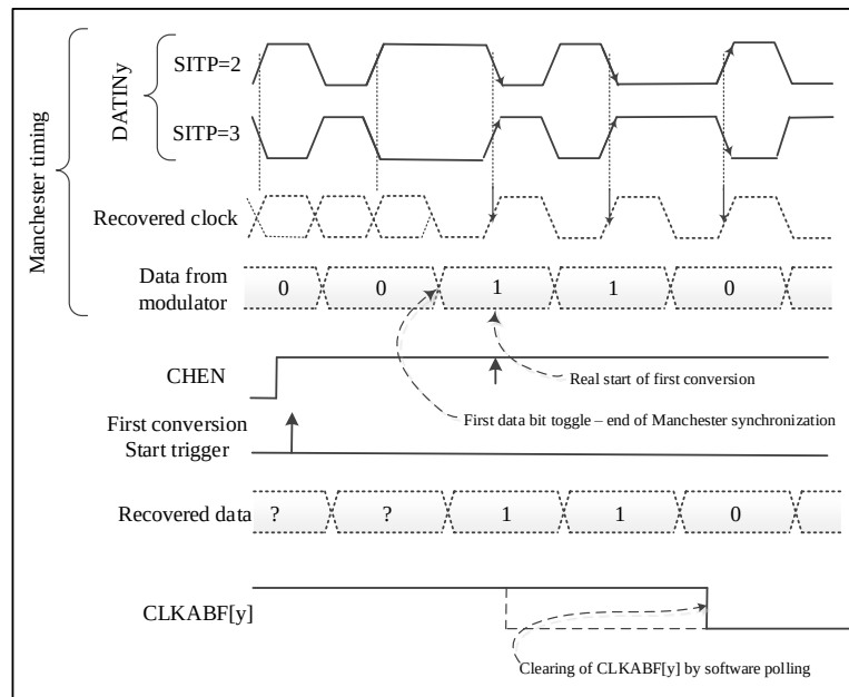
Figure 31-5 First conversion for Manchester coding (Manchester synchronization)
