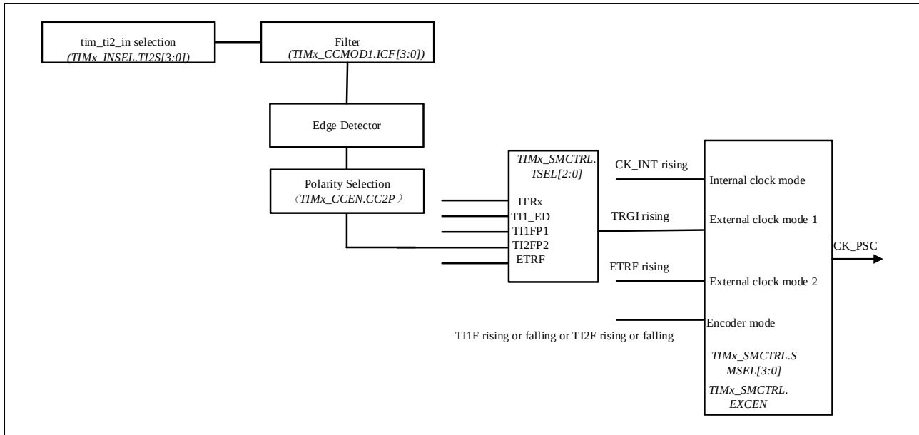
Figure 11-9 TI2 External Clock Connection Example
