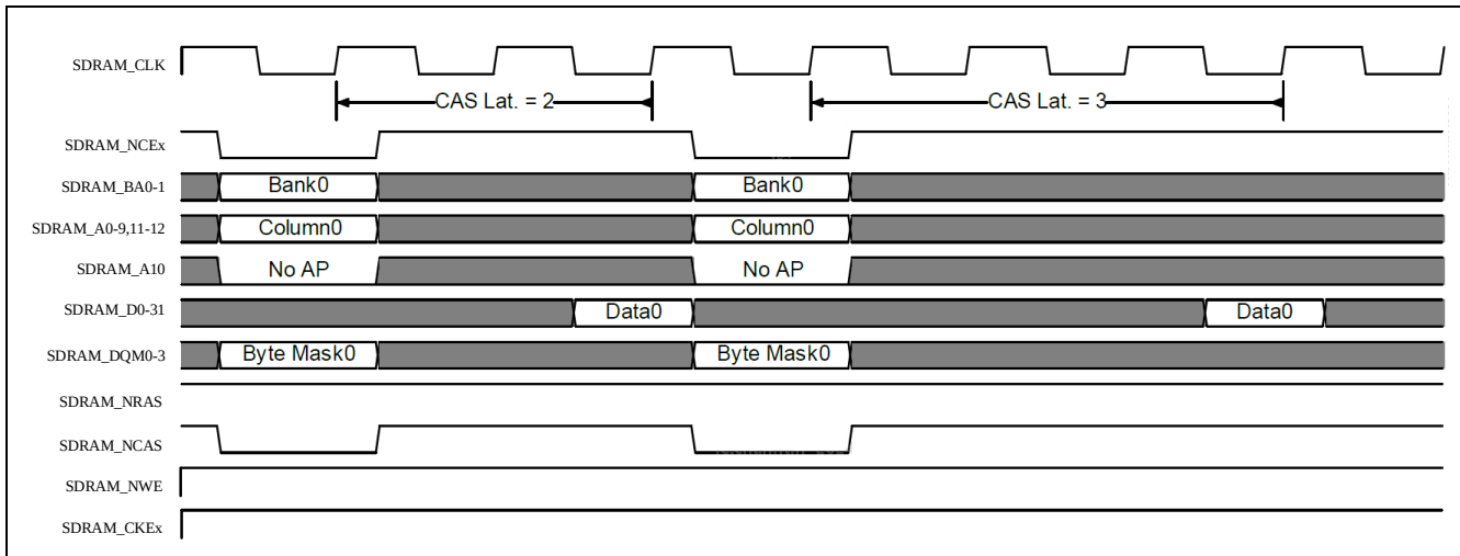
Figure 29-8 Single SDRAM read without Auto Precharge
