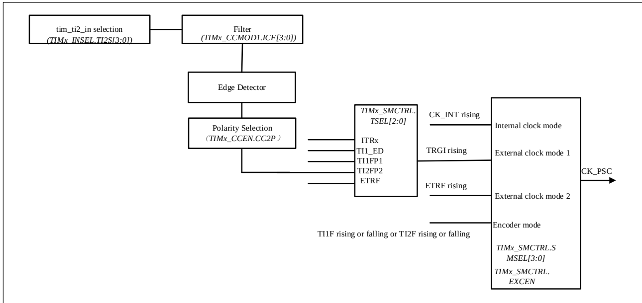
Figure 10-9 T12 External Clock Connection Example
