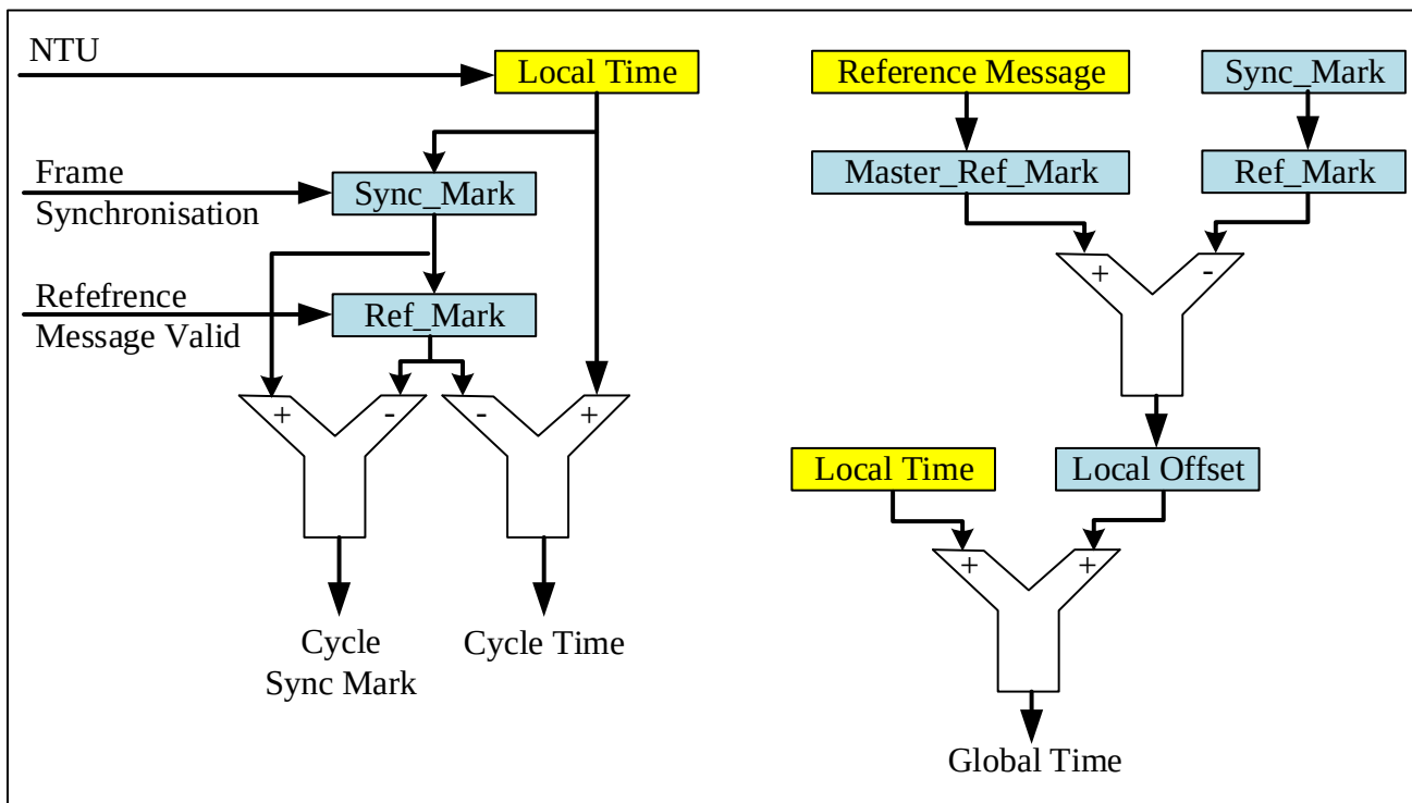
Figure 23-15 Cycle time and global time synchronization
