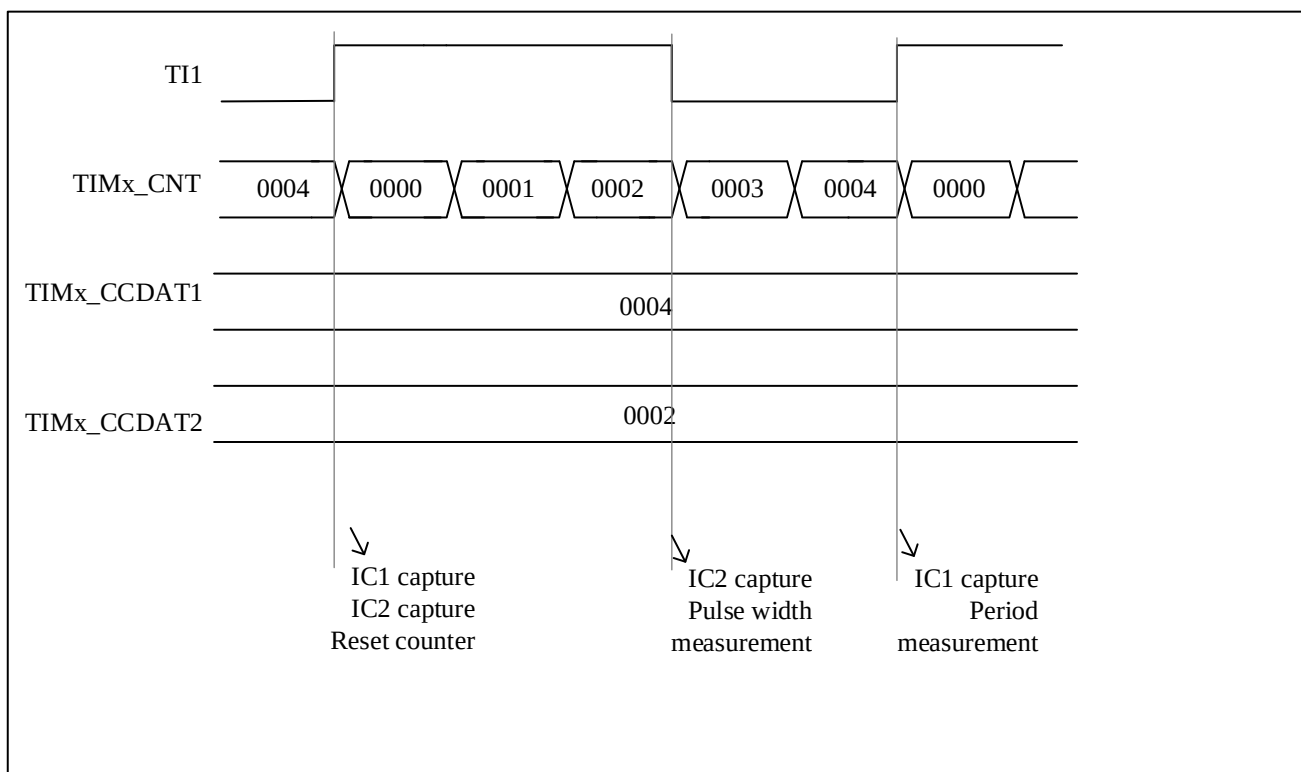
Figure 11-17 PWM Input Mode Timing
