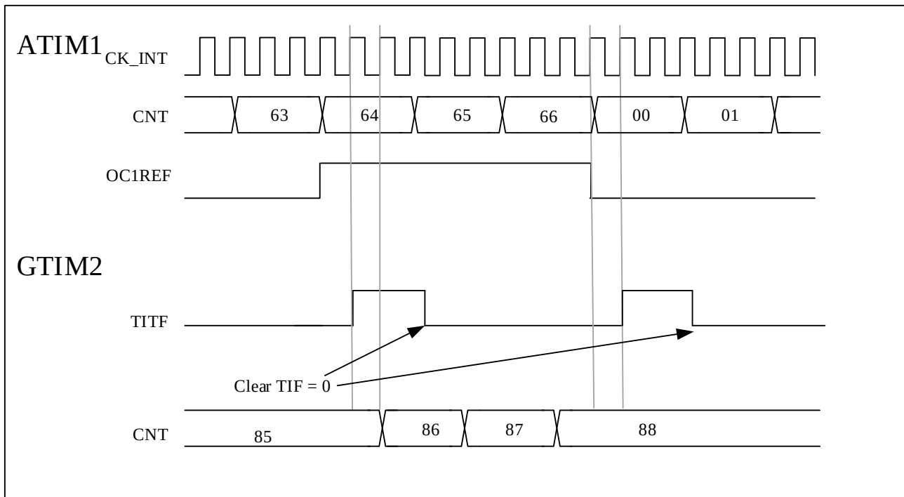
Figure 11-29 GTIM2 Gated By OC1REF Of ATIM1
