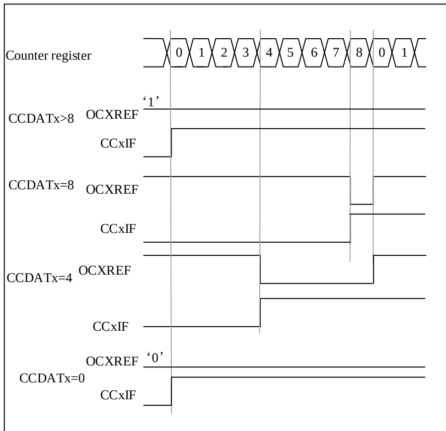
Figure 11-20 Edge-Aligned PWM waveform (AR=8)
