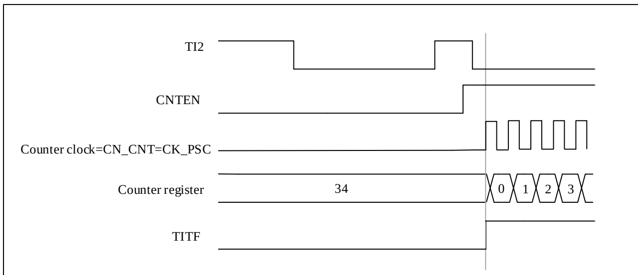
Figure 9-41 Control Circuit in Combined Reset + Trigger Mode
