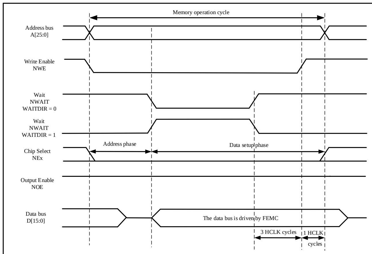
Figure 28-17 Asynchronous Wait During A Write Access
