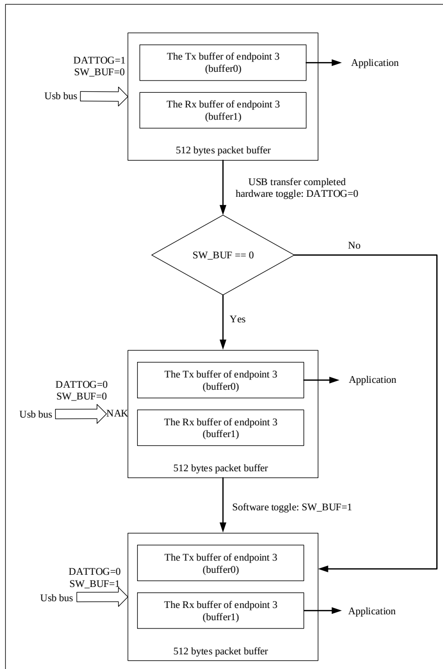
Figure 32-4 Double Buffered Bulk Endpoint Example
