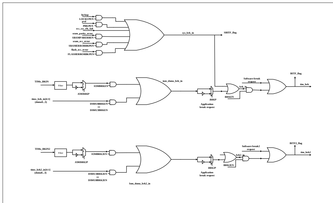
Figure 9-31 Break and Break2 circuitry overview
