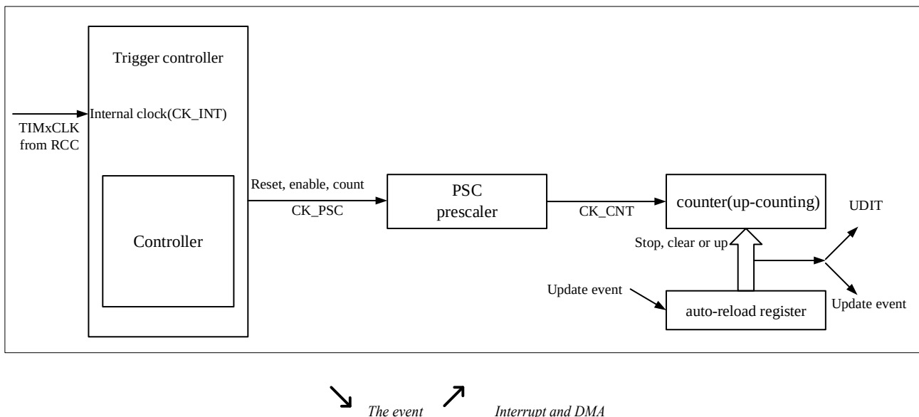
Figure 13-1 Block Diagram Of BTIM x (x = 1,2)
