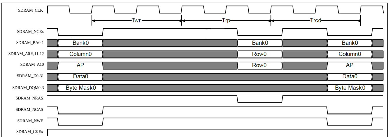
Figure 29-4 Single SDRAM Write with Auto Precharge
