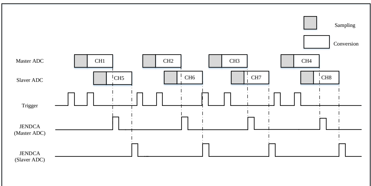
Figure 17-30 Alternate trigger: Injection channel group in Discontinuous mode
