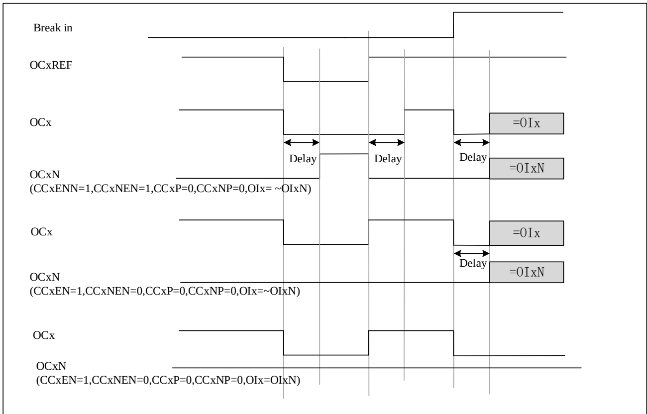
Figure 12-32 The output behavior in response to the break
