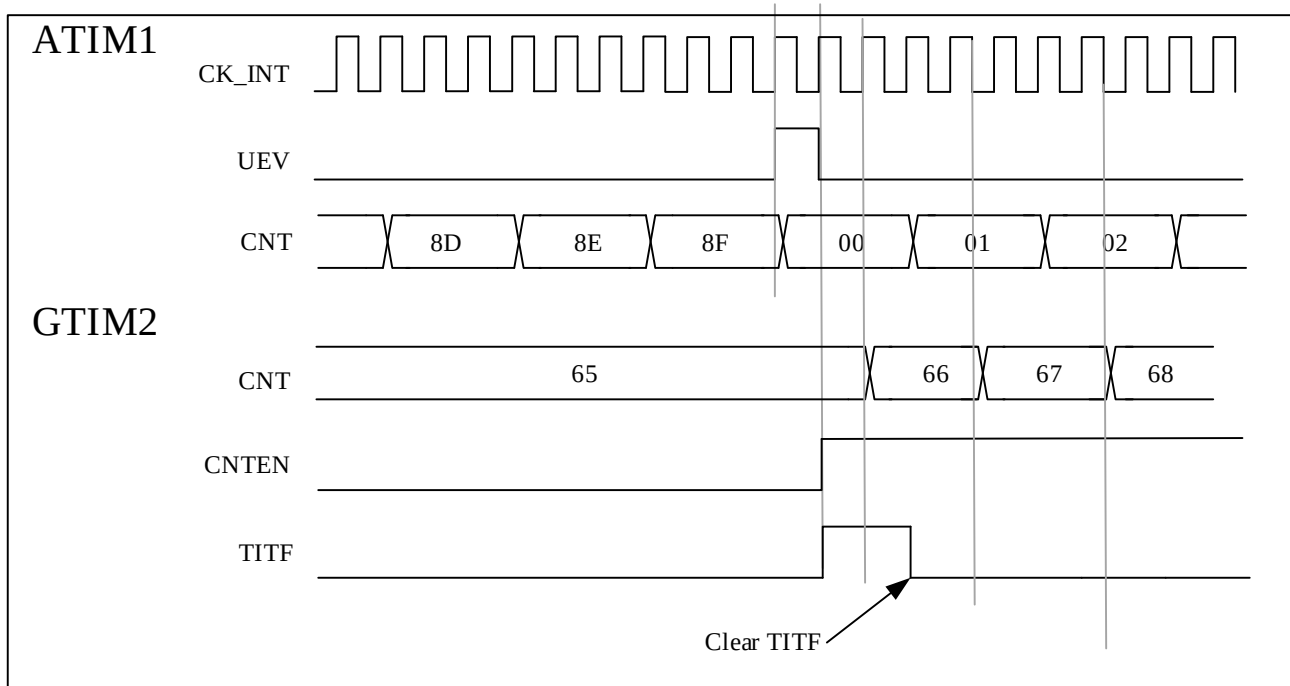
Figure 11-31 Trigger GTIM2 with An Update Of ATIM1
