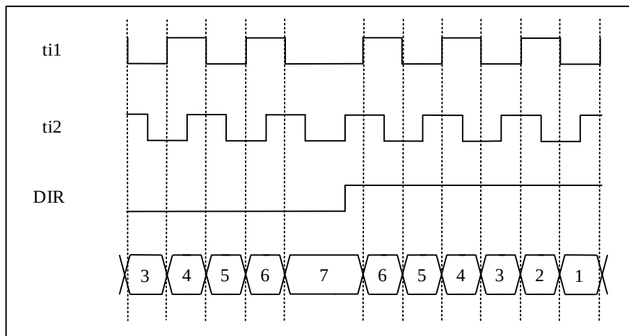
Figure 9-45 The Encoder Counts Only on TI2
