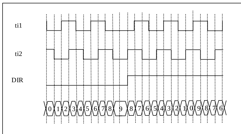
Figure 11-35 The Encoder Counts on Both TI1 and TI2
