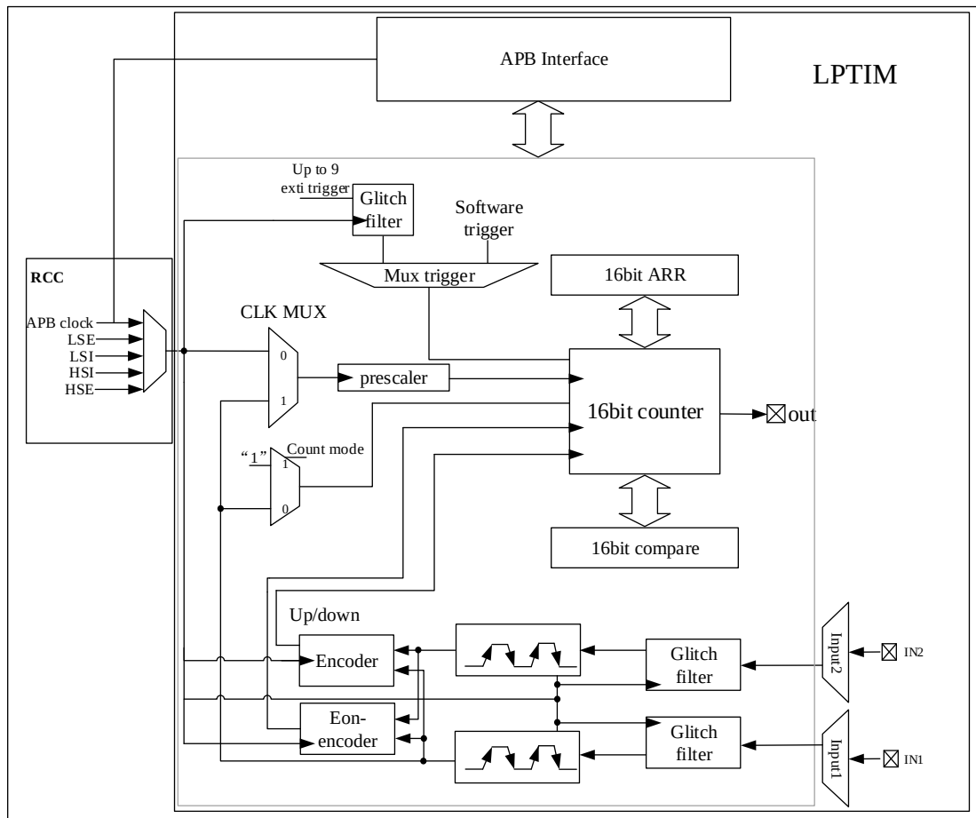
Figure 14-1 LPTIM Block Diagram
