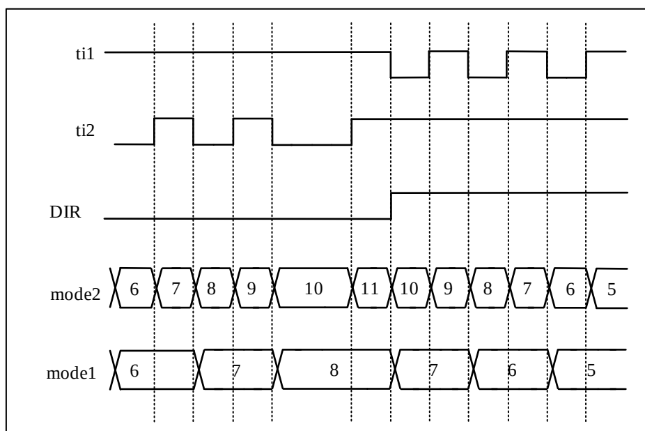
Figure 9-52 Dual-Pulse Encoder Mode (CC1P = CC2P = 0)
