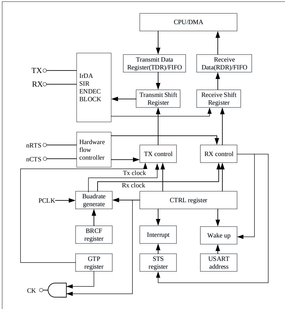
Figure 21-1 USART Block Diagram
