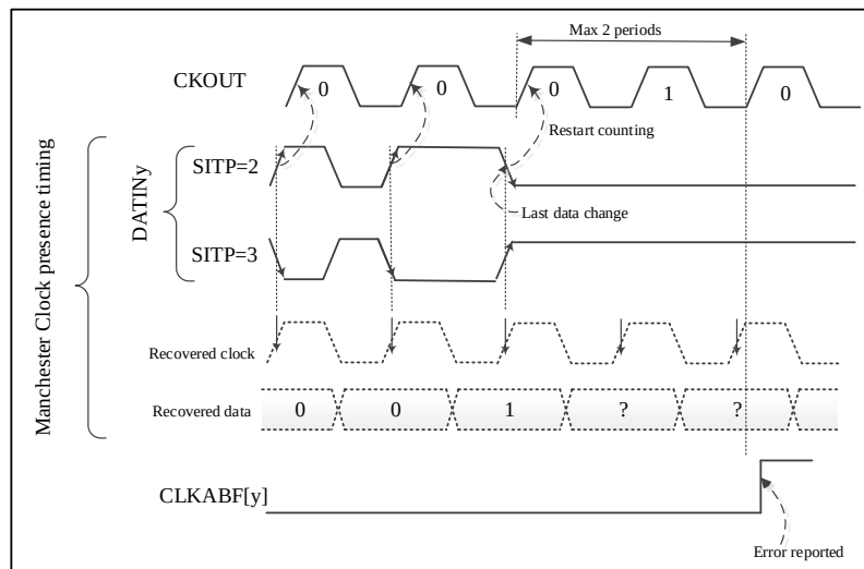
Figure 31-4 Clock absence timing diagram for Manchester coding
