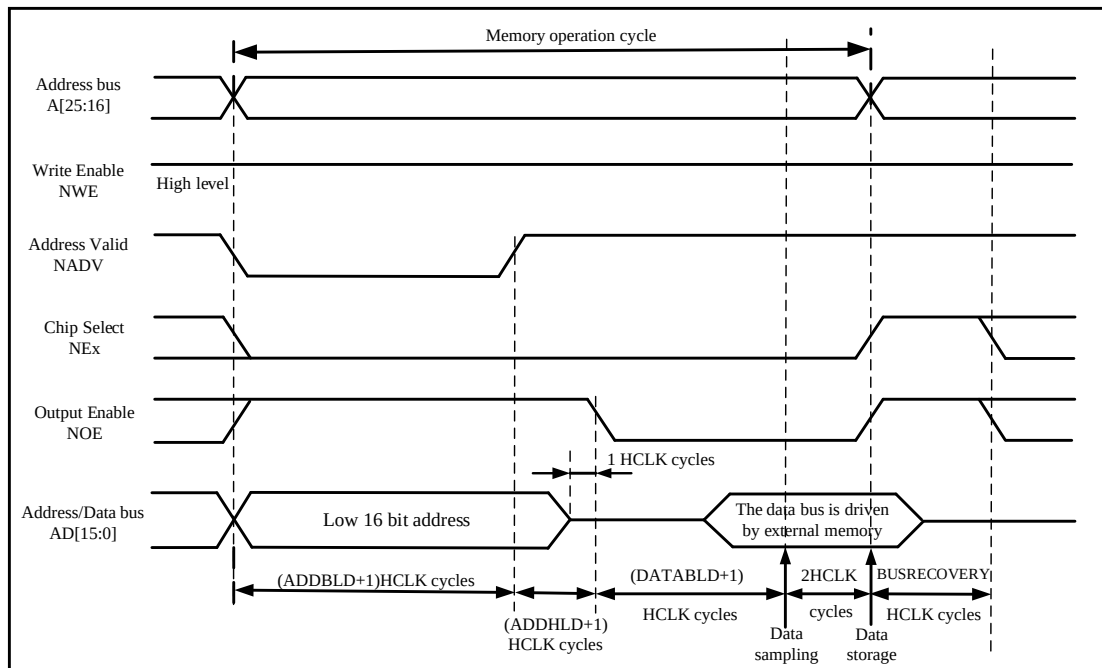
Figure 28-7 Multiplexed Read Accesses
