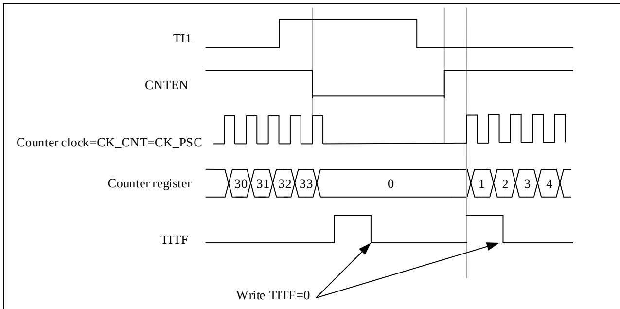
Figure 12-40 Control Circuit in Combined Gated + Reset Mode
