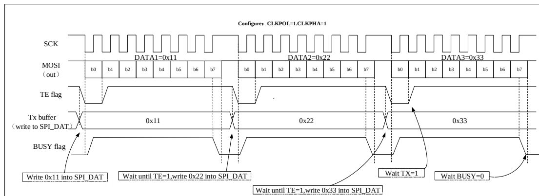
Figure 24-10 TE/BUSY Behavior in Non-Continuous Transmission (BIDIRMODE = 0 and ONLY = 0).
