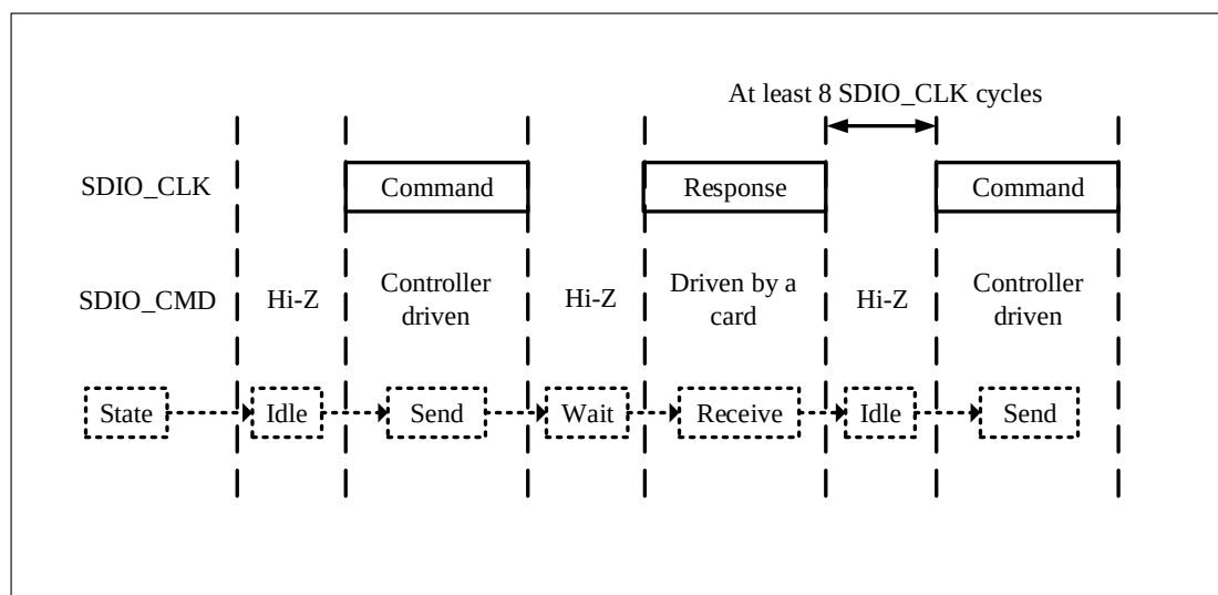
Figure 30-11 SDIO Command Transmission
