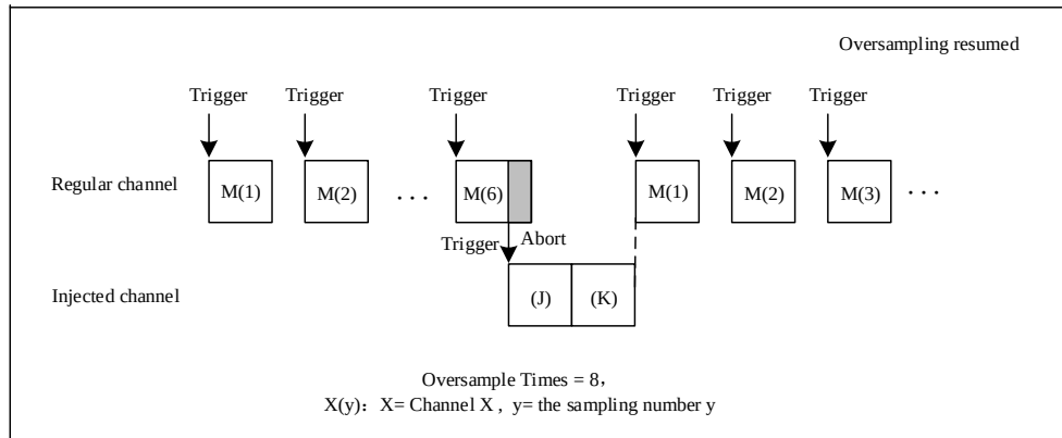
Figure 17-20 Triggered Regular Channel Oversampling with Injection Conversions
