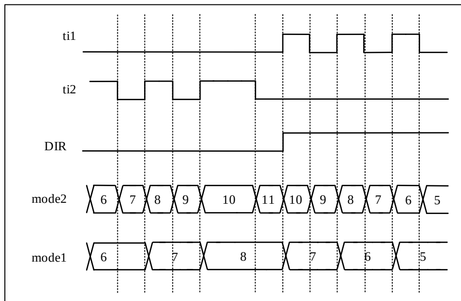
Figure 9-53 Dual-Pulse Encoder Mode (CC1P = CC2P = 1)
