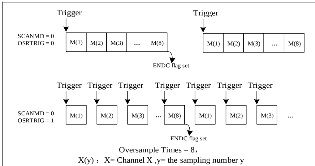
Figure 17-16 External Trigger Regular Oversampling Mode
