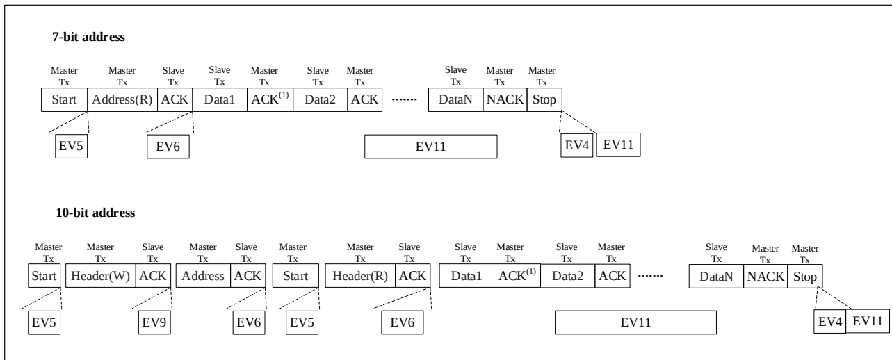
Figure 22-10 Enable FIFO for the master receiver transmission sequence diagram
