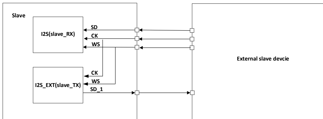
Figure 24-18 I2S slave receive (I2SCFG=01), I2S_EXT slave transmit (I2SCFG=00)
