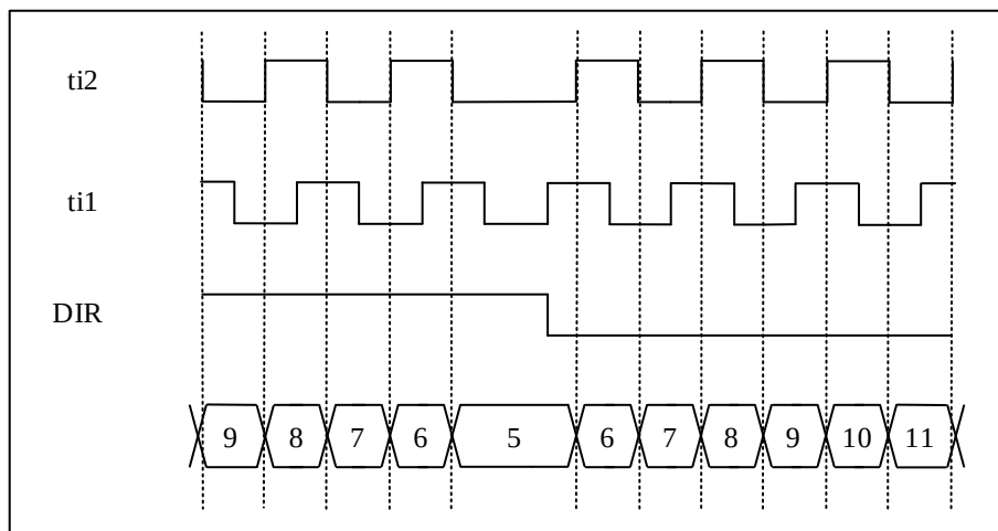
Figure 11-35 The Encoder Counts on Both TI1 and TI2
