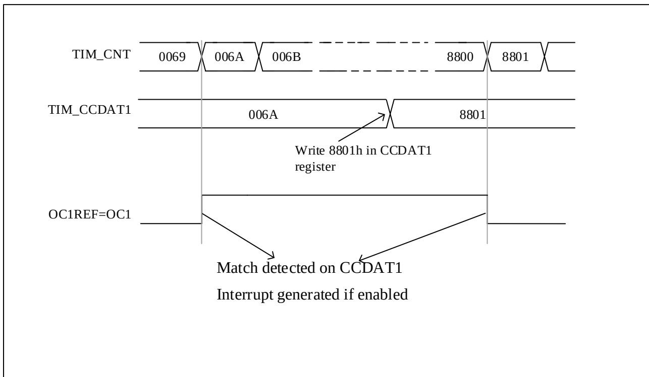
Figure 9-24 Output Compare Mode, Toggle on OC1
