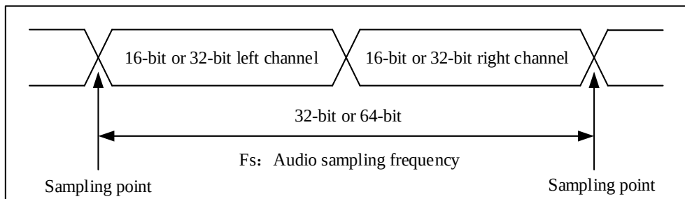
Figure 26-24-31 Audio Sampling Frequency Definition
