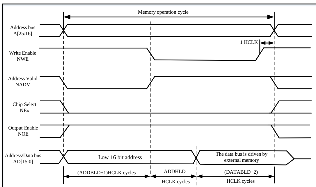
Figure 28-15 Multiplexed Write Accesses
