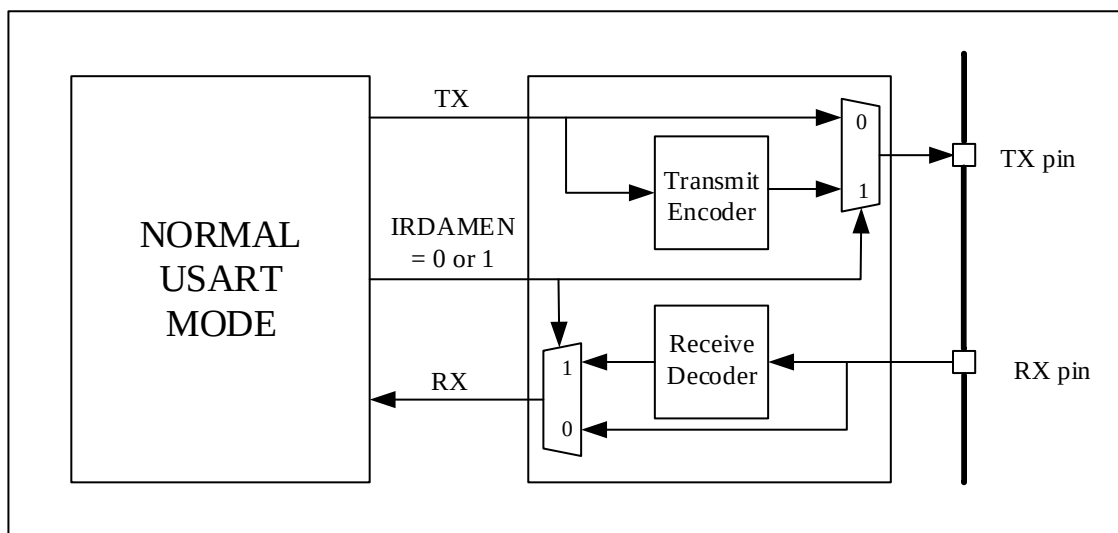
Figure 21-18 IrDA SIR ENDEC–Block Diagram
