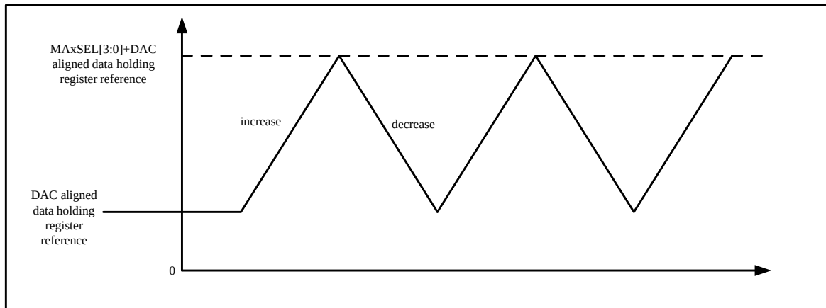
Figure 18-8 DAC Conversion with Triangular Wave Generation (Enable Software Trigger, HFSEL[1:0] = 0b'01)
