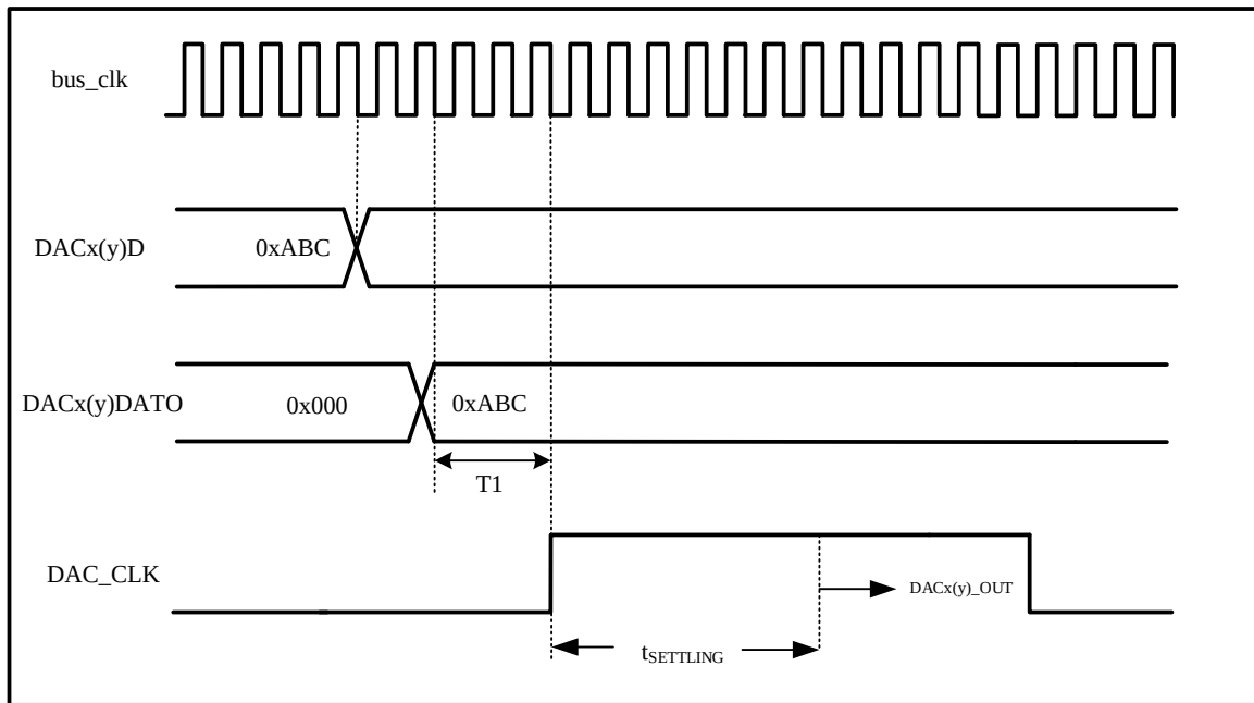
Figure 18-4 Timing diagram for conversion when trigger is disabled(HFSEL = 0b'10)
