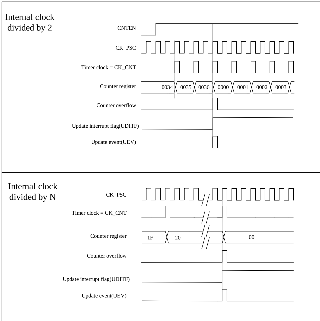
Figure 11-3 Timing Diagram Of Up-Counting. When The Internal Clock Divider Factor = 2/N
