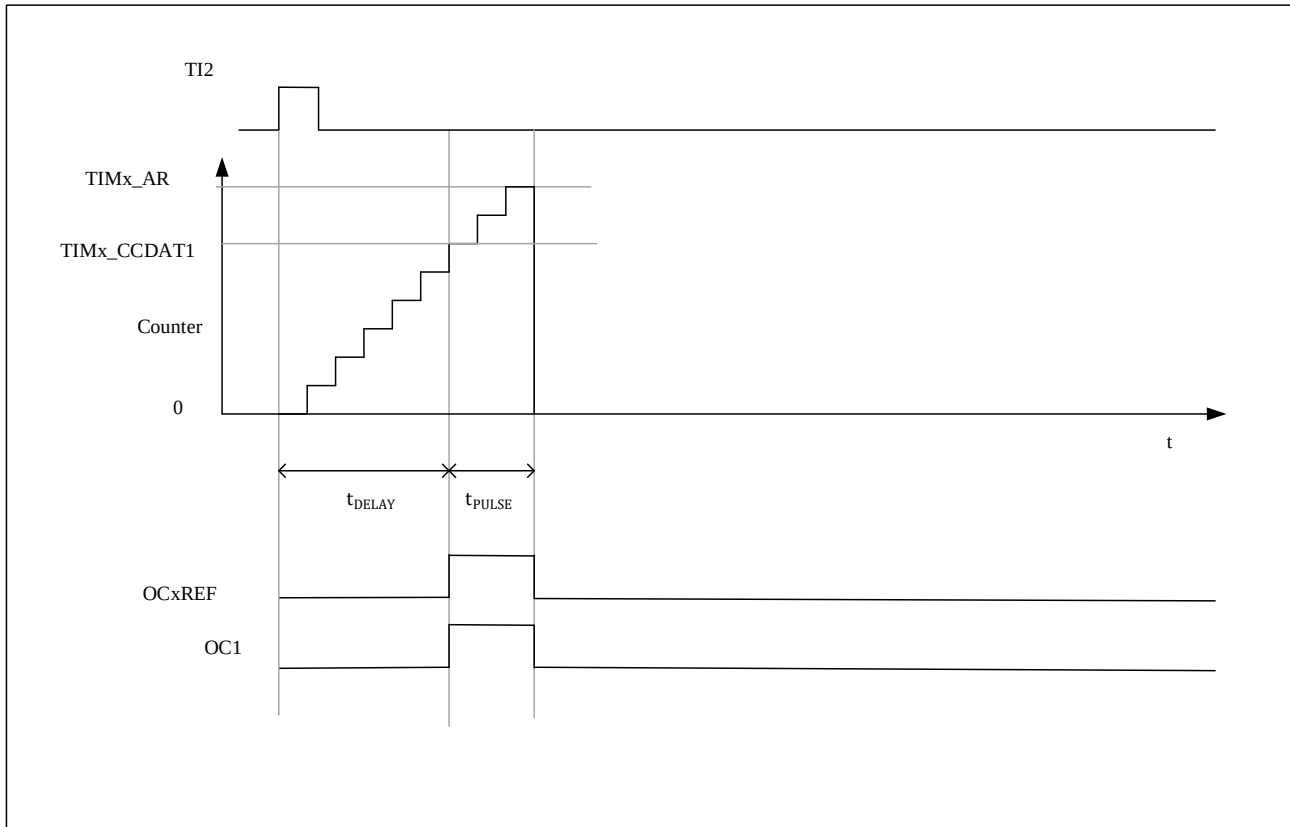
Figure 11-21 Example Of One-pulse Mode
