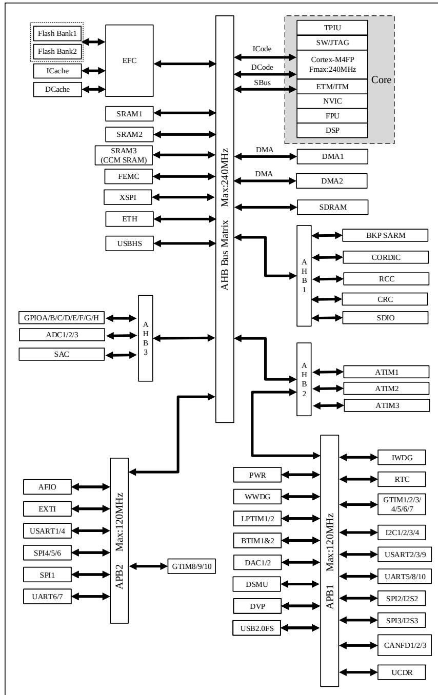
Figure 2-1 Bus Architecture
