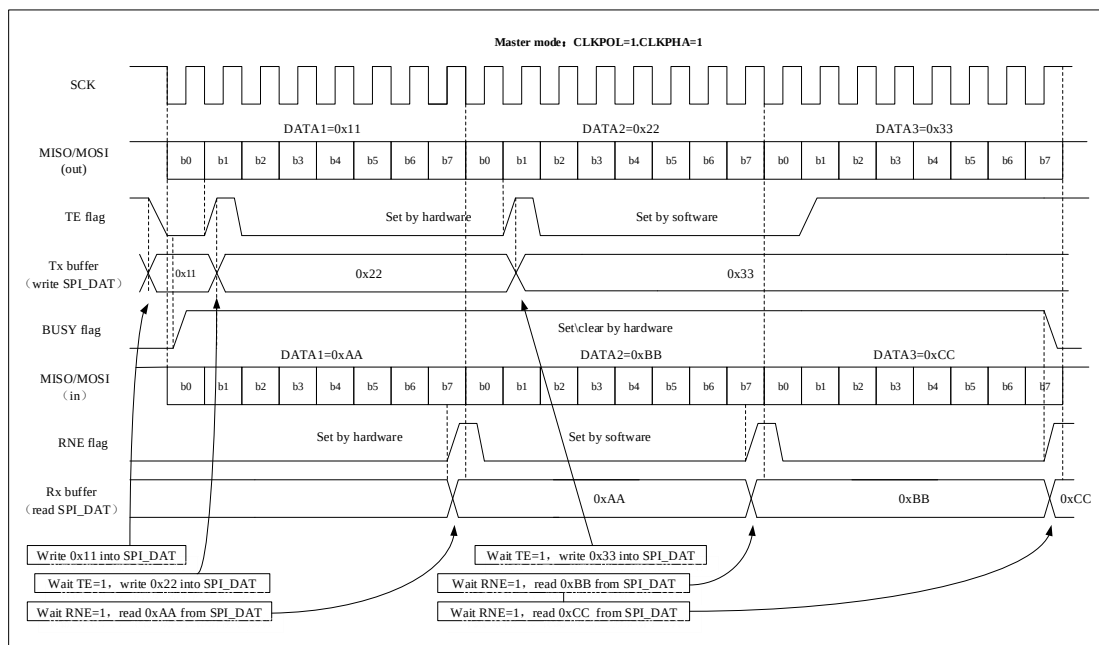
Figure 24-5 TE/RNE/BUSY Behavior in Master / Full-Duplex Mode(BIDIRMODE = 0, RONLY = 0) during Continuous Transmission
