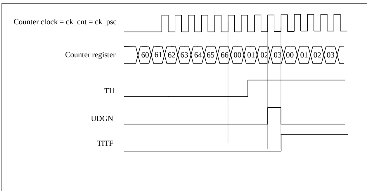
Figure 12-35 Control Circuit in the Reset Mode
