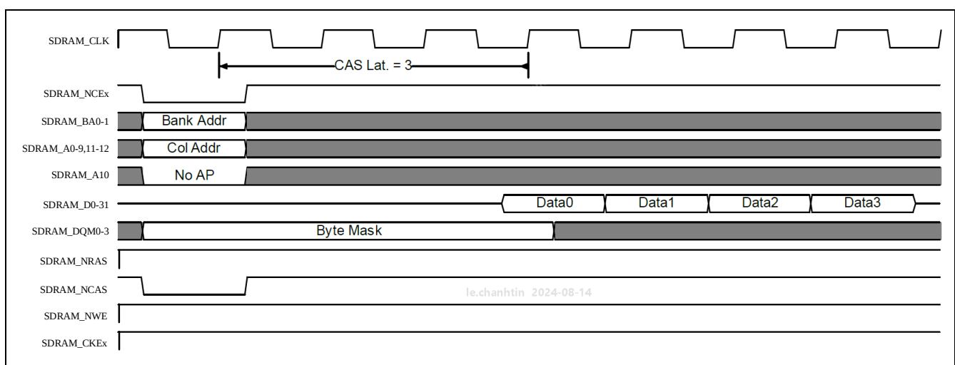
Figure 29-10 Burst SDRAM read without Auto Precharge
