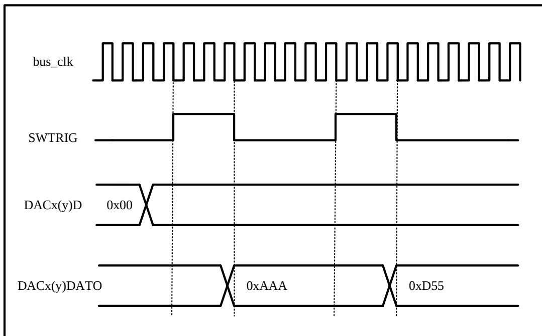
Figure 18-6 DAC Conversion with LFSR Waveform Generation (Enable Software Trigger)
