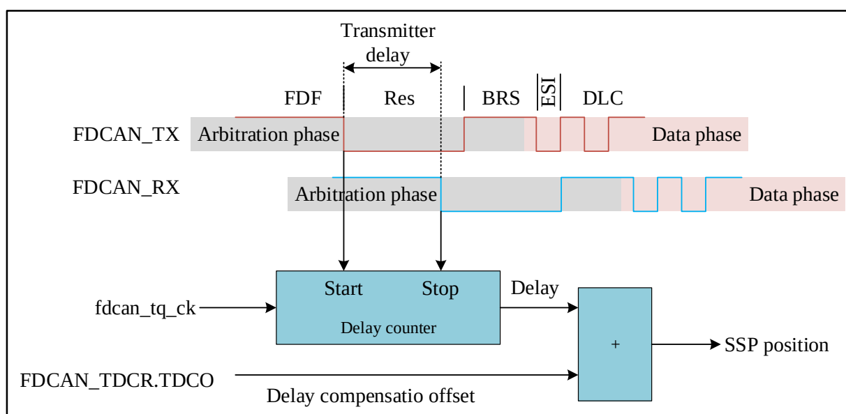
Figure 23-3 FDCAN Transceiver Delay Measurement
