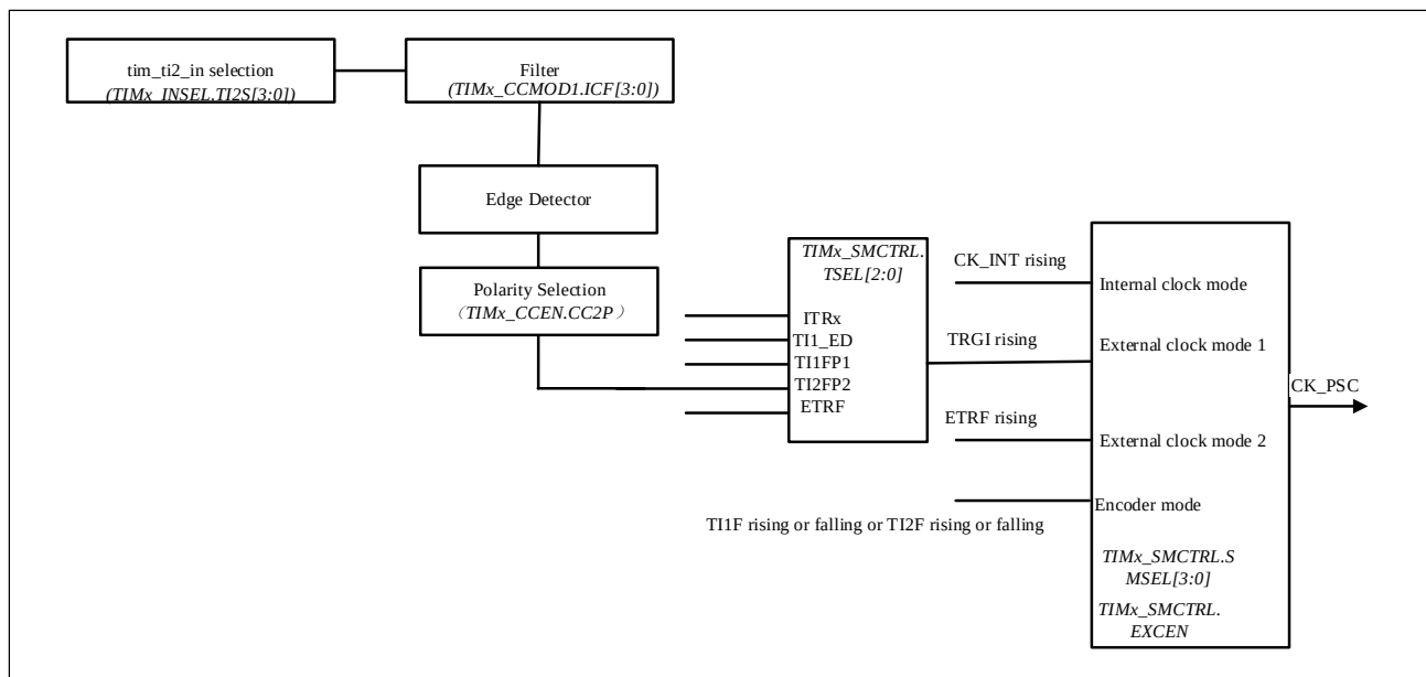
Figure 9-16 TI2 TI2 External Clock Connection Example
