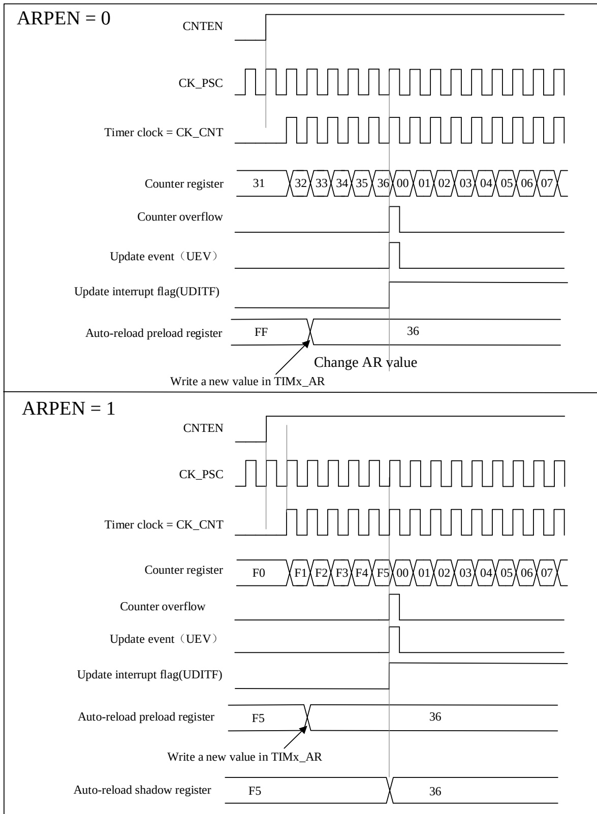
Figure 10-4 Timing Diagram Of The Up-Counting, When ARPEN=0/1 Generates an Update Event
