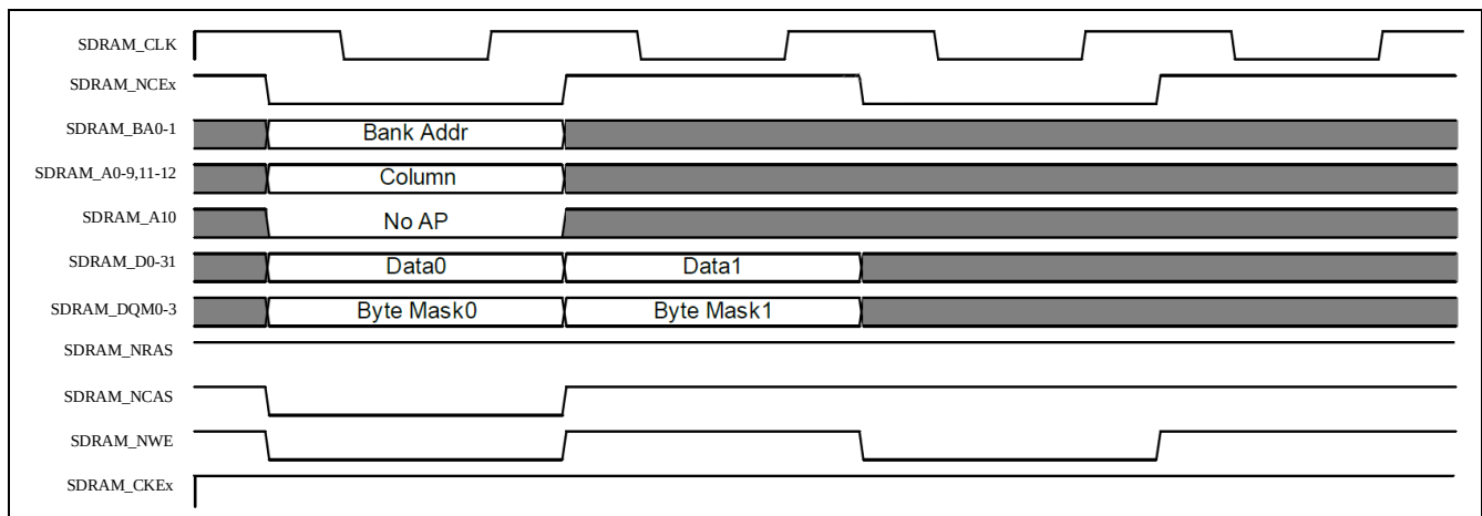
Figure 29-6 Write Burst Terminate
