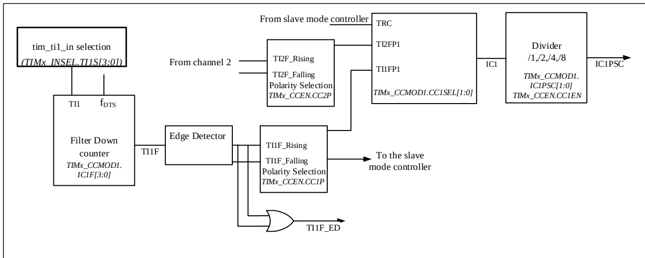
Figure 11-13 Capture/Compare Channel (Example: Channel 1 Input Stage)
