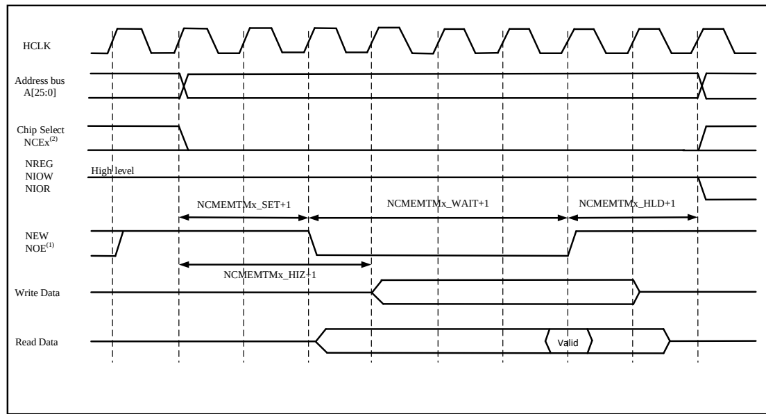
Figure 28-20 Common Memory Space Access Timing for NAND Flash
