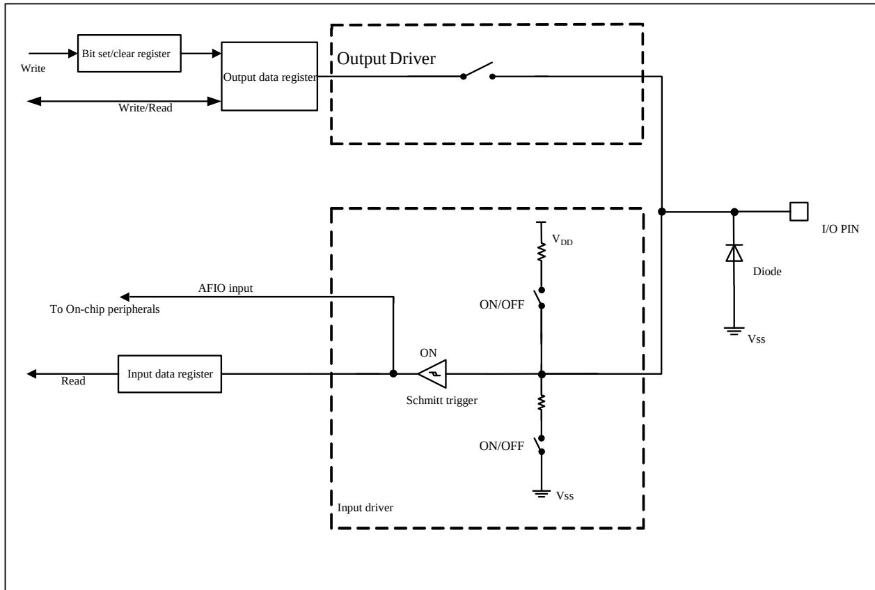
Figure 5-2 Input Floating/Pull-up/Pull-Down/Alternate Configuration
