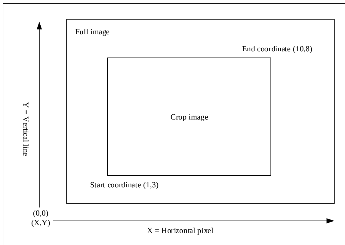
Figure 30-5 DVP Crop Function
