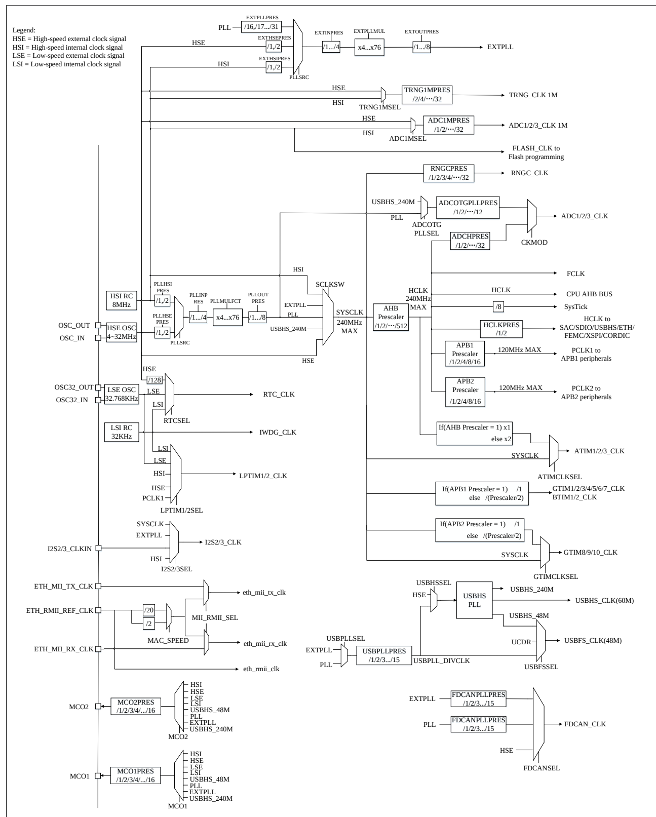
Figure 4-2 Clock Tree
