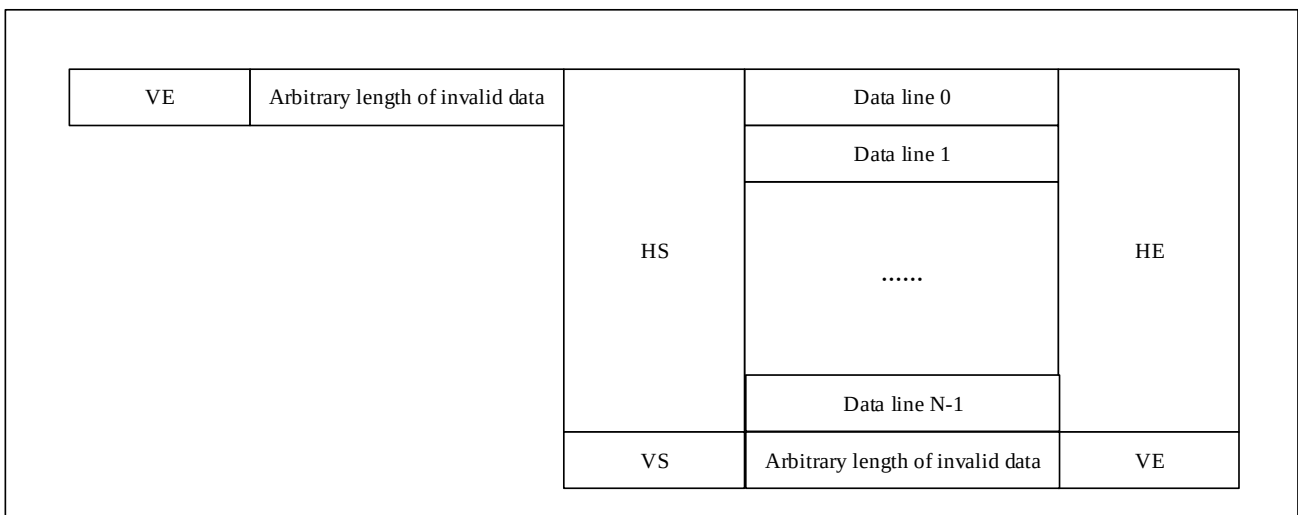
Figure 30-3 Frame Format in Sony Mode
