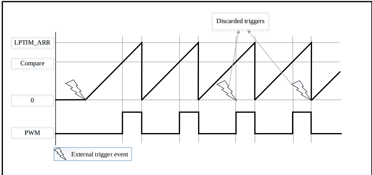
Figure 14-3 LPTIM Output Waveform, Continuous Counting Mode Configuration
