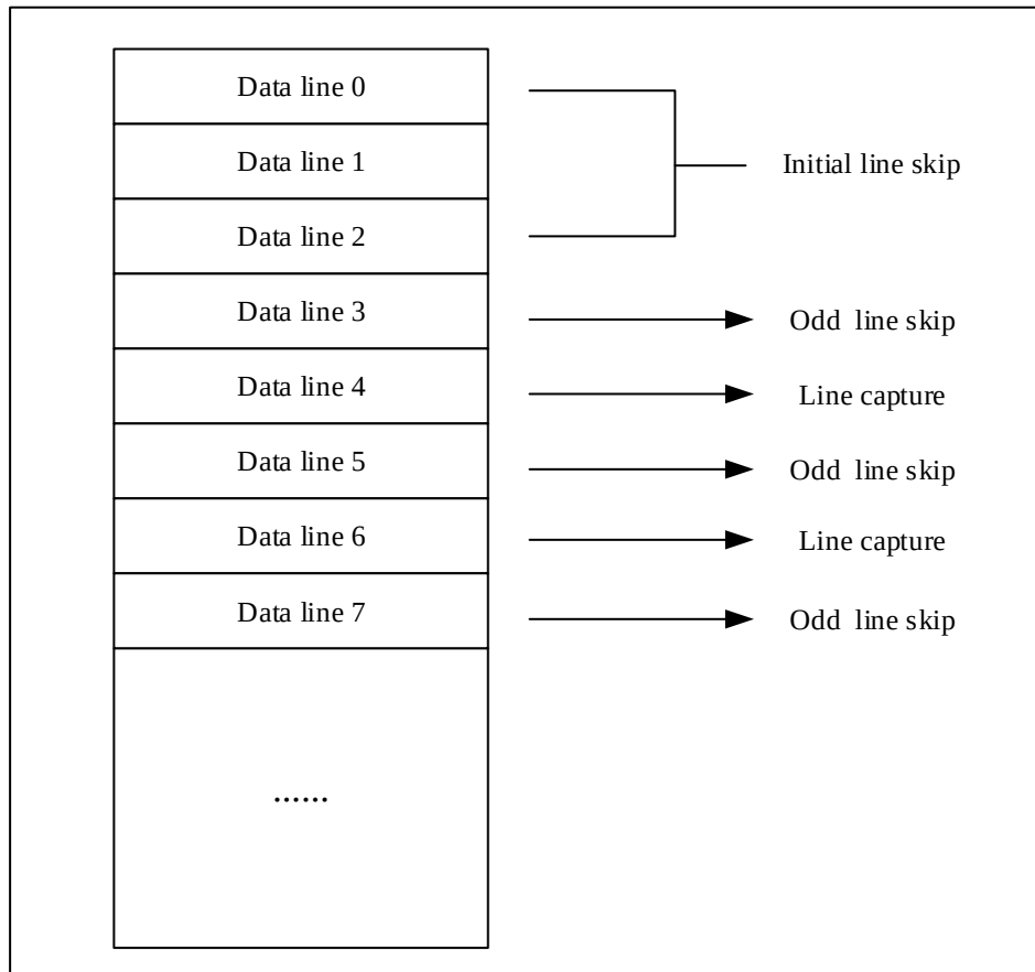
Figure 30-7 Line Skip Function(HISKIP=3, HRSKIP=14)
