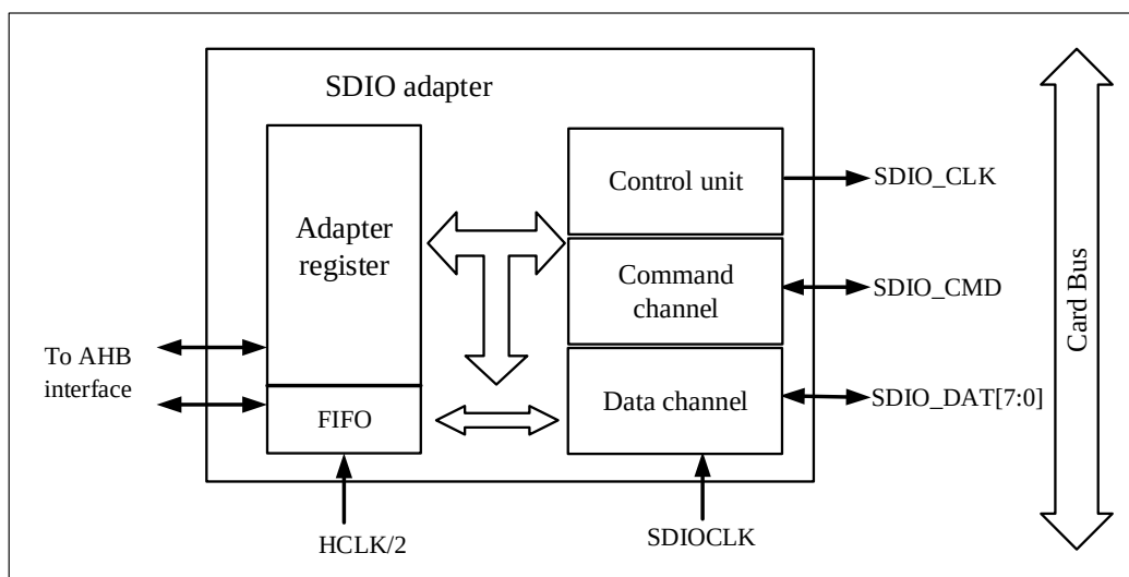
Figure 30-7 SDIO Adapter
