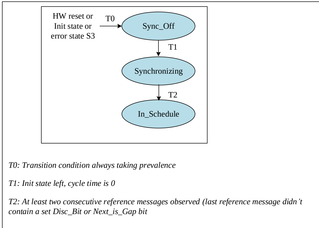
Figure 23-17 Level 0 schedule synchronization state machine
