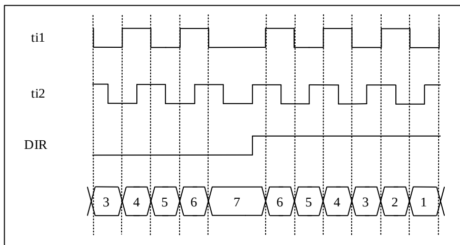
Figure 11-34 The Encode Counts Only on TI2
