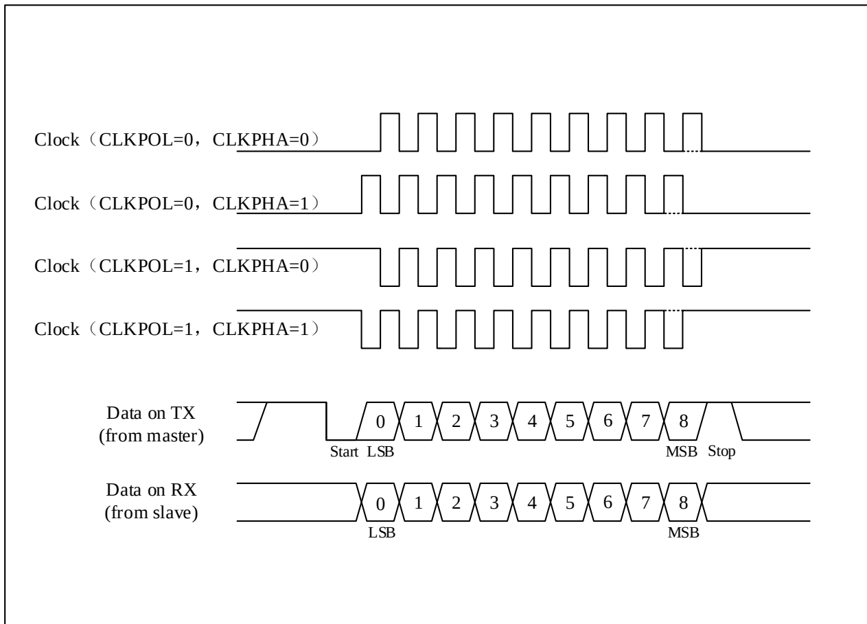
Figure 21-17 RX Data Sampling / Holding Time
