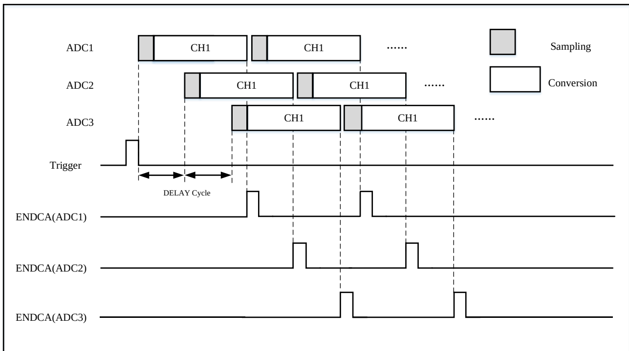
Figure 17-28 Schematic diagram of fast Interleave mode conversion with continuous conversion of one channel
