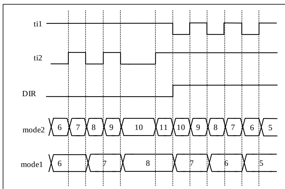
Figure 12-50 Dual Pulse Encoding Mode (CC1P=CC2P=0)
