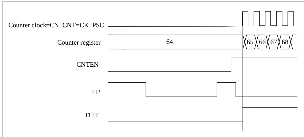
Figure 9-38 Control Circuit in Trigger Mode
