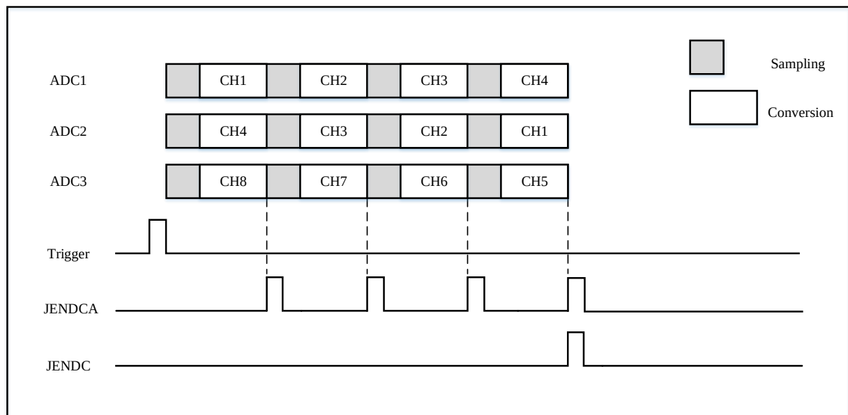
Figure 17-26 Synchronous injection mode with 4 channels for three ADCs.
