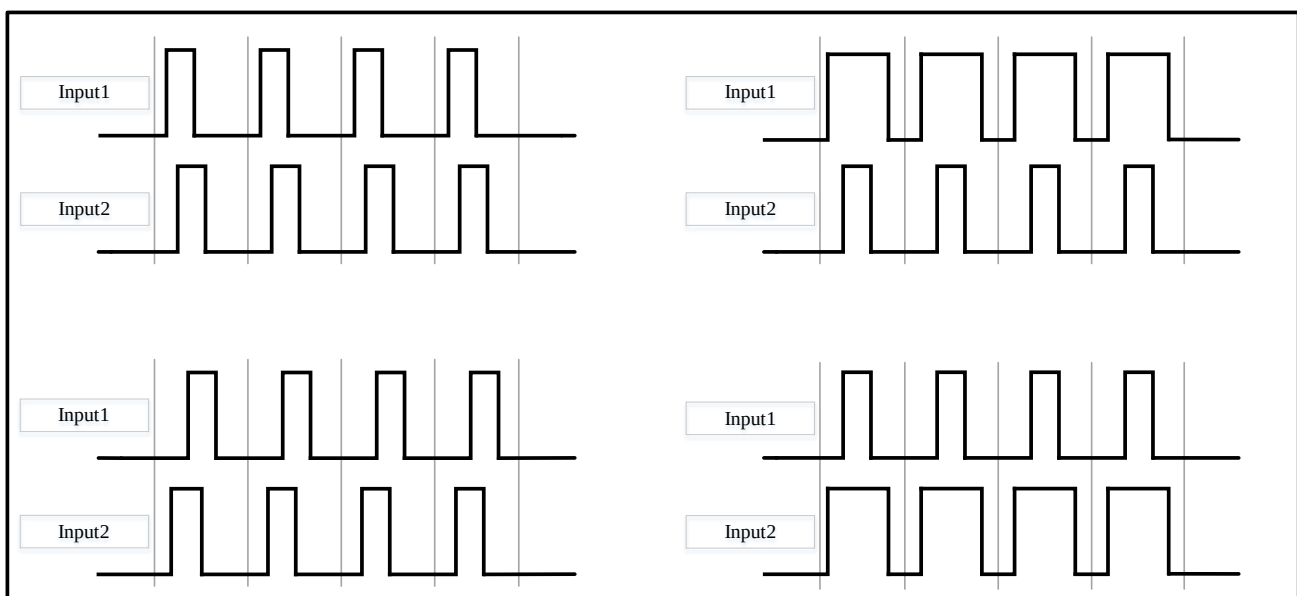
Figure 14-9 Input1 and Input2 input waveforms when decoder module is not working
