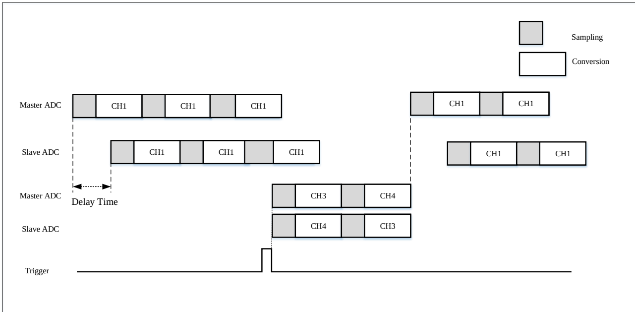
Figure 17-35 The interleaved single-channel conversion is interrupted by the injection sequences CH3 and CH4
