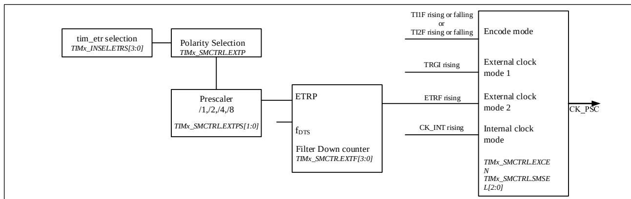
Figure 11-11 External Trigger Input Block Diagram
