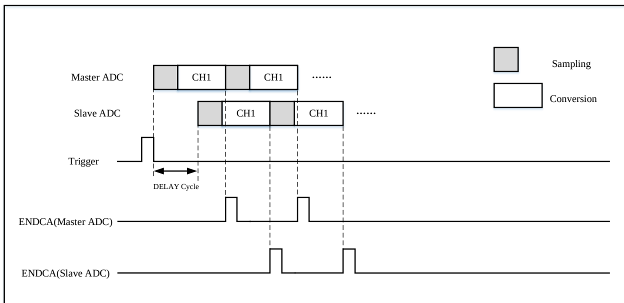
Figure 17-27 Schematic diagram of fast interleaved mode conversion with continuous conversion of one channel.
