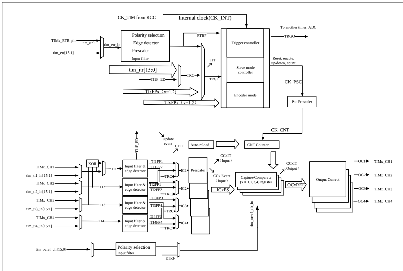
Figure 11-1 Block Diagram Of GTIMx (x=2,3,5,6,7)
