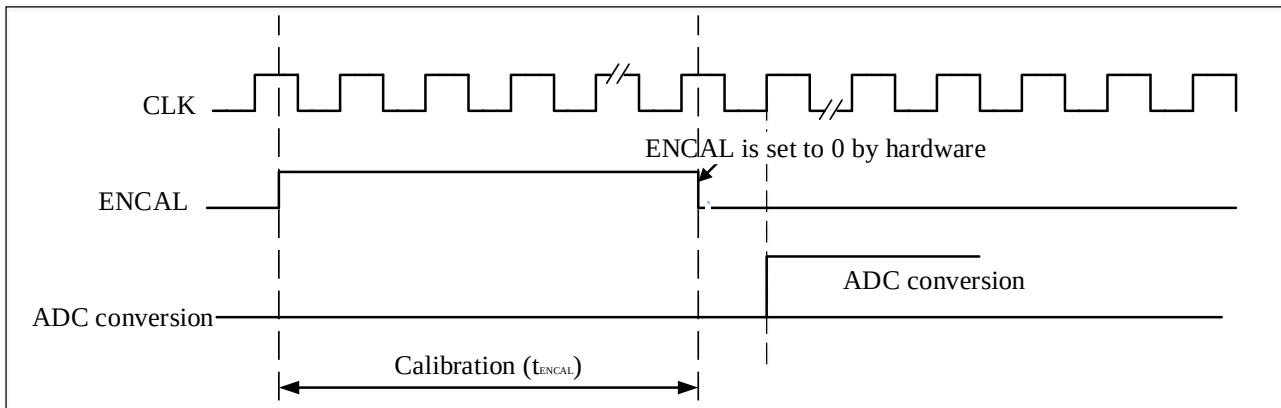
Figure 17-5 Calibration Timing Diagram
