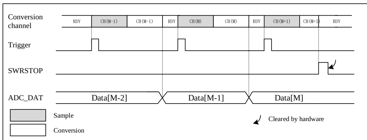
Figure 17-7 Stop Ongoing Regular Channel Conversions
