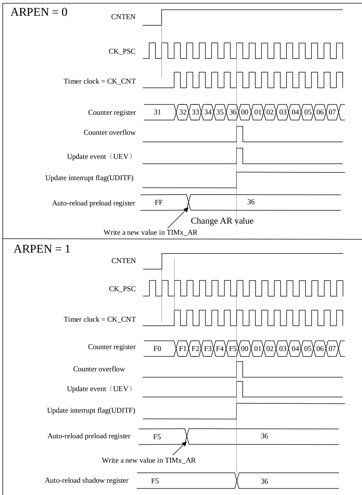
Figure 11-4 Timing Diagram Of The Up-Counting, When ARPEN=0/1 Generates an Update Event
