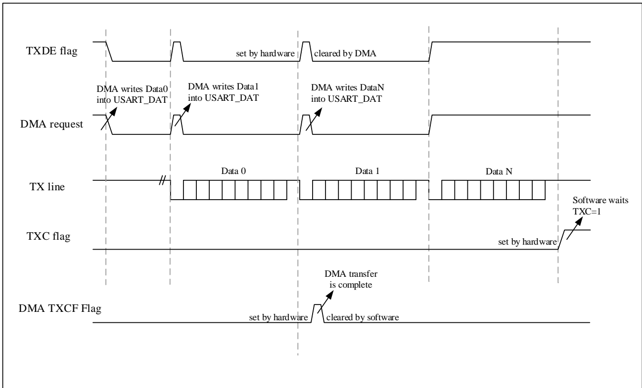
Figure 19-8 Transmission Using DMA
