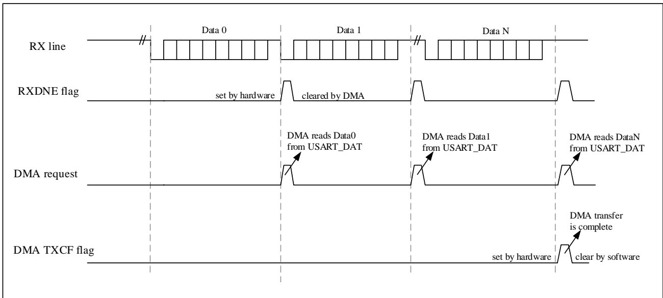
Figure 19-9 Reception Using DMA
