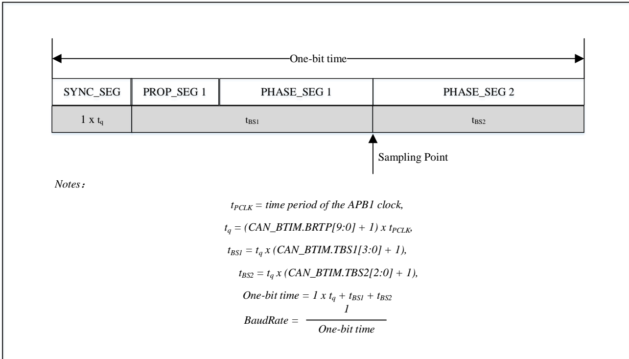
Figure 20-11 Bit Timing
