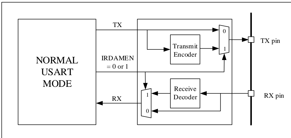
Figure 19-13 IrDA Data Modulation (3/16)-Normal Mode
