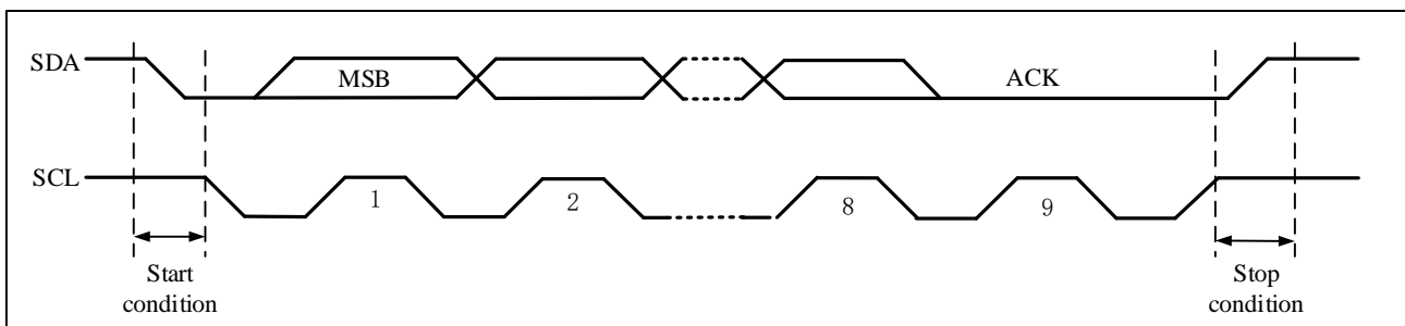
Figure 18-2 I 2 C Bus Protocol
