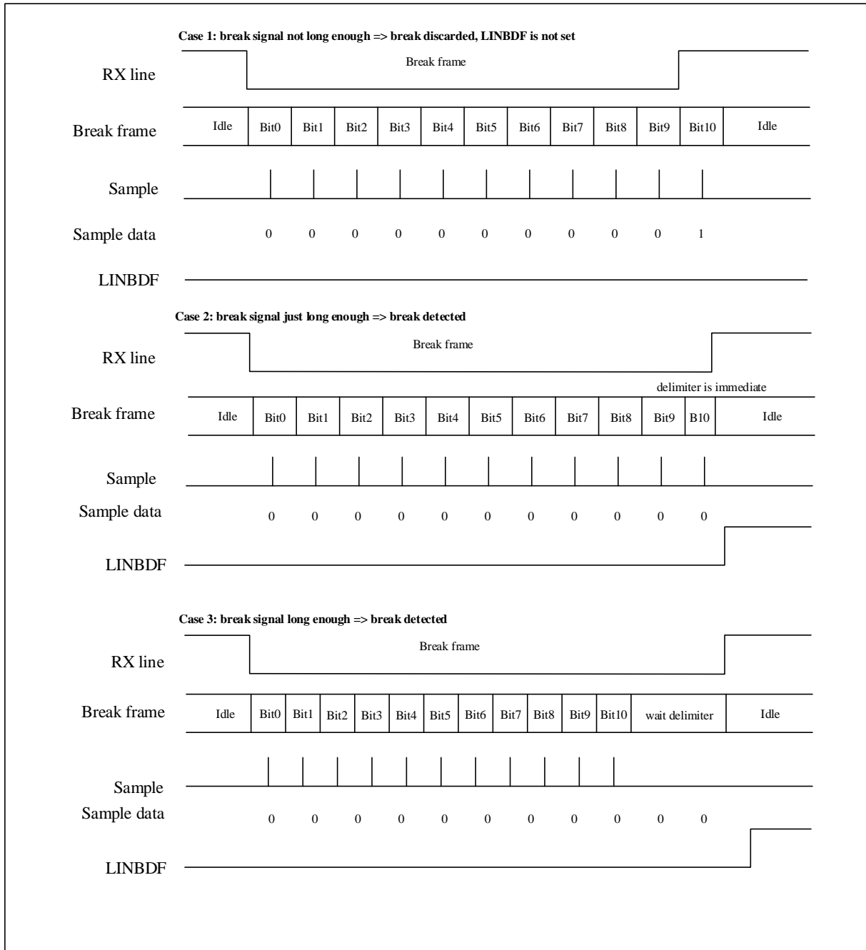
Figure 19-14 Break Detection in LIN Mode (11-bit Break Length, The LINBDL Bit Is Set)
