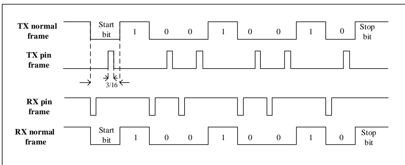
Figure 19-13 IrDA Data Modulation (3/16)-Normal Mode
