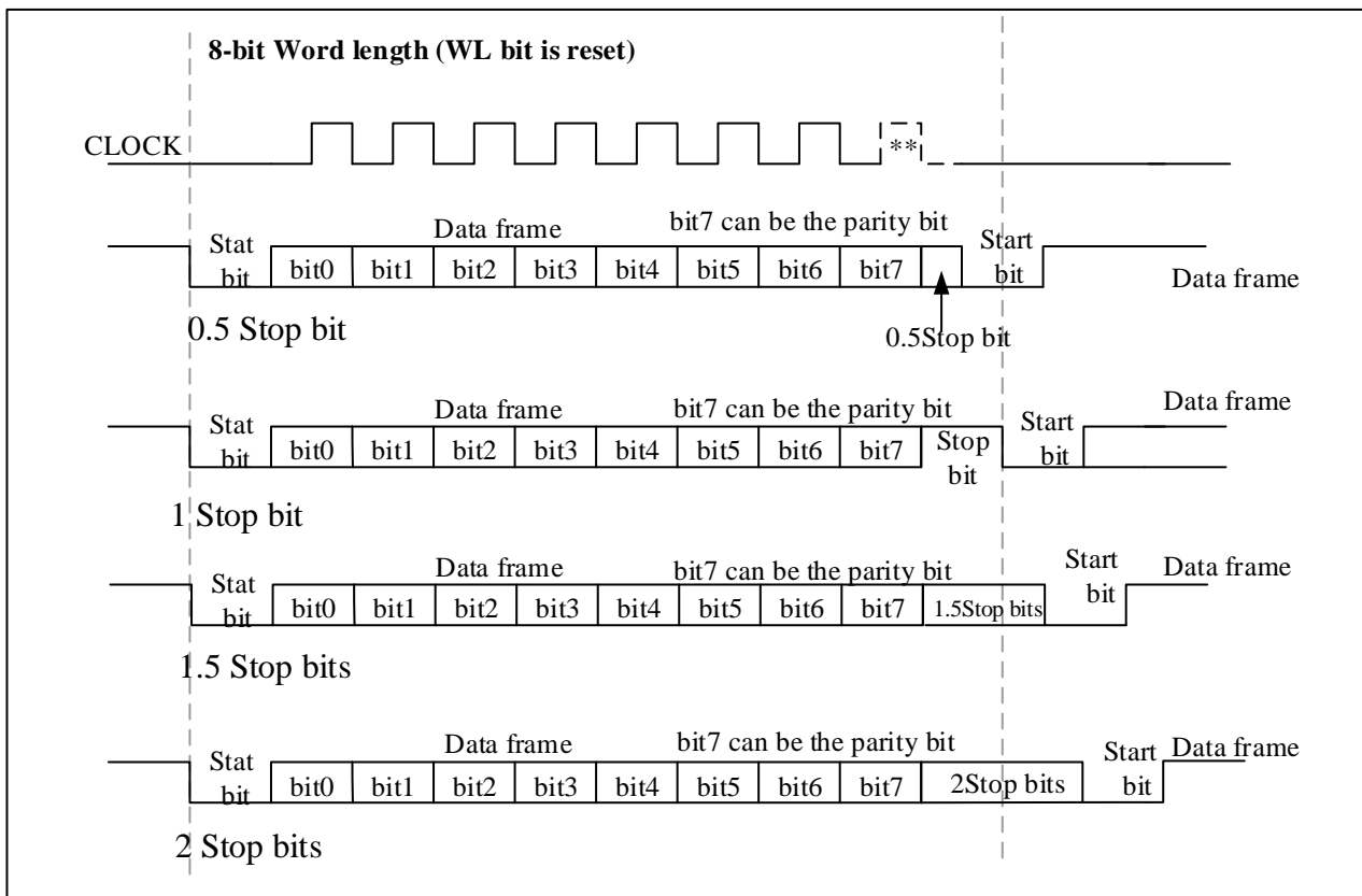
Figure 19-4 Configuration Stop Bit
