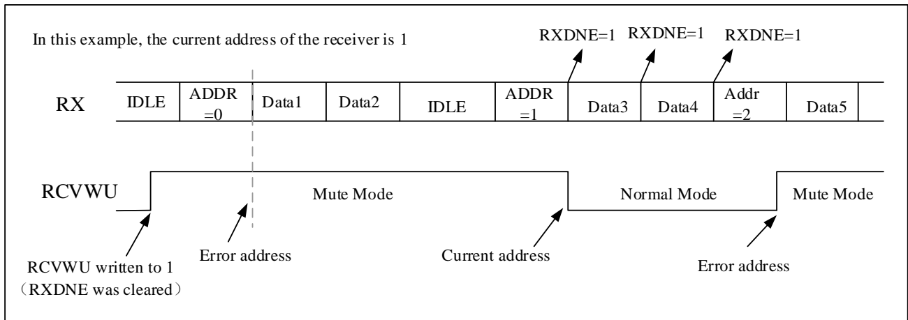
Figure 19-11 Mute Mode Detected Using Address Mark
