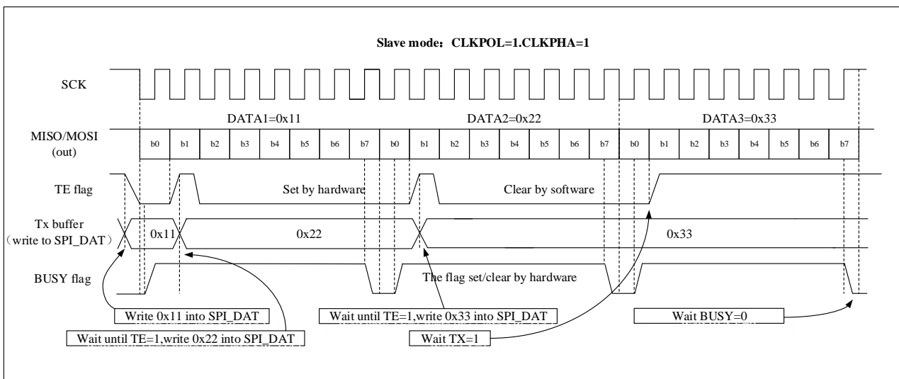
Figure 21-9 TE/BUSY Behavior in Slave Transmit-Only Mode in Case of Continuous Transfers
