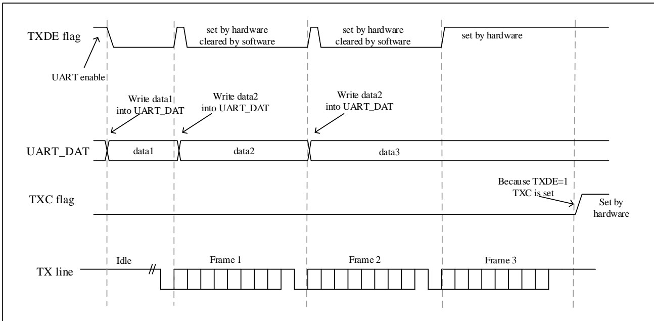
Figure 19-6 TXC/TXDE Changes During Transmission
