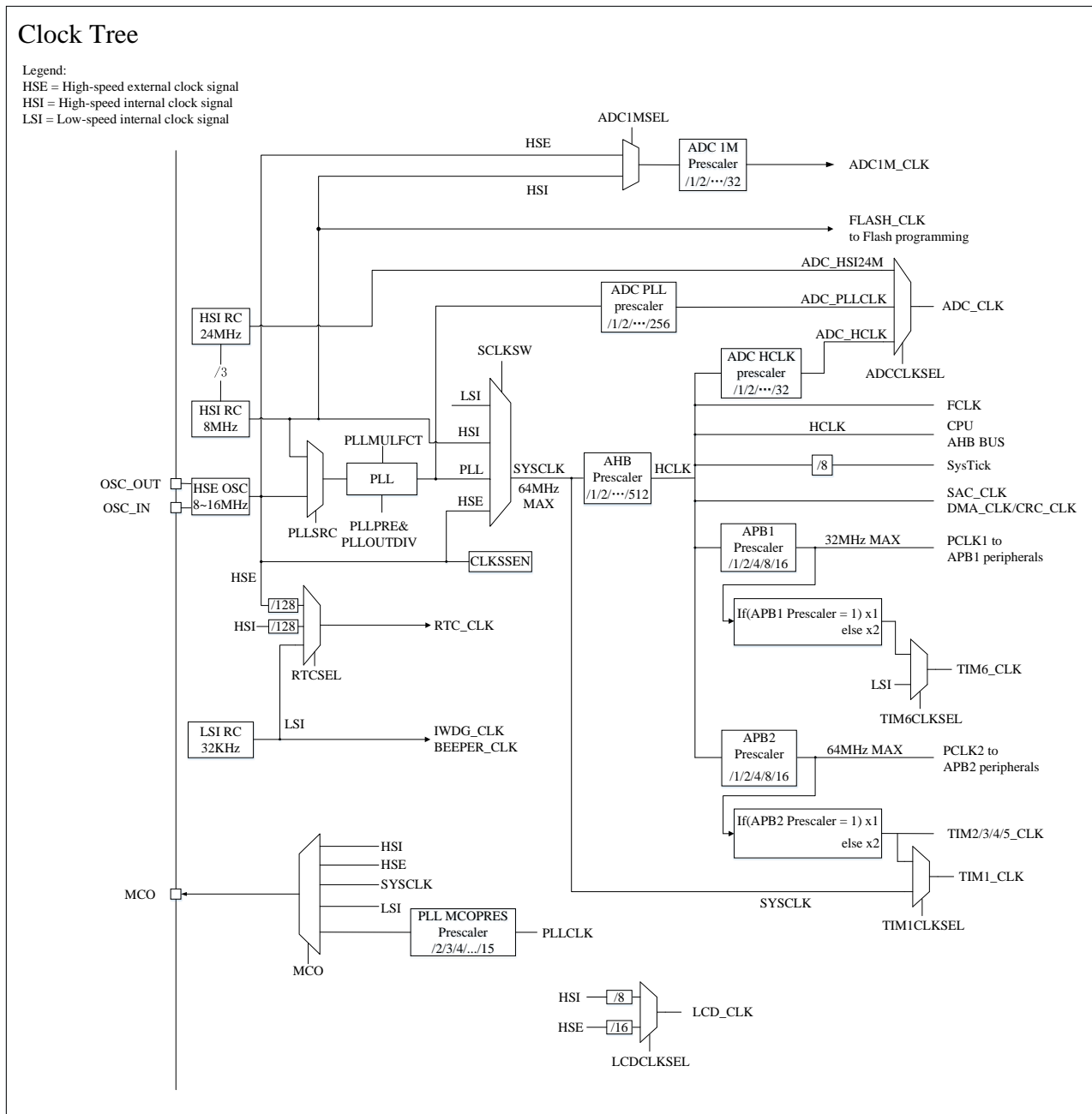
Figure 4-2 Clock Tree
