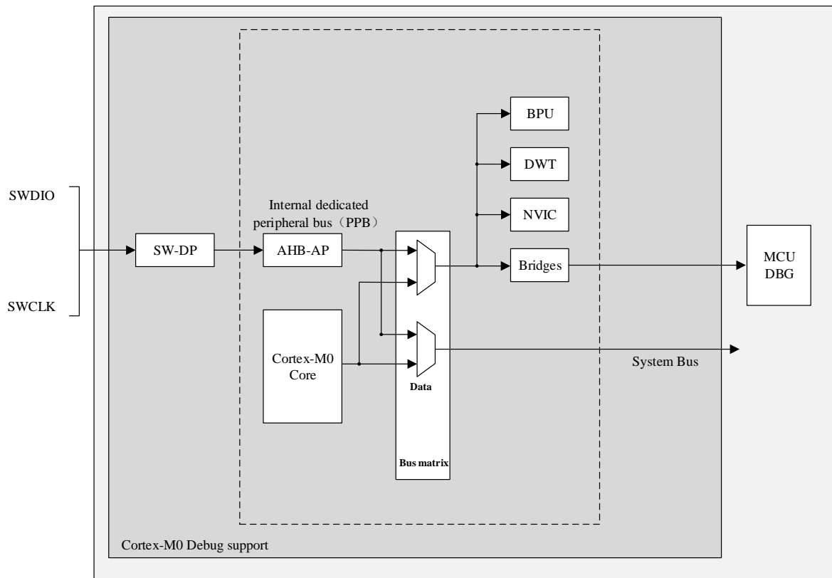
Figure 25-1 N32A052 Level And Cortex ® -M0 Level Debugging Block Diagram
