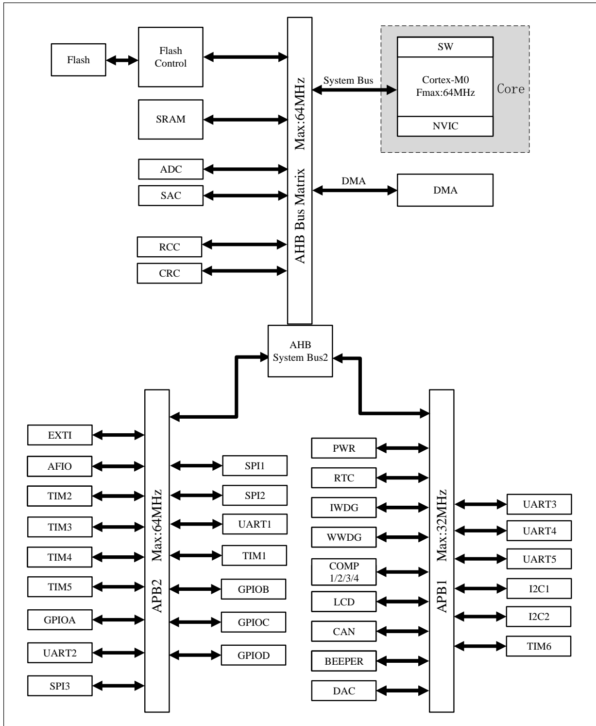
Figure 2-1 Bus Architecture
