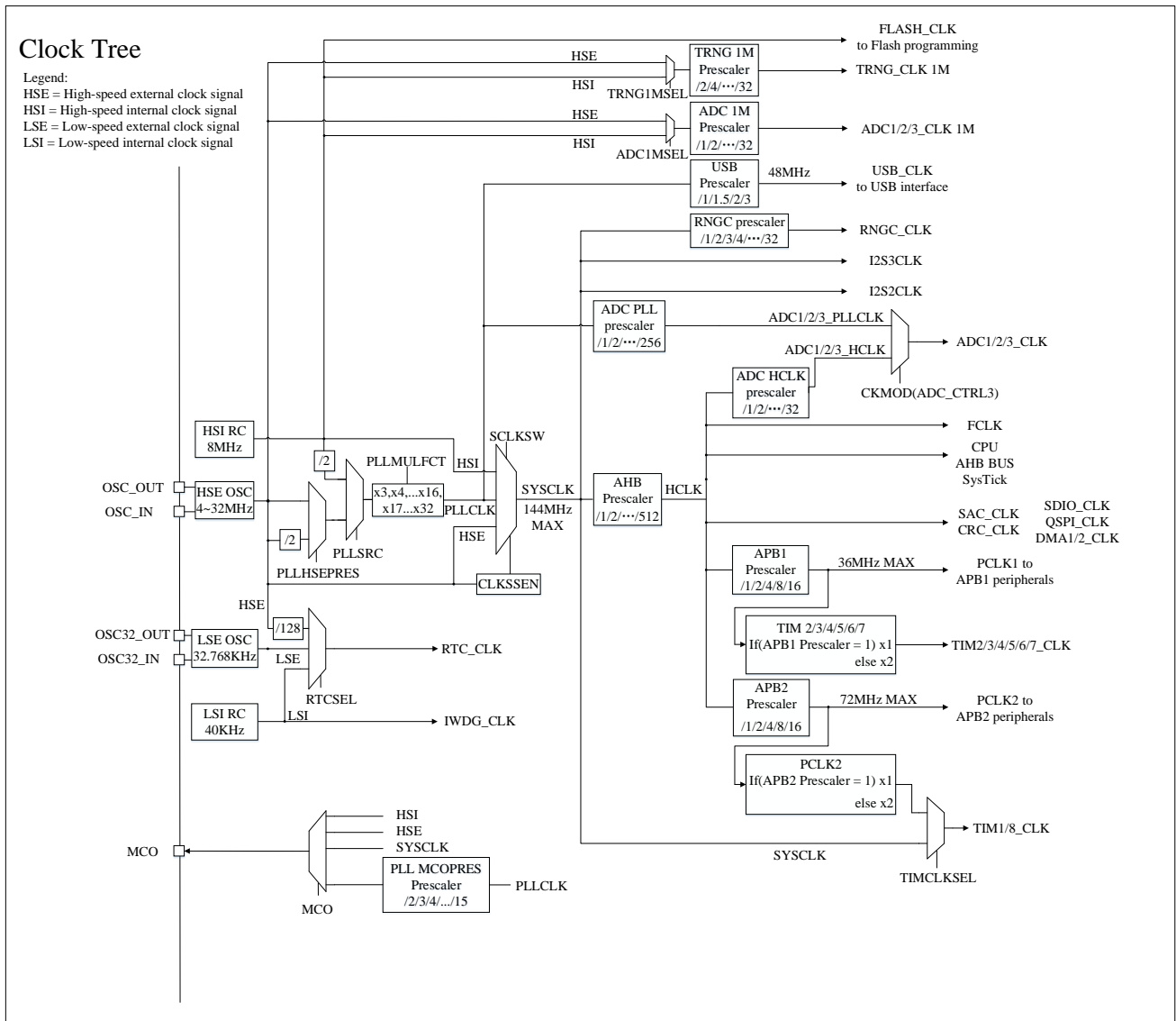
Figure 2-2 Clock tree
