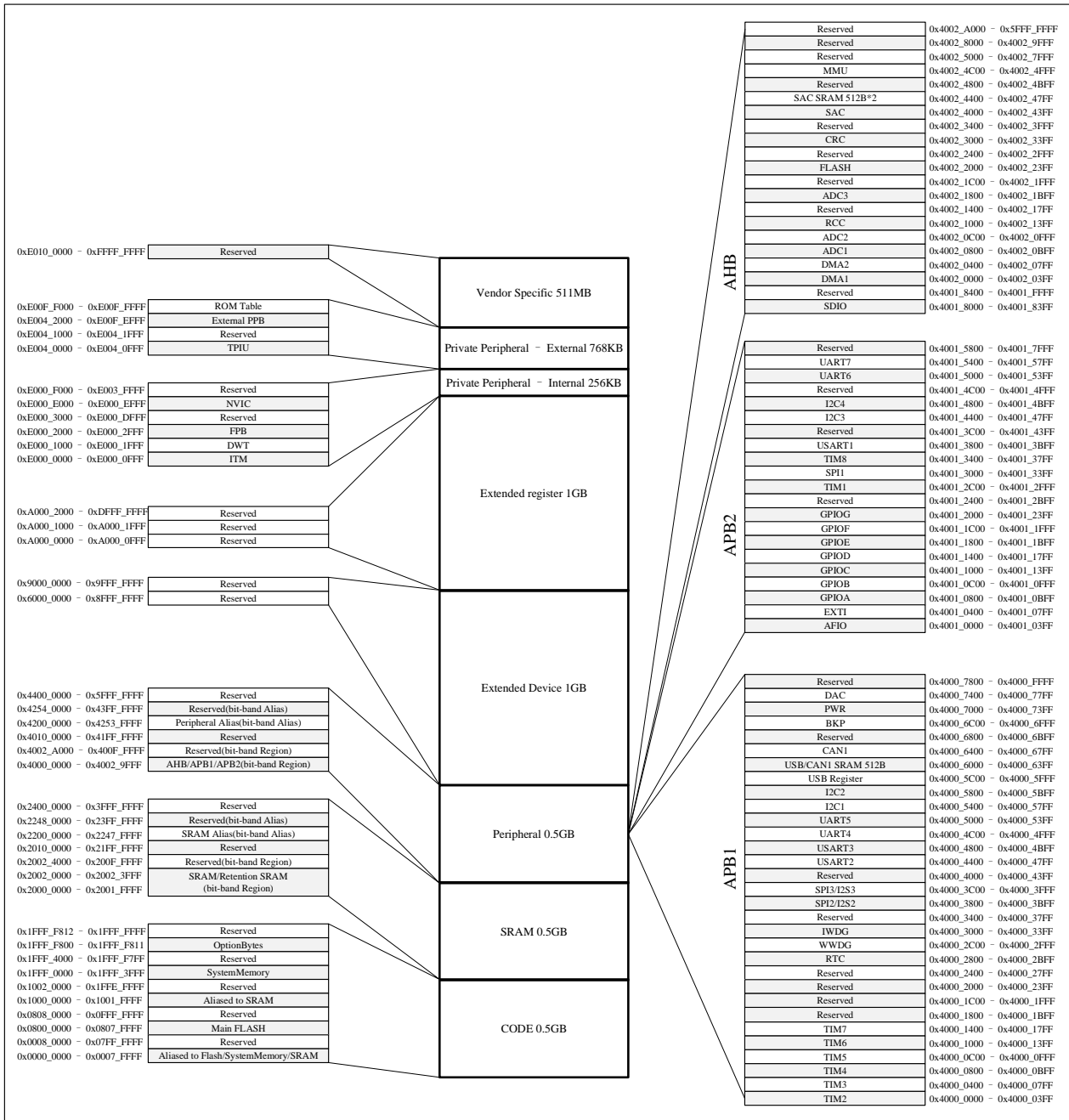
Figure 2-1 Memory map
