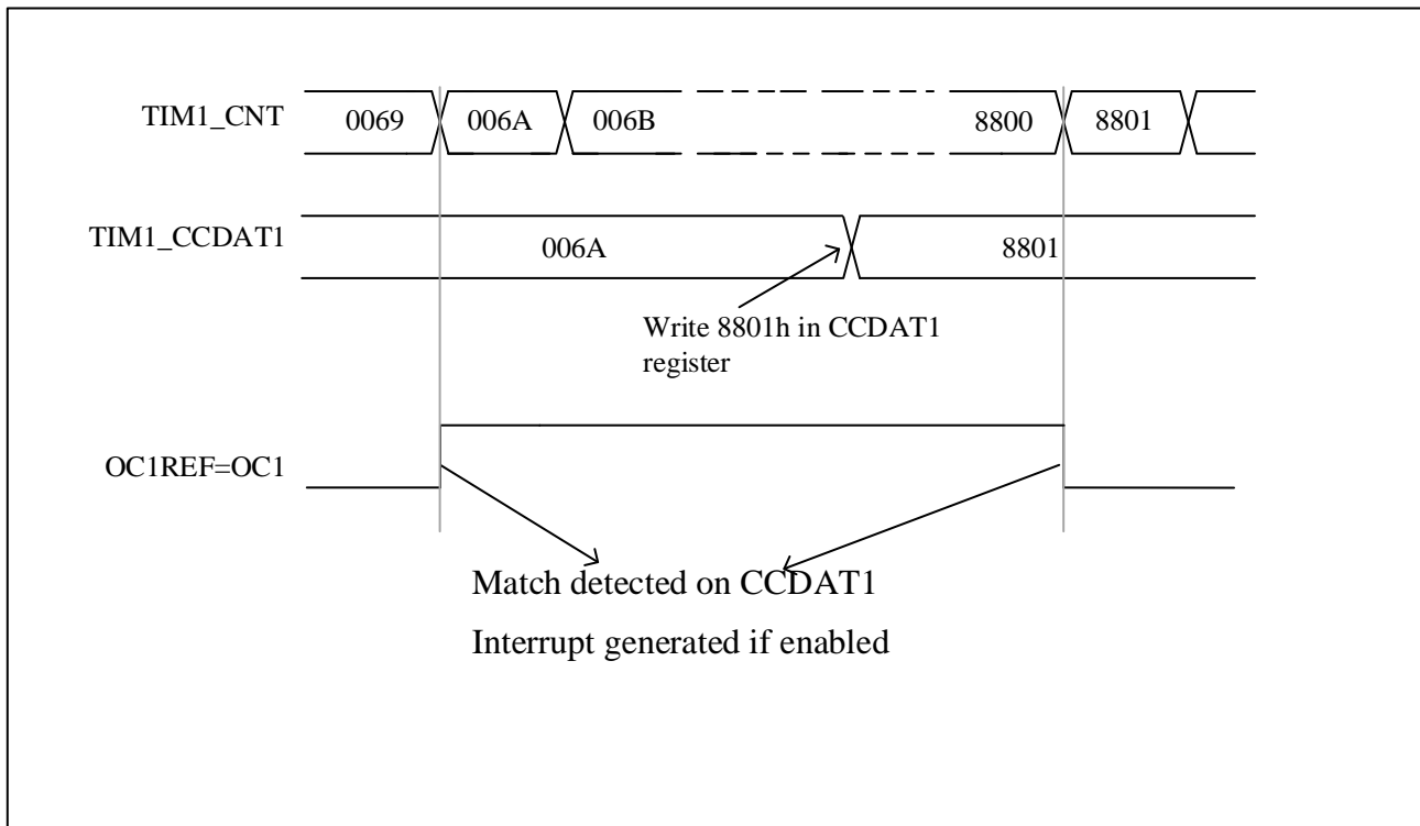
Figure 11-17 Output compare mode, toggle on OC1
