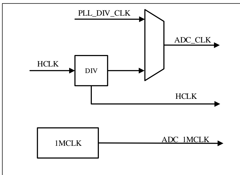
Figure 17-2 ADC clock
