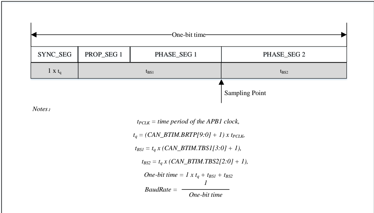
Figure 25-11 Bit sequence
