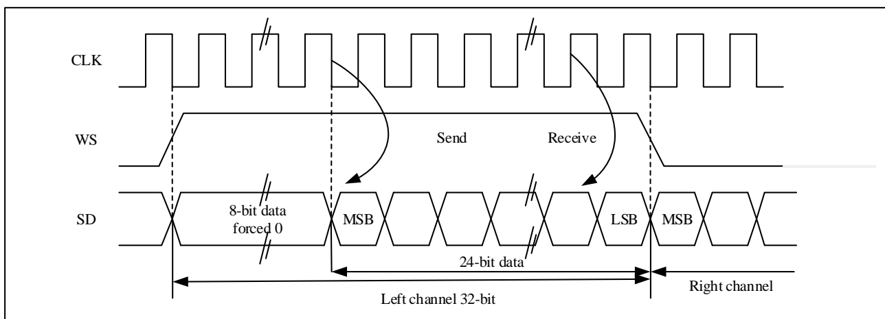
Figure 24-21 LSB aligns 24-bit data, CLKPOL = 0
