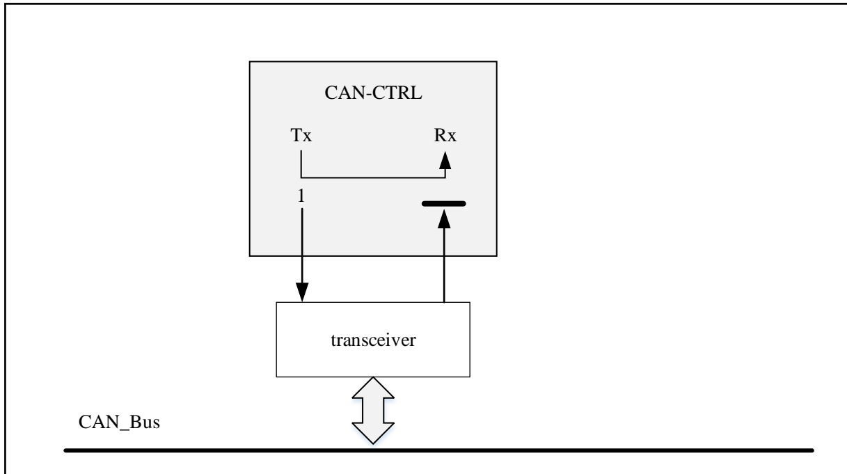
Figure 25-6 Loopback silent mode
