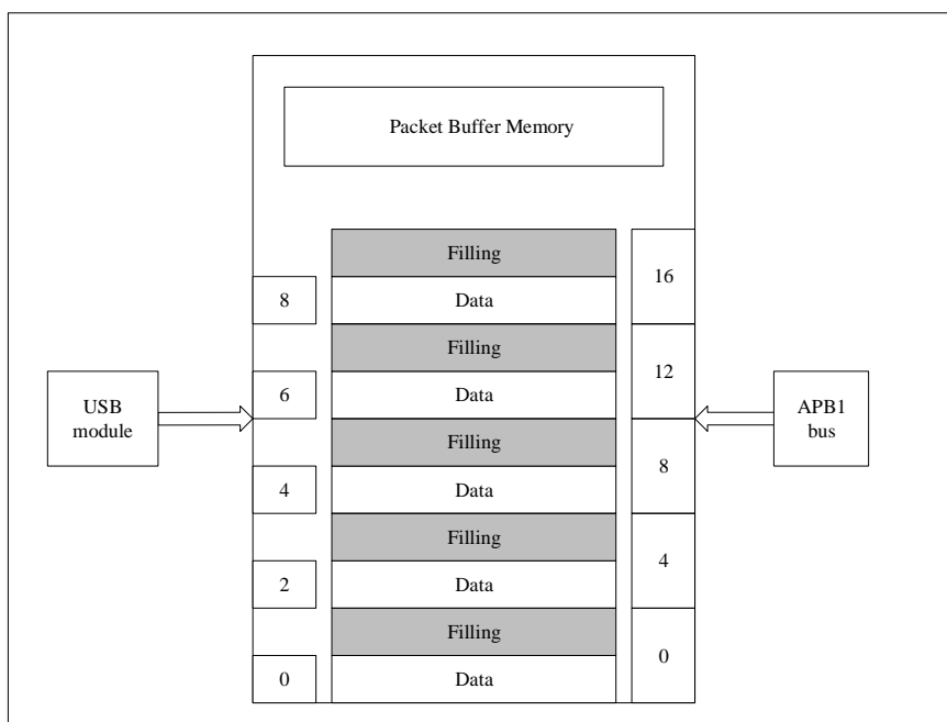
Figure 26-2 The user applications on the microcontrollers and the USB modules access Packet Buffer Memory
