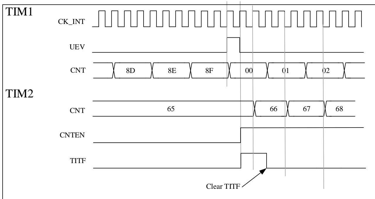
Figure 13-25 Trigger TIM2 with an update of TIM1
