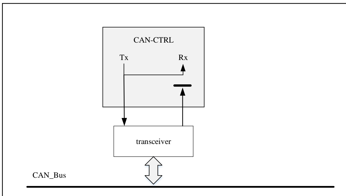
Figure 21-4 loopback mode
