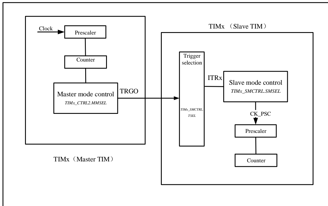
Figure 13-22 Block diagram of timer interconnection
