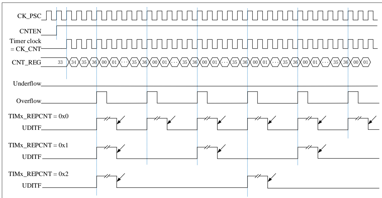
Figure 12-9 Repeat count sequence diagram in up-counting mode
