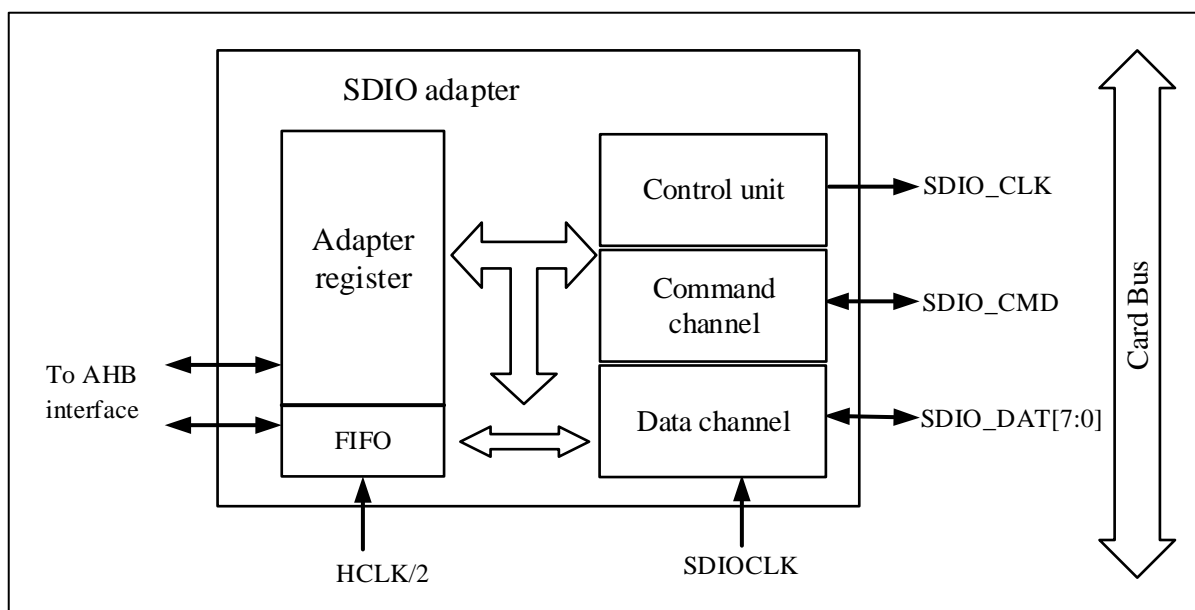
Figure 19-7 SDIO adapter
