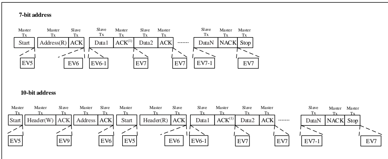
Figure 23-6 Master receiver transfer sequence diagram
