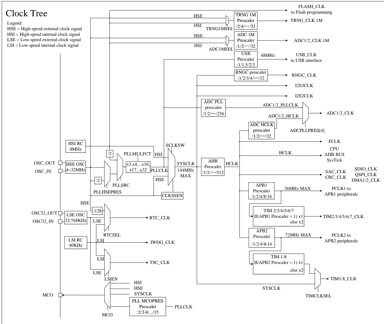
Figure 5-2 Clock Tree
