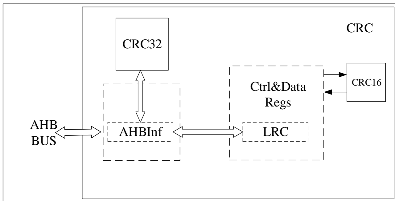
Figure 16-1 CRC calculation unit block diagram
