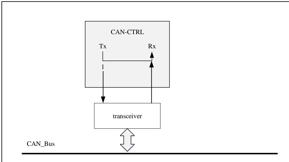
Figure 21-5 silent mode
