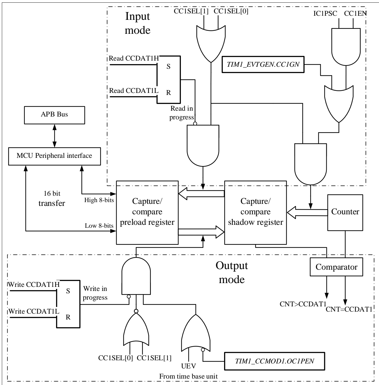
Figure 13-14 Capture/compare channel 1 main circuit
