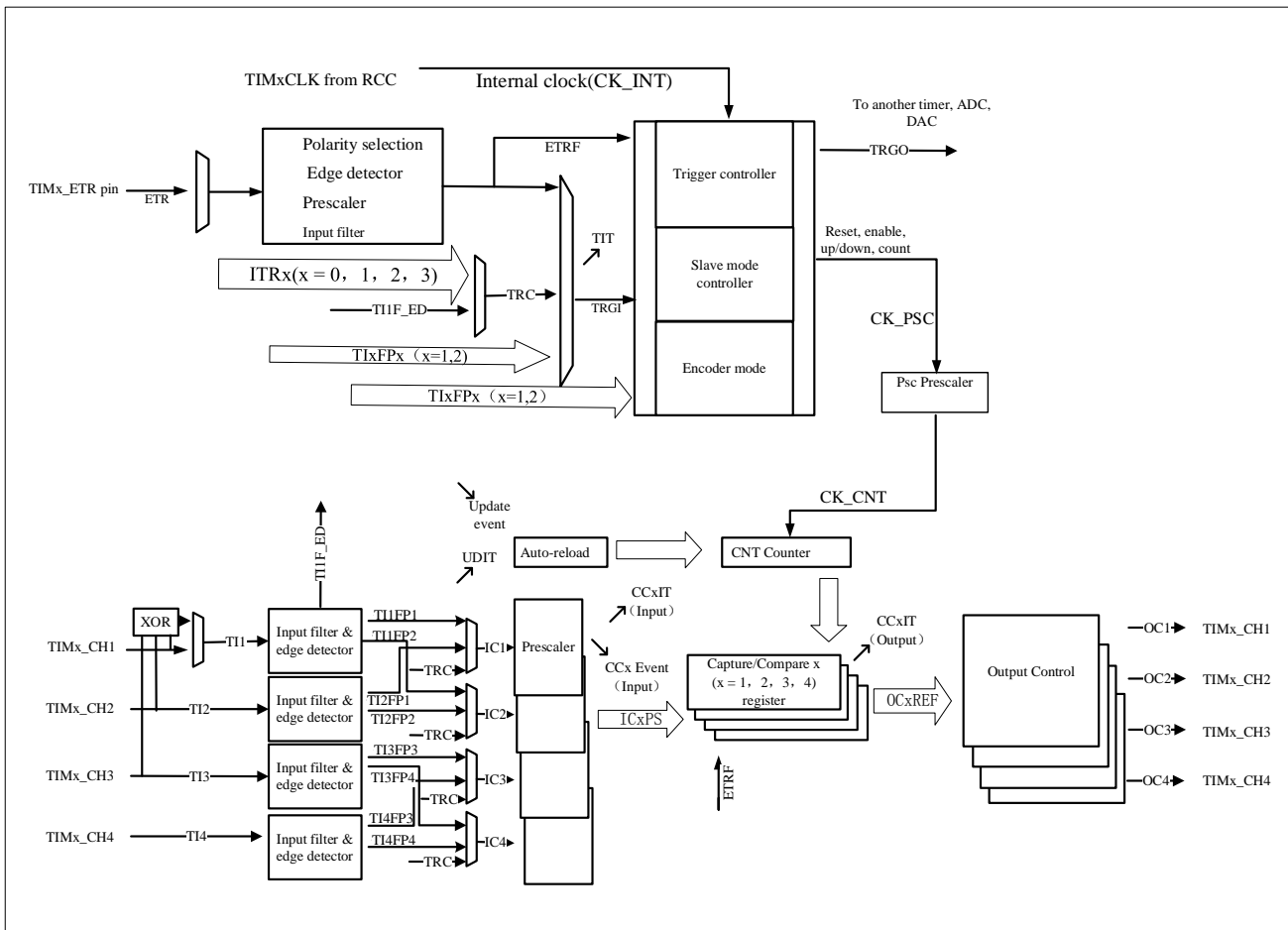
Figure 13-1 Block diagram of TIMx (x=2, 3, 4 and 5)
