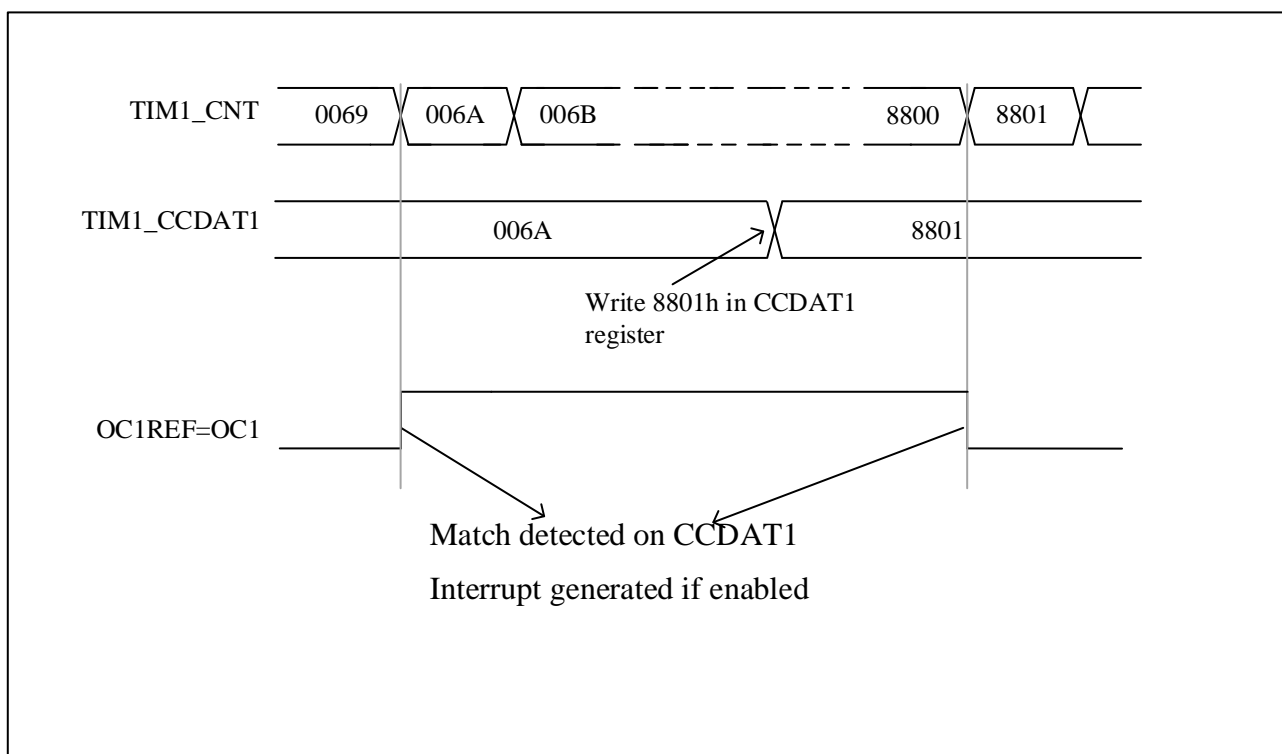
Figure 13-17 Output compare mode, toggle on OC1
