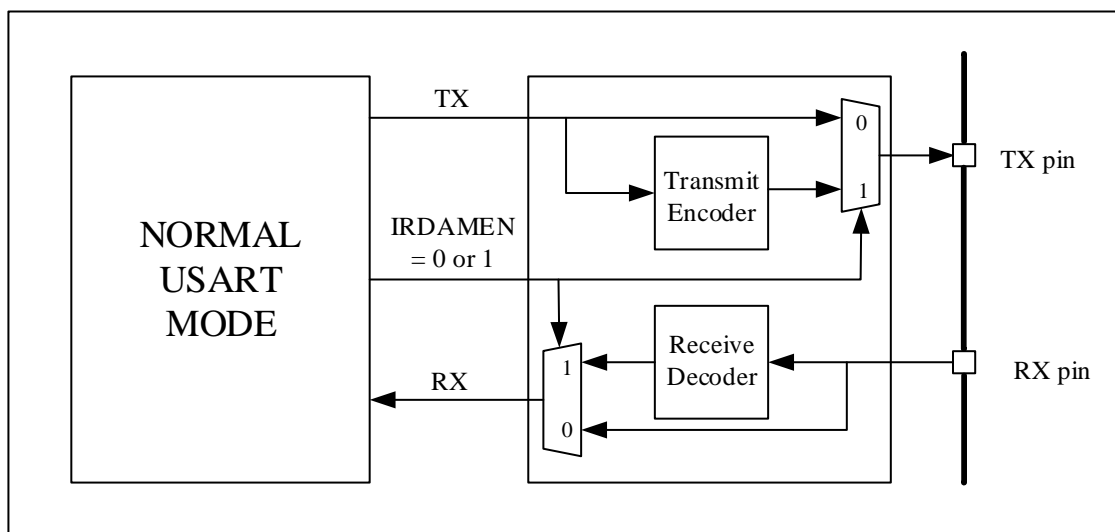
Figure 24-19 IrDA data Modulation (3/16)-normal mode
