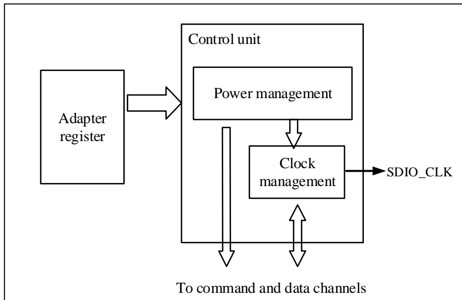
Figure 19-8 Control unit
