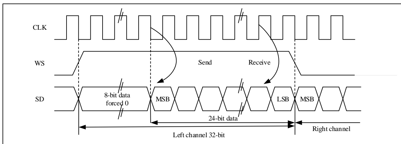
Figure 22-21 LSB aligns 24-bit data, CLKPOL = 0
