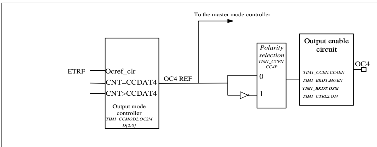
Figure 12-19 Output part of channelx (x= 4)
