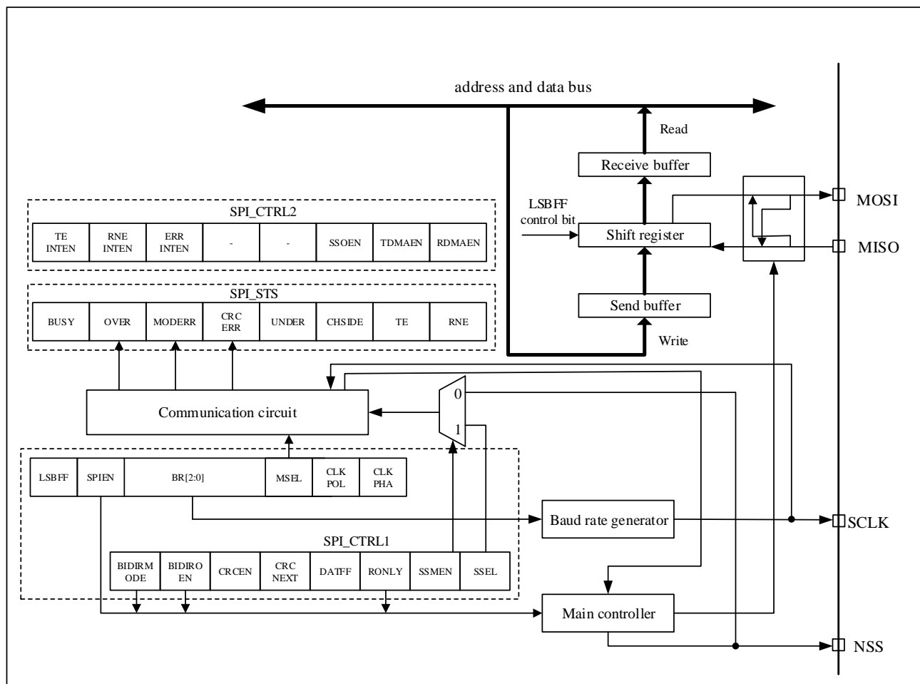
Figure 22-1 SPI block diagram
