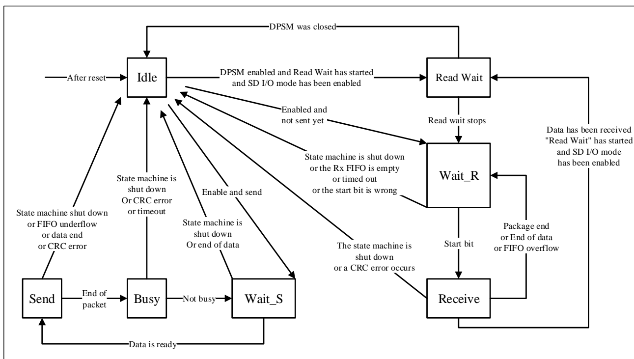
Figure 19-13 Data Path State Machine (DPSM)
