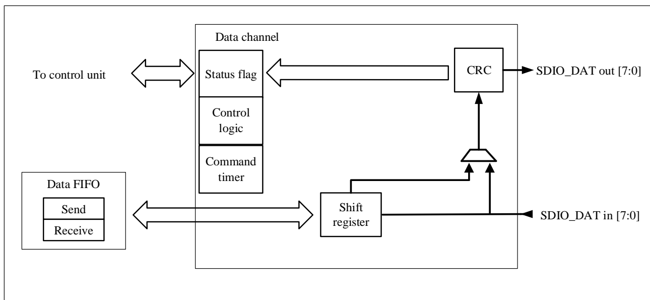
Figure 19-12 Data Channel
