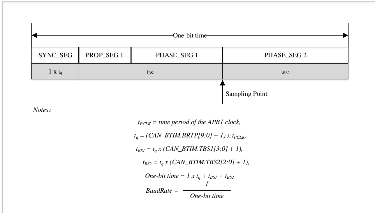
Figure 21-11 Bit sequence
