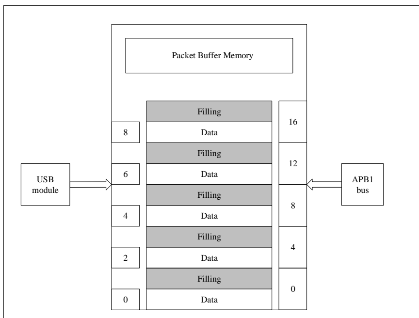
Figure 20-2 The user applications on the microcontrollers and the USB modules access Packet Buffer Memory
