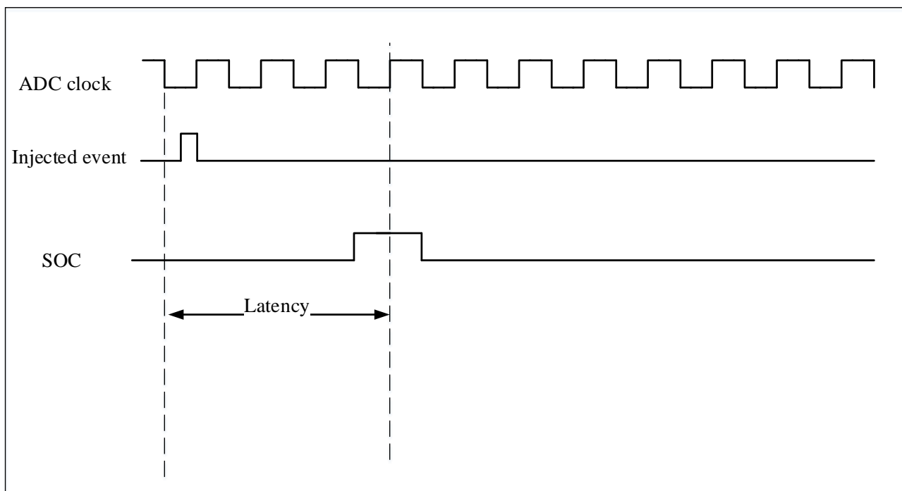
Figure 10-5 Injection conversion delay
