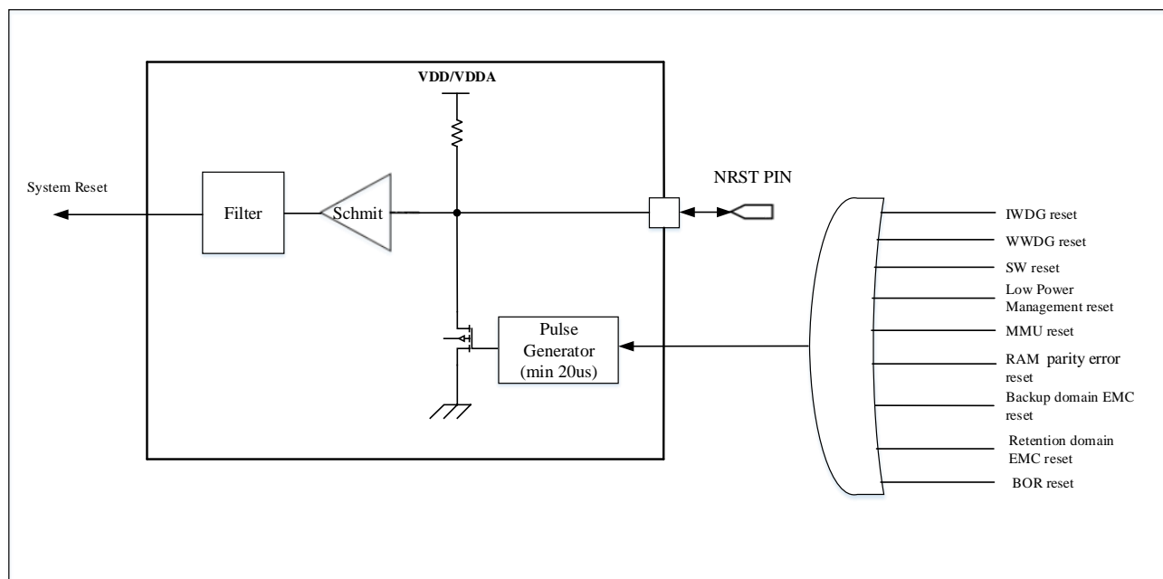
Figure 5-1 System reset generation
