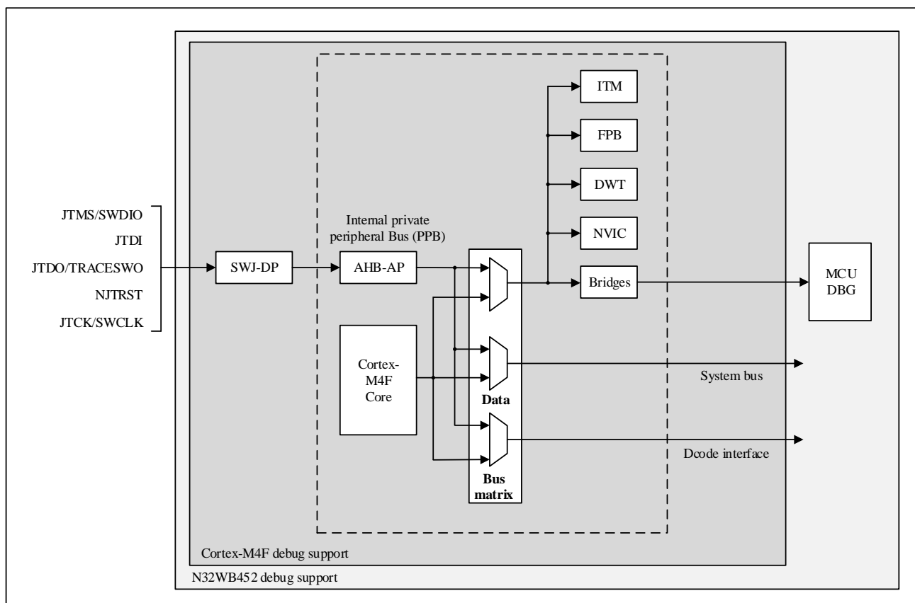
Figure 26-1 N32WB452 level and Cortex™-M4F level debugging block diagram
