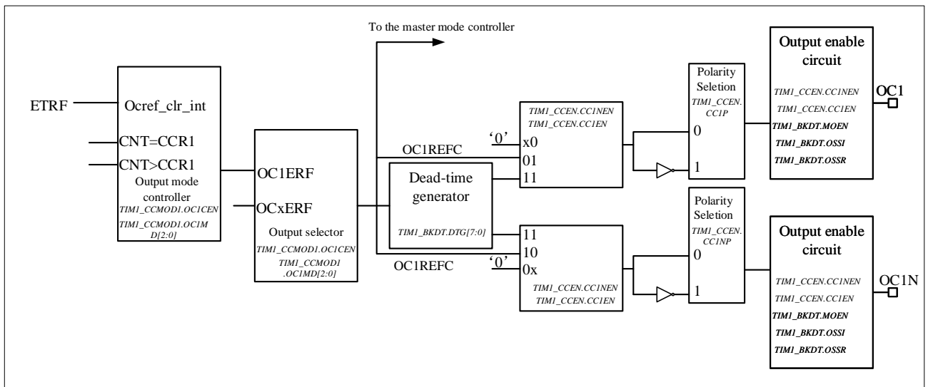
Figure 12-18 Output part of channelx (x= 1,2,3, take channel 1 as example)
