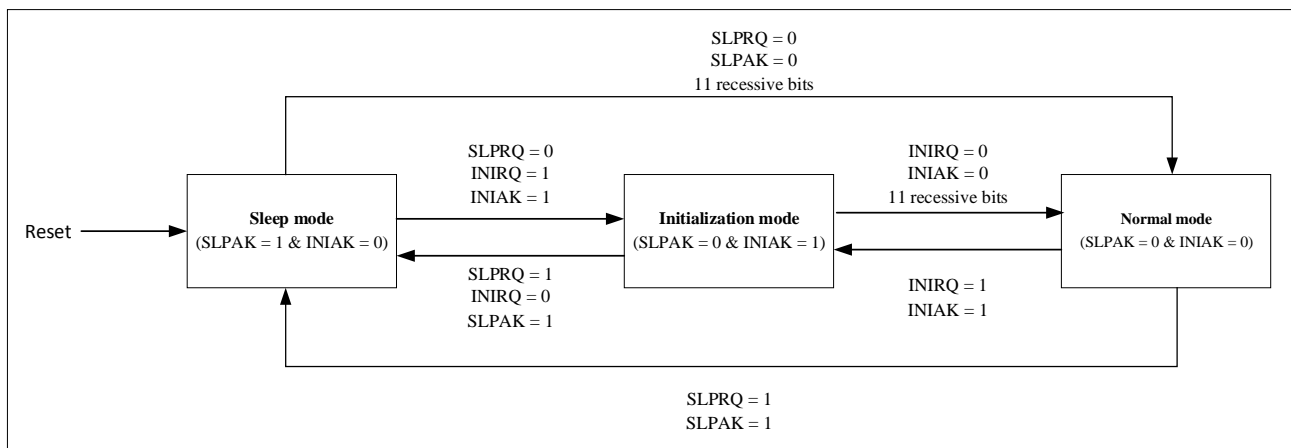
Figure 21-2 CAN working mode
