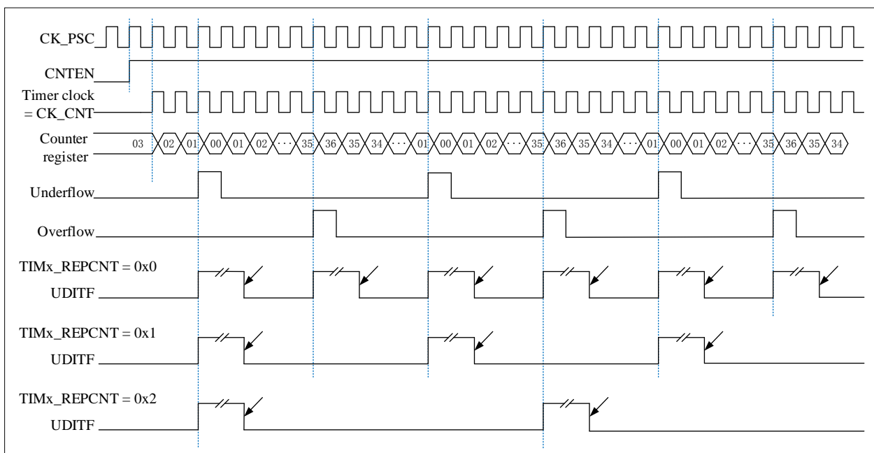
Figure 12-10 Repeat count sequence diagram in center-aligned mode
