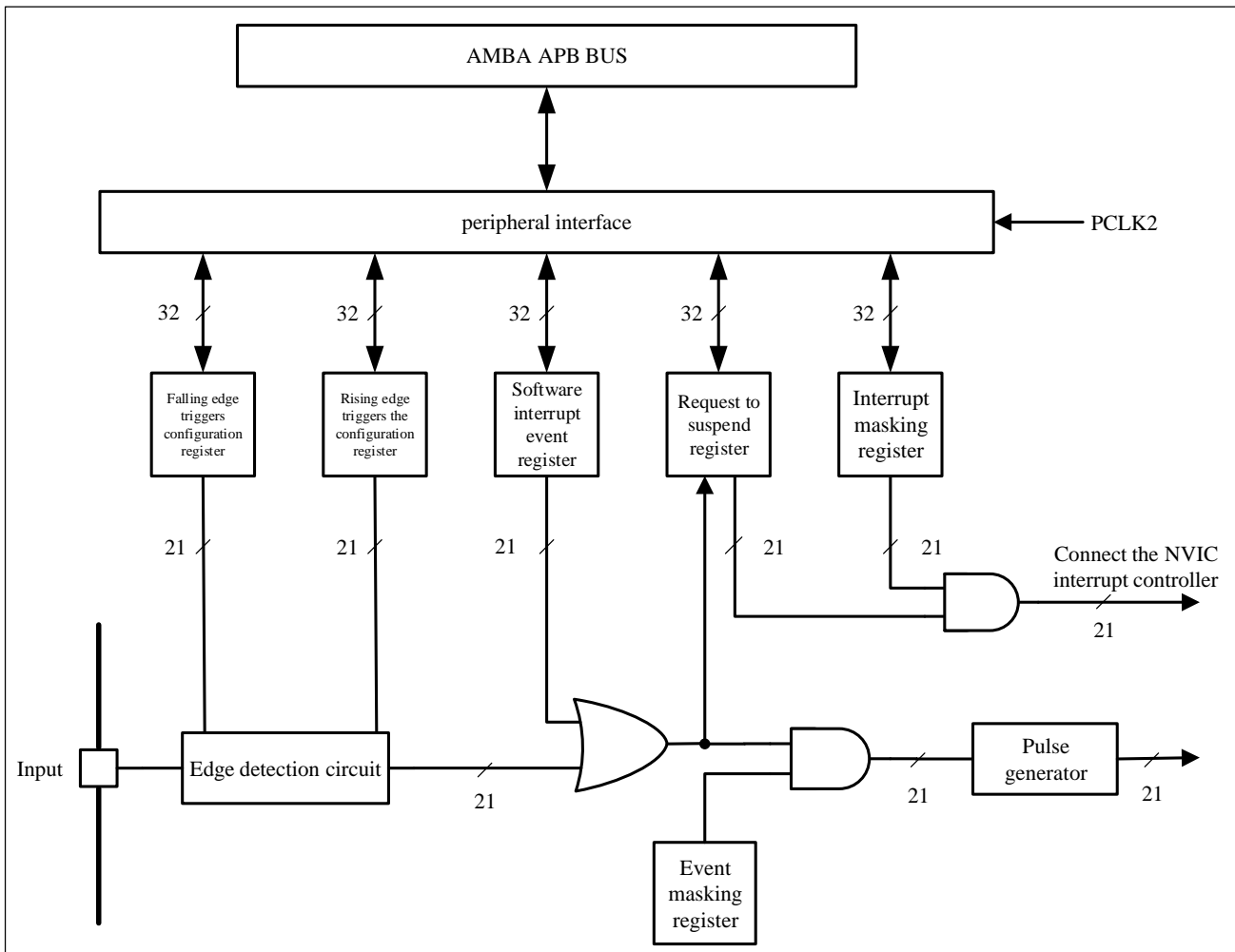
Figure 8-1 External interrupt/event controller block diagram
