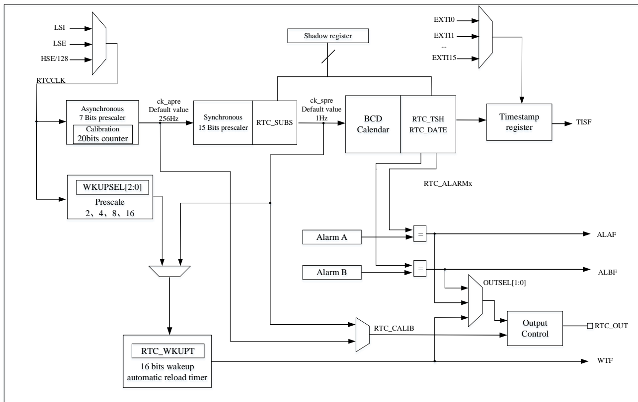
Figure 15-1 RTC Block Diagram
